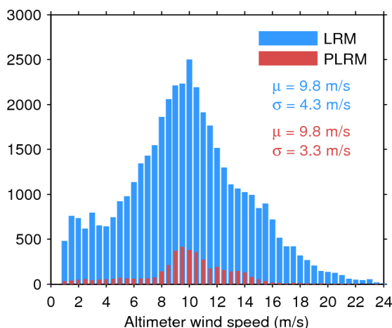
Figure 33. Histogram of flag-valid wind over oceans and lakes for LRM (blue) and PLRM (red) for 01/12/2016. The mean ( \mu ) and standard deviation ( \sigma ) are also shown. Note that values larger than 24 m/s are excluded from the histogram for the sake of readability but not from the computation of \mu and \sigma .
