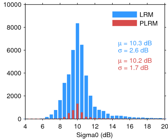
Figure 25. Histogram of flag-valid sigma0 over oceans and lakes for LRM (blue) and PLRM (red) for 01/12/2016. The mean ( \mu ) and standard deviation ( \sigma ) are also shown. Note that values outside [4 20] dB are excluded from the histogram for the sake of readability but not from the computation of \mu and \sigma .
