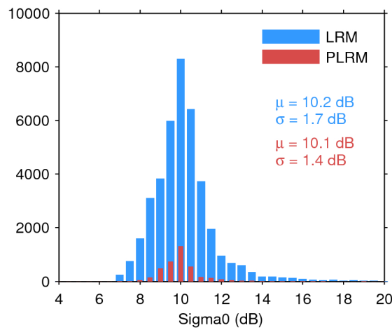
Figure 28. Histogram of science-valid sigma0 over oceans and lakes for LRM (blue) and PLRM (red) for 01/12/2016. The mean ( \mu ) and standard deviation ( \sigma ) are also shown. Note that values outside [4 20] dB are excluded from the histogram for the sake of readability but not from the computation of \mu and \sigma .
