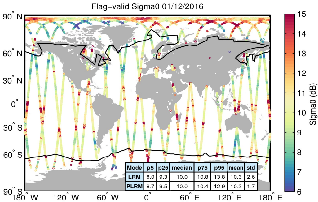
Figure 23. Geographical distribution of flag-valid sigma0 data over oceans and lakes for 01/12/2016. The statistical values shown in the table refer to the sigma0 in dB and are calculated separately for LRM and PLRM regions. Measurements taken over polar polygons have been excluded from the computation of the statistical values. The black lines mark the outer limit of the Arctic and Antarctic polar polygons.
