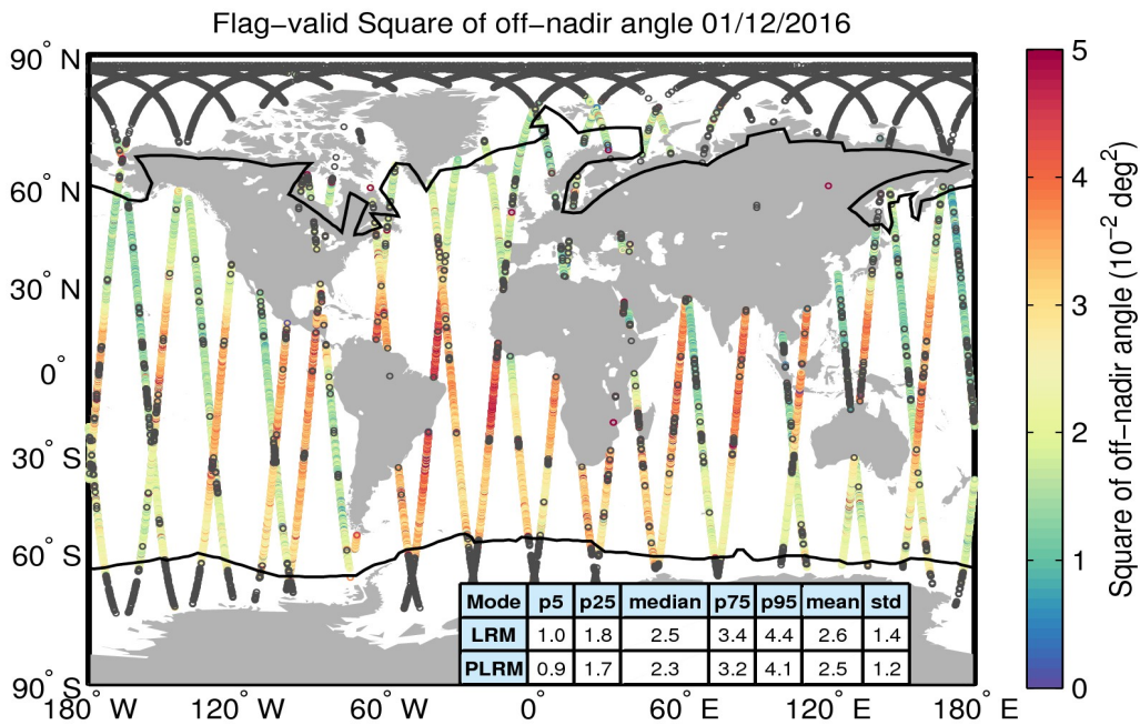
Figure 37. Geographical distribution of flag-valid mispointing data over oceans and lakes for 01/12/2016. The statistical values shown in the table refer to the mispointing in 10^{-2} deg 2 and are calculated separately for LRM and PLRM regions. Measurements taken over polar polygons have been excluded from the computation of the statistical values. The black lines mark the outer limit of the Arctic and Antarctic polar polygons. Gray circles denote negative values.
