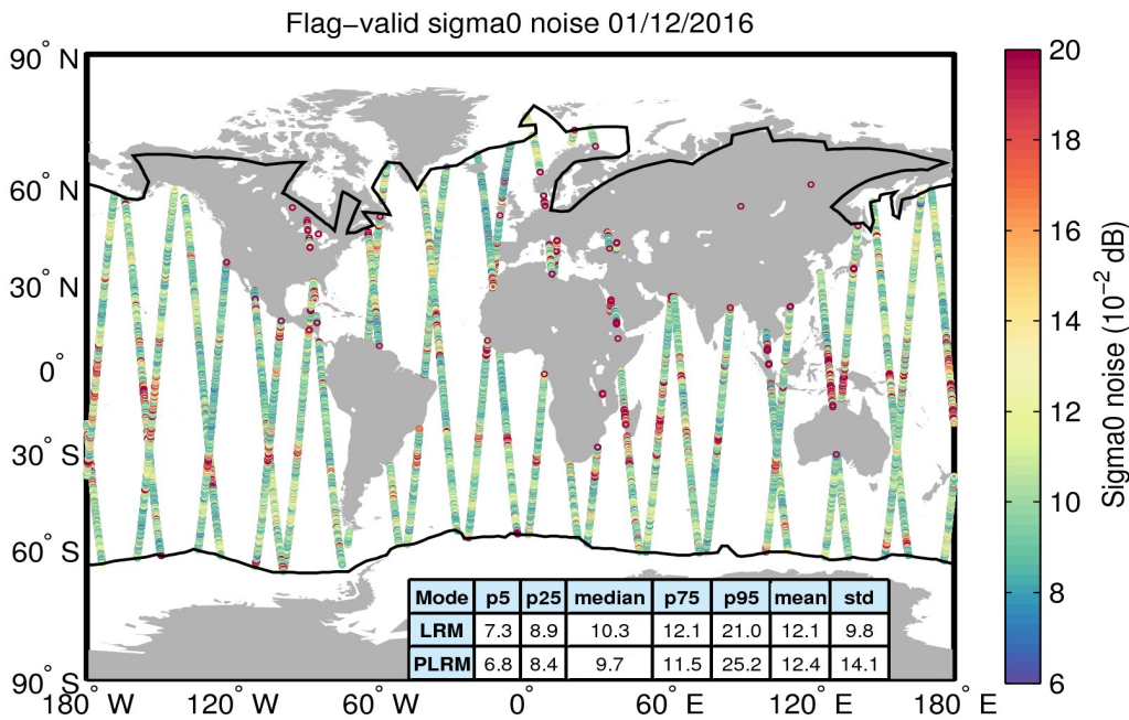
Figure 26. Geographical distribution of flag-valid 20-Hz sigma0 measurement noise over oceans and lakes for 01/12/2016. The statistical values shown in the table refer to the sigma0 noise and are calculated separately for LRM and PLRM regions. Measurements taken over polar polygons have been excluded from the computation of the statistical values. The black lines mark the outer limit of the Arctic and Antarctic polar polygons.
