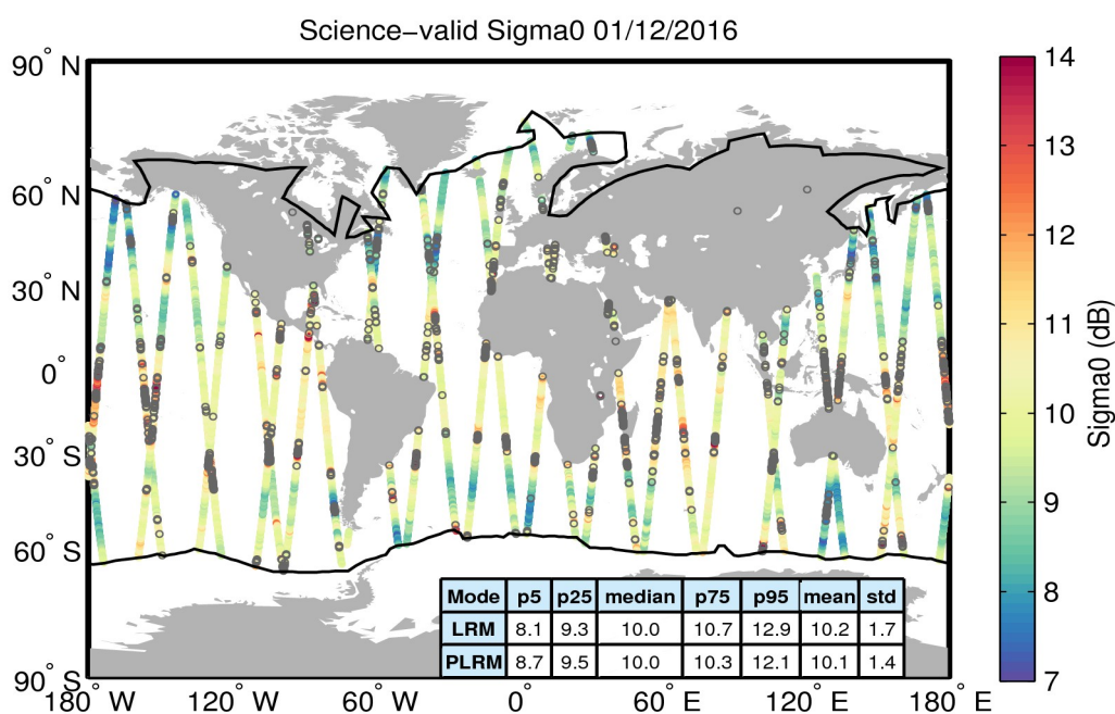
Figure 27. Geographical distribution of science-valid sigma0 data over oceans and lakes for 01/12/2016. The statistical values shown in the table refer to the sigma0 in dB and are calculated separately for LRM and PLRM regions. The black lines mark the outer limit of the Arctic and Antarctic polar polygons. Gray circles denote records that have been rejected based on the editing criteria described in Table 4.
