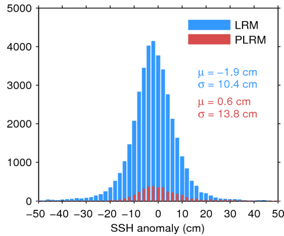
Figure 11. Histogram of science-valid SSH anomaly over oceans and lakes for LRM (blue) and PLRM (red) for 01/12/2016. The mean ( \mu ) and standard deviation ( \sigma ) are also shown. Note that values outside [-50\ 50] cm are excluded from the histogram for the sake of readability but not from the computation of \mu and \sigma .
