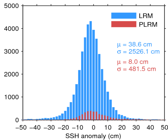
Figure 7. Histogram of flag-valid SSH anomaly over oceans and lakes for LRM (blue) and PLRM (red) for 01/12/2016. The mean ( \mu ) and standard deviation ( \sigma ) are also shown. Note that values outside [-50\ 50] cm are excluded from the histogram for the sake of readability but not from the computation of \mu and \sigma .
