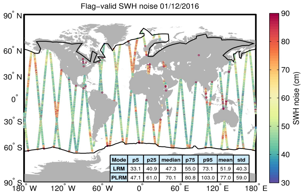
Figure 18. Geographical distribution of flag-valid 20-Hz SWH measurement noise over oceans and lakes for 01/12/2016. The statistical values shown in the table refer to the SWH noise and are calculated separately for LRM and PLRM regions. Measurements taken over polar polygons have been excluded from the computation of the statistical values. The black lines mark the outer limit of the Arctic and Antarctic polar polygons.
