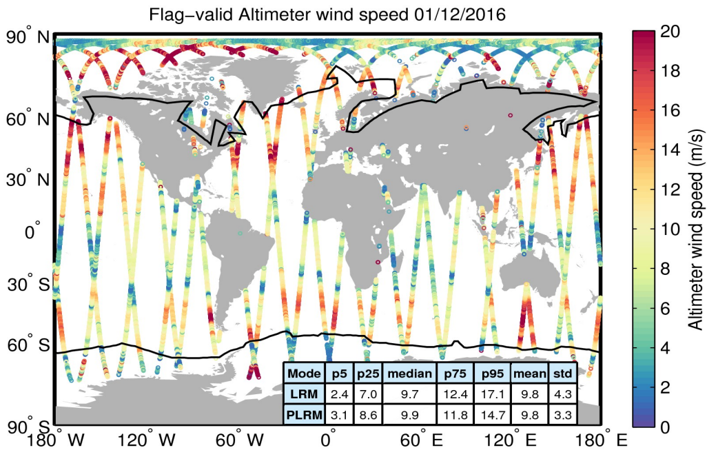
Figure 31. Geographical distribution of flag-valid wind data over oceans and lakes for 01/12/2016. The statistical values shown in the table refer to the wind in m/s and are calculated separately for LRM and PLRM regions. Measurements taken over polar polygons have been excluded from the computation of the statistical values. The black lines mark the outer limit of the Arctic and Antarctic polar polygons.
