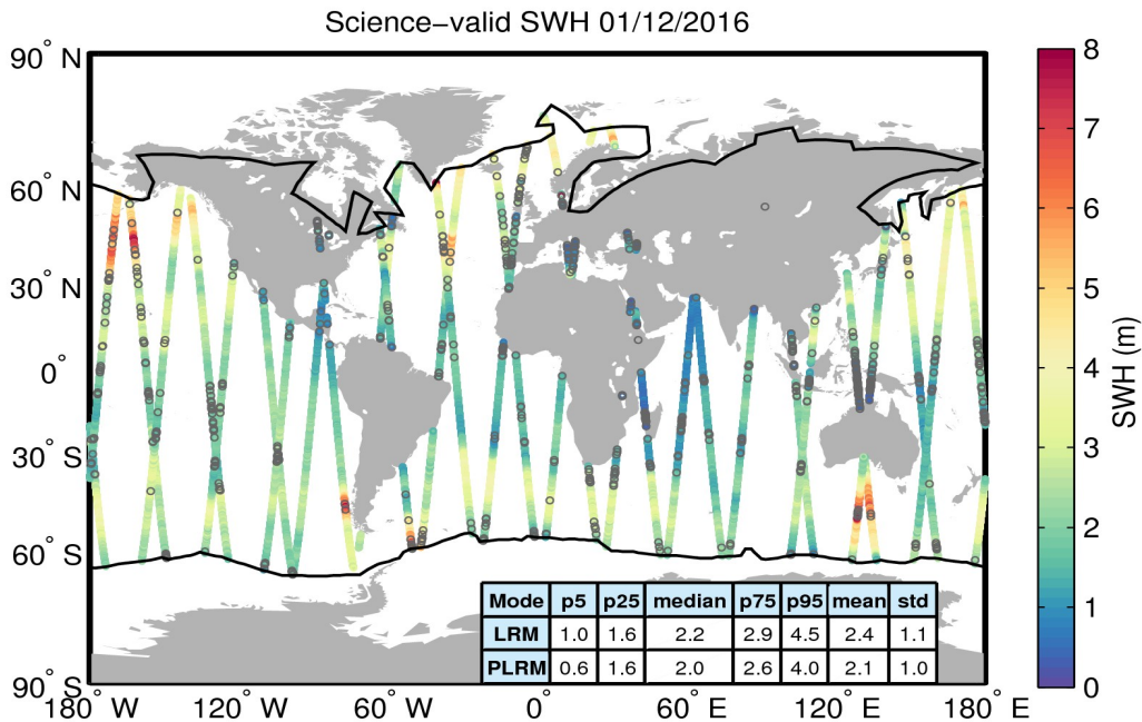
Figure 19. Geographical distribution of science-valid SWH data over oceans and lakes for 01/12/2016. The statistical values shown in the table refer to the SWH in m and are calculated separately for LRM and PLRM regions. The black lines mark the outer limit of the Arctic and Antarctic polar polygons. Gray circles denote records that have been rejected based on the editing criteria described in Table 3.
