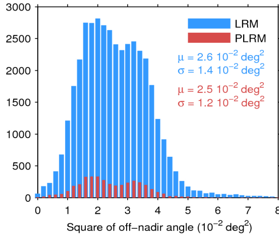
Figure 39. Histogram of flag-valid mispointing over oceans and lakes for LRM (blue) and PLRM (red) for 01/12/2016. Only positive values have been considered. The mean ( \mu ) and standard deviation ( \sigma ) are also shown. Note that values larger than 8 \cdot 10^{-2} \text{ deg}^2 are excluded from the histogram for the sake of readability but not from the computation of \mu and \sigma .
