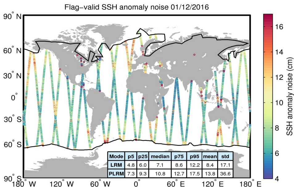
Figure 8. Geographical distribution of flag-valid 20-Hz SSH anomaly measurement noise over oceans and lakes for 01/12/2016. The statistical values shown in the table refer to the SSH anomaly noise and are calculated separately for LRM and PLRM regions. Measurements taken over polar polygons have been excluded from the computation of the statistical values. The black lines mark the outer limit of the Arctic and Antarctic polar polygons.
