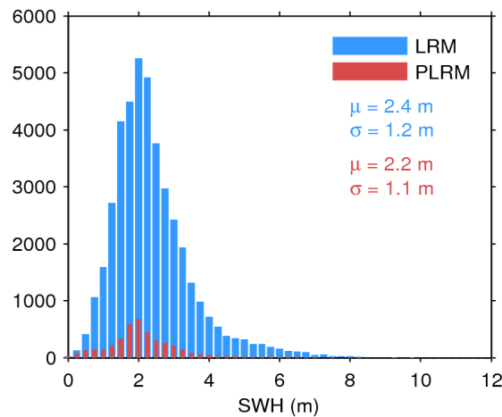
Figure 17. Histogram of flag-valid SWH over oceans and lakes for LRM (blue) and PLRM (red) for 01/12/2016. The mean ( \mu ) and standard deviation ( \sigma ) are also shown. Note that values larger than 12 m are excluded from the histogram for the sake of readability but not from the computation of \mu and \sigma .
