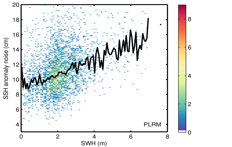
Figure 9. 2D histogram showing flag-valid SSH anomaly noise as a function of SWH for LRM (top) and PLRM (bottom) for 01/12/2016. The black line denotes the median SSH anomaly noise as a function of SWH.
