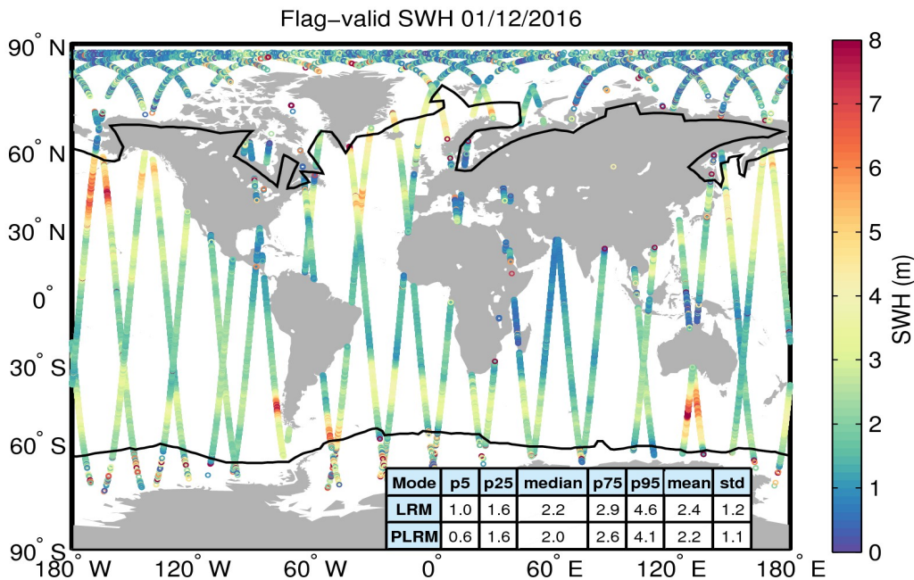
Figure 15. Geographical distribution of flag-valid SWH data over oceans and lakes for 01/12/2016. The statistical values shown in the table refer to the SWH in m and are calculated separately for LRM and PLRM regions. Measurements taken over polar polygons have been excluded from the computation of the statistical values. The black lines mark the outer limit of the Arctic and Antarctic polar polygons.
