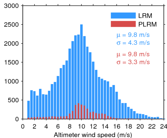
Figure 35. Histogram of science-valid wind over oceans and lakes for LRM (blue) and PLRM (red) for 01/12/2016. The mean ( \mu ) and standard deviation ( \sigma ) are also shown. Note that values larger than 24 m/s are excluded from the histogram for the sake of readability but not from the computation of \mu and \sigma .
