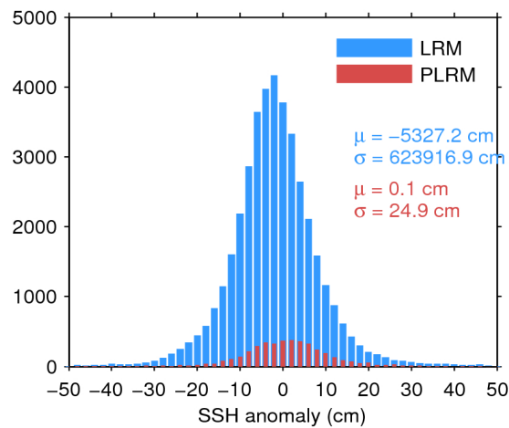
Figure 7. Histogram of flag-valid SSH anomaly over oceans and lakes for LRM (blue) and PLRM (red) for 27/11/2016. The mean ( \mu ) and standard deviation ( \sigma ) are also shown. Note that values outside [-50\ 50] cm are excluded from the histogram for the sake of readability but not from the computation of \mu and \sigma .
