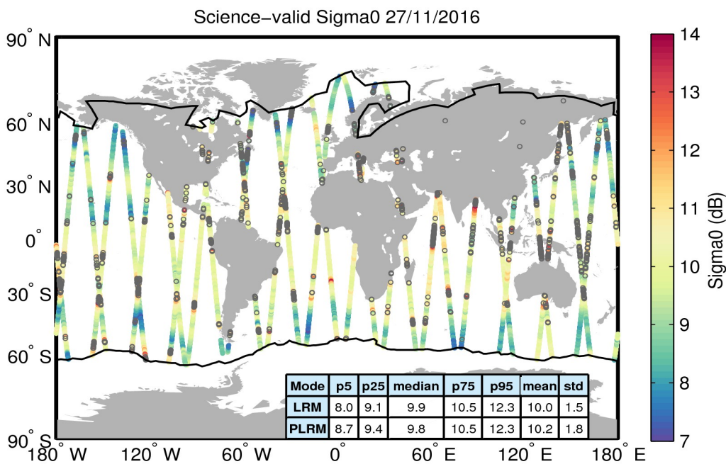
Figure 27. Geographical distribution of science-valid sigma0 data over oceans and lakes for 27/11/2016. The statistical values shown in the table refer to the sigma0 in dB and are calculated separately for LRM and PLRM regions. The black lines mark the outer limit of the Arctic and Antarctic polar polygons. Gray circles denote records that have been rejected based on the editing criteria described in Table 4.
