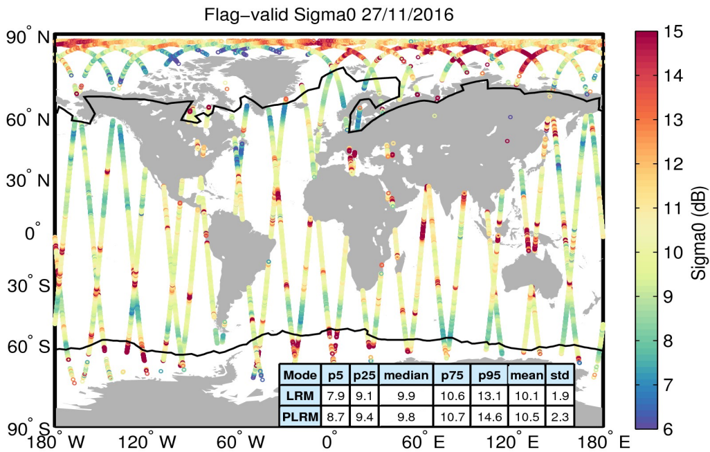
Figure 23. Geographical distribution of flag-valid sigma0 data over oceans and lakes for 27/11/2016. The statistical values shown in the table refer to the sigma0 in dB and are calculated separately for LRM and PLRM regions. Measurements taken over polar polygons have been excluded from the computation of the statistical values. The black lines mark the outer limit of the Arctic and Antarctic polar polygons.
