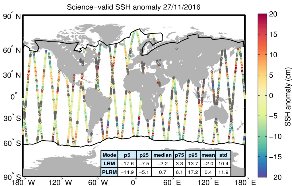
Figure 10. Geographical distribution of science-valid SSH anomaly data over oceans and lakes for 27/11/2016. The statistical values shown in the table refer to the SSH anomaly in cm and are calculated separately for LRM and PLRM regions. The black lines mark the outer limit of the Arctic and Antarctic polar polygons. Gray circles denote records that have been rejected based on the editing criteria described in Table 2.
