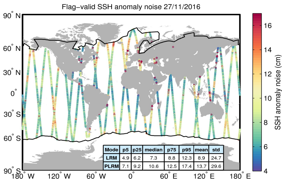
Figure 8. Geographical distribution of flag-valid 20-Hz SSH anomaly measurement noise over oceans and lakes for 27/11/2016. The statistical values shown in the table refer to the SSH anomaly noise and are calculated separately for LRM and PLRM regions. Measurements taken over polar polygons have been excluded from the computation of the statistical values. The black lines mark the outer limit of the Arctic and Antarctic polar polygons.
