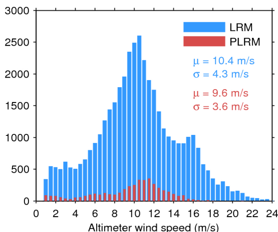
Figure 33. Histogram of flag-valid wind over oceans and lakes for LRM (blue) and PLRM (red) for 27/11/2016. The mean ( \mu ) and standard deviation ( \sigma ) are also shown. Note that values larger than 24 m/s are excluded from the histogram for the sake of readability but not from the computation of \mu and \sigma .
