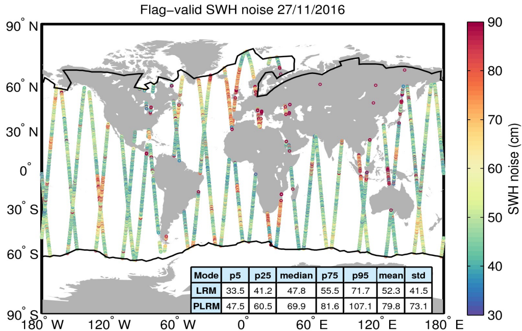
Figure 18. Geographical distribution of flag-valid 20-Hz SWH measurement noise over oceans and lakes for 27/11/2016. The statistical values shown in the table refer to the SWH noise and are calculated separately for LRM and PLRM regions. Measurements taken over polar polygons have been excluded from the computation of the statistical values. The black lines mark the outer limit of the Arctic and Antarctic polar polygons.
