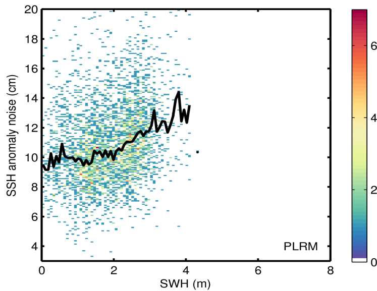
Figure 9. 2D histogram showing flag-valid SSH anomaly noise as a function of SWH for LRM (top) and PLRM (bottom) for 27/11/2016. The black line denotes the median SSH anomaly noise as a function of SWH.
