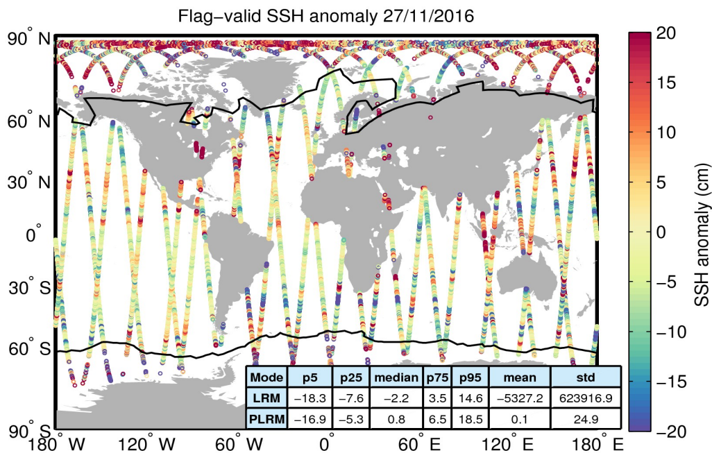
Figure 5. Geographical distribution of flag-valid 1-Hz SSH anomaly data over oceans and lakes for 27/11/2016. The statistical values shown in the table refer to the SSH anomaly in cm and are calculated separately for LRM and PLRM regions. Measurements taken over polar polygons have been excluded from the computation of the statistical values. The black lines mark the outer limit of the Arctic and Antarctic polar polygons.
