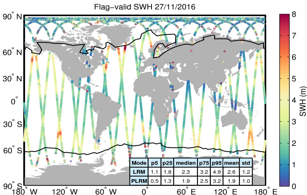
Figure 15. Geographical distribution of flag-valid SWH data over oceans and lakes for 27/11/2016. The statistical values shown in the table refer to the SWH in m and are calculated separately for LRM and PLRM regions. Measurements taken over polar polygons have been excluded from the computation of the statistical values. The black lines mark the outer limit of the Arctic and Antarctic polar polygons.
