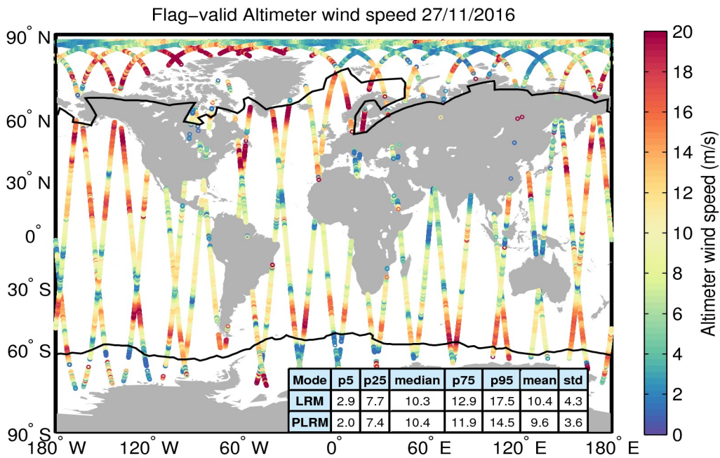
Figure 31. Geographical distribution of flag-valid wind data over oceans and lakes for 27/11/2016. The statistical values shown in the table refer to the wind in m/s and are calculated separately for LRM and PLRM regions. Measurements taken over polar polygons have been excluded from the computation of the statistical values. The black lines mark the outer limit of the Arctic and Antarctic polar polygons.
