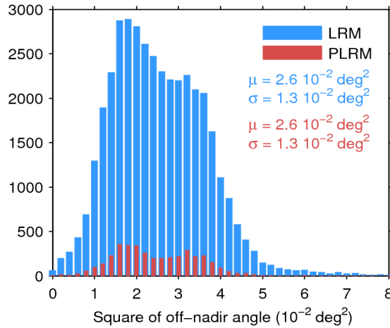
Figure 39. Histogram of flag-valid mispointing over oceans and lakes for LRM (blue) and PLRM (red) for 27/11/2016. Only positive values have been considered. The mean ( \mu ) and standard deviation ( \sigma ) are also shown. Note that values larger than 8 \cdot 10^{-2} \text{ deg}^2 are excluded from the histogram for the sake of readability but not from the computation of \mu and \sigma .
