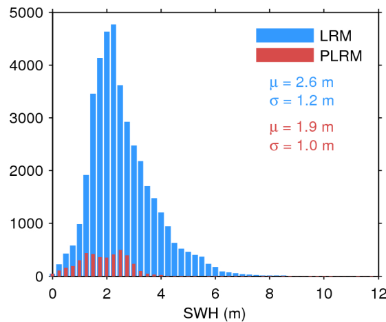
Figure 17. Histogram of flag-valid SWH over oceans and lakes for LRM (blue) and PLRM (red) for 27/11/2016. The mean ( \mu ) and standard deviation ( \sigma ) are also shown. Note that values larger than 12 m are excluded from the histogram for the sake of readability but not from the computation of \mu and \sigma .
