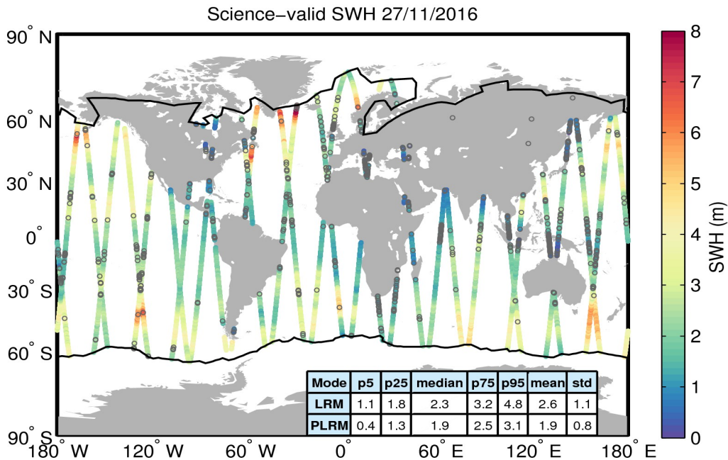
Figure 19. Geographical distribution of science-valid SWH data over oceans and lakes for 27/11/2016. The statistical values shown in the table refer to the SWH in m and are calculated separately for LRM and PLRM regions. The black lines mark the outer limit of the Arctic and Antarctic polar polygons. Gray circles denote records that have been rejected based on the editing criteria described in Table 3.
