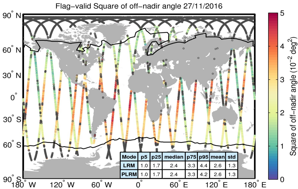
Figure 37. Geographical distribution of flag-valid mispointing data over oceans and lakes for 27/11/2016. The statistical values shown in the table refer to the mispointing in 10^{-2} deg 2 and are calculated separately for LRM and PLRM regions. Measurements taken over polar polygons have been excluded from the computation of the statistical values. The black lines mark the outer limit of the Arctic and Antarctic polar polygons. Gray circles denote negative values.
