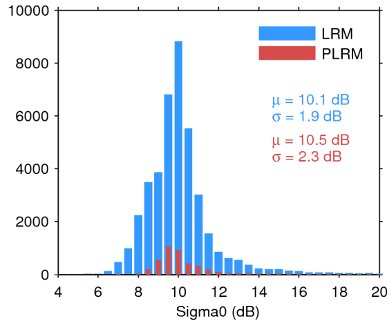
Figure 25. Histogram of flag-valid sigma0 over oceans and lakes for LRM (blue) and PLRM (red) for 27/11/2016. The mean ( \mu ) and standard deviation ( \sigma ) are also shown. Note that values outside [4 20] dB are excluded from the histogram for the sake of readability but not from the computation of \mu and \sigma .
