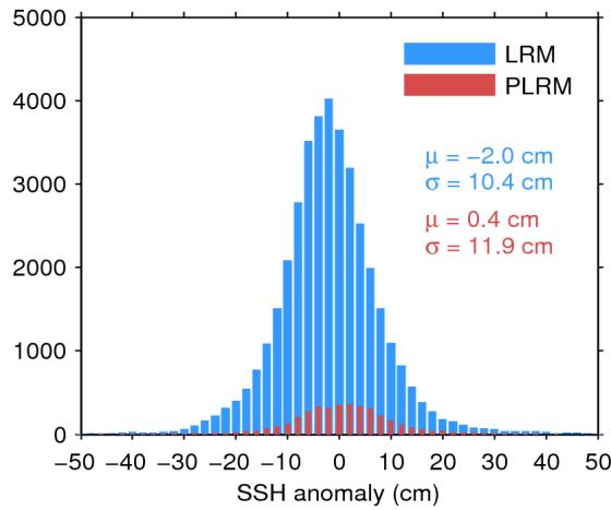
Figure 11. Histogram of science-valid SSH anomaly over oceans and lakes for LRM (blue) and PLRM (red) for 27/11/2016. The mean ( \mu ) and standard deviation ( \sigma ) are also shown. Note that values outside [-50 50] cm are excluded from the histogram for the sake of readability but not from the computation of \mu and \sigma .
