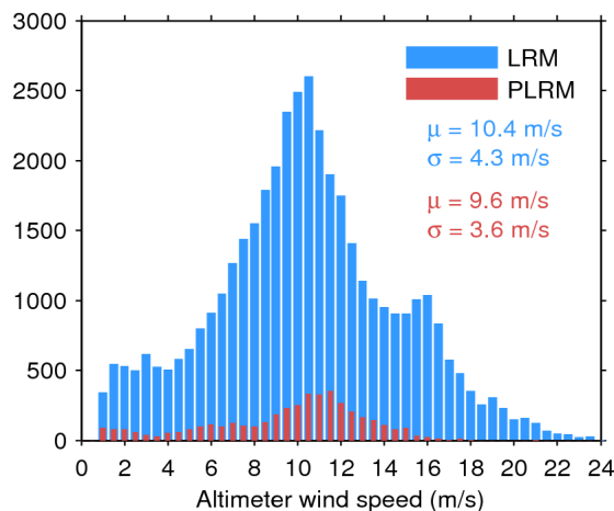
Figure 35. Histogram of science-valid wind over oceans and lakes for LRM (blue) and PLRM (red) for 27/11/2016. The mean ( \mu ) and standard deviation ( \sigma ) are also shown. Note that values larger than 24 m/s are excluded from the histogram for the sake of readability but not from the computation of \mu and \sigma .
