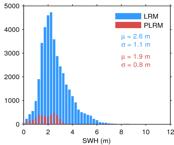
Figure 20. Histogram of science-valid SWH over oceans and lakes for LRM (blue) and PLRM (red) for 27/11/2016. The mean ( \mu ) and standard deviation ( \sigma ) are also shown. Note that values larger than 12 m are excluded from the histogram for the sake of readability but not from the computation of \mu and \sigma .
