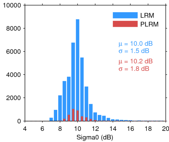
Figure 28. Histogram of science-valid sigma0 over oceans and lakes for LRM (blue) and PLRM (red) for 27/11/2016. The mean ( \mu ) and standard deviation ( \sigma ) are also shown. Note that values outside [4 20] dB are excluded from the histogram for the sake of readability but not from the computation of \mu and \sigma .
