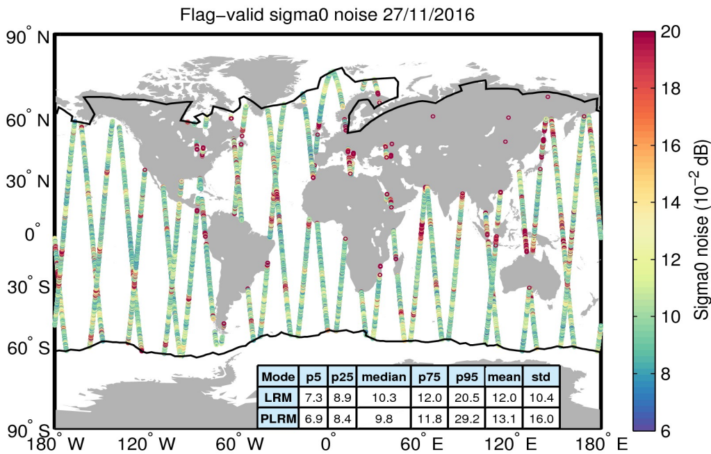
Figure 26. Geographical distribution of flag-valid 20-Hz sigma0 measurement noise over oceans and lakes for 27/11/2016. The statistical values shown in the table refer to the sigma0 noise and are calculated separately for LRM and PLRM regions. Measurements taken over polar polygons have been excluded from the computation of the statistical values. The black lines mark the outer limit of the Arctic and Antarctic polar polygons.
