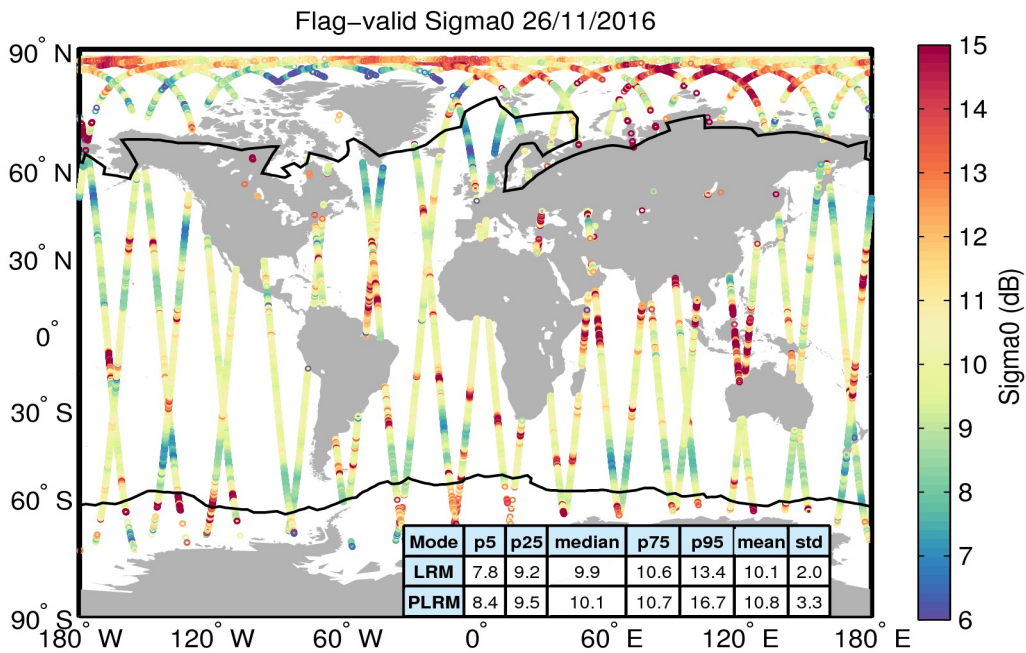
Figure 23. Geographical distribution of flag-valid sigma0 data over oceans and lakes for 26/11/2016. The statistical values shown in the table refer to the sigma0 in dB and are calculated separately for LRM and PLRM regions. Measurements taken over polar polygons have been excluded from the computation of the statistical values. The black lines mark the outer limit of the Arctic and Antarctic polar polygons.
