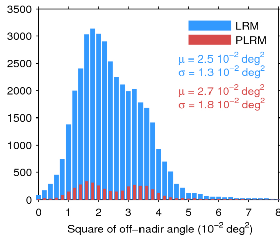
Figure 39. Histogram of flag-valid mispointing over oceans and lakes for LRM (blue) and PLRM (red) for 26/11/2016. Only positive values have been considered. The mean ( \mu ) and standard deviation ( \sigma ) are also shown. Note that values larger than 8 \cdot 10^{-2} \text{ deg}^2 are excluded from the histogram for the sake of readability but not from the computation of \mu and \sigma .
