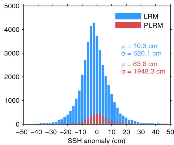
Figure 7. Histogram of flag-valid SSH anomaly over oceans and lakes for LRM (blue) and PLRM (red) for 26/11/2016. The mean ( \mu ) and standard deviation ( \sigma ) are also shown. Note that values outside [-50\ 50] cm are excluded from the histogram for the sake of readability but not from the computation of \mu and \sigma .
