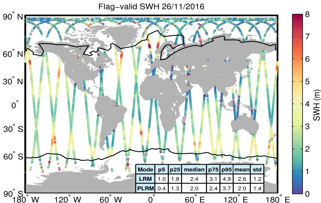
Figure 15. Geographical distribution of flag-valid SWH data over oceans and lakes for 26/11/2016. The statistical values shown in the table refer to the SWH in m and are calculated separately for LRM and PLRM regions. Measurements taken over polar polygons have been excluded from the computation of the statistical values. The black lines mark the outer limit of the Arctic and Antarctic polar polygons.
