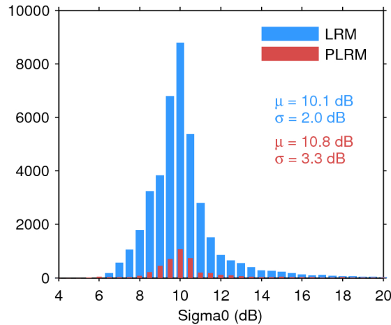
Figure 25. Histogram of flag-valid sigma0 over oceans and lakes for LRM (blue) and PLRM (red) for 26/11/2016. The mean ( \mu ) and standard deviation ( \sigma ) are also shown. Note that values outside [4 20] dB are excluded from the histogram for the sake of readability but not from the computation of \mu and \sigma .
