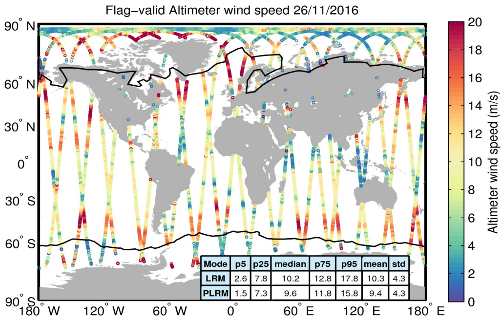
Figure 31. Geographical distribution of flag-valid wind data over oceans and lakes for 26/11/2016. The statistical values shown in the table refer to the wind in m/s and are calculated separately for LRM and PLRM regions. Measurements taken over polar polygons have been excluded from the computation of the statistical values. The black lines mark the outer limit of the Arctic and Antarctic polar polygons.
