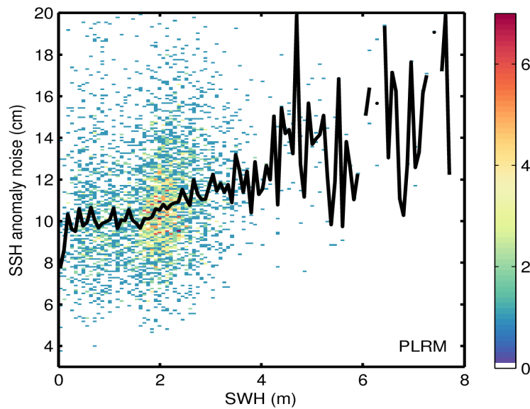
Figure 9. 2D histogram showing flag-valid SSH anomaly noise as a function of SWH for LRM (top) and PLRM (bottom) for 26/11/2016. The black line denotes the median SSH anomaly noise as a function of SWH.
