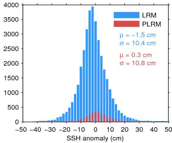
Figure 11. Histogram of science-valid SSH anomaly over oceans and lakes for LRM (blue) and PLRM (red) for 26/11/2016. The mean ( \mu ) and standard deviation ( \sigma ) are also shown. Note that values outside [-50 50] cm are excluded from the histogram for the sake of readability but not from the computation of \mu and \sigma .
