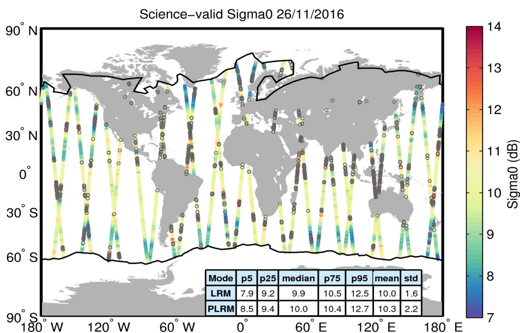
Figure 27. Geographical distribution of science-valid sigma0 data over oceans and lakes for 26/11/2016. The statistical values shown in the table refer to the sigma0 in dB and are calculated separately for LRM and PLRM regions. The black lines mark the outer limit of the Arctic and Antarctic polar polygons. Gray circles denote records that have been rejected based on the editing criteria described in Table 4.
