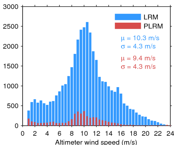
Figure 33. Histogram of flag-valid wind over oceans and lakes for LRM (blue) and PLRM (red) for 26/11/2016. The mean ( \mu ) and standard deviation ( \sigma ) are also shown. Note that values larger than 24 m/s are excluded from the histogram for the sake of readability but not from the computation of \mu and \sigma .
