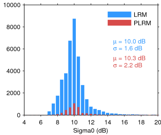
Figure 28. Histogram of science-valid sigma0 over oceans and lakes for LRM (blue) and PLRM (red) for 26/11/2016. The mean ( \mu ) and standard deviation ( \sigma ) are also shown. Note that values outside [4 20] dB are excluded from the histogram for the sake of readability but not from the computation of \mu and \sigma .
