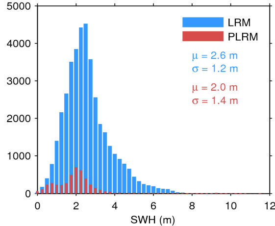
Figure 17. Histogram of flag-valid SWH over oceans and lakes for LRM (blue) and PLRM (red) for 26/11/2016. The mean ( \mu ) and standard deviation ( \sigma ) are also shown. Note that values larger than 12 m are excluded from the histogram for the sake of readability but not from the computation of \mu and \sigma .
