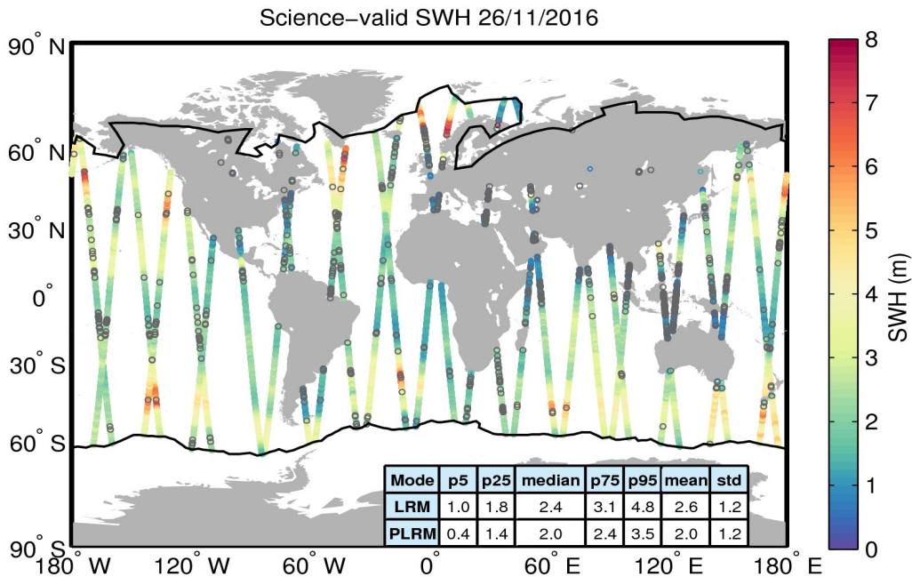
Figure 19. Geographical distribution of science-valid SWH data over oceans and lakes for 26/11/2016. The statistical values shown in the table refer to the SWH in m and are calculated separately for LRM and PLRM regions. The black lines mark the outer limit of the Arctic and Antarctic polar polygons. Gray circles denote records that have been rejected based on the editing criteria described in Table 3.
