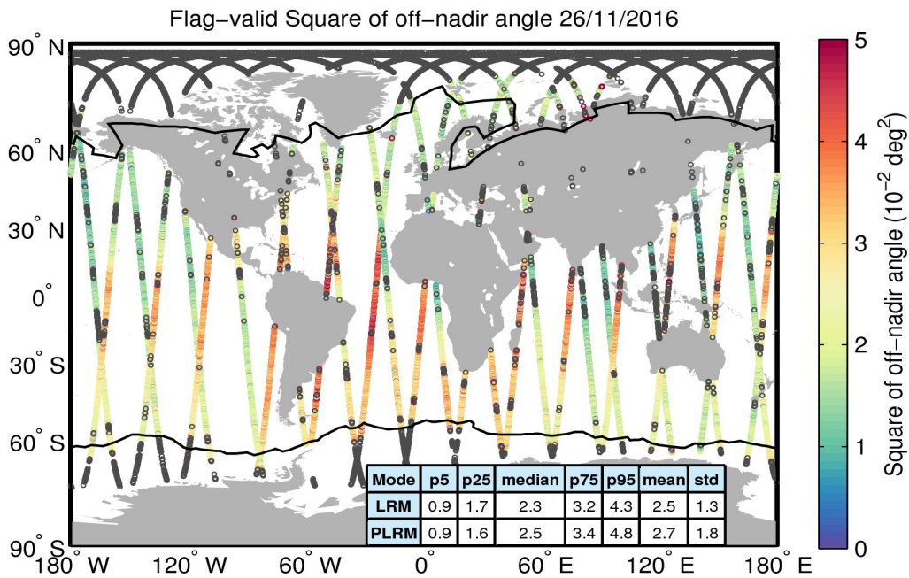
Figure 37. Geographical distribution of flag-valid mispointing data over oceans and lakes for 26/11/2016. The statistical values shown in the table refer to the mispointing in 10^{-2} \text{ deg}^2 and are calculated separately for LRM and PLRM regions. Measurements taken over polar polygons have been excluded from the computation of the statistical values. The black lines mark the outer limit of the Arctic and Antarctic polar polygons. Gray circles denote negative values.
