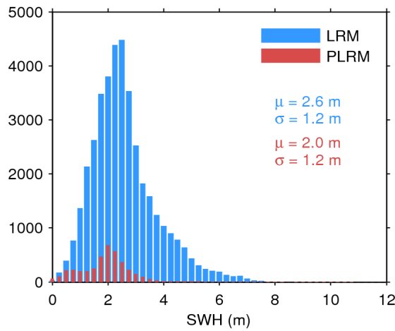
Figure 20. Histogram of science-valid SWH over oceans and lakes for LRM (blue) and PLRM (red) for 26/11/2016. The mean ( \mu ) and standard deviation ( \sigma ) are also shown. Note that values larger than 12 m are excluded from the histogram for the sake of readability but not from the computation of \mu and \sigma .
