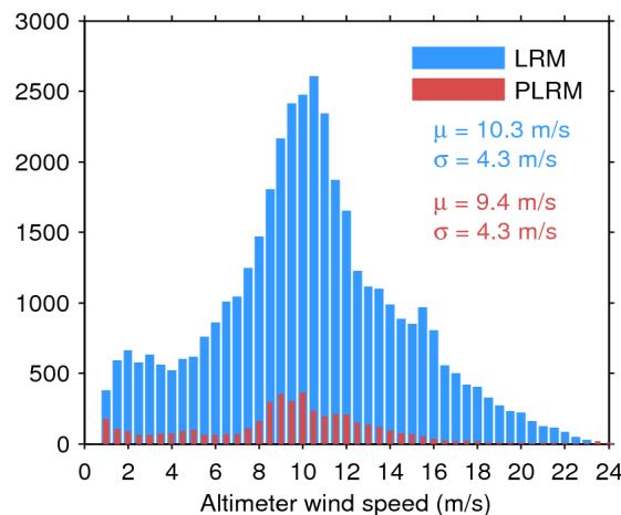
Figure 35. Histogram of science-valid wind over oceans and lakes for LRM (blue) and PLRM (red) for 26/11/2016. The mean ( \mu ) and standard deviation ( \sigma ) are also shown. Note that values larger than 24 m/s are excluded from the histogram for the sake of readability but not from the computation of \mu and \sigma .
