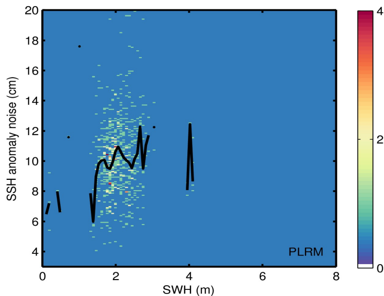
Figure 9. 2D histogram showing flag-valid SSH anomaly noise as a function of SWH for LRM (top) and PLRM (bottom) for 24/11/2016. The black line denotes the median SSH anomaly noise as a function of SWH.
