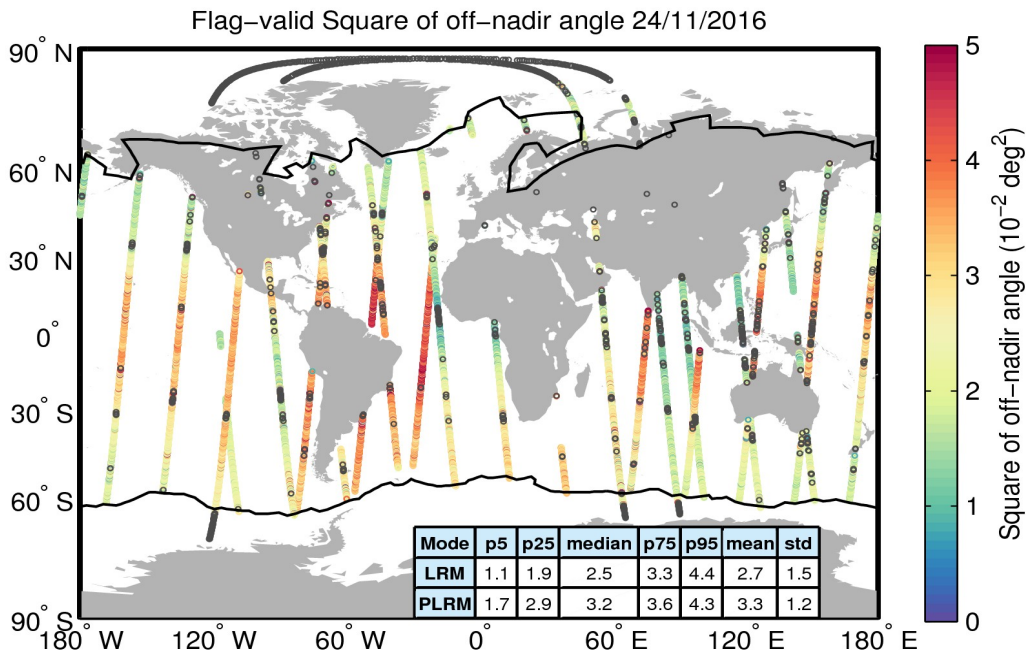
Figure 37. Geographical distribution of flag-valid mispointing data over oceans and lakes for 24/11/2016. The statistical values shown in the table refer to the mispointing in 10^{-2} \text{ deg}^2 and are calculated separately for LRM and PLRM regions. Measurements taken over polar polygons have been excluded from the computation of the statistical values. The black lines mark the outer limit of the Arctic and Antarctic polar polygons. Gray circles denote negative values.
