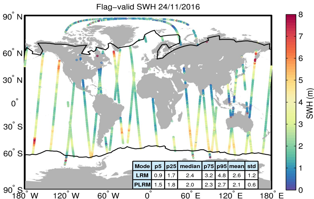
Figure 15. Geographical distribution of flag-valid SWH data over oceans and lakes for 24/11/2016. The statistical values shown in the table refer to the SWH in m and are calculated separately for LRM and PLRM regions. Measurements taken over polar polygons have been excluded from the computation of the statistical values. The black lines mark the outer limit of the Arctic and Antarctic polar polygons.
