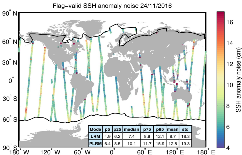
Figure 8. Geographical distribution of flag-valid 20-Hz SSH anomaly measurement noise over oceans and lakes for 24/11/2016. The statistical values shown in the table refer to the SSH anomaly noise and are calculated separately for LRM and PLRM regions. Measurements taken over polar polygons have been excluded from the computation of the statistical values. The black lines mark the outer limit of the Arctic and Antarctic polar polygons.
