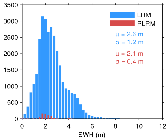
Figure 20. Histogram of science-valid SWH over oceans and lakes for LRM (blue) and PLRM (red) for 24/11/2016. The mean ( \mu ) and standard deviation ( \sigma ) are also shown. Note that values larger than 12 m are excluded from the histogram for the sake of readability but not from the computation of \mu and \sigma .
