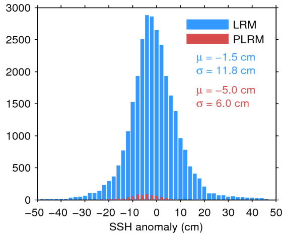
Figure 11. Histogram of science-valid SSH anomaly over oceans and lakes for LRM (blue) and PLRM (red) for 24/11/2016. The mean ( \mu ) and standard deviation ( \sigma ) are also shown. Note that values outside [-50 50] cm are excluded from the histogram for the sake of readability but not from the computation of \mu and \sigma .
