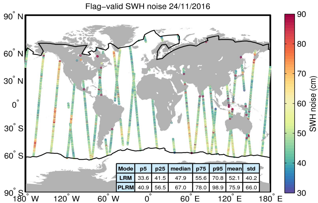
Figure 18. Geographical distribution of flag-valid 20-Hz SWH measurement noise over oceans and lakes for 24/11/2016. The statistical values shown in the table refer to the SWH noise and are calculated separately for LRM and PLRM regions. Measurements taken over polar polygons have been excluded from the computation of the statistical values. The black lines mark the outer limit of the Arctic and Antarctic polar polygons.
