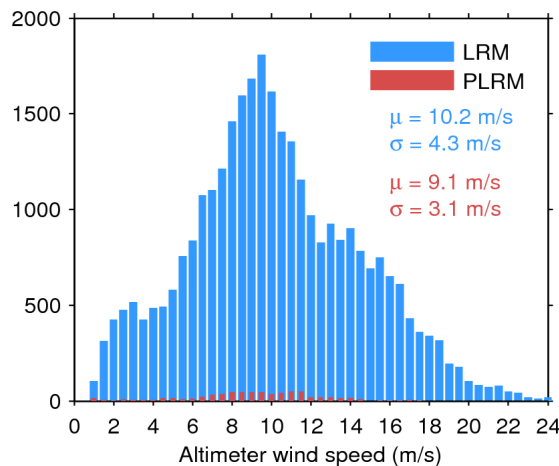
Figure 35. Histogram of science-valid wind over oceans and lakes for LRM (blue) and PLRM (red) for 24/11/2016. The mean ( \mu ) and standard deviation ( \sigma ) are also shown. Note that values larger than 24 m/s are excluded from the histogram for the sake of readability but not from the computation of \mu and \sigma .
