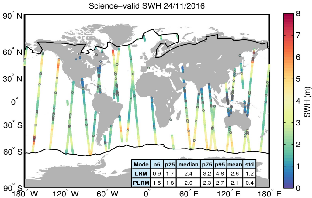
Figure 19. Geographical distribution of science-valid SWH data over oceans and lakes for 24/11/2016. The statistical values shown in the table refer to the SWH in m and are calculated separately for LRM and PLRM regions. The black lines mark the outer limit of the Arctic and Antarctic polar polygons. Gray circles denote records that have been rejected based on the editing criteria described in Table 3.
