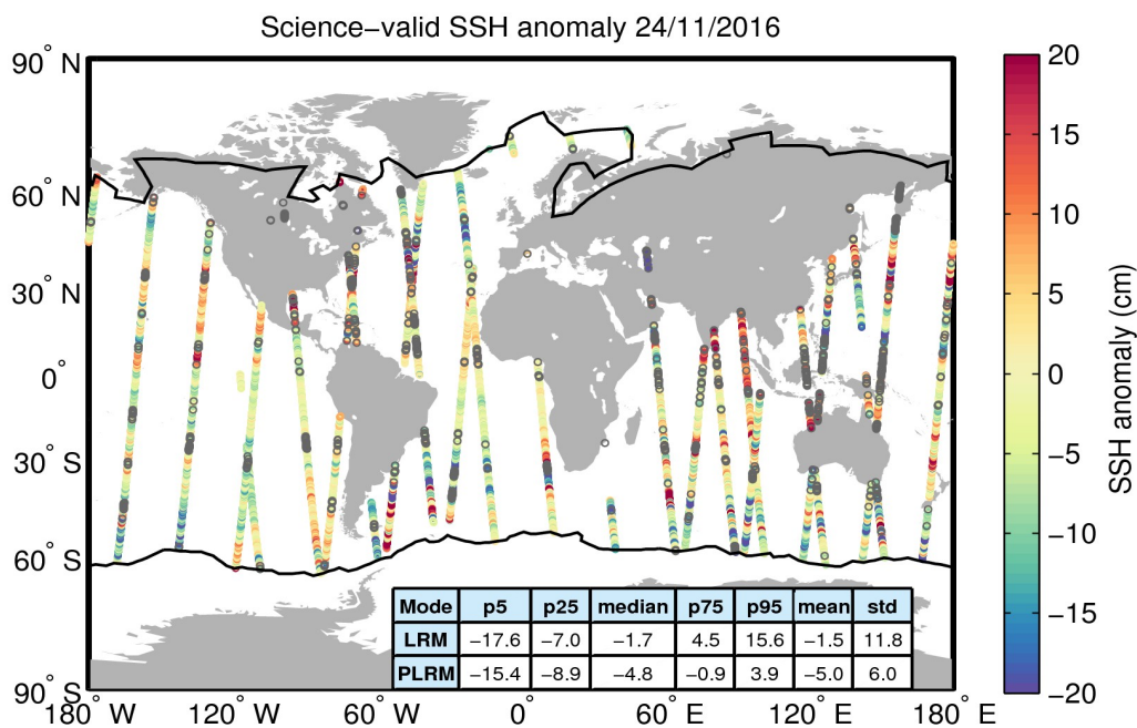
Figure 10. Geographical distribution of science-valid SSH anomaly data over oceans and lakes for 24/11/2016. The statistical values shown in the table refer to the SSH anomaly in cm and are calculated separately for LRM and PLRM regions. The black lines mark the outer limit of the Arctic and Antarctic polar polygons. Gray circles denote records that have been rejected based on the editing criteria described in Table 2.
