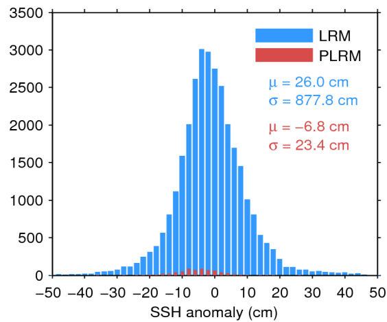
Figure 7. Histogram of flag-valid SSH anomaly over oceans and lakes for LRM (blue) and PLRM (red) for 24/11/2016. The mean ( \mu ) and standard deviation ( \sigma ) are also shown. Note that values outside [-50\ 50] cm are excluded from the histogram for the sake of readability but not from the computation of \mu and \sigma .
