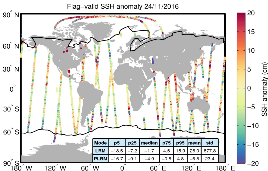
Figure 5. Geographical distribution of flag-valid 1-Hz SSH anomaly data over oceans and lakes for 24/11/2016. The statistical values shown in the table refer to the SSH anomaly in cm and are calculated separately for LRM and PLRM regions. Measurements taken over polar polygons have been excluded from the computation of the statistical values. The black lines mark the outer limit of the Arctic and Antarctic polar polygons.
