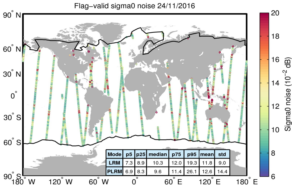
Figure 26. Geographical distribution of flag-valid 20-Hz sigma0 measurement noise over oceans and lakes for 24/11/2016. The statistical values shown in the table refer to the sigma0 noise and are calculated separately for LRM and PLRM regions. Measurements taken over polar polygons have been excluded from the computation of the statistical values. The black lines mark the outer limit of the Arctic and Antarctic polar polygons.
