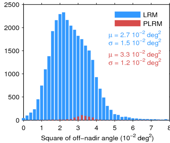
Figure 39. Histogram of flag-valid mispointing over oceans and lakes for LRM (blue) and PLRM (red) for 24/11/2016. Only positive values have been considered. The mean ( \mu ) and standard deviation ( \sigma ) are also shown. Note that values larger than 8 \cdot 10^{-2} \text{ deg}^2 are excluded from the histogram for the sake of readability but not from the computation of \mu and \sigma .
