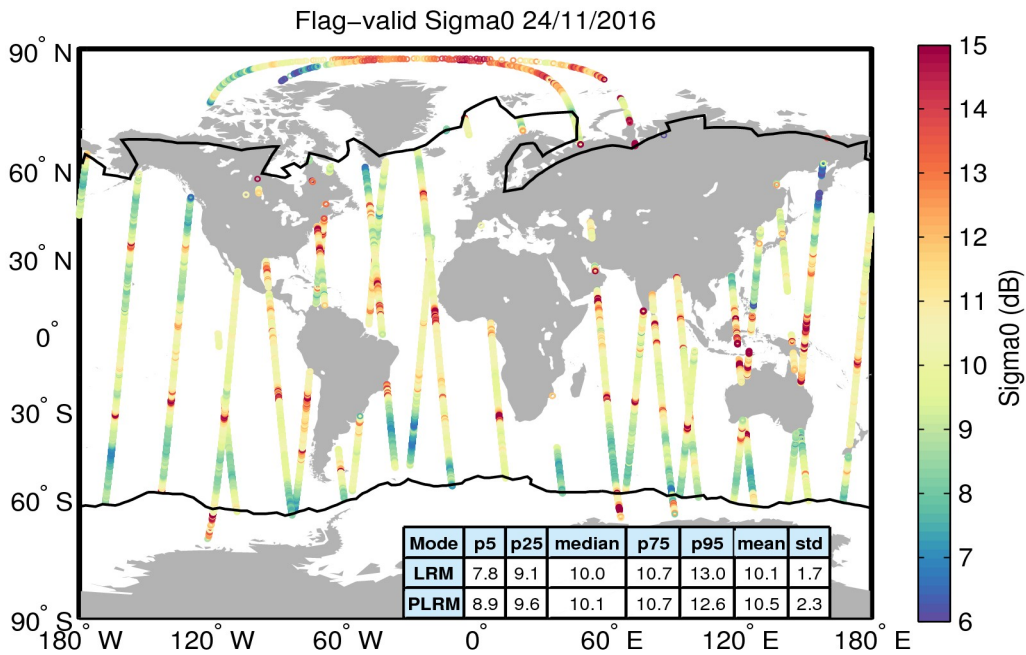
Figure 23. Geographical distribution of flag-valid sigma0 data over oceans and lakes for 24/11/2016. The statistical values shown in the table refer to the sigma0 in dB and are calculated separately for LRM and PLRM regions. Measurements taken over polar polygons have been excluded from the computation of the statistical values. The black lines mark the outer limit of the Arctic and Antarctic polar polygons.
