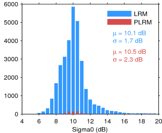
Figure 25. Histogram of flag-valid sigma0 over oceans and lakes for LRM (blue) and PLRM (red) for 24/11/2016. The mean ( \mu ) and standard deviation ( \sigma ) are also shown. Note that values outside [4 20] dB are excluded from the histogram for the sake of readability but not from the computation of \mu and \sigma .
