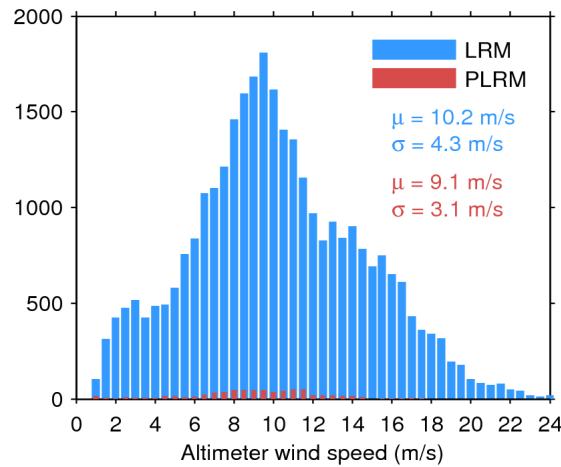
Figure 33. Histogram of flag-valid wind over oceans and lakes for LRM (blue) and PLRM (red) for 24/11/2016. The mean ( \mu ) and standard deviation ( \sigma ) are also shown. Note that values larger than 24 m/s are excluded from the histogram for the sake of readability but not from the computation of \mu and \sigma .
