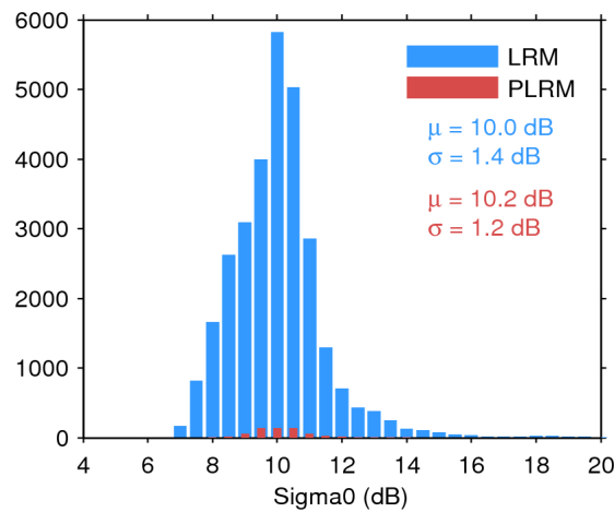
Figure 28. Histogram of science-valid sigma0 over oceans and lakes for LRM (blue) and PLRM (red) for 24/11/2016. The mean ( \mu ) and standard deviation ( \sigma ) are also shown. Note that values outside [4 20] dB are excluded from the histogram for the sake of readability but not from the computation of \mu and \sigma .
