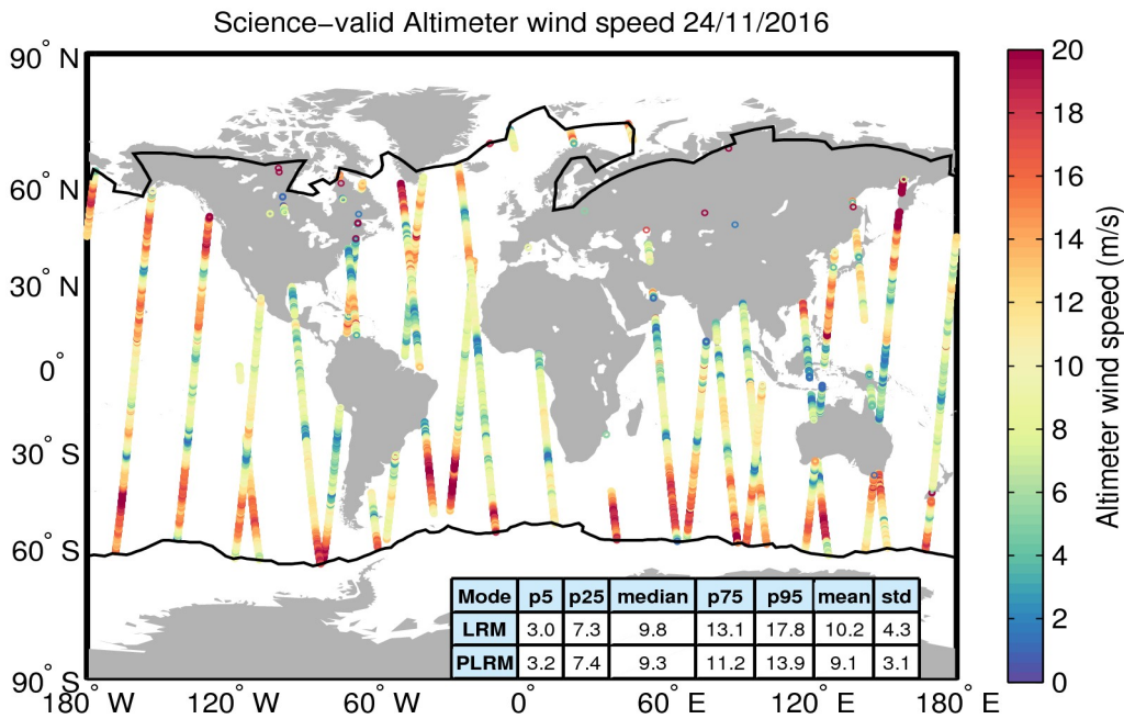
Figure 34. Geographical distribution of science-valid wind data over oceans and lakes for 24/11/2016. The statistical values shown in the table refer to the wind in m/s and are calculated separately for LRM and PLRM regions. The black lines mark the outer limit of the Arctic and Antarctic polar polygons. Gray circles denote records that have been rejected based on the editing criteria described in Table 5.
