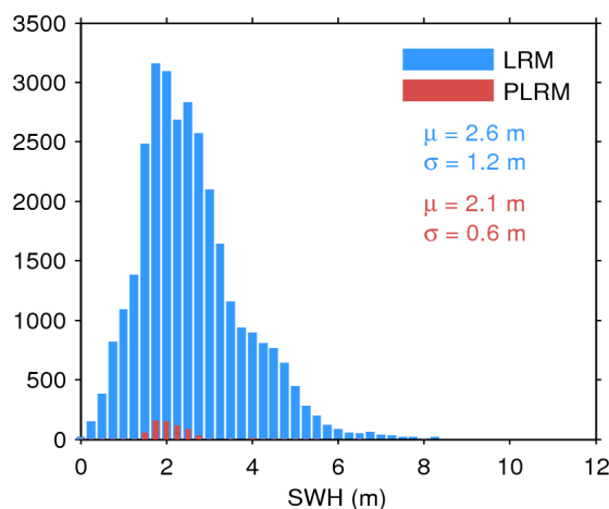
Figure 17. Histogram of flag-valid SWH over oceans and lakes for LRM (blue) and PLRM (red) for 24/11/2016. The mean ( \mu ) and standard deviation ( \sigma ) are also shown. Note that values larger than 12 m are excluded from the histogram for the sake of readability but not from the computation of \mu and \sigma .
