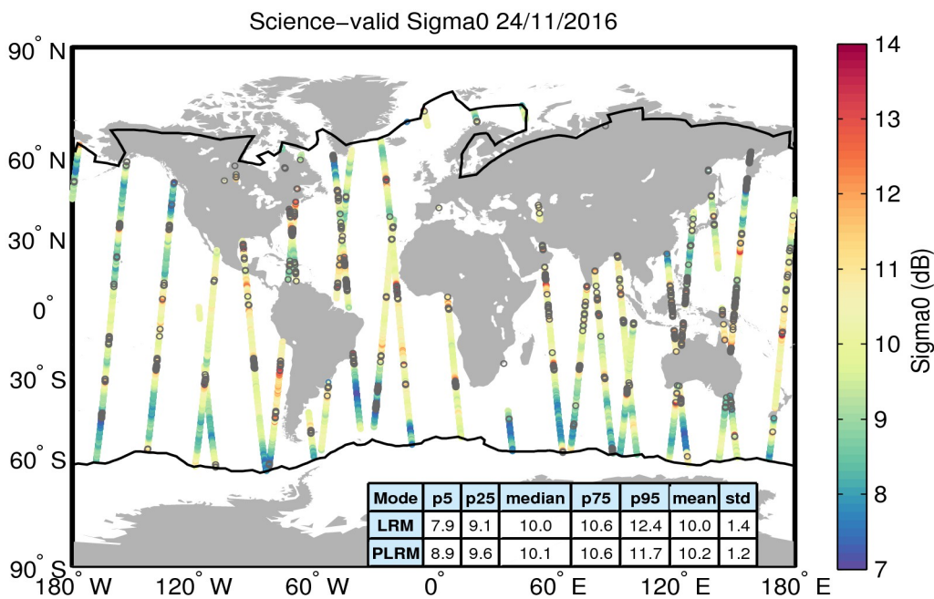
Figure 27. Geographical distribution of science-valid sigma0 data over oceans and lakes for 24/11/2016. The statistical values shown in the table refer to the sigma0 in dB and are calculated separately for LRM and PLRM regions. The black lines mark the outer limit of the Arctic and Antarctic polar polygons. Gray circles denote records that have been rejected based on the editing criteria described in Table 4.
