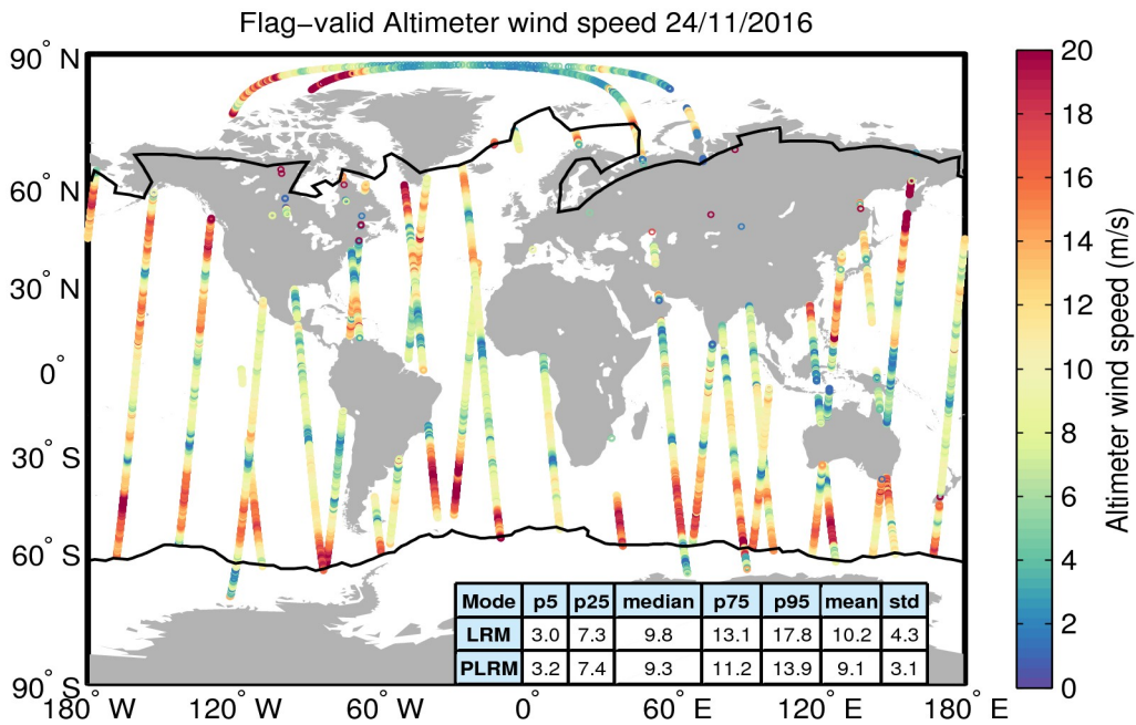
Figure 31. Geographical distribution of flag-valid wind data over oceans and lakes for 24/11/2016. The statistical values shown in the table refer to the wind in m/s and are calculated separately for LRM and PLRM regions. Measurements taken over polar polygons have been excluded from the computation of the statistical values. The black lines mark the outer limit of the Arctic and Antarctic polar polygons.
