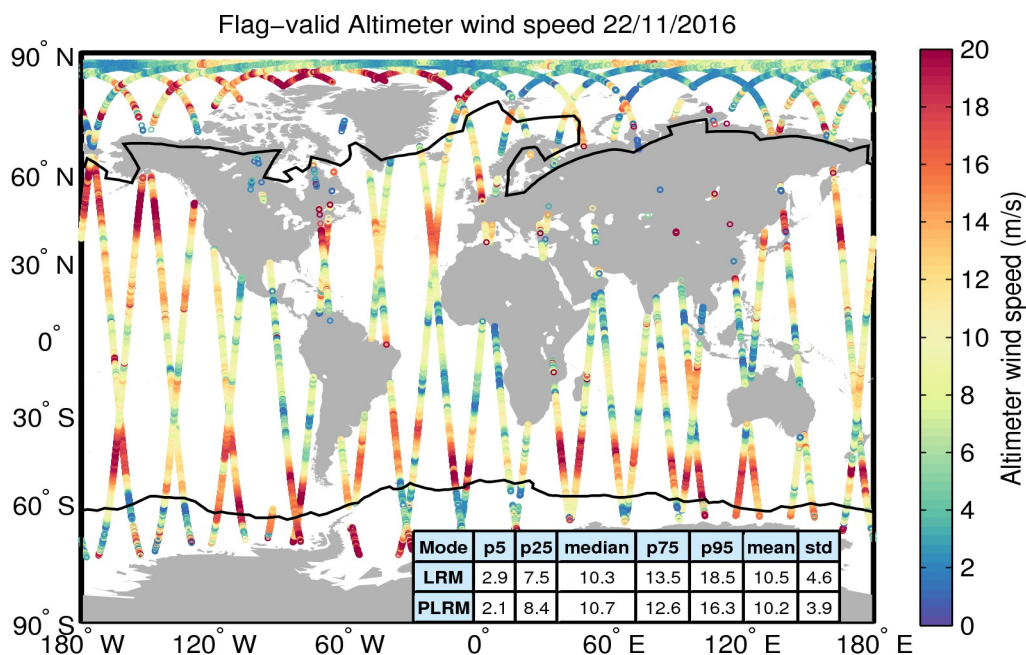
Figure 31. Geographical distribution of flag-valid wind data over oceans and lakes for 22/11/2016. The statistical values shown in the table refer to the wind in m/s and are calculated separately for LRM and PLRM regions. Measurements taken over polar polygons have been excluded from the computation of the statistical values. The black lines mark the outer limit of the Arctic and Antarctic polar polygons.
