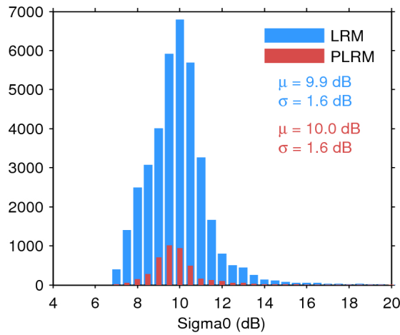
Figure 28. Histogram of science-valid sigma0 over oceans and lakes for LRM (blue) and PLRM (red) for 22/11/2016. The mean ( \mu ) and standard deviation ( \sigma ) are also shown. Note that values outside [4 20] dB are excluded from the histogram for the sake of readability but not from the computation of \mu and \sigma .
