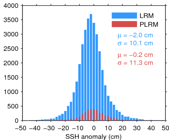
Figure 11. Histogram of science-valid SSH anomaly over oceans and lakes for LRM (blue) and PLRM (red) for 22/11/2016. The mean ( \mu ) and standard deviation ( \sigma ) are also shown. Note that values outside [-50 50] cm are excluded from the histogram for the sake of readability but not from the computation of \mu and \sigma .
