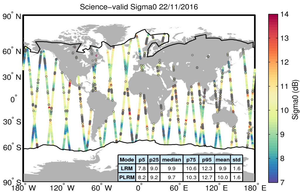
Figure 27. Geographical distribution of science-valid sigma0 data over oceans and lakes for 22/11/2016. The statistical values shown in the table refer to the sigma0 in dB and are calculated separately for LRM and PLRM regions. The black lines mark the outer limit of the Arctic and Antarctic polar polygons. Gray circles denote records that have been rejected based on the editing criteria described in Table 4.
