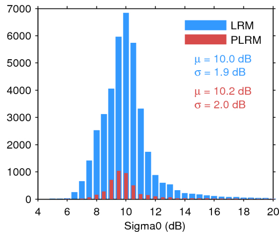
Figure 25. Histogram of flag-valid sigma0 over oceans and lakes for LRM (blue) and PLRM (red) for 22/11/2016. The mean ( \mu ) and standard deviation ( \sigma ) are also shown. Note that values outside [4 20] dB are excluded from the histogram for the sake of readability but not from the computation of \mu and \sigma .
