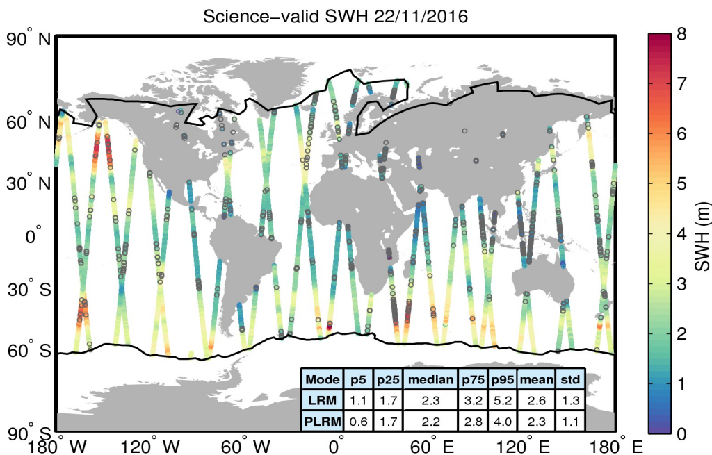
Figure 19. Geographical distribution of science-valid SWH data over oceans and lakes for 22/11/2016. The statistical values shown in the table refer to the SWH in m and are calculated separately for LRM and PLRM regions. The black lines mark the outer limit of the Arctic and Antarctic polar polygons. Gray circles denote records that have been rejected based on the editing criteria described in Table 3.
