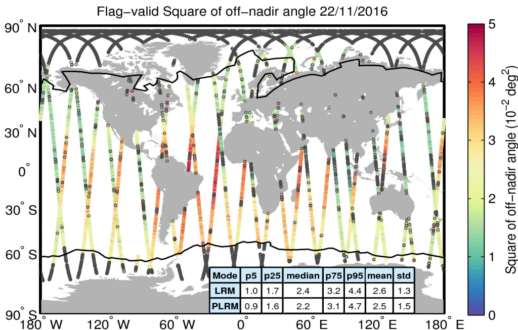
Figure 37. Geographical distribution of flag-valid mispointing data over oceans and lakes for 22/11/2016. The statistical values shown in the table refer to the mispointing in 10^{-2} deg 2 and are calculated separately for LRM and PLRM regions. Measurements taken over polar polygons have been excluded from the computation of the statistical values. The black lines mark the outer limit of the Arctic and Antarctic polar polygons. Gray circles denote negative values.
