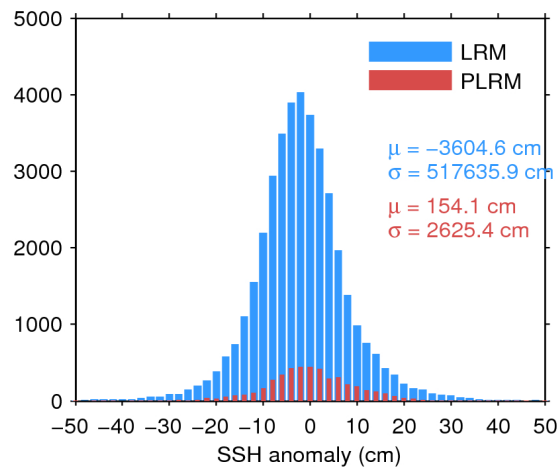
Figure 7. Histogram of flag-valid SSH anomaly over oceans and lakes for LRM (blue) and PLRM (red) for 22/11/2016. The mean ( \mu ) and standard deviation ( \sigma ) are also shown. Note that values outside [-50\ 50] cm are excluded from the histogram for the sake of readability but not from the computation of \mu and \sigma .
