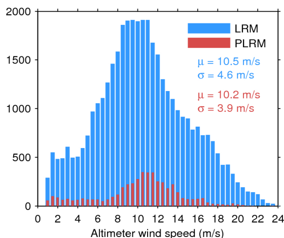
Figure 35. Histogram of science-valid wind over oceans and lakes for LRM (blue) and PLRM (red) for 22/11/2016. The mean ( \mu ) and standard deviation ( \sigma ) are also shown. Note that values larger than 24 m/s are excluded from the histogram for the sake of readability but not from the computation of \mu and \sigma .
