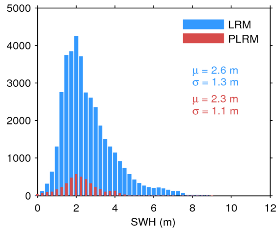
Figure 20. Histogram of science-valid SWH over oceans and lakes for LRM (blue) and PLRM (red) for 22/11/2016. The mean ( \mu ) and standard deviation ( \sigma ) are also shown. Note that values larger than 12 m are excluded from the histogram for the sake of readability but not from the computation of \mu and \sigma .
