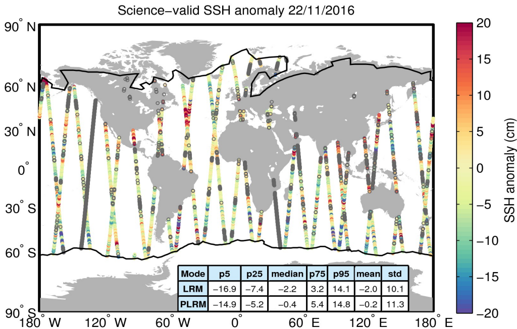
Figure 10. Geographical distribution of science-valid SSH anomaly data over oceans and lakes for 22/11/2016. The statistical values shown in the table refer to the SSH anomaly in cm and are calculated separately for LRM and PLRM regions. The black lines mark the outer limit of the Arctic and Antarctic polar polygons. Gray circles denote records that have been rejected based on the editing criteria described in Table 2.
