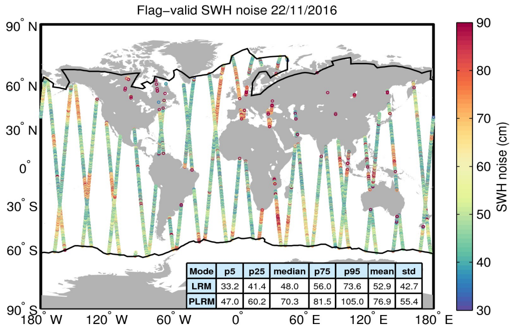
Figure 18. Geographical distribution of flag-valid 20-Hz SWH measurement noise over oceans and lakes for 22/11/2016. The statistical values shown in the table refer to the SWH noise and are calculated separately for LRM and PLRM regions. Measurements taken over polar polygons have been excluded from the computation of the statistical values. The black lines mark the outer limit of the Arctic and Antarctic polar polygons.
