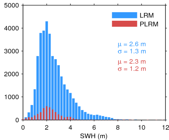
Figure 17. Histogram of flag-valid SWH over oceans and lakes for LRM (blue) and PLRM (red) for 22/11/2016. The mean ( \mu ) and standard deviation ( \sigma ) are also shown. Note that values larger than 12 m are excluded from the histogram for the sake of readability but not from the computation of \mu and \sigma .
