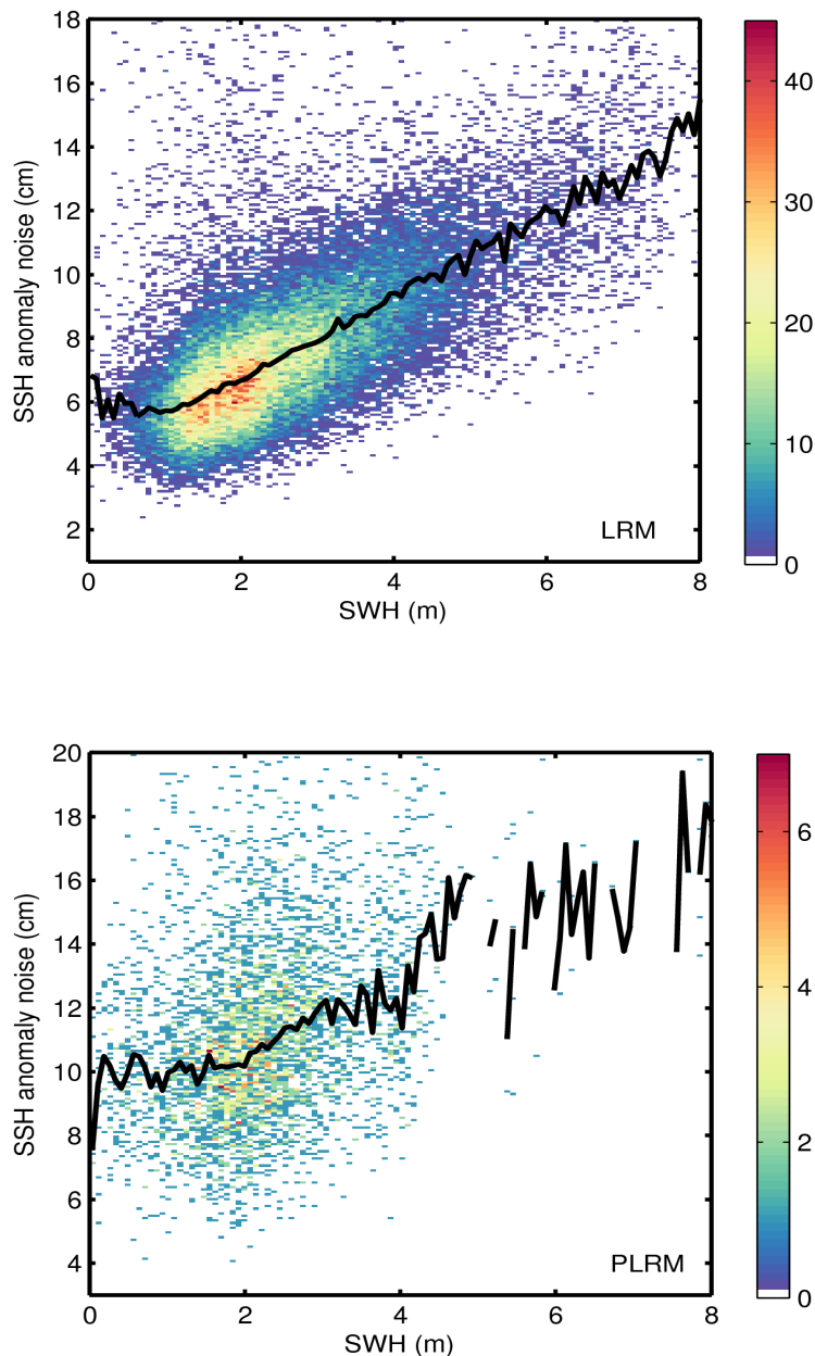
Figure 9. 2D histogram showing flag-valid SSH anomaly noise as a function of SWH for LRM (top) and PLRM (bottom) for 22/11/2016. The black line denotes the median SSH anomaly noise as a function of SWH.
