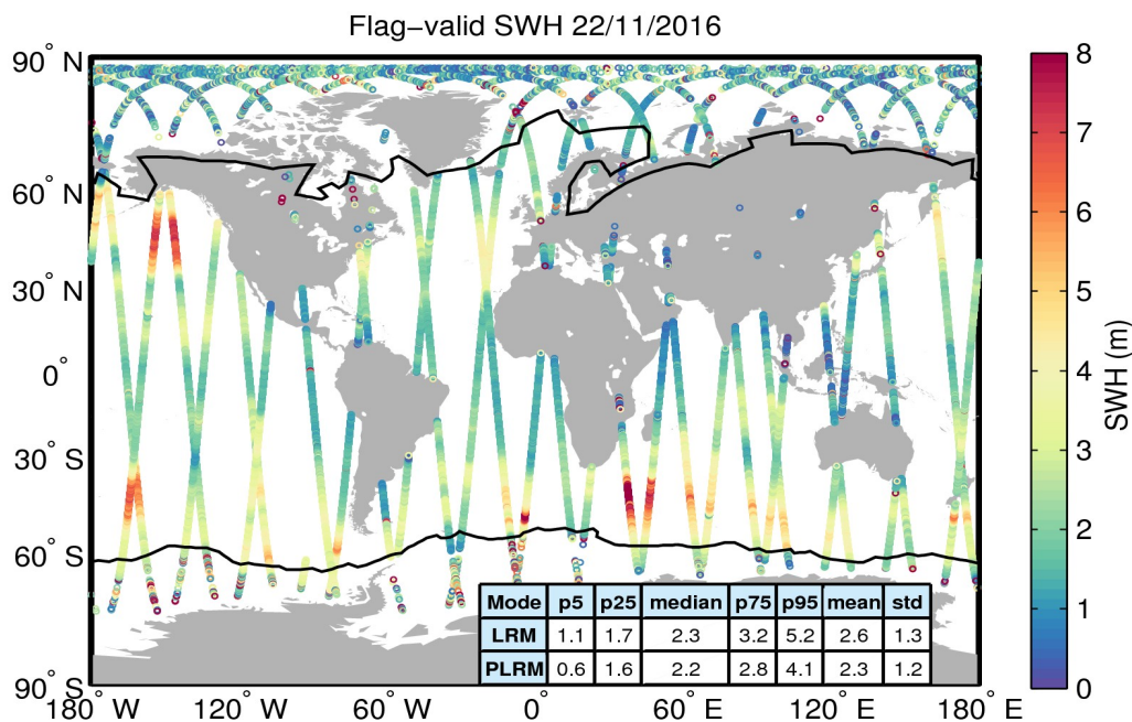
Figure 15. Geographical distribution of flag-valid SWH data over oceans and lakes for 22/11/2016. The statistical values shown in the table refer to the SWH in m and are calculated separately for LRM and PLRM regions. Measurements taken over polar polygons have been excluded from the computation of the statistical values. The black lines mark the outer limit of the Arctic and Antarctic polar polygons.
