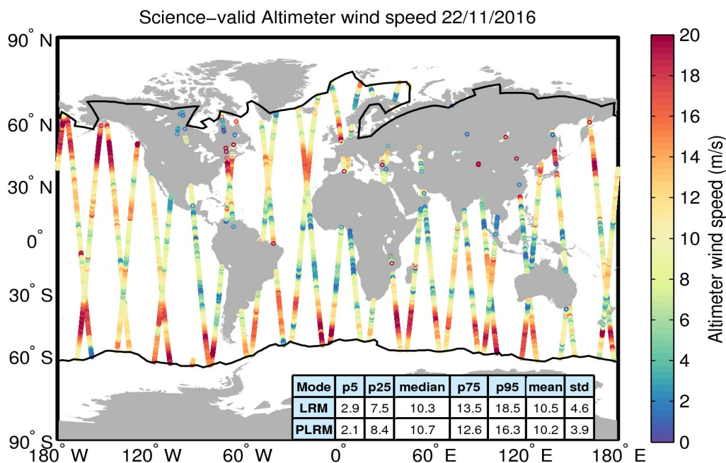
Figure 34. Geographical distribution of science-valid wind data over oceans and lakes for 22/11/2016. The statistical values shown in the table refer to the wind in m/s and are calculated separately for LRM and PLRM regions. The black lines mark the outer limit of the Arctic and Antarctic polar polygons. Gray circles denote records that have been rejected based on the editing criteria described in Table 5.
