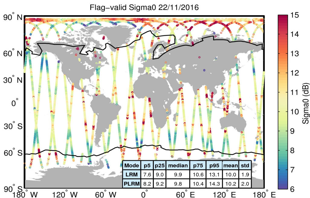
Figure 23. Geographical distribution of flag-valid sigma0 data over oceans and lakes for 22/11/2016. The statistical values shown in the table refer to the sigma0 in dB and are calculated separately for LRM and PLRM regions. Measurements taken over polar polygons have been excluded from the computation of the statistical values. The black lines mark the outer limit of the Arctic and Antarctic polar polygons.
