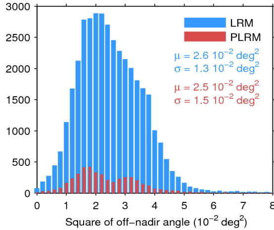
Figure 39. Histogram of flag-valid mispointing over oceans and lakes for LRM (blue) and PLRM (red) for 22/11/2016. Only positive values have been considered. The mean ( \mu ) and standard deviation ( \sigma ) are also shown. Note that values larger than 8 \cdot 10^{-2} \text{ deg}^2 are excluded from the histogram for the sake of readability but not from the computation of \mu and \sigma .
