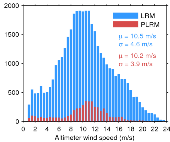
Figure 33. Histogram of flag-valid wind over oceans and lakes for LRM (blue) and PLRM (red) for 22/11/2016. The mean ( \mu ) and standard deviation ( \sigma ) are also shown. Note that values larger than 24 m/s are excluded from the histogram for the sake of readability but not from the computation of \mu and \sigma .
