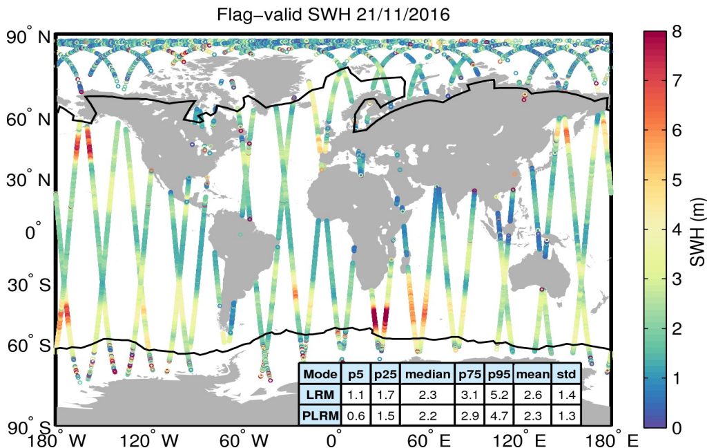
Figure 15. Geographical distribution of flag-valid SWH data over oceans and lakes for 21/11/2016. The statistical values shown in the table refer to the SWH in m and are calculated separately for LRM and PLRM regions. Measurements taken over polar polygons have been excluded from the computation of the statistical values. The black lines mark the outer limit of the Arctic and Antarctic polar polygons.
