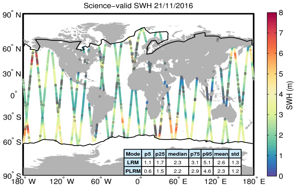
Figure 19. Geographical distribution of science-valid SWH data over oceans and lakes for 21/11/2016. The statistical values shown in the table refer to the SWH in m and are calculated separately for LRM and PLRM regions. The black lines mark the outer limit of the Arctic and Antarctic polar polygons. Gray circles denote records that have been rejected based on the editing criteria described in Table 3.
