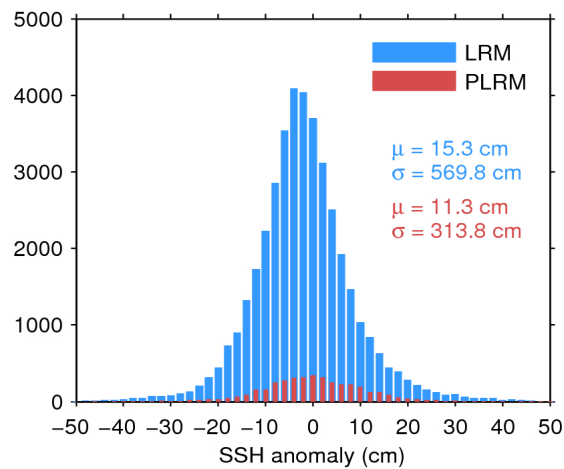
Figure 7. Histogram of flag-valid SSH anomaly over oceans and lakes for LRM (blue) and PLRM (red) for 21/11/2016. The mean ( \mu ) and standard deviation ( \sigma ) are also shown. Note that values outside [-50 50] cm are excluded from the histogram for the sake of readability but not from the computation of \mu and \sigma .
