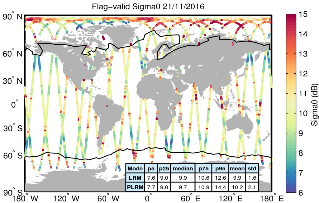
Figure 23. Geographical distribution of flag-valid sigma0 data over oceans and lakes for 21/11/2016. The statistical values shown in the table refer to the sigma0 in dB and are calculated separately for LRM and PLRM regions. Measurements taken over polar polygons have been excluded from the computation of the statistical values. The black lines mark the outer limit of the Arctic and Antarctic polar polygons.
