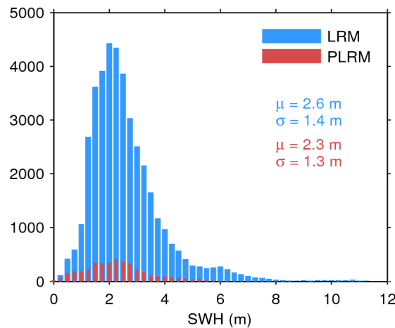
Figure 17. Histogram of flag-valid SWH over oceans and lakes for LRM (blue) and PLRM (red) for 21/11/2016. The mean ( \mu ) and standard deviation ( \sigma ) are also shown. Note that values larger than 12 m are excluded from the histogram for the sake of readability but not from the computation of \mu and \sigma .
