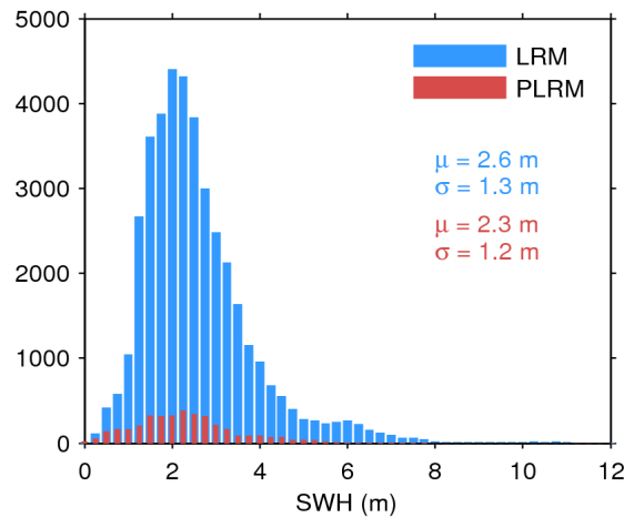
Figure 20. Histogram of science-valid SWH over oceans and lakes for LRM (blue) and PLRM (red) for 21/11/2016. The mean ( \mu ) and standard deviation ( \sigma ) are also shown. Note that values larger than 12 m are excluded from the histogram for the sake of readability but not from the computation of \mu and \sigma .
