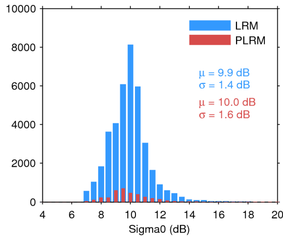
Figure 28. Histogram of science-valid sigma0 over oceans and lakes for LRM (blue) and PLRM (red) for 21/11/2016. The mean ( \mu ) and standard deviation ( \sigma ) are also shown. Note that values outside [4 20] dB are excluded from the histogram for the sake of readability but not from the computation of \mu and \sigma .
