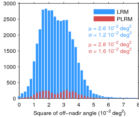
Figure 39. Histogram of flag-valid mispointing over oceans and lakes for LRM (blue) and PLRM (red) for 21/11/2016. Only positive values have been considered. The mean ( \mu ) and standard deviation ( \sigma ) are also shown. Note that values larger than 8 \cdot 10^{-2} \text{ deg}^2 are excluded from the histogram for the sake of readability but not from the computation of \mu and \sigma .
