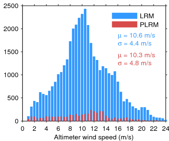
Figure 35. Histogram of science-valid wind over oceans and lakes for LRM (blue) and PLRM (red) for 21/11/2016. The mean ( \mu ) and standard deviation ( \sigma ) are also shown. Note that values larger than 24 m/s are excluded from the histogram for the sake of readability but not from the computation of \mu and \sigma .
