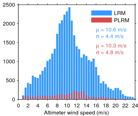
Figure 33. Histogram of flag-valid wind over oceans and lakes for LRM (blue) and PLRM (red) for 21/11/2016. The mean ( \mu ) and standard deviation ( \sigma ) are also shown. Note that values larger than 24 m/s are excluded from the histogram for the sake of readability but not from the computation of \mu and \sigma .
