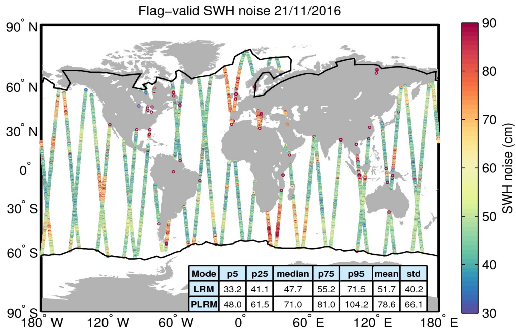
Figure 18. Geographical distribution of flag-valid 20-Hz SWH measurement noise over oceans and lakes for 21/11/2016. The statistical values shown in the table refer to the SWH noise and are calculated separately for LRM and PLRM regions. Measurements taken over polar polygons have been excluded from the computation of the statistical values. The black lines mark the outer limit of the Arctic and Antarctic polar polygons.
