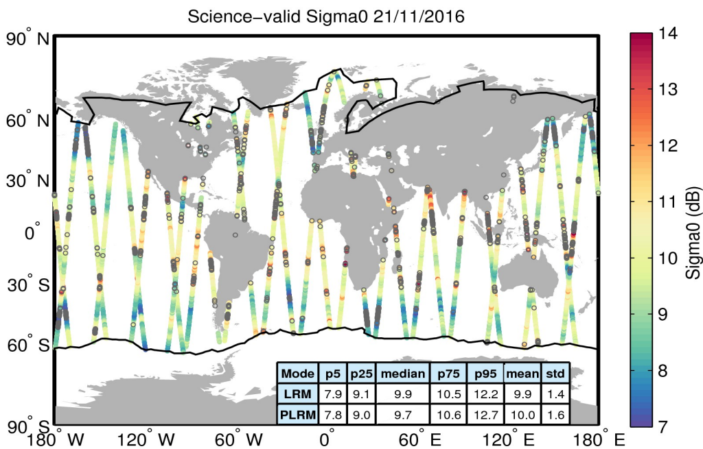
Figure 27. Geographical distribution of science-valid sigma0 data over oceans and lakes for 21/11/2016. The statistical values shown in the table refer to the sigma0 in dB and are calculated separately for LRM and PLRM regions. The black lines mark the outer limit of the Arctic and Antarctic polar polygons. Gray circles denote records that have been rejected based on the editing criteria described in Table 4.
