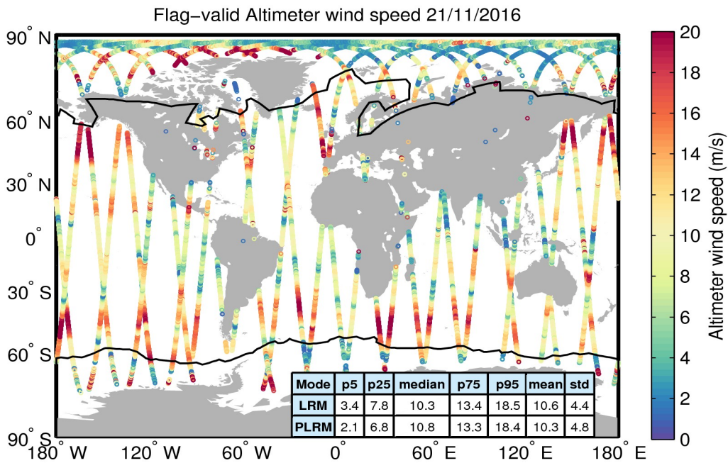
Figure 31. Geographical distribution of flag-valid wind data over oceans and lakes for 21/11/2016. The statistical values shown in the table refer to the wind in m/s and are calculated separately for LRM and PLRM regions. Measurements taken over polar polygons have been excluded from the computation of the statistical values. The black lines mark the outer limit of the Arctic and Antarctic polar polygons.
