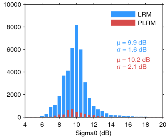
Figure 25. Histogram of flag-valid sigma0 over oceans and lakes for LRM (blue) and PLRM (red) for 21/11/2016. The mean ( \mu ) and standard deviation ( \sigma ) are also shown. Note that values outside [4 20] dB are excluded from the histogram for the sake of readability but not from the computation of \mu and \sigma .
