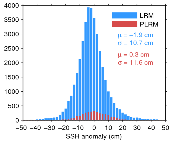
Figure 11. Histogram of science-valid SSH anomaly over oceans and lakes for LRM (blue) and PLRM (red) for 21/11/2016. The mean ( \mu ) and standard deviation ( \sigma ) are also shown. Note that values outside [-50\ 50] cm are excluded from the histogram for the sake of readability but not from the computation of \mu and \sigma .
