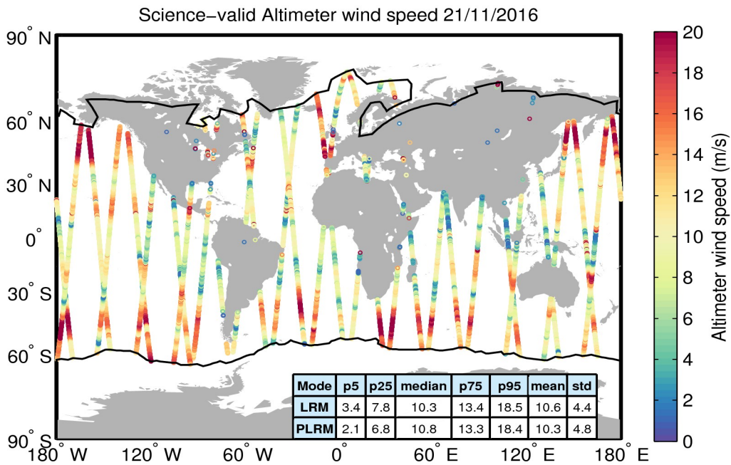
Figure 34. Geographical distribution of science-valid wind data over oceans and lakes for 21/11/2016. The statistical values shown in the table refer to the wind in m/s and are calculated separately for LRM and PLRM regions. The black lines mark the outer limit of the Arctic and Antarctic polar polygons. Gray circles denote records that have been rejected based on the editing criteria described in Table 5.
