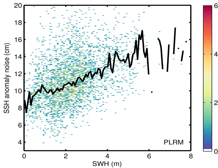
Figure 9. 2D histogram showing flag-valid SSH anomaly noise as a function of SWH for LRM (top) and PLRM (bottom) for 21/11/2016. The black line denotes the median SSH anomaly noise as a function of SWH.
