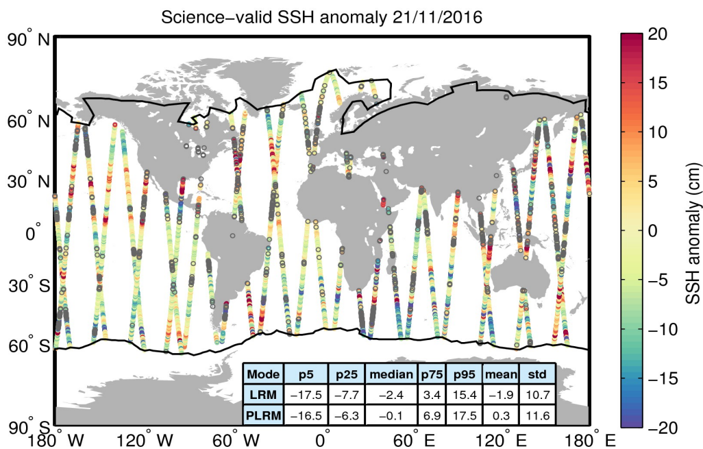
Figure 10. Geographical distribution of science-valid SSH anomaly data over oceans and lakes for 21/11/2016. The statistical values shown in the table refer to the SSH anomaly in cm and are calculated separately for LRM and PLRM regions. The black lines mark the outer limit of the Arctic and Antarctic polar polygons. Gray circles denote records that have been rejected based on the editing criteria described in Table 2.
