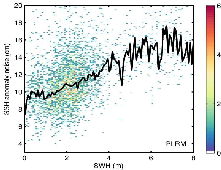
Figure 9. 2D histogram showing flag-valid SSH anomaly noise as a function of SWH for LRM (top) and PLRM (bottom) for 20/11/2016. The black line denotes the median SSH anomaly noise as a function of SWH.
