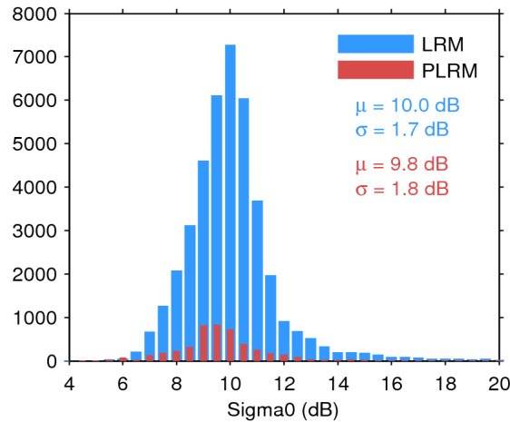
Figure 25. Histogram of flag-valid sigma0 over oceans and lakes for LRM (blue) and PLRM (red) for 20/11/2016. The mean ( \mu ) and standard deviation ( \sigma ) are also shown. Note that values outside [4 20] dB are excluded from the histogram for the sake of readability but not from the computation of \mu and \sigma .
