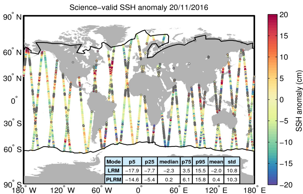
Figure 10. Geographical distribution of science-valid SSH anomaly data over oceans and lakes for 20/11/2016. The statistical values shown in the table refer to the SSH anomaly in cm and are calculated separately for LRM and PLRM regions. The black lines mark the outer limit of the Arctic and Antarctic polar polygons. Gray circles denote records that have been rejected based on the editing criteria described in Table 2.
