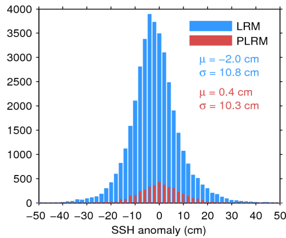
Figure 11. Histogram of science-valid SSH anomaly over oceans and lakes for LRM (blue) and PLRM (red) for 20/11/2016. The mean ( \mu ) and standard deviation ( \sigma ) are also shown. Note that values outside [-50 50] cm are excluded from the histogram for the sake of readability but not from the computation of \mu and \sigma .
