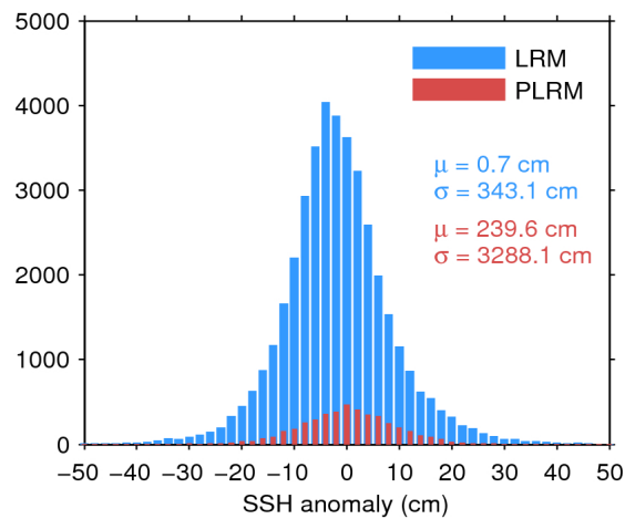
Figure 7. Histogram of flag-valid SSH anomaly over oceans and lakes for LRM (blue) and PLRM (red) for 20/11/2016. The mean ( \mu ) and standard deviation ( \sigma ) are also shown. Note that values outside [-50 50] cm are excluded from the histogram for the sake of readability but not from the computation of \mu and \sigma .
