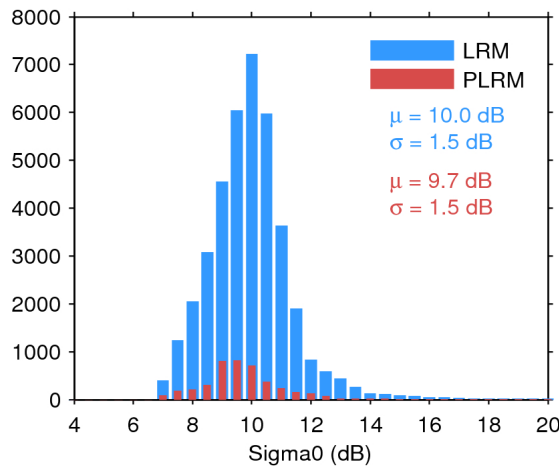
Figure 28. Histogram of science-valid sigma0 over oceans and lakes for LRM (blue) and PLRM (red) for 20/11/2016. The mean ( \mu ) and standard deviation ( \sigma ) are also shown. Note that values outside [4 20] dB are excluded from the histogram for the sake of readability but not from the computation of \mu and \sigma .
