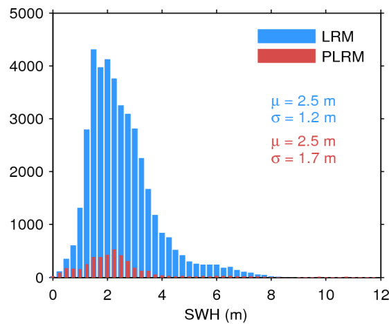
Figure 20. Histogram of science-valid SWH over oceans and lakes for LRM (blue) and PLRM (red) for 20/11/2016. The mean ( \mu ) and standard deviation ( \sigma ) are also shown. Note that values larger than 12 m are excluded from the histogram for the sake of readability but not from the computation of \mu and \sigma .
