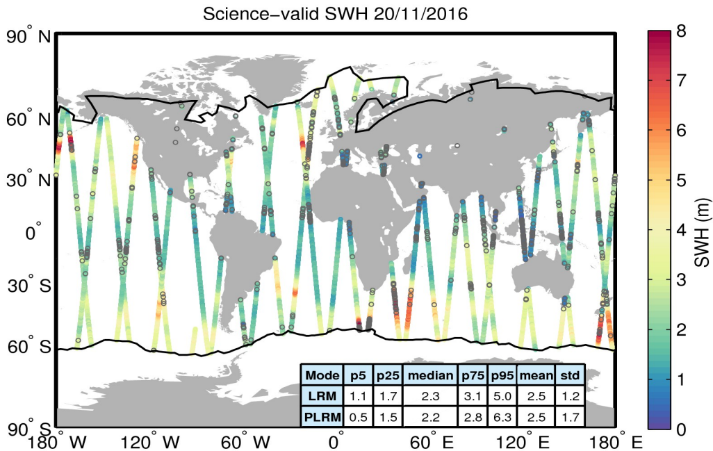
Figure 19. Geographical distribution of science-valid SWH data over oceans and lakes for 20/11/2016. The statistical values shown in the table refer to the SWH in m and are calculated separately for LRM and PLRM regions. The black lines mark the outer limit of the Arctic and Antarctic polar polygons. Gray circles denote records that have been rejected based on the editing criteria described in Table 3.
