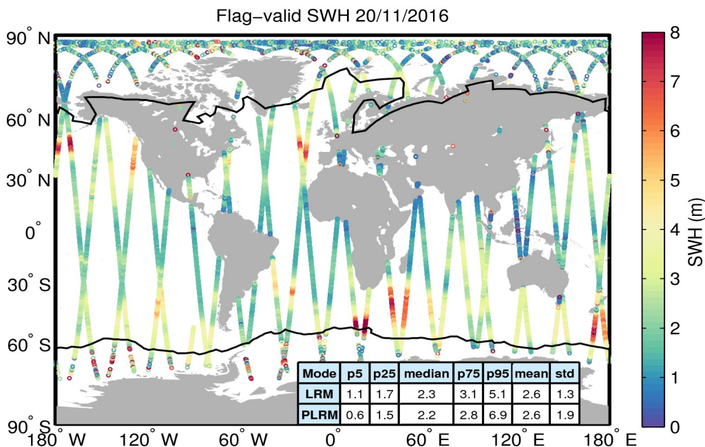
Figure 15. Geographical distribution of flag-valid SWH data over oceans and lakes for 20/11/2016. The statistical values shown in the table refer to the SWH in m and are calculated separately for LRM and PLRM regions. Measurements taken over polar polygons have been excluded from the computation of the statistical values. The black lines mark the outer limit of the Arctic and Antarctic polar polygons.
