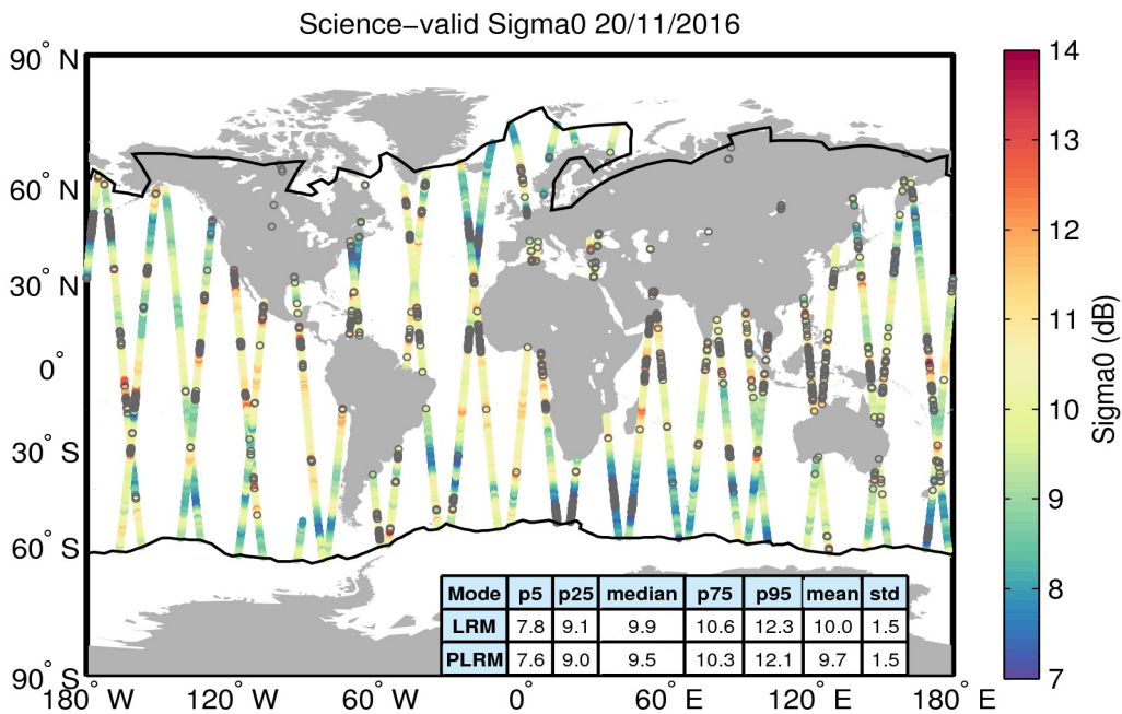
Figure 27. Geographical distribution of science-valid sigma0 data over oceans and lakes for 20/11/2016. The statistical values shown in the table refer to the sigma0 in dB and are calculated separately for LRM and PLRM regions. The black lines mark the outer limit of the Arctic and Antarctic polar polygons. Gray circles denote records that have been rejected based on the editing criteria described in Table 4.
