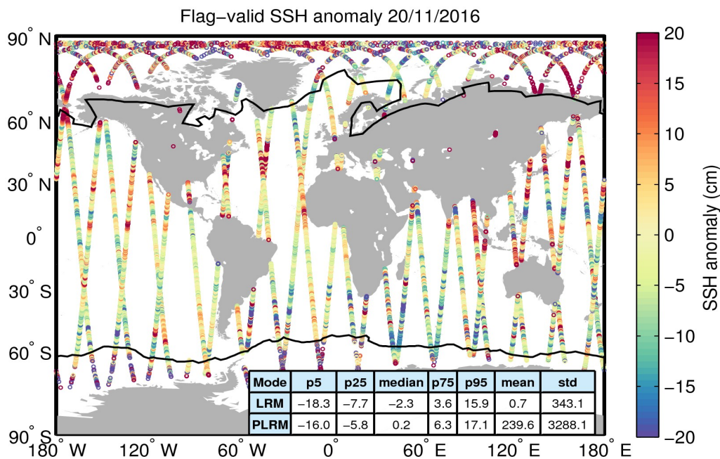
Figure 5. Geographical distribution of flag-valid 1-Hz SSH anomaly data over oceans and lakes for 20/11/2016. The statistical values shown in the table refer to the SSH anomaly in cm and are calculated separately for LRM and PLRM regions. Measurements taken over polar polygons have been excluded from the computation of the statistical values. The black lines mark the outer limit of the Arctic and Antarctic polar polygons.
