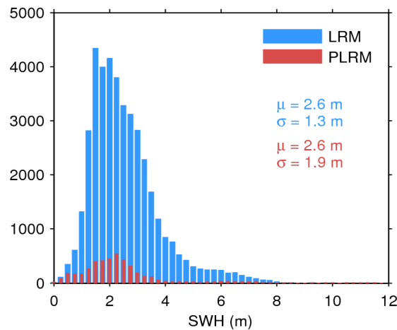
Figure 17. Histogram of flag-valid SWH over oceans and lakes for LRM (blue) and PLRM (red) for 20/11/2016. The mean ( \mu ) and standard deviation ( \sigma ) are also shown. Note that values larger than 12 m are excluded from the histogram for the sake of readability but not from the computation of \mu and \sigma .
