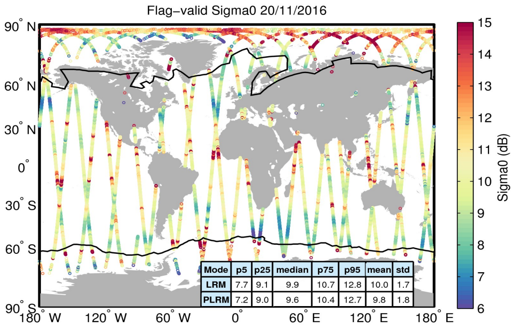
Figure 23. Geographical distribution of flag-valid sigma0 data over oceans and lakes for 20/11/2016. The statistical values shown in the table refer to the sigma0 in dB and are calculated separately for LRM and PLRM regions. Measurements taken over polar polygons have been excluded from the computation of the statistical values. The black lines mark the outer limit of the Arctic and Antarctic polar polygons.
