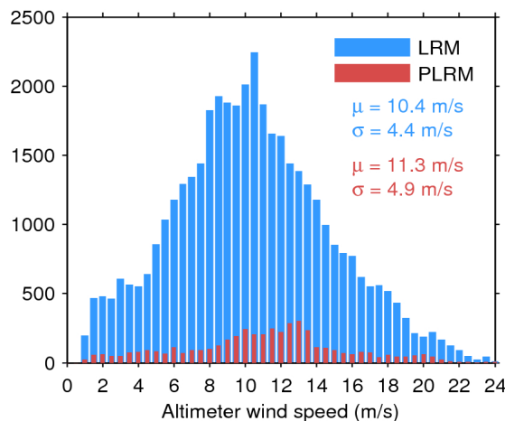
Figure 35. Histogram of science-valid wind over oceans and lakes for LRM (blue) and PLRM (red) for 20/11/2016. The mean ( \mu ) and standard deviation ( \sigma ) are also shown. Note that values larger than 24 m/s are excluded from the histogram for the sake of readability but not from the computation of \mu and \sigma .
