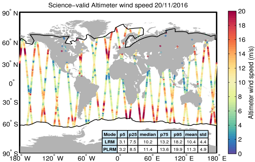
Figure 34. Geographical distribution of science-valid wind data over oceans and lakes for 20/11/2016. The statistical values shown in the table refer to the wind in m/s and are calculated separately for LRM and PLRM regions. The black lines mark the outer limit of the Arctic and Antarctic polar polygons. Gray circles denote records that have been rejected based on the editing criteria described in Table 5.
