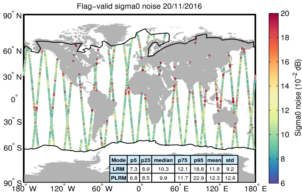
Figure 26. Geographical distribution of flag-valid 20-Hz sigma0 measurement noise over oceans and lakes for 20/11/2016. The statistical values shown in the table refer to the sigma0 noise and are calculated separately for LRM and PLRM regions. Measurements taken over polar polygons have been excluded from the computation of the statistical values. The black lines mark the outer limit of the Arctic and Antarctic polar polygons.
