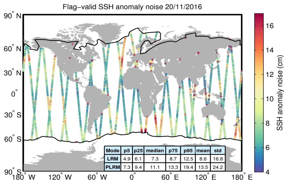
Figure 8. Geographical distribution of flag-valid 20-Hz SSH anomaly measurement noise over oceans and lakes for 20/11/2016. The statistical values shown in the table refer to the SSH anomaly noise and are calculated separately for LRM and PLRM regions. Measurements taken over polar polygons have been excluded from the computation of the statistical values. The black lines mark the outer limit of the Arctic and Antarctic polar polygons.
