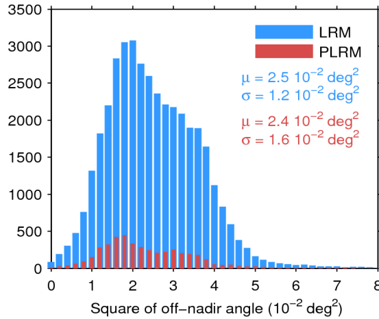
Figure 39. Histogram of flag-valid mispointing over oceans and lakes for LRM (blue) and PLRM (red) for 20/11/2016. Only positive values have been considered. The mean ( \mu ) and standard deviation ( \sigma ) are also shown. Note that values larger than 8 \cdot 10^{-2} \text{ deg}^2 are excluded from the histogram for the sake of readability but not from the computation of \mu and \sigma .
