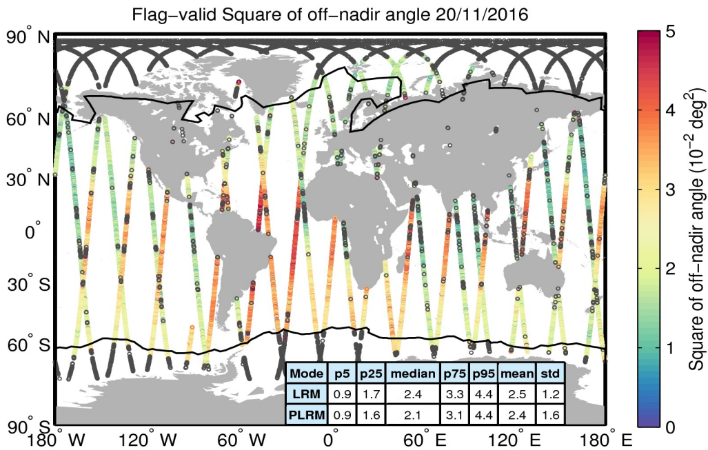
Figure 37. Geographical distribution of flag-valid mispointing data over oceans and lakes for 20/11/2016. The statistical values shown in the table refer to the mispointing in 10^{-2} \text{ deg}^2 and are calculated separately for LRM and PLRM regions. Measurements taken over polar polygons have been excluded from the computation of the statistical values. The black lines mark the outer limit of the Arctic and Antarctic polar polygons. Gray circles denote negative values.
