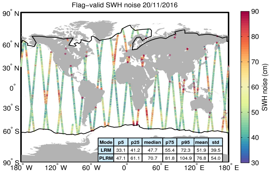
Figure 18. Geographical distribution of flag-valid 20-Hz SWH measurement noise over oceans and lakes for 20/11/2016. The statistical values shown in the table refer to the SWH noise and are calculated separately for LRM and PLRM regions. Measurements taken over polar polygons have been excluded from the computation of the statistical values. The black lines mark the outer limit of the Arctic and Antarctic polar polygons.
