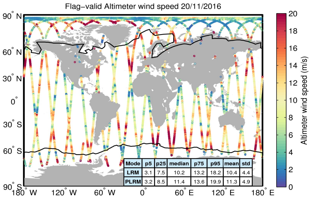
Figure 31. Geographical distribution of flag-valid wind data over oceans and lakes for 20/11/2016. The statistical values shown in the table refer to the wind in m/s and are calculated separately for LRM and PLRM regions. Measurements taken over polar polygons have been excluded from the computation of the statistical values. The black lines mark the outer limit of the Arctic and Antarctic polar polygons.
