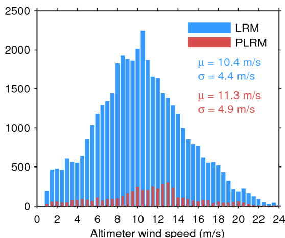
Figure 33. Histogram of flag-valid wind over oceans and lakes for LRM (blue) and PLRM (red) for 20/11/2016. The mean ( \mu ) and standard deviation ( \sigma ) are also shown. Note that values larger than 24 m/s are excluded from the histogram for the sake of readability but not from the computation of \mu and \sigma .
