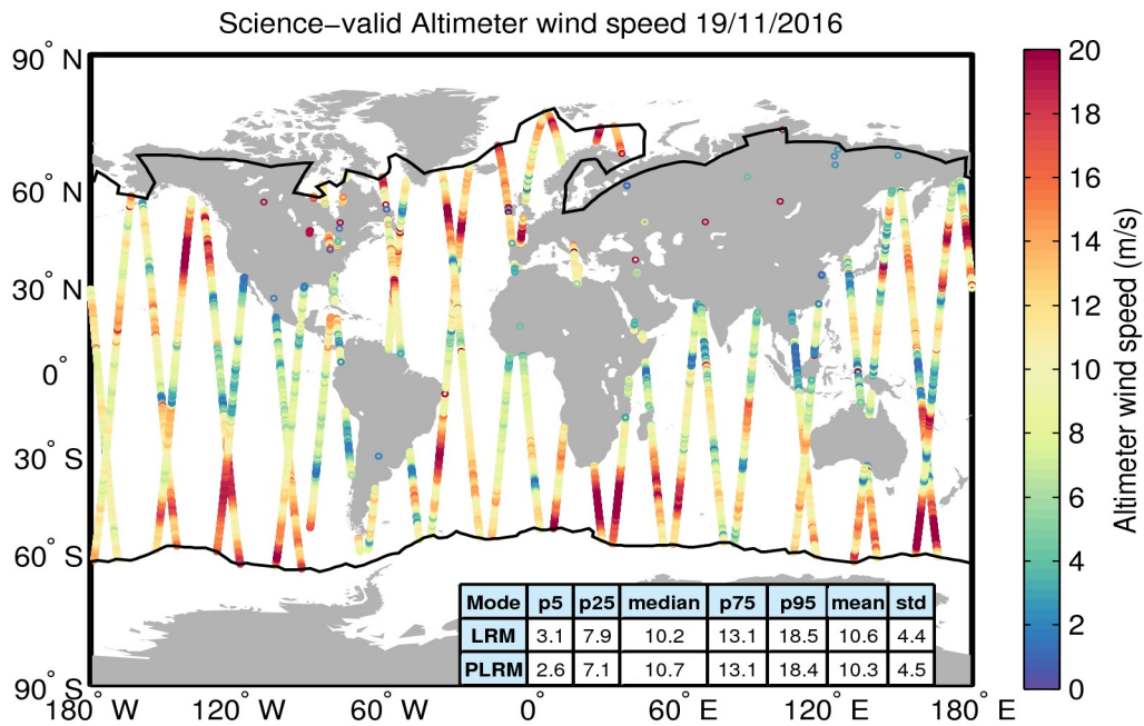
Figure 34. Geographical distribution of science-valid wind data over oceans and lakes for 19/11/2016. The statistical values shown in the table refer to the wind in m/s and are calculated separately for LRM and PLRM regions. The black lines mark the outer limit of the Arctic and Antarctic polar polygons. Gray circles denote records that have been rejected based on the editing criteria described in Table 5.
