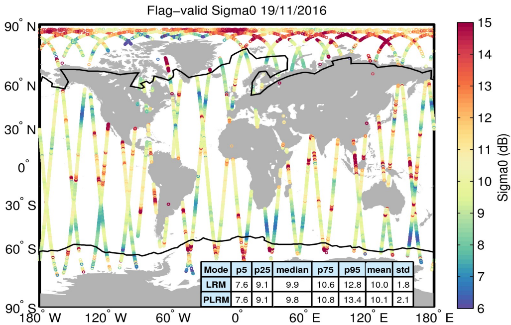
Figure 23. Geographical distribution of flag-valid sigma0 data over oceans and lakes for 19/11/2016. The statistical values shown in the table refer to the sigma0 in dB and are calculated separately for LRM and PLRM regions. Measurements taken over polar polygons have been excluded from the computation of the statistical values. The black lines mark the outer limit of the Arctic and Antarctic polar polygons.
