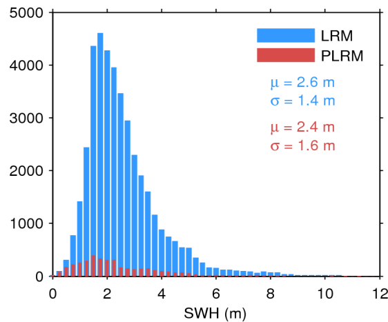
Figure 17. Histogram of flag-valid SWH over oceans and lakes for LRM (blue) and PLRM (red) for 19/11/2016. The mean ( \mu ) and standard deviation ( \sigma ) are also shown. Note that values larger than 12 m are excluded from the histogram for the sake of readability but not from the computation of \mu and \sigma .
