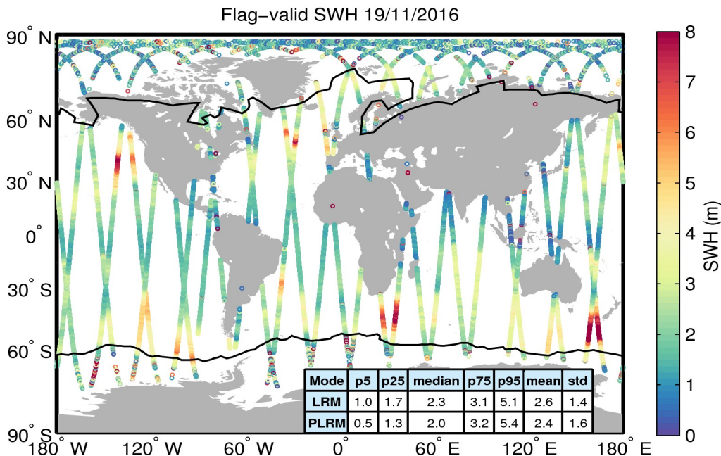
Figure 15. Geographical distribution of flag-valid SWH data over oceans and lakes for 19/11/2016. The statistical values shown in the table refer to the SWH in m and are calculated separately for LRM and PLRM regions. Measurements taken over polar polygons have been excluded from the computation of the statistical values. The black lines mark the outer limit of the Arctic and Antarctic polar polygons.
