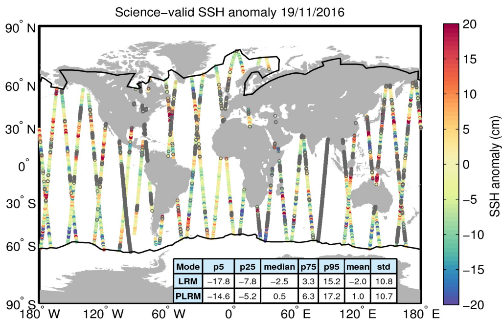
Figure 10. Geographical distribution of science-valid SSH anomaly data over oceans and lakes for 19/11/2016. The statistical values shown in the table refer to the SSH anomaly in cm and are calculated separately for LRM and PLRM regions. The black lines mark the outer limit of the Arctic and Antarctic polar polygons. Gray circles denote records that have been rejected based on the editing criteria described in Table 2.
