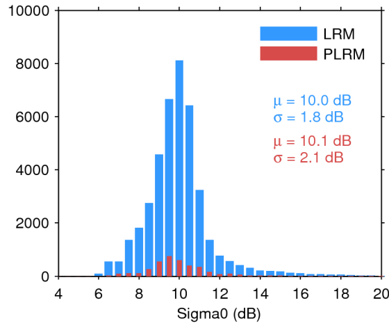
Figure 25. Histogram of flag-valid sigma0 over oceans and lakes for LRM (blue) and PLRM (red) for 19/11/2016. The mean ( \mu ) and standard deviation ( \sigma ) are also shown. Note that values outside [4 20] dB are excluded from the histogram for the sake of readability but not from the computation of \mu and \sigma .
