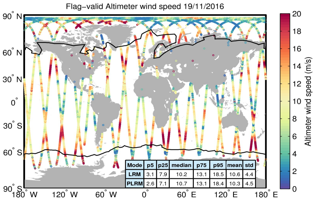
Figure 31. Geographical distribution of flag-valid wind data over oceans and lakes for 19/11/2016. The statistical values shown in the table refer to the wind in m/s and are calculated separately for LRM and PLRM regions. Measurements taken over polar polygons have been excluded from the computation of the statistical values. The black lines mark the outer limit of the Arctic and Antarctic polar polygons.
