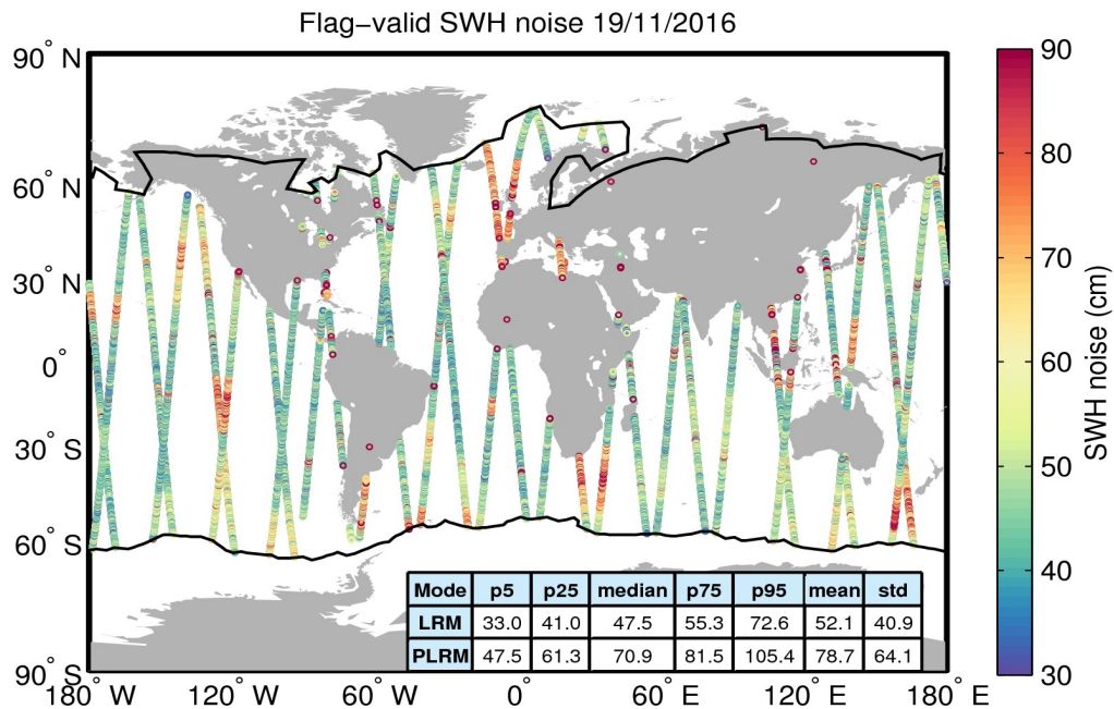
Figure 18. Geographical distribution of flag-valid 20-Hz SWH measurement noise over oceans and lakes for 19/11/2016. The statistical values shown in the table refer to the SWH noise and are calculated separately for LRM and PLRM regions. Measurements taken over polar polygons have been excluded from the computation of the statistical values. The black lines mark the outer limit of the Arctic and Antarctic polar polygons.
