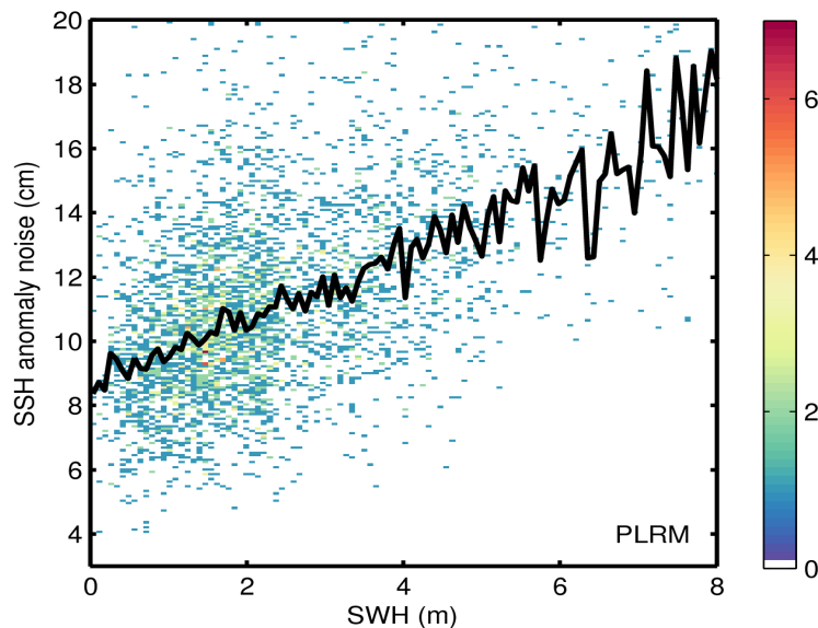
Figure 9. 2D histogram showing flag-valid SSH anomaly noise as a function of SWH for LRM (top) and PLRM (bottom) for 19/11/2016. The black line denotes the median SSH anomaly noise as a function of SWH.
