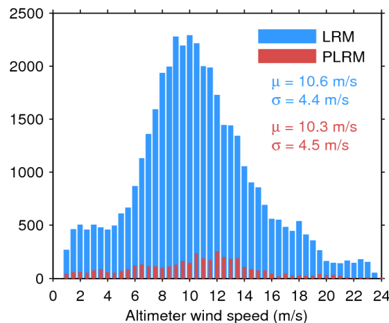
Figure 35. Histogram of science-valid wind over oceans and lakes for LRM (blue) and PLRM (red) for 19/11/2016. The mean ( \mu ) and standard deviation ( \sigma ) are also shown. Note that values larger than 24 m/s are excluded from the histogram for the sake of readability but not from the computation of \mu and \sigma .
