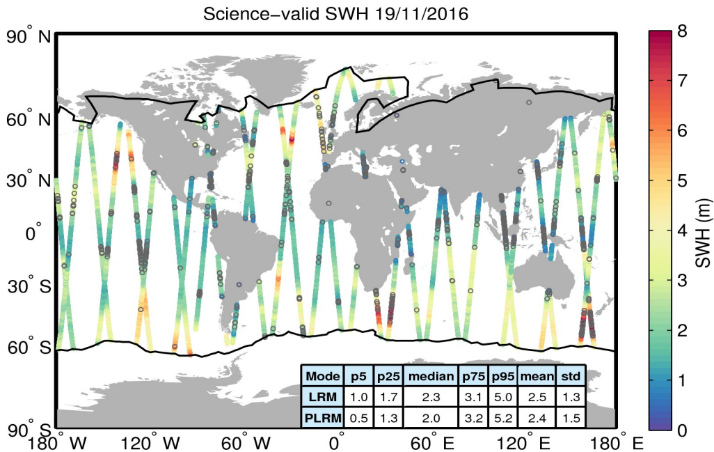
Figure 19. Geographical distribution of science-valid SWH data over oceans and lakes for 19/11/2016. The statistical values shown in the table refer to the SWH in m and are calculated separately for LRM and PLRM regions. The black lines mark the outer limit of the Arctic and Antarctic polar polygons. Gray circles denote records that have been rejected based on the editing criteria described in Table 3.
