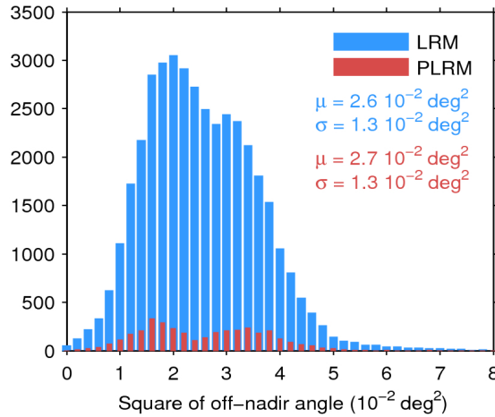
Figure 39. Histogram of flag-valid mispointing over oceans and lakes for LRM (blue) and PLRM (red) for 19/11/2016. Only positive values have been considered. The mean ( \mu ) and standard deviation ( \sigma ) are also shown. Note that values larger than 8 \cdot 10^{-2} \text{ deg}^2 are excluded from the histogram for the sake of readability but not from the computation of \mu and \sigma .
