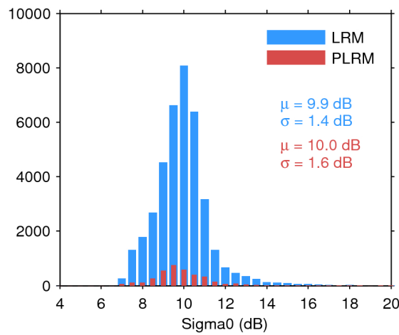
Figure 28. Histogram of science-valid sigma0 over oceans and lakes for LRM (blue) and PLRM (red) for 19/11/2016. The mean ( \mu ) and standard deviation ( \sigma ) are also shown. Note that values outside [4 20] dB are excluded from the histogram for the sake of readability but not from the computation of \mu and \sigma .
