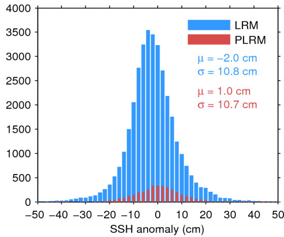
Figure 11. Histogram of science-valid SSH anomaly over oceans and lakes for LRM (blue) and PLRM (red) for 19/11/2016. The mean ( \mu ) and standard deviation ( \sigma ) are also shown. Note that values outside [-50\ 50] cm are excluded from the histogram for the sake of readability but not from the computation of \mu and \sigma .
