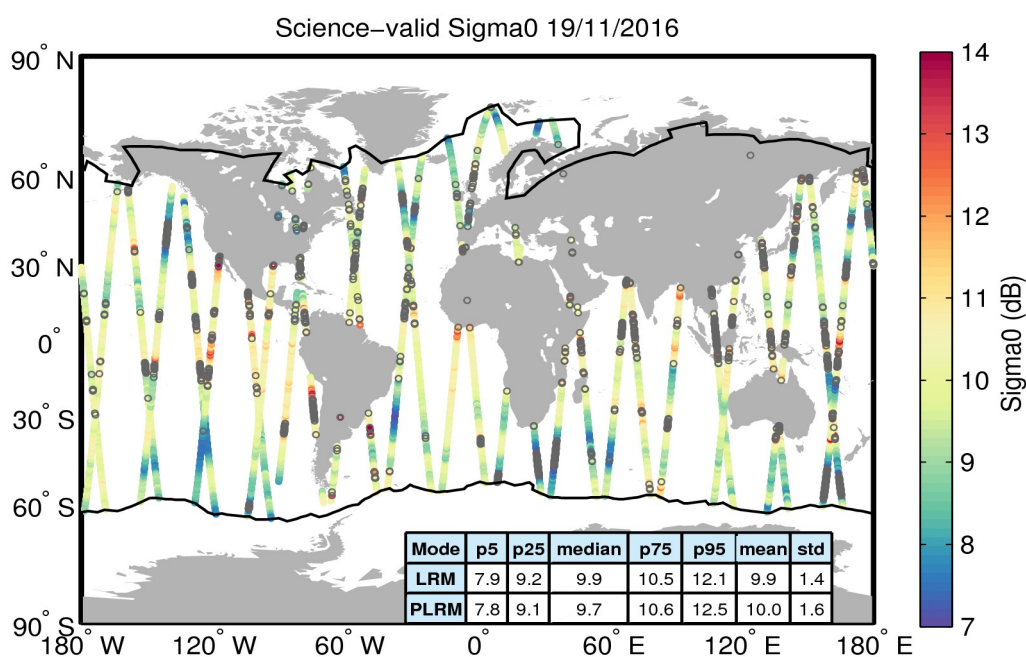
Figure 27. Geographical distribution of science-valid sigma0 data over oceans and lakes for 19/11/2016. The statistical values shown in the table refer to the sigma0 in dB and are calculated separately for LRM and PLRM regions. The black lines mark the outer limit of the Arctic and Antarctic polar polygons. Gray circles denote records that have been rejected based on the editing criteria described in Table 4.
