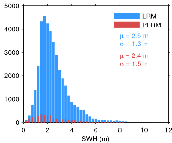
Figure 20. Histogram of science-valid SWH over oceans and lakes for LRM (blue) and PLRM (red) for 19/11/2016. The mean ( \mu ) and standard deviation ( \sigma ) are also shown. Note that values larger than 12 m are excluded from the histogram for the sake of readability but not from the computation of \mu and \sigma .
