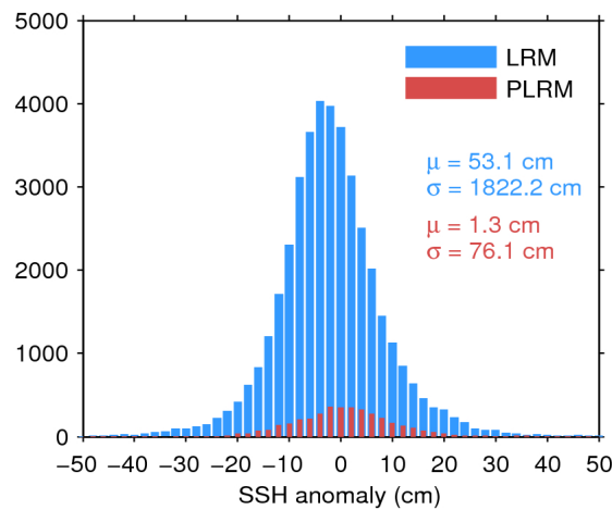
Figure 7. Histogram of flag-valid SSH anomaly over oceans and lakes for LRM (blue) and PLRM (red) for 19/11/2016. The mean ( \mu ) and standard deviation ( \sigma ) are also shown. Note that values outside [-50\ 50] cm are excluded from the histogram for the sake of readability but not from the computation of \mu and \sigma .
