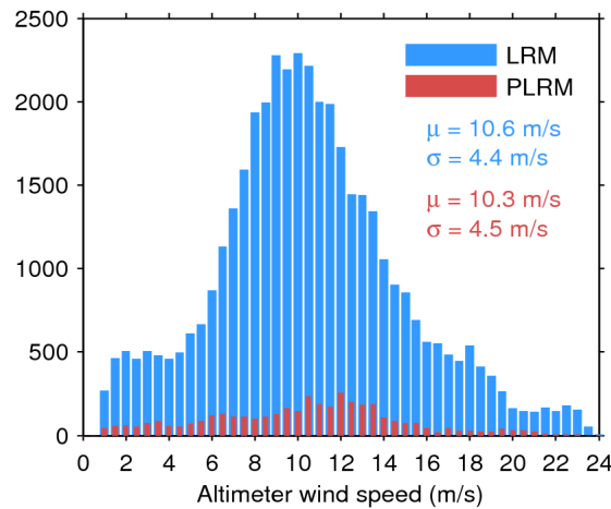
Figure 33. Histogram of flag-valid wind over oceans and lakes for LRM (blue) and PLRM (red) for 19/11/2016. The mean ( \mu ) and standard deviation ( \sigma ) are also shown. Note that values larger than 24 m/s are excluded from the histogram for the sake of readability but not from the computation of \mu and \sigma .
