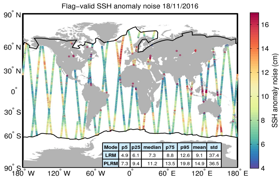
Figure 8. Geographical distribution of flag-valid 20-Hz SSH anomaly measurement noise over oceans and lakes for 18/11/2016. The statistical values shown in the table refer to the SSH anomaly noise and are calculated separately for LRM and PLRM regions. Measurements taken over polar polygons have been excluded from the computation of the statistical values. The black lines mark the outer limit of the Arctic and Antarctic polar polygons.
