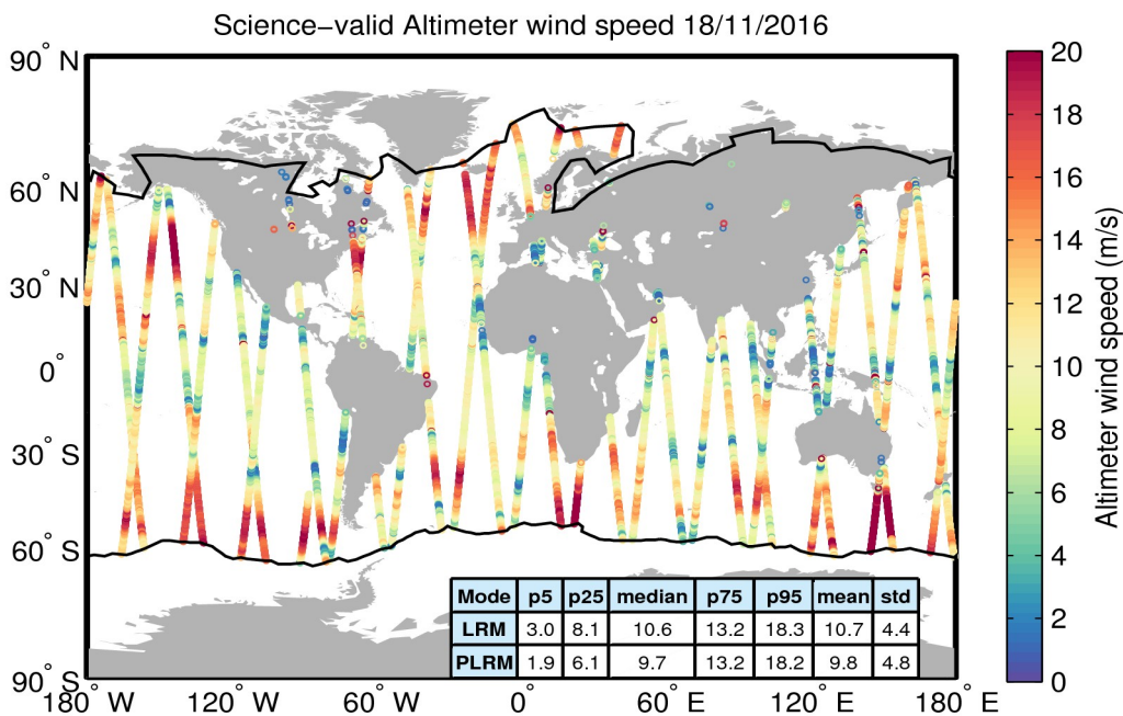
Figure 34. Geographical distribution of science-valid wind data over oceans and lakes for 18/11/2016. The statistical values shown in the table refer to the wind in m/s and are calculated separately for LRM and PLRM regions. The black lines mark the outer limit of the Arctic and Antarctic polar polygons. Gray circles denote records that have been rejected based on the editing criteria described in Table 5.
