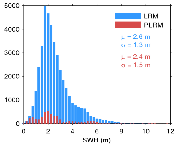
Figure 17. Histogram of flag-valid SWH over oceans and lakes for LRM (blue) and PLRM (red) for 18/11/2016. The mean ( \mu ) and standard deviation ( \sigma ) are also shown. Note that values larger than 12 m are excluded from the histogram for the sake of readability but not from the computation of \mu and \sigma .
