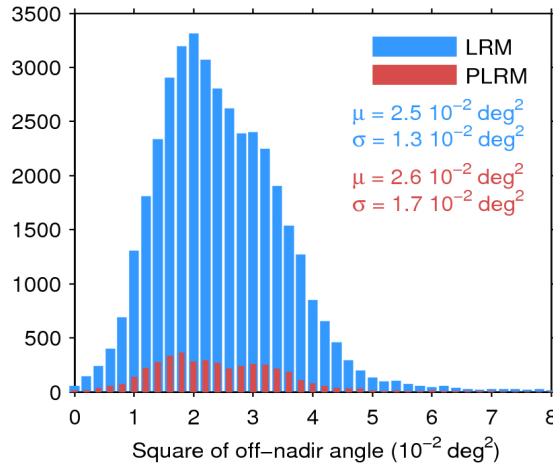
Figure 39. Histogram of flag-valid mispointing over oceans and lakes for LRM (blue) and PLRM (red) for 18/11/2016. Only positive values have been considered. The mean ( \mu ) and standard deviation ( \sigma ) are also shown. Note that values larger than 8 \cdot 10^{-2} \text{ deg}^2 are excluded from the histogram for the sake of readability but not from the computation of \mu and \sigma .
