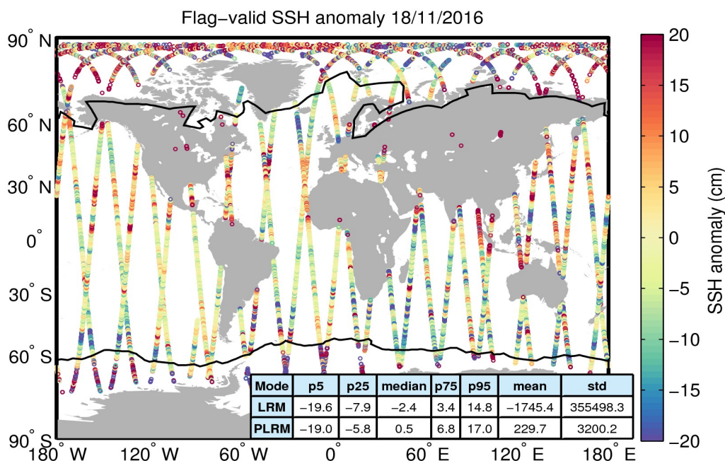
Figure 5. Geographical distribution of flag-valid 1-Hz SSH anomaly data over oceans and lakes for 18/11/2016. The statistical values shown in the table refer to the SSH anomaly in cm and are calculated separately for LRM and PLRM regions. Measurements taken over polar polygons have been excluded from the computation of the statistical values. The black lines mark the outer limit of the Arctic and Antarctic polar polygons.
