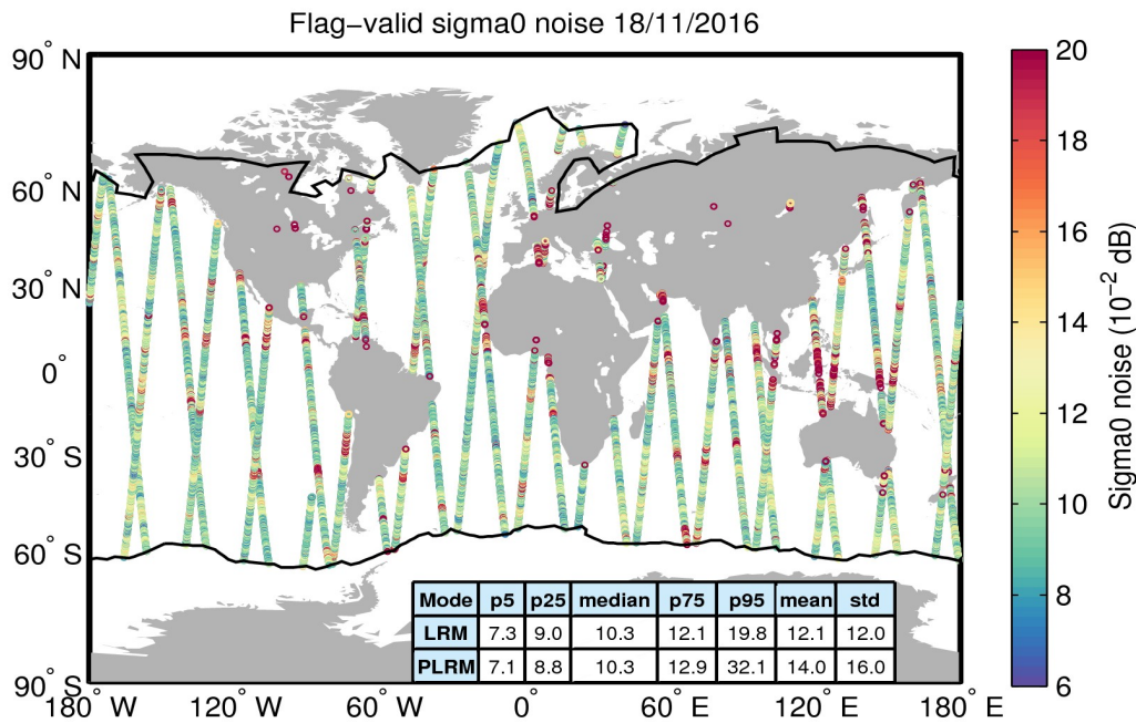
Figure 26. Geographical distribution of flag-valid 20-Hz sigma0 measurement noise over oceans and lakes for 18/11/2016. The statistical values shown in the table refer to the sigma0 noise and are calculated separately for LRM and PLRM regions. Measurements taken over polar polygons have been excluded from the computation of the statistical values. The black lines mark the outer limit of the Arctic and Antarctic polar polygons.
