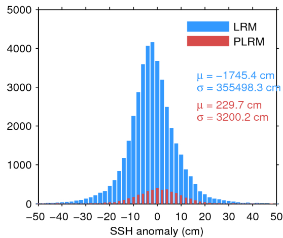
Figure 7. Histogram of flag-valid SSH anomaly over oceans and lakes for LRM (blue) and PLRM (red) for 18/11/2016. The mean ( \mu ) and standard deviation ( \sigma ) are also shown. Note that values outside [-50\ 50] cm are excluded from the histogram for the sake of readability but not from the computation of \mu and \sigma .
