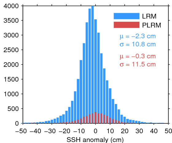
Figure 11. Histogram of science-valid SSH anomaly over oceans and lakes for LRM (blue) and PLRM (red) for 18/11/2016. The mean ( \mu ) and standard deviation ( \sigma ) are also shown. Note that values outside [-50 50] cm are excluded from the histogram for the sake of readability but not from the computation of \mu and \sigma .
