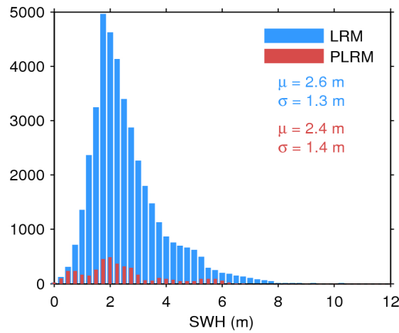
Figure 20. Histogram of science-valid SWH over oceans and lakes for LRM (blue) and PLRM (red) for 18/11/2016. The mean ( \mu ) and standard deviation ( \sigma ) are also shown. Note that values larger than 12 m are excluded from the histogram for the sake of readability but not from the computation of \mu and \sigma .
