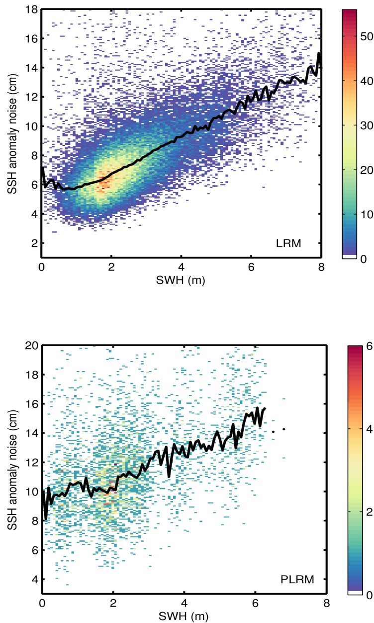
Figure 9. 2D histogram showing flag-valid SSH anomaly noise as a function of SWH for LRM (top) and PLRM (bottom) for 18/11/2016. The black line denotes the median SSH anomaly noise as a function of SWH.
