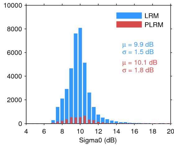
Figure 28. Histogram of science-valid sigma0 over oceans and lakes for LRM (blue) and PLRM (red) for 18/11/2016. The mean ( \mu ) and standard deviation ( \sigma ) are also shown. Note that values outside [4 20] dB are excluded from the histogram for the sake of readability but not from the computation of \mu and \sigma .
