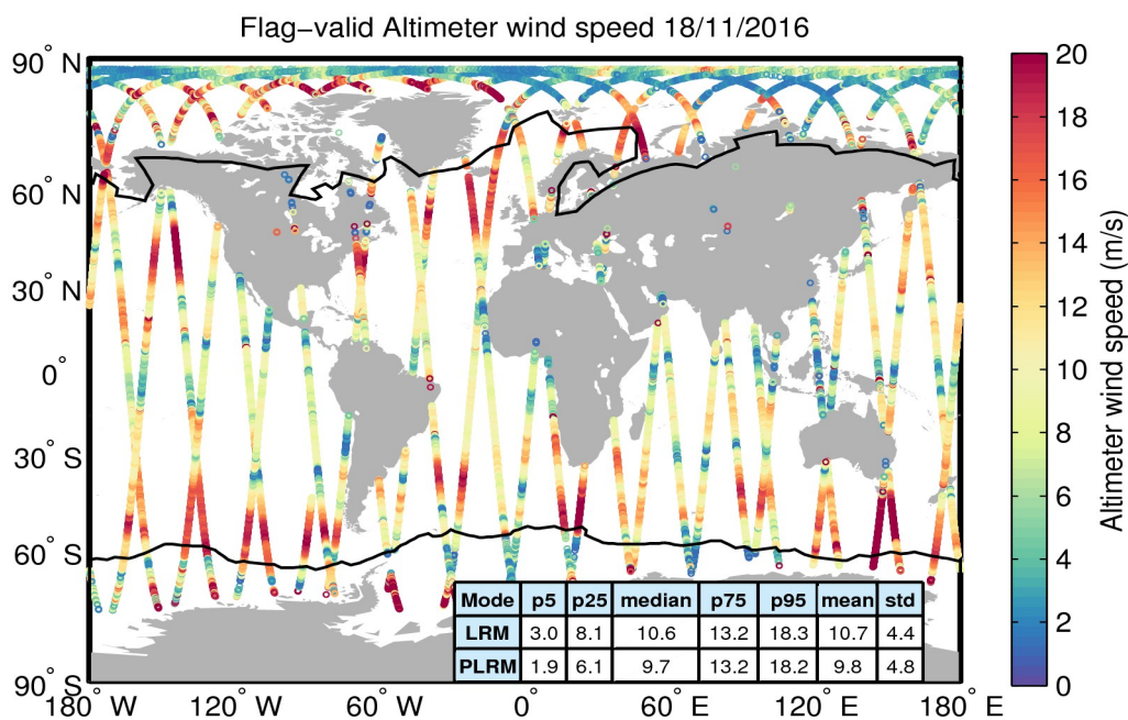
Figure 31. Geographical distribution of flag-valid wind data over oceans and lakes for 18/11/2016. The statistical values shown in the table refer to the wind in m/s and are calculated separately for LRM and PLRM regions. Measurements taken over polar polygons have been excluded from the computation of the statistical values. The black lines mark the outer limit of the Arctic and Antarctic polar polygons.
