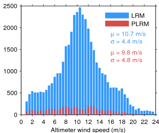
Figure 35. Histogram of science-valid wind over oceans and lakes for LRM (blue) and PLRM (red) for 18/11/2016. The mean ( \mu ) and standard deviation ( \sigma ) are also shown. Note that values larger than 24 m/s are excluded from the histogram for the sake of readability but not from the computation of \mu and \sigma .
