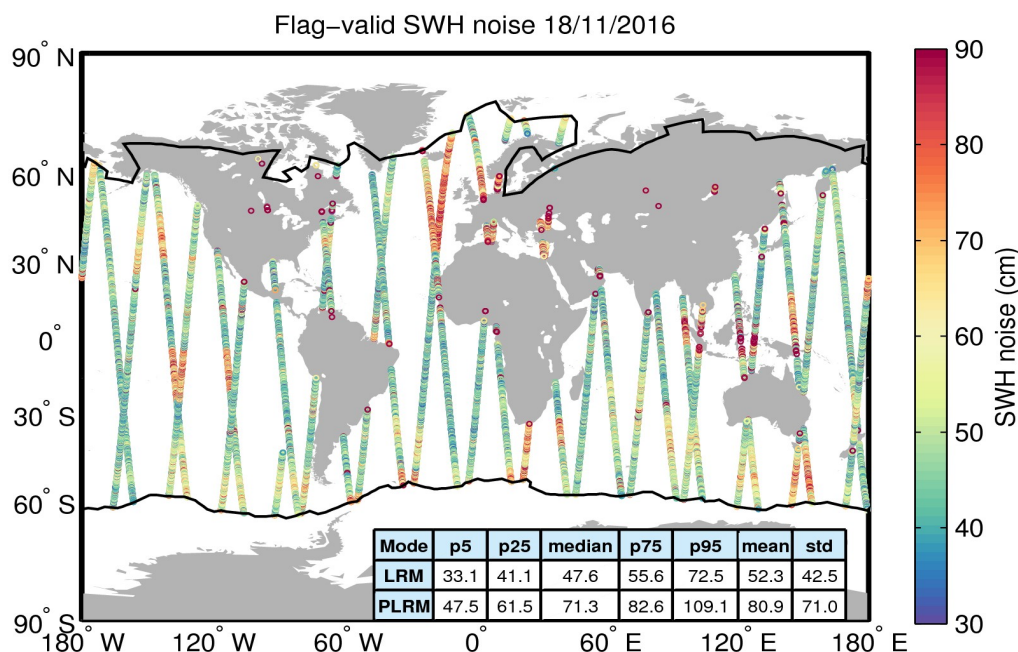
Figure 18. Geographical distribution of flag-valid 20-Hz SWH measurement noise over oceans and lakes for 18/11/2016. The statistical values shown in the table refer to the SWH noise and are calculated separately for LRM and PLRM regions. Measurements taken over polar polygons have been excluded from the computation of the statistical values. The black lines mark the outer limit of the Arctic and Antarctic polar polygons.
