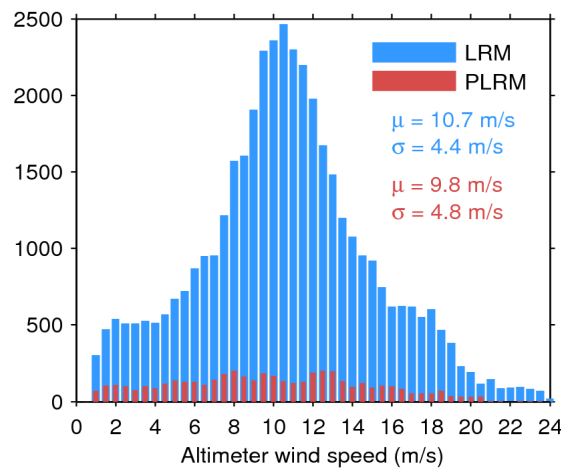
Figure 33. Histogram of flag-valid wind over oceans and lakes for LRM (blue) and PLRM (red) for 18/11/2016. The mean ( \mu ) and standard deviation ( \sigma ) are also shown. Note that values larger than 24 m/s are excluded from the histogram for the sake of readability but not from the computation of \mu and \sigma .
