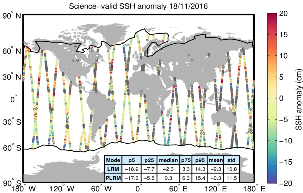
Figure 10. Geographical distribution of science-valid SSH anomaly data over oceans and lakes for 18/11/2016. The statistical values shown in the table refer to the SSH anomaly in cm and are calculated separately for LRM and PLRM regions. The black lines mark the outer limit of the Arctic and Antarctic polar polygons. Gray circles denote records that have been rejected based on the editing criteria described in Table 2.
