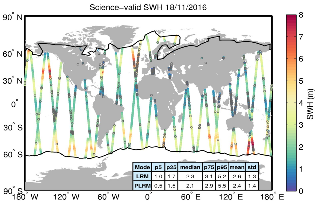
Figure 19. Geographical distribution of science-valid SWH data over oceans and lakes for 18/11/2016. The statistical values shown in the table refer to the SWH in m and are calculated separately for LRM and PLRM regions. The black lines mark the outer limit of the Arctic and Antarctic polar polygons. Gray circles denote records that have been rejected based on the editing criteria described in Table 3.
