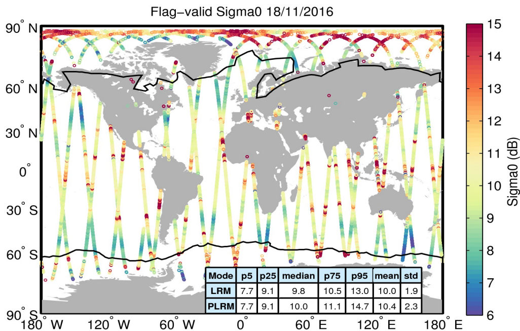
Figure 23. Geographical distribution of flag-valid sigma0 data over oceans and lakes for 18/11/2016. The statistical values shown in the table refer to the sigma0 in dB and are calculated separately for LRM and PLRM regions. Measurements taken over polar polygons have been excluded from the computation of the statistical values. The black lines mark the outer limit of the Arctic and Antarctic polar polygons.
