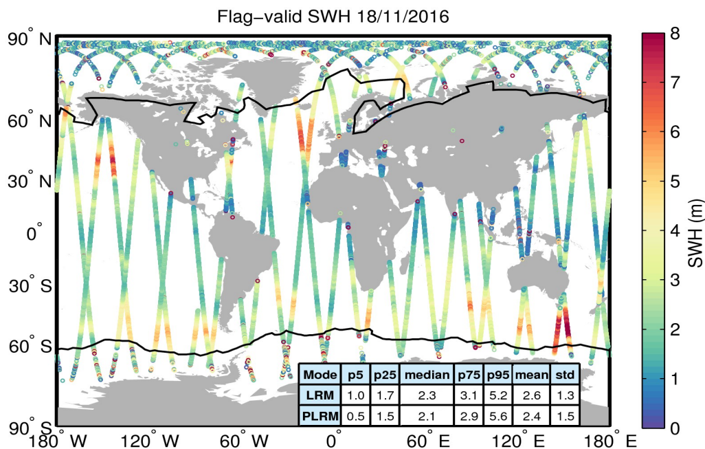
Figure 15. Geographical distribution of flag-valid SWH data over oceans and lakes for 18/11/2016. The statistical values shown in the table refer to the SWH in m and are calculated separately for LRM and PLRM regions. Measurements taken over polar polygons have been excluded from the computation of the statistical values. The black lines mark the outer limit of the Arctic and Antarctic polar polygons.
