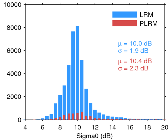
Figure 25. Histogram of flag-valid sigma0 over oceans and lakes for LRM (blue) and PLRM (red) for 18/11/2016. The mean ( \mu ) and standard deviation ( \sigma ) are also shown. Note that values outside [4 20] dB are excluded from the histogram for the sake of readability but not from the computation of \mu and \sigma .
