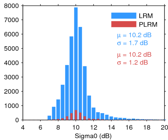
Figure 28. Histogram of science-valid sigma0 over oceans and lakes for LRM (blue) and PLRM (red) for 11/11/2016. The mean ( \mu ) and standard deviation ( \sigma ) are also shown. Note that values outside [4 20] dB are excluded from the histogram for the sake of readability but not from the computation of \mu and \sigma .
