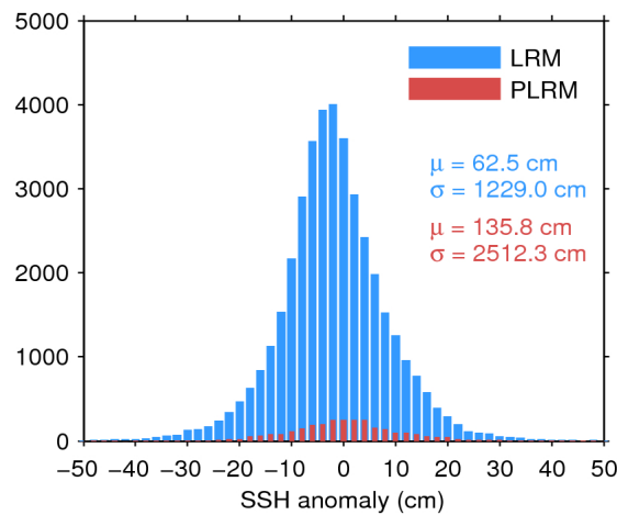
Figure 7. Histogram of flag-valid SSH anomaly over oceans and lakes for LRM (blue) and PLRM (red) for 11/11/2016. The mean ( \mu ) and standard deviation ( \sigma ) are also shown. Note that values outside [-50\ 50] cm are excluded from the histogram for the sake of readability but not from the computation of \mu and \sigma .
