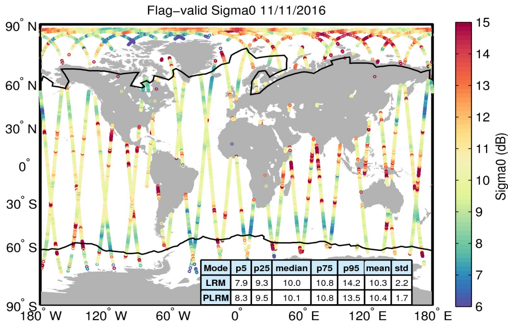
Figure 23. Geographical distribution of flag-valid sigma0 data over oceans and lakes for 11/11/2016. The statistical values shown in the table refer to the sigma0 in dB and are calculated separately for LRM and PLRM regions. Measurements taken over polar polygons have been excluded from the computation of the statistical values. The black lines mark the outer limit of the Arctic and Antarctic polar polygons.
