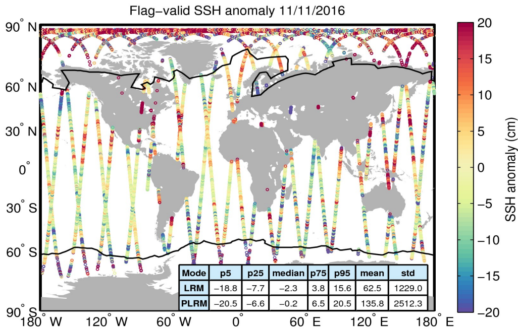
Figure 5. Geographical distribution of flag-valid 1-Hz SSH anomaly data over oceans and lakes for 11/11/2016. The statistical values shown in the table refer to the SSH anomaly in cm and are calculated separately for LRM and PLRM regions. Measurements taken over polar polygons have been excluded from the computation of the statistical values. The black lines mark the outer limit of the Arctic and Antarctic polar polygons.
