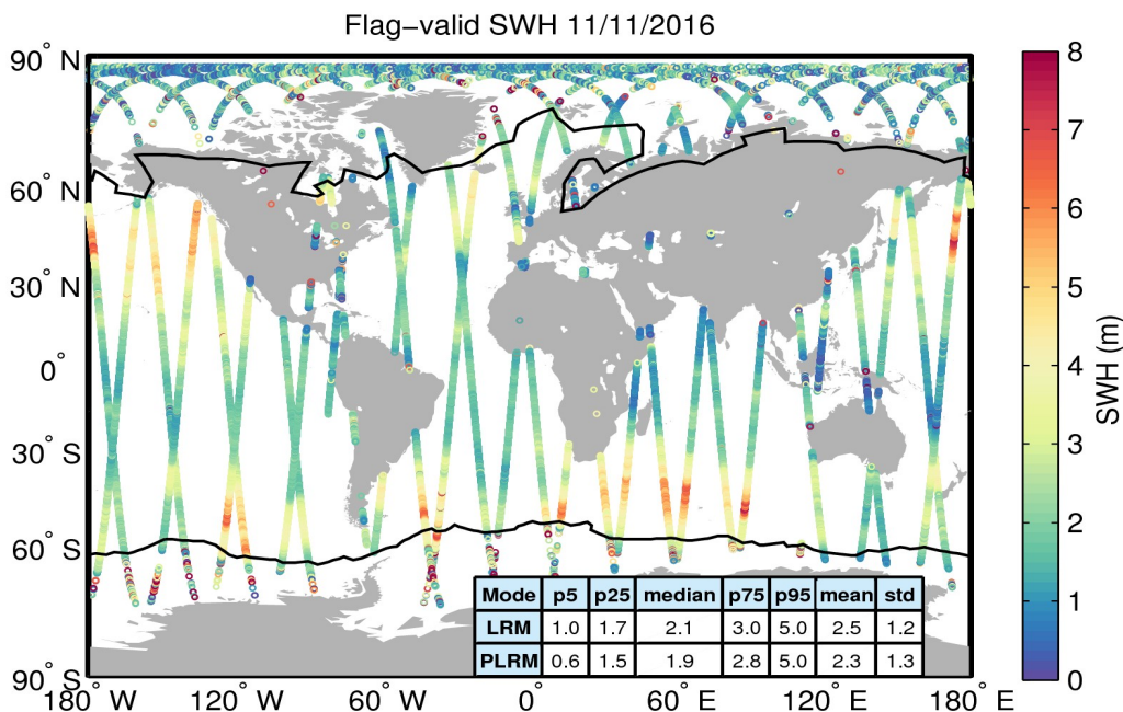
Figure 15. Geographical distribution of flag-valid SWH data over oceans and lakes for 11/11/2016. The statistical values shown in the table refer to the SWH in m and are calculated separately for LRM and PLRM regions. Measurements taken over polar polygons have been excluded from the computation of the statistical values. The black lines mark the outer limit of the Arctic and Antarctic polar polygons.
