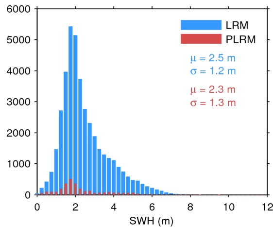
Figure 17. Histogram of flag-valid SWH over oceans and lakes for LRM (blue) and PLRM (red) for 11/11/2016. The mean ( \mu ) and standard deviation ( \sigma ) are also shown. Note that values larger than 12 m are excluded from the histogram for the sake of readability but not from the computation of \mu and \sigma .
