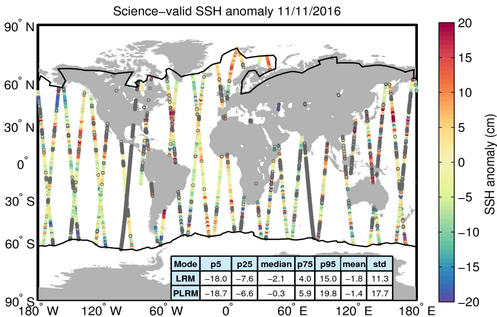
Figure 10. Geographical distribution of science-valid SSH anomaly data over oceans and lakes for 11/11/2016. The statistical values shown in the table refer to the SSH anomaly in cm and are calculated separately for LRM and PLRM regions. The black lines mark the outer limit of the Arctic and Antarctic polar polygons. Gray circles denote records that have been rejected based on the editing criteria described in Table 2.
