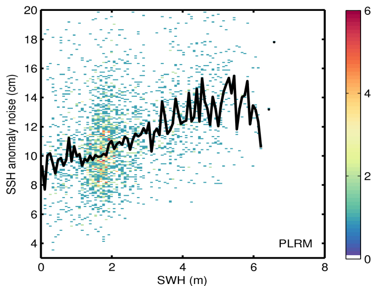
Figure 9. 2D histogram showing flag-valid SSH anomaly noise as a function of SWH for LRM (top) and PLRM (bottom) for 11/11/2016. The black line denotes the median SSH anomaly noise as a function of SWH.
