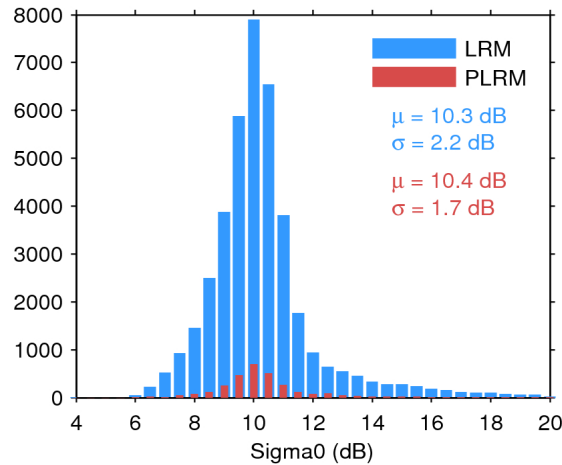
Figure 25. Histogram of flag-valid sigma0 over oceans and lakes for LRM (blue) and PLRM (red) for 11/11/2016. The mean ( \mu ) and standard deviation ( \sigma ) are also shown. Note that values outside [4 20] dB are excluded from the histogram for the sake of readability but not from the computation of \mu and \sigma .
