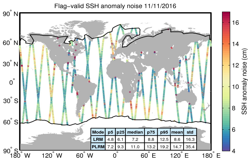
Figure 8. Geographical distribution of flag-valid 20-Hz SSH anomaly measurement noise over oceans and lakes for 11/11/2016. The statistical values shown in the table refer to the SSH anomaly noise and are calculated separately for LRM and PLRM regions. Measurements taken over polar polygons have been excluded from the computation of the statistical values. The black lines mark the outer limit of the Arctic and Antarctic polar polygons.
