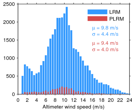
Figure 33. Histogram of flag-valid wind over oceans and lakes for LRM (blue) and PLRM (red) for 11/11/2016. The mean ( \mu ) and standard deviation ( \sigma ) are also shown. Note that values larger than 24 m/s are excluded from the histogram for the sake of readability but not from the computation of \mu and \sigma .
