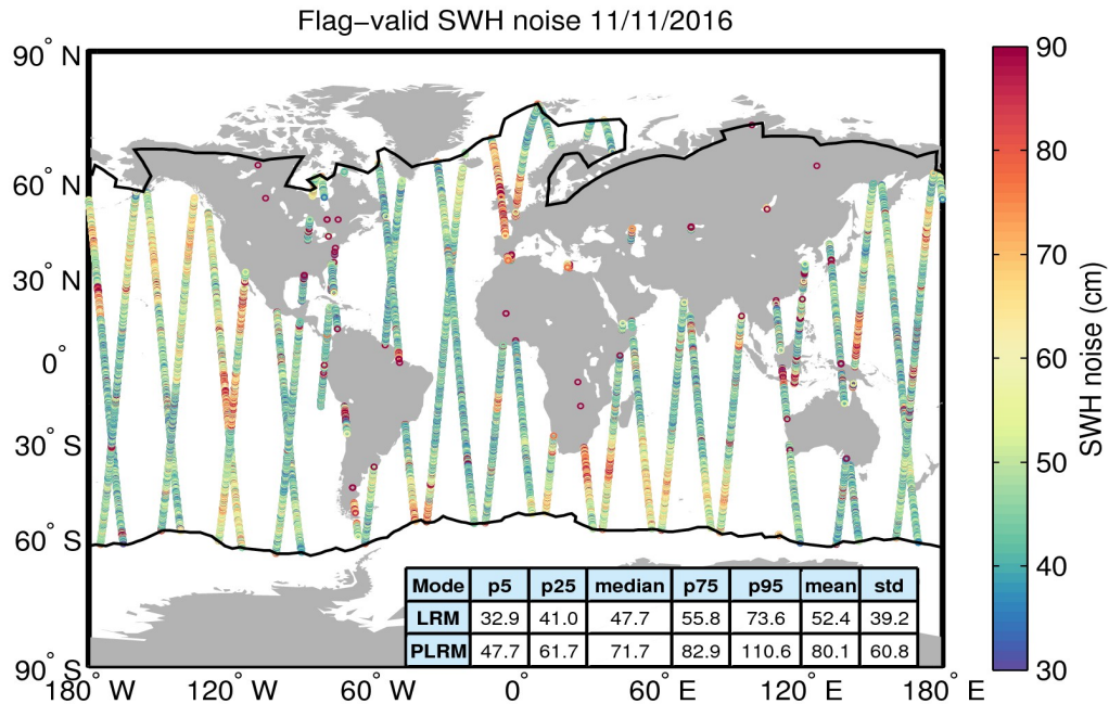
Figure 18. Geographical distribution of flag-valid 20-Hz SWH measurement noise over oceans and lakes for 11/11/2016. The statistical values shown in the table refer to the SWH noise and are calculated separately for LRM and PLRM regions. Measurements taken over polar polygons have been excluded from the computation of the statistical values. The black lines mark the outer limit of the Arctic and Antarctic polar polygons.
