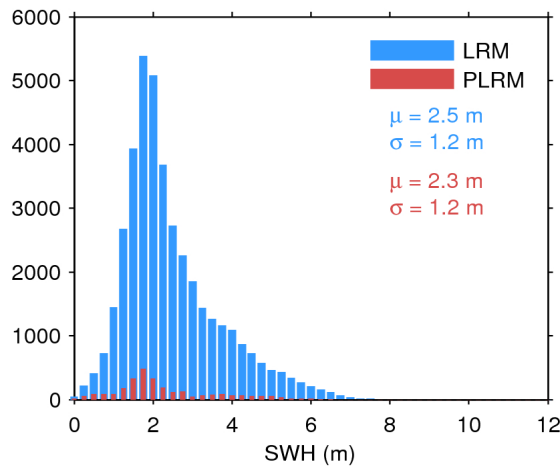
Figure 20. Histogram of science-valid SWH over oceans and lakes for LRM (blue) and PLRM (red) for 11/11/2016. The mean ( \mu ) and standard deviation ( \sigma ) are also shown. Note that values larger than 12 m are excluded from the histogram for the sake of readability but not from the computation of \mu and \sigma .
