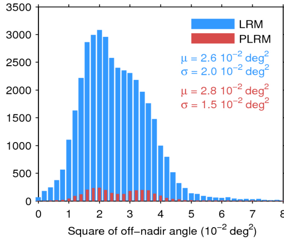
Figure 39. Histogram of flag-valid mispointing over oceans and lakes for LRM (blue) and PLRM (red) for 11/11/2016. Only positive values have been considered. The mean ( \mu ) and standard deviation ( \sigma ) are also shown. Note that values larger than 8 \cdot 10^{-2} \text{ deg}^2 are excluded from the histogram for the sake of readability but not from the computation of \mu and \sigma .
