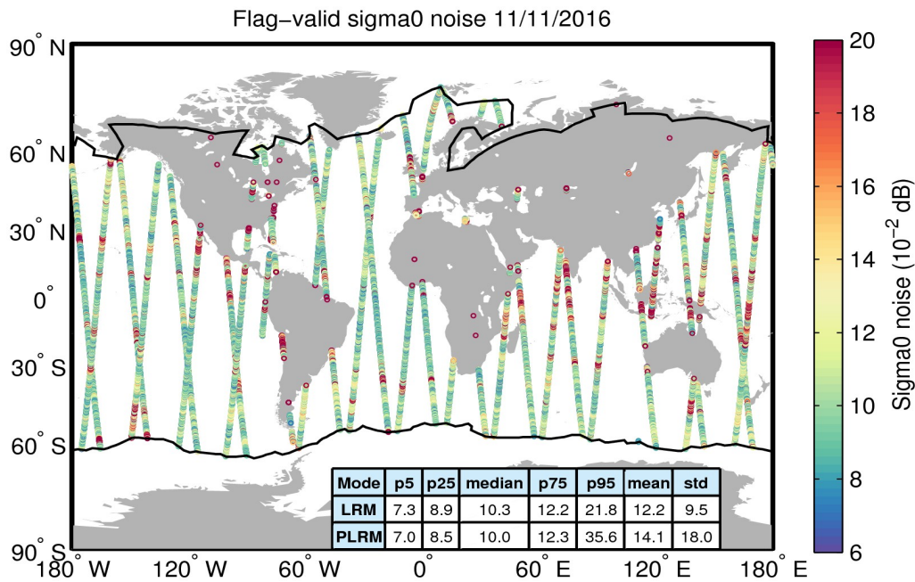
Figure 26. Geographical distribution of flag-valid 20-Hz sigma0 measurement noise over oceans and lakes for 11/11/2016. The statistical values shown in the table refer to the sigma0 noise and are calculated separately for LRM and PLRM regions. Measurements taken over polar polygons have been excluded from the computation of the statistical values. The black lines mark the outer limit of the Arctic and Antarctic polar polygons.
