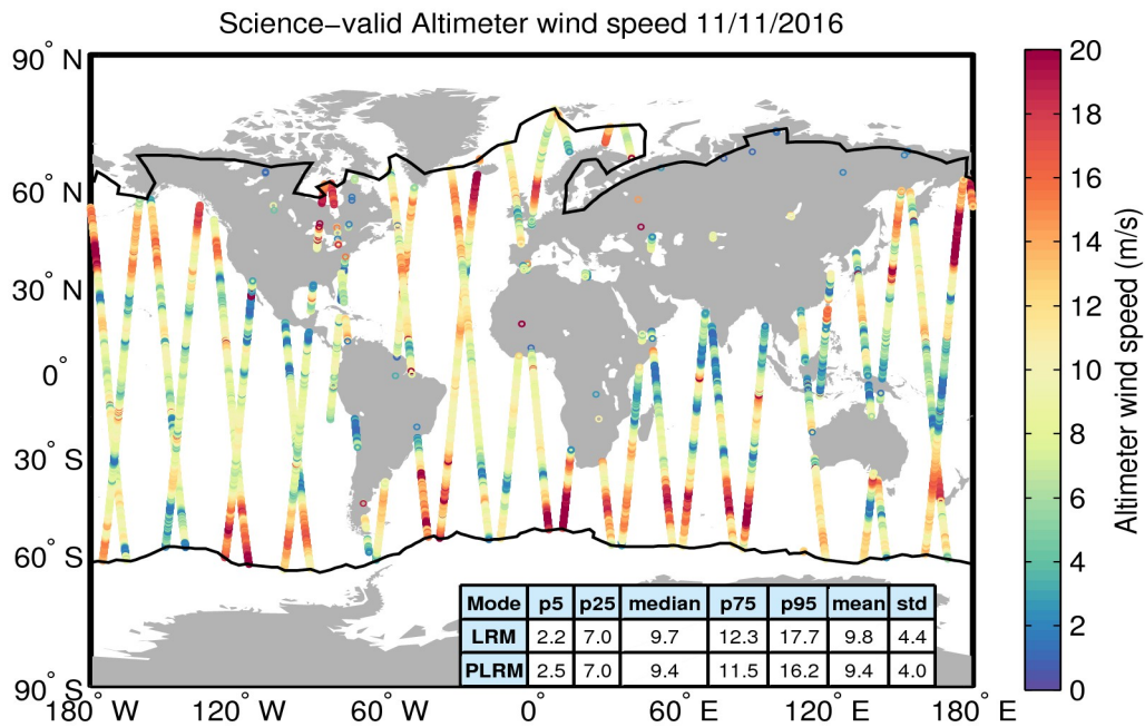
Figure 34. Geographical distribution of science-valid wind data over oceans and lakes for 11/11/2016. The statistical values shown in the table refer to the wind in m/s and are calculated separately for LRM and PLRM regions. The black lines mark the outer limit of the Arctic and Antarctic polar polygons. Gray circles denote records that have been rejected based on the editing criteria described in Table 5.
