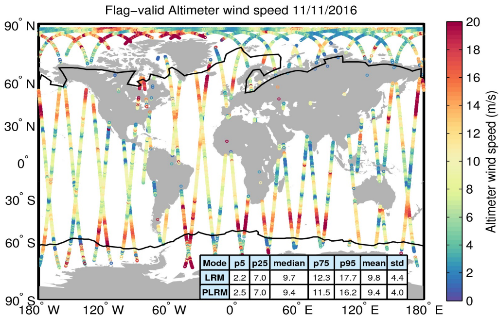
Figure 31. Geographical distribution of flag-valid wind data over oceans and lakes for 11/11/2016. The statistical values shown in the table refer to the wind in m/s and are calculated separately for LRM and PLRM regions. Measurements taken over polar polygons have been excluded from the computation of the statistical values. The black lines mark the outer limit of the Arctic and Antarctic polar polygons.
