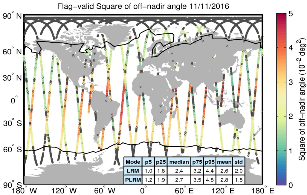
Figure 37. Geographical distribution of flag-valid mispointing data over oceans and lakes for 11/11/2016. The statistical values shown in the table refer to the mispointing in 10^{-2} \text{ deg}^2 and are calculated separately for LRM and PLRM regions. Measurements taken over polar polygons have been excluded from the computation of the statistical values. The black lines mark the outer limit of the Arctic and Antarctic polar polygons. Gray circles denote negative values.
