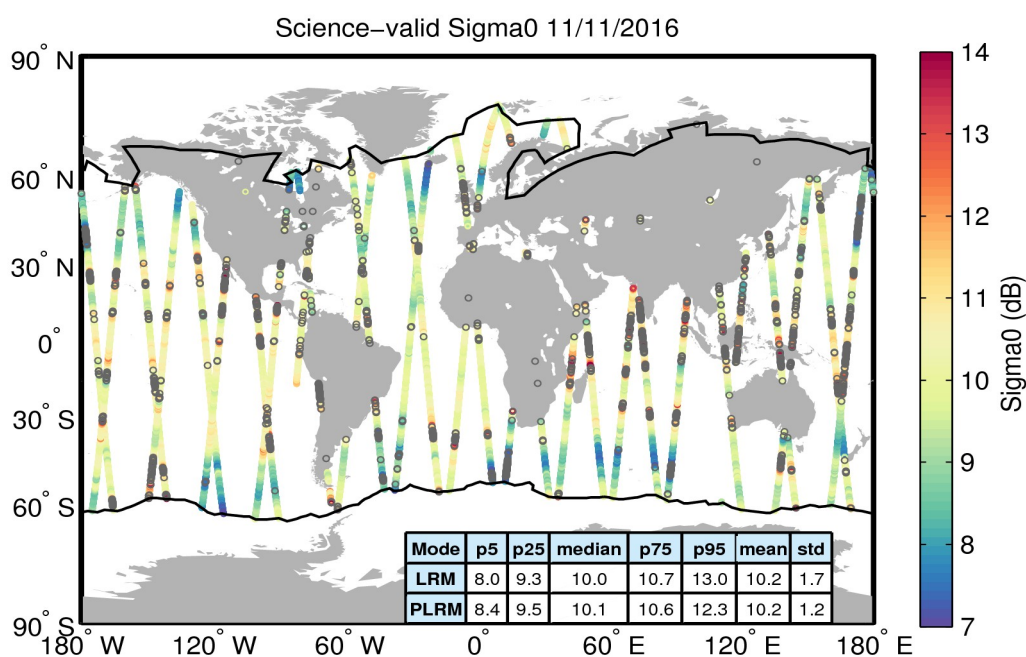
Figure 27. Geographical distribution of science-valid sigma0 data over oceans and lakes for 11/11/2016. The statistical values shown in the table refer to the sigma0 in dB and are calculated separately for LRM and PLRM regions. The black lines mark the outer limit of the Arctic and Antarctic polar polygons. Gray circles denote records that have been rejected based on the editing criteria described in Table 4.
