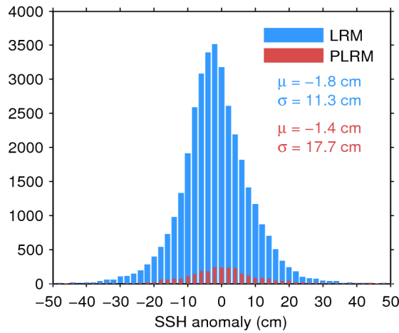
Figure 11. Histogram of science-valid SSH anomaly over oceans and lakes for LRM (blue) and PLRM (red) for 11/11/2016. The mean ( \mu ) and standard deviation ( \sigma ) are also shown. Note that values outside [-50 50] cm are excluded from the histogram for the sake of readability but not from the computation of \mu and \sigma .
