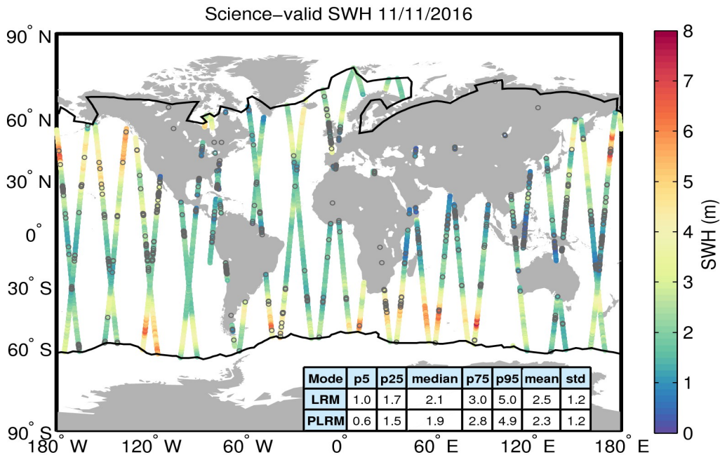
Figure 19. Geographical distribution of science-valid SWH data over oceans and lakes for 11/11/2016. The statistical values shown in the table refer to the SWH in m and are calculated separately for LRM and PLRM regions. The black lines mark the outer limit of the Arctic and Antarctic polar polygons. Gray circles denote records that have been rejected based on the editing criteria described in Table 3.
