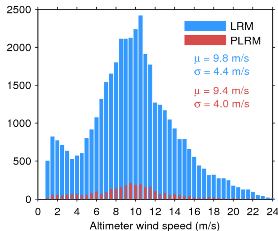
Figure 35. Histogram of science-valid wind over oceans and lakes for LRM (blue) and PLRM (red) for 11/11/2016. The mean ( \mu ) and standard deviation ( \sigma ) are also shown. Note that values larger than 24 m/s are excluded from the histogram for the sake of readability but not from the computation of \mu and \sigma .
