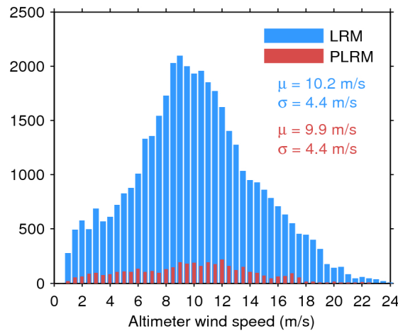
Figure 33. Histogram of flag-valid wind over oceans and lakes for LRM (blue) and PLRM (red) for 05/11/2016. The mean ( \mu ) and standard deviation ( \sigma ) are also shown. Note that values larger than 24 m/s are excluded from the histogram for the sake of readability but not from the computation of \mu and \sigma .
