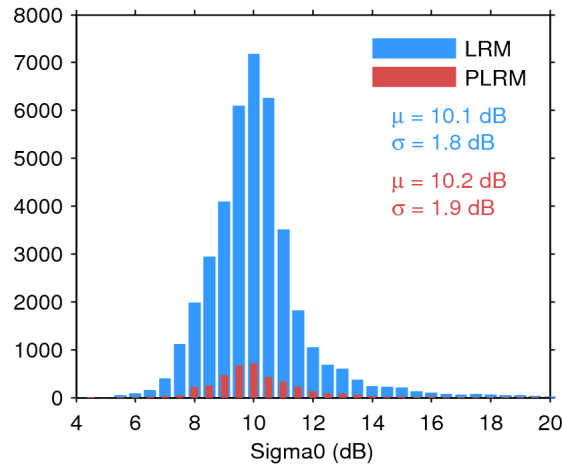
Figure 25. Histogram of flag-valid sigma0 over oceans and lakes for LRM (blue) and PLRM (red) for 05/11/2016. The mean ( \mu ) and standard deviation ( \sigma ) are also shown. Note that values outside [4 20] dB are excluded from the histogram for the sake of readability but not from the computation of \mu and \sigma .
