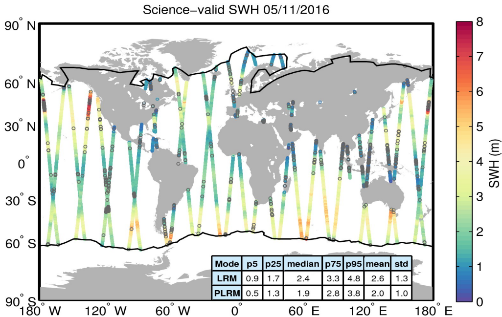
Figure 19. Geographical distribution of science-valid SWH data over oceans and lakes for 05/11/2016. The statistical values shown in the table refer to the SWH in m and are calculated separately for LRM and PLRM regions. The black lines mark the outer limit of the Arctic and Antarctic polar polygons. Gray circles denote records that have been rejected based on the editing criteria described in Table 3.
