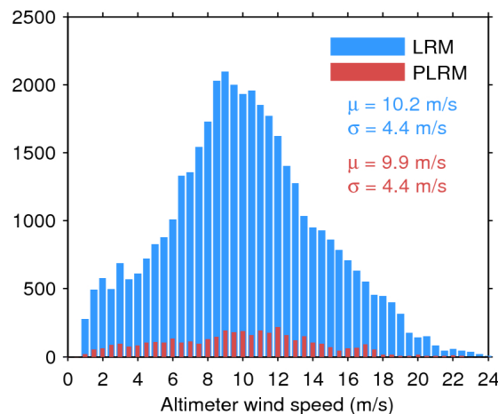
Figure 35. Histogram of science-valid wind over oceans and lakes for LRM (blue) and PLRM (red) for 05/11/2016. The mean ( \mu ) and standard deviation ( \sigma ) are also shown. Note that values larger than 24 m/s are excluded from the histogram for the sake of readability but not from the computation of \mu and \sigma .
