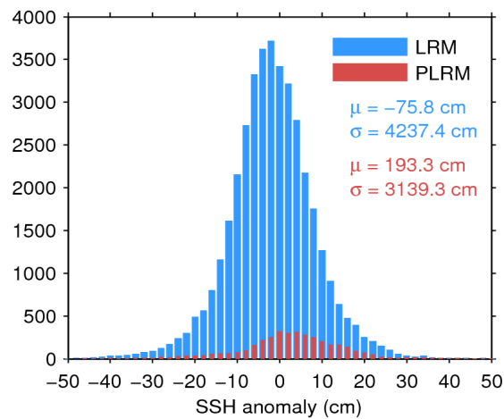
Figure 7. Histogram of flag-valid SSH anomaly over oceans and lakes for LRM (blue) and PLRM (red) for 05/11/2016. The mean ( \mu ) and standard deviation ( \sigma ) are also shown. Note that values outside [-50 \ 50] cm are excluded from the histogram for the sake of readability but not from the computation of \mu and \sigma .
