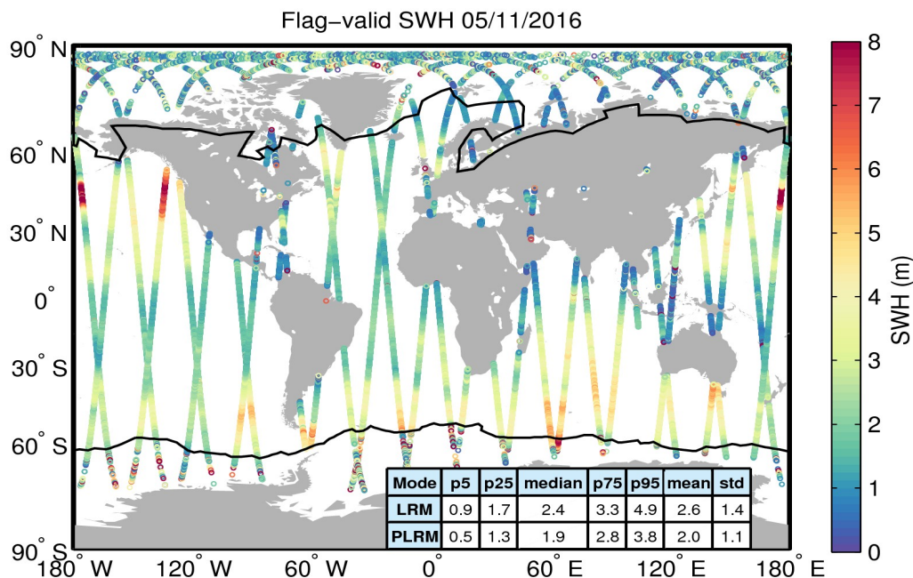
Figure 15. Geographical distribution of flag-valid SWH data over oceans and lakes for 05/11/2016. The statistical values shown in the table refer to the SWH in m and are calculated separately for LRM and PLRM regions. Measurements taken over polar polygons have been excluded from the computation of the statistical values. The black lines mark the outer limit of the Arctic and Antarctic polar polygons.
