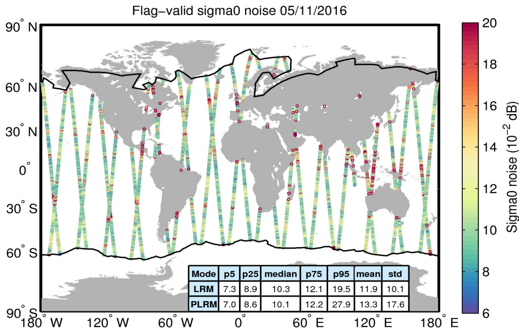
Figure 26. Geographical distribution of flag-valid 20-Hz sigma0 measurement noise over oceans and lakes for 05/11/2016. The statistical values shown in the table refer to the sigma0 noise and are calculated separately for LRM and PLRM regions. Measurements taken over polar polygons have been excluded from the computation of the statistical values. The black lines mark the outer limit of the Arctic and Antarctic polar polygons.
