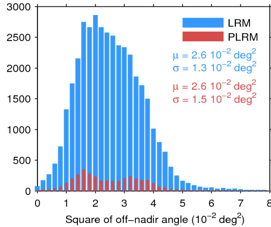
Figure 39. Histogram of flag-valid mispointing over oceans and lakes for LRM (blue) and PLRM (red) for 05/11/2016. Only positive values have been considered. The mean ( \mu ) and standard deviation ( \sigma ) are also shown. Note that values larger than 8 \cdot 10^{-2} \text{ deg}^2 are excluded from the histogram for the sake of readability but not from the computation of \mu and \sigma .
