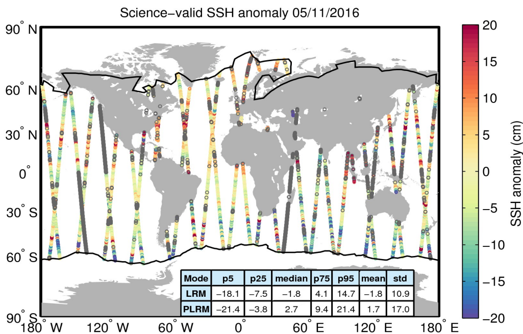
Figure 10. Geographical distribution of science-valid SSH anomaly data over oceans and lakes for 05/11/2016. The statistical values shown in the table refer to the SSH anomaly in cm and are calculated separately for LRM and PLRM regions. The black lines mark the outer limit of the Arctic and Antarctic polar polygons. Gray circles denote records that have been rejected based on the editing criteria described in Table 2.
