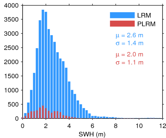
Figure 17. Histogram of flag-valid SWH over oceans and lakes for LRM (blue) and PLRM (red) for 05/11/2016. The mean ( \mu ) and standard deviation ( \sigma ) are also shown. Note that values larger than 12 m are excluded from the histogram for the sake of readability but not from the computation of \mu and \sigma .
