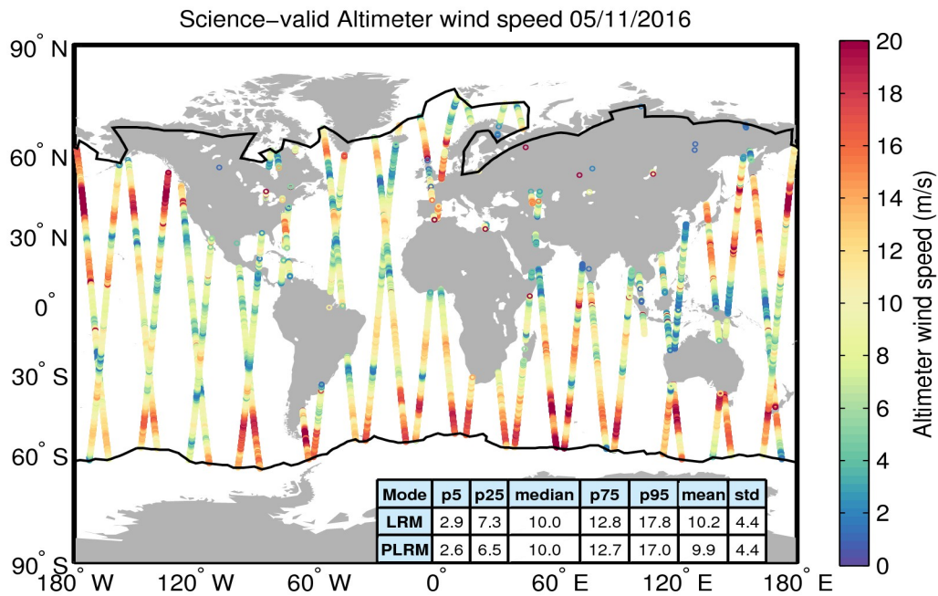
Figure 34. Geographical distribution of science-valid wind data over oceans and lakes for 05/11/2016. The statistical values shown in the table refer to the wind in m/s and are calculated separately for LRM and PLRM regions. The black lines mark the outer limit of the Arctic and Antarctic polar polygons. Gray circles denote records that have been rejected based on the editing criteria described in Table 5.
