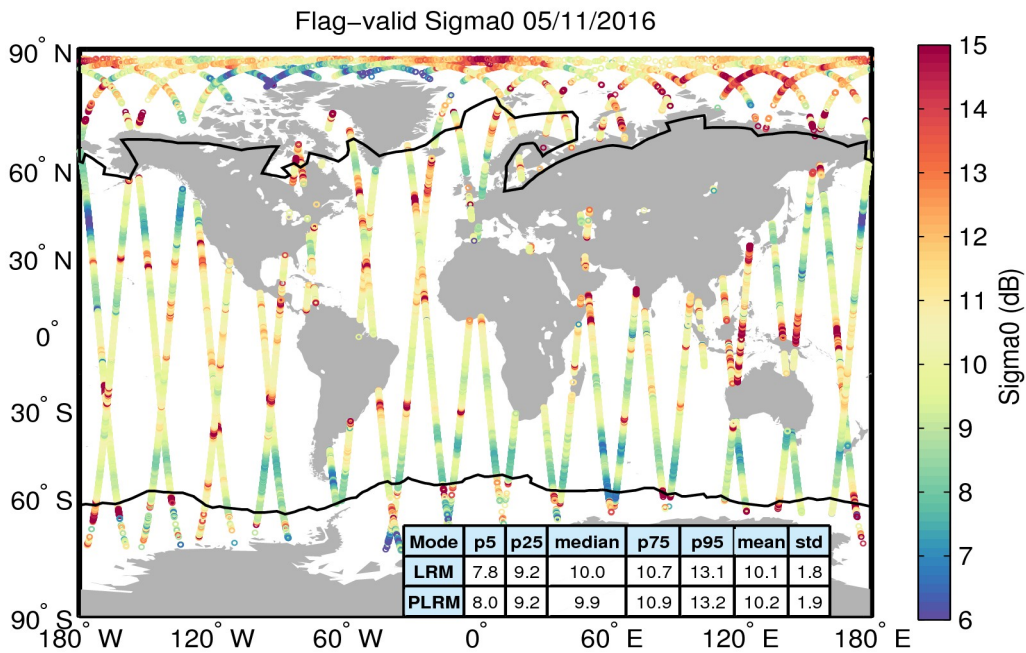
Figure 23. Geographical distribution of flag-valid sigma0 data over oceans and lakes for 05/11/2016. The statistical values shown in the table refer to the sigma0 in dB and are calculated separately for LRM and PLRM regions. Measurements taken over polar polygons have been excluded from the computation of the statistical values. The black lines mark the outer limit of the Arctic and Antarctic polar polygons.
