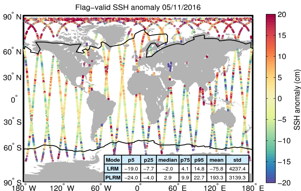
Figure 5. Geographical distribution of flag-valid 1-Hz SSH anomaly data over oceans and lakes for 05/11/2016. The statistical values shown in the table refer to the SSH anomaly in cm and are calculated separately for LRM and PLRM regions. Measurements taken over polar polygons have been excluded from the computation of the statistical values. The black lines mark the outer limit of the Arctic and Antarctic polar polygons.
