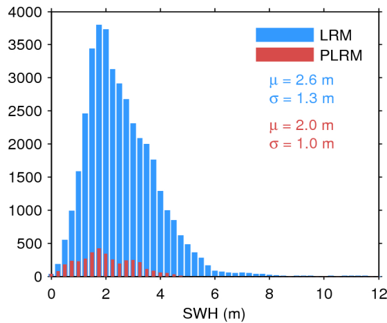
Figure 20. Histogram of science-valid SWH over oceans and lakes for LRM (blue) and PLRM (red) for 05/11/2016. The mean ( \mu ) and standard deviation ( \sigma ) are also shown. Note that values larger than 12 m are excluded from the histogram for the sake of readability but not from the computation of \mu and \sigma .
