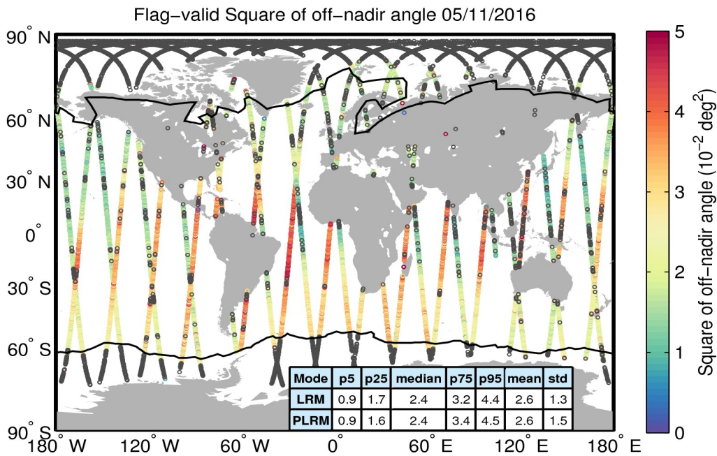
Figure 37. Geographical distribution of flag-valid mispointing data over oceans and lakes for 05/11/2016. The statistical values shown in the table refer to the mispointing in 10^{-2} \text{ deg}^2 and are calculated separately for LRM and PLRM regions. Measurements taken over polar polygons have been excluded from the computation of the statistical values. The black lines mark the outer limit of the Arctic and Antarctic polar polygons. Gray circles denote negative values.
