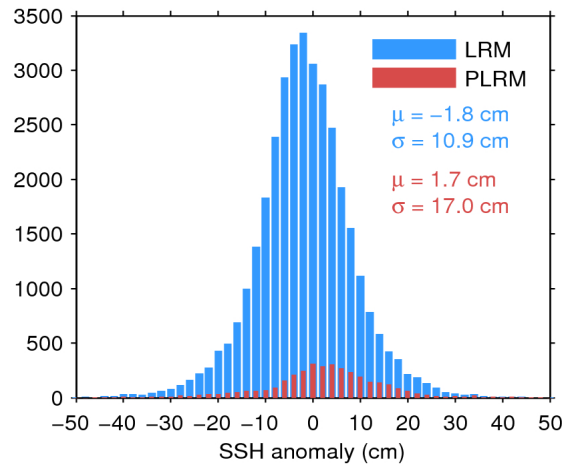
Figure 11. Histogram of science-valid SSH anomaly over oceans and lakes for LRM (blue) and PLRM (red) for 05/11/2016. The mean ( \mu ) and standard deviation ( \sigma ) are also shown. Note that values outside [-50 50] cm are excluded from the histogram for the sake of readability but not from the computation of \mu and \sigma .
