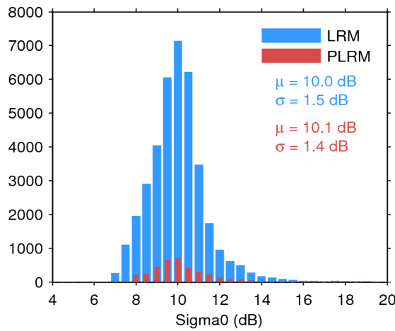
Figure 28. Histogram of science-valid sigma0 over oceans and lakes for LRM (blue) and PLRM (red) for 05/11/2016. The mean ( \mu ) and standard deviation ( \sigma ) are also shown. Note that values outside [4 20] dB are excluded from the histogram for the sake of readability but not from the computation of \mu and \sigma .
