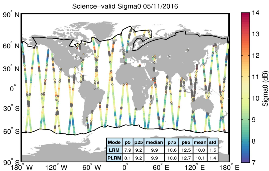
Figure 27. Geographical distribution of science-valid sigma0 data over oceans and lakes for 05/11/2016. The statistical values shown in the table refer to the sigma0 in dB and are calculated separately for LRM and PLRM regions. The black lines mark the outer limit of the Arctic and Antarctic polar polygons. Gray circles denote records that have been rejected based on the editing criteria described in Table 4.
