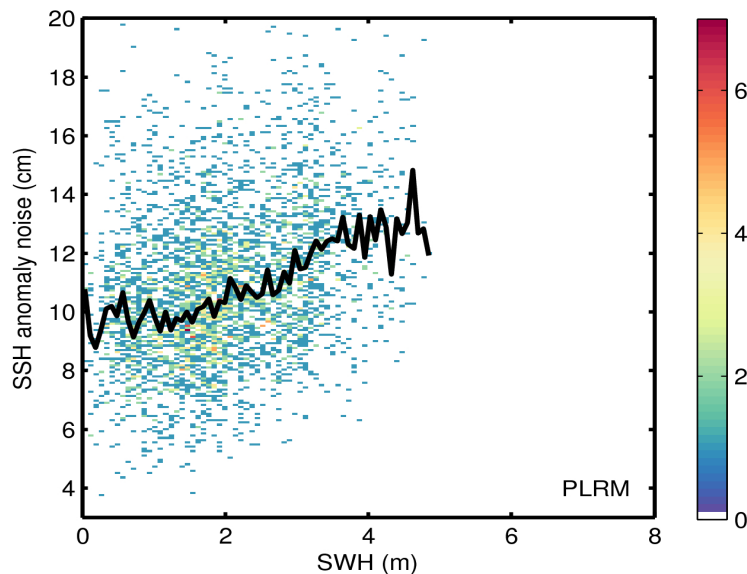
Figure 9. 2D histogram showing flag-valid SSH anomaly noise as a function of SWH for LRM (top) and PLRM (bottom) for 05/11/2016. The black line denotes the median SSH anomaly noise as a function of SWH.
