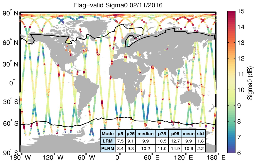
Figure 23. Geographical distribution of flag-valid sigma0 data over oceans and lakes for 02/11/2016. The statistical values shown in the table refer to the sigma0 in dB and are calculated separately for LRM and PLRM regions. Measurements taken over polar polygons have been excluded from the computation of the statistical values. The black lines mark the outer limit of the Arctic and Antarctic polar polygons.
