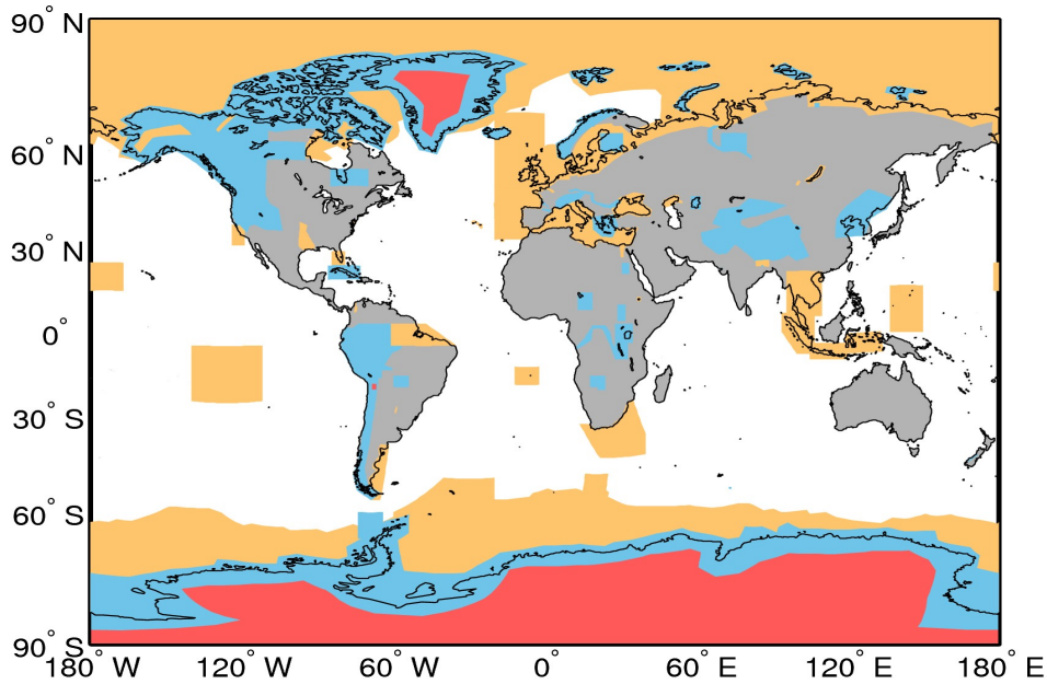
Figure A1. Extent of the regions defining the geographical mode mask for 02/11/2016. The regions where SAR, and SARIn are operated are denoted by the orange and blue polygons, respectively. LRM is operated over areas of the continental ice sheets (red polygons) and over oceans and land not covered by other modes.
