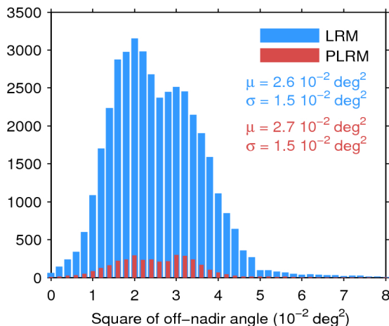
Figure 39. Histogram of flag-valid mispointing over oceans and lakes for LRM (blue) and PLRM (red) for 02/11/2016. Only positive values have been considered. The mean ( \mu ) and standard deviation ( \sigma ) are also shown. Note that values larger than 8 \cdot 10^{-2} \text{ deg}^2 are excluded from the histogram for the sake of readability but not from the computation of \mu and \sigma .
