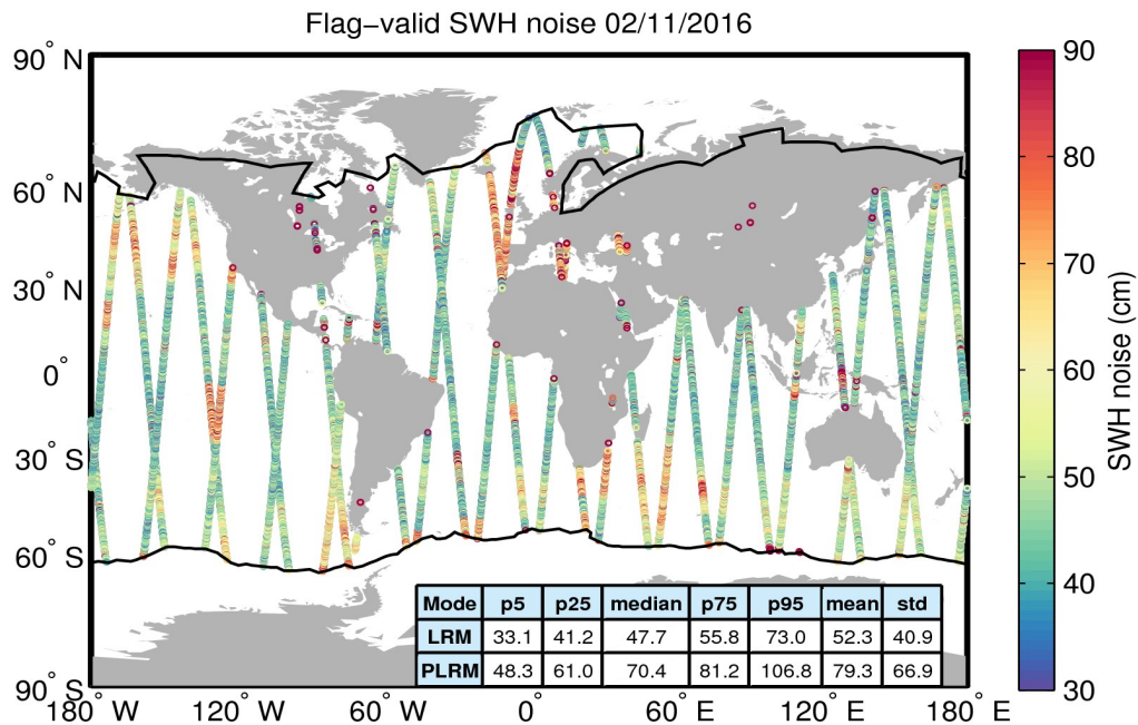
Figure 18. Geographical distribution of flag-valid 20-Hz SWH measurement noise over oceans and lakes for 02/11/2016. The statistical values shown in the table refer to the SWH noise and are calculated separately for LRM and PLRM regions. Measurements taken over polar polygons have been excluded from the computation of the statistical values. The black lines mark the outer limit of the Arctic and Antarctic polar polygons.
