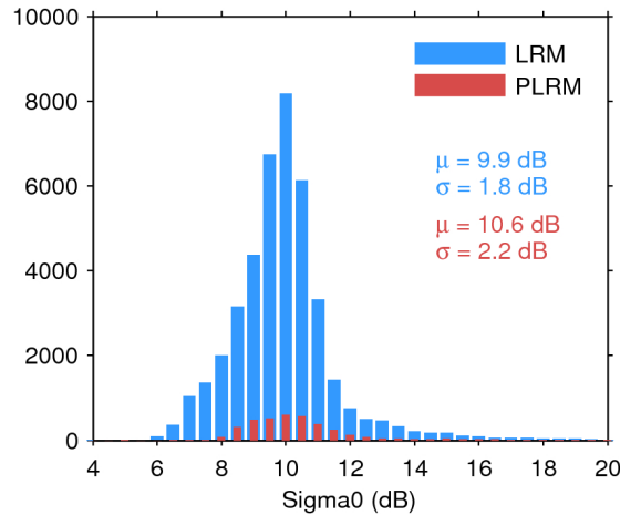
Figure 25. Histogram of flag-valid sigma0 over oceans and lakes for LRM (blue) and PLRM (red) for 02/11/2016. The mean ( \mu ) and standard deviation ( \sigma ) are also shown. Note that values outside [4 20] dB are excluded from the histogram for the sake of readability but not from the computation of \mu and \sigma .
