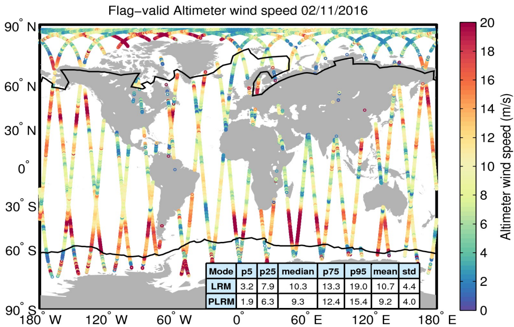
Figure 31. Geographical distribution of flag-valid wind data over oceans and lakes for 02/11/2016. The statistical values shown in the table refer to the wind in m/s and are calculated separately for LRM and PLRM regions. Measurements taken over polar polygons have been excluded from the computation of the statistical values. The black lines mark the outer limit of the Arctic and Antarctic polar polygons.
