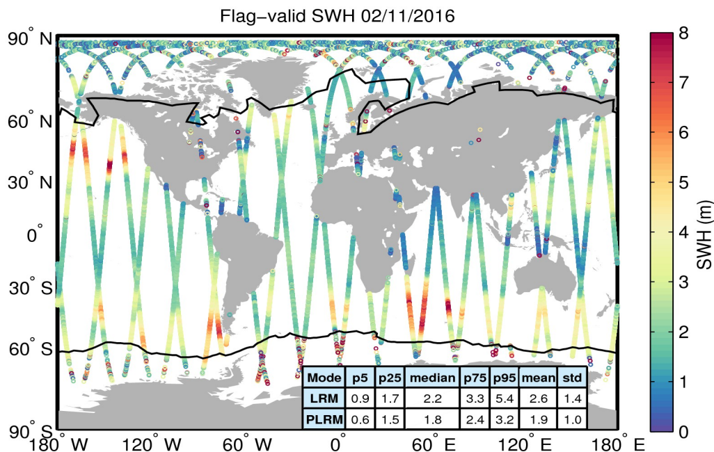
Figure 15. Geographical distribution of flag-valid SWH data over oceans and lakes for 02/11/2016. The statistical values shown in the table refer to the SWH in m and are calculated separately for LRM and PLRM regions. Measurements taken over polar polygons have been excluded from the computation of the statistical values. The black lines mark the outer limit of the Arctic and Antarctic polar polygons.
