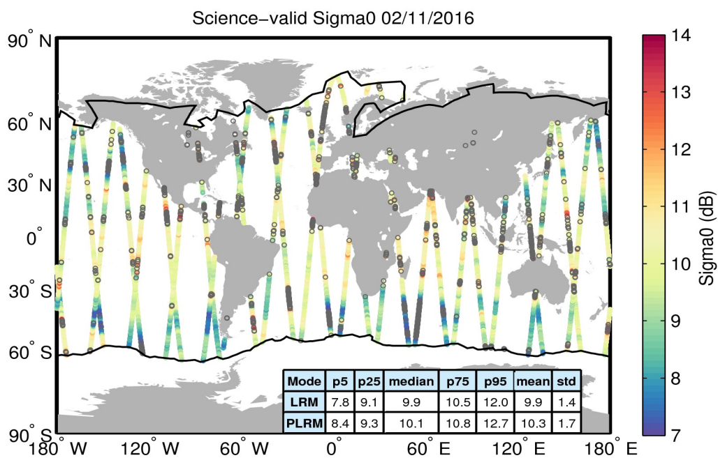
Figure 27. Geographical distribution of science-valid sigma0 data over oceans and lakes for 02/11/2016. The statistical values shown in the table refer to the sigma0 in dB and are calculated separately for LRM and PLRM regions. The black lines mark the outer limit of the Arctic and Antarctic polar polygons. Gray circles denote records that have been rejected based on the editing criteria described in Table 4.
