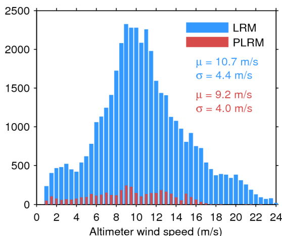
Figure 33. Histogram of flag-valid wind over oceans and lakes for LRM (blue) and PLRM (red) for 02/11/2016. The mean ( \mu ) and standard deviation ( \sigma ) are also shown. Note that values larger than 24 m/s are excluded from the histogram for the sake of readability but not from the computation of \mu and \sigma .
