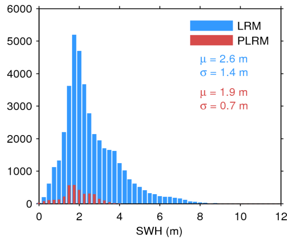
Figure 20. Histogram of science-valid SWH over oceans and lakes for LRM (blue) and PLRM (red) for 02/11/2016. The mean ( \mu ) and standard deviation ( \sigma ) are also shown. Note that values larger than 12 m are excluded from the histogram for the sake of readability but not from the computation of \mu and \sigma .
