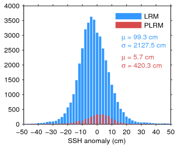
Figure 7. Histogram of flag-valid SSH anomaly over oceans and lakes for LRM (blue) and PLRM (red) for 02/11/2016. The mean ( \mu ) and standard deviation ( \sigma ) are also shown. Note that values outside [-50 \ 50] cm are excluded from the histogram for the sake of readability but not from the computation of \mu and \sigma .
