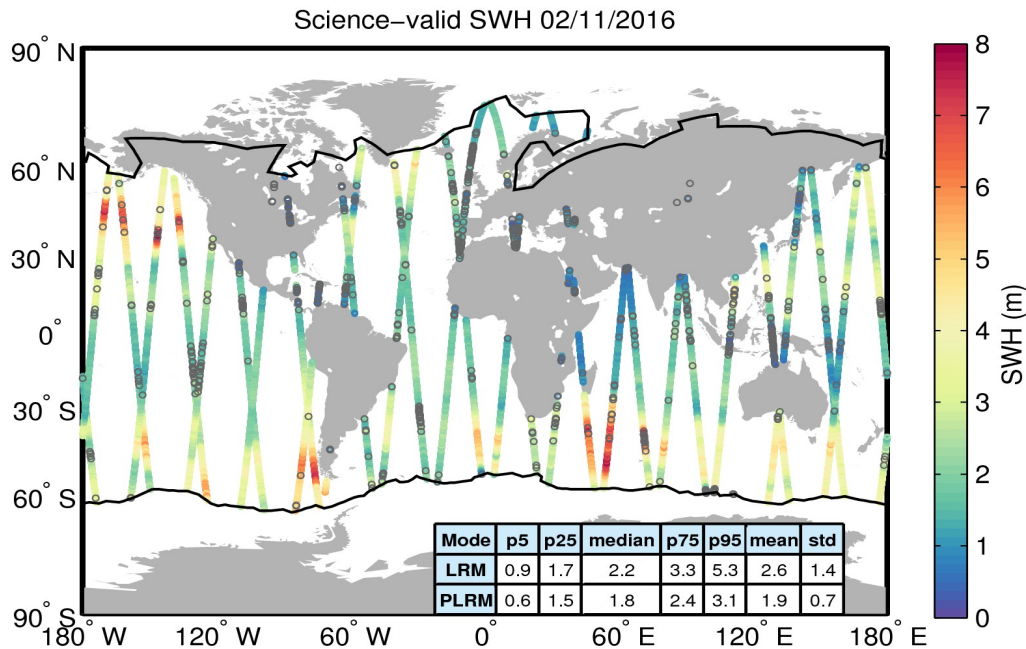
Figure 19. Geographical distribution of science-valid SWH data over oceans and lakes for 02/11/2016. The statistical values shown in the table refer to the SWH in m and are calculated separately for LRM and PLRM regions. The black lines mark the outer limit of the Arctic and Antarctic polar polygons. Gray circles denote records that have been rejected based on the editing criteria described in Table 3.
