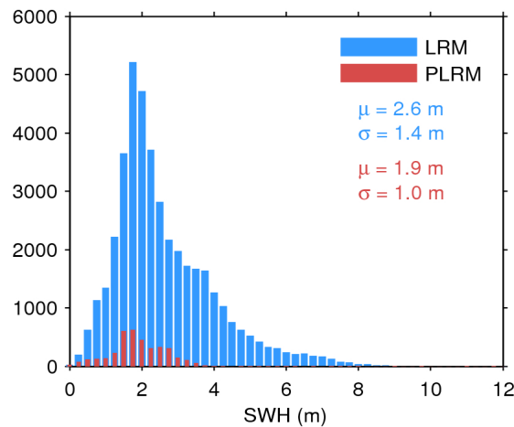
Figure 17. Histogram of flag-valid SWH over oceans and lakes for LRM (blue) and PLRM (red) for 02/11/2016. The mean ( \mu ) and standard deviation ( \sigma ) are also shown. Note that values larger than 12 m are excluded from the histogram for the sake of readability but not from the computation of \mu and \sigma .
