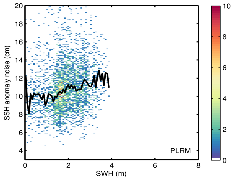
Figure 9. 2D histogram showing flag-valid SSH anomaly noise as a function of SWH for LRM (top) and PLRM (bottom) for 02/11/2016. The black line denotes the median SSH anomaly noise as a function of SWH.
