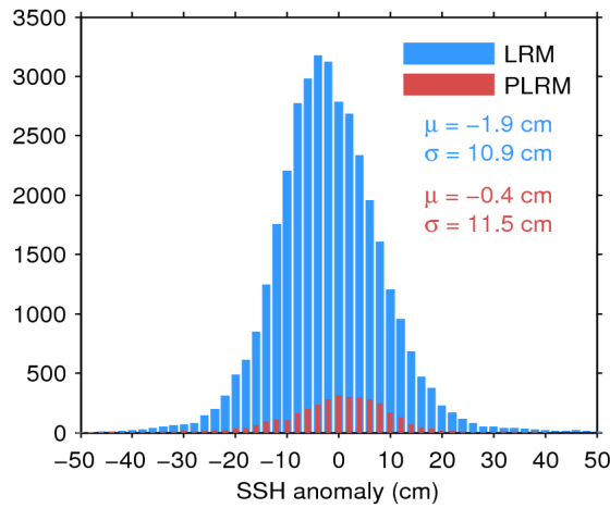
Figure 11. Histogram of science-valid SSH anomaly over oceans and lakes for LRM (blue) and PLRM (red) for 02/11/2016. The mean ( \mu ) and standard deviation ( \sigma ) are also shown. Note that values outside [-50 50] cm are excluded from the histogram for the sake of readability but not from the computation of \mu and \sigma .
