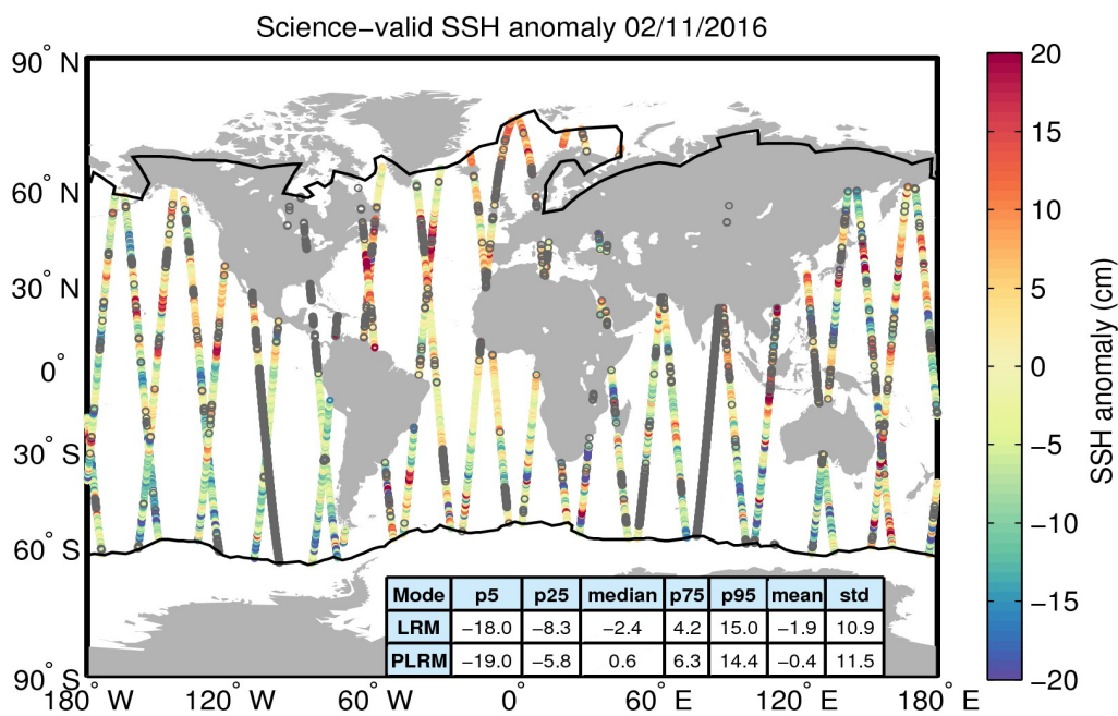
Figure 10. Geographical distribution of science-valid SSH anomaly data over oceans and lakes for 02/11/2016. The statistical values shown in the table refer to the SSH anomaly in cm and are calculated separately for LRM and PLRM regions. The black lines mark the outer limit of the Arctic and Antarctic polar polygons. Gray circles denote records that have been rejected based on the editing criteria described in Table 2.
