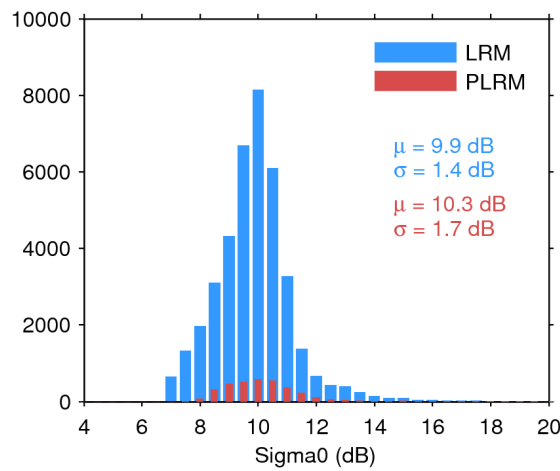
Figure 28. Histogram of science-valid sigma0 over oceans and lakes for LRM (blue) and PLRM (red) for 02/11/2016. The mean ( \mu ) and standard deviation ( \sigma ) are also shown. Note that values outside [4 20] dB are excluded from the histogram for the sake of readability but not from the computation of \mu and \sigma .
