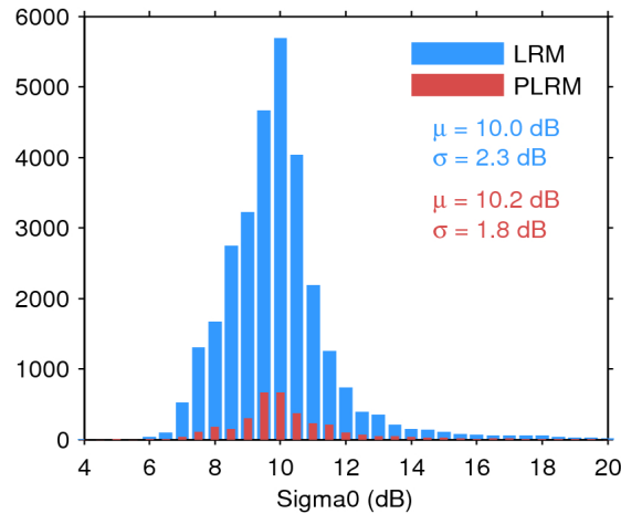
Figure 25. Histogram of flag-valid sigma0 over oceans and lakes for LRM (blue) and PLRM (red) for 28/10/2016. The mean ( \mu ) and standard deviation ( \sigma ) are also shown. Note that values outside [4 20] dB are excluded from the histogram for the sake of readability but not from the computation of \mu and \sigma .
