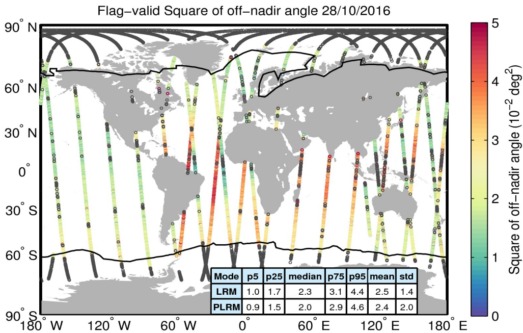
Figure 37. Geographical distribution of flag-valid mispointing data over oceans and lakes for 28/10/2016. The statistical values shown in the table refer to the mispointing in 10^{-2} \text{ deg}^2 and are calculated separately for LRM and PLRM regions. Measurements taken over polar polygons have been excluded from the computation of the statistical values. The black lines mark the outer limit of the Arctic and Antarctic polar polygons. Gray circles denote negative values.
