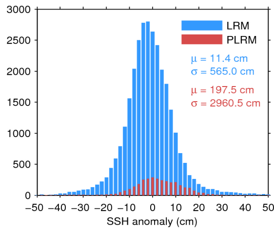
Figure 7. Histogram of flag-valid SSH anomaly over oceans and lakes for LRM (blue) and PLRM (red) for 28/10/2016. The mean ( \mu ) and standard deviation ( \sigma ) are also shown. Note that values outside [-50\ 50] cm are excluded from the histogram for the sake of readability but not from the computation of \mu and \sigma .
