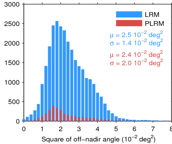
Figure 39. Histogram of flag-valid mispointing over oceans and lakes for LRM (blue) and PLRM (red) for 28/10/2016. Only positive values have been considered. The mean ( \mu ) and standard deviation ( \sigma ) are also shown. Note that values larger than 8 \cdot 10^{-2} \text{ deg}^2 are excluded from the histogram for the sake of readability but not from the computation of \mu and \sigma .
