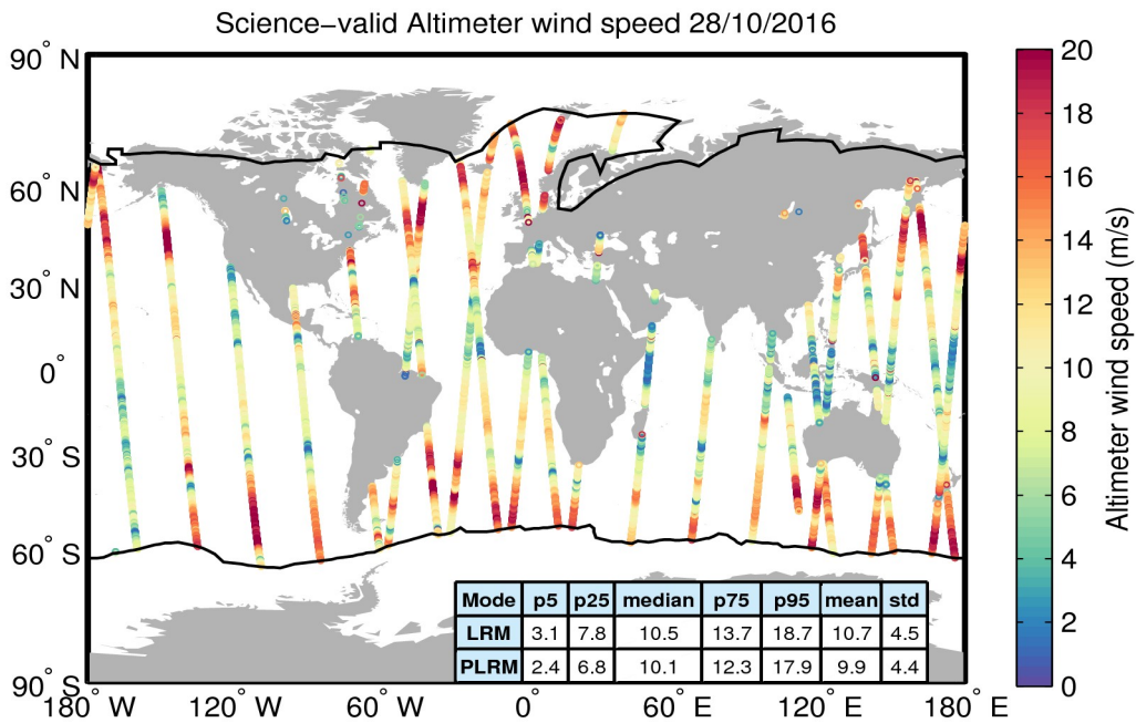
Figure 34. Geographical distribution of science-valid wind data over oceans and lakes for 28/10/2016. The statistical values shown in the table refer to the wind in m/s and are calculated separately for LRM and PLRM regions. The black lines mark the outer limit of the Arctic and Antarctic polar polygons. Gray circles denote records that have been rejected based on the editing criteria described in Table 5.
