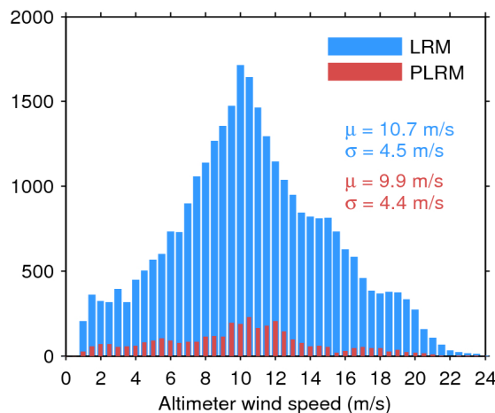
Figure 35. Histogram of science-valid wind over oceans and lakes for LRM (blue) and PLRM (red) for 28/10/2016. The mean ( \mu ) and standard deviation ( \sigma ) are also shown. Note that values larger than 24 m/s are excluded from the histogram for the sake of readability but not from the computation of \mu and \sigma .
