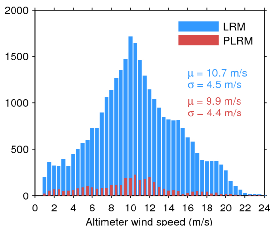
Figure 33. Histogram of flag-valid wind over oceans and lakes for LRM (blue) and PLRM (red) for 28/10/2016. The mean ( \mu ) and standard deviation ( \sigma ) are also shown. Note that values larger than 24 m/s are excluded from the histogram for the sake of readability but not from the computation of \mu and \sigma .
