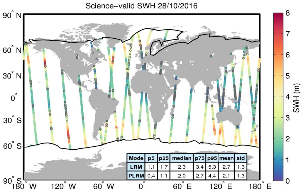
Figure 19. Geographical distribution of science-valid SWH data over oceans and lakes for 28/10/2016. The statistical values shown in the table refer to the SWH in m and are calculated separately for LRM and PLRM regions. The black lines mark the outer limit of the Arctic and Antarctic polar polygons. Gray circles denote records that have been rejected based on the editing criteria described in Table 3.
