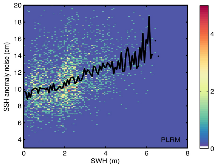
Figure 9. 2D histogram showing flag-valid SSH anomaly noise as a function of SWH for LRM (top) and PLRM (bottom) for 28/10/2016. The black line denotes the median SSH anomaly noise as a function of SWH.
