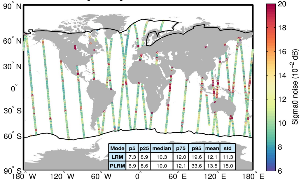
Flag-valid sigma0 noise 28/10/2016
