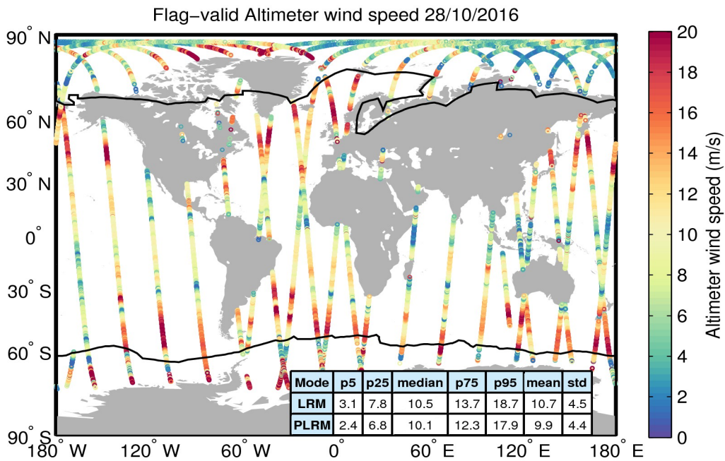
Figure 31. Geographical distribution of flag-valid wind data over oceans and lakes for 28/10/2016. The statistical values shown in the table refer to the wind in m/s and are calculated separately for LRM and PLRM regions. Measurements taken over polar polygons have been excluded from the computation of the statistical values. The black lines mark the outer limit of the Arctic and Antarctic polar polygons.
