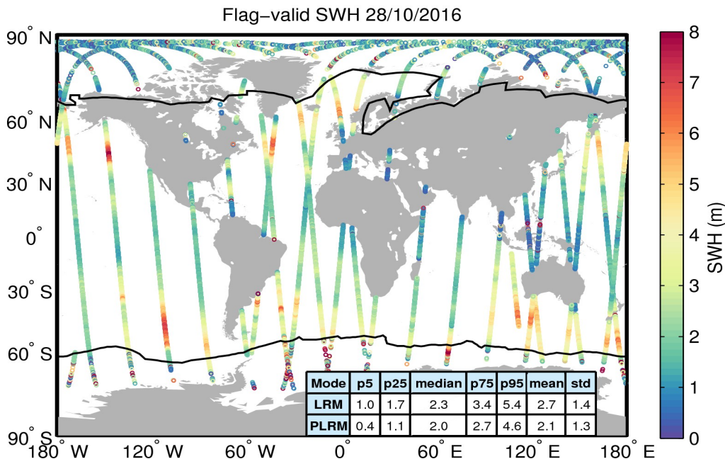
Figure 15. Geographical distribution of flag-valid SWH data over oceans and lakes for 28/10/2016. The statistical values shown in the table refer to the SWH in m and are calculated separately for LRM and PLRM regions. Measurements taken over polar polygons have been excluded from the computation of the statistical values. The black lines mark the outer limit of the Arctic and Antarctic polar polygons.
