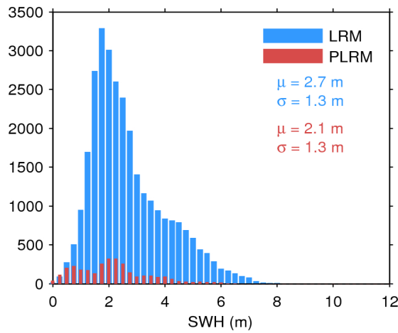
Figure 20. Histogram of science-valid SWH over oceans and lakes for LRM (blue) and PLRM (red) for 28/10/2016. The mean ( \mu ) and standard deviation ( \sigma ) are also shown. Note that values larger than 12 m are excluded from the histogram for the sake of readability but not from the computation of \mu and \sigma .
