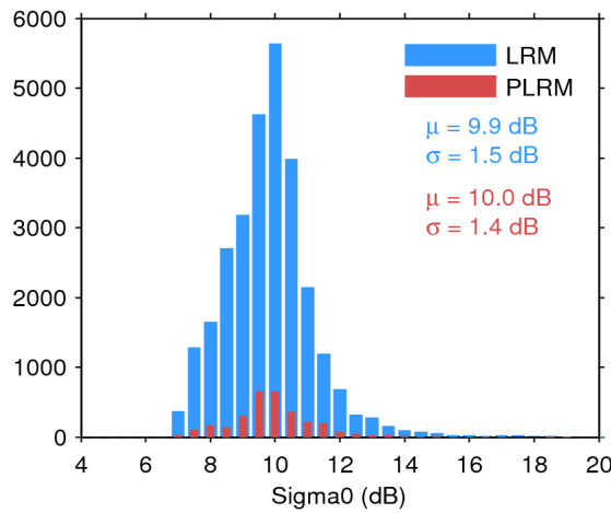
Figure 28. Histogram of science-valid sigma0 over oceans and lakes for LRM (blue) and PLRM (red) for 28/10/2016. The mean ( \mu ) and standard deviation ( \sigma ) are also shown. Note that values outside [4 20] dB are excluded from the histogram for the sake of readability but not from the computation of \mu and \sigma .
