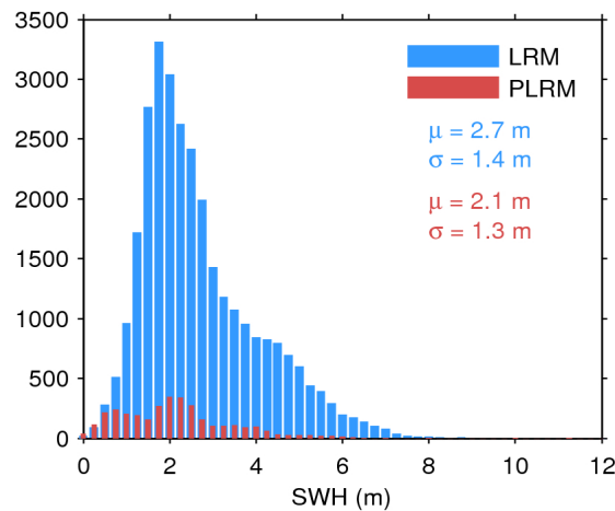
Figure 17. Histogram of flag-valid SWH over oceans and lakes for LRM (blue) and PLRM (red) for 28/10/2016. The mean ( \mu ) and standard deviation ( \sigma ) are also shown. Note that values larger than 12 m are excluded from the histogram for the sake of readability but not from the computation of \mu and \sigma .
