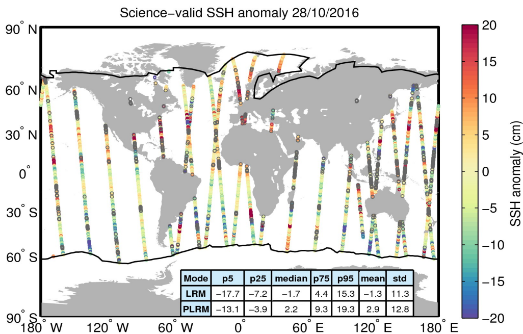
Figure 10. Geographical distribution of science-valid SSH anomaly data over oceans and lakes for 28/10/2016. The statistical values shown in the table refer to the SSH anomaly in cm and are calculated separately for LRM and PLRM regions. The black lines mark the outer limit of the Arctic and Antarctic polar polygons. Gray circles denote records that have been rejected based on the editing criteria described in Table 2.
