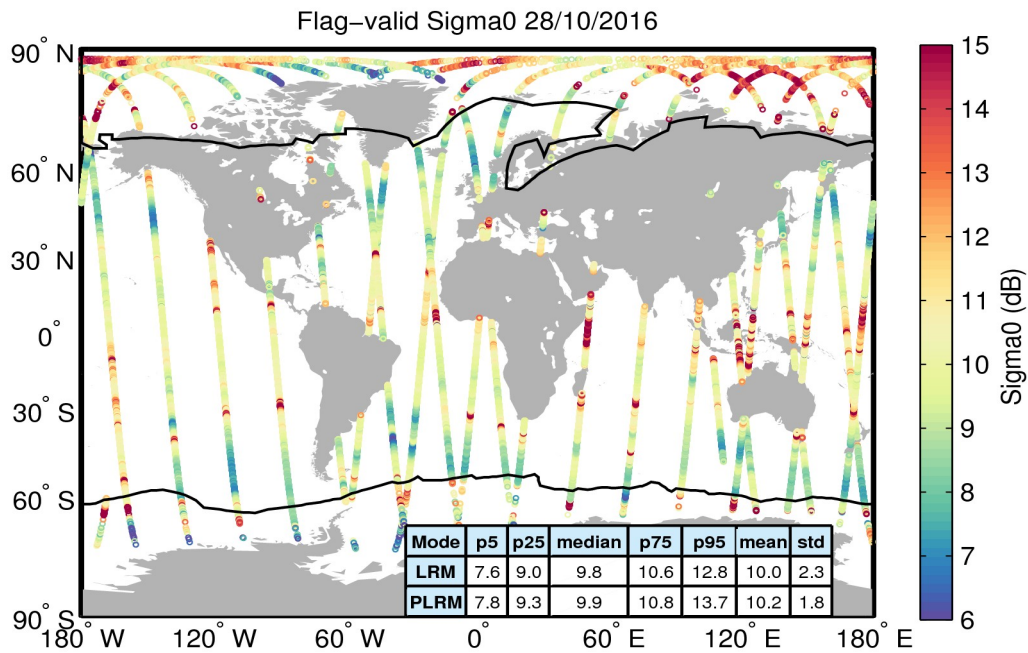
Figure 23. Geographical distribution of flag-valid sigma0 data over oceans and lakes for 28/10/2016. The statistical values shown in the table refer to the sigma0 in dB and are calculated separately for LRM and PLRM regions. Measurements taken over polar polygons have been excluded from the computation of the statistical values. The black lines mark the outer limit of the Arctic and Antarctic polar polygons.
