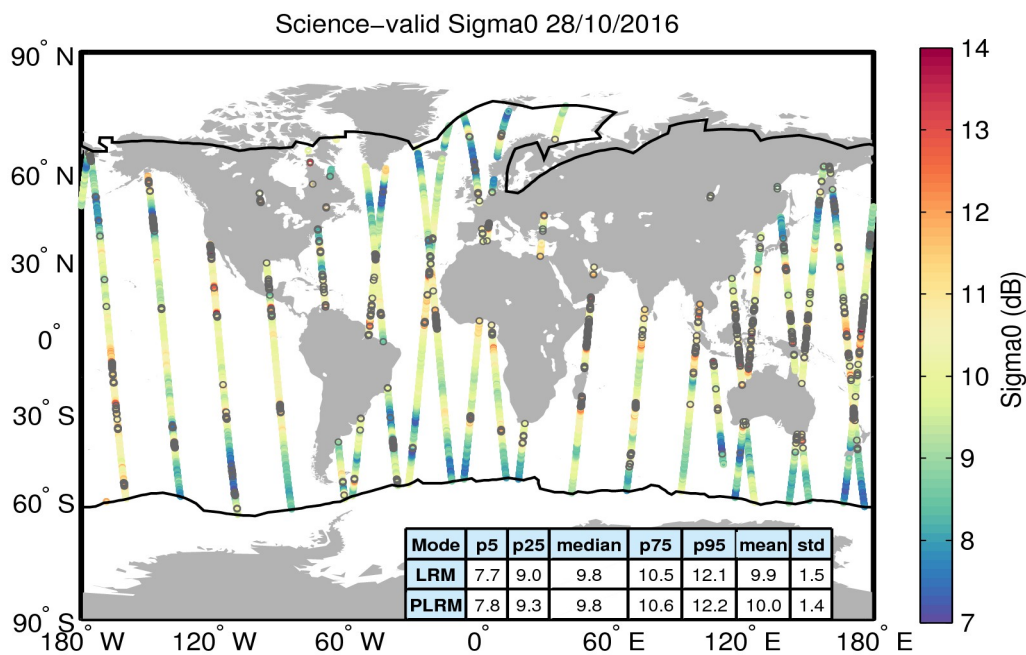
Figure 27. Geographical distribution of science-valid sigma0 data over oceans and lakes for 28/10/2016. The statistical values shown in the table refer to the sigma0 in dB and are calculated separately for LRM and PLRM regions. The black lines mark the outer limit of the Arctic and Antarctic polar polygons. Gray circles denote records that have been rejected based on the editing criteria described in Table 4.
