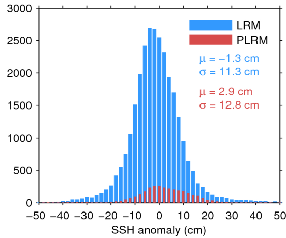
Figure 11. Histogram of science-valid SSH anomaly over oceans and lakes for LRM (blue) and PLRM (red) for 28/10/2016. The mean ( \mu ) and standard deviation ( \sigma ) are also shown. Note that values outside [-50\ 50] cm are excluded from the histogram for the sake of readability but not from the computation of \mu and \sigma .
