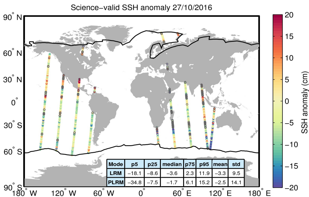
Figure 10. Geographical distribution of science-valid SSH anomaly data over oceans and lakes for 27/10/2016. The statistical values shown in the table refer to the SSH anomaly in cm and are calculated separately for LRM and PLRM regions. The black lines mark the outer limit of the Arctic and Antarctic polar polygons. Gray circles denote records that have been rejected based on the editing criteria described in Table 2.
