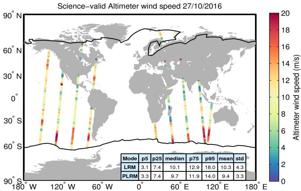
Figure 34. Geographical distribution of science-valid wind data over oceans and lakes for 27/10/2016. The statistical values shown in the table refer to the wind in m/s and are calculated separately for LRM and PLRM regions. The black lines mark the outer limit of the Arctic and Antarctic polar polygons. Gray circles denote records that have been rejected based on the editing criteria described in Table 5.
