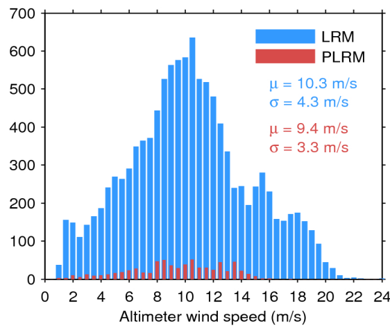
Figure 33. Histogram of flag-valid wind over oceans and lakes for LRM (blue) and PLRM (red) for 27/10/2016. The mean ( \mu ) and standard deviation ( \sigma ) are also shown. Note that values larger than 24 m/s are excluded from the histogram for the sake of readability but not from the computation of \mu and \sigma .
