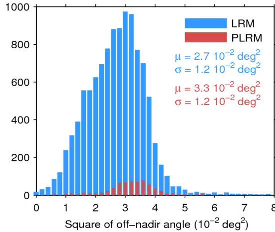
Figure 39. Histogram of flag-valid mispointing over oceans and lakes for LRM (blue) and PLRM (red) for 27/10/2016. Only positive values have been considered. The mean ( \mu ) and standard deviation ( \sigma ) are also shown. Note that values larger than 8 \cdot 10^{-2} \text{ deg}^2 are excluded from the histogram for the sake of readability but not from the computation of \mu and \sigma .
