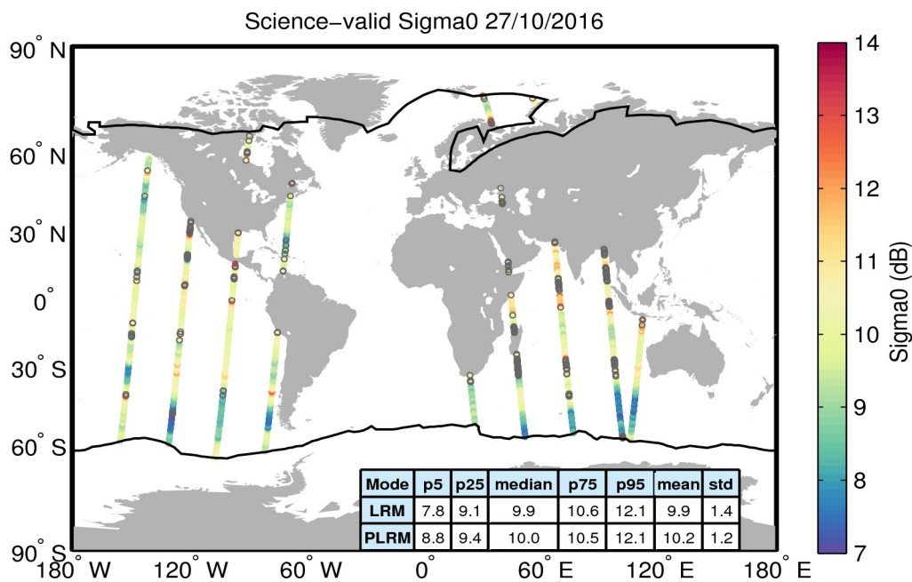
Figure 27. Geographical distribution of science-valid sigma0 data over oceans and lakes for 27/10/2016. The statistical values shown in the table refer to the sigma0 in dB and are calculated separately for LRM and PLRM regions. The black lines mark the outer limit of the Arctic and Antarctic polar polygons. Gray circles denote records that have been rejected based on the editing criteria described in Table 4.
