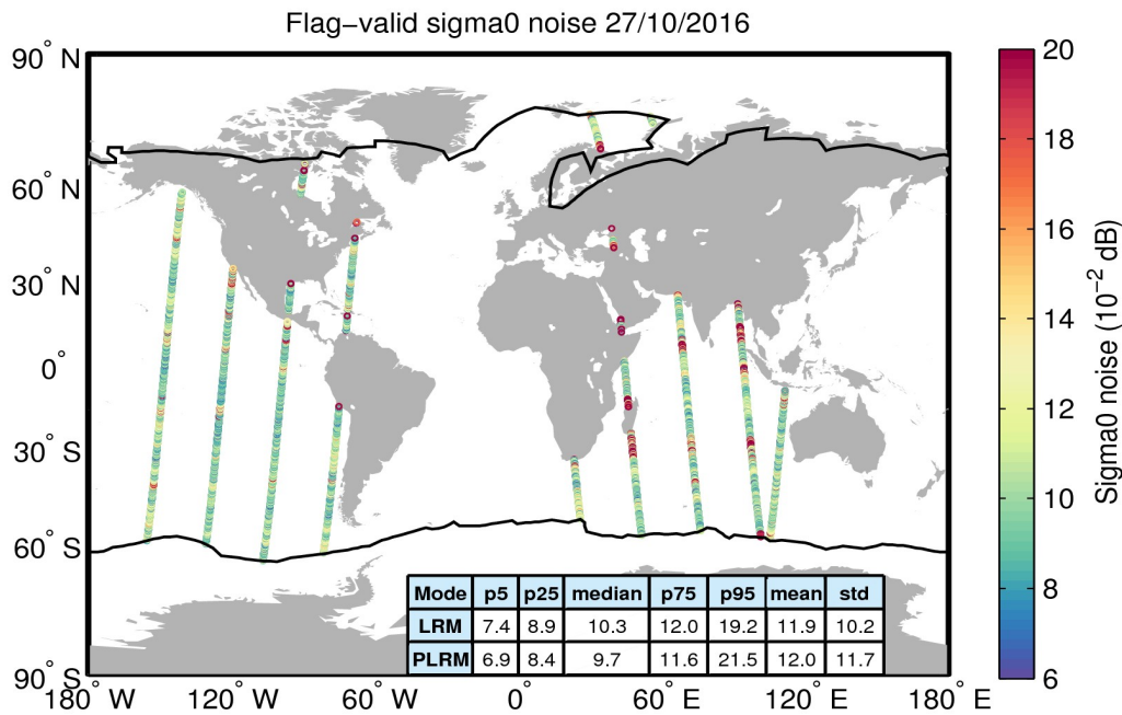
Figure 26. Geographical distribution of flag-valid 20-Hz sigma0 measurement noise over oceans and lakes for 27/10/2016. The statistical values shown in the table refer to the sigma0 noise and are calculated separately for LRM and PLRM regions. Measurements taken over polar polygons have been excluded from the computation of the statistical values. The black lines mark the outer limit of the Arctic and Antarctic polar polygons.
