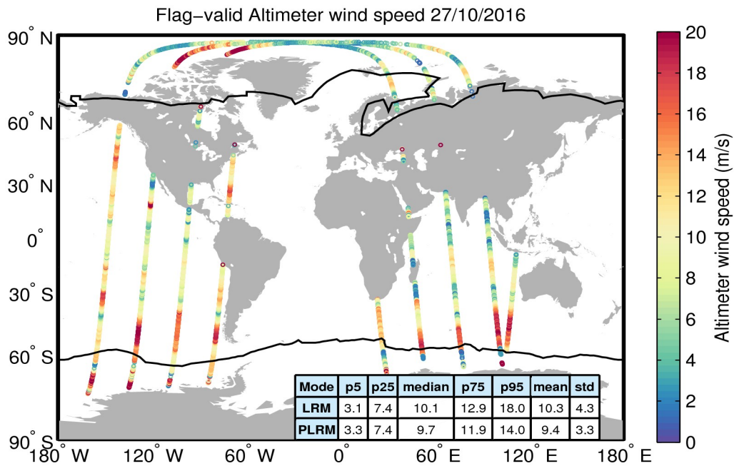
Figure 31. Geographical distribution of flag-valid wind data over oceans and lakes for 27/10/2016. The statistical values shown in the table refer to the wind in m/s and are calculated separately for LRM and PLRM regions. Measurements taken over polar polygons have been excluded from the computation of the statistical values. The black lines mark the outer limit of the Arctic and Antarctic polar polygons.
