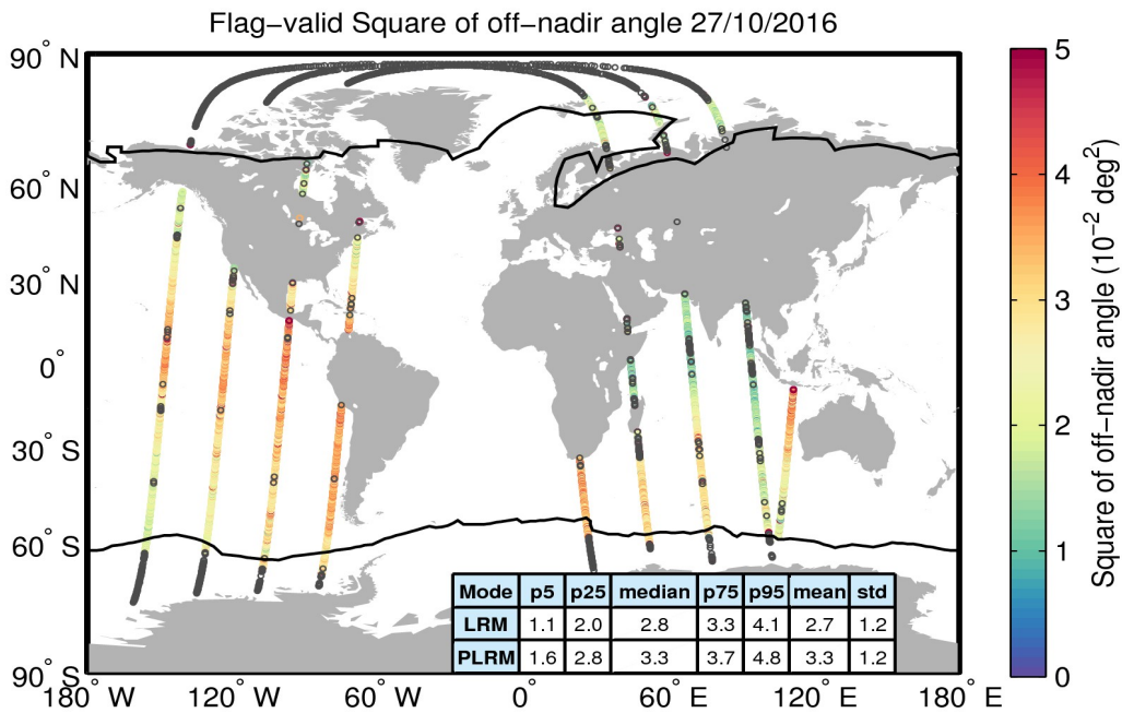
Figure 37. Geographical distribution of flag-valid mispointing data over oceans and lakes for 27/10/2016. The statistical values shown in the table refer to the mispointing in 10^{-2} deg 2 and are calculated separately for LRM and PLRM regions. Measurements taken over polar polygons have been excluded from the computation of the statistical values. The black lines mark the outer limit of the Arctic and Antarctic polar polygons. Gray circles denote negative values.
