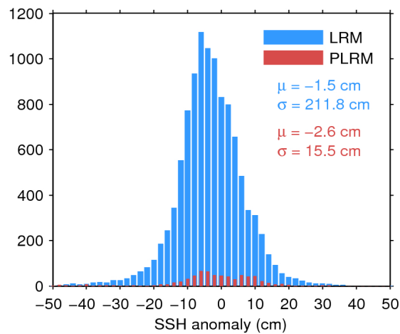
Figure 7. Histogram of flag-valid SSH anomaly over oceans and lakes for LRM (blue) and PLRM (red) for 27/10/2016. The mean ( \mu ) and standard deviation ( \sigma ) are also shown. Note that values outside [-50\ 50] cm are excluded from the histogram for the sake of readability but not from the computation of \mu and \sigma .
