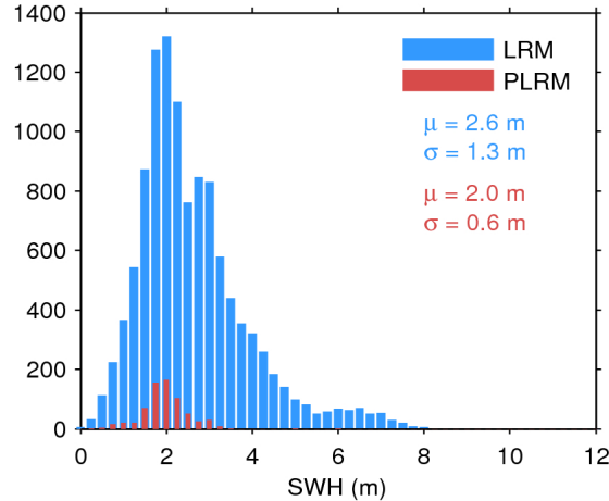
Figure 17. Histogram of flag-valid SWH over oceans and lakes for LRM (blue) and PLRM (red) for 27/10/2016. The mean ( \mu ) and standard deviation ( \sigma ) are also shown. Note that values larger than 12 m are excluded from the histogram for the sake of readability but not from the computation of \mu and \sigma .
