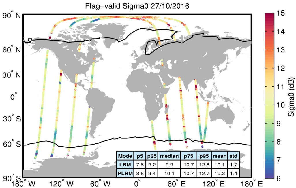
Figure 23. Geographical distribution of flag-valid sigma0 data over oceans and lakes for 27/10/2016. The statistical values shown in the table refer to the sigma0 in dB and are calculated separately for LRM and PLRM regions. Measurements taken over polar polygons have been excluded from the computation of the statistical values. The black lines mark the outer limit of the Arctic and Antarctic polar polygons.
