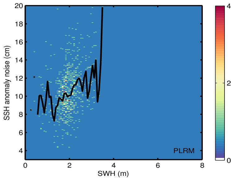
Figure 9. 2D histogram showing flag-valid SSH anomaly noise as a function of SWH for LRM (top) and PLRM (bottom) for 27/10/2016. The black line denotes the median SSH anomaly noise as a function of SWH.
