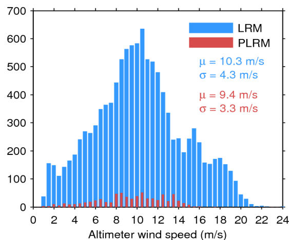
Figure 35. Histogram of science-valid wind over oceans and lakes for LRM (blue) and PLRM (red) for 27/10/2016. The mean ( \mu ) and standard deviation ( \sigma ) are also shown. Note that values larger than 24 m/s are excluded from the histogram for the sake of readability but not from the computation of \mu and \sigma .
