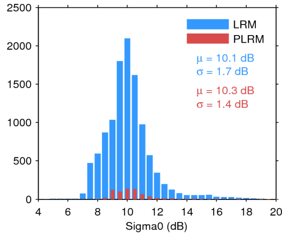
Figure 25. Histogram of flag-valid sigma0 over oceans and lakes for LRM (blue) and PLRM (red) for 27/10/2016. The mean ( \mu ) and standard deviation ( \sigma ) are also shown. Note that values outside [4 20] dB are excluded from the histogram for the sake of readability but not from the computation of \mu and \sigma .
