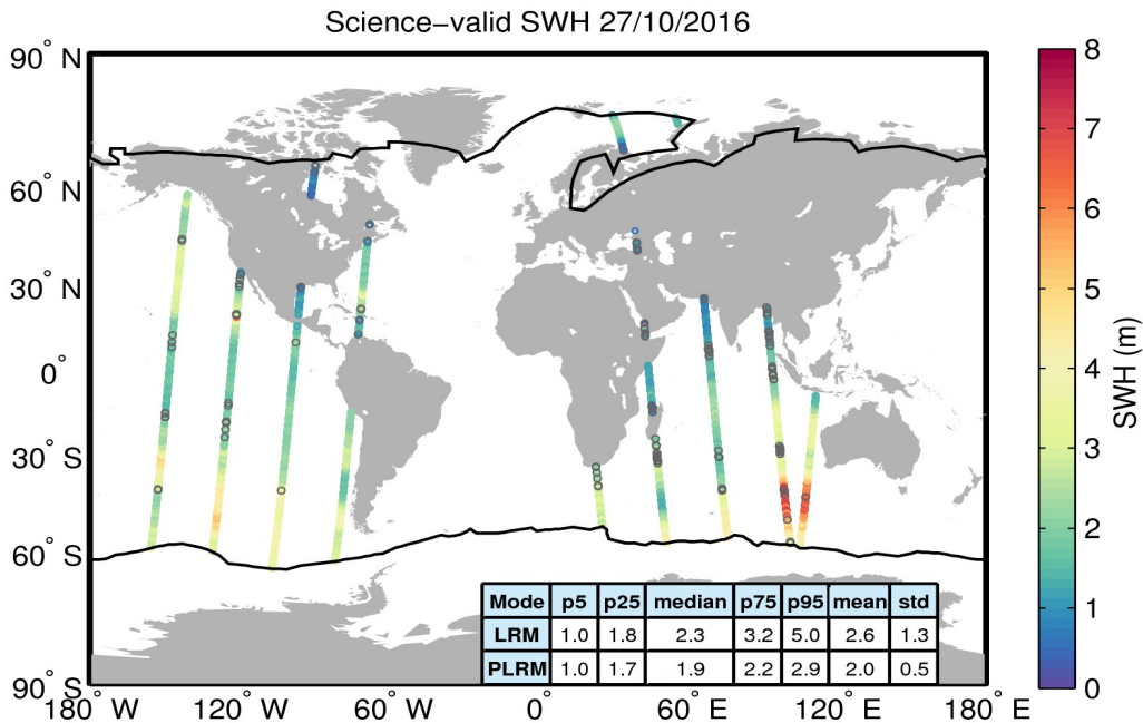
Figure 19. Geographical distribution of science-valid SWH data over oceans and lakes for 27/10/2016. The statistical values shown in the table refer to the SWH in m and are calculated separately for LRM and PLRM regions. The black lines mark the outer limit of the Arctic and Antarctic polar polygons. Gray circles denote records that have been rejected based on the editing criteria described in Table 3.
