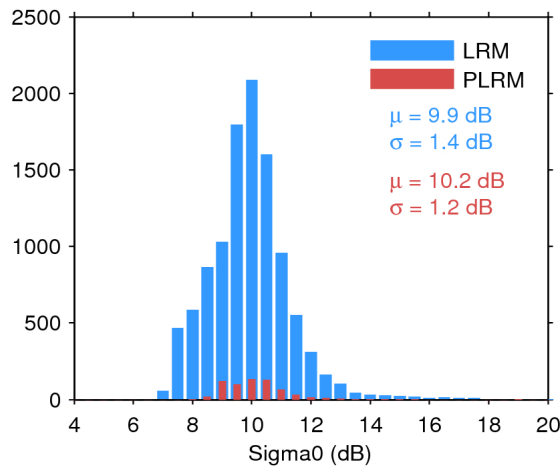
Figure 28. Histogram of science-valid sigma0 over oceans and lakes for LRM (blue) and PLRM (red) for 27/10/2016. The mean ( \mu ) and standard deviation ( \sigma ) are also shown. Note that values outside [4 20] dB are excluded from the histogram for the sake of readability but not from the computation of \mu and \sigma .
