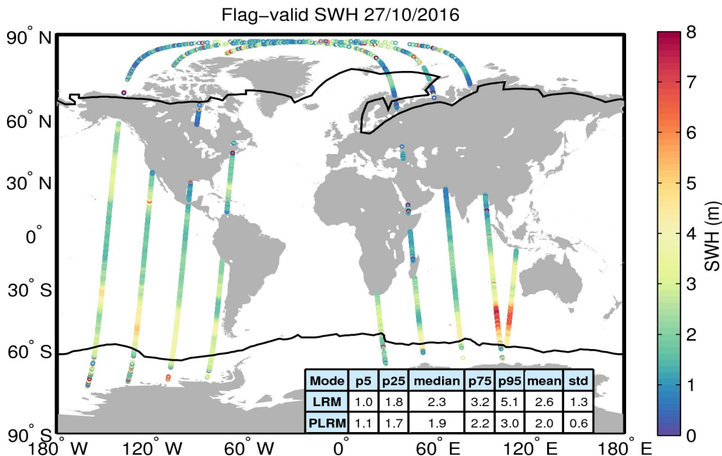
Figure 15. Geographical distribution of flag-valid SWH data over oceans and lakes for 27/10/2016. The statistical values shown in the table refer to the SWH in m and are calculated separately for LRM and PLRM regions. Measurements taken over polar polygons have been excluded from the computation of the statistical values. The black lines mark the outer limit of the Arctic and Antarctic polar polygons.
