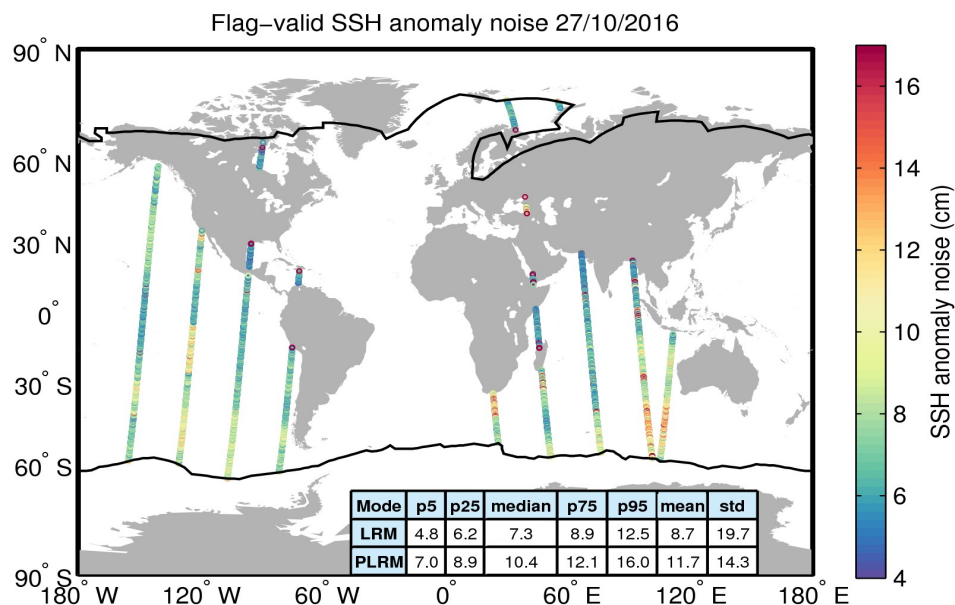
Figure 8. Geographical distribution of flag-valid 20-Hz SSH anomaly measurement noise over oceans and lakes for 27/10/2016. The statistical values shown in the table refer to the SSH anomaly noise and are calculated separately for LRM and PLRM regions. Measurements taken over polar polygons have been excluded from the computation of the statistical values. The black lines mark the outer limit of the Arctic and Antarctic polar polygons.
