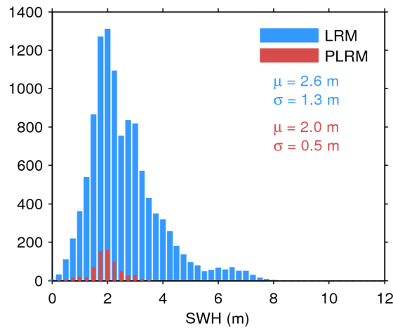
Figure 20. Histogram of science-valid SWH over oceans and lakes for LRM (blue) and PLRM (red) for 27/10/2016. The mean ( \mu ) and standard deviation ( \sigma ) are also shown. Note that values larger than 12 m are excluded from the histogram for the sake of readability but not from the computation of \mu and \sigma .
