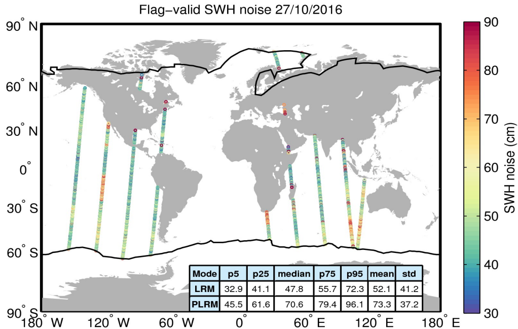
Figure 18. Geographical distribution of flag-valid 20-Hz SWH measurement noise over oceans and lakes for 27/10/2016. The statistical values shown in the table refer to the SWH noise and are calculated separately for LRM and PLRM regions. Measurements taken over polar polygons have been excluded from the computation of the statistical values. The black lines mark the outer limit of the Arctic and Antarctic polar polygons.
