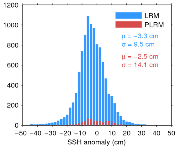
Figure 11. Histogram of science-valid SSH anomaly over oceans and lakes for LRM (blue) and PLRM (red) for 27/10/2016. The mean ( \mu ) and standard deviation ( \sigma ) are also shown. Note that values outside [-50 50] cm are excluded from the histogram for the sake of readability but not from the computation of \mu and \sigma .
