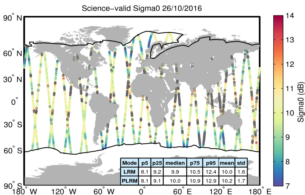
Figure 27. Geographical distribution of science-valid sigma0 data over oceans and lakes for 26/10/2016. The statistical values shown in the table refer to the sigma0 in dB and are calculated separately for LRM and PLRM regions. The black lines mark the outer limit of the Arctic and Antarctic polar polygons. Gray circles denote records that have been rejected based on the editing criteria described in Table 4.
