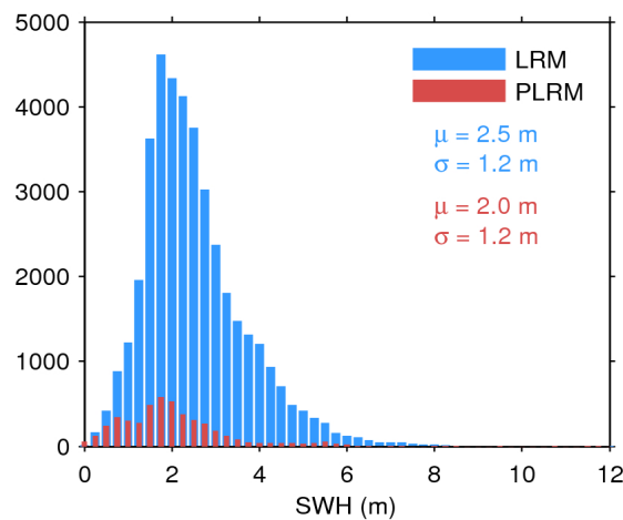
Figure 17. Histogram of flag-valid SWH over oceans and lakes for LRM (blue) and PLRM (red) for 26/10/2016. The mean ( \mu ) and standard deviation ( \sigma ) are also shown. Note that values larger than 12 m are excluded from the histogram for the sake of readability but not from the computation of \mu and \sigma .
