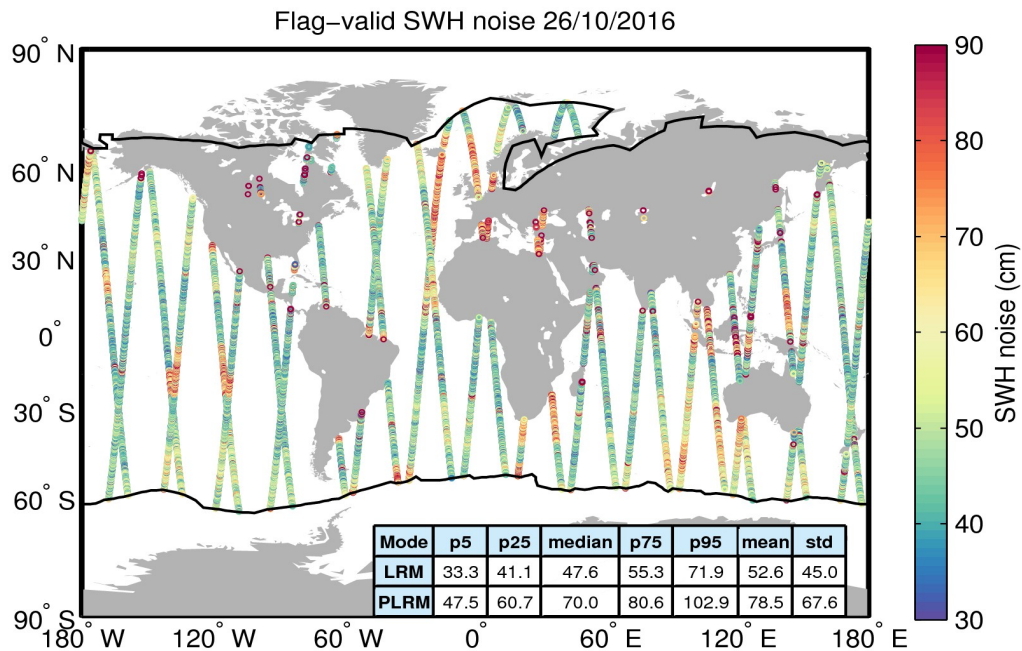
Figure 18. Geographical distribution of flag-valid 20-Hz SWH measurement noise over oceans and lakes for 26/10/2016. The statistical values shown in the table refer to the SWH noise and are calculated separately for LRM and PLRM regions. Measurements taken over polar polygons have been excluded from the computation of the statistical values. The black lines mark the outer limit of the Arctic and Antarctic polar polygons.
