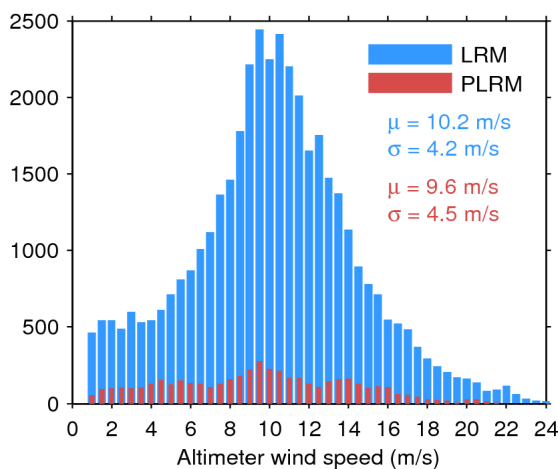
Figure 33. Histogram of flag-valid wind over oceans and lakes for LRM (blue) and PLRM (red) for 26/10/2016. The mean ( \mu ) and standard deviation ( \sigma ) are also shown. Note that values larger than 24 m/s are excluded from the histogram for the sake of readability but not from the computation of \mu and \sigma .
