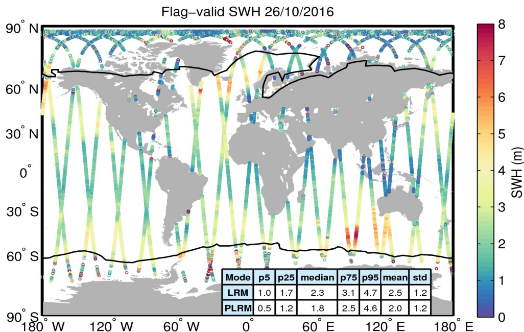
Figure 15. Geographical distribution of flag-valid SWH data over oceans and lakes for 26/10/2016. The statistical values shown in the table refer to the SWH in m and are calculated separately for LRM and PLRM regions. Measurements taken over polar polygons have been excluded from the computation of the statistical values. The black lines mark the outer limit of the Arctic and Antarctic polar polygons.
