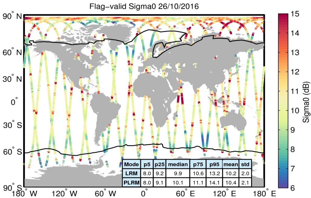
Figure 23. Geographical distribution of flag-valid sigma0 data over oceans and lakes for 26/10/2016. The statistical values shown in the table refer to the sigma0 in dB and are calculated separately for LRM and PLRM regions. Measurements taken over polar polygons have been excluded from the computation of the statistical values. The black lines mark the outer limit of the Arctic and Antarctic polar polygons.
