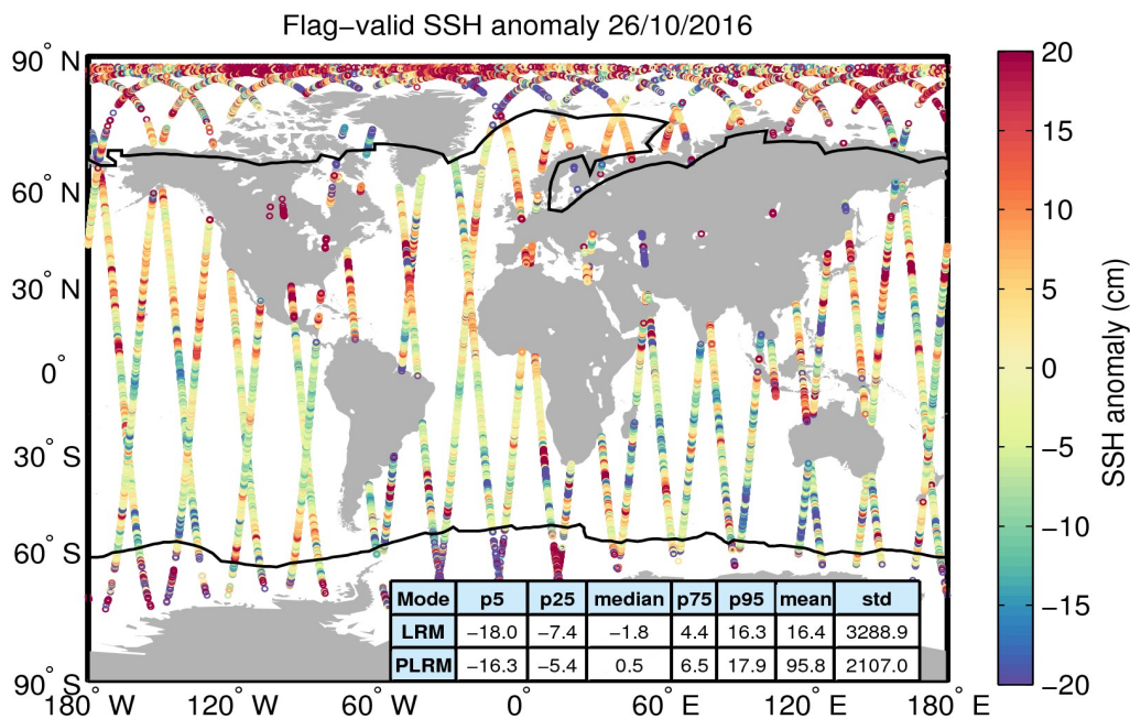
Figure 5. Geographical distribution of flag-valid 1-Hz SSH anomaly data over oceans and lakes for 26/10/2016. The statistical values shown in the table refer to the SSH anomaly in cm and are calculated separately for LRM and PLRM regions. Measurements taken over polar polygons have been excluded from the computation of the statistical values. The black lines mark the outer limit of the Arctic and Antarctic polar polygons.
