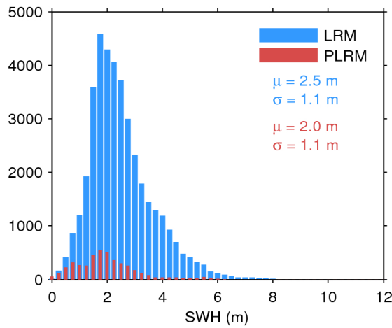
Figure 20. Histogram of science-valid SWH over oceans and lakes for LRM (blue) and PLRM (red) for 26/10/2016. The mean ( \mu ) and standard deviation ( \sigma ) are also shown. Note that values larger than 12 m are excluded from the histogram for the sake of readability but not from the computation of \mu and \sigma .
