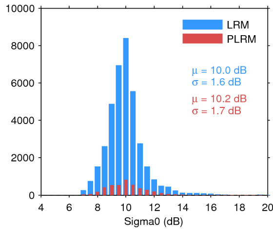
Figure 28. Histogram of science-valid sigma0 over oceans and lakes for LRM (blue) and PLRM (red) for 26/10/2016. The mean ( \mu ) and standard deviation ( \sigma ) are also shown. Note that values outside [4 20] dB are excluded from the histogram for the sake of readability but not from the computation of \mu and \sigma .
