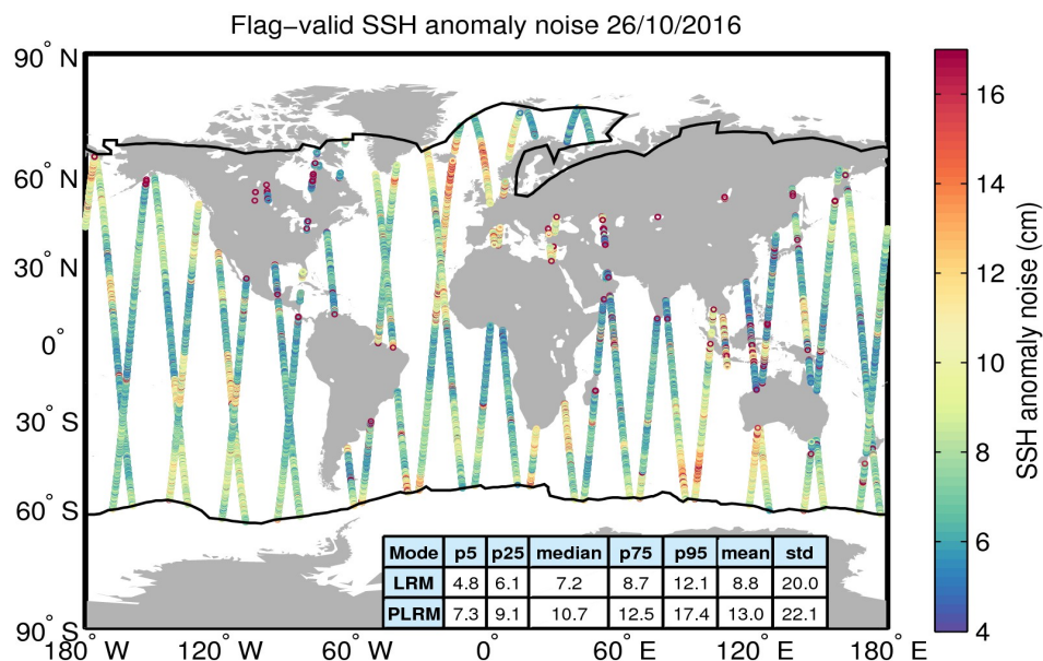
Figure 8. Geographical distribution of flag-valid 20-Hz SSH anomaly measurement noise over oceans and lakes for 26/10/2016. The statistical values shown in the table refer to the SSH anomaly noise and are calculated separately for LRM and PLRM regions. Measurements taken over polar polygons have been excluded from the computation of the statistical values. The black lines mark the outer limit of the Arctic and Antarctic polar polygons.
