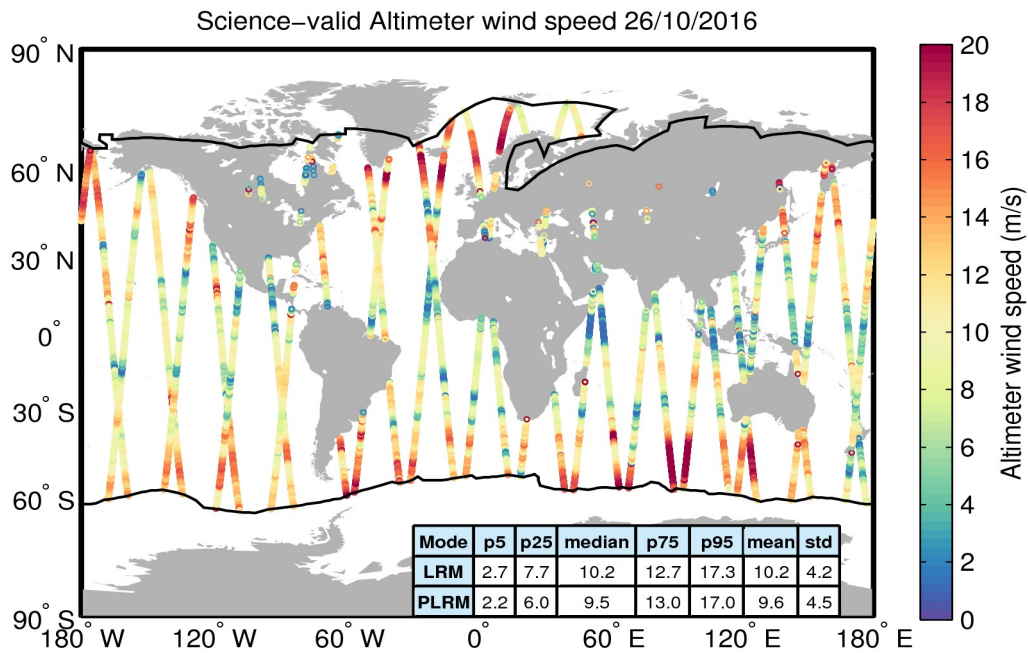
Figure 34. Geographical distribution of science-valid wind data over oceans and lakes for 26/10/2016. The statistical values shown in the table refer to the wind in m/s and are calculated separately for LRM and PLRM regions. The black lines mark the outer limit of the Arctic and Antarctic polar polygons. Gray circles denote records that have been rejected based on the editing criteria described in Table 5.
