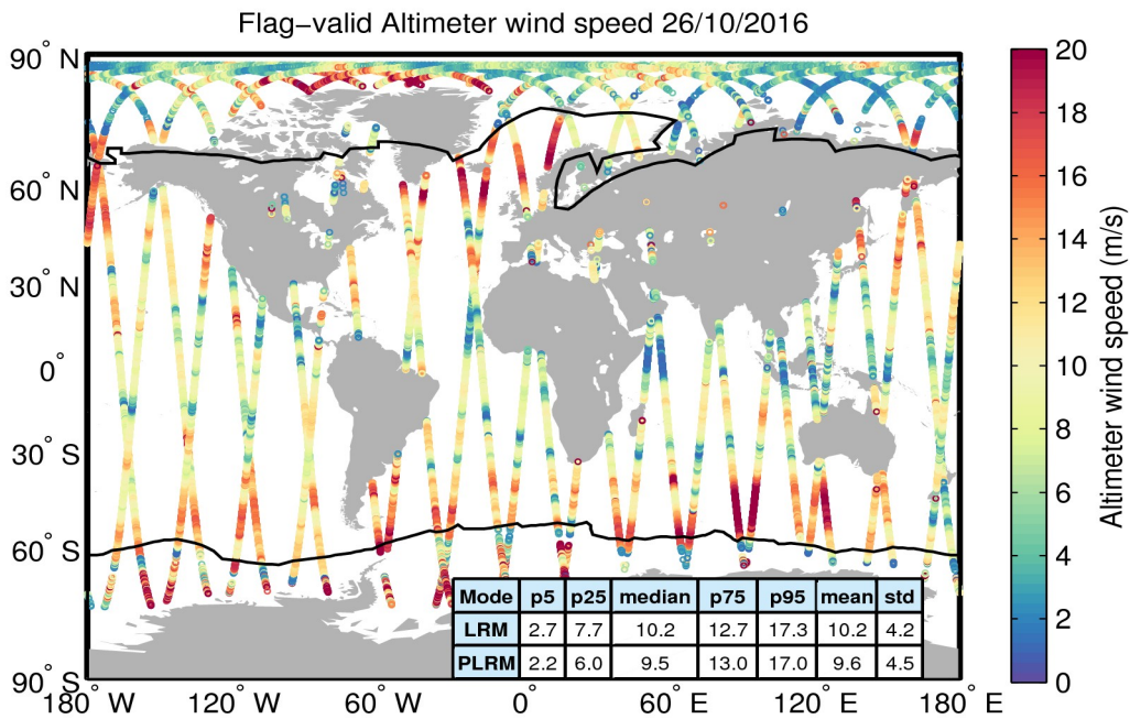
Figure 31. Geographical distribution of flag-valid wind data over oceans and lakes for 26/10/2016. The statistical values shown in the table refer to the wind in m/s and are calculated separately for LRM and PLRM regions. Measurements taken over polar polygons have been excluded from the computation of the statistical values. The black lines mark the outer limit of the Arctic and Antarctic polar polygons.
