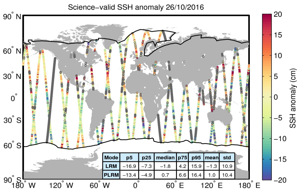
Figure 10. Geographical distribution of science-valid SSH anomaly data over oceans and lakes for 26/10/2016. The statistical values shown in the table refer to the SSH anomaly in cm and are calculated separately for LRM and PLRM regions. The black lines mark the outer limit of the Arctic and Antarctic polar polygons. Gray circles denote records that have been rejected based on the editing criteria described in Table 2.
