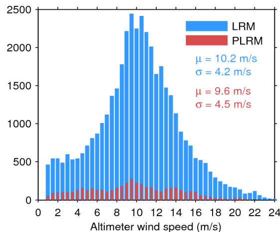
Figure 35. Histogram of science-valid wind over oceans and lakes for LRM (blue) and PLRM (red) for 26/10/2016. The mean ( \mu ) and standard deviation ( \sigma ) are also shown. Note that values larger than 24 m/s are excluded from the histogram for the sake of readability but not from the computation of \mu and \sigma .
