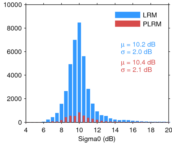
Figure 25. Histogram of flag-valid sigma0 over oceans and lakes for LRM (blue) and PLRM (red) for 26/10/2016. The mean ( \mu ) and standard deviation ( \sigma ) are also shown. Note that values outside [4 20] dB are excluded from the histogram for the sake of readability but not from the computation of \mu and \sigma .
