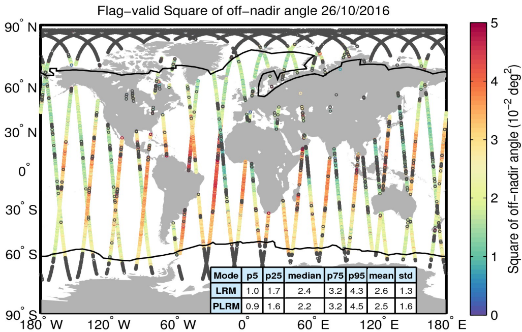
Figure 37. Geographical distribution of flag-valid mispointing data over oceans and lakes for 26/10/2016. The statistical values shown in the table refer to the mispointing in 10^{-2} \text{ deg}^2 and are calculated separately for LRM and PLRM regions. Measurements taken over polar polygons have been excluded from the computation of the statistical values. The black lines mark the outer limit of the Arctic and Antarctic polar polygons. Gray circles denote negative values.
