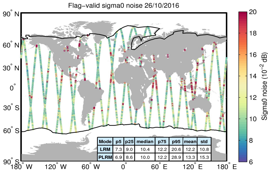
Figure 26. Geographical distribution of flag-valid 20-Hz sigma0 measurement noise over oceans and lakes for 26/10/2016. The statistical values shown in the table refer to the sigma0 noise and are calculated separately for LRM and PLRM regions. Measurements taken over polar polygons have been excluded from the computation of the statistical values. The black lines mark the outer limit of the Arctic and Antarctic polar polygons.
