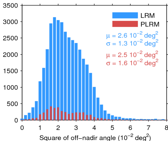
Figure 39. Histogram of flag-valid mispointing over oceans and lakes for LRM (blue) and PLRM (red) for 26/10/2016. Only positive values have been considered. The mean ( \mu ) and standard deviation ( \sigma ) are also shown. Note that values larger than 8 \cdot 10^{-2} \text{ deg}^2 are excluded from the histogram for the sake of readability but not from the computation of \mu and \sigma .
