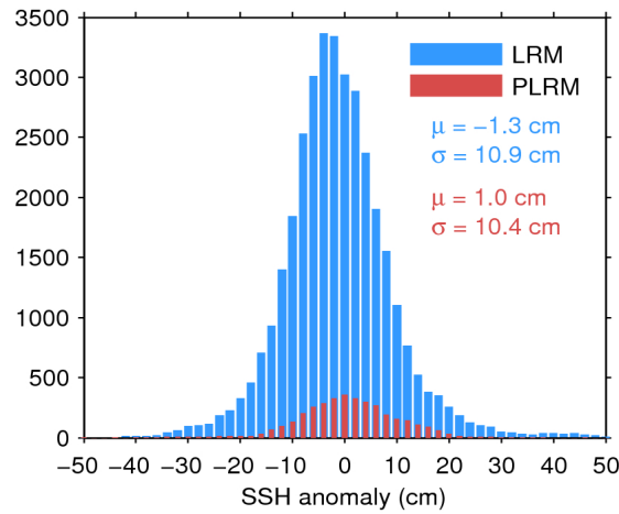
Figure 11. Histogram of science-valid SSH anomaly over oceans and lakes for LRM (blue) and PLRM (red) for 26/10/2016. The mean ( \mu ) and standard deviation ( \sigma ) are also shown. Note that values outside [-50\ 50] cm are excluded from the histogram for the sake of readability but not from the computation of \mu and \sigma .
