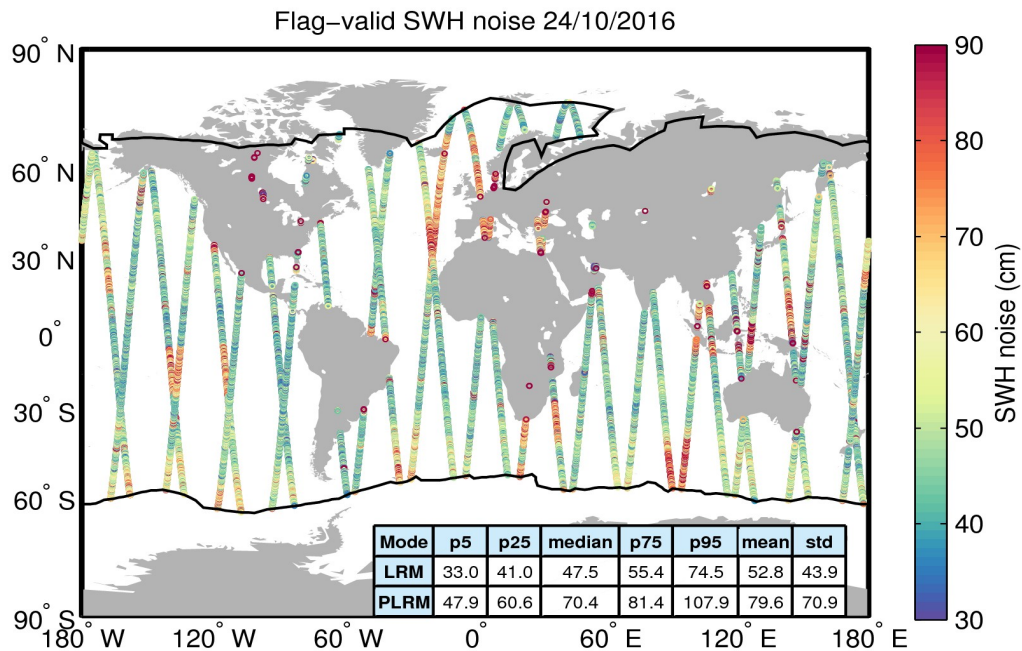
Figure 18. Geographical distribution of flag-valid 20-Hz SWH measurement noise over oceans and lakes for 24/10/2016. The statistical values shown in the table refer to the SWH noise and are calculated separately for LRM and PLRM regions. Measurements taken over polar polygons have been excluded from the computation of the statistical values. The black lines mark the outer limit of the Arctic and Antarctic polar polygons.
