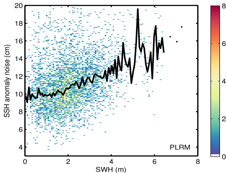
Figure 9. 2D histogram showing flag-valid SSH anomaly noise as a function of SWH for LRM (top) and PLRM (bottom) for 24/10/2016. The black line denotes the median SSH anomaly noise as a function of SWH.
