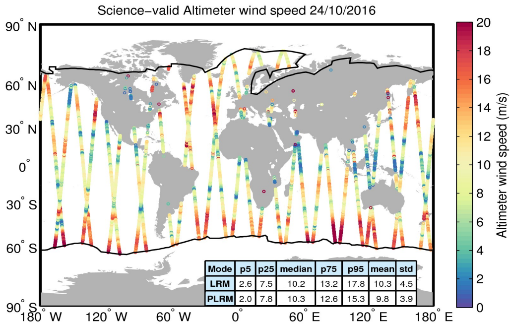
Figure 34. Geographical distribution of science-valid wind data over oceans and lakes for 24/10/2016. The statistical values shown in the table refer to the wind in m/s and are calculated separately for LRM and PLRM regions. The black lines mark the outer limit of the Arctic and Antarctic polar polygons. Gray circles denote records that have been rejected based on the editing criteria described in Table 5.
