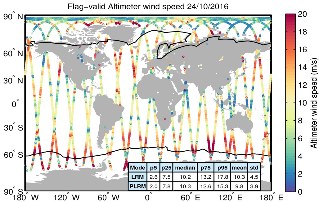
Figure 31. Geographical distribution of flag-valid wind data over oceans and lakes for 24/10/2016. The statistical values shown in the table refer to the wind in m/s and are calculated separately for LRM and PLRM regions. Measurements taken over polar polygons have been excluded from the computation of the statistical values. The black lines mark the outer limit of the Arctic and Antarctic polar polygons.
