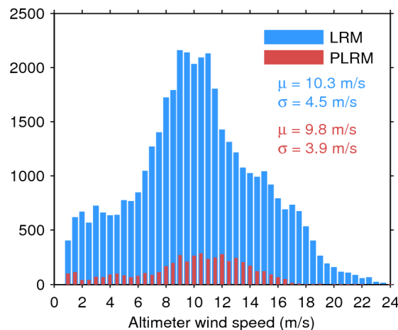
Figure 35. Histogram of science-valid wind over oceans and lakes for LRM (blue) and PLRM (red) for 24/10/2016. The mean ( \mu ) and standard deviation ( \sigma ) are also shown. Note that values larger than 24 m/s are excluded from the histogram for the sake of readability but not from the computation of \mu and \sigma .
