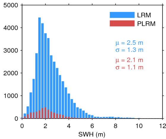
Figure 20. Histogram of science-valid SWH over oceans and lakes for LRM (blue) and PLRM (red) for 24/10/2016. The mean ( \mu ) and standard deviation ( \sigma ) are also shown. Note that values larger than 12 m are excluded from the histogram for the sake of readability but not from the computation of \mu and \sigma .
