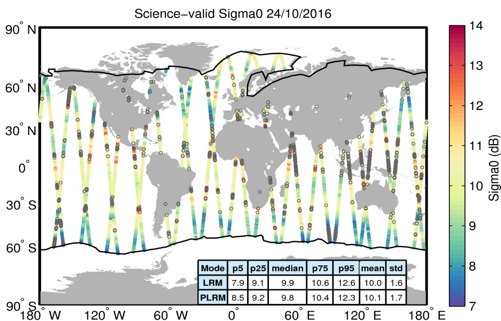
Figure 27. Geographical distribution of science-valid sigma0 data over oceans and lakes for 24/10/2016. The statistical values shown in the table refer to the sigma0 in dB and are calculated separately for LRM and PLRM regions. The black lines mark the outer limit of the Arctic and Antarctic polar polygons. Gray circles denote records that have been rejected based on the editing criteria described in Table 4.
