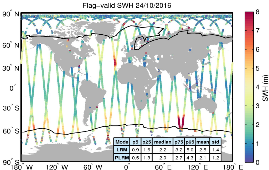
Figure 15. Geographical distribution of flag-valid SWH data over oceans and lakes for 24/10/2016. The statistical values shown in the table refer to the SWH in m and are calculated separately for LRM and PLRM regions. Measurements taken over polar polygons have been excluded from the computation of the statistical values. The black lines mark the outer limit of the Arctic and Antarctic polar polygons.
