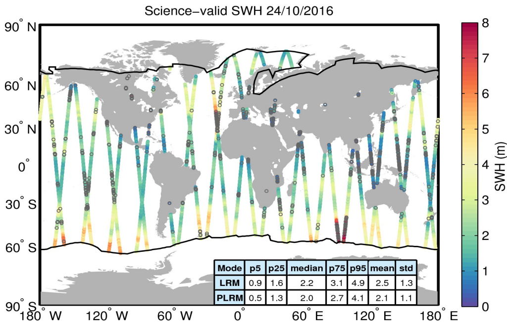
Figure 19. Geographical distribution of science-valid SWH data over oceans and lakes for 24/10/2016. The statistical values shown in the table refer to the SWH in m and are calculated separately for LRM and PLRM regions. The black lines mark the outer limit of the Arctic and Antarctic polar polygons. Gray circles denote records that have been rejected based on the editing criteria described in Table 3.
