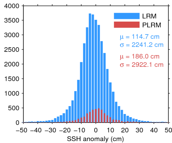
Figure 7. Histogram of flag-valid SSH anomaly over oceans and lakes for LRM (blue) and PLRM (red) for 24/10/2016. The mean ( \mu ) and standard deviation ( \sigma ) are also shown. Note that values outside [-50 50] cm are excluded from the histogram for the sake of readability but not from the computation of \mu and \sigma .
