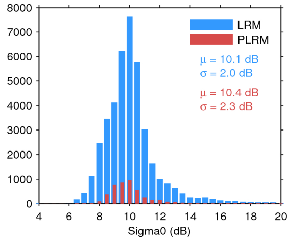
Figure 25. Histogram of flag-valid sigma0 over oceans and lakes for LRM (blue) and PLRM (red) for 24/10/2016. The mean ( \mu ) and standard deviation ( \sigma ) are also shown. Note that values outside [4 20] dB are excluded from the histogram for the sake of readability but not from the computation of \mu and \sigma .
