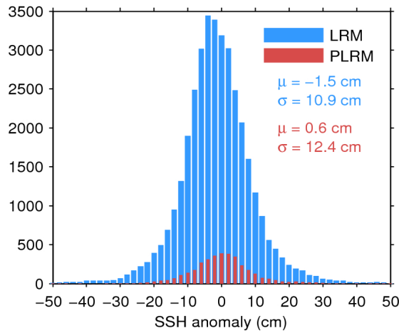
Figure 11. Histogram of science-valid SSH anomaly over oceans and lakes for LRM (blue) and PLRM (red) for 24/10/2016. The mean ( \mu ) and standard deviation ( \sigma ) are also shown. Note that values outside [-50\ 50] cm are excluded from the histogram for the sake of readability but not from the computation of \mu and \sigma .
