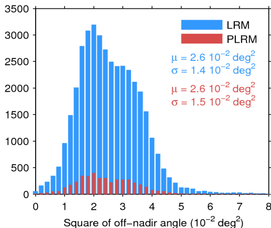
Figure 39. Histogram of flag-valid mispointing over oceans and lakes for LRM (blue) and PLRM (red) for 24/10/2016. Only positive values have been considered. The mean ( \mu ) and standard deviation ( \sigma ) are also shown. Note that values larger than 8 \cdot 10^{-2} \text{ deg}^2 are excluded from the histogram for the sake of readability but not from the computation of \mu and \sigma .
