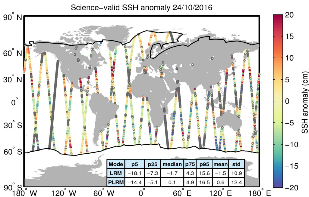
Figure 10. Geographical distribution of science-valid SSH anomaly data over oceans and lakes for 24/10/2016. The statistical values shown in the table refer to the SSH anomaly in cm and are calculated separately for LRM and PLRM regions. The black lines mark the outer limit of the Arctic and Antarctic polar polygons. Gray circles denote records that have been rejected based on the editing criteria described in Table 2.
