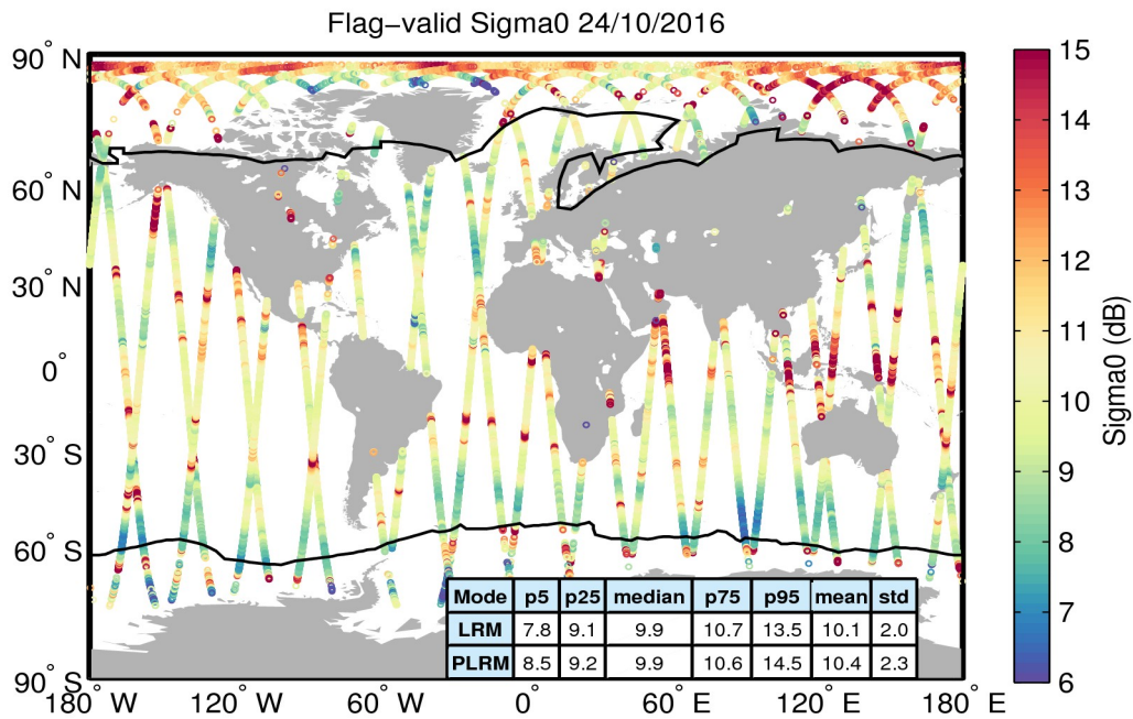
Figure 23. Geographical distribution of flag-valid sigma0 data over oceans and lakes for 24/10/2016. The statistical values shown in the table refer to the sigma0 in dB and are calculated separately for LRM and PLRM regions. Measurements taken over polar polygons have been excluded from the computation of the statistical values. The black lines mark the outer limit of the Arctic and Antarctic polar polygons.
