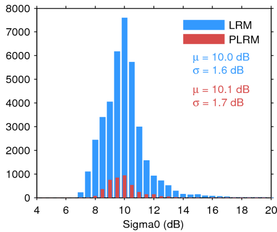
Figure 28. Histogram of science-valid sigma0 over oceans and lakes for LRM (blue) and PLRM (red) for 24/10/2016. The mean ( \mu ) and standard deviation ( \sigma ) are also shown. Note that values outside [4 20] dB are excluded from the histogram for the sake of readability but not from the computation of \mu and \sigma .
