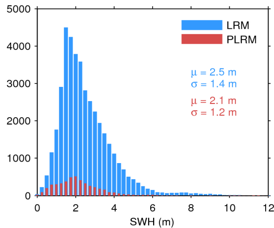
Figure 17. Histogram of flag-valid SWH over oceans and lakes for LRM (blue) and PLRM (red) for 24/10/2016. The mean ( \mu ) and standard deviation ( \sigma ) are also shown. Note that values larger than 12 m are excluded from the histogram for the sake of readability but not from the computation of \mu and \sigma .
