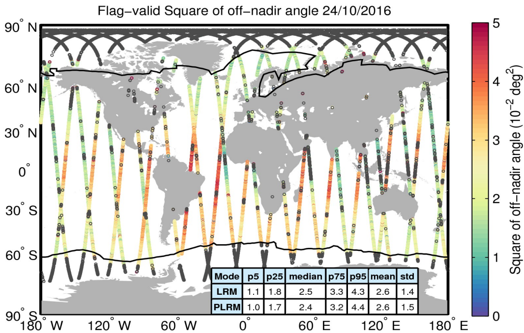
Figure 37. Geographical distribution of flag-valid mispointing data over oceans and lakes for 24/10/2016. The statistical values shown in the table refer to the mispointing in 10^{-2} \text{ deg}^2 and are calculated separately for LRM and PLRM regions. Measurements taken over polar polygons have been excluded from the computation of the statistical values. The black lines mark the outer limit of the Arctic and Antarctic polar polygons. Gray circles denote negative values.
