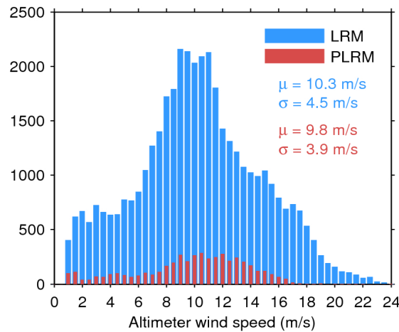
Figure 33. Histogram of flag-valid wind over oceans and lakes for LRM (blue) and PLRM (red) for 24/10/2016. The mean ( \mu ) and standard deviation ( \sigma ) are also shown. Note that values larger than 24 m/s are excluded from the histogram for the sake of readability but not from the computation of \mu and \sigma .
