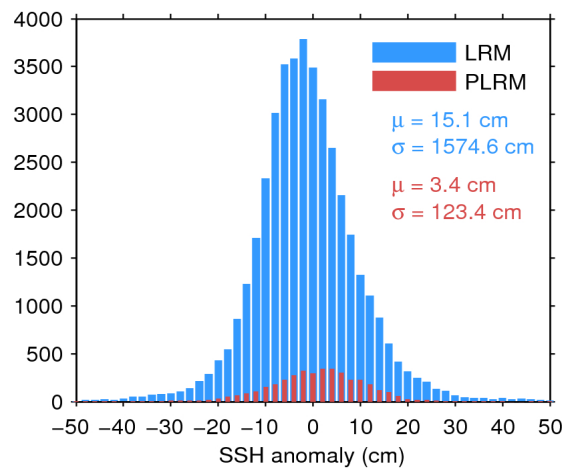
Figure 7. Histogram of flag-valid SSH anomaly over oceans and lakes for LRM (blue) and PLRM (red) for 23/10/2016. The mean ( \mu ) and standard deviation ( \sigma ) are also shown. Note that values outside [-50\ 50] cm are excluded from the histogram for the sake of readability but not from the computation of \mu and \sigma .
