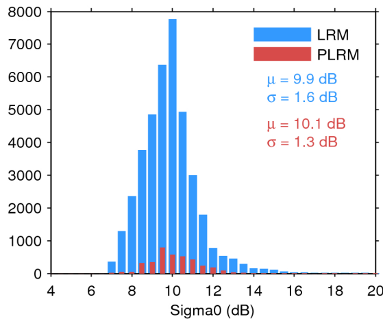
Figure 28. Histogram of science-valid sigma0 over oceans and lakes for LRM (blue) and PLRM (red) for 23/10/2016. The mean ( \mu ) and standard deviation ( \sigma ) are also shown. Note that values outside [4 20] dB are excluded from the histogram for the sake of readability but not from the computation of \mu and \sigma .
