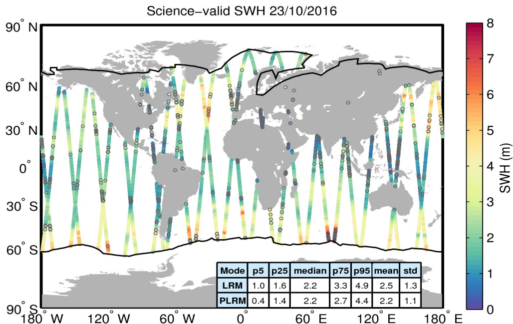
Figure 19. Geographical distribution of science-valid SWH data over oceans and lakes for 23/10/2016. The statistical values shown in the table refer to the SWH in m and are calculated separately for LRM and PLRM regions. The black lines mark the outer limit of the Arctic and Antarctic polar polygons. Gray circles denote records that have been rejected based on the editing criteria described in Table 3.
