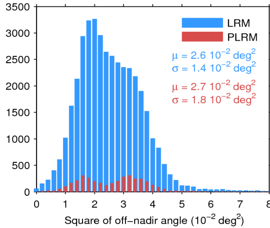
Figure 39. Histogram of flag-valid mispointing over oceans and lakes for LRM (blue) and PLRM (red) for 23/10/2016. Only positive values have been considered. The mean ( \mu ) and standard deviation ( \sigma ) are also shown. Note that values larger than 8 \cdot 10^{-2} \text{ deg}^2 are excluded from the histogram for the sake of readability but not from the computation of \mu and \sigma .
