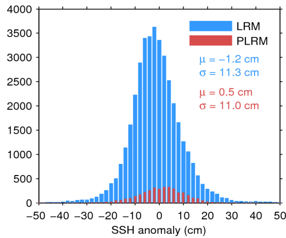
Figure 11. Histogram of science-valid SSH anomaly over oceans and lakes for LRM (blue) and PLRM (red) for 23/10/2016. The mean ( \mu ) and standard deviation ( \sigma ) are also shown. Note that values outside [-50 50] cm are excluded from the histogram for the sake of readability but not from the computation of \mu and \sigma .
