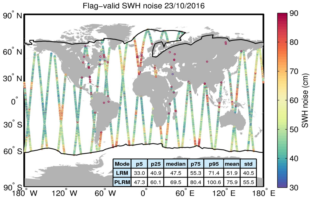
Figure 18. Geographical distribution of flag-valid 20-Hz SWH measurement noise over oceans and lakes for 23/10/2016. The statistical values shown in the table refer to the SWH noise and are calculated separately for LRM and PLRM regions. Measurements taken over polar polygons have been excluded from the computation of the statistical values. The black lines mark the outer limit of the Arctic and Antarctic polar polygons.
