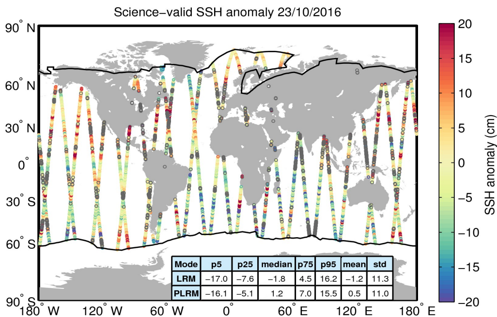
Figure 10. Geographical distribution of science-valid SSH anomaly data over oceans and lakes for 23/10/2016. The statistical values shown in the table refer to the SSH anomaly in cm and are calculated separately for LRM and PLRM regions. The black lines mark the outer limit of the Arctic and Antarctic polar polygons. Gray circles denote records that have been rejected based on the editing criteria described in Table 2.
