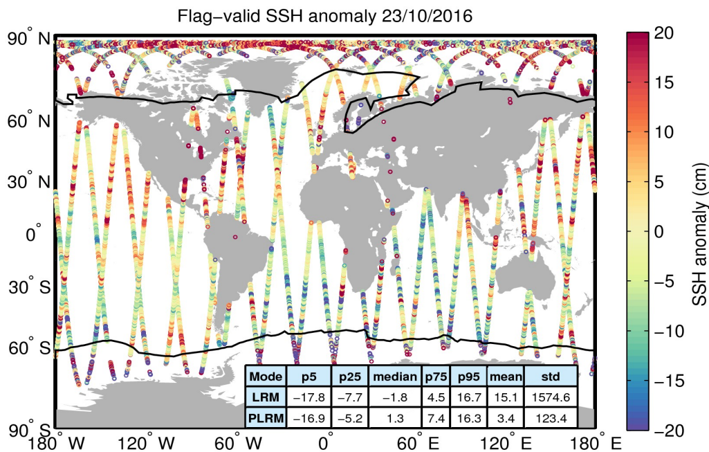
Figure 5. Geographical distribution of flag-valid 1-Hz SSH anomaly data over oceans and lakes for 23/10/2016. The statistical values shown in the table refer to the SSH anomaly in cm and are calculated separately for LRM and PLRM regions. Measurements taken over polar polygons have been excluded from the computation of the statistical values. The black lines mark the outer limit of the Arctic and Antarctic polar polygons.
