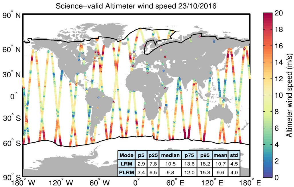
Figure 34. Geographical distribution of science-valid wind data over oceans and lakes for 23/10/2016. The statistical values shown in the table refer to the wind in m/s and are calculated separately for LRM and PLRM regions. The black lines mark the outer limit of the Arctic and Antarctic polar polygons. Gray circles denote records that have been rejected based on the editing criteria described in Table 5.
