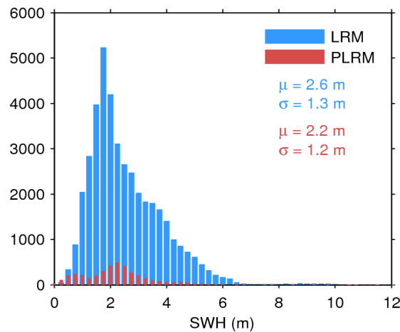
Figure 17. Histogram of flag-valid SWH over oceans and lakes for LRM (blue) and PLRM (red) for 23/10/2016. The mean ( \mu ) and standard deviation ( \sigma ) are also shown. Note that values larger than 12 m are excluded from the histogram for the sake of readability but not from the computation of \mu and \sigma .
