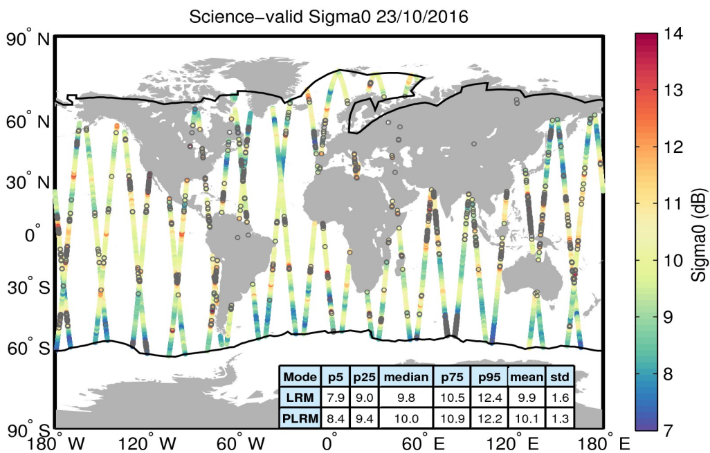
Figure 27. Geographical distribution of science-valid sigma0 data over oceans and lakes for 23/10/2016. The statistical values shown in the table refer to the sigma0 in dB and are calculated separately for LRM and PLRM regions. The black lines mark the outer limit of the Arctic and Antarctic polar polygons. Gray circles denote records that have been rejected based on the editing criteria described in Table 4.
