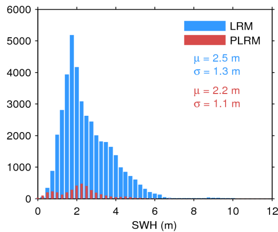
Figure 20. Histogram of science-valid SWH over oceans and lakes for LRM (blue) and PLRM (red) for 23/10/2016. The mean ( \mu ) and standard deviation ( \sigma ) are also shown. Note that values larger than 12 m are excluded from the histogram for the sake of readability but not from the computation of \mu and \sigma .
