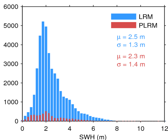
Figure 17. Histogram of flag-valid SWH over oceans and lakes for LRM (blue) and PLRM (red) for 22/10/2016. The mean ( \mu ) and standard deviation ( \sigma ) are also shown. Note that values larger than 12 m are excluded from the histogram for the sake of readability but not from the computation of \mu and \sigma .
