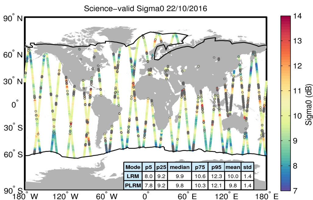
Figure 27. Geographical distribution of science-valid sigma0 data over oceans and lakes for 22/10/2016. The statistical values shown in the table refer to the sigma0 in dB and are calculated separately for LRM and PLRM regions. The black lines mark the outer limit of the Arctic and Antarctic polar polygons. Gray circles denote records that have been rejected based on the editing criteria described in Table 4.
