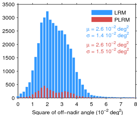
Figure 39. Histogram of flag-valid mispointing over oceans and lakes for LRM (blue) and PLRM (red) for 22/10/2016. Only positive values have been considered. The mean ( \mu ) and standard deviation ( \sigma ) are also shown. Note that values larger than 8 \cdot 10^{-2} \text{ deg}^2 are excluded from the histogram for the sake of readability but not from the computation of \mu and \sigma .
