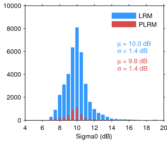
Figure 28. Histogram of science-valid sigma0 over oceans and lakes for LRM (blue) and PLRM (red) for 22/10/2016. The mean ( \mu ) and standard deviation ( \sigma ) are also shown. Note that values outside [4 20] dB are excluded from the histogram for the sake of readability but not from the computation of \mu and \sigma .
