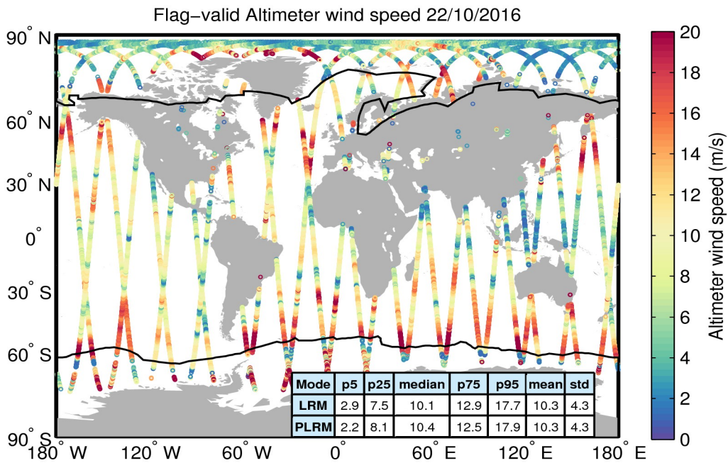
Figure 31. Geographical distribution of flag-valid wind data over oceans and lakes for 22/10/2016. The statistical values shown in the table refer to the wind in m/s and are calculated separately for LRM and PLRM regions. Measurements taken over polar polygons have been excluded from the computation of the statistical values. The black lines mark the outer limit of the Arctic and Antarctic polar polygons.
