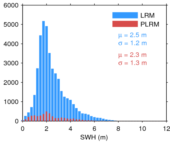
Figure 20. Histogram of science-valid SWH over oceans and lakes for LRM (blue) and PLRM (red) for 22/10/2016. The mean ( \mu ) and standard deviation ( \sigma ) are also shown. Note that values larger than 12 m are excluded from the histogram for the sake of readability but not from the computation of \mu and \sigma .
