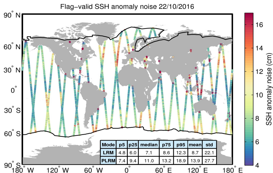
Figure 8. Geographical distribution of flag-valid 20-Hz SSH anomaly measurement noise over oceans and lakes for 22/10/2016. The statistical values shown in the table refer to the SSH anomaly noise and are calculated separately for LRM and PLRM regions. Measurements taken over polar polygons have been excluded from the computation of the statistical values. The black lines mark the outer limit of the Arctic and Antarctic polar polygons.
