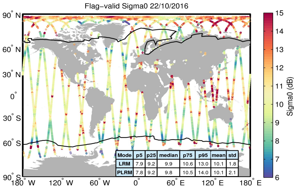
Figure 23. Geographical distribution of flag-valid sigma0 data over oceans and lakes for 22/10/2016. The statistical values shown in the table refer to the sigma0 in dB and are calculated separately for LRM and PLRM regions. Measurements taken over polar polygons have been excluded from the computation of the statistical values. The black lines mark the outer limit of the Arctic and Antarctic polar polygons.
