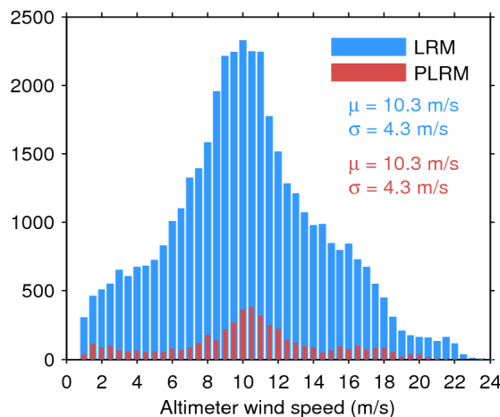
Figure 35. Histogram of science-valid wind over oceans and lakes for LRM (blue) and PLRM (red) for 22/10/2016. The mean ( \mu ) and standard deviation ( \sigma ) are also shown. Note that values larger than 24 m/s are excluded from the histogram for the sake of readability but not from the computation of \mu and \sigma .
