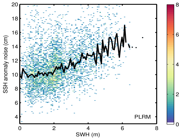
Figure 9. 2D histogram showing flag-valid SSH anomaly noise as a function of SWH for LRM (top) and PLRM (bottom) for 22/10/2016. The black line denotes the median SSH anomaly noise as a function of SWH.
