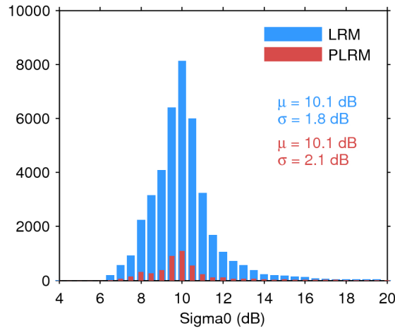
Figure 25. Histogram of flag-valid sigma0 over oceans and lakes for LRM (blue) and PLRM (red) for 22/10/2016. The mean ( \mu ) and standard deviation ( \sigma ) are also shown. Note that values outside [4 20] dB are excluded from the histogram for the sake of readability but not from the computation of \mu and \sigma .
