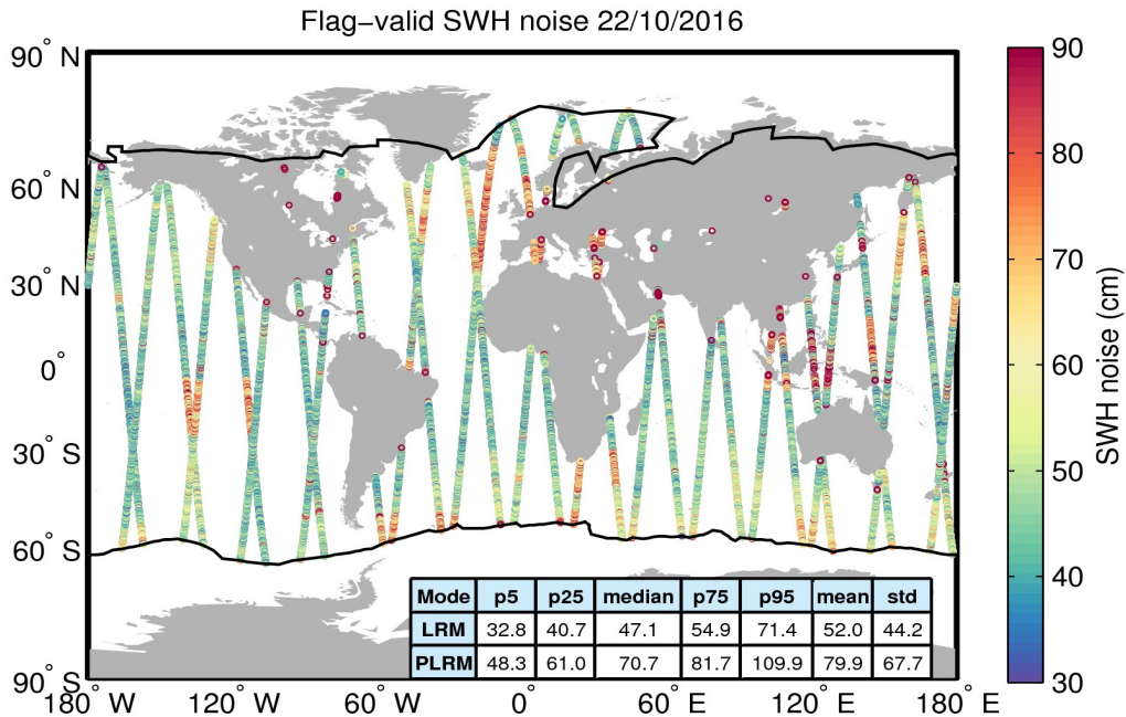
Figure 18. Geographical distribution of flag-valid 20-Hz SWH measurement noise over oceans and lakes for 22/10/2016. The statistical values shown in the table refer to the SWH noise and are calculated separately for LRM and PLRM regions. Measurements taken over polar polygons have been excluded from the computation of the statistical values. The black lines mark the outer limit of the Arctic and Antarctic polar polygons.
