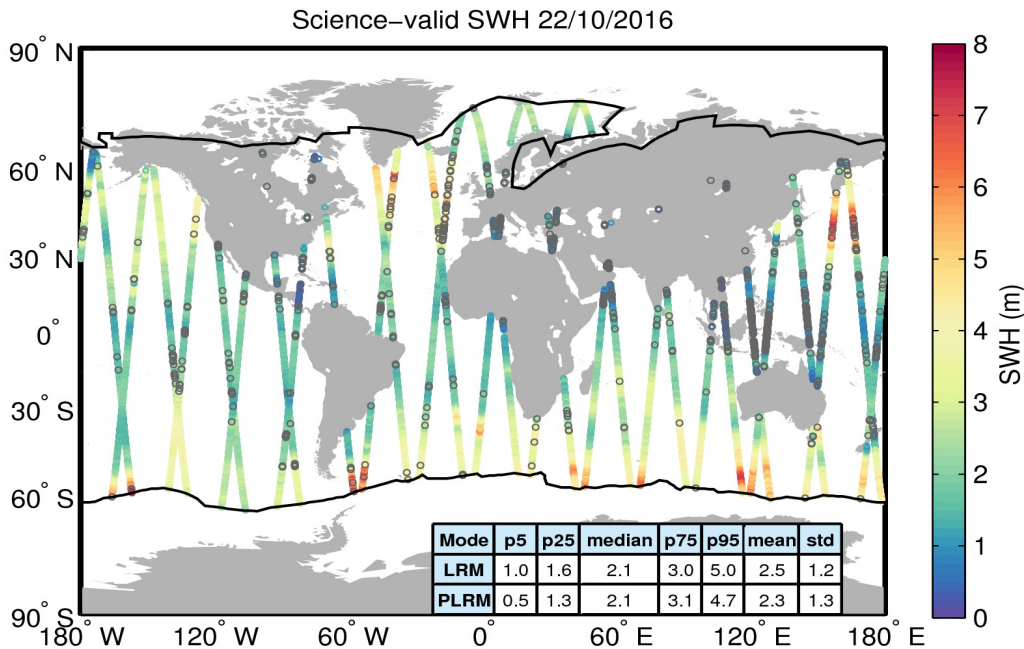
Figure 19. Geographical distribution of science-valid SWH data over oceans and lakes for 22/10/2016. The statistical values shown in the table refer to the SWH in m and are calculated separately for LRM and PLRM regions. The black lines mark the outer limit of the Arctic and Antarctic polar polygons. Gray circles denote records that have been rejected based on the editing criteria described in Table 3.
