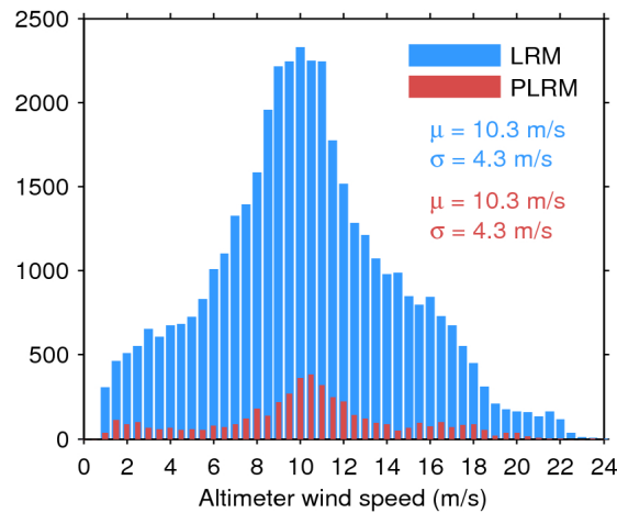
Figure 33. Histogram of flag-valid wind over oceans and lakes for LRM (blue) and PLRM (red) for 22/10/2016. The mean ( \mu ) and standard deviation ( \sigma ) are also shown. Note that values larger than 24 m/s are excluded from the histogram for the sake of readability but not from the computation of \mu and \sigma .
