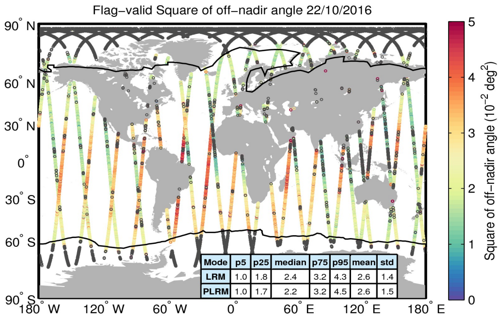
Figure 37. Geographical distribution of flag-valid mispointing data over oceans and lakes for 22/10/2016. The statistical values shown in the table refer to the mispointing in 10^{-2} \text{ deg}^2 and are calculated separately for LRM and PLRM regions. Measurements taken over polar polygons have been excluded from the computation of the statistical values. The black lines mark the outer limit of the Arctic and Antarctic polar polygons. Gray circles denote negative values.
