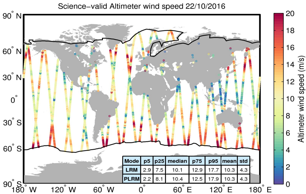
Figure 34. Geographical distribution of science-valid wind data over oceans and lakes for 22/10/2016. The statistical values shown in the table refer to the wind in m/s and are calculated separately for LRM and PLRM regions. The black lines mark the outer limit of the Arctic and Antarctic polar polygons. Gray circles denote records that have been rejected based on the editing criteria described in Table 5.
