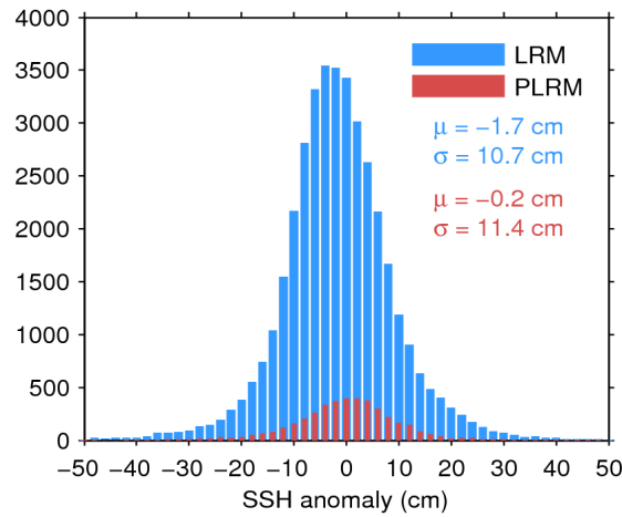
Figure 11. Histogram of science-valid SSH anomaly over oceans and lakes for LRM (blue) and PLRM (red) for 22/10/2016. The mean ( \mu ) and standard deviation ( \sigma ) are also shown. Note that values outside [-50\ 50] cm are excluded from the histogram for the sake of readability but not from the computation of \mu and \sigma .
