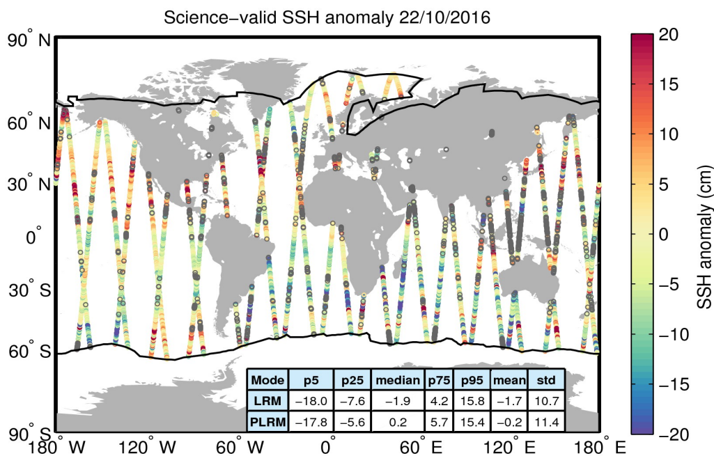
Figure 10. Geographical distribution of science-valid SSH anomaly data over oceans and lakes for 22/10/2016. The statistical values shown in the table refer to the SSH anomaly in cm and are calculated separately for LRM and PLRM regions. The black lines mark the outer limit of the Arctic and Antarctic polar polygons. Gray circles denote records that have been rejected based on the editing criteria described in Table 2.
