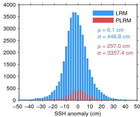
Figure 7. Histogram of flag-valid SSH anomaly over oceans and lakes for LRM (blue) and PLRM (red) for 22/10/2016. The mean ( \mu ) and standard deviation ( \sigma ) are also shown. Note that values outside [-50 50] cm are excluded from the histogram for the sake of readability but not from the computation of \mu and \sigma .
