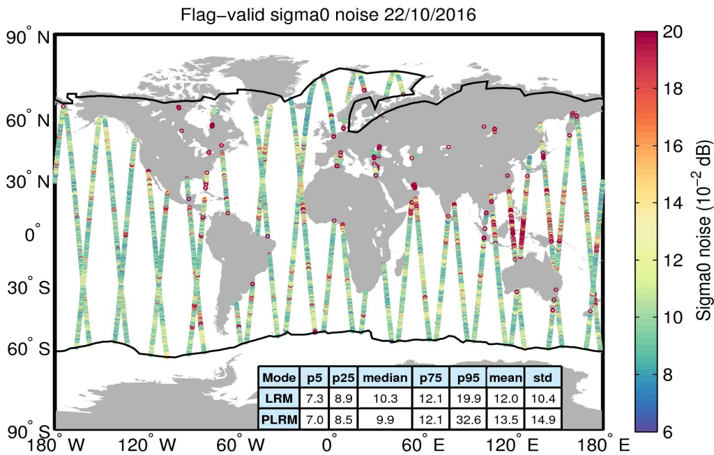
Figure 26. Geographical distribution of flag-valid 20-Hz sigma0 measurement noise over oceans and lakes for 22/10/2016. The statistical values shown in the table refer to the sigma0 noise and are calculated separately for LRM and PLRM regions. Measurements taken over polar polygons have been excluded from the computation of the statistical values. The black lines mark the outer limit of the Arctic and Antarctic polar polygons.
