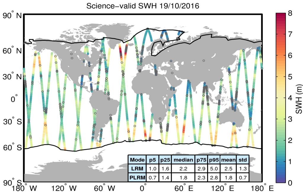
Figure 19. Geographical distribution of science-valid SWH data over oceans and lakes for 19/10/2016. The statistical values shown in the table refer to the SWH in m and are calculated separately for LRM and PLRM regions. The black lines mark the outer limit of the Arctic and Antarctic polar polygons. Gray circles denote records that have been rejected based on the editing criteria described in Table 3.
