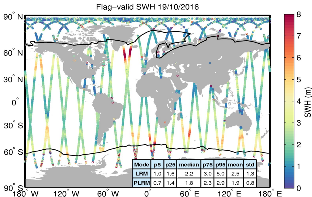
Figure 15. Geographical distribution of flag-valid SWH data over oceans and lakes for 19/10/2016. The statistical values shown in the table refer to the SWH in m and are calculated separately for LRM and PLRM regions. Measurements taken over polar polygons have been excluded from the computation of the statistical values. The black lines mark the outer limit of the Arctic and Antarctic polar polygons.
