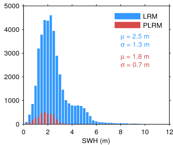
Figure 20. Histogram of science-valid SWH over oceans and lakes for LRM (blue) and PLRM (red) for 19/10/2016. The mean ( \mu ) and standard deviation ( \sigma ) are also shown. Note that values larger than 12 m are excluded from the histogram for the sake of readability but not from the computation of \mu and \sigma .
