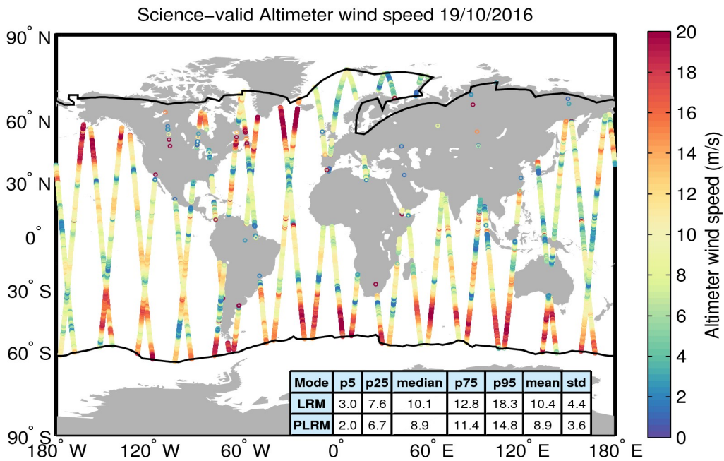
Figure 34. Geographical distribution of science-valid wind data over oceans and lakes for 19/10/2016. The statistical values shown in the table refer to the wind in m/s and are calculated separately for LRM and PLRM regions. The black lines mark the outer limit of the Arctic and Antarctic polar polygons. Gray circles denote records that have been rejected based on the editing criteria described in Table 5.
