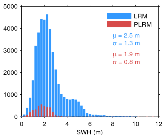
Figure 17. Histogram of flag-valid SWH over oceans and lakes for LRM (blue) and PLRM (red) for 19/10/2016. The mean ( \mu ) and standard deviation ( \sigma ) are also shown. Note that values larger than 12 m are excluded from the histogram for the sake of readability but not from the computation of \mu and \sigma .
