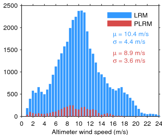
Figure 35. Histogram of science-valid wind over oceans and lakes for LRM (blue) and PLRM (red) for 19/10/2016. The mean ( \mu ) and standard deviation ( \sigma ) are also shown. Note that values larger than 24 m/s are excluded from the histogram for the sake of readability but not from the computation of \mu and \sigma .
