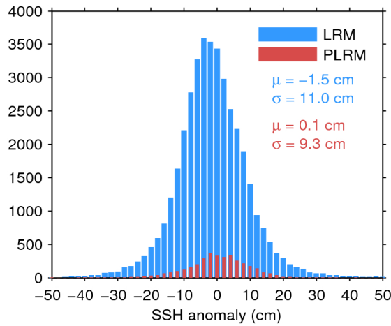
Figure 11. Histogram of science-valid SSH anomaly over oceans and lakes for LRM (blue) and PLRM (red) for 19/10/2016. The mean ( \mu ) and standard deviation ( \sigma ) are also shown. Note that values outside [-50 50] cm are excluded from the histogram for the sake of readability but not from the computation of \mu and \sigma .
