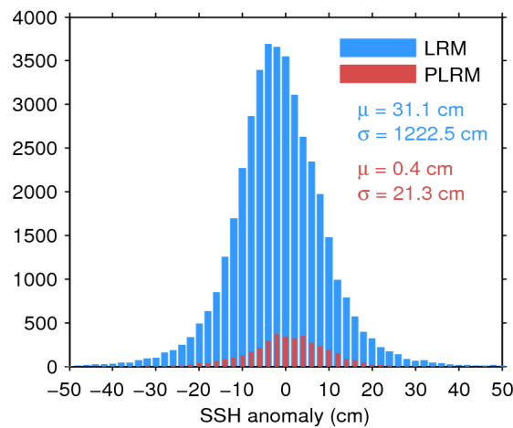
Figure 7. Histogram of flag-valid SSH anomaly over oceans and lakes for LRM (blue) and PLRM (red) for 19/10/2016. The mean ( \mu ) and standard deviation ( \sigma ) are also shown. Note that values outside [-50\ 50] cm are excluded from the histogram for the sake of readability but not from the computation of \mu and \sigma .
