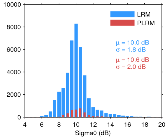
Figure 25. Histogram of flag-valid sigma0 over oceans and lakes for LRM (blue) and PLRM (red) for 19/10/2016. The mean ( \mu ) and standard deviation ( \sigma ) are also shown. Note that values outside [4 20] dB are excluded from the histogram for the sake of readability but not from the computation of \mu and \sigma .
