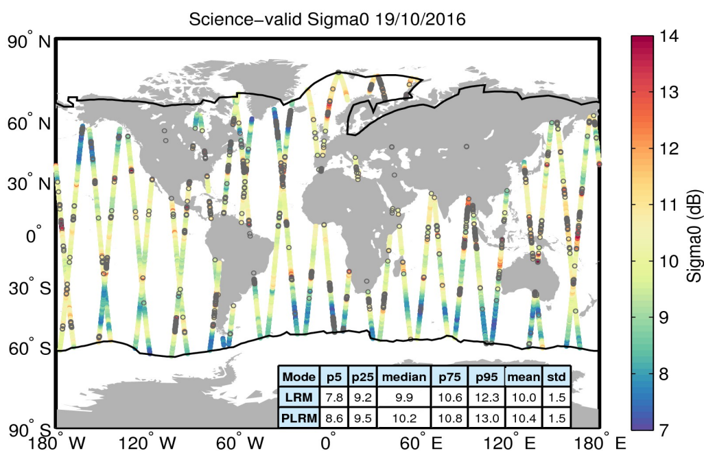
Figure 27. Geographical distribution of science-valid sigma0 data over oceans and lakes for 19/10/2016. The statistical values shown in the table refer to the sigma0 in dB and are calculated separately for LRM and PLRM regions. The black lines mark the outer limit of the Arctic and Antarctic polar polygons. Gray circles denote records that have been rejected based on the editing criteria described in Table 4.
