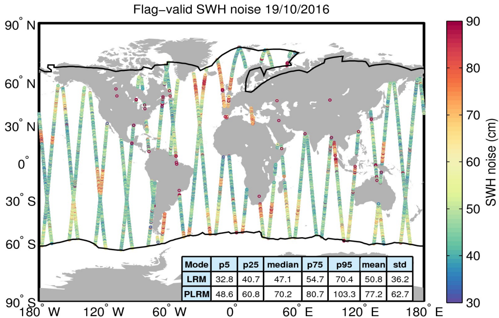
Figure 18. Geographical distribution of flag-valid 20-Hz SWH measurement noise over oceans and lakes for 19/10/2016. The statistical values shown in the table refer to the SWH noise and are calculated separately for LRM and PLRM regions. Measurements taken over polar polygons have been excluded from the computation of the statistical values. The black lines mark the outer limit of the Arctic and Antarctic polar polygons.
