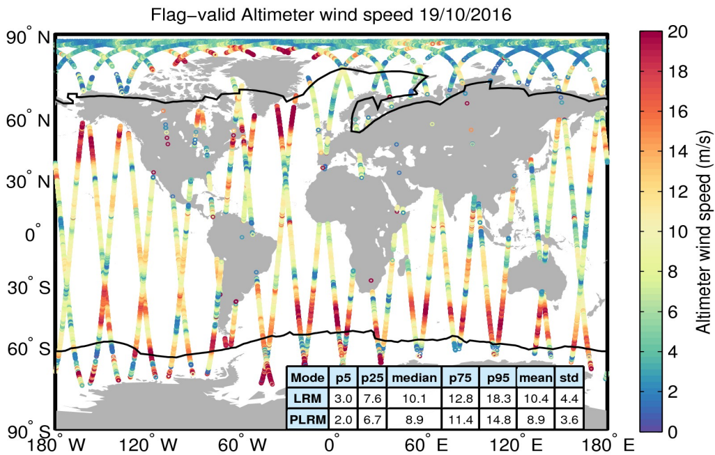
Figure 31. Geographical distribution of flag-valid wind data over oceans and lakes for 19/10/2016. The statistical values shown in the table refer to the wind in m/s and are calculated separately for LRM and PLRM regions. Measurements taken over polar polygons have been excluded from the computation of the statistical values. The black lines mark the outer limit of the Arctic and Antarctic polar polygons.
