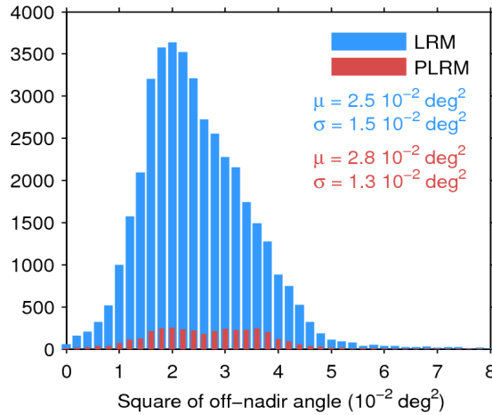
Figure 39. Histogram of flag-valid mispointing over oceans and lakes for LRM (blue) and PLRM (red) for 19/10/2016. Only positive values have been considered. The mean ( \mu ) and standard deviation ( \sigma ) are also shown. Note that values larger than 8 \cdot 10^{-2} \text{ deg}^2 are excluded from the histogram for the sake of readability but not from the computation of \mu and \sigma .
