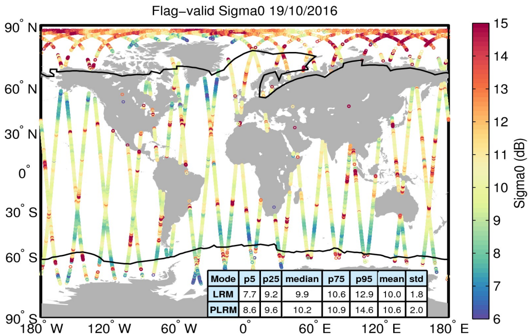
Figure 23. Geographical distribution of flag-valid sigma0 data over oceans and lakes for 19/10/2016. The statistical values shown in the table refer to the sigma0 in dB and are calculated separately for LRM and PLRM regions. Measurements taken over polar polygons have been excluded from the computation of the statistical values. The black lines mark the outer limit of the Arctic and Antarctic polar polygons.
