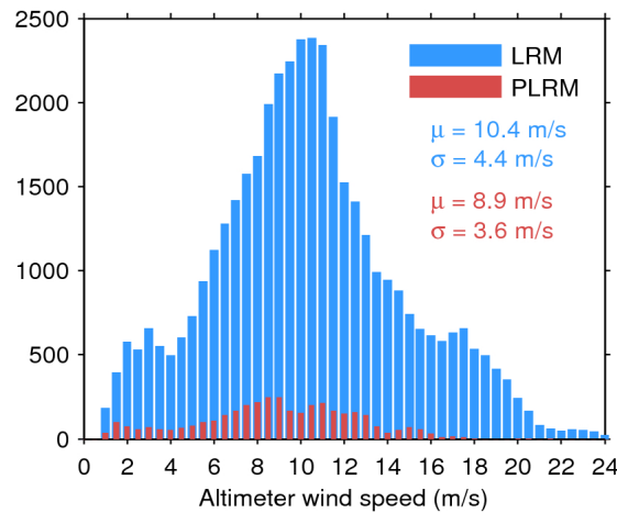
Figure 33. Histogram of flag-valid wind over oceans and lakes for LRM (blue) and PLRM (red) for 19/10/2016. The mean ( \mu ) and standard deviation ( \sigma ) are also shown. Note that values larger than 24 m/s are excluded from the histogram for the sake of readability but not from the computation of \mu and \sigma .
