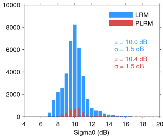
Figure 28. Histogram of science-valid sigma0 over oceans and lakes for LRM (blue) and PLRM (red) for 19/10/2016. The mean ( \mu ) and standard deviation ( \sigma ) are also shown. Note that values outside [4 20] dB are excluded from the histogram for the sake of readability but not from the computation of \mu and \sigma .
