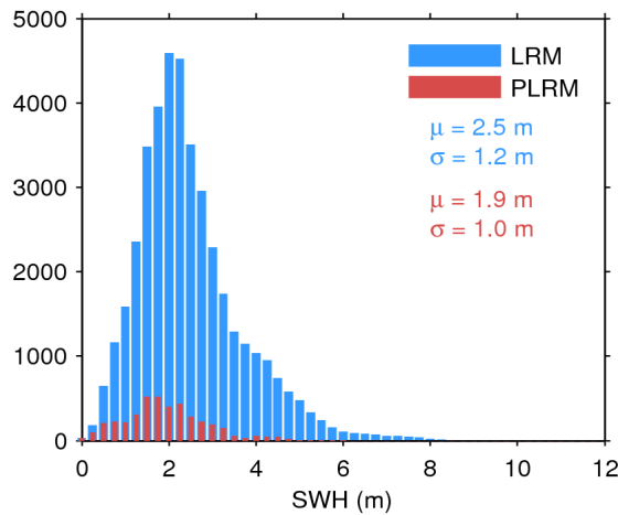
Figure 20. Histogram of science-valid SWH over oceans and lakes for LRM (blue) and PLRM (red) for 18/10/2016. The mean ( \mu ) and standard deviation ( \sigma ) are also shown. Note that values larger than 12 m are excluded from the histogram for the sake of readability but not from the computation of \mu and \sigma .
