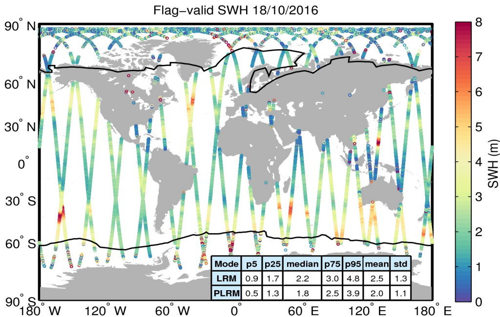
Figure 15. Geographical distribution of flag-valid SWH data over oceans and lakes for 18/10/2016. The statistical values shown in the table refer to the SWH in m and are calculated separately for LRM and PLRM regions. Measurements taken over polar polygons have been excluded from the computation of the statistical values. The black lines mark the outer limit of the Arctic and Antarctic polar polygons.
