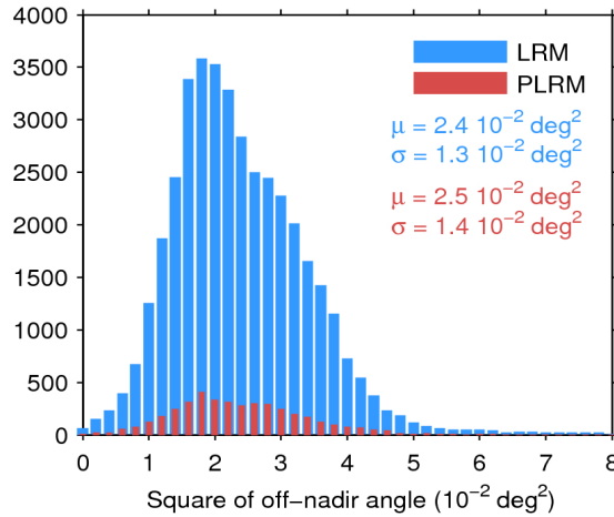
Figure 39. Histogram of flag-valid mispointing over oceans and lakes for LRM (blue) and PLRM (red) for 18/10/2016. Only positive values have been considered. The mean ( \mu ) and standard deviation ( \sigma ) are also shown. Note that values larger than 8 \cdot 10^{-2} \text{ deg}^2 are excluded from the histogram for the sake of readability but not from the computation of \mu and \sigma .
