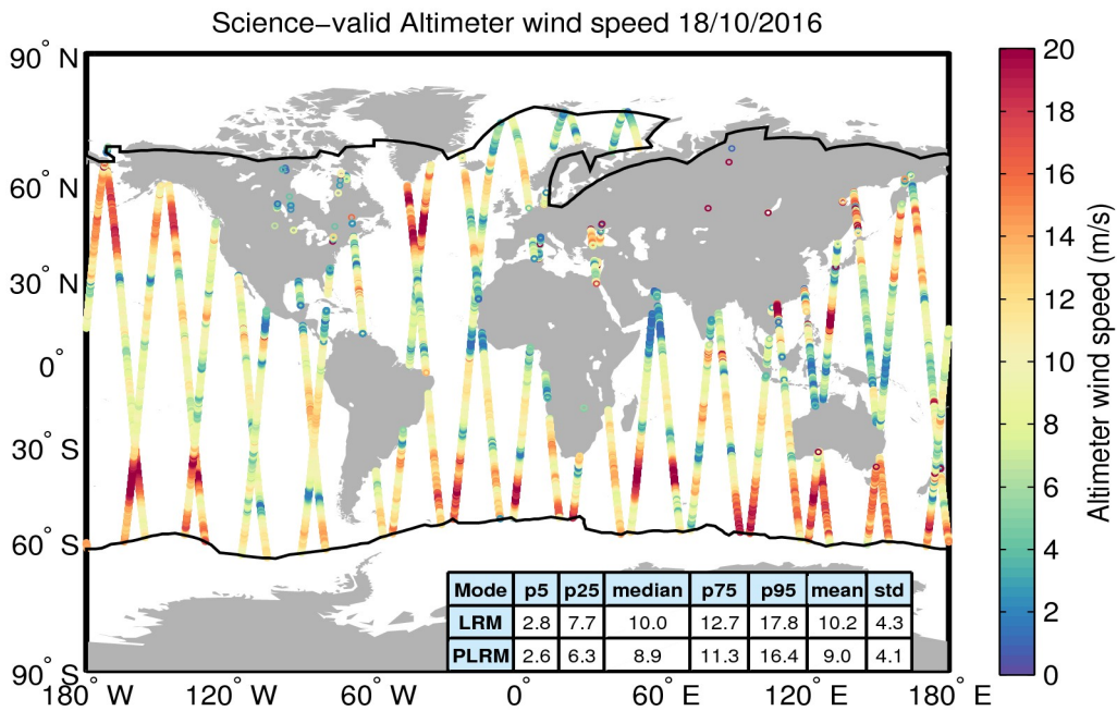
Figure 34. Geographical distribution of science-valid wind data over oceans and lakes for 18/10/2016. The statistical values shown in the table refer to the wind in m/s and are calculated separately for LRM and PLRM regions. The black lines mark the outer limit of the Arctic and Antarctic polar polygons. Gray circles denote records that have been rejected based on the editing criteria described in Table 5.
