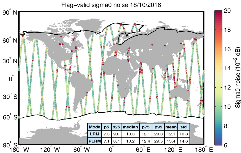
Figure 26. Geographical distribution of flag-valid 20-Hz sigma0 measurement noise over oceans and lakes for 18/10/2016. The statistical values shown in the table refer to the sigma0 noise and are calculated separately for LRM and PLRM regions. Measurements taken over polar polygons have been excluded from the computation of the statistical values. The black lines mark the outer limit of the Arctic and Antarctic polar polygons.
