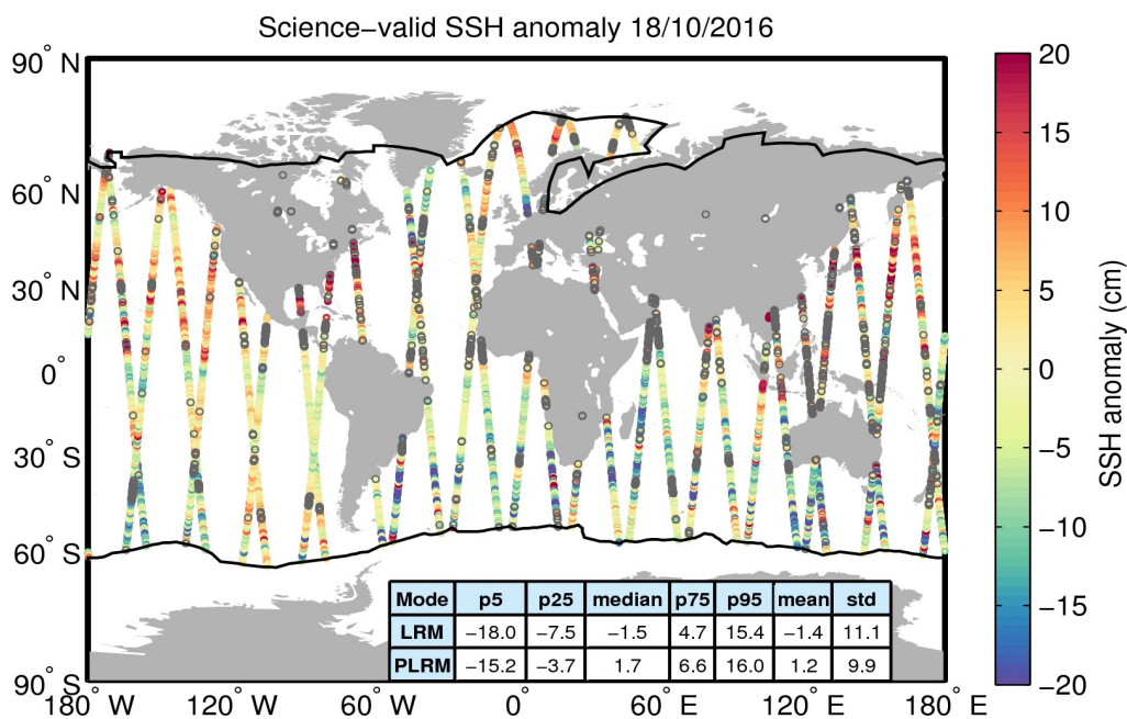
Figure 10. Geographical distribution of science-valid SSH anomaly data over oceans and lakes for 18/10/2016. The statistical values shown in the table refer to the SSH anomaly in cm and are calculated separately for LRM and PLRM regions. The black lines mark the outer limit of the Arctic and Antarctic polar polygons. Gray circles denote records that have been rejected based on the editing criteria described in Table 2.
