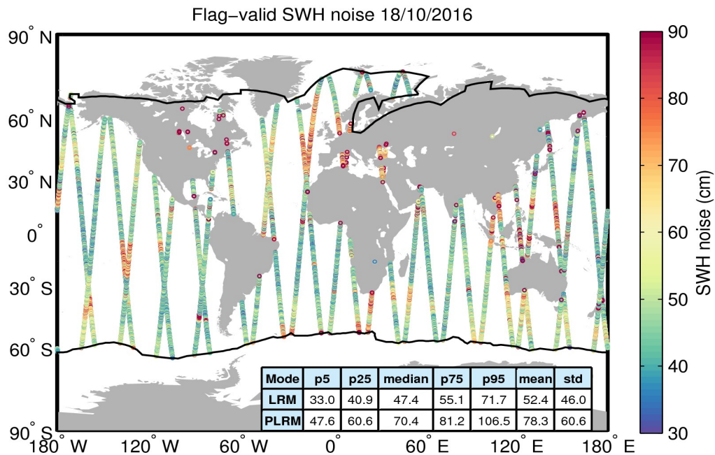
Figure 18. Geographical distribution of flag-valid 20-Hz SWH measurement noise over oceans and lakes for 18/10/2016. The statistical values shown in the table refer to the SWH noise and are calculated separately for LRM and PLRM regions. Measurements taken over polar polygons have been excluded from the computation of the statistical values. The black lines mark the outer limit of the Arctic and Antarctic polar polygons.
