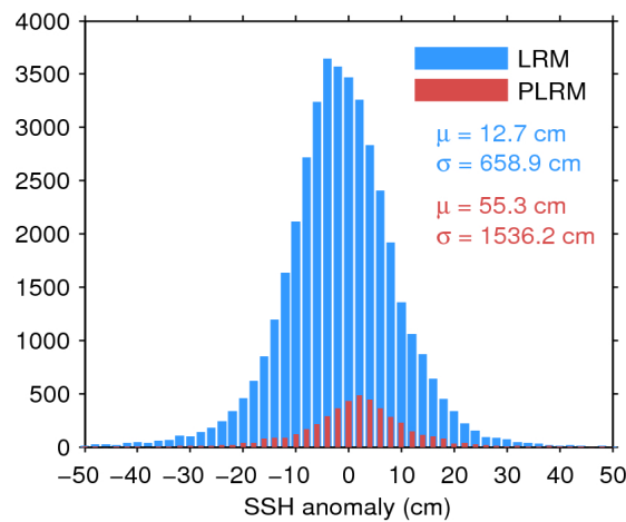
Figure 7. Histogram of flag-valid SSH anomaly over oceans and lakes for LRM (blue) and PLRM (red) for 18/10/2016. The mean ( \mu ) and standard deviation ( \sigma ) are also shown. Note that values outside [-50 \ 50] cm are excluded from the histogram for the sake of readability but not from the computation of \mu and \sigma .
