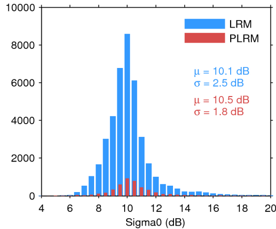
Figure 25. Histogram of flag-valid sigma0 over oceans and lakes for LRM (blue) and PLRM (red) for 18/10/2016. The mean ( \mu ) and standard deviation ( \sigma ) are also shown. Note that values outside [4 20] dB are excluded from the histogram for the sake of readability but not from the computation of \mu and \sigma .
