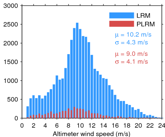
Figure 35. Histogram of science-valid wind over oceans and lakes for LRM (blue) and PLRM (red) for 18/10/2016. The mean ( \mu ) and standard deviation ( \sigma ) are also shown. Note that values larger than 24 m/s are excluded from the histogram for the sake of readability but not from the computation of \mu and \sigma .
