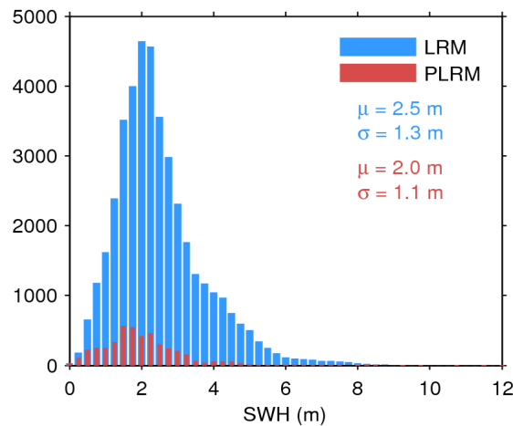
Figure 17. Histogram of flag-valid SWH over oceans and lakes for LRM (blue) and PLRM (red) for 18/10/2016. The mean ( \mu ) and standard deviation ( \sigma ) are also shown. Note that values larger than 12 m are excluded from the histogram for the sake of readability but not from the computation of \mu and \sigma .
