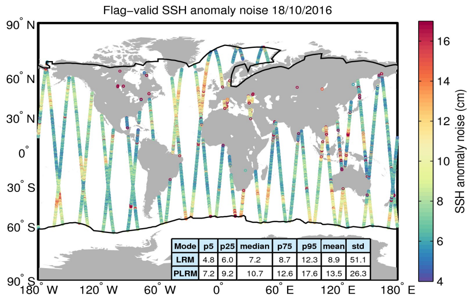
Figure 8. Geographical distribution of flag-valid 20-Hz SSH anomaly measurement noise over oceans and lakes for 18/10/2016. The statistical values shown in the table refer to the SSH anomaly noise and are calculated separately for LRM and PLRM regions. Measurements taken over polar polygons have been excluded from the computation of the statistical values. The black lines mark the outer limit of the Arctic and Antarctic polar polygons.
