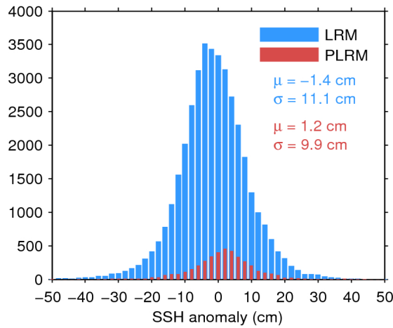
Figure 11. Histogram of science-valid SSH anomaly over oceans and lakes for LRM (blue) and PLRM (red) for 18/10/2016. The mean ( \mu ) and standard deviation ( \sigma ) are also shown. Note that values outside [-50\ 50] cm are excluded from the histogram for the sake of readability but not from the computation of \mu and \sigma .
