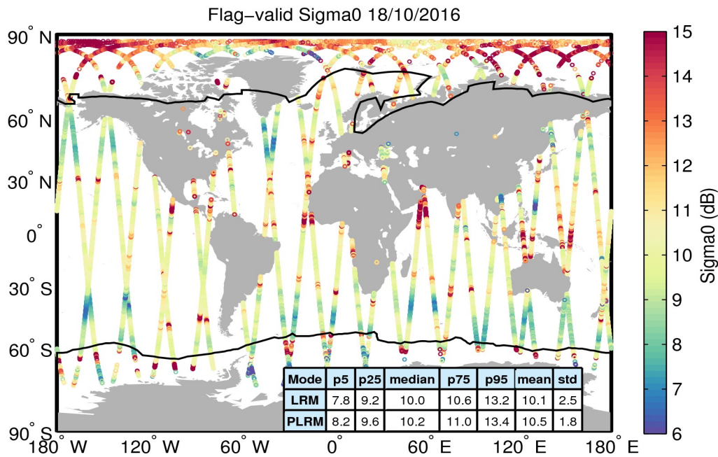
Figure 23. Geographical distribution of flag-valid sigma0 data over oceans and lakes for 18/10/2016. The statistical values shown in the table refer to the sigma0 in dB and are calculated separately for LRM and PLRM regions. Measurements taken over polar polygons have been excluded from the computation of the statistical values. The black lines mark the outer limit of the Arctic and Antarctic polar polygons.
