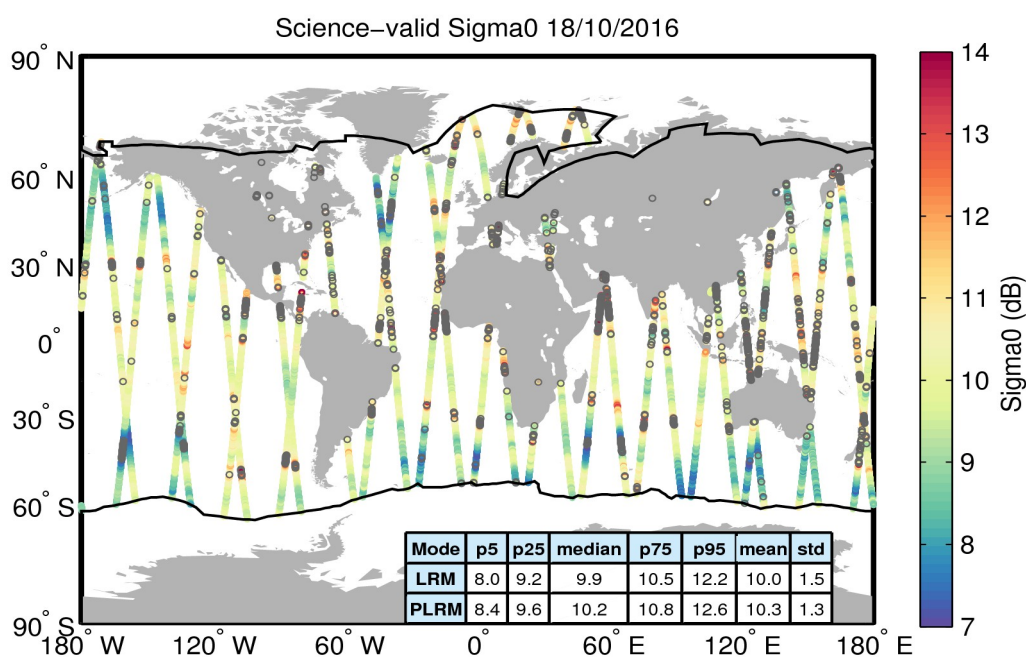
Figure 27. Geographical distribution of science-valid sigma0 data over oceans and lakes for 18/10/2016. The statistical values shown in the table refer to the sigma0 in dB and are calculated separately for LRM and PLRM regions. The black lines mark the outer limit of the Arctic and Antarctic polar polygons. Gray circles denote records that have been rejected based on the editing criteria described in Table 4.
