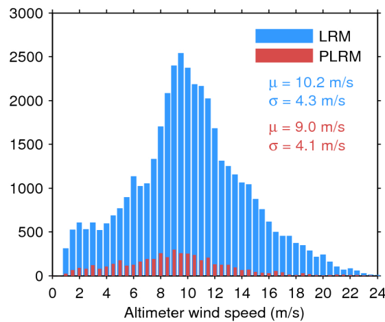
Figure 33. Histogram of flag-valid wind over oceans and lakes for LRM (blue) and PLRM (red) for 18/10/2016. The mean ( \mu ) and standard deviation ( \sigma ) are also shown. Note that values larger than 24 m/s are excluded from the histogram for the sake of readability but not from the computation of \mu and \sigma .
