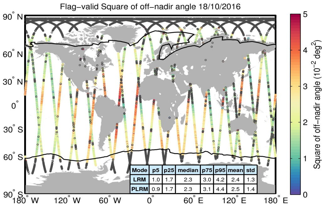
Figure 37. Geographical distribution of flag-valid mispointing data over oceans and lakes for 18/10/2016. The statistical values shown in the table refer to the mispointing in 10^{-2} deg 2 and are calculated separately for LRM and PLRM regions. Measurements taken over polar polygons have been excluded from the computation of the statistical values. The black lines mark the outer limit of the Arctic and Antarctic polar polygons. Gray circles denote negative values.
