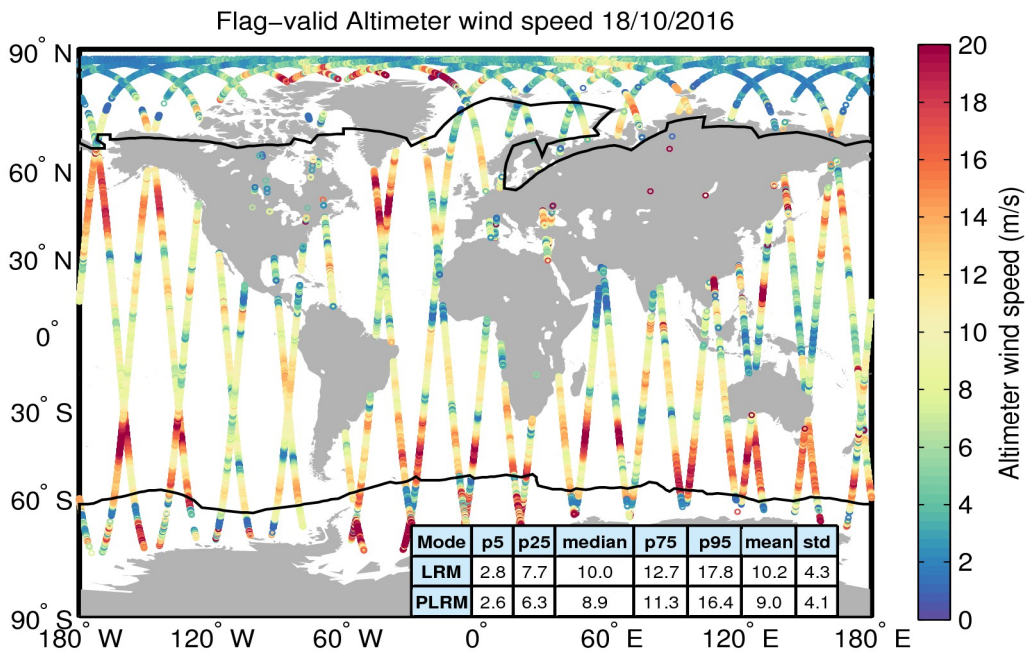
Figure 31. Geographical distribution of flag-valid wind data over oceans and lakes for 18/10/2016. The statistical values shown in the table refer to the wind in m/s and are calculated separately for LRM and PLRM regions. Measurements taken over polar polygons have been excluded from the computation of the statistical values. The black lines mark the outer limit of the Arctic and Antarctic polar polygons.
