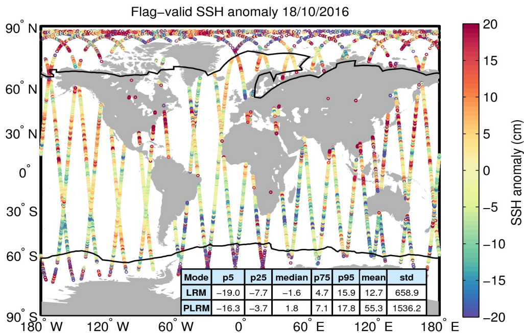
Figure 5. Geographical distribution of flag-valid 1-Hz SSH anomaly data over oceans and lakes for 18/10/2016. The statistical values shown in the table refer to the SSH anomaly in cm and are calculated separately for LRM and PLRM regions. Measurements taken over polar polygons have been excluded from the computation of the statistical values. The black lines mark the outer limit of the Arctic and Antarctic polar polygons.
