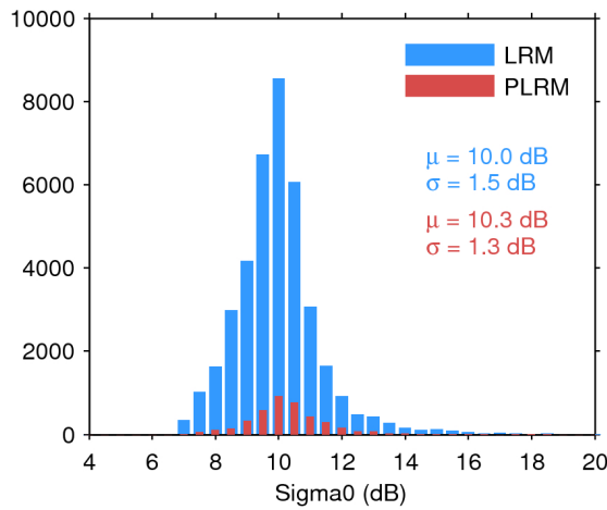
Figure 28. Histogram of science-valid sigma0 over oceans and lakes for LRM (blue) and PLRM (red) for 18/10/2016. The mean ( \mu ) and standard deviation ( \sigma ) are also shown. Note that values outside [4 20] dB are excluded from the histogram for the sake of readability but not from the computation of \mu and \sigma .
