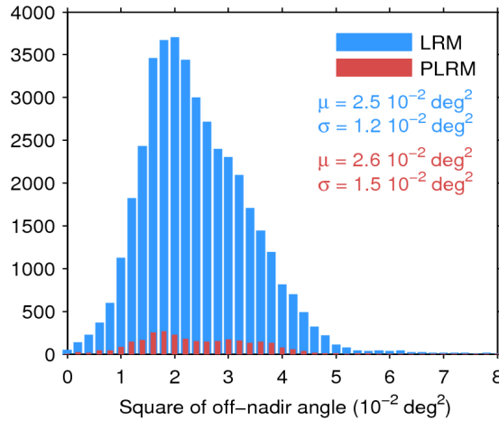
Figure 39. Histogram of flag-valid mispointing over oceans and lakes for LRM (blue) and PLRM (red) for 17/10/2016. Only positive values have been considered. The mean ( \mu ) and standard deviation ( \sigma ) are also shown. Note that values larger than 8 \cdot 10^{-2} \text{ deg}^2 are excluded from the histogram for the sake of readability but not from the computation of \mu and \sigma .
