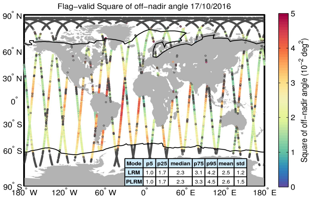
Figure 37. Geographical distribution of flag-valid mispointing data over oceans and lakes for 17/10/2016. The statistical values shown in the table refer to the mispointing in 10^{-2} deg 2 and are calculated separately for LRM and PLRM regions. Measurements taken over polar polygons have been excluded from the computation of the statistical values. The black lines mark the outer limit of the Arctic and Antarctic polar polygons. Gray circles denote negative values.
