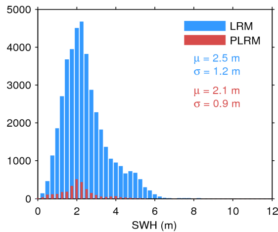
Figure 20. Histogram of science-valid SWH over oceans and lakes for LRM (blue) and PLRM (red) for 17/10/2016. The mean ( \mu ) and standard deviation ( \sigma ) are also shown. Note that values larger than 12 m are excluded from the histogram for the sake of readability but not from the computation of \mu and \sigma .
