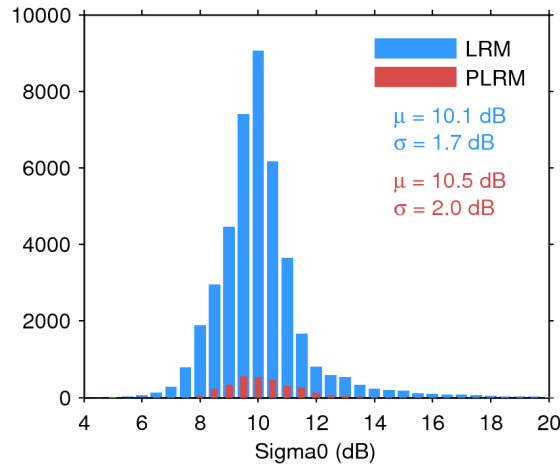
Figure 25. Histogram of flag-valid sigma0 over oceans and lakes for LRM (blue) and PLRM (red) for 17/10/2016. The mean ( \mu ) and standard deviation ( \sigma ) are also shown. Note that values outside [4 20] dB are excluded from the histogram for the sake of readability but not from the computation of \mu and \sigma .
