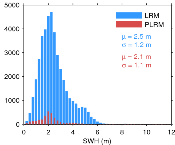
Figure 17. Histogram of flag-valid SWH over oceans and lakes for LRM (blue) and PLRM (red) for 17/10/2016. The mean ( \mu ) and standard deviation ( \sigma ) are also shown. Note that values larger than 12 m are excluded from the histogram for the sake of readability but not from the computation of \mu and \sigma .
