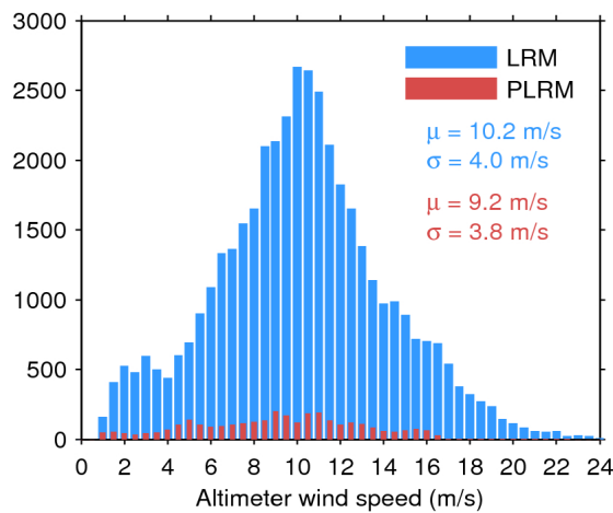
Figure 33. Histogram of flag-valid wind over oceans and lakes for LRM (blue) and PLRM (red) for 17/10/2016. The mean ( \mu ) and standard deviation ( \sigma ) are also shown. Note that values larger than 24 m/s are excluded from the histogram for the sake of readability but not from the computation of \mu and \sigma .
