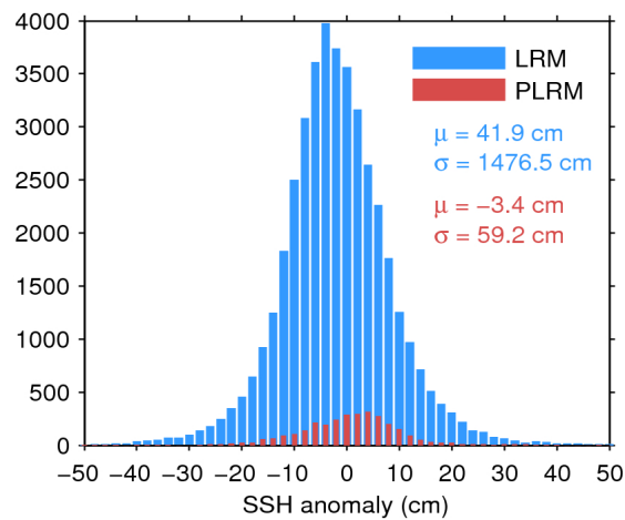
Figure 7. Histogram of flag-valid SSH anomaly over oceans and lakes for LRM (blue) and PLRM (red) for 17/10/2016. The mean ( \mu ) and standard deviation ( \sigma ) are also shown. Note that values outside [-50\ 50] cm are excluded from the histogram for the sake of readability but not from the computation of \mu and \sigma .
