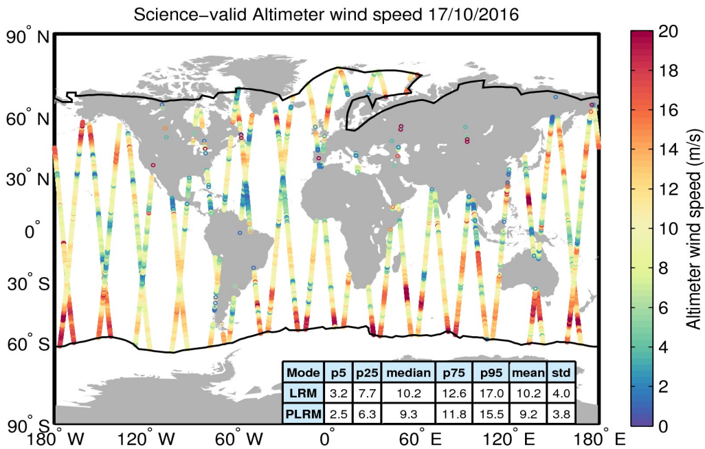
Figure 34. Geographical distribution of science-valid wind data over oceans and lakes for 17/10/2016. The statistical values shown in the table refer to the wind in m/s and are calculated separately for LRM and PLRM regions. The black lines mark the outer limit of the Arctic and Antarctic polar polygons. Gray circles denote records that have been rejected based on the editing criteria described in Table 5.
