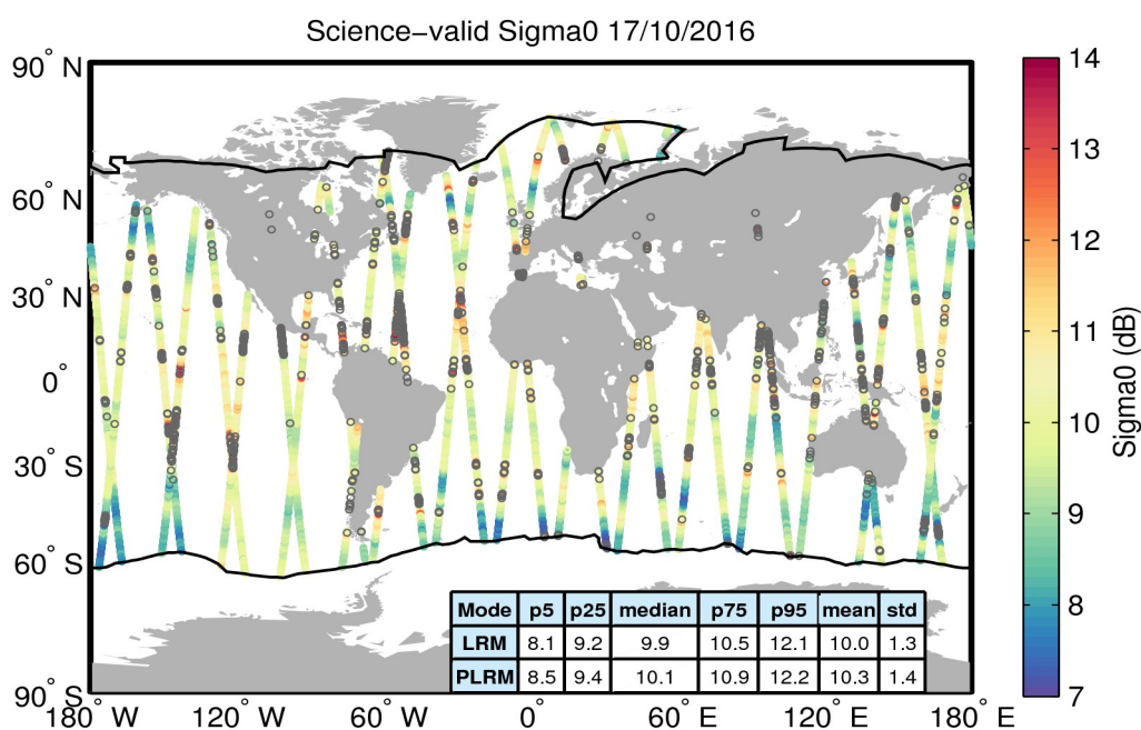
Figure 27. Geographical distribution of science-valid sigma0 data over oceans and lakes for 17/10/2016. The statistical values shown in the table refer to the sigma0 in dB and are calculated separately for LRM and PLRM regions. The black lines mark the outer limit of the Arctic and Antarctic polar polygons. Gray circles denote records that have been rejected based on the editing criteria described in Table 4.
