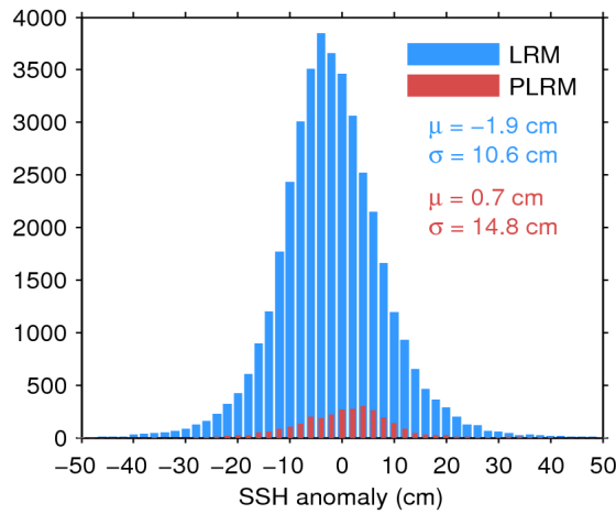
Figure 11. Histogram of science-valid SSH anomaly over oceans and lakes for LRM (blue) and PLRM (red) for 17/10/2016. The mean ( \mu ) and standard deviation ( \sigma ) are also shown. Note that values outside [-50 50] cm are excluded from the histogram for the sake of readability but not from the computation of \mu and \sigma .
