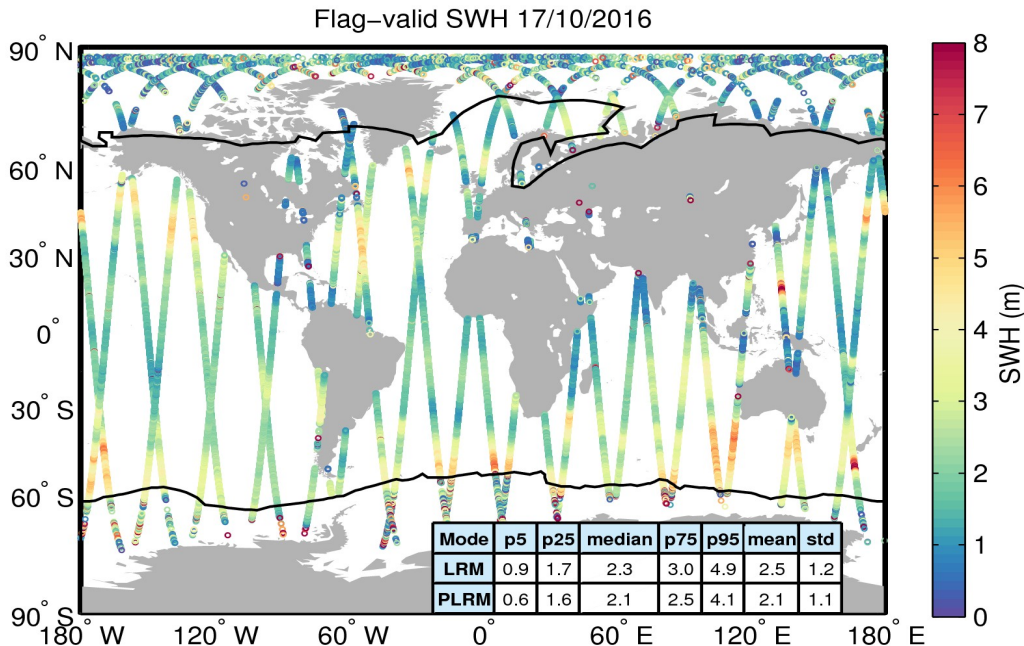
Figure 15. Geographical distribution of flag-valid SWH data over oceans and lakes for 17/10/2016. The statistical values shown in the table refer to the SWH in m and are calculated separately for LRM and PLRM regions. Measurements taken over polar polygons have been excluded from the computation of the statistical values. The black lines mark the outer limit of the Arctic and Antarctic polar polygons.
