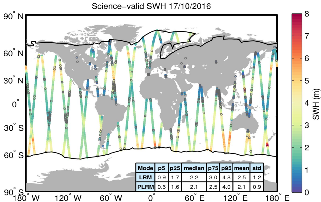
Figure 19. Geographical distribution of science-valid SWH data over oceans and lakes for 17/10/2016. The statistical values shown in the table refer to the SWH in m and are calculated separately for LRM and PLRM regions. The black lines mark the outer limit of the Arctic and Antarctic polar polygons. Gray circles denote records that have been rejected based on the editing criteria described in Table 3.
