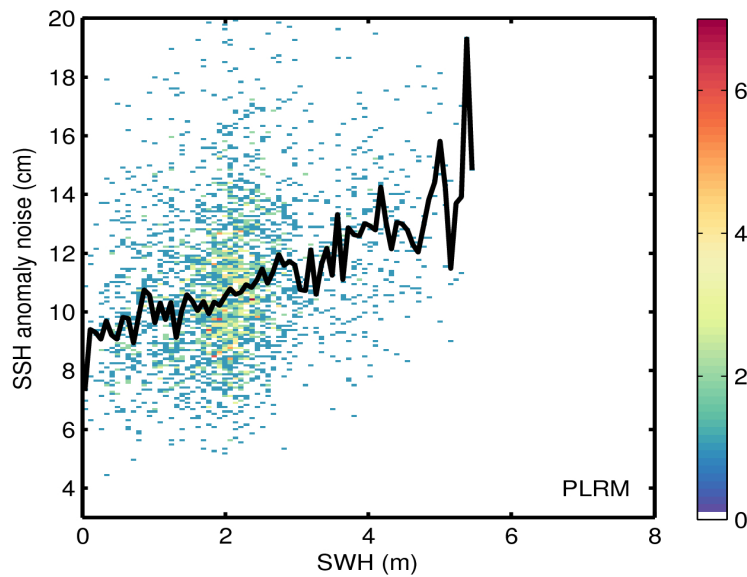
Figure 9. 2D histogram showing flag-valid SSH anomaly noise as a function of SWH for LRM (top) and PLRM (bottom) for 17/10/2016. The black line denotes the median SSH anomaly noise as a function of SWH.
