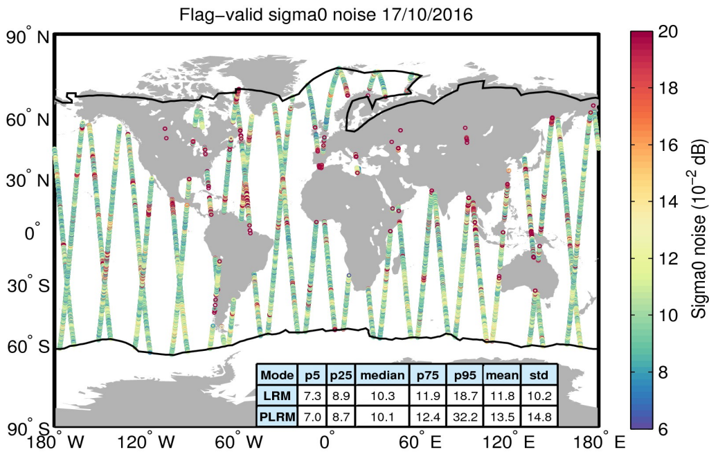
Figure 26. Geographical distribution of flag-valid 20-Hz sigma0 measurement noise over oceans and lakes for 17/10/2016. The statistical values shown in the table refer to the sigma0 noise and are calculated separately for LRM and PLRM regions. Measurements taken over polar polygons have been excluded from the computation of the statistical values. The black lines mark the outer limit of the Arctic and Antarctic polar polygons.
