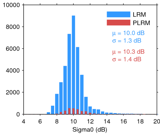
Figure 28. Histogram of science-valid sigma0 over oceans and lakes for LRM (blue) and PLRM (red) for 17/10/2016. The mean ( \mu ) and standard deviation ( \sigma ) are also shown. Note that values outside [4 20] dB are excluded from the histogram for the sake of readability but not from the computation of \mu and \sigma .
