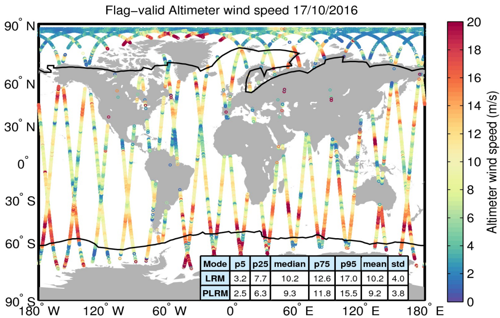
Figure 31. Geographical distribution of flag-valid wind data over oceans and lakes for 17/10/2016. The statistical values shown in the table refer to the wind in m/s and are calculated separately for LRM and PLRM regions. Measurements taken over polar polygons have been excluded from the computation of the statistical values. The black lines mark the outer limit of the Arctic and Antarctic polar polygons.
