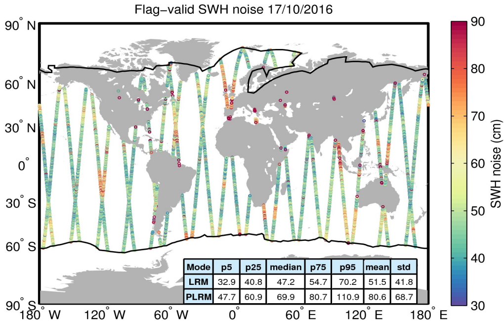
Figure 18. Geographical distribution of flag-valid 20-Hz SWH measurement noise over oceans and lakes for 17/10/2016. The statistical values shown in the table refer to the SWH noise and are calculated separately for LRM and PLRM regions. Measurements taken over polar polygons have been excluded from the computation of the statistical values. The black lines mark the outer limit of the Arctic and Antarctic polar polygons.
