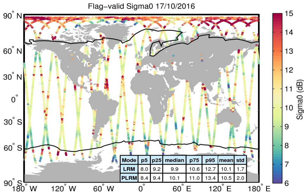
Figure 23. Geographical distribution of flag-valid sigma0 data over oceans and lakes for 17/10/2016. The statistical values shown in the table refer to the sigma0 in dB and are calculated separately for LRM and PLRM regions. Measurements taken over polar polygons have been excluded from the computation of the statistical values. The black lines mark the outer limit of the Arctic and Antarctic polar polygons.
