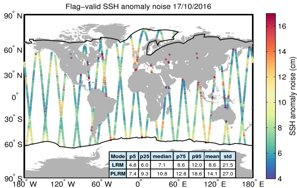
Figure 8. Geographical distribution of flag-valid 20-Hz SSH anomaly measurement noise over oceans and lakes for 17/10/2016. The statistical values shown in the table refer to the SSH anomaly noise and are calculated separately for LRM and PLRM regions. Measurements taken over polar polygons have been excluded from the computation of the statistical values. The black lines mark the outer limit of the Arctic and Antarctic polar polygons.
