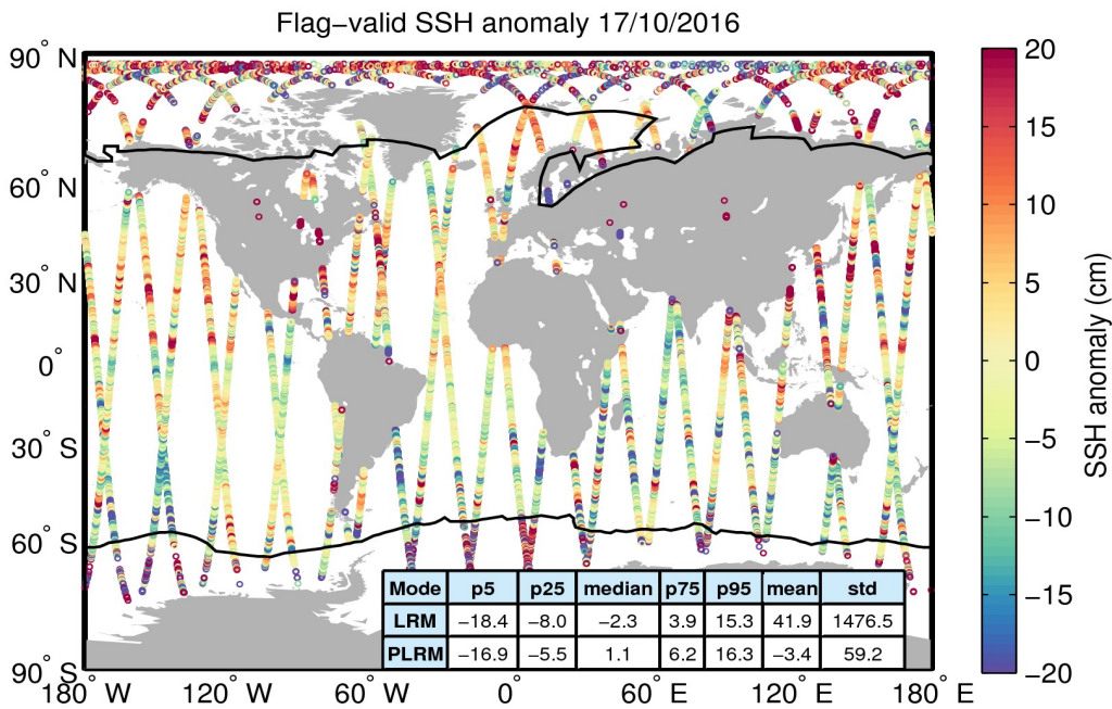
Figure 5. Geographical distribution of flag-valid 1-Hz SSH anomaly data over oceans and lakes for 17/10/2016. The statistical values shown in the table refer to the SSH anomaly in cm and are calculated separately for LRM and PLRM regions. Measurements taken over polar polygons have been excluded from the computation of the statistical values. The black lines mark the outer limit of the Arctic and Antarctic polar polygons.
