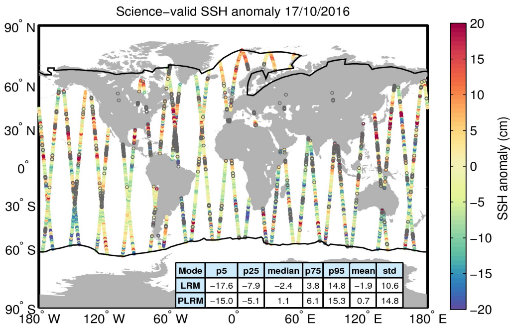
Figure 10. Geographical distribution of science-valid SSH anomaly data over oceans and lakes for 17/10/2016. The statistical values shown in the table refer to the SSH anomaly in cm and are calculated separately for LRM and PLRM regions. The black lines mark the outer limit of the Arctic and Antarctic polar polygons. Gray circles denote records that have been rejected based on the editing criteria described in Table 2.
