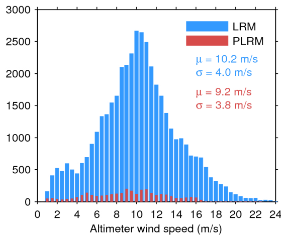
Figure 35. Histogram of science-valid wind over oceans and lakes for LRM (blue) and PLRM (red) for 17/10/2016. The mean ( \mu ) and standard deviation ( \sigma ) are also shown. Note that values larger than 24 m/s are excluded from the histogram for the sake of readability but not from the computation of \mu and \sigma .
