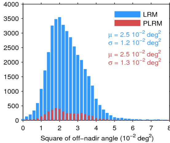
Figure 39. Histogram of flag-valid mispointing over oceans and lakes for LRM (blue) and PLRM (red) for 16/10/2016. Only positive values have been considered. The mean ( \mu ) and standard deviation ( \sigma ) are also shown. Note that values larger than 8 \cdot 10^{-2} \text{ deg}^2 are excluded from the histogram for the sake of readability but not from the computation of \mu and \sigma .
