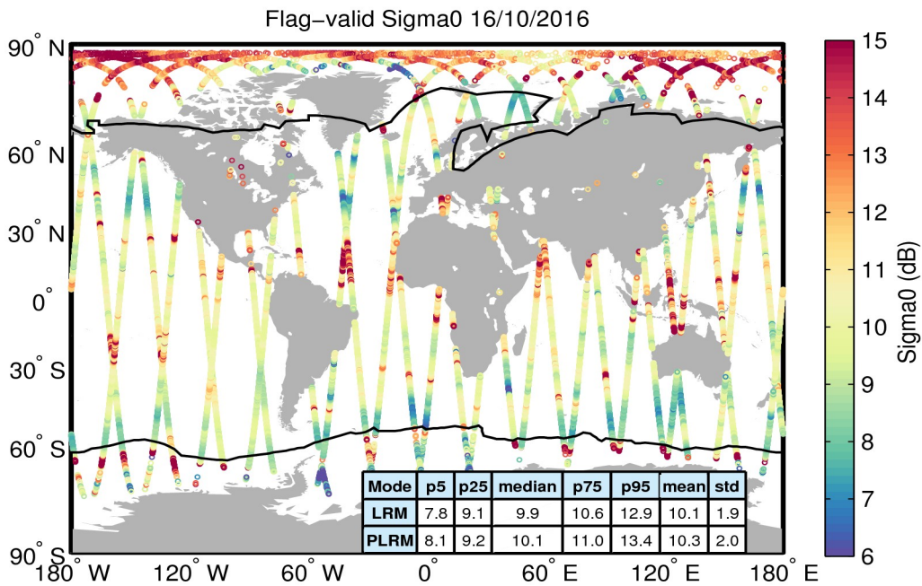
Figure 23. Geographical distribution of flag-valid sigma0 data over oceans and lakes for 16/10/2016. The statistical values shown in the table refer to the sigma0 in dB and are calculated separately for LRM and PLRM regions. Measurements taken over polar polygons have been excluded from the computation of the statistical values. The black lines mark the outer limit of the Arctic and Antarctic polar polygons.
