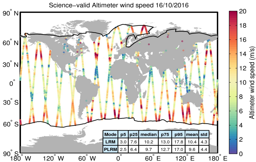
Figure 34. Geographical distribution of science-valid wind data over oceans and lakes for 16/10/2016. The statistical values shown in the table refer to the wind in m/s and are calculated separately for LRM and PLRM regions. The black lines mark the outer limit of the Arctic and Antarctic polar polygons. Gray circles denote records that have been rejected based on the editing criteria described in Table 5.
