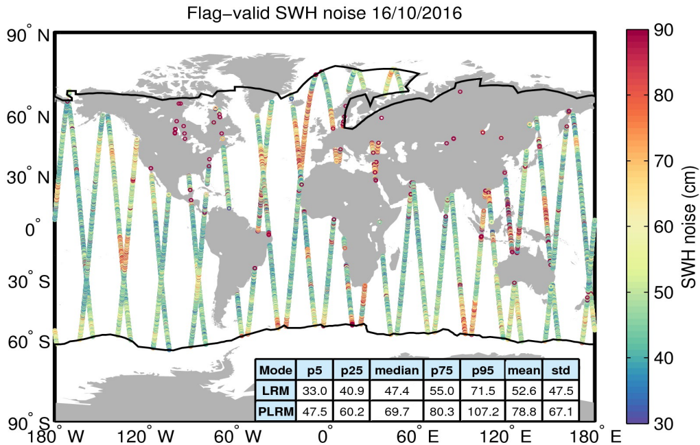
Figure 18. Geographical distribution of flag-valid 20-Hz SWH measurement noise over oceans and lakes for 16/10/2016. The statistical values shown in the table refer to the SWH noise and are calculated separately for LRM and PLRM regions. Measurements taken over polar polygons have been excluded from the computation of the statistical values. The black lines mark the outer limit of the Arctic and Antarctic polar polygons.
