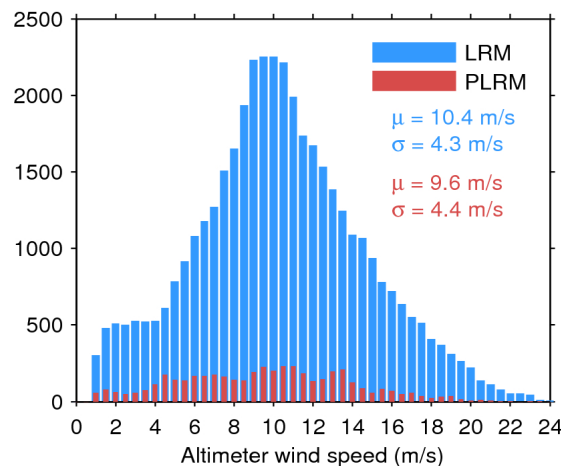
Figure 35. Histogram of science-valid wind over oceans and lakes for LRM (blue) and PLRM (red) for 16/10/2016. The mean ( \mu ) and standard deviation ( \sigma ) are also shown. Note that values larger than 24 m/s are excluded from the histogram for the sake of readability but not from the computation of \mu and \sigma .
