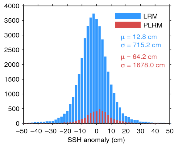
Figure 7. Histogram of flag-valid SSH anomaly over oceans and lakes for LRM (blue) and PLRM (red) for 16/10/2016. The mean ( \mu ) and standard deviation ( \sigma ) are also shown. Note that values outside [-50\ 50] cm are excluded from the histogram for the sake of readability but not from the computation of \mu and \sigma .
