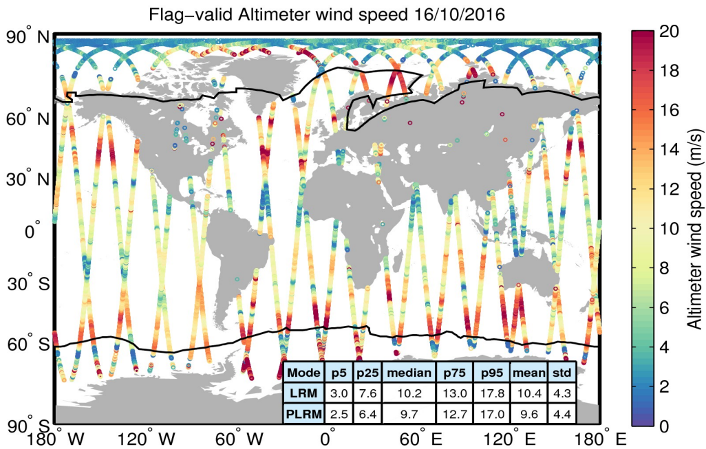
Figure 31. Geographical distribution of flag-valid wind data over oceans and lakes for 16/10/2016. The statistical values shown in the table refer to the wind in m/s and are calculated separately for LRM and PLRM regions. Measurements taken over polar polygons have been excluded from the computation of the statistical values. The black lines mark the outer limit of the Arctic and Antarctic polar polygons.
