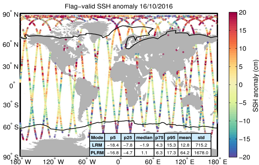
Figure 5. Geographical distribution of flag-valid 1-Hz SSH anomaly data over oceans and lakes for 16/10/2016. The statistical values shown in the table refer to the SSH anomaly in cm and are calculated separately for LRM and PLRM regions. Measurements taken over polar polygons have been excluded from the computation of the statistical values. The black lines mark the outer limit of the Arctic and Antarctic polar polygons.
