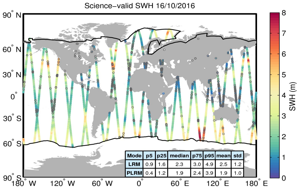
Figure 19. Geographical distribution of science-valid SWH data over oceans and lakes for 16/10/2016. The statistical values shown in the table refer to the SWH in m and are calculated separately for LRM and PLRM regions. The black lines mark the outer limit of the Arctic and Antarctic polar polygons. Gray circles denote records that have been rejected based on the editing criteria described in Table 3.
