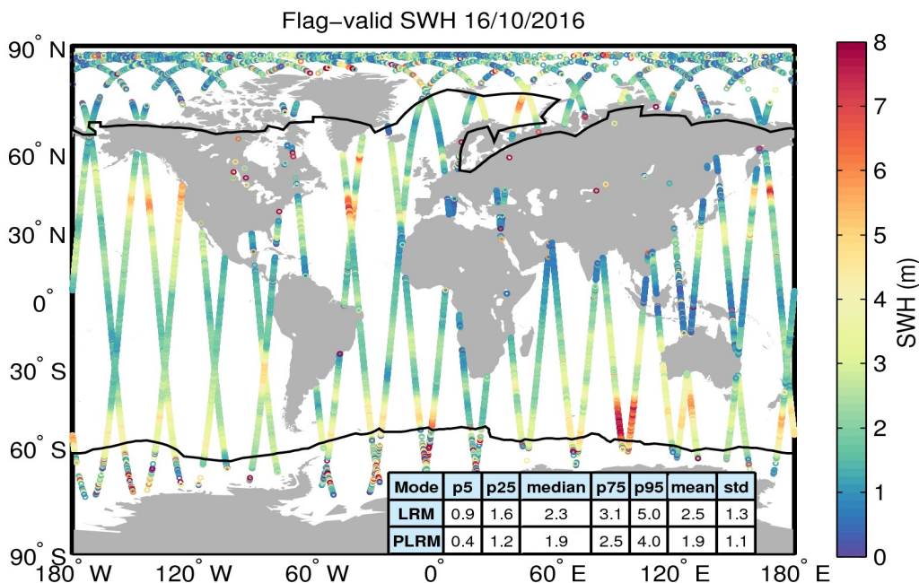
Figure 15. Geographical distribution of flag-valid SWH data over oceans and lakes for 16/10/2016. The statistical values shown in the table refer to the SWH in m and are calculated separately for LRM and PLRM regions. Measurements taken over polar polygons have been excluded from the computation of the statistical values. The black lines mark the outer limit of the Arctic and Antarctic polar polygons.
