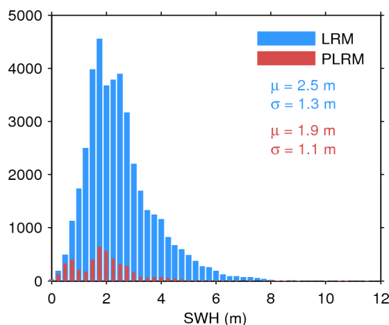
Figure 17. Histogram of flag-valid SWH over oceans and lakes for LRM (blue) and PLRM (red) for 16/10/2016. The mean ( \mu ) and standard deviation ( \sigma ) are also shown. Note that values larger than 12 m are excluded from the histogram for the sake of readability but not from the computation of \mu and \sigma .
