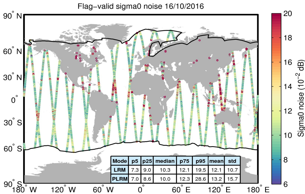
Figure 26. Geographical distribution of flag-valid 20-Hz sigma0 measurement noise over oceans and lakes for 16/10/2016. The statistical values shown in the table refer to the sigma0 noise and are calculated separately for LRM and PLRM regions. Measurements taken over polar polygons have been excluded from the computation of the statistical values. The black lines mark the outer limit of the Arctic and Antarctic polar polygons.
