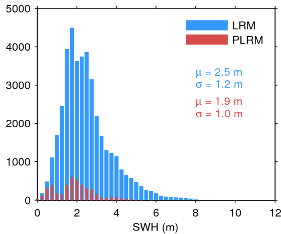
Figure 20. Histogram of science-valid SWH over oceans and lakes for LRM (blue) and PLRM (red) for 16/10/2016. The mean ( \mu ) and standard deviation ( \sigma ) are also shown. Note that values larger than 12 m are excluded from the histogram for the sake of readability but not from the computation of \mu and \sigma .
