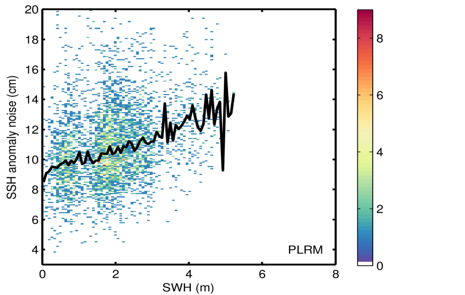
Figure 9. 2D histogram showing flag-valid SSH anomaly noise as a function of SWH for LRM (top) and PLRM (bottom) for 16/10/2016. The black line denotes the median SSH anomaly noise as a function of SWH.
