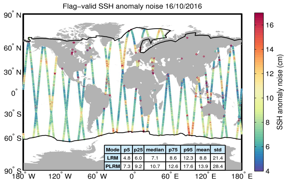
Figure 8. Geographical distribution of flag-valid 20-Hz SSH anomaly measurement noise over oceans and lakes for 16/10/2016. The statistical values shown in the table refer to the SSH anomaly noise and are calculated separately for LRM and PLRM regions. Measurements taken over polar polygons have been excluded from the computation of the statistical values. The black lines mark the outer limit of the Arctic and Antarctic polar polygons.
