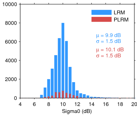
Figure 28. Histogram of science-valid sigma0 over oceans and lakes for LRM (blue) and PLRM (red) for 16/10/2016. The mean ( \mu ) and standard deviation ( \sigma ) are also shown. Note that values outside [4 20] dB are excluded from the histogram for the sake of readability but not from the computation of \mu and \sigma .
