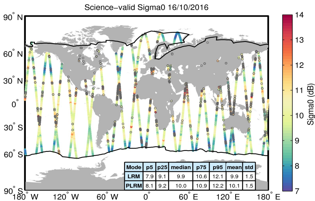
Figure 27. Geographical distribution of science-valid sigma0 data over oceans and lakes for 16/10/2016. The statistical values shown in the table refer to the sigma0 in dB and are calculated separately for LRM and PLRM regions. The black lines mark the outer limit of the Arctic and Antarctic polar polygons. Gray circles denote records that have been rejected based on the editing criteria described in Table 4.
