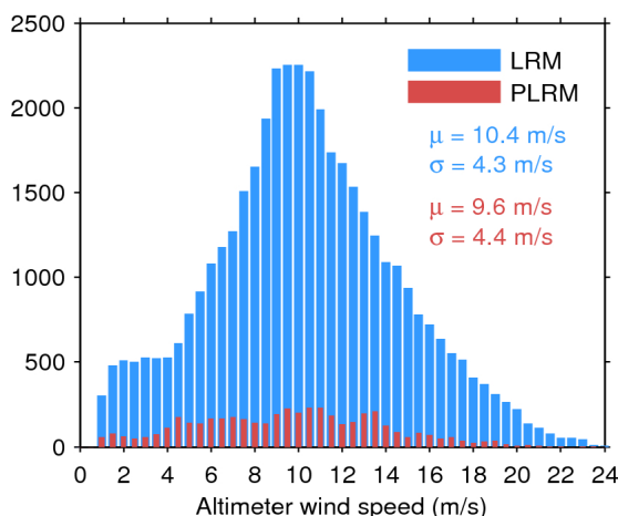
Figure 33. Histogram of flag-valid wind over oceans and lakes for LRM (blue) and PLRM (red) for 16/10/2016. The mean ( \mu ) and standard deviation ( \sigma ) are also shown. Note that values larger than 24 m/s are excluded from the histogram for the sake of readability but not from the computation of \mu and \sigma .
