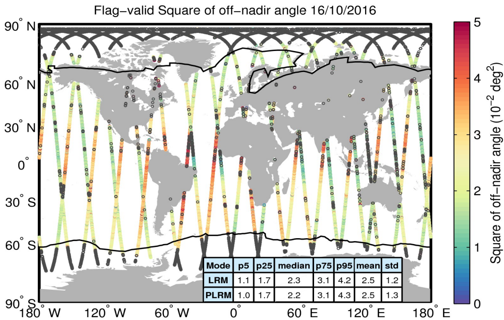
Figure 37. Geographical distribution of flag-valid mispointing data over oceans and lakes for 16/10/2016. The statistical values shown in the table refer to the mispointing in 10^{-2} deg 2 and are calculated separately for LRM and PLRM regions. Measurements taken over polar polygons have been excluded from the computation of the statistical values. The black lines mark the outer limit of the Arctic and Antarctic polar polygons. Gray circles denote negative values.
