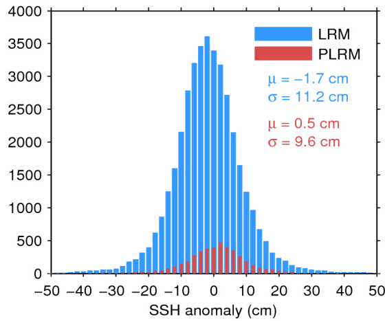
Figure 11. Histogram of science-valid SSH anomaly over oceans and lakes for LRM (blue) and PLRM (red) for 16/10/2016. The mean ( \mu ) and standard deviation ( \sigma ) are also shown. Note that values outside [-50 50] cm are excluded from the histogram for the sake of readability but not from the computation of \mu and \sigma .
