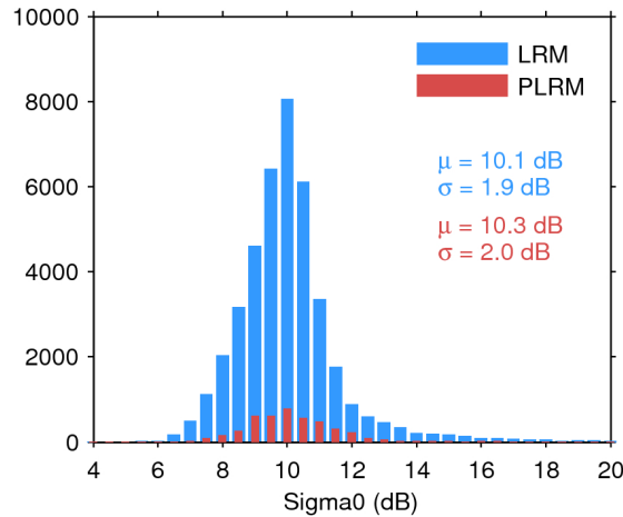
Figure 25. Histogram of flag-valid sigma0 over oceans and lakes for LRM (blue) and PLRM (red) for 16/10/2016. The mean ( \mu ) and standard deviation ( \sigma ) are also shown. Note that values outside [4 20] dB are excluded from the histogram for the sake of readability but not from the computation of \mu and \sigma .
