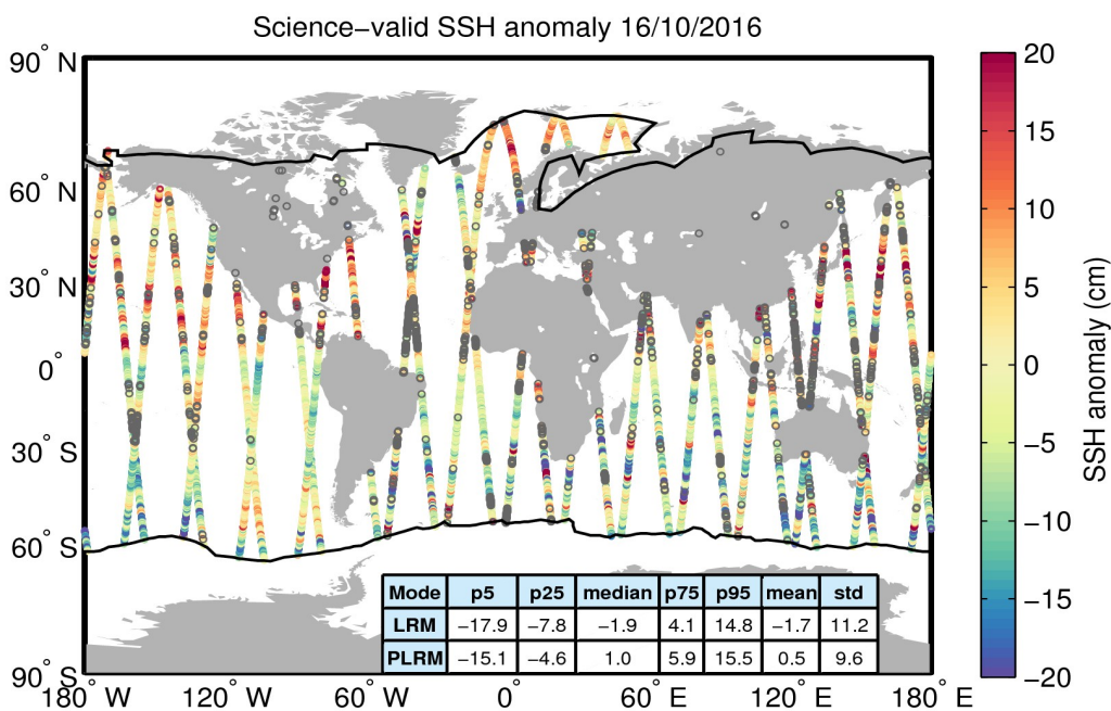
Figure 10. Geographical distribution of science-valid SSH anomaly data over oceans and lakes for 16/10/2016. The statistical values shown in the table refer to the SSH anomaly in cm and are calculated separately for LRM and PLRM regions. The black lines mark the outer limit of the Arctic and Antarctic polar polygons. Gray circles denote records that have been rejected based on the editing criteria described in Table 2.
