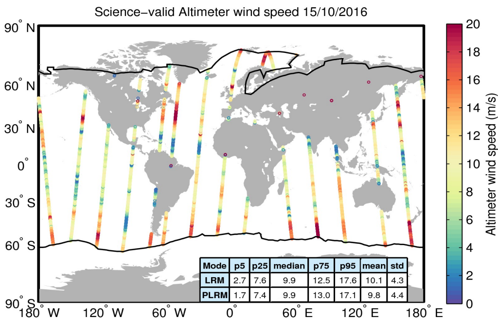
Figure 34. Geographical distribution of science-valid wind data over oceans and lakes for 15/10/2016. The statistical values shown in the table refer to the wind in m/s and are calculated separately for LRM and PLRM regions. The black lines mark the outer limit of the Arctic and Antarctic polar polygons. Gray circles denote records that have been rejected based on the editing criteria described in Table 5.
