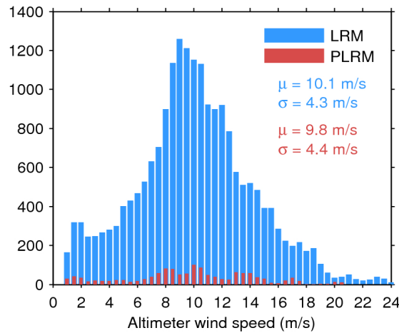
Figure 33. Histogram of flag-valid wind over oceans and lakes for LRM (blue) and PLRM (red) for 15/10/2016. The mean ( \mu ) and standard deviation ( \sigma ) are also shown. Note that values larger than 24 m/s are excluded from the histogram for the sake of readability but not from the computation of \mu and \sigma .
