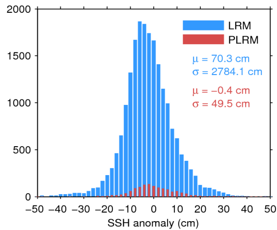
Figure 7. Histogram of flag-valid SSH anomaly over oceans and lakes for LRM (blue) and PLRM (red) for 15/10/2016. The mean ( \mu ) and standard deviation ( \sigma ) are also shown. Note that values outside [-50\ 50] cm are excluded from the histogram for the sake of readability but not from the computation of \mu and \sigma .
