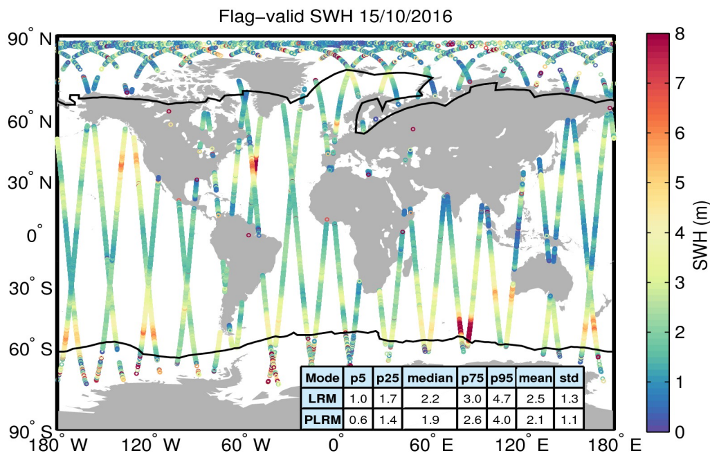
Figure 15. Geographical distribution of flag-valid SWH data over oceans and lakes for 15/10/2016. The statistical values shown in the table refer to the SWH in m and are calculated separately for LRM and PLRM regions. Measurements taken over polar polygons have been excluded from the computation of the statistical values. The black lines mark the outer limit of the Arctic and Antarctic polar polygons.
