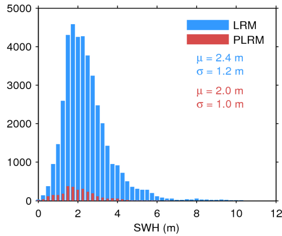
Figure 20. Histogram of science-valid SWH over oceans and lakes for LRM (blue) and PLRM (red) for 15/10/2016. The mean ( \mu ) and standard deviation ( \sigma ) are also shown. Note that values larger than 12 m are excluded from the histogram for the sake of readability but not from the computation of \mu and \sigma .
