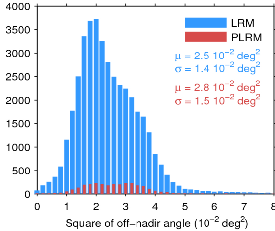
Figure 39. Histogram of flag-valid mispointing over oceans and lakes for LRM (blue) and PLRM (red) for 15/10/2016. Only positive values have been considered. The mean ( \mu ) and standard deviation ( \sigma ) are also shown. Note that values larger than 8 \cdot 10^{-2} \text{ deg}^2 are excluded from the histogram for the sake of readability but not from the computation of \mu and \sigma .
