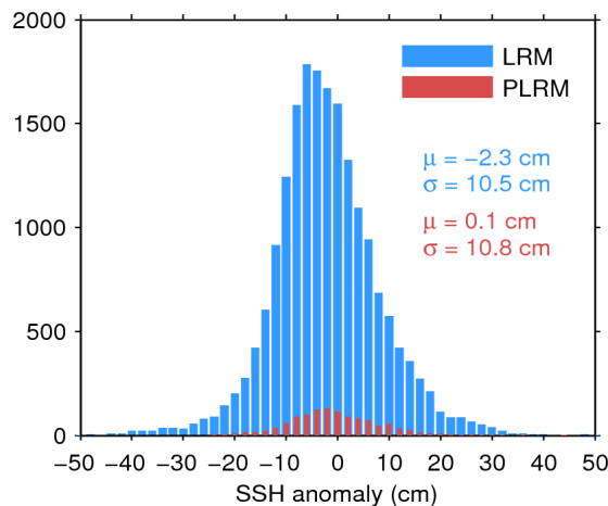
Figure 11. Histogram of science-valid SSH anomaly over oceans and lakes for LRM (blue) and PLRM (red) for 15/10/2016. The mean ( \mu ) and standard deviation ( \sigma ) are also shown. Note that values outside [-50 50] cm are excluded from the histogram for the sake of readability but not from the computation of \mu and \sigma .
