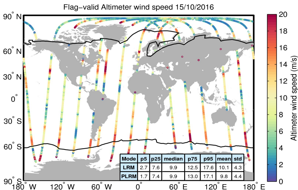
Figure 31. Geographical distribution of flag-valid wind data over oceans and lakes for 15/10/2016. The statistical values shown in the table refer to the wind in m/s and are calculated separately for LRM and PLRM regions. Measurements taken over polar polygons have been excluded from the computation of the statistical values. The black lines mark the outer limit of the Arctic and Antarctic polar polygons.
