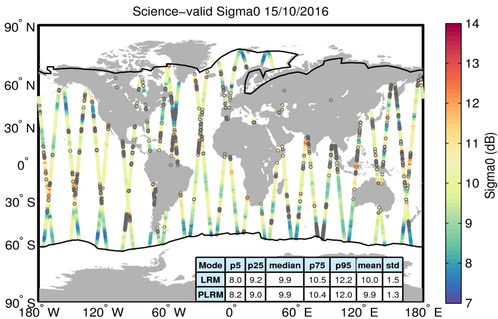
Figure 27. Geographical distribution of science-valid sigma0 data over oceans and lakes for 15/10/2016. The statistical values shown in the table refer to the sigma0 in dB and are calculated separately for LRM and PLRM regions. The black lines mark the outer limit of the Arctic and Antarctic polar polygons. Gray circles denote records that have been rejected based on the editing criteria described in Table 4.
