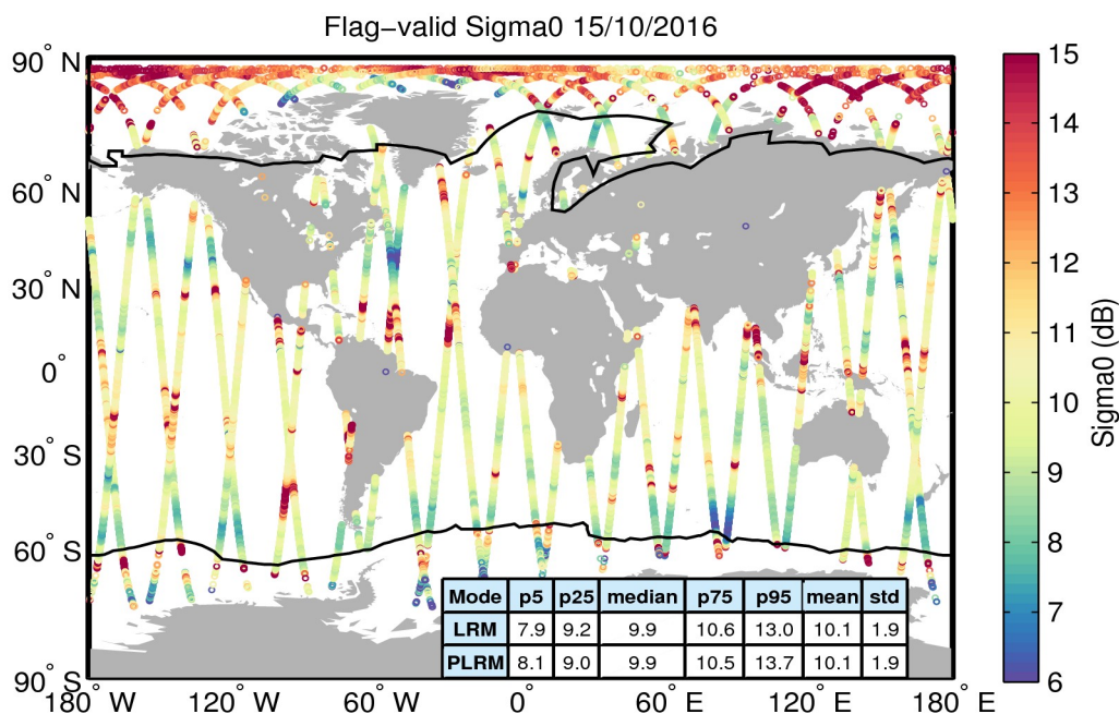
Figure 23. Geographical distribution of flag-valid sigma0 data over oceans and lakes for 15/10/2016. The statistical values shown in the table refer to the sigma0 in dB and are calculated separately for LRM and PLRM regions. Measurements taken over polar polygons have been excluded from the computation of the statistical values. The black lines mark the outer limit of the Arctic and Antarctic polar polygons.
