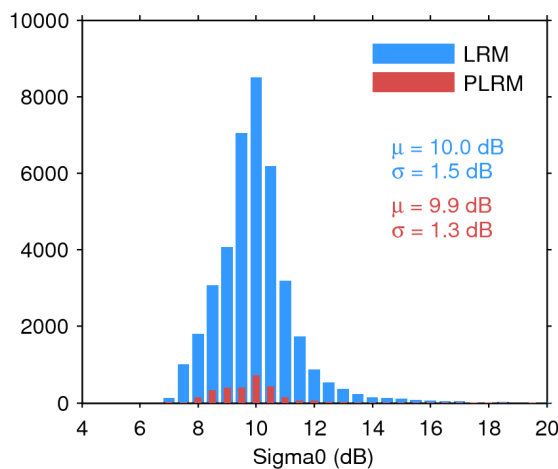
Figure 28. Histogram of science-valid sigma0 over oceans and lakes for LRM (blue) and PLRM (red) for 15/10/2016. The mean ( \mu ) and standard deviation ( \sigma ) are also shown. Note that values outside [4 20] dB are excluded from the histogram for the sake of readability but not from the computation of \mu and \sigma .
