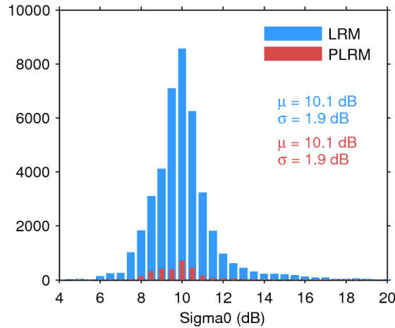
Figure 25. Histogram of flag-valid sigma0 over oceans and lakes for LRM (blue) and PLRM (red) for 15/10/2016. The mean ( \mu ) and standard deviation ( \sigma ) are also shown. Note that values outside [4 20] dB are excluded from the histogram for the sake of readability but not from the computation of \mu and \sigma .
