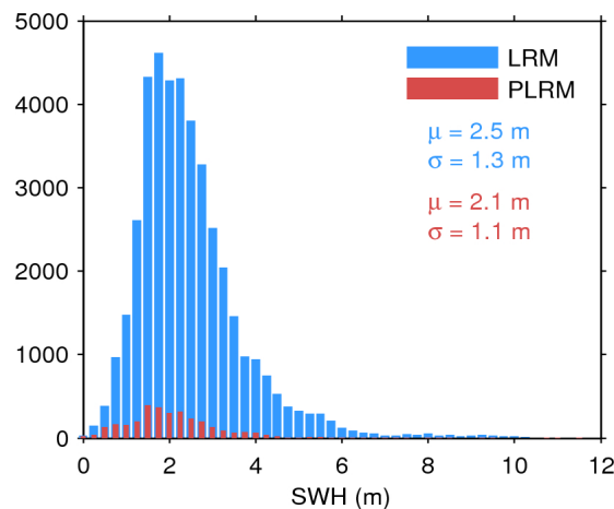
Figure 17. Histogram of flag-valid SWH over oceans and lakes for LRM (blue) and PLRM (red) for 15/10/2016. The mean ( \mu ) and standard deviation ( \sigma ) are also shown. Note that values larger than 12 m are excluded from the histogram for the sake of readability but not from the computation of \mu and \sigma .
