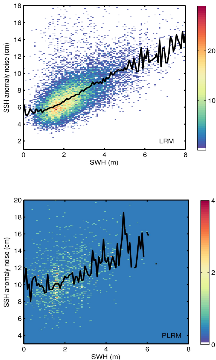
Figure 9. 2D histogram showing flag-valid SSH anomaly noise as a function of SWH for LRM (top) and PLRM (bottom) for 15/10/2016. The black line denotes the median SSH anomaly noise as a function of SWH.
