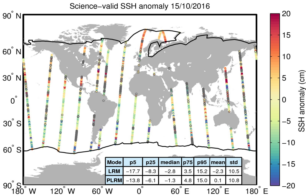
Figure 10. Geographical distribution of science-valid SSH anomaly data over oceans and lakes for 15/10/2016. The statistical values shown in the table refer to the SSH anomaly in cm and are calculated separately for LRM and PLRM regions. The black lines mark the outer limit of the Arctic and Antarctic polar polygons. Gray circles denote records that have been rejected based on the editing criteria described in Table 2.
