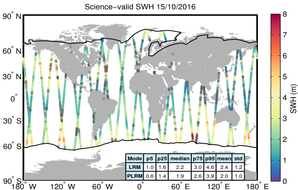
Figure 19. Geographical distribution of science-valid SWH data over oceans and lakes for 15/10/2016. The statistical values shown in the table refer to the SWH in m and are calculated separately for LRM and PLRM regions. The black lines mark the outer limit of the Arctic and Antarctic polar polygons. Gray circles denote records that have been rejected based on the editing criteria described in Table 3.
