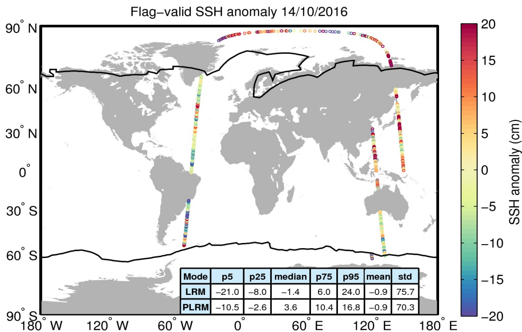
Figure 5. Geographical distribution of flag-valid 1-Hz SSH anomaly data over oceans and lakes for 14/10/2016. The statistical values shown in the table refer to the SSH anomaly in cm and are calculated separately for LRM and PLRM regions. Measurements taken over polar polygons have been excluded from the computation of the statistical values. The black lines mark the outer limit of the Arctic and Antarctic polar polygons.
