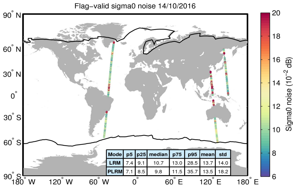
Figure 26. Geographical distribution of flag-valid 20-Hz sigma0 measurement noise over oceans and lakes for 14/10/2016. The statistical values shown in the table refer to the sigma0 noise and are calculated separately for LRM and PLRM regions. Measurements taken over polar polygons have been excluded from the computation of the statistical values. The black lines mark the outer limit of the Arctic and Antarctic polar polygons.
