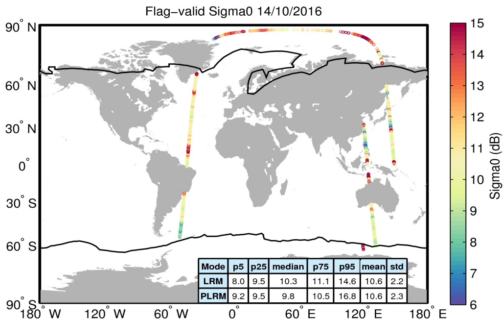
Figure 23. Geographical distribution of flag-valid sigma0 data over oceans and lakes for 14/10/2016. The statistical values shown in the table refer to the sigma0 in dB and are calculated separately for LRM and PLRM regions. Measurements taken over polar polygons have been excluded from the computation of the statistical values. The black lines mark the outer limit of the Arctic and Antarctic polar polygons.
