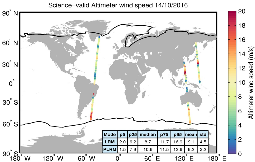
Figure 34. Geographical distribution of science-valid wind data over oceans and lakes for 14/10/2016. The statistical values shown in the table refer to the wind in m/s and are calculated separately for LRM and PLRM regions. The black lines mark the outer limit of the Arctic and Antarctic polar polygons. Gray circles denote records that have been rejected based on the editing criteria described in Table 5.
