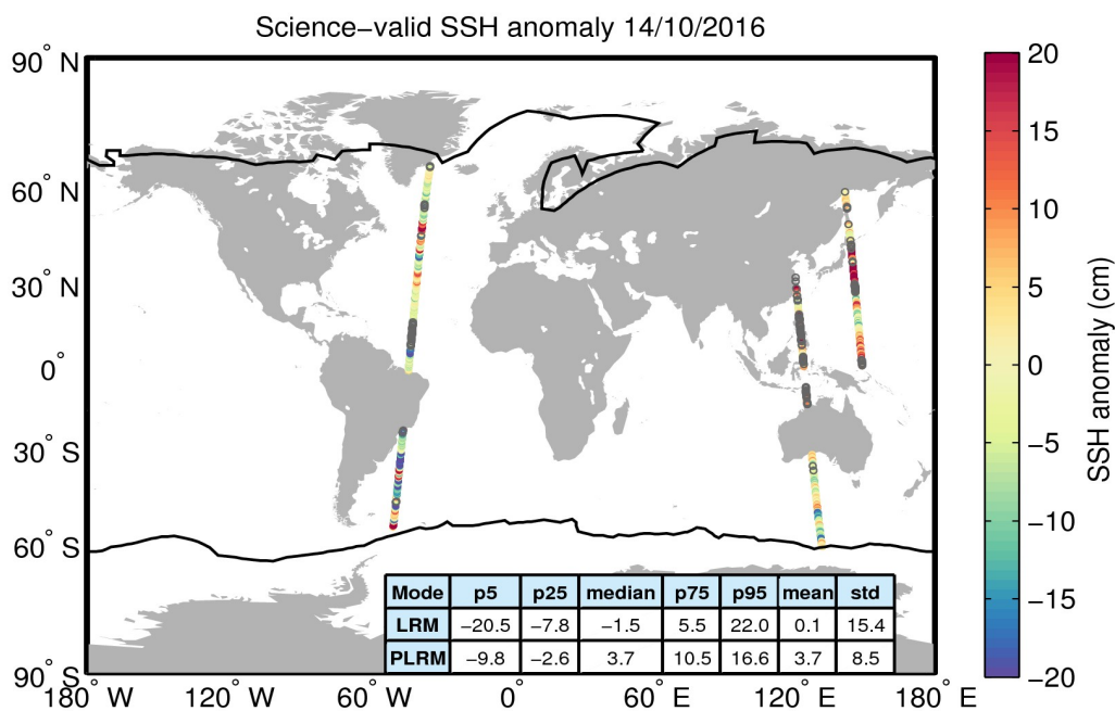
Figure 10. Geographical distribution of science-valid SSH anomaly data over oceans and lakes for 14/10/2016. The statistical values shown in the table refer to the SSH anomaly in cm and are calculated separately for LRM and PLRM regions. The black lines mark the outer limit of the Arctic and Antarctic polar polygons. Gray circles denote records that have been rejected based on the editing criteria described in Table 2.
