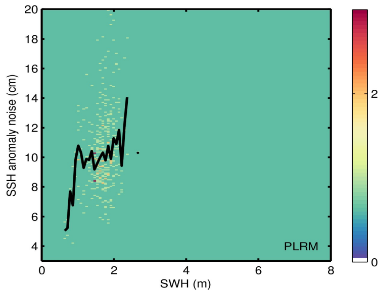
Figure 9. 2D histogram showing flag-valid SSH anomaly noise as a function of SWH for LRM (top) and PLRM (bottom) for 14/10/2016. The black line denotes the median SSH anomaly noise as a function of SWH.
