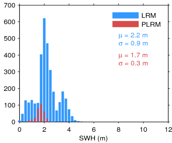
Figure 20. Histogram of science-valid SWH over oceans and lakes for LRM (blue) and PLRM (red) for 14/10/2016. The mean ( \mu ) and standard deviation ( \sigma ) are also shown. Note that values larger than 12 m are excluded from the histogram for the sake of readability but not from the computation of \mu and \sigma .
