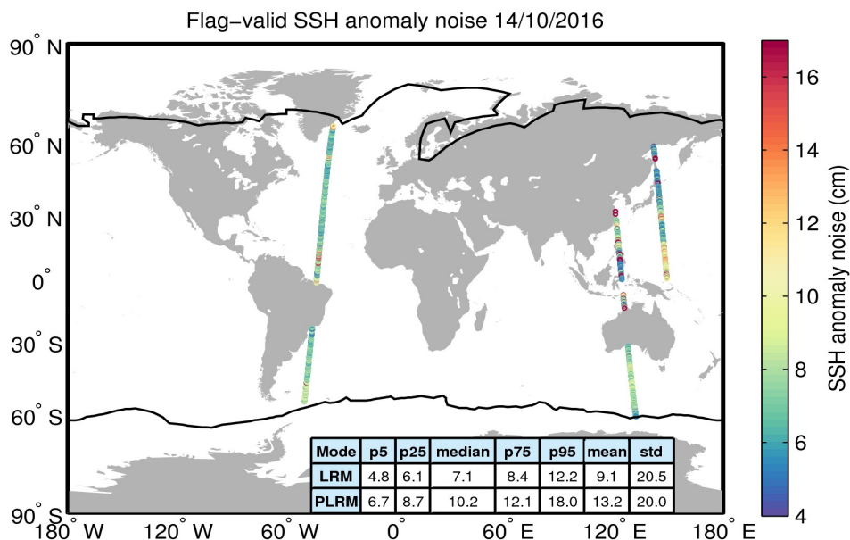
Figure 8. Geographical distribution of flag-valid 20-Hz SSH anomaly measurement noise over oceans and lakes for 14/10/2016. The statistical values shown in the table refer to the SSH anomaly noise and are calculated separately for LRM and PLRM regions. Measurements taken over polar polygons have been excluded from the computation of the statistical values. The black lines mark the outer limit of the Arctic and Antarctic polar polygons.
