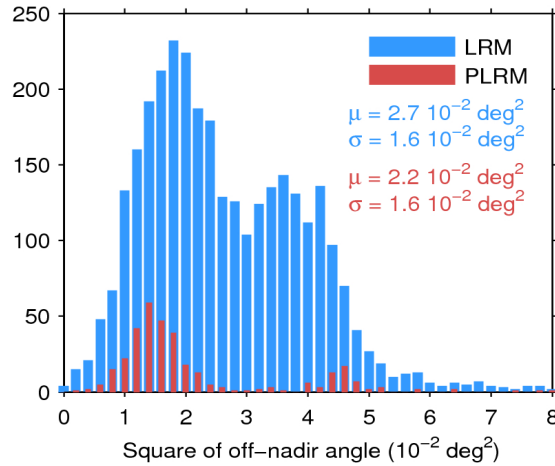
Figure 39. Histogram of flag-valid mispointing over oceans and lakes for LRM (blue) and PLRM (red) for 14/10/2016. Only positive values have been considered. The mean ( \mu ) and standard deviation ( \sigma ) are also shown. Note that values larger than 8 \cdot 10^{-2} \text{ deg}^2 are excluded from the histogram for the sake of readability but not from the computation of \mu and \sigma .
