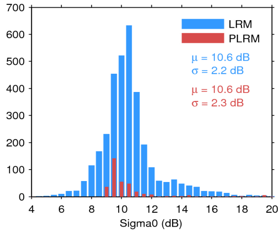
Figure 25. Histogram of flag-valid sigma0 over oceans and lakes for LRM (blue) and PLRM (red) for 14/10/2016. The mean ( \mu ) and standard deviation ( \sigma ) are also shown. Note that values outside [4 20] dB are excluded from the histogram for the sake of readability but not from the computation of \mu and \sigma .
