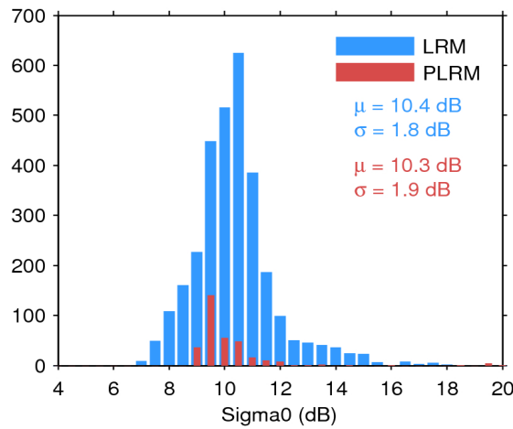
Figure 28. Histogram of science-valid sigma0 over oceans and lakes for LRM (blue) and PLRM (red) for 14/10/2016. The mean ( \mu ) and standard deviation ( \sigma ) are also shown. Note that values outside [4 20] dB are excluded from the histogram for the sake of readability but not from the computation of \mu and \sigma .
