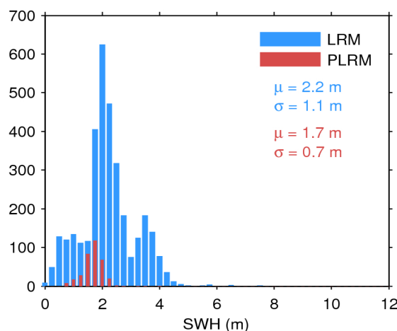
Figure 17. Histogram of flag-valid SWH over oceans and lakes for LRM (blue) and PLRM (red) for 14/10/2016. The mean ( \mu ) and standard deviation ( \sigma ) are also shown. Note that values larger than 12 m are excluded from the histogram for the sake of readability but not from the computation of \mu and \sigma .
