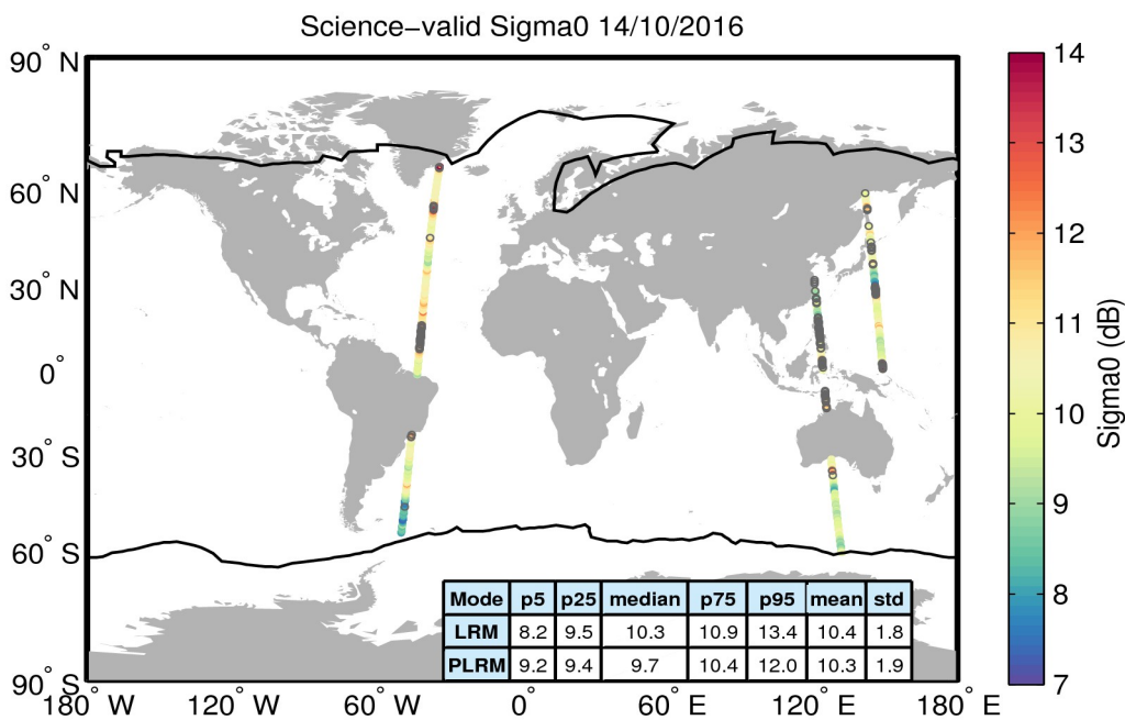
Figure 27. Geographical distribution of science-valid sigma0 data over oceans and lakes for 14/10/2016. The statistical values shown in the table refer to the sigma0 in dB and are calculated separately for LRM and PLRM regions. The black lines mark the outer limit of the Arctic and Antarctic polar polygons. Gray circles denote records that have been rejected based on the editing criteria described in Table 4.
