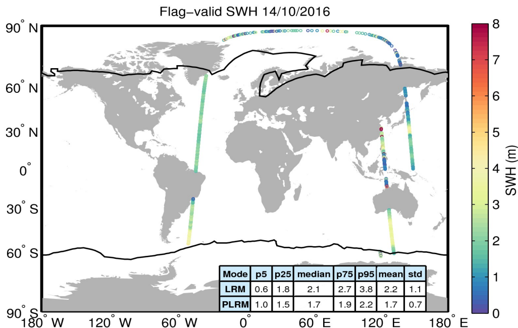
Figure 15. Geographical distribution of flag-valid SWH data over oceans and lakes for 14/10/2016. The statistical values shown in the table refer to the SWH in m and are calculated separately for LRM and PLRM regions. Measurements taken over polar polygons have been excluded from the computation of the statistical values. The black lines mark the outer limit of the Arctic and Antarctic polar polygons.
