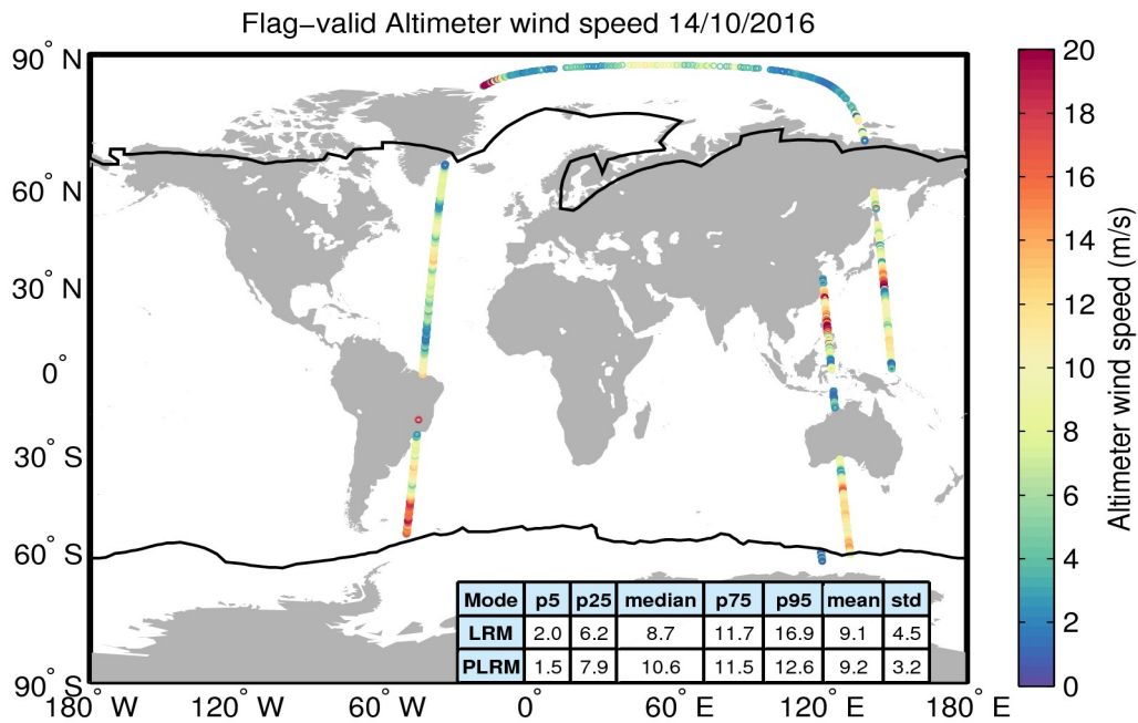
Figure 31. Geographical distribution of flag-valid wind data over oceans and lakes for 14/10/2016. The statistical values shown in the table refer to the wind in m/s and are calculated separately for LRM and PLRM regions. Measurements taken over polar polygons have been excluded from the computation of the statistical values. The black lines mark the outer limit of the Arctic and Antarctic polar polygons.
