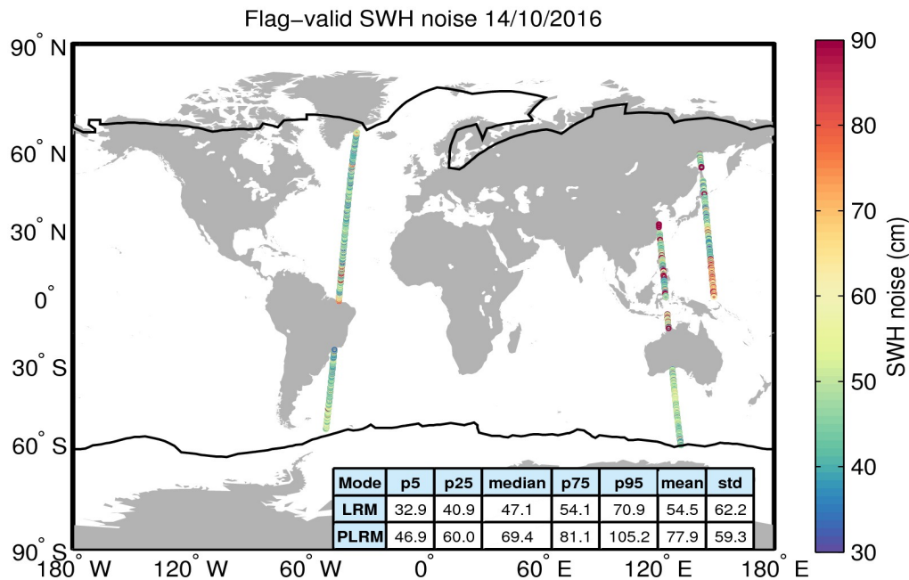
Figure 18. Geographical distribution of flag-valid 20-Hz SWH measurement noise over oceans and lakes for 14/10/2016. The statistical values shown in the table refer to the SWH noise and are calculated separately for LRM and PLRM regions. Measurements taken over polar polygons have been excluded from the computation of the statistical values. The black lines mark the outer limit of the Arctic and Antarctic polar polygons.
