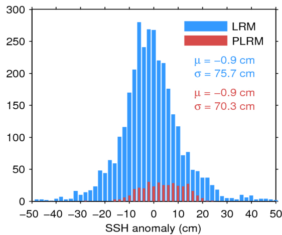
Figure 7. Histogram of flag-valid SSH anomaly over oceans and lakes for LRM (blue) and PLRM (red) for 14/10/2016. The mean ( \mu ) and standard deviation ( \sigma ) are also shown. Note that values outside [-50\ 50] cm are excluded from the histogram for the sake of readability but not from the computation of \mu and \sigma .
