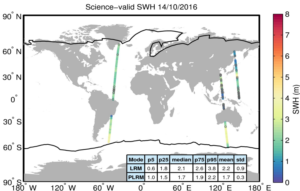
Figure 19. Geographical distribution of science-valid SWH data over oceans and lakes for 14/10/2016. The statistical values shown in the table refer to the SWH in m and are calculated separately for LRM and PLRM regions. The black lines mark the outer limit of the Arctic and Antarctic polar polygons. Gray circles denote records that have been rejected based on the editing criteria described in Table 3.
