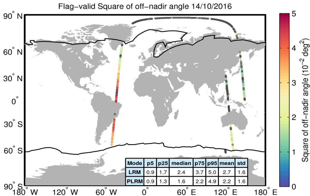
Figure 37. Geographical distribution of flag-valid mispointing data over oceans and lakes for 14/10/2016. The statistical values shown in the table refer to the mispointing in 10^{-2} deg 2 and are calculated separately for LRM and PLRM regions. Measurements taken over polar polygons have been excluded from the computation of the statistical values. The black lines mark the outer limit of the Arctic and Antarctic polar polygons. Gray circles denote negative values.
