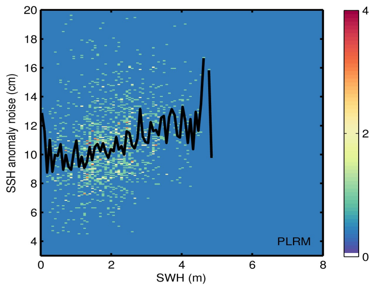
Figure 9. 2D histogram showing flag-valid SSH anomaly noise as a function of SWH for LRM (top) and PLRM (bottom) for 13/10/2016. The black line denotes the median SSH anomaly noise as a function of SWH.
