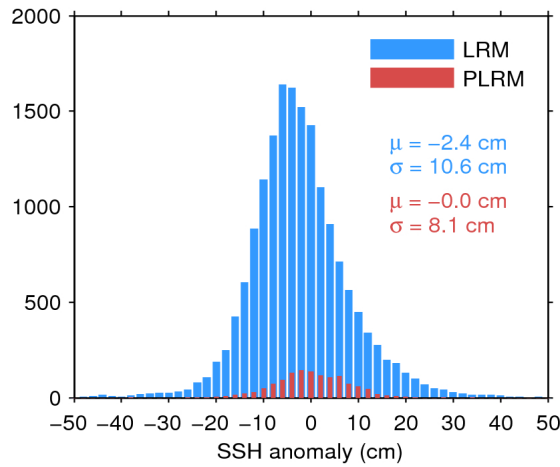
Figure 11. Histogram of science-valid SSH anomaly over oceans and lakes for LRM (blue) and PLRM (red) for 13/10/2016. The mean ( \mu ) and standard deviation ( \sigma ) are also shown. Note that values outside [-50\ 50] cm are excluded from the histogram for the sake of readability but not from the computation of \mu and \sigma .
