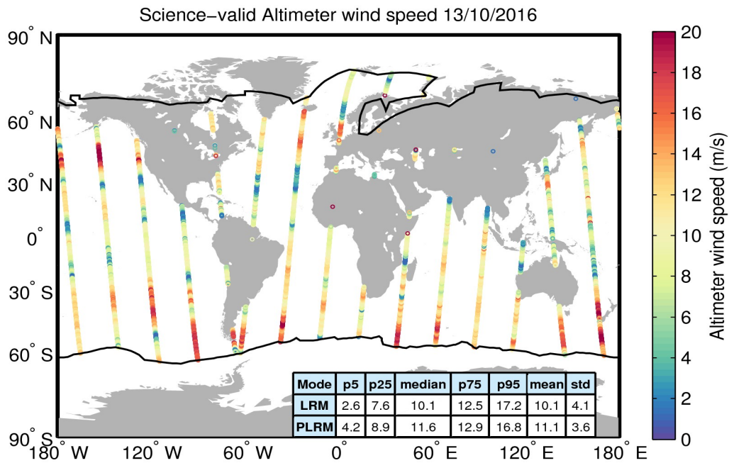
Figure 34. Geographical distribution of science-valid wind data over oceans and lakes for 13/10/2016. The statistical values shown in the table refer to the wind in m/s and are calculated separately for LRM and PLRM regions. The black lines mark the outer limit of the Arctic and Antarctic polar polygons. Gray circles denote records that have been rejected based on the editing criteria described in Table 5.
