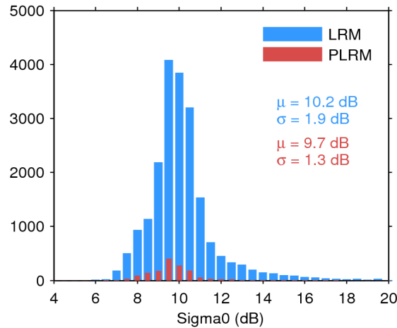
Figure 25. Histogram of flag-valid sigma0 over oceans and lakes for LRM (blue) and PLRM (red) for 13/10/2016. The mean ( \mu ) and standard deviation ( \sigma ) are also shown. Note that values outside [4 20] dB are excluded from the histogram for the sake of readability but not from the computation of \mu and \sigma .
