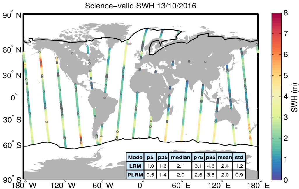
Figure 19. Geographical distribution of science-valid SWH data over oceans and lakes for 13/10/2016. The statistical values shown in the table refer to the SWH in m and are calculated separately for LRM and PLRM regions. The black lines mark the outer limit of the Arctic and Antarctic polar polygons. Gray circles denote records that have been rejected based on the editing criteria described in Table 3.
