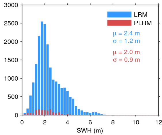
Figure 20. Histogram of science-valid SWH over oceans and lakes for LRM (blue) and PLRM (red) for 13/10/2016. The mean ( \mu ) and standard deviation ( \sigma ) are also shown. Note that values larger than 12 m are excluded from the histogram for the sake of readability but not from the computation of \mu and \sigma .
