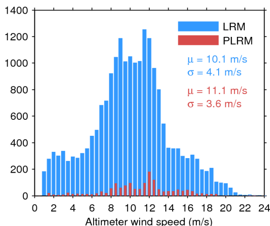
Figure 33. Histogram of flag-valid wind over oceans and lakes for LRM (blue) and PLRM (red) for 13/10/2016. The mean ( \mu ) and standard deviation ( \sigma ) are also shown. Note that values larger than 24 m/s are excluded from the histogram for the sake of readability but not from the computation of \mu and \sigma .
