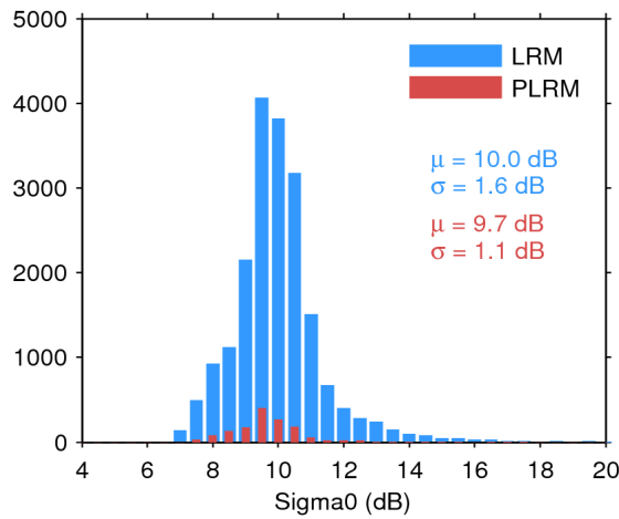
Figure 28. Histogram of science-valid sigma0 over oceans and lakes for LRM (blue) and PLRM (red) for 13/10/2016. The mean ( \mu ) and standard deviation ( \sigma ) are also shown. Note that values outside [4 20] dB are excluded from the histogram for the sake of readability but not from the computation of \mu and \sigma .
