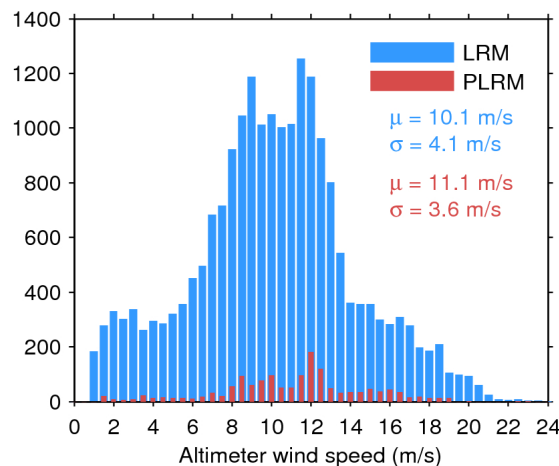
Figure 35. Histogram of science-valid wind over oceans and lakes for LRM (blue) and PLRM (red) for 13/10/2016. The mean ( \mu ) and standard deviation ( \sigma ) are also shown. Note that values larger than 24 m/s are excluded from the histogram for the sake of readability but not from the computation of \mu and \sigma .
