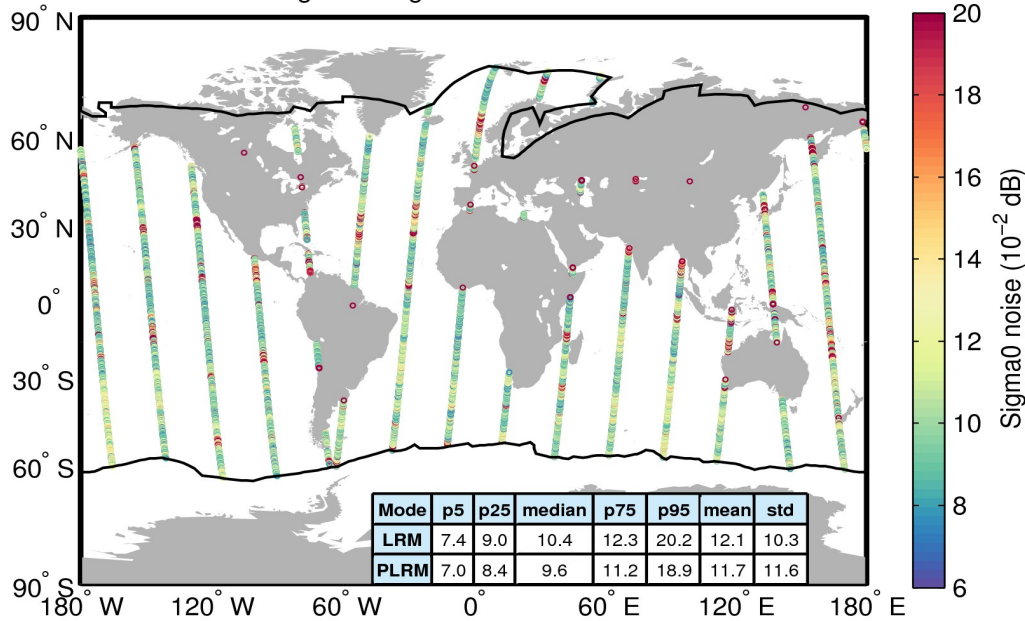
Flag-valid sigma0 noise 13/10/2016
