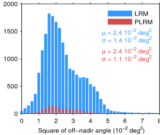
Figure 39. Histogram of flag-valid mispointing over oceans and lakes for LRM (blue) and PLRM (red) for 13/10/2016. Only positive values have been considered. The mean ( \mu ) and standard deviation ( \sigma ) are also shown. Note that values larger than 8 \cdot 10^{-2} \text{ deg}^2 are excluded from the histogram for the sake of readability but not from the computation of \mu and \sigma .
