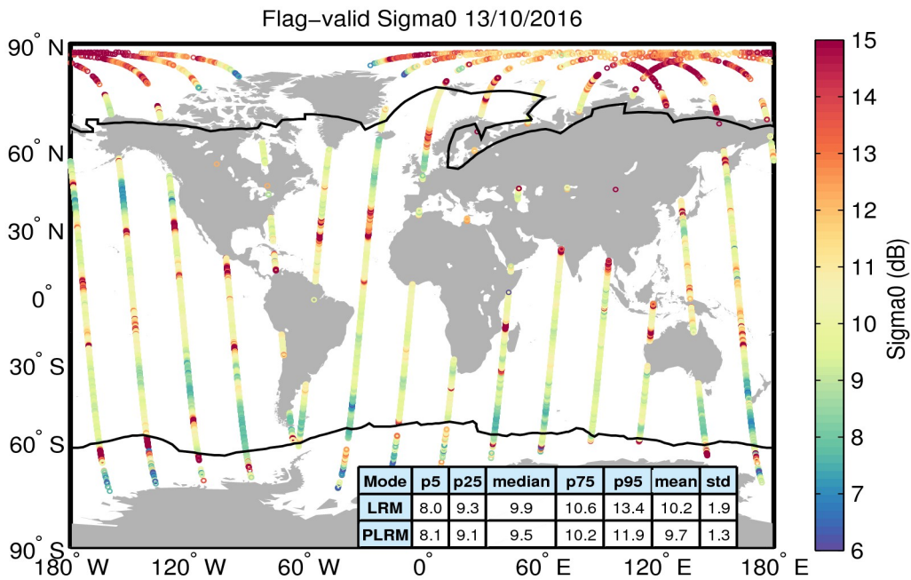
Figure 23. Geographical distribution of flag-valid sigma0 data over oceans and lakes for 13/10/2016. The statistical values shown in the table refer to the sigma0 in dB and are calculated separately for LRM and PLRM regions. Measurements taken over polar polygons have been excluded from the computation of the statistical values. The black lines mark the outer limit of the Arctic and Antarctic polar polygons.
