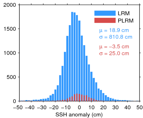
Figure 7. Histogram of flag-valid SSH anomaly over oceans and lakes for LRM (blue) and PLRM (red) for 13/10/2016. The mean ( \mu ) and standard deviation ( \sigma ) are also shown. Note that values outside [-50 50] cm are excluded from the histogram for the sake of readability but not from the computation of \mu and \sigma .
