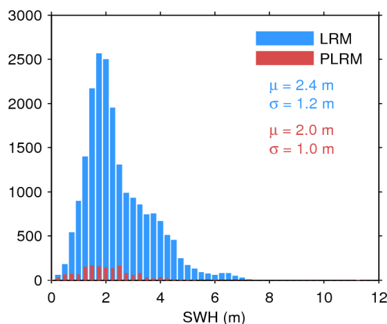
Figure 17. Histogram of flag-valid SWH over oceans and lakes for LRM (blue) and PLRM (red) for 13/10/2016. The mean ( \mu ) and standard deviation ( \sigma ) are also shown. Note that values larger than 12 m are excluded from the histogram for the sake of readability but not from the computation of \mu and \sigma .
