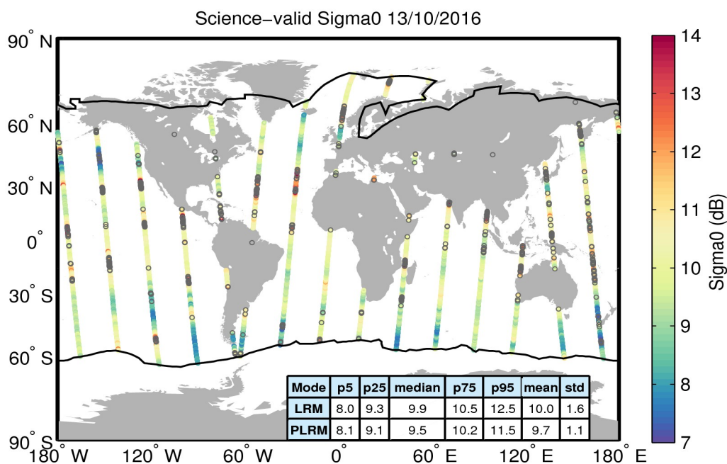
Figure 27. Geographical distribution of science-valid sigma0 data over oceans and lakes for 13/10/2016. The statistical values shown in the table refer to the sigma0 in dB and are calculated separately for LRM and PLRM regions. The black lines mark the outer limit of the Arctic and Antarctic polar polygons. Gray circles denote records that have been rejected based on the editing criteria described in Table 4.
