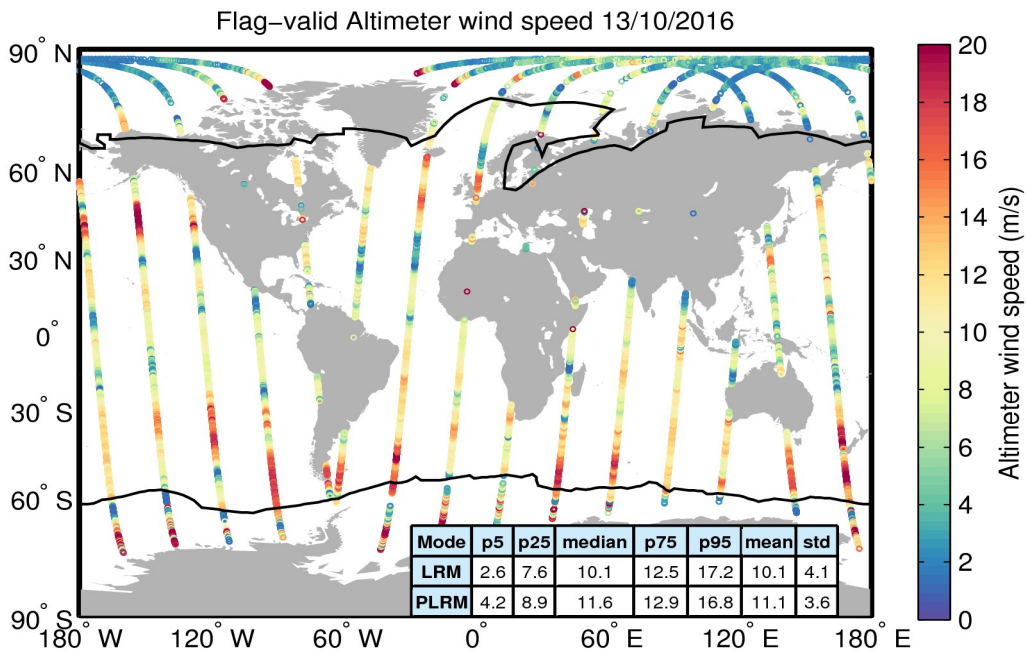
Figure 31. Geographical distribution of flag-valid wind data over oceans and lakes for 13/10/2016. The statistical values shown in the table refer to the wind in m/s and are calculated separately for LRM and PLRM regions. Measurements taken over polar polygons have been excluded from the computation of the statistical values. The black lines mark the outer limit of the Arctic and Antarctic polar polygons.
