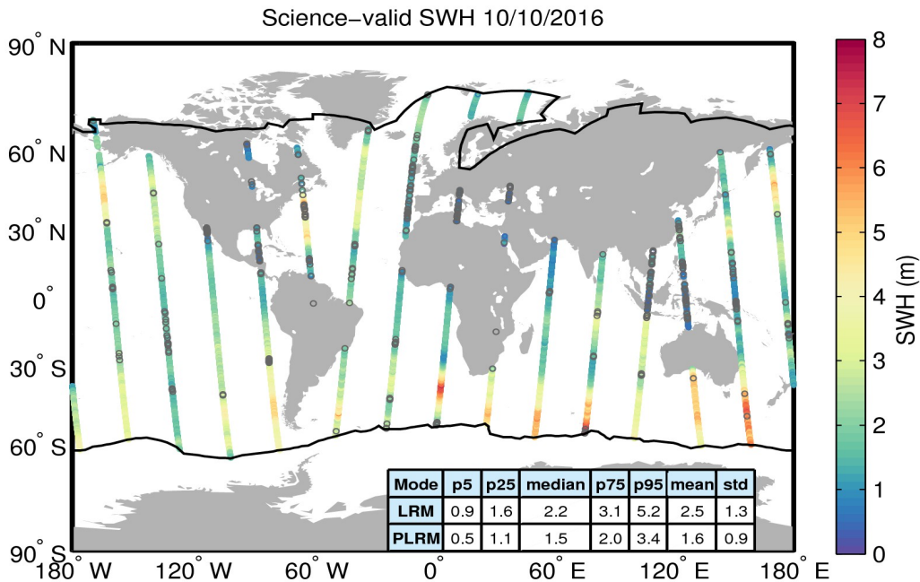
Figure 19. Geographical distribution of science-valid SWH data over oceans and lakes for 10/10/2016. The statistical values shown in the table refer to the SWH in m and are calculated separately for LRM and PLRM regions. The black lines mark the outer limit of the Arctic and Antarctic polar polygons. Gray circles denote records that have been rejected based on the editing criteria described in Table 3.
