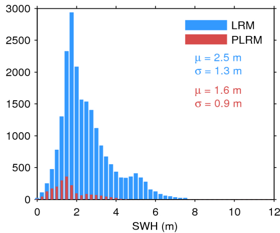
Figure 20. Histogram of science-valid SWH over oceans and lakes for LRM (blue) and PLRM (red) for 10/10/2016. The mean ( \mu ) and standard deviation ( \sigma ) are also shown. Note that values larger than 12 m are excluded from the histogram for the sake of readability but not from the computation of \mu and \sigma .
