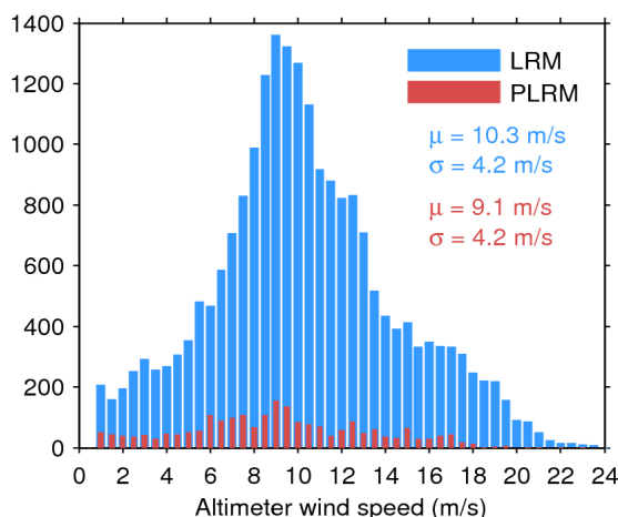
Figure 33. Histogram of flag-valid wind over oceans and lakes for LRM (blue) and PLRM (red) for 10/10/2016. The mean ( \mu ) and standard deviation ( \sigma ) are also shown. Note that values larger than 24 m/s are excluded from the histogram for the sake of readability but not from the computation of \mu and \sigma .
