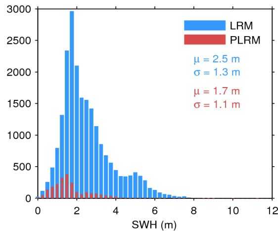
Figure 17. Histogram of flag-valid SWH over oceans and lakes for LRM (blue) and PLRM (red) for 10/10/2016. The mean ( \mu ) and standard deviation ( \sigma ) are also shown. Note that values larger than 12 m are excluded from the histogram for the sake of readability but not from the computation of \mu and \sigma .
