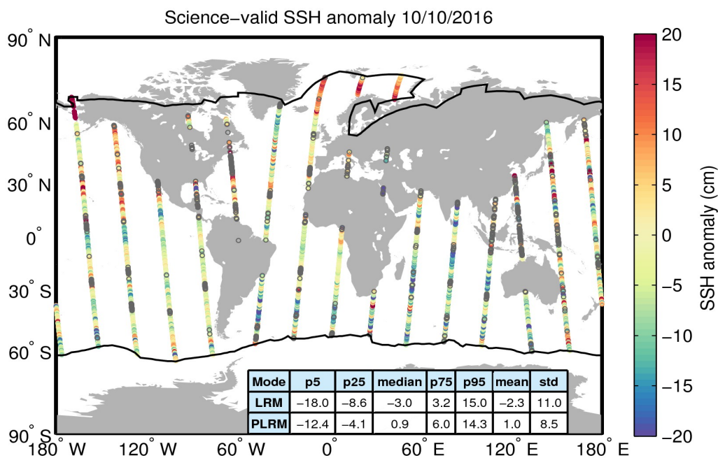
Figure 10. Geographical distribution of science-valid SSH anomaly data over oceans and lakes for 10/10/2016. The statistical values shown in the table refer to the SSH anomaly in cm and are calculated separately for LRM and PLRM regions. The black lines mark the outer limit of the Arctic and Antarctic polar polygons. Gray circles denote records that have been rejected based on the editing criteria described in Table 2.
