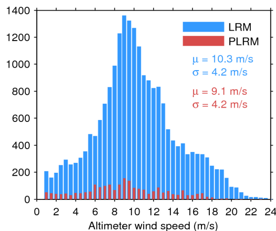
Figure 35. Histogram of science-valid wind over oceans and lakes for LRM (blue) and PLRM (red) for 10/10/2016. The mean ( \mu ) and standard deviation ( \sigma ) are also shown. Note that values larger than 24 m/s are excluded from the histogram for the sake of readability but not from the computation of \mu and \sigma .
