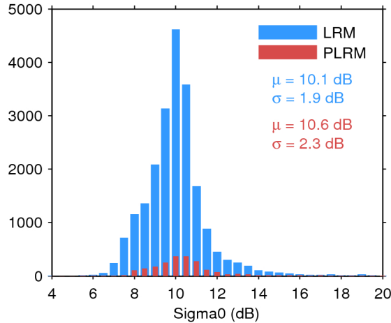
Figure 25. Histogram of flag-valid sigma0 over oceans and lakes for LRM (blue) and PLRM (red) for 10/10/2016. The mean ( \mu ) and standard deviation ( \sigma ) are also shown. Note that values outside [4 20] dB are excluded from the histogram for the sake of readability but not from the computation of \mu and \sigma .
