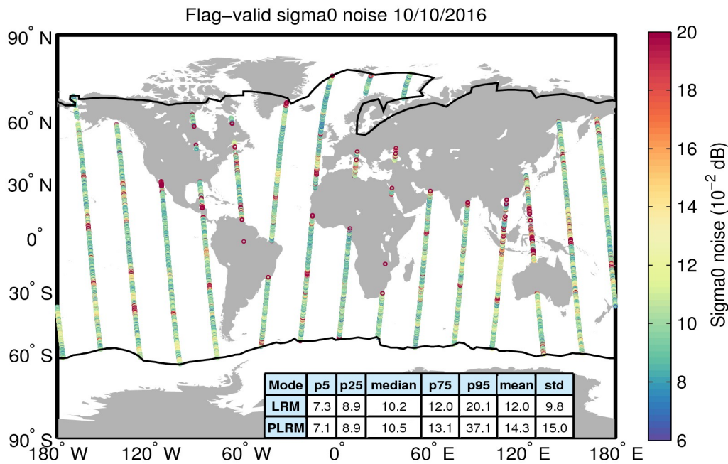
Figure 26. Geographical distribution of flag-valid 20-Hz sigma0 measurement noise over oceans and lakes for 10/10/2016. The statistical values shown in the table refer to the sigma0 noise and are calculated separately for LRM and PLRM regions. Measurements taken over polar polygons have been excluded from the computation of the statistical values. The black lines mark the outer limit of the Arctic and Antarctic polar polygons.
