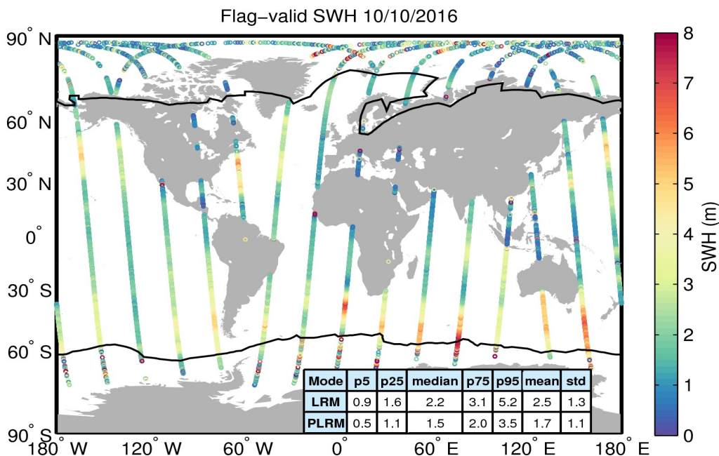
Figure 15. Geographical distribution of flag-valid SWH data over oceans and lakes for 10/10/2016. The statistical values shown in the table refer to the SWH in m and are calculated separately for LRM and PLRM regions. Measurements taken over polar polygons have been excluded from the computation of the statistical values. The black lines mark the outer limit of the Arctic and Antarctic polar polygons.
