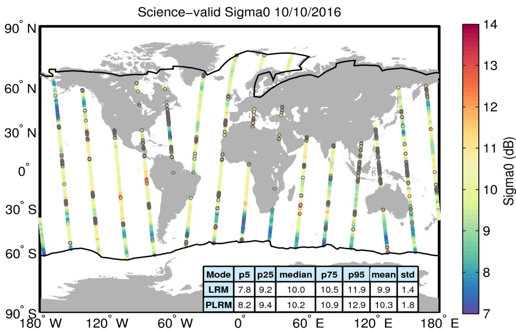
Figure 27. Geographical distribution of science-valid sigma0 data over oceans and lakes for 10/10/2016. The statistical values shown in the table refer to the sigma0 in dB and are calculated separately for LRM and PLRM regions. The black lines mark the outer limit of the Arctic and Antarctic polar polygons. Gray circles denote records that have been rejected based on the editing criteria described in Table 4.
