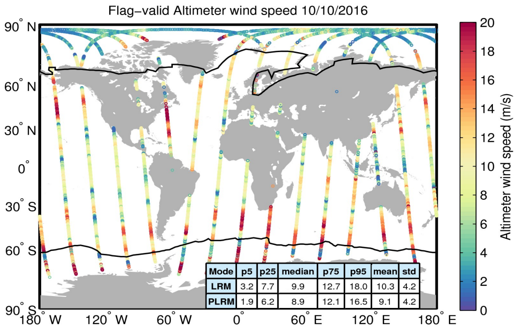
Figure 31. Geographical distribution of flag-valid wind data over oceans and lakes for 10/10/2016. The statistical values shown in the table refer to the wind in m/s and are calculated separately for LRM and PLRM regions. Measurements taken over polar polygons have been excluded from the computation of the statistical values. The black lines mark the outer limit of the Arctic and Antarctic polar polygons.
