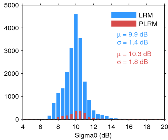
Figure 28. Histogram of science-valid sigma0 over oceans and lakes for LRM (blue) and PLRM (red) for 10/10/2016. The mean ( \mu ) and standard deviation ( \sigma ) are also shown. Note that values outside [4 20] dB are excluded from the histogram for the sake of readability but not from the computation of \mu and \sigma .
