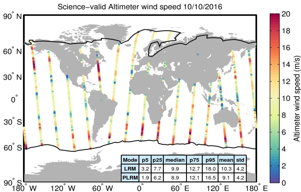
Figure 34. Geographical distribution of science-valid wind data over oceans and lakes for 10/10/2016. The statistical values shown in the table refer to the wind in m/s and are calculated separately for LRM and PLRM regions. The black lines mark the outer limit of the Arctic and Antarctic polar polygons. Gray circles denote records that have been rejected based on the editing criteria described in Table 5.
