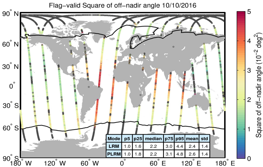
Figure 37. Geographical distribution of flag-valid mispointing data over oceans and lakes for 10/10/2016. The statistical values shown in the table refer to the mispointing in 10^{-2} deg 2 and are calculated separately for LRM and PLRM regions. Measurements taken over polar polygons have been excluded from the computation of the statistical values. The black lines mark the outer limit of the Arctic and Antarctic polar polygons. Gray circles denote negative values.
