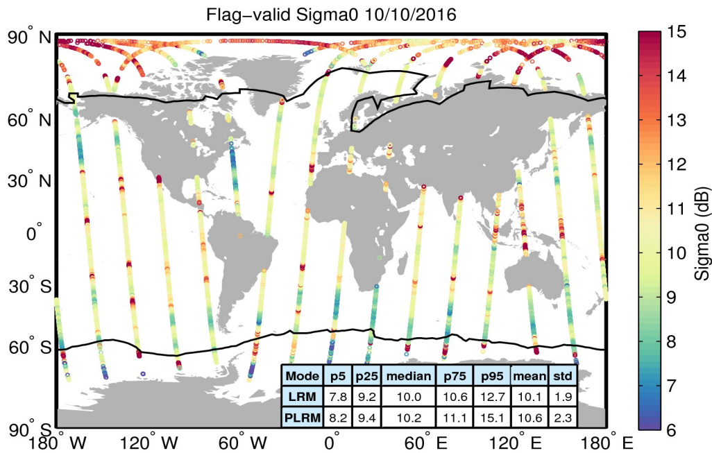
Figure 23. Geographical distribution of flag-valid sigma0 data over oceans and lakes for 10/10/2016. The statistical values shown in the table refer to the sigma0 in dB and are calculated separately for LRM and PLRM regions. Measurements taken over polar polygons have been excluded from the computation of the statistical values. The black lines mark the outer limit of the Arctic and Antarctic polar polygons.
