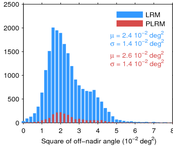
Figure 39. Histogram of flag-valid mispointing over oceans and lakes for LRM (blue) and PLRM (red) for 10/10/2016. Only positive values have been considered. The mean ( \mu ) and standard deviation ( \sigma ) are also shown. Note that values larger than 8 \cdot 10^{-2} \text{ deg}^2 are excluded from the histogram for the sake of readability but not from the computation of \mu and \sigma .
