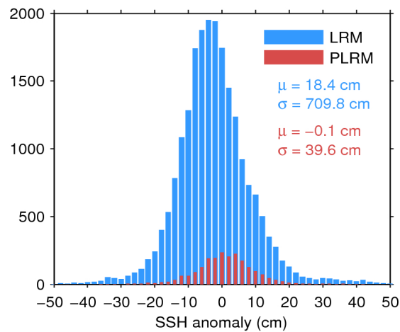
Figure 7. Histogram of flag-valid SSH anomaly over oceans and lakes for LRM (blue) and PLRM (red) for 10/10/2016. The mean ( \mu ) and standard deviation ( \sigma ) are also shown. Note that values outside [-50\ 50] cm are excluded from the histogram for the sake of readability but not from the computation of \mu and \sigma .
