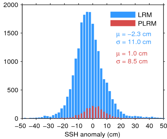
Figure 11. Histogram of science-valid SSH anomaly over oceans and lakes for LRM (blue) and PLRM (red) for 10/10/2016. The mean ( \mu ) and standard deviation ( \sigma ) are also shown. Note that values outside [-50 50] cm are excluded from the histogram for the sake of readability but not from the computation of \mu and \sigma .
