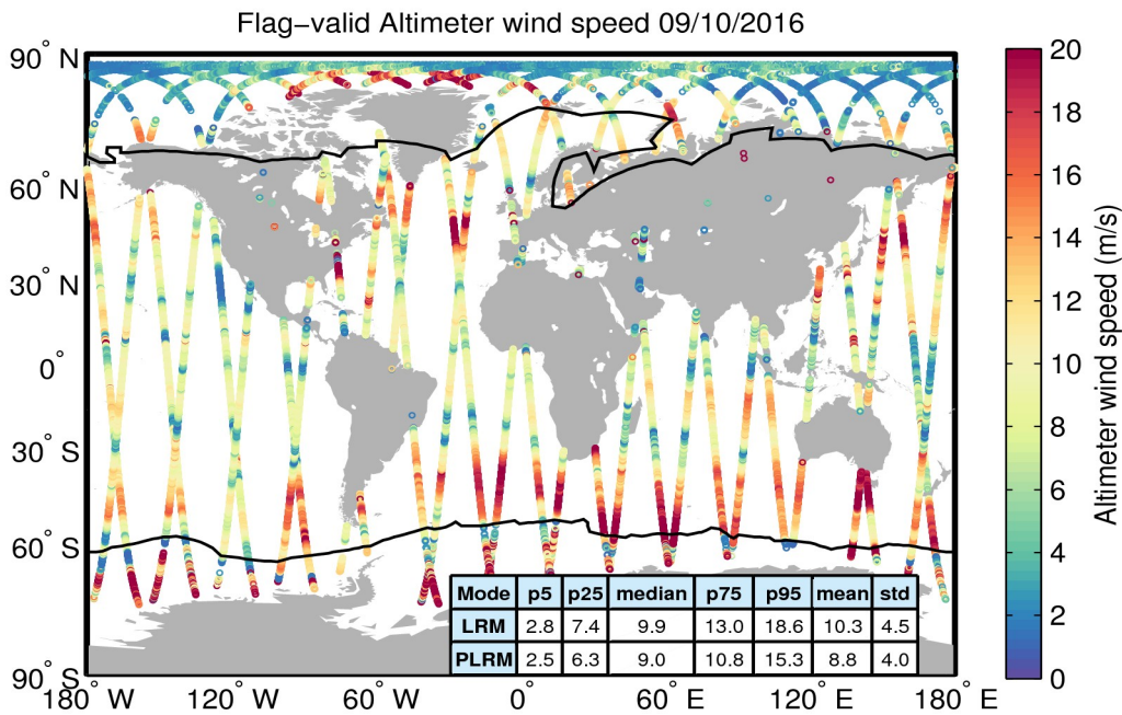
Figure 31. Geographical distribution of flag-valid wind data over oceans and lakes for 09/10/2016. The statistical values shown in the table refer to the wind in m/s and are calculated separately for LRM and PLRM regions. Measurements taken over polar polygons have been excluded from the computation of the statistical values. The black lines mark the outer limit of the Arctic and Antarctic polar polygons.
