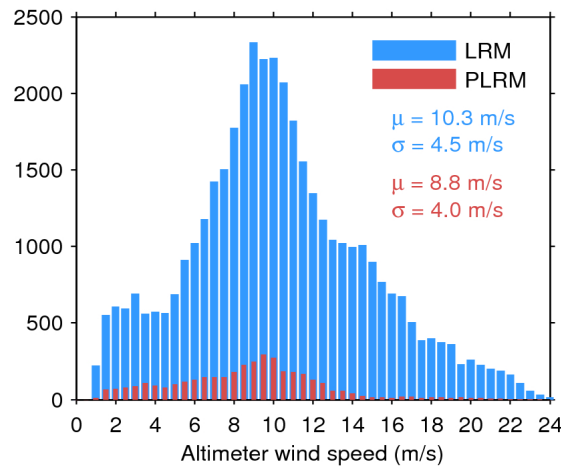
Figure 33. Histogram of flag-valid wind over oceans and lakes for LRM (blue) and PLRM (red) for 09/10/2016. The mean ( \mu ) and standard deviation ( \sigma ) are also shown. Note that values larger than 24 m/s are excluded from the histogram for the sake of readability but not from the computation of \mu and \sigma .
