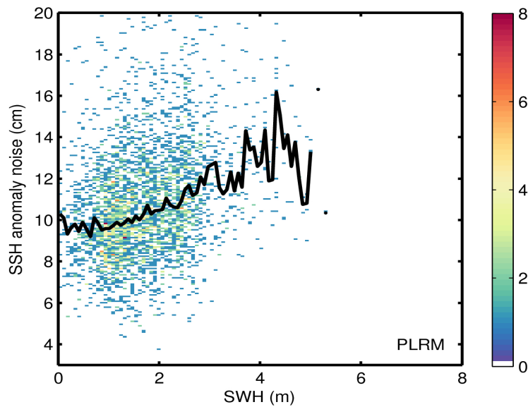
Figure 9. 2D histogram showing flag-valid SSH anomaly noise as a function of SWH for LRM (top) and PLRM (bottom) for 09/10/2016. The black line denotes the median SSH anomaly noise as a function of SWH.
