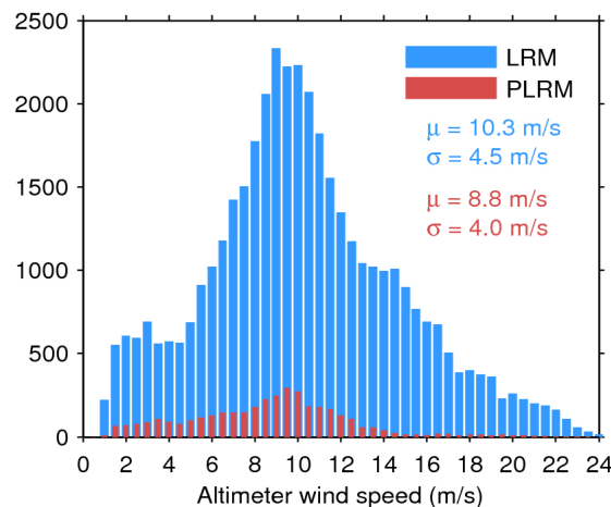
Figure 35. Histogram of science-valid wind over oceans and lakes for LRM (blue) and PLRM (red) for 09/10/2016. The mean ( \mu ) and standard deviation ( \sigma ) are also shown. Note that values larger than 24 m/s are excluded from the histogram for the sake of readability but not from the computation of \mu and \sigma .
