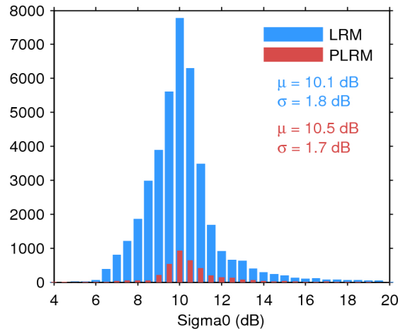
Figure 25. Histogram of flag-valid sigma0 over oceans and lakes for LRM (blue) and PLRM (red) for 09/10/2016. The mean ( \mu ) and standard deviation ( \sigma ) are also shown. Note that values outside [4 20] dB are excluded from the histogram for the sake of readability but not from the computation of \mu and \sigma .
