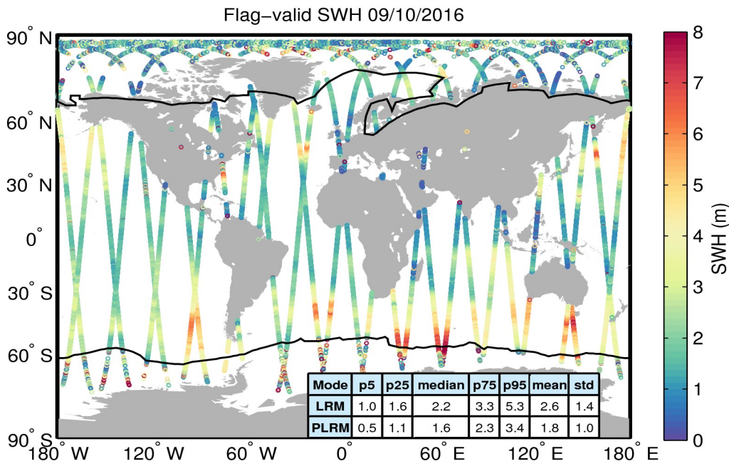
Figure 15. Geographical distribution of flag-valid SWH data over oceans and lakes for 09/10/2016. The statistical values shown in the table refer to the SWH in m and are calculated separately for LRM and PLRM regions. Measurements taken over polar polygons have been excluded from the computation of the statistical values. The black lines mark the outer limit of the Arctic and Antarctic polar polygons.
