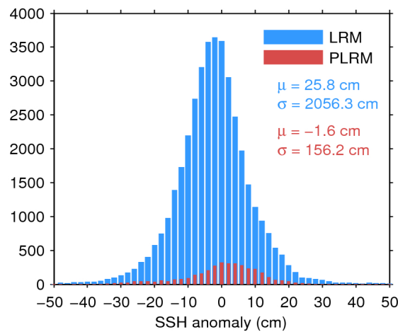
Figure 7. Histogram of flag-valid SSH anomaly over oceans and lakes for LRM (blue) and PLRM (red) for 09/10/2016. The mean ( \mu ) and standard deviation ( \sigma ) are also shown. Note that values outside [-50 50] cm are excluded from the histogram for the sake of readability but not from the computation of \mu and \sigma .
