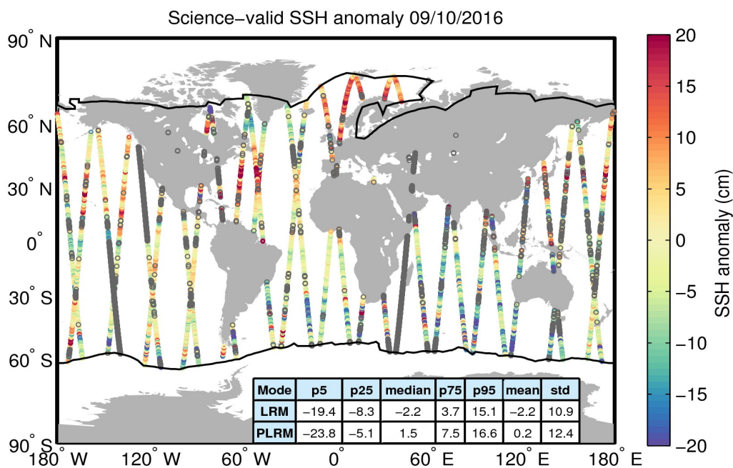
Figure 10. Geographical distribution of science-valid SSH anomaly data over oceans and lakes for 09/10/2016. The statistical values shown in the table refer to the SSH anomaly in cm and are calculated separately for LRM and PLRM regions. The black lines mark the outer limit of the Arctic and Antarctic polar polygons. Gray circles denote records that have been rejected based on the editing criteria described in Table 2.
