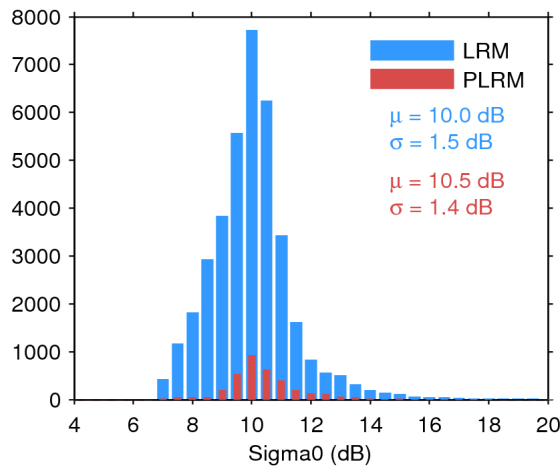
Figure 28. Histogram of science-valid sigma0 over oceans and lakes for LRM (blue) and PLRM (red) for 09/10/2016. The mean ( \mu ) and standard deviation ( \sigma ) are also shown. Note that values outside [4 20] dB are excluded from the histogram for the sake of readability but not from the computation of \mu and \sigma .
