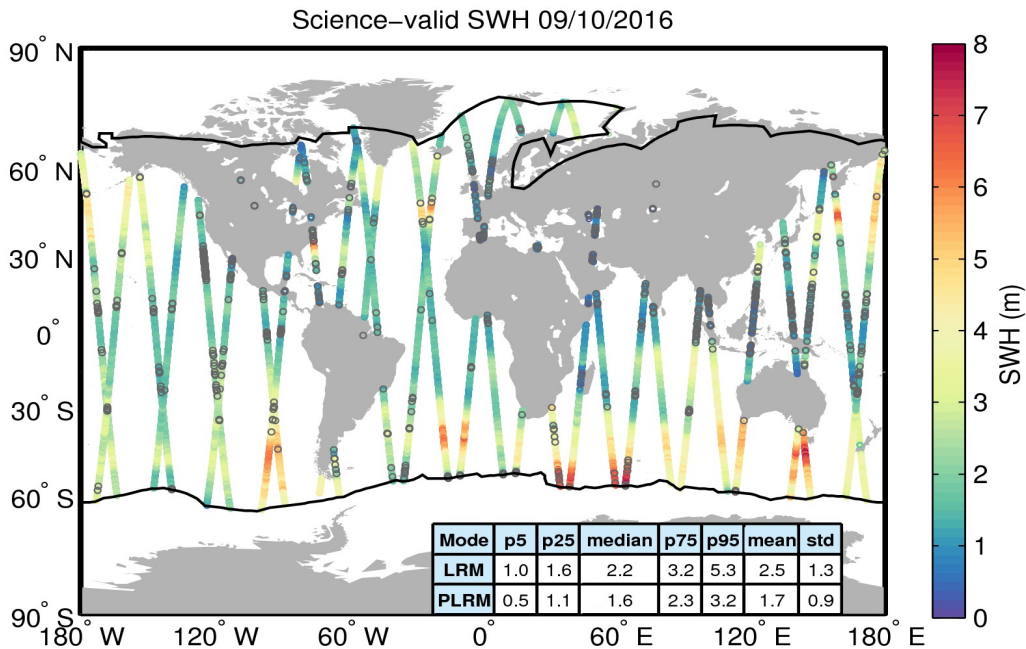
Figure 19. Geographical distribution of science-valid SWH data over oceans and lakes for 09/10/2016. The statistical values shown in the table refer to the SWH in m and are calculated separately for LRM and PLRM regions. The black lines mark the outer limit of the Arctic and Antarctic polar polygons. Gray circles denote records that have been rejected based on the editing criteria described in Table 3.
