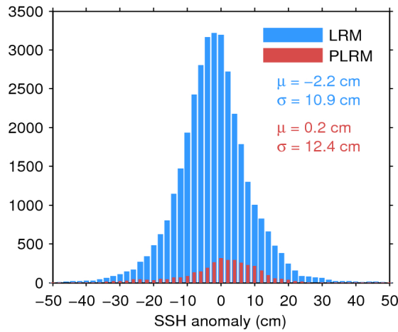
Figure 11. Histogram of science-valid SSH anomaly over oceans and lakes for LRM (blue) and PLRM (red) for 09/10/2016. The mean ( \mu ) and standard deviation ( \sigma ) are also shown. Note that values outside [-50\ 50] cm are excluded from the histogram for the sake of readability but not from the computation of \mu and \sigma .
