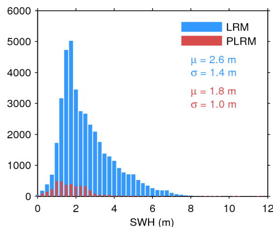
Figure 17. Histogram of flag-valid SWH over oceans and lakes for LRM (blue) and PLRM (red) for 09/10/2016. The mean ( \mu ) and standard deviation ( \sigma ) are also shown. Note that values larger than 12 m are excluded from the histogram for the sake of readability but not from the computation of \mu and \sigma .
