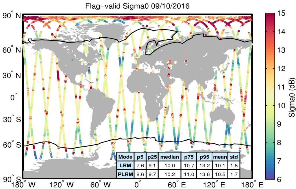
Figure 23. Geographical distribution of flag-valid sigma0 data over oceans and lakes for 09/10/2016. The statistical values shown in the table refer to the sigma0 in dB and are calculated separately for LRM and PLRM regions. Measurements taken over polar polygons have been excluded from the computation of the statistical values. The black lines mark the outer limit of the Arctic and Antarctic polar polygons.
