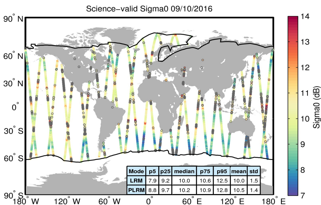
Figure 27. Geographical distribution of science-valid sigma0 data over oceans and lakes for 09/10/2016. The statistical values shown in the table refer to the sigma0 in dB and are calculated separately for LRM and PLRM regions. The black lines mark the outer limit of the Arctic and Antarctic polar polygons. Gray circles denote records that have been rejected based on the editing criteria described in Table 4.
