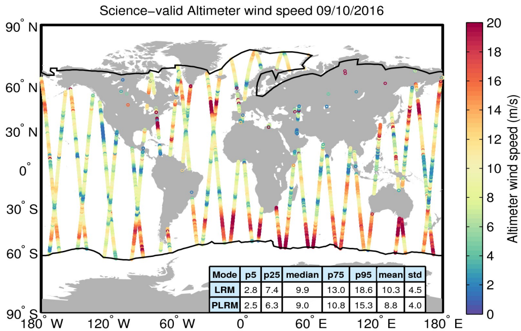
Figure 34. Geographical distribution of science-valid wind data over oceans and lakes for 09/10/2016. The statistical values shown in the table refer to the wind in m/s and are calculated separately for LRM and PLRM regions. The black lines mark the outer limit of the Arctic and Antarctic polar polygons. Gray circles denote records that have been rejected based on the editing criteria described in Table 5.
