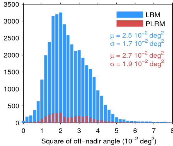
Figure 39. Histogram of flag-valid mispointing over oceans and lakes for LRM (blue) and PLRM (red) for 09/10/2016. Only positive values have been considered. The mean ( \mu ) and standard deviation ( \sigma ) are also shown. Note that values larger than 8 \cdot 10^{-2} \text{ deg}^2 are excluded from the histogram for the sake of readability but not from the computation of \mu and \sigma .
