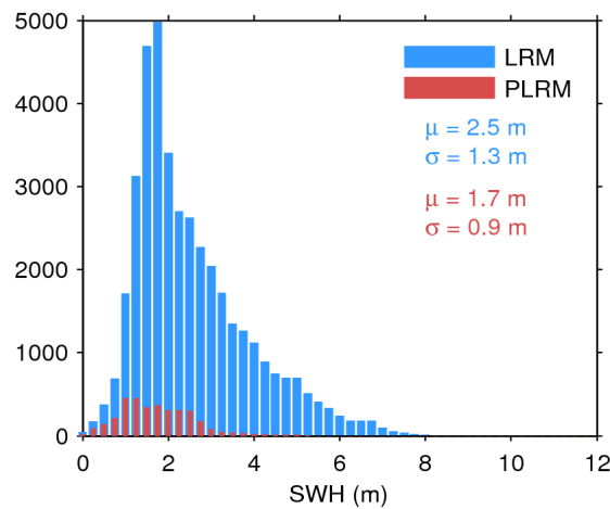
Figure 20. Histogram of science-valid SWH over oceans and lakes for LRM (blue) and PLRM (red) for 09/10/2016. The mean ( \mu ) and standard deviation ( \sigma ) are also shown. Note that values larger than 12 m are excluded from the histogram for the sake of readability but not from the computation of \mu and \sigma .
