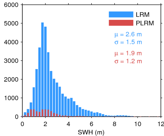
Figure 17. Histogram of flag-valid SWH over oceans and lakes for LRM (blue) and PLRM (red) for 07/10/2016. The mean ( \mu ) and standard deviation ( \sigma ) are also shown. Note that values larger than 12 m are excluded from the histogram for the sake of readability but not from the computation of \mu and \sigma .
