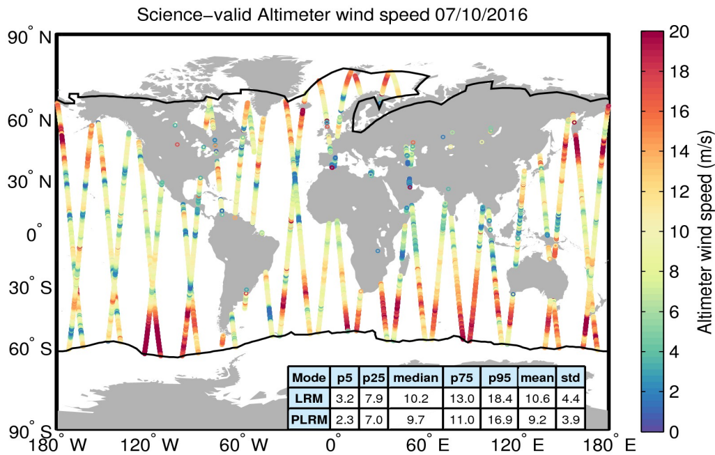
Figure 34. Geographical distribution of science-valid wind data over oceans and lakes for 07/10/2016. The statistical values shown in the table refer to the wind in m/s and are calculated separately for LRM and PLRM regions. The black lines mark the outer limit of the Arctic and Antarctic polar polygons. Gray circles denote records that have been rejected based on the editing criteria described in Table 5.
