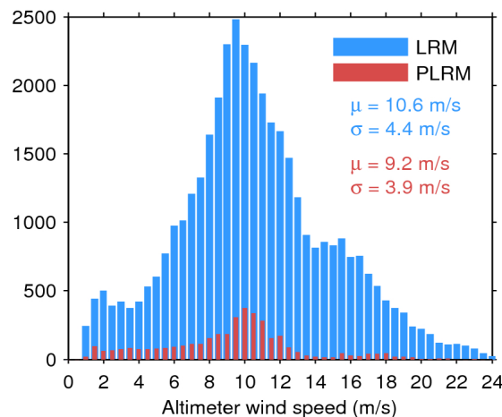
Figure 35. Histogram of science-valid wind over oceans and lakes for LRM (blue) and PLRM (red) for 07/10/2016. The mean ( \mu ) and standard deviation ( \sigma ) are also shown. Note that values larger than 24 m/s are excluded from the histogram for the sake of readability but not from the computation of \mu and \sigma .
