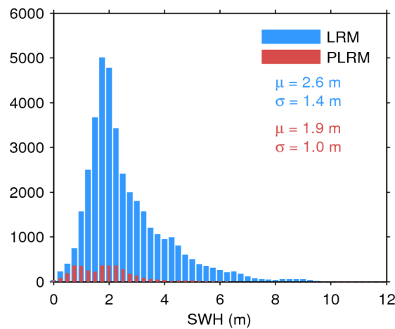
Figure 20. Histogram of science-valid SWH over oceans and lakes for LRM (blue) and PLRM (red) for 07/10/2016. The mean ( \mu ) and standard deviation ( \sigma ) are also shown. Note that values larger than 12 m are excluded from the histogram for the sake of readability but not from the computation of \mu and \sigma .
