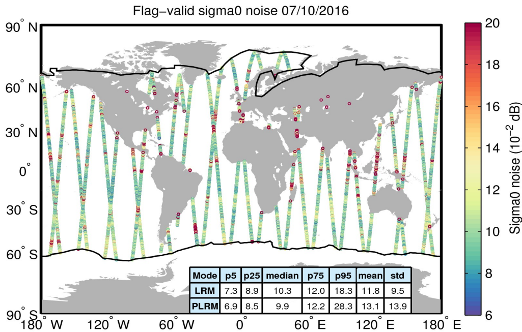
Figure 26. Geographical distribution of flag-valid 20-Hz sigma0 measurement noise over oceans and lakes for 07/10/2016. The statistical values shown in the table refer to the sigma0 noise and are calculated separately for LRM and PLRM regions. Measurements taken over polar polygons have been excluded from the computation of the statistical values. The black lines mark the outer limit of the Arctic and Antarctic polar polygons.
