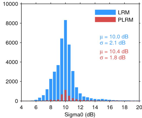
Figure 25. Histogram of flag-valid sigma0 over oceans and lakes for LRM (blue) and PLRM (red) for 07/10/2016. The mean ( \mu ) and standard deviation ( \sigma ) are also shown. Note that values outside [4 20] dB are excluded from the histogram for the sake of readability but not from the computation of \mu and \sigma .
