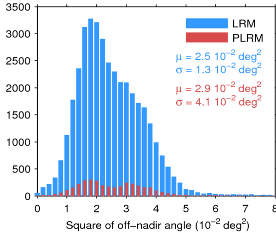
Figure 39. Histogram of flag-valid mispointing over oceans and lakes for LRM (blue) and PLRM (red) for 07/10/2016. Only positive values have been considered. The mean ( \mu ) and standard deviation ( \sigma ) are also shown. Note that values larger than 8 \cdot 10^{-2} \text{ deg}^2 are excluded from the histogram for the sake of readability but not from the computation of \mu and \sigma .
