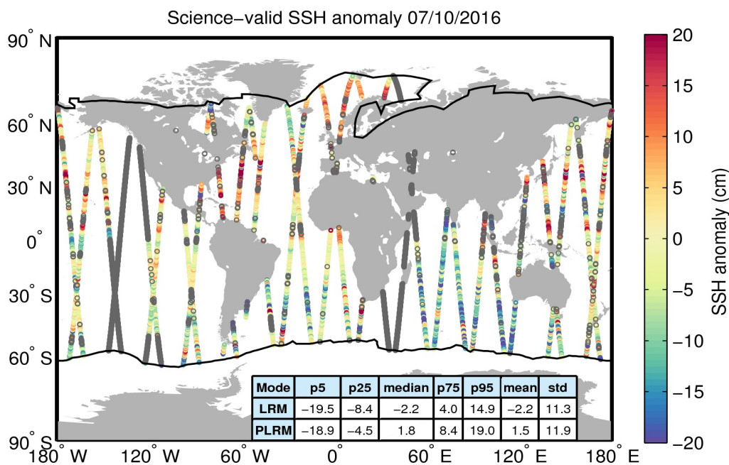
Figure 10. Geographical distribution of science-valid SSH anomaly data over oceans and lakes for 07/10/2016. The statistical values shown in the table refer to the SSH anomaly in cm and are calculated separately for LRM and PLRM regions. The black lines mark the outer limit of the Arctic and Antarctic polar polygons. Gray circles denote records that have been rejected based on the editing criteria described in Table 2.
