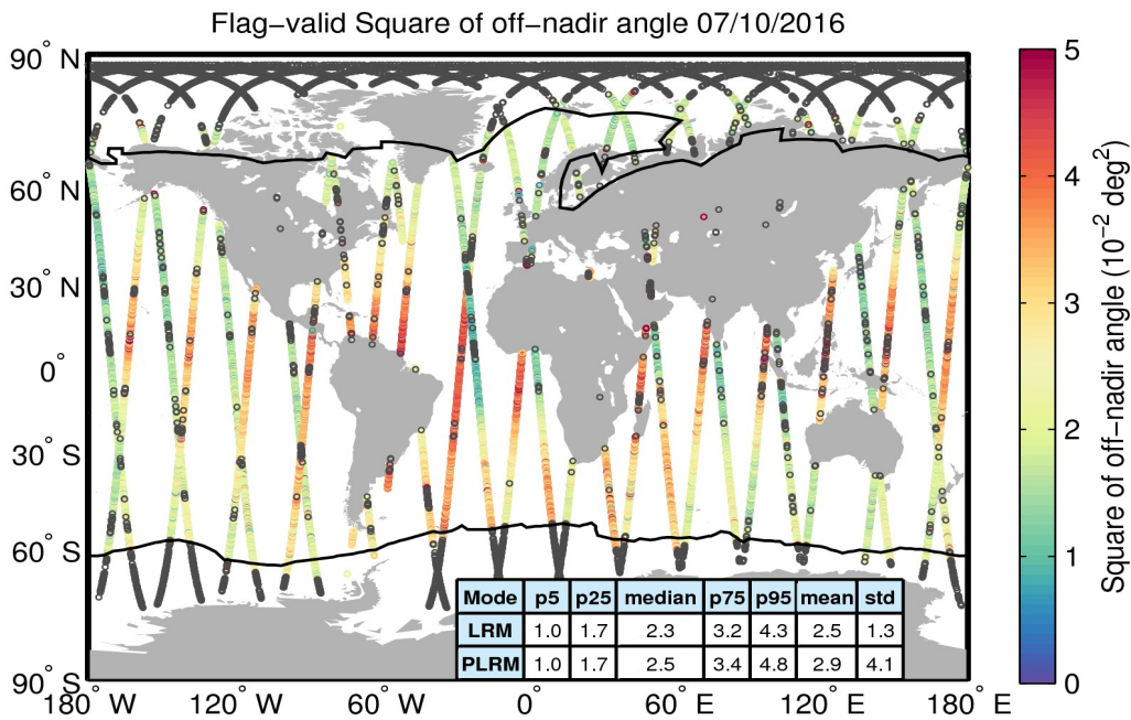
Figure 37. Geographical distribution of flag-valid mispointing data over oceans and lakes for 07/10/2016. The statistical values shown in the table refer to the mispointing in 10^{-2} deg 2 and are calculated separately for LRM and PLRM regions. Measurements taken over polar polygons have been excluded from the computation of the statistical values. The black lines mark the outer limit of the Arctic and Antarctic polar polygons. Gray circles denote negative values.
