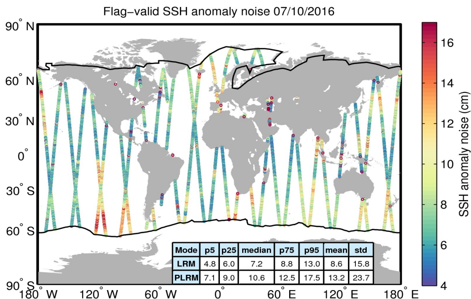
Figure 8. Geographical distribution of flag-valid 20-Hz SSH anomaly measurement noise over oceans and lakes for 07/10/2016. The statistical values shown in the table refer to the SSH anomaly noise and are calculated separately for LRM and PLRM regions. Measurements taken over polar polygons have been excluded from the computation of the statistical values. The black lines mark the outer limit of the Arctic and Antarctic polar polygons.
