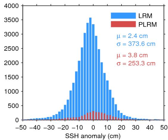
Figure 7. Histogram of flag-valid SSH anomaly over oceans and lakes for LRM (blue) and PLRM (red) for 07/10/2016. The mean ( \mu ) and standard deviation ( \sigma ) are also shown. Note that values outside [-50\ 50] cm are excluded from the histogram for the sake of readability but not from the computation of \mu and \sigma .
