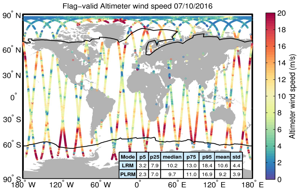
Figure 31. Geographical distribution of flag-valid wind data over oceans and lakes for 07/10/2016. The statistical values shown in the table refer to the wind in m/s and are calculated separately for LRM and PLRM regions. Measurements taken over polar polygons have been excluded from the computation of the statistical values. The black lines mark the outer limit of the Arctic and Antarctic polar polygons.
