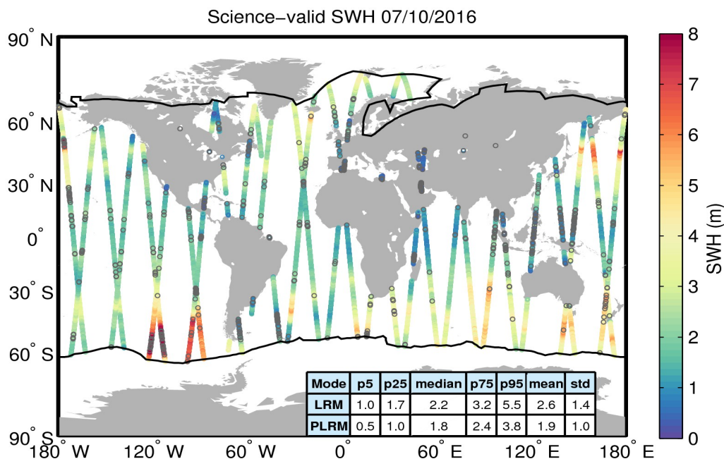
Figure 19. Geographical distribution of science-valid SWH data over oceans and lakes for 07/10/2016. The statistical values shown in the table refer to the SWH in m and are calculated separately for LRM and PLRM regions. The black lines mark the outer limit of the Arctic and Antarctic polar polygons. Gray circles denote records that have been rejected based on the editing criteria described in Table 3.
