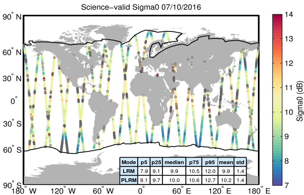
Figure 27. Geographical distribution of science-valid sigma0 data over oceans and lakes for 07/10/2016. The statistical values shown in the table refer to the sigma0 in dB and are calculated separately for LRM and PLRM regions. The black lines mark the outer limit of the Arctic and Antarctic polar polygons. Gray circles denote records that have been rejected based on the editing criteria described in Table 4.
