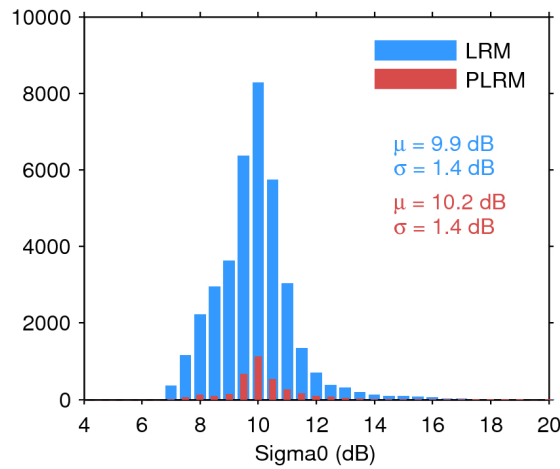
Figure 28. Histogram of science-valid sigma0 over oceans and lakes for LRM (blue) and PLRM (red) for 07/10/2016. The mean ( \mu ) and standard deviation ( \sigma ) are also shown. Note that values outside [4 20] dB are excluded from the histogram for the sake of readability but not from the computation of \mu and \sigma .
