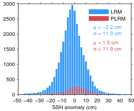
Figure 11. Histogram of science-valid SSH anomaly over oceans and lakes for LRM (blue) and PLRM (red) for 07/10/2016. The mean ( \mu ) and standard deviation ( \sigma ) are also shown. Note that values outside [-50 50] cm are excluded from the histogram for the sake of readability but not from the computation of \mu and \sigma .
