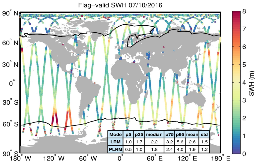
Figure 15. Geographical distribution of flag-valid SWH data over oceans and lakes for 07/10/2016. The statistical values shown in the table refer to the SWH in m and are calculated separately for LRM and PLRM regions. Measurements taken over polar polygons have been excluded from the computation of the statistical values. The black lines mark the outer limit of the Arctic and Antarctic polar polygons.
