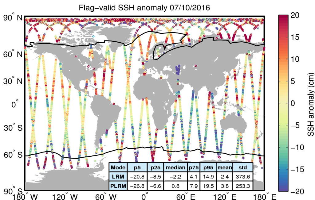
Figure 5. Geographical distribution of flag-valid 1-Hz SSH anomaly data over oceans and lakes for 07/10/2016. The statistical values shown in the table refer to the SSH anomaly in cm and are calculated separately for LRM and PLRM regions. Measurements taken over polar polygons have been excluded from the computation of the statistical values. The black lines mark the outer limit of the Arctic and Antarctic polar polygons.
