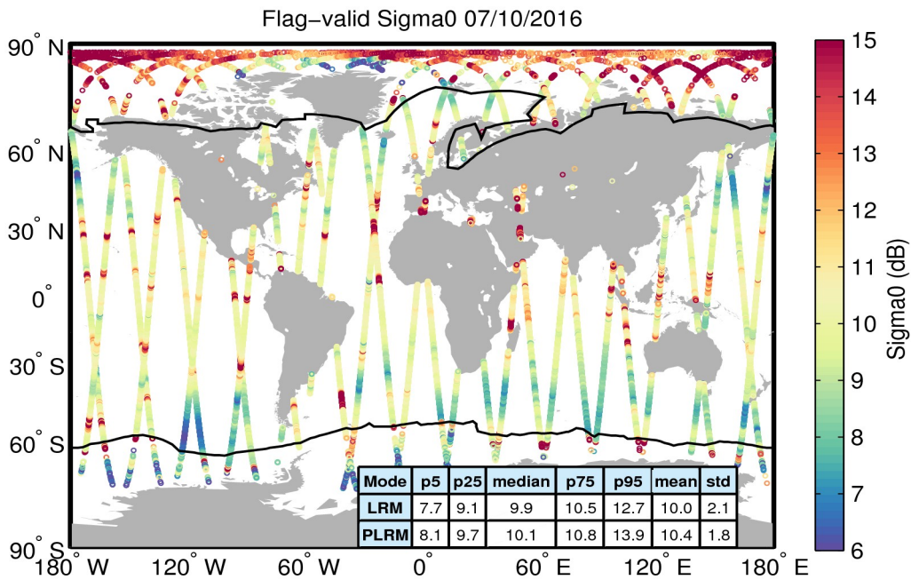
Figure 23. Geographical distribution of flag-valid sigma0 data over oceans and lakes for 07/10/2016. The statistical values shown in the table refer to the sigma0 in dB and are calculated separately for LRM and PLRM regions. Measurements taken over polar polygons have been excluded from the computation of the statistical values. The black lines mark the outer limit of the Arctic and Antarctic polar polygons.
