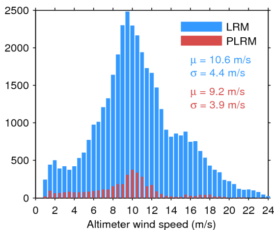
Figure 33. Histogram of flag-valid wind over oceans and lakes for LRM (blue) and PLRM (red) for 07/10/2016. The mean ( \mu ) and standard deviation ( \sigma ) are also shown. Note that values larger than 24 m/s are excluded from the histogram for the sake of readability but not from the computation of \mu and \sigma .
