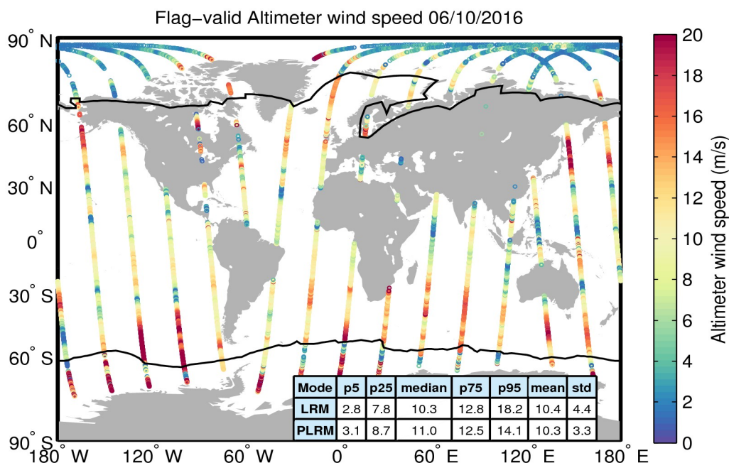
Figure 31. Geographical distribution of flag-valid wind data over oceans and lakes for 06/10/2016. The statistical values shown in the table refer to the wind in m/s and are calculated separately for LRM and PLRM regions. Measurements taken over polar polygons have been excluded from the computation of the statistical values. The black lines mark the outer limit of the Arctic and Antarctic polar polygons.
