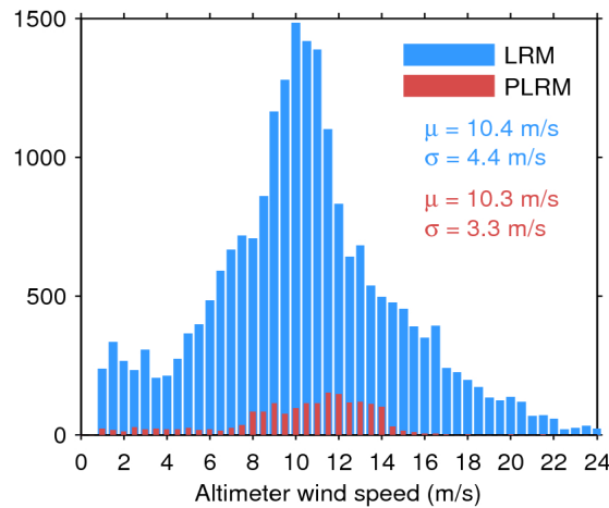
Figure 33. Histogram of flag-valid wind over oceans and lakes for LRM (blue) and PLRM (red) for 06/10/2016. The mean ( \mu ) and standard deviation ( \sigma ) are also shown. Note that values larger than 24 m/s are excluded from the histogram for the sake of readability but not from the computation of \mu and \sigma .
