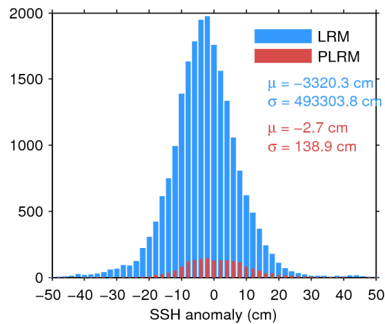
Figure 7. Histogram of flag-valid SSH anomaly over oceans and lakes for LRM (blue) and PLRM (red) for 06/10/2016. The mean ( \mu ) and standard deviation ( \sigma ) are also shown. Note that values outside [-50\ 50] cm are excluded from the histogram for the sake of readability but not from the computation of \mu and \sigma .
