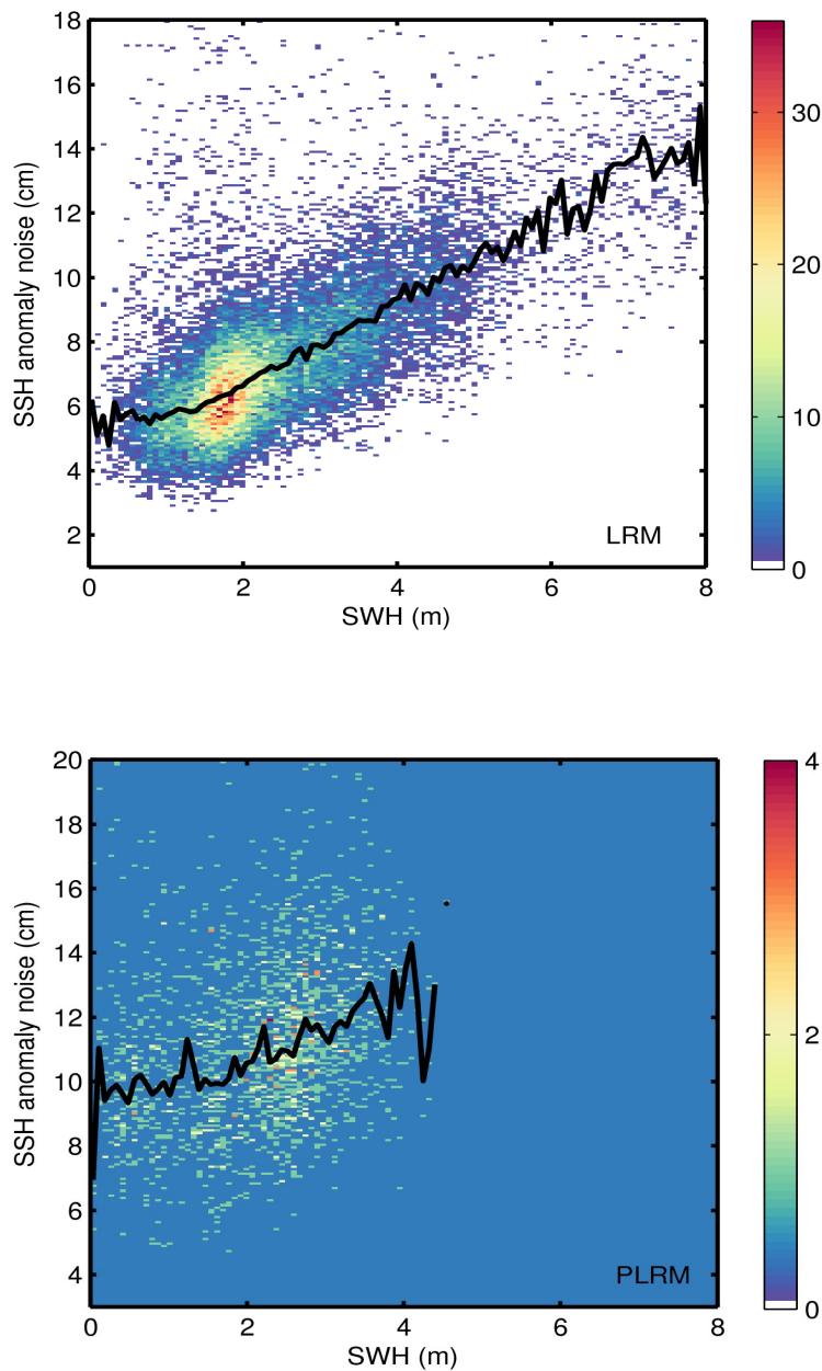
Figure 9. 2D histogram showing flag-valid SSH anomaly noise as a function of SWH for LRM (top) and PLRM (bottom) for 06/10/2016. The black line denotes the median SSH anomaly noise as a function of SWH.
