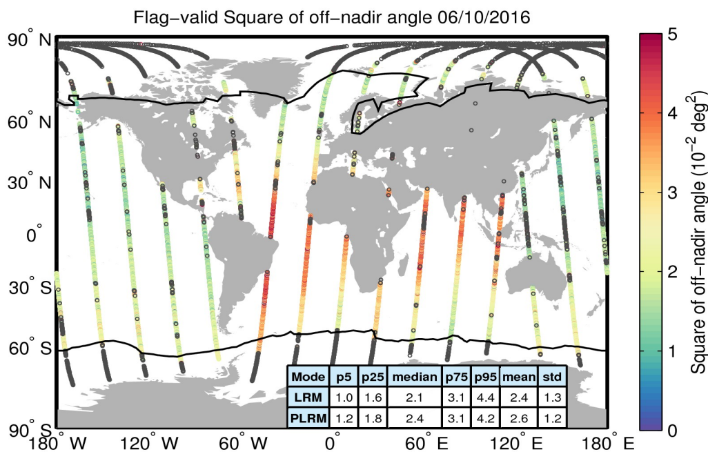
Figure 37. Geographical distribution of flag-valid mispointing data over oceans and lakes for 06/10/2016. The statistical values shown in the table refer to the mispointing in 10^{-2} deg 2 and are calculated separately for LRM and PLRM regions. Measurements taken over polar polygons have been excluded from the computation of the statistical values. The black lines mark the outer limit of the Arctic and Antarctic polar polygons. Gray circles denote negative values.
