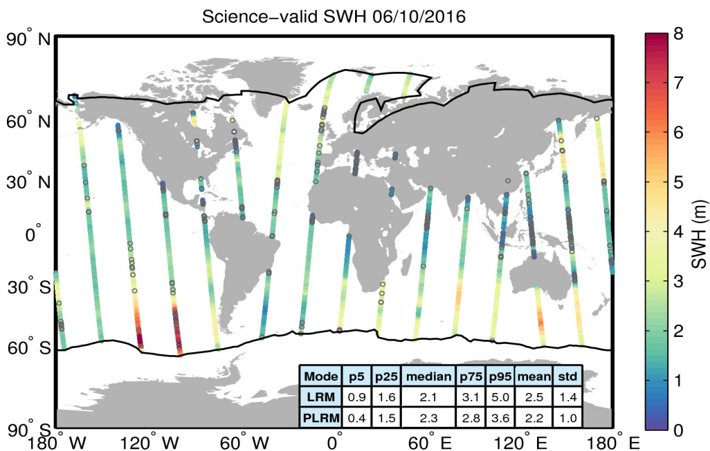
Figure 19. Geographical distribution of science-valid SWH data over oceans and lakes for 06/10/2016. The statistical values shown in the table refer to the SWH in m and are calculated separately for LRM and PLRM regions. The black lines mark the outer limit of the Arctic and Antarctic polar polygons. Gray circles denote records that have been rejected based on the editing criteria described in Table 3.
