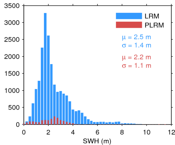
Figure 17. Histogram of flag-valid SWH over oceans and lakes for LRM (blue) and PLRM (red) for 06/10/2016. The mean ( \mu ) and standard deviation ( \sigma ) are also shown. Note that values larger than 12 m are excluded from the histogram for the sake of readability but not from the computation of \mu and \sigma .
