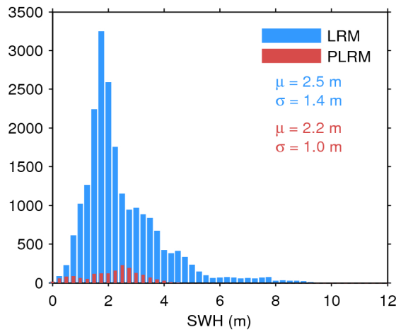
Figure 20. Histogram of science-valid SWH over oceans and lakes for LRM (blue) and PLRM (red) for 06/10/2016. The mean ( \mu ) and standard deviation ( \sigma ) are also shown. Note that values larger than 12 m are excluded from the histogram for the sake of readability but not from the computation of \mu and \sigma .
