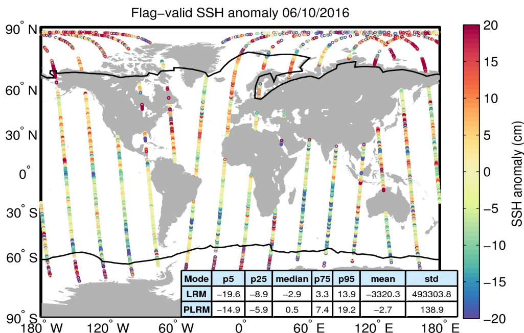
Figure 5. Geographical distribution of flag-valid 1-Hz SSH anomaly data over oceans and lakes for 06/10/2016. The statistical values shown in the table refer to the SSH anomaly in cm and are calculated separately for LRM and PLRM regions. Measurements taken over polar polygons have been excluded from the computation of the statistical values. The black lines mark the outer limit of the Arctic and Antarctic polar polygons.
