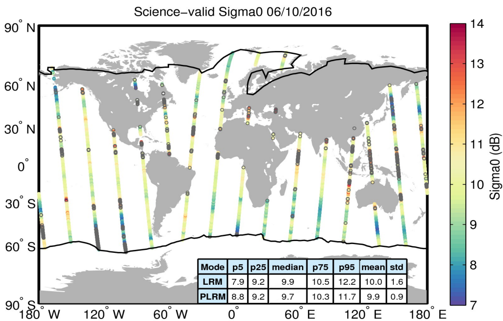
Figure 27. Geographical distribution of science-valid sigma0 data over oceans and lakes for 06/10/2016. The statistical values shown in the table refer to the sigma0 in dB and are calculated separately for LRM and PLRM regions. The black lines mark the outer limit of the Arctic and Antarctic polar polygons. Gray circles denote records that have been rejected based on the editing criteria described in Table 4.
