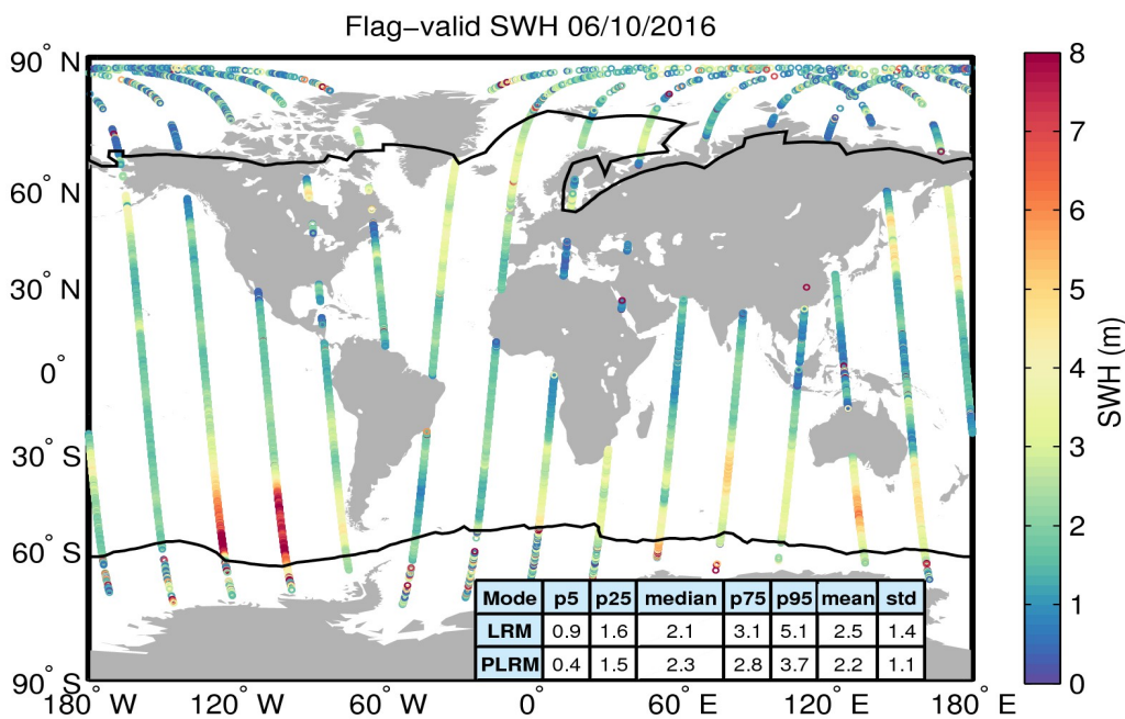
Figure 15. Geographical distribution of flag-valid SWH data over oceans and lakes for 06/10/2016. The statistical values shown in the table refer to the SWH in m and are calculated separately for LRM and PLRM regions. Measurements taken over polar polygons have been excluded from the computation of the statistical values. The black lines mark the outer limit of the Arctic and Antarctic polar polygons.
