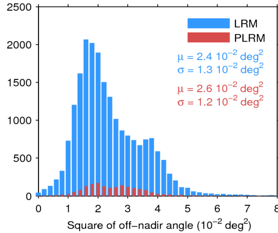
Figure 39. Histogram of flag-valid mispointing over oceans and lakes for LRM (blue) and PLRM (red) for 06/10/2016. Only positive values have been considered. The mean ( \mu ) and standard deviation ( \sigma ) are also shown. Note that values larger than 8 \cdot 10^{-2} \text{ deg}^2 are excluded from the histogram for the sake of readability but not from the computation of \mu and \sigma .
