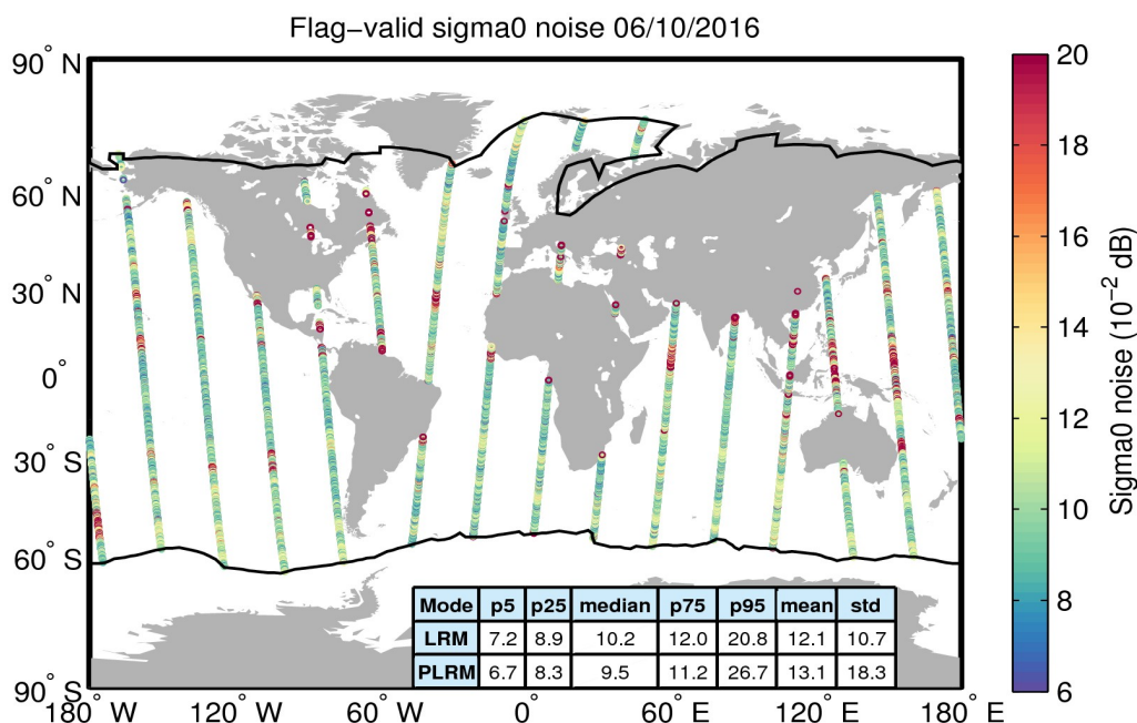
Figure 26. Geographical distribution of flag-valid 20-Hz sigma0 measurement noise over oceans and lakes for 06/10/2016. The statistical values shown in the table refer to the sigma0 noise and are calculated separately for LRM and PLRM regions. Measurements taken over polar polygons have been excluded from the computation of the statistical values. The black lines mark the outer limit of the Arctic and Antarctic polar polygons.
