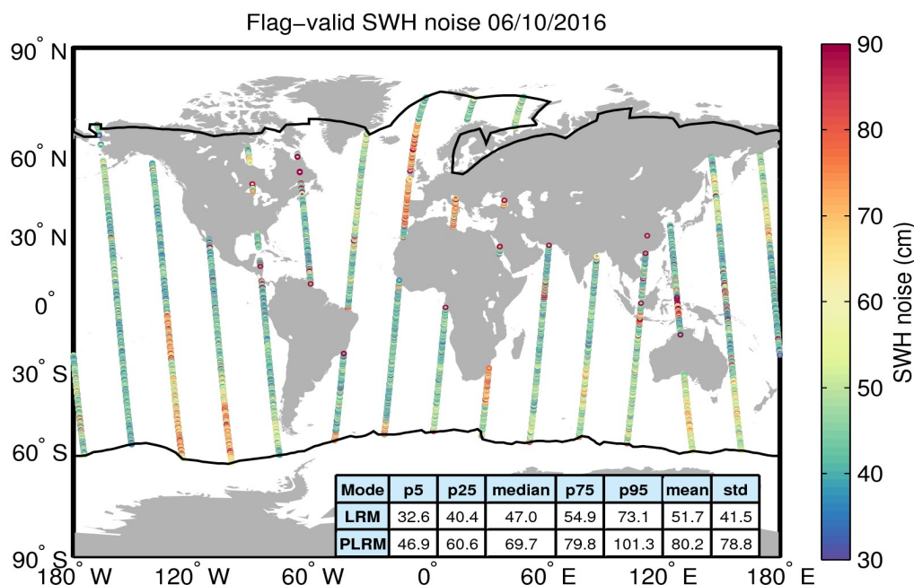
Figure 18. Geographical distribution of flag-valid 20-Hz SWH measurement noise over oceans and lakes for 06/10/2016. The statistical values shown in the table refer to the SWH noise and are calculated separately for LRM and PLRM regions. Measurements taken over polar polygons have been excluded from the computation of the statistical values. The black lines mark the outer limit of the Arctic and Antarctic polar polygons.
