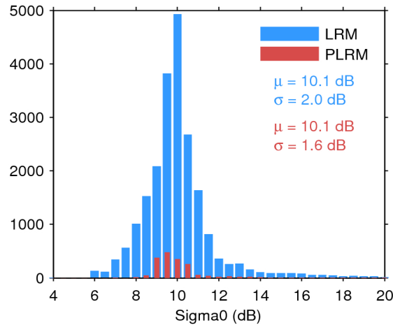
Figure 25. Histogram of flag-valid sigma0 over oceans and lakes for LRM (blue) and PLRM (red) for 06/10/2016. The mean ( \mu ) and standard deviation ( \sigma ) are also shown. Note that values outside [4 20] dB are excluded from the histogram for the sake of readability but not from the computation of \mu and \sigma .
