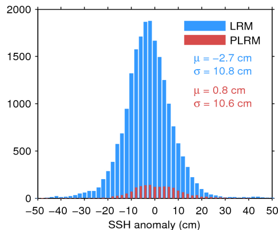
Figure 11. Histogram of science-valid SSH anomaly over oceans and lakes for LRM (blue) and PLRM (red) for 06/10/2016. The mean ( \mu ) and standard deviation ( \sigma ) are also shown. Note that values outside [-50 50] cm are excluded from the histogram for the sake of readability but not from the computation of \mu and \sigma .
