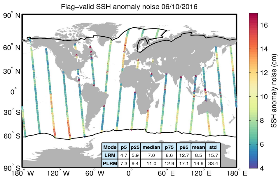
Figure 8. Geographical distribution of flag-valid 20-Hz SSH anomaly measurement noise over oceans and lakes for 06/10/2016. The statistical values shown in the table refer to the SSH anomaly noise and are calculated separately for LRM and PLRM regions. Measurements taken over polar polygons have been excluded from the computation of the statistical values. The black lines mark the outer limit of the Arctic and Antarctic polar polygons.
