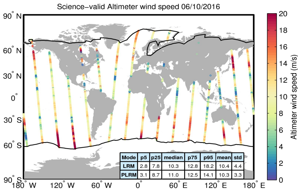
Figure 34. Geographical distribution of science-valid wind data over oceans and lakes for 06/10/2016. The statistical values shown in the table refer to the wind in m/s and are calculated separately for LRM and PLRM regions. The black lines mark the outer limit of the Arctic and Antarctic polar polygons. Gray circles denote records that have been rejected based on the editing criteria described in Table 5.
