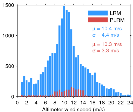
Figure 35. Histogram of science-valid wind over oceans and lakes for LRM (blue) and PLRM (red) for 06/10/2016. The mean ( \mu ) and standard deviation ( \sigma ) are also shown. Note that values larger than 24 m/s are excluded from the histogram for the sake of readability but not from the computation of \mu and \sigma .
