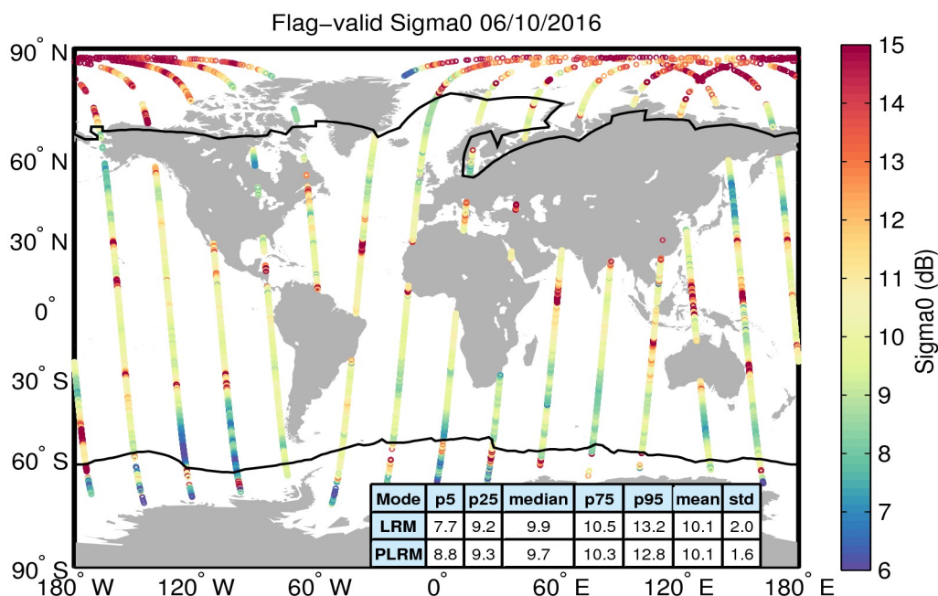
Figure 23. Geographical distribution of flag-valid sigma0 data over oceans and lakes for 06/10/2016. The statistical values shown in the table refer to the sigma0 in dB and are calculated separately for LRM and PLRM regions. Measurements taken over polar polygons have been excluded from the computation of the statistical values. The black lines mark the outer limit of the Arctic and Antarctic polar polygons.
