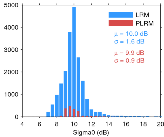
Figure 28. Histogram of science-valid sigma0 over oceans and lakes for LRM (blue) and PLRM (red) for 06/10/2016. The mean ( \mu ) and standard deviation ( \sigma ) are also shown. Note that values outside [4 20] dB are excluded from the histogram for the sake of readability but not from the computation of \mu and \sigma .
