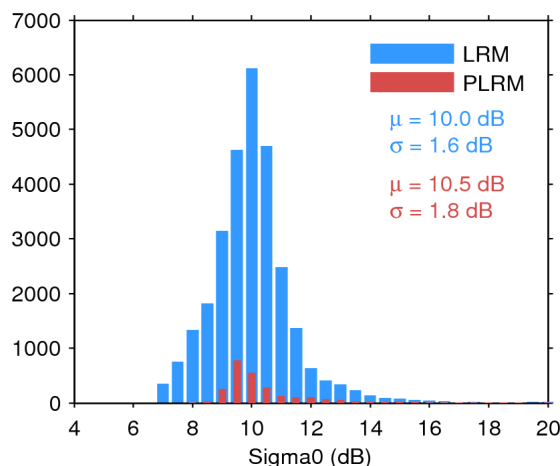
Figure 28. Histogram of science-valid sigma0 over oceans and lakes for LRM (blue) and PLRM (red) for 05/10/2016. The mean ( \mu ) and standard deviation ( \sigma ) are also shown. Note that values outside [4 20] dB are excluded from the histogram for the sake of readability but not from the computation of \mu and \sigma .
