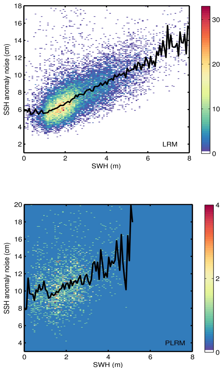
Figure 9. 2D histogram showing flag-valid SSH anomaly noise as a function of SWH for LRM (top) and PLRM (bottom) for 05/10/2016. The black line denotes the median SSH anomaly noise as a function of SWH.
