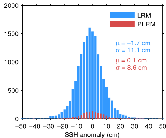
Figure 11. Histogram of science-valid SSH anomaly over oceans and lakes for LRM (blue) and PLRM (red) for 05/10/2016. The mean ( \mu ) and standard deviation ( \sigma ) are also shown. Note that values outside [-50 50] cm are excluded from the histogram for the sake of readability but not from the computation of \mu and \sigma .
