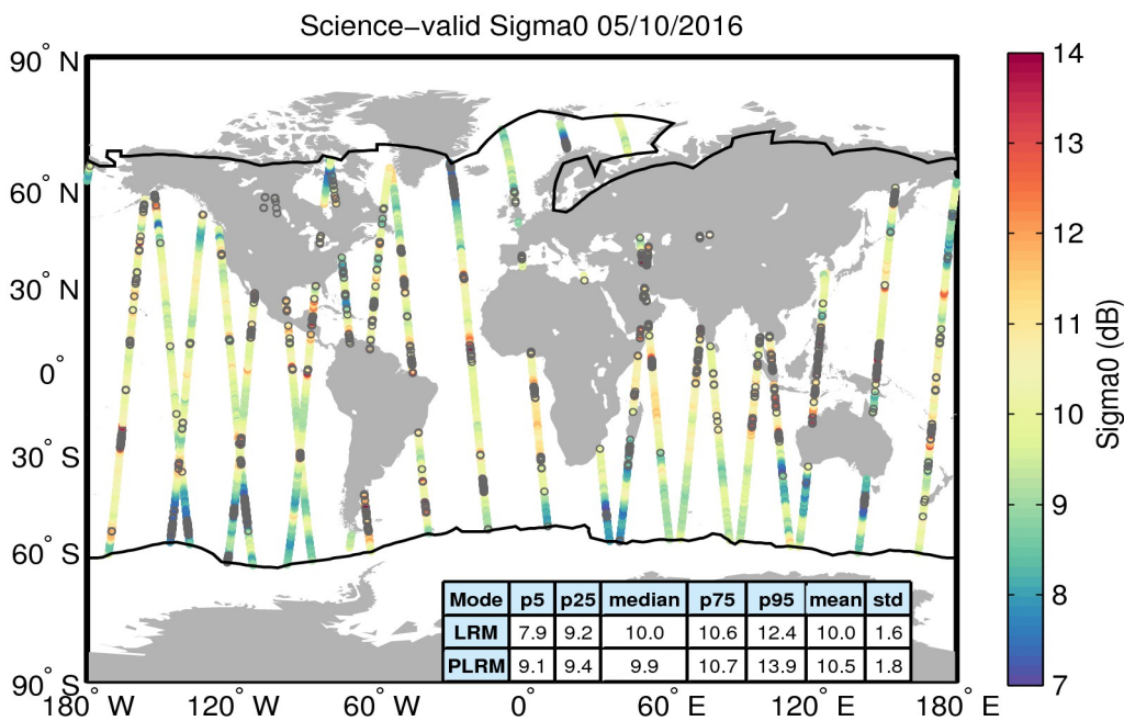
Figure 27. Geographical distribution of science-valid sigma0 data over oceans and lakes for 05/10/2016. The statistical values shown in the table refer to the sigma0 in dB and are calculated separately for LRM and PLRM regions. The black lines mark the outer limit of the Arctic and Antarctic polar polygons. Gray circles denote records that have been rejected based on the editing criteria described in Table 4.
