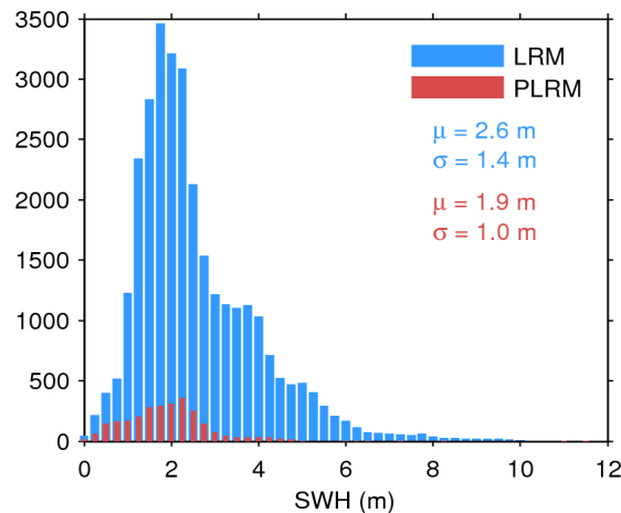
Figure 17. Histogram of flag-valid SWH over oceans and lakes for LRM (blue) and PLRM (red) for 05/10/2016. The mean ( \mu ) and standard deviation ( \sigma ) are also shown. Note that values larger than 12 m are excluded from the histogram for the sake of readability but not from the computation of \mu and \sigma .
