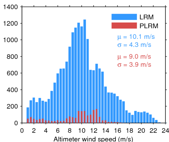
Figure 35. Histogram of science-valid wind over oceans and lakes for LRM (blue) and PLRM (red) for 05/10/2016. The mean ( \mu ) and standard deviation ( \sigma ) are also shown. Note that values larger than 24 m/s are excluded from the histogram for the sake of readability but not from the computation of \mu and \sigma .
