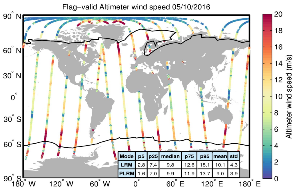
Figure 31. Geographical distribution of flag-valid wind data over oceans and lakes for 05/10/2016. The statistical values shown in the table refer to the wind in m/s and are calculated separately for LRM and PLRM regions. Measurements taken over polar polygons have been excluded from the computation of the statistical values. The black lines mark the outer limit of the Arctic and Antarctic polar polygons.
