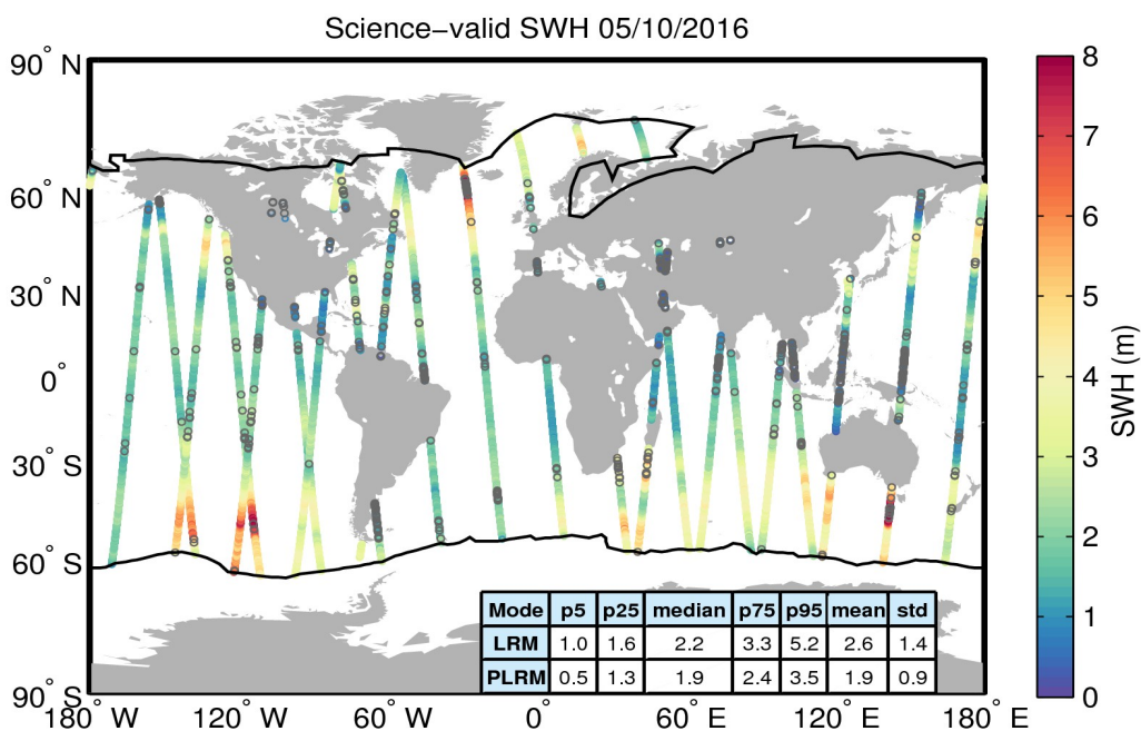
Figure 19. Geographical distribution of science-valid SWH data over oceans and lakes for 05/10/2016. The statistical values shown in the table refer to the SWH in m and are calculated separately for LRM and PLRM regions. The black lines mark the outer limit of the Arctic and Antarctic polar polygons. Gray circles denote records that have been rejected based on the editing criteria described in Table 3.
