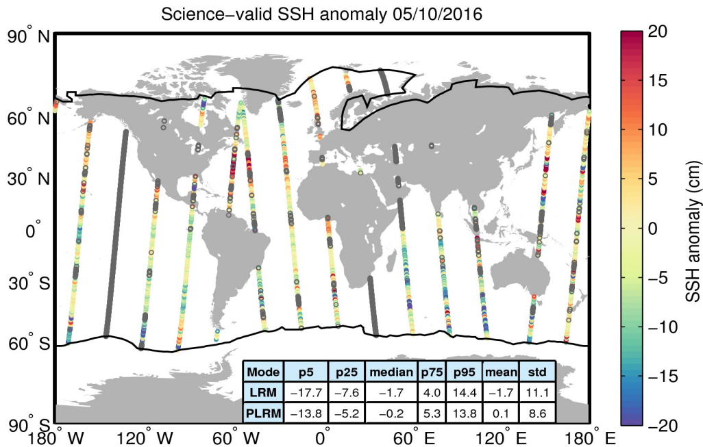
Figure 10. Geographical distribution of science-valid SSH anomaly data over oceans and lakes for 05/10/2016. The statistical values shown in the table refer to the SSH anomaly in cm and are calculated separately for LRM and PLRM regions. The black lines mark the outer limit of the Arctic and Antarctic polar polygons. Gray circles denote records that have been rejected based on the editing criteria described in Table 2.
