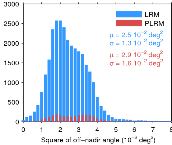
Figure 39. Histogram of flag-valid mispointing over oceans and lakes for LRM (blue) and PLRM (red) for 05/10/2016. Only positive values have been considered. The mean ( \mu ) and standard deviation ( \sigma ) are also shown. Note that values larger than 8 \cdot 10^{-2} \text{ deg}^2 are excluded from the histogram for the sake of readability but not from the computation of \mu and \sigma .
