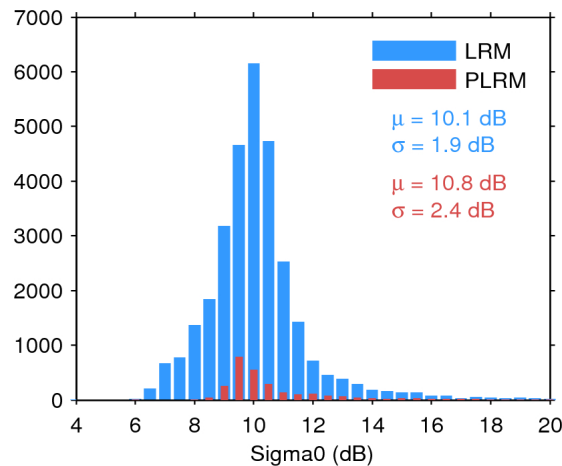
Figure 25. Histogram of flag-valid sigma0 over oceans and lakes for LRM (blue) and PLRM (red) for 05/10/2016. The mean ( \mu ) and standard deviation ( \sigma ) are also shown. Note that values outside [4 20] dB are excluded from the histogram for the sake of readability but not from the computation of \mu and \sigma .
