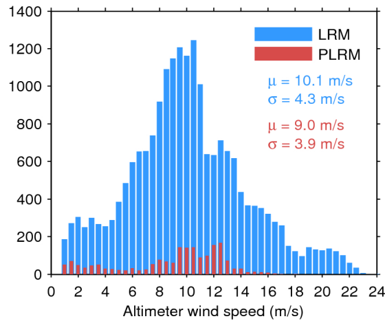
Figure 33. Histogram of flag-valid wind over oceans and lakes for LRM (blue) and PLRM (red) for 05/10/2016. The mean ( \mu ) and standard deviation ( \sigma ) are also shown. Note that values larger than 24 m/s are excluded from the histogram for the sake of readability but not from the computation of \mu and \sigma .
