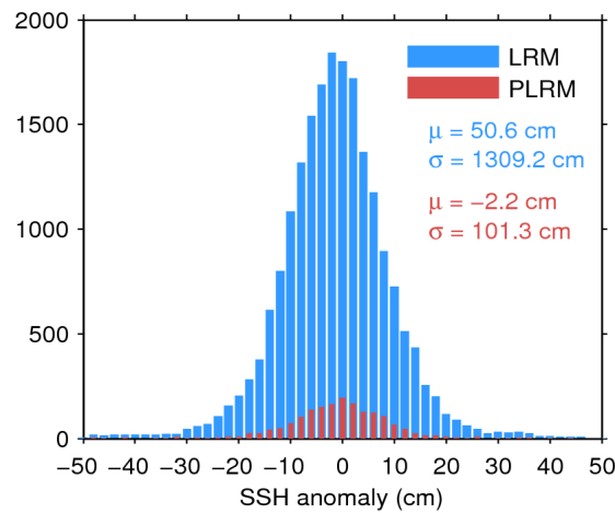
Figure 7. Histogram of flag-valid SSH anomaly over oceans and lakes for LRM (blue) and PLRM (red) for 05/10/2016. The mean ( \mu ) and standard deviation ( \sigma ) are also shown. Note that values outside [-50 \ 50] cm are excluded from the histogram for the sake of readability but not from the computation of \mu and \sigma .
