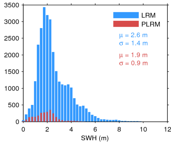
Figure 20. Histogram of science-valid SWH over oceans and lakes for LRM (blue) and PLRM (red) for 05/10/2016. The mean ( \mu ) and standard deviation ( \sigma ) are also shown. Note that values larger than 12 m are excluded from the histogram for the sake of readability but not from the computation of \mu and \sigma .
