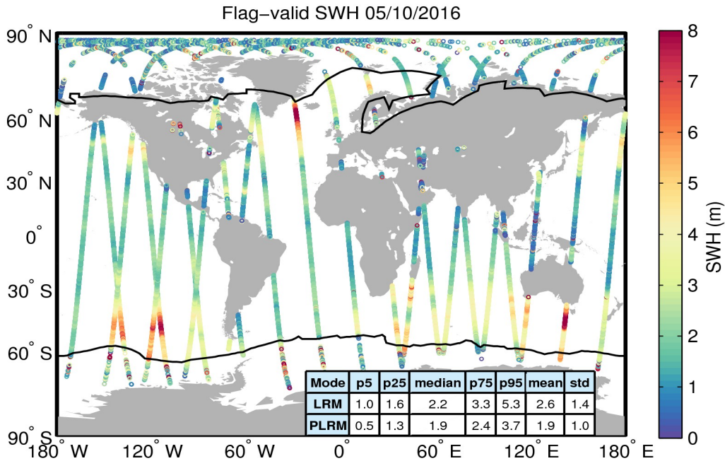
Figure 15. Geographical distribution of flag-valid SWH data over oceans and lakes for 05/10/2016. The statistical values shown in the table refer to the SWH in m and are calculated separately for LRM and PLRM regions. Measurements taken over polar polygons have been excluded from the computation of the statistical values. The black lines mark the outer limit of the Arctic and Antarctic polar polygons.
