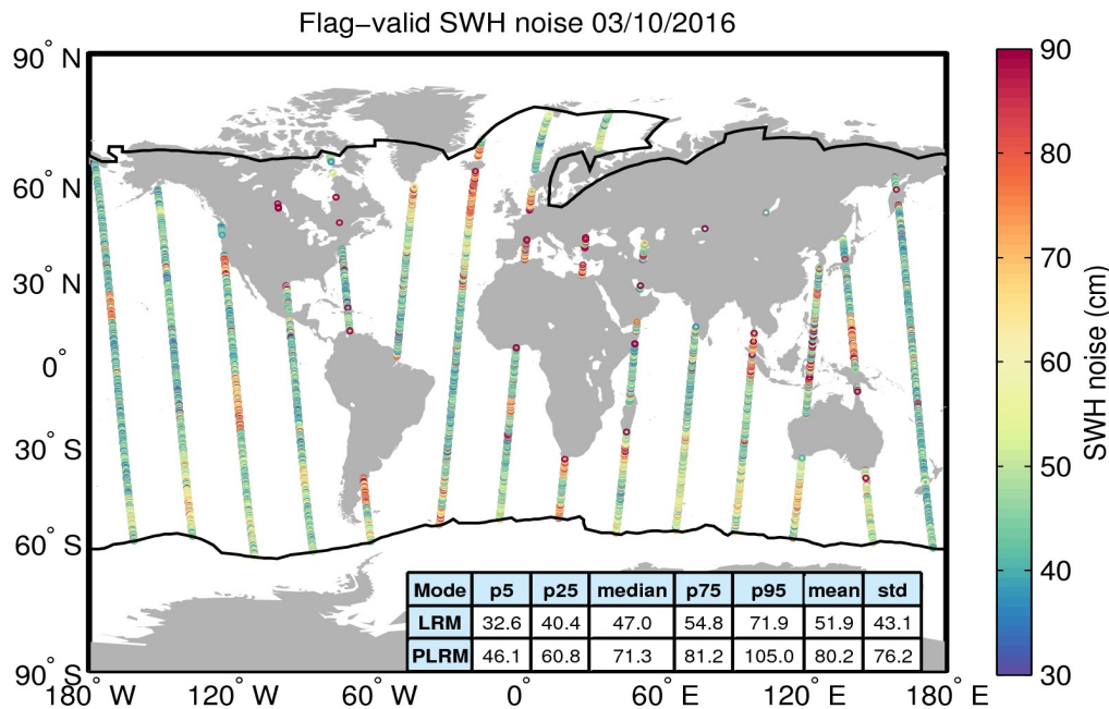
Figure 18. Geographical distribution of flag-valid 20-Hz SWH measurement noise over oceans and lakes for 03/10/2016. The statistical values shown in the table refer to the SWH noise and are calculated separately for LRM and PLRM regions. Measurements taken over polar polygons have been excluded from the computation of the statistical values. The black lines mark the outer limit of the Arctic and Antarctic polar polygons.
