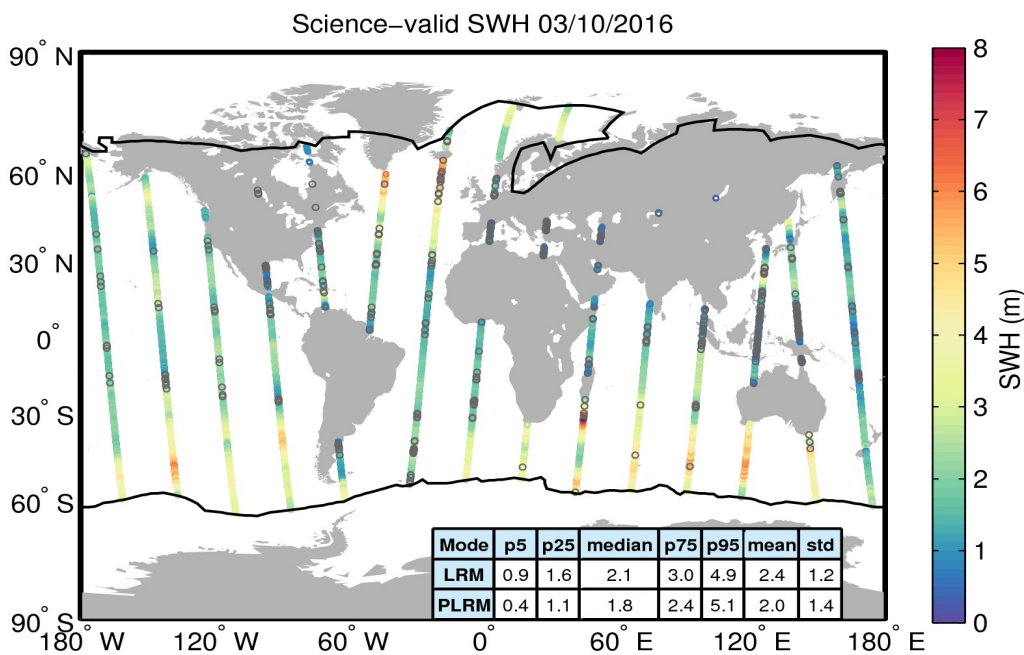
Figure 19. Geographical distribution of science-valid SWH data over oceans and lakes for 03/10/2016. The statistical values shown in the table refer to the SWH in m and are calculated separately for LRM and PLRM regions. The black lines mark the outer limit of the Arctic and Antarctic polar polygons. Gray circles denote records that have been rejected based on the editing criteria described in Table 3.
