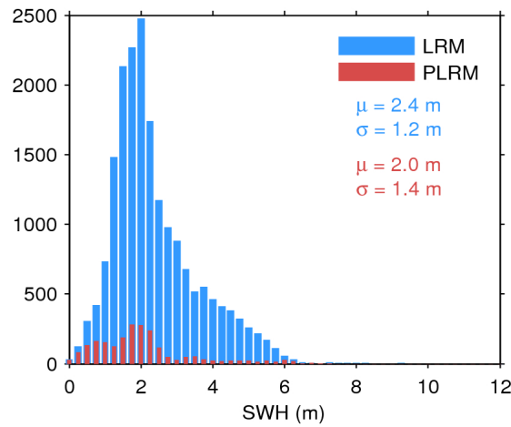
Figure 20. Histogram of science-valid SWH over oceans and lakes for LRM (blue) and PLRM (red) for 03/10/2016. The mean ( \mu ) and standard deviation ( \sigma ) are also shown. Note that values larger than 12 m are excluded from the histogram for the sake of readability but not from the computation of \mu and \sigma .
