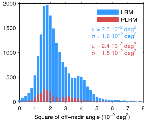
Figure 39. Histogram of flag-valid mispointing over oceans and lakes for LRM (blue) and PLRM (red) for 03/10/2016. Only positive values have been considered. The mean ( \mu ) and standard deviation ( \sigma ) are also shown. Note that values larger than 8 \cdot 10^{-2} \text{ deg}^2 are excluded from the histogram for the sake of readability but not from the computation of \mu and \sigma .
