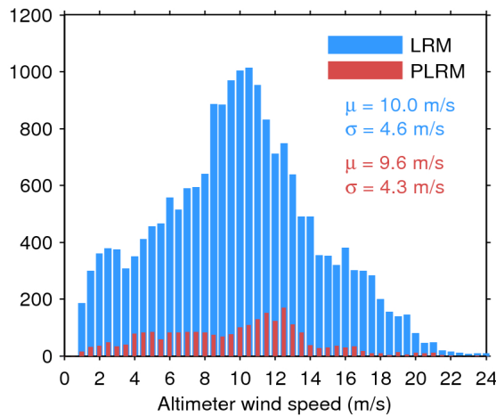
Figure 33. Histogram of flag-valid wind over oceans and lakes for LRM (blue) and PLRM (red) for 03/10/2016. The mean ( \mu ) and standard deviation ( \sigma ) are also shown. Note that values larger than 24 m/s are excluded from the histogram for the sake of readability but not from the computation of \mu and \sigma .
