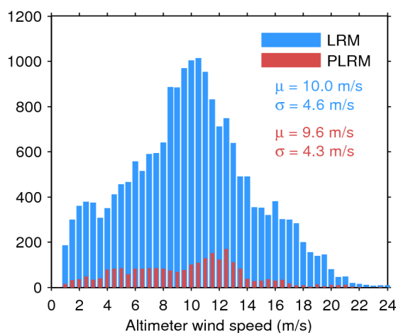
Figure 35. Histogram of science-valid wind over oceans and lakes for LRM (blue) and PLRM (red) for 03/10/2016. The mean ( \mu ) and standard deviation ( \sigma ) are also shown. Note that values larger than 24 m/s are excluded from the histogram for the sake of readability but not from the computation of \mu and \sigma .
