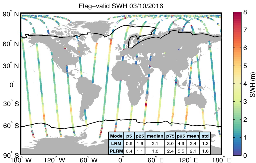
Figure 15. Geographical distribution of flag-valid SWH data over oceans and lakes for 03/10/2016. The statistical values shown in the table refer to the SWH in m and are calculated separately for LRM and PLRM regions. Measurements taken over polar polygons have been excluded from the computation of the statistical values. The black lines mark the outer limit of the Arctic and Antarctic polar polygons.
