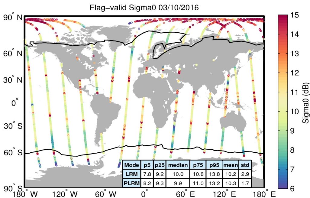
Figure 23. Geographical distribution of flag-valid sigma0 data over oceans and lakes for 03/10/2016. The statistical values shown in the table refer to the sigma0 in dB and are calculated separately for LRM and PLRM regions. Measurements taken over polar polygons have been excluded from the computation of the statistical values. The black lines mark the outer limit of the Arctic and Antarctic polar polygons.
