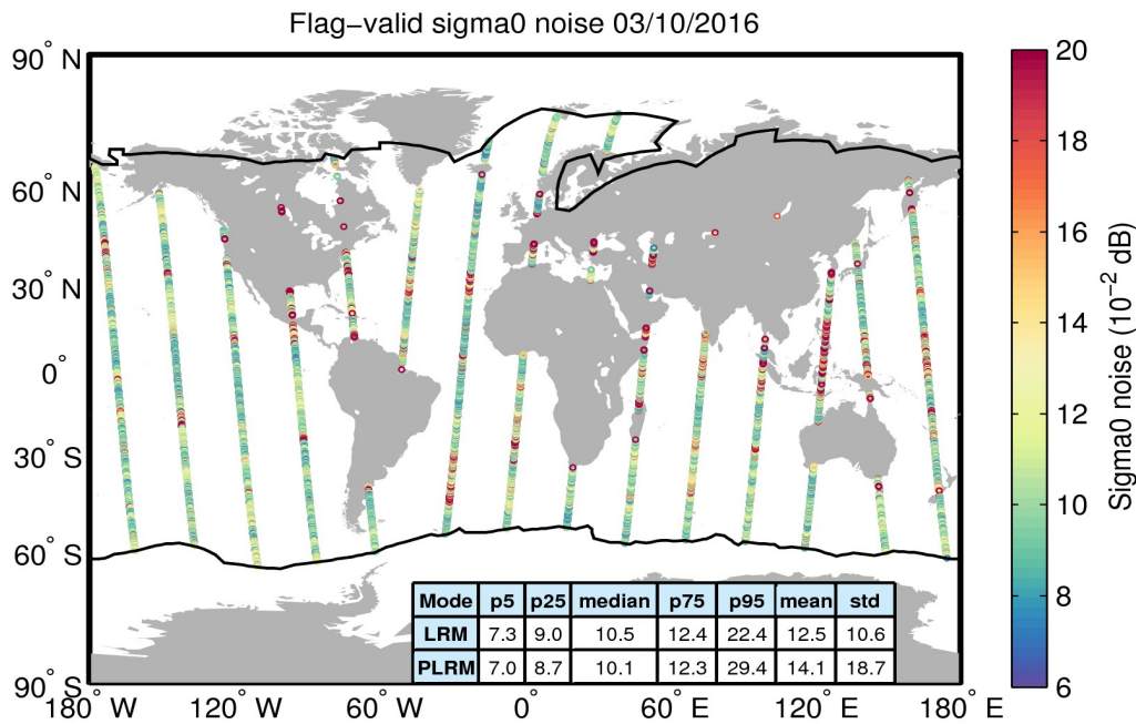
Figure 26. Geographical distribution of flag-valid 20-Hz sigma0 measurement noise over oceans and lakes for 03/10/2016. The statistical values shown in the table refer to the sigma0 noise and are calculated separately for LRM and PLRM regions. Measurements taken over polar polygons have been excluded from the computation of the statistical values. The black lines mark the outer limit of the Arctic and Antarctic polar polygons.
