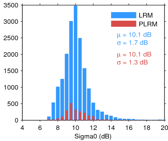
Figure 28. Histogram of science-valid sigma0 over oceans and lakes for LRM (blue) and PLRM (red) for 03/10/2016. The mean ( \mu ) and standard deviation ( \sigma ) are also shown. Note that values outside [4 20] dB are excluded from the histogram for the sake of readability but not from the computation of \mu and \sigma .
