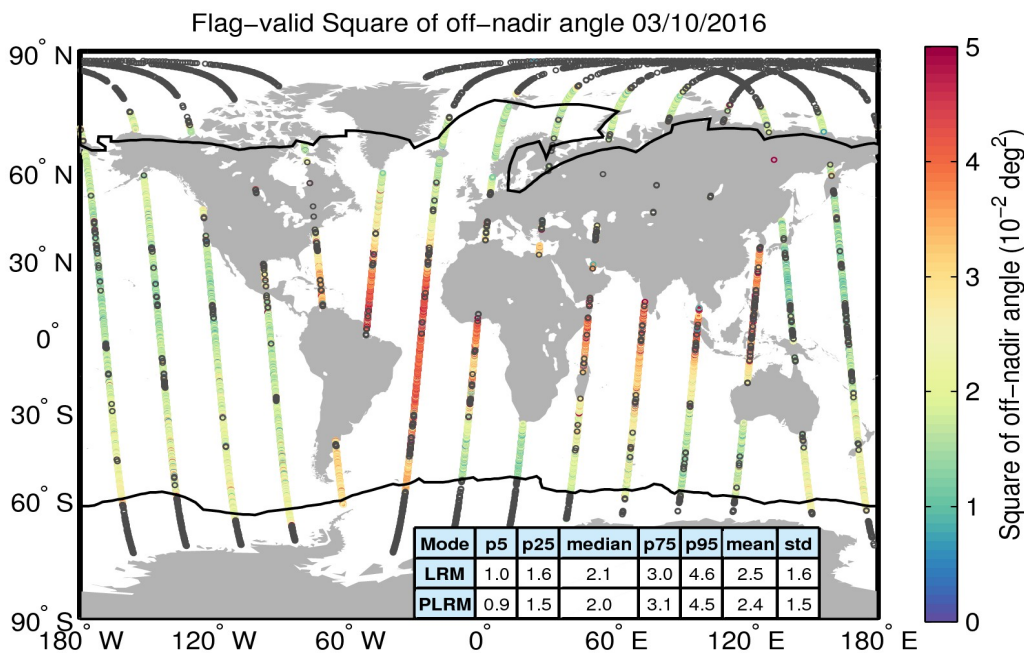
Figure 37. Geographical distribution of flag-valid mispointing data over oceans and lakes for 03/10/2016. The statistical values shown in the table refer to the mispointing in 10^{-2} deg 2 and are calculated separately for LRM and PLRM regions. Measurements taken over polar polygons have been excluded from the computation of the statistical values. The black lines mark the outer limit of the Arctic and Antarctic polar polygons. Gray circles denote negative values.
