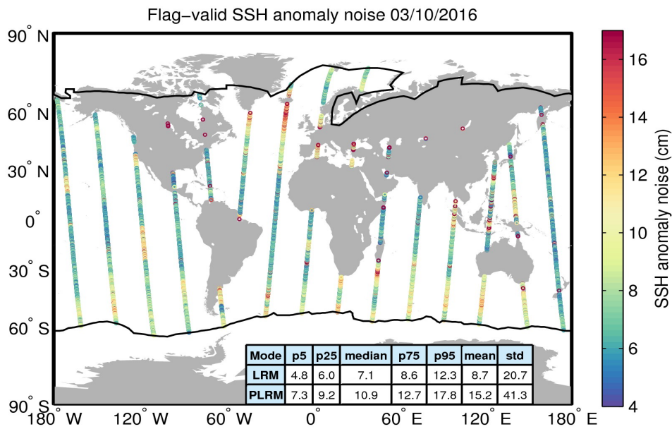
Figure 8. Geographical distribution of flag-valid 20-Hz SSH anomaly measurement noise over oceans and lakes for 03/10/2016. The statistical values shown in the table refer to the SSH anomaly noise and are calculated separately for LRM and PLRM regions. Measurements taken over polar polygons have been excluded from the computation of the statistical values. The black lines mark the outer limit of the Arctic and Antarctic polar polygons.
