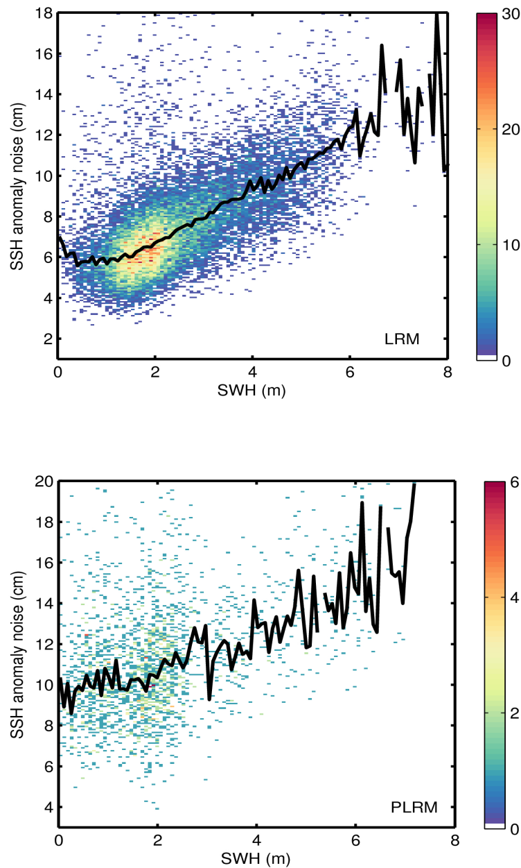
Figure 9. 2D histogram showing flag-valid SSH anomaly noise as a function of SWH for LRM (top) and PLRM (bottom) for 03/10/2016. The black line denotes the median SSH anomaly noise as a function of SWH.
