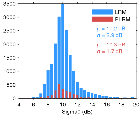
Figure 25. Histogram of flag-valid sigma0 over oceans and lakes for LRM (blue) and PLRM (red) for 03/10/2016. The mean ( \mu ) and standard deviation ( \sigma ) are also shown. Note that values outside [4 20] dB are excluded from the histogram for the sake of readability but not from the computation of \mu and \sigma .
