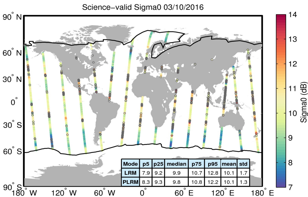
Figure 27. Geographical distribution of science-valid sigma0 data over oceans and lakes for 03/10/2016. The statistical values shown in the table refer to the sigma0 in dB and are calculated separately for LRM and PLRM regions. The black lines mark the outer limit of the Arctic and Antarctic polar polygons. Gray circles denote records that have been rejected based on the editing criteria described in Table 4.
