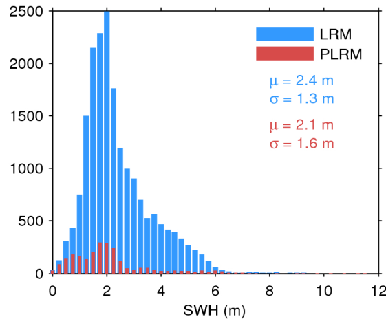
Figure 17. Histogram of flag-valid SWH over oceans and lakes for LRM (blue) and PLRM (red) for 03/10/2016. The mean ( \mu ) and standard deviation ( \sigma ) are also shown. Note that values larger than 12 m are excluded from the histogram for the sake of readability but not from the computation of \mu and \sigma .
