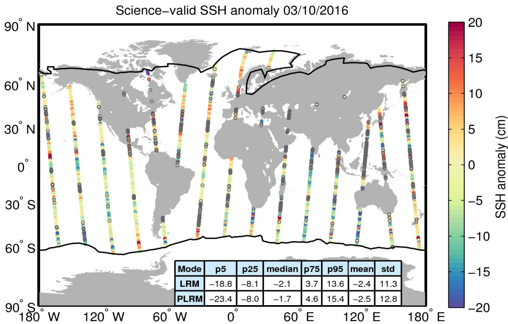
Figure 10. Geographical distribution of science-valid SSH anomaly data over oceans and lakes for 03/10/2016. The statistical values shown in the table refer to the SSH anomaly in cm and are calculated separately for LRM and PLRM regions. The black lines mark the outer limit of the Arctic and Antarctic polar polygons. Gray circles denote records that have been rejected based on the editing criteria described in Table 2.
