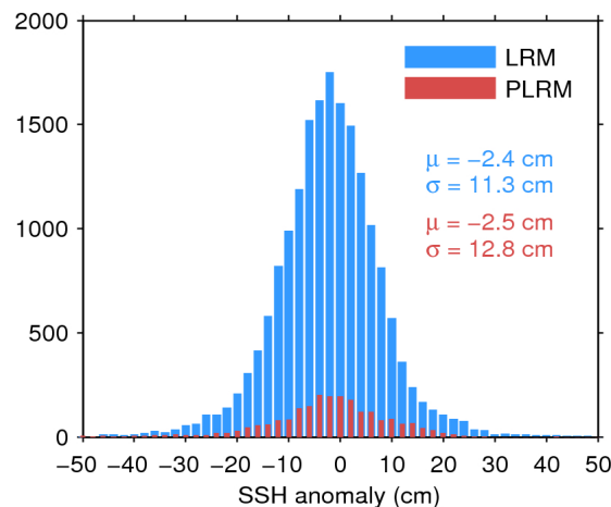
Figure 11. Histogram of science-valid SSH anomaly over oceans and lakes for LRM (blue) and PLRM (red) for 03/10/2016. The mean ( \mu ) and standard deviation ( \sigma ) are also shown. Note that values outside [-50 50] cm are excluded from the histogram for the sake of readability but not from the computation of \mu and \sigma .
