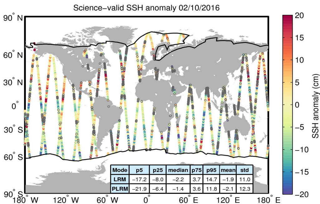
Figure 10. Geographical distribution of science-valid SSH anomaly data over oceans and lakes for 02/10/2016. The statistical values shown in the table refer to the SSH anomaly in cm and are calculated separately for LRM and PLRM regions. The black lines mark the outer limit of the Arctic and Antarctic polar polygons. Gray circles denote records that have been rejected based on the editing criteria described in Table 2.
