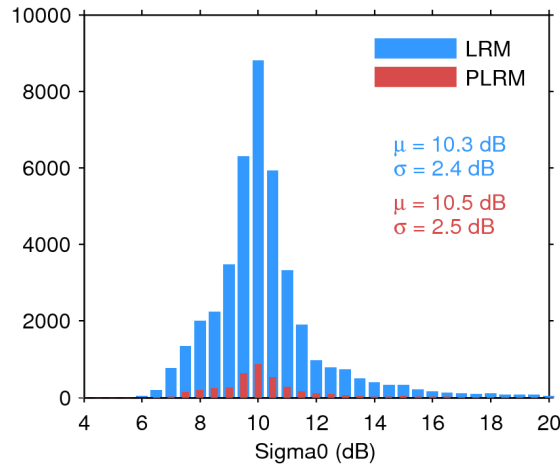
Figure 25. Histogram of flag-valid sigma0 over oceans and lakes for LRM (blue) and PLRM (red) for 02/10/2016. The mean ( \mu ) and standard deviation ( \sigma ) are also shown. Note that values outside [4 20] dB are excluded from the histogram for the sake of readability but not from the computation of \mu and \sigma .
