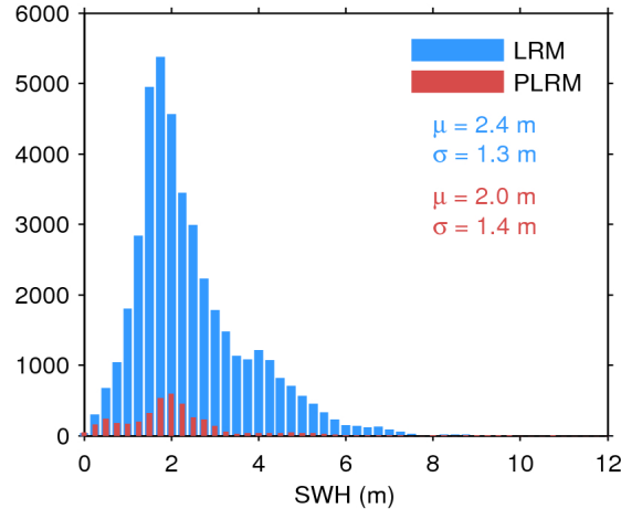
Figure 17. Histogram of flag-valid SWH over oceans and lakes for LRM (blue) and PLRM (red) for 02/10/2016. The mean ( \mu ) and standard deviation ( \sigma ) are also shown. Note that values larger than 12 m are excluded from the histogram for the sake of readability but not from the computation of \mu and \sigma .
