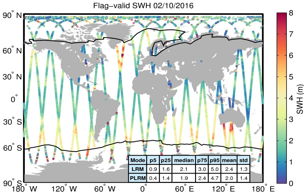
Figure 15. Geographical distribution of flag-valid SWH data over oceans and lakes for 02/10/2016. The statistical values shown in the table refer to the SWH in m and are calculated separately for LRM and PLRM regions. Measurements taken over polar polygons have been excluded from the computation of the statistical values. The black lines mark the outer limit of the Arctic and Antarctic polar polygons.
