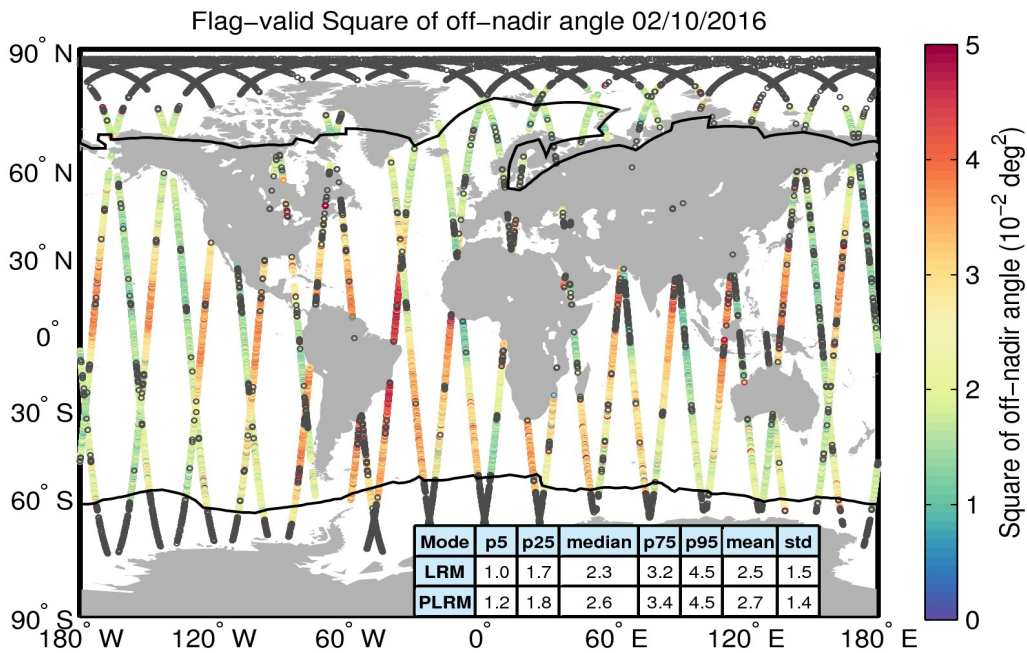
Figure 37. Geographical distribution of flag-valid mispointing data over oceans and lakes for 02/10/2016. The statistical values shown in the table refer to the mispointing in 10^{-2} deg 2 and are calculated separately for LRM and PLRM regions. Measurements taken over polar polygons have been excluded from the computation of the statistical values. The black lines mark the outer limit of the Arctic and Antarctic polar polygons. Gray circles denote negative values.
