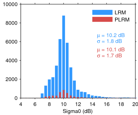
Figure 28. Histogram of science-valid sigma0 over oceans and lakes for LRM (blue) and PLRM (red) for 02/10/2016. The mean ( \mu ) and standard deviation ( \sigma ) are also shown. Note that values outside [4 20] dB are excluded from the histogram for the sake of readability but not from the computation of \mu and \sigma .
