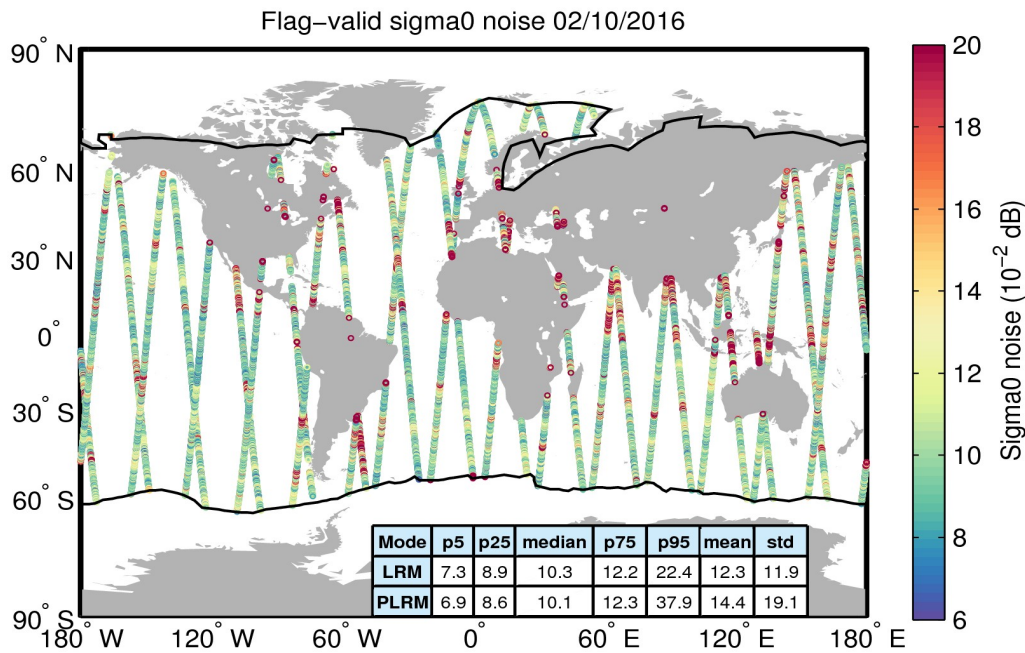
Figure 26. Geographical distribution of flag-valid 20-Hz sigma0 measurement noise over oceans and lakes for 02/10/2016. The statistical values shown in the table refer to the sigma0 noise and are calculated separately for LRM and PLRM regions. Measurements taken over polar polygons have been excluded from the computation of the statistical values. The black lines mark the outer limit of the Arctic and Antarctic polar polygons.
