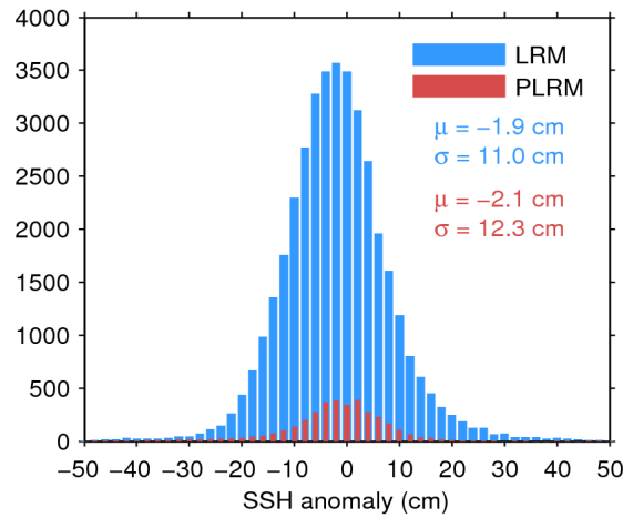
Figure 11. Histogram of science-valid SSH anomaly over oceans and lakes for LRM (blue) and PLRM (red) for 02/10/2016. The mean ( \mu ) and standard deviation ( \sigma ) are also shown. Note that values outside [-50\ 50] cm are excluded from the histogram for the sake of readability but not from the computation of \mu and \sigma .
