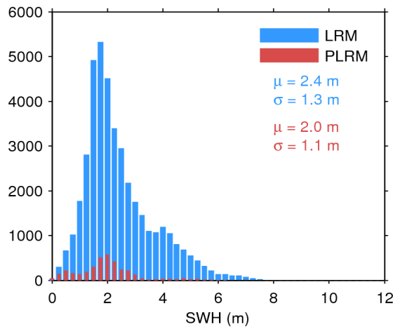
Figure 20. Histogram of science-valid SWH over oceans and lakes for LRM (blue) and PLRM (red) for 02/10/2016. The mean ( \mu ) and standard deviation ( \sigma ) are also shown. Note that values larger than 12 m are excluded from the histogram for the sake of readability but not from the computation of \mu and \sigma .
