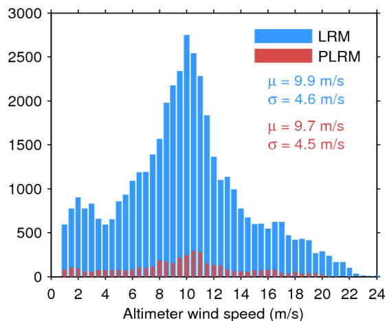
Figure 35. Histogram of science-valid wind over oceans and lakes for LRM (blue) and PLRM (red) for 02/10/2016. The mean ( \mu ) and standard deviation ( \sigma ) are also shown. Note that values larger than 24 m/s are excluded from the histogram for the sake of readability but not from the computation of \mu and \sigma .
