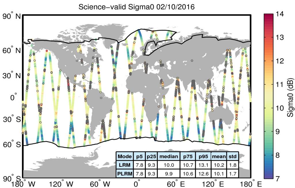
Figure 27. Geographical distribution of science-valid sigma0 data over oceans and lakes for 02/10/2016. The statistical values shown in the table refer to the sigma0 in dB and are calculated separately for LRM and PLRM regions. The black lines mark the outer limit of the Arctic and Antarctic polar polygons. Gray circles denote records that have been rejected based on the editing criteria described in Table 4.
