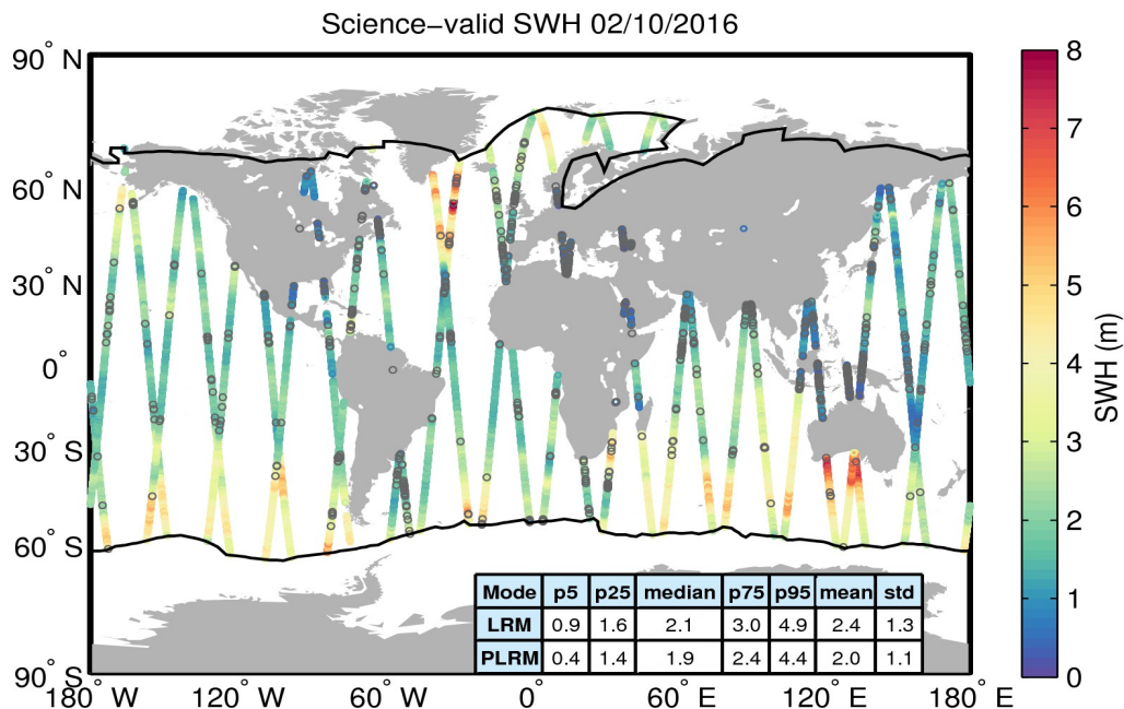
Figure 19. Geographical distribution of science-valid SWH data over oceans and lakes for 02/10/2016. The statistical values shown in the table refer to the SWH in m and are calculated separately for LRM and PLRM regions. The black lines mark the outer limit of the Arctic and Antarctic polar polygons. Gray circles denote records that have been rejected based on the editing criteria described in Table 3.
