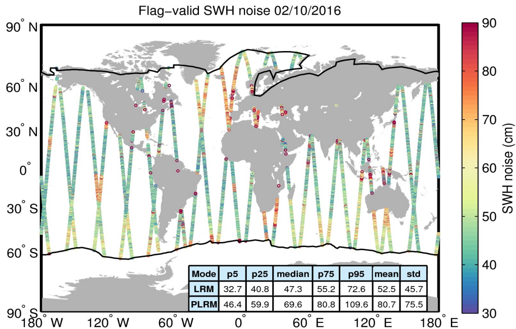
Figure 18. Geographical distribution of flag-valid 20-Hz SWH measurement noise over oceans and lakes for 02/10/2016. The statistical values shown in the table refer to the SWH noise and are calculated separately for LRM and PLRM regions. Measurements taken over polar polygons have been excluded from the computation of the statistical values. The black lines mark the outer limit of the Arctic and Antarctic polar polygons.
