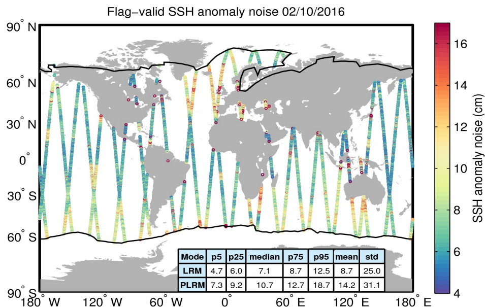
Figure 8. Geographical distribution of flag-valid 20-Hz SSH anomaly measurement noise over oceans and lakes for 02/10/2016. The statistical values shown in the table refer to the SSH anomaly noise and are calculated separately for LRM and PLRM regions. Measurements taken over polar polygons have been excluded from the computation of the statistical values. The black lines mark the outer limit of the Arctic and Antarctic polar polygons.
