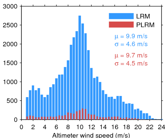
Figure 33. Histogram of flag-valid wind over oceans and lakes for LRM (blue) and PLRM (red) for 02/10/2016. The mean ( \mu ) and standard deviation ( \sigma ) are also shown. Note that values larger than 24 m/s are excluded from the histogram for the sake of readability but not from the computation of \mu and \sigma .
