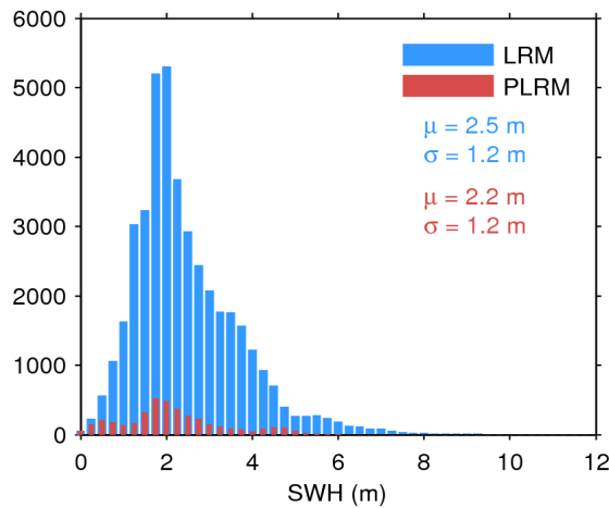
Figure 20. Histogram of science-valid SWH over oceans and lakes for LRM (blue) and PLRM (red) for 30/09/2016. The mean ( \mu ) and standard deviation ( \sigma ) are also shown. Note that values larger than 12 m are excluded from the histogram for the sake of readability but not from the computation of \mu and \sigma .
