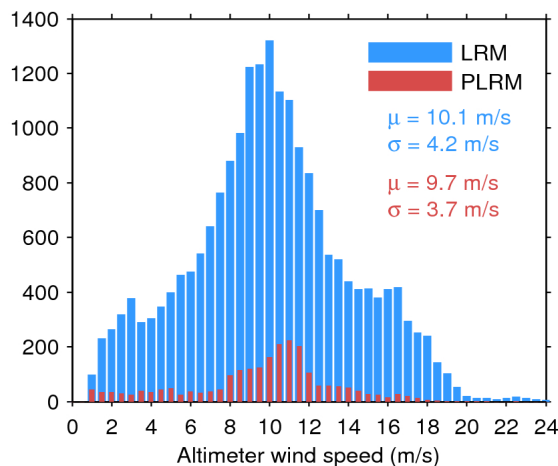
Figure 35. Histogram of science-valid wind over oceans and lakes for LRM (blue) and PLRM (red) for 30/09/2016. The mean ( \mu ) and standard deviation ( \sigma ) are also shown. Note that values larger than 24 m/s are excluded from the histogram for the sake of readability but not from the computation of \mu and \sigma .
