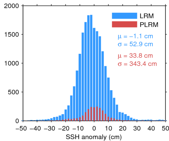
Figure 7. Histogram of flag-valid SSH anomaly over oceans and lakes for LRM (blue) and PLRM (red) for 30/09/2016. The mean ( \mu ) and standard deviation ( \sigma ) are also shown. Note that values outside [-50 50] cm are excluded from the histogram for the sake of readability but not from the computation of \mu and \sigma .
