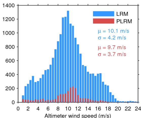
Figure 33. Histogram of flag-valid wind over oceans and lakes for LRM (blue) and PLRM (red) for 30/09/2016. The mean ( \mu ) and standard deviation ( \sigma ) are also shown. Note that values larger than 24 m/s are excluded from the histogram for the sake of readability but not from the computation of \mu and \sigma .
