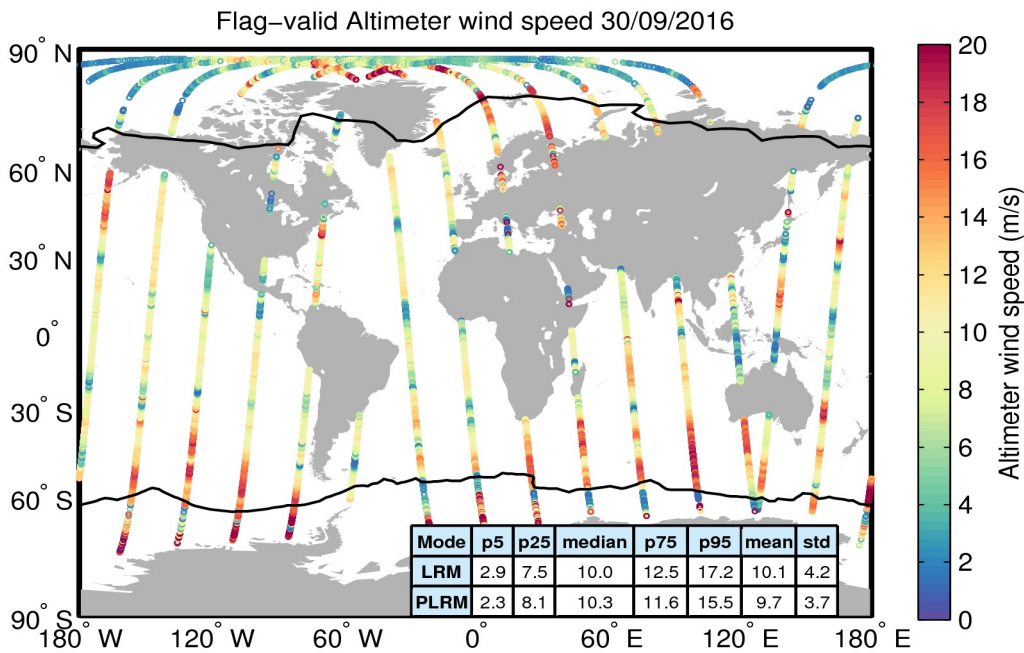
Figure 31. Geographical distribution of flag-valid wind data over oceans and lakes for 30/09/2016. The statistical values shown in the table refer to the wind in m/s and are calculated separately for LRM and PLRM regions. Measurements taken over polar polygons have been excluded from the computation of the statistical values. The black lines mark the outer limit of the Arctic and Antarctic polar polygons.
