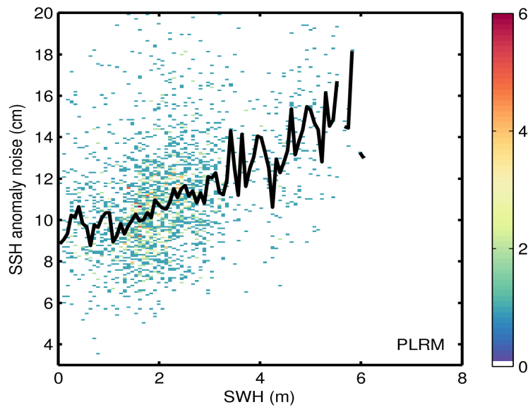
Figure 9. 2D histogram showing flag-valid SSH anomaly noise as a function of SWH for LRM (top) and PLRM (bottom) for 30/09/2016. The black line denotes the median SSH anomaly noise as a function of SWH.
