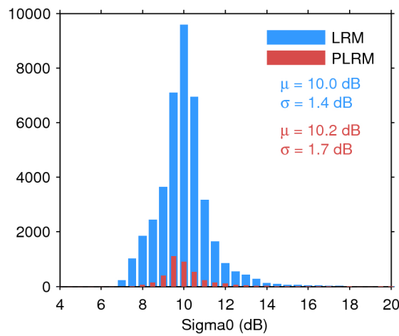
Figure 28. Histogram of science-valid sigma0 over oceans and lakes for LRM (blue) and PLRM (red) for 30/09/2016. The mean ( \mu ) and standard deviation ( \sigma ) are also shown. Note that values outside [4 20] dB are excluded from the histogram for the sake of readability but not from the computation of \mu and \sigma .
