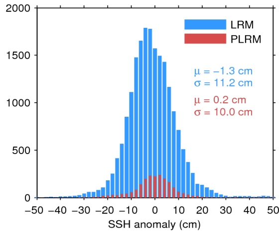
Figure 11. Histogram of science-valid SSH anomaly over oceans and lakes for LRM (blue) and PLRM (red) for 30/09/2016. The mean ( \mu ) and standard deviation ( \sigma ) are also shown. Note that values outside [-50\ 50] cm are excluded from the histogram for the sake of readability but not from the computation of \mu and \sigma .
