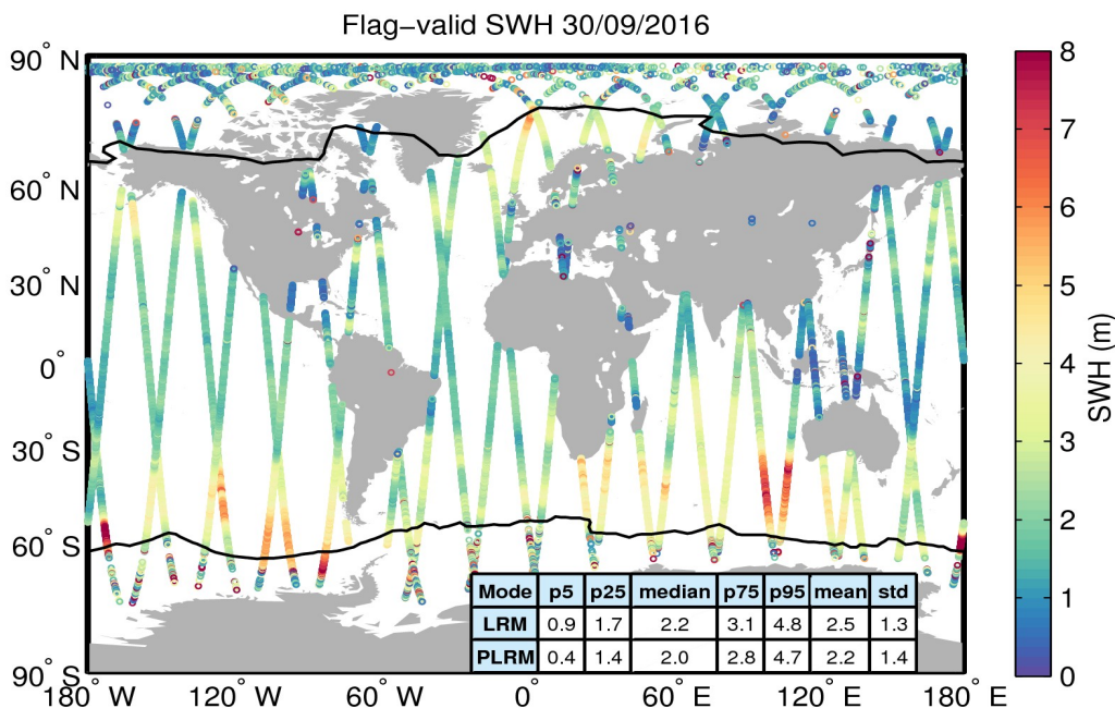
Figure 15. Geographical distribution of flag-valid SWH data over oceans and lakes for 30/09/2016. The statistical values shown in the table refer to the SWH in m and are calculated separately for LRM and PLRM regions. Measurements taken over polar polygons have been excluded from the computation of the statistical values. The black lines mark the outer limit of the Arctic and Antarctic polar polygons.
