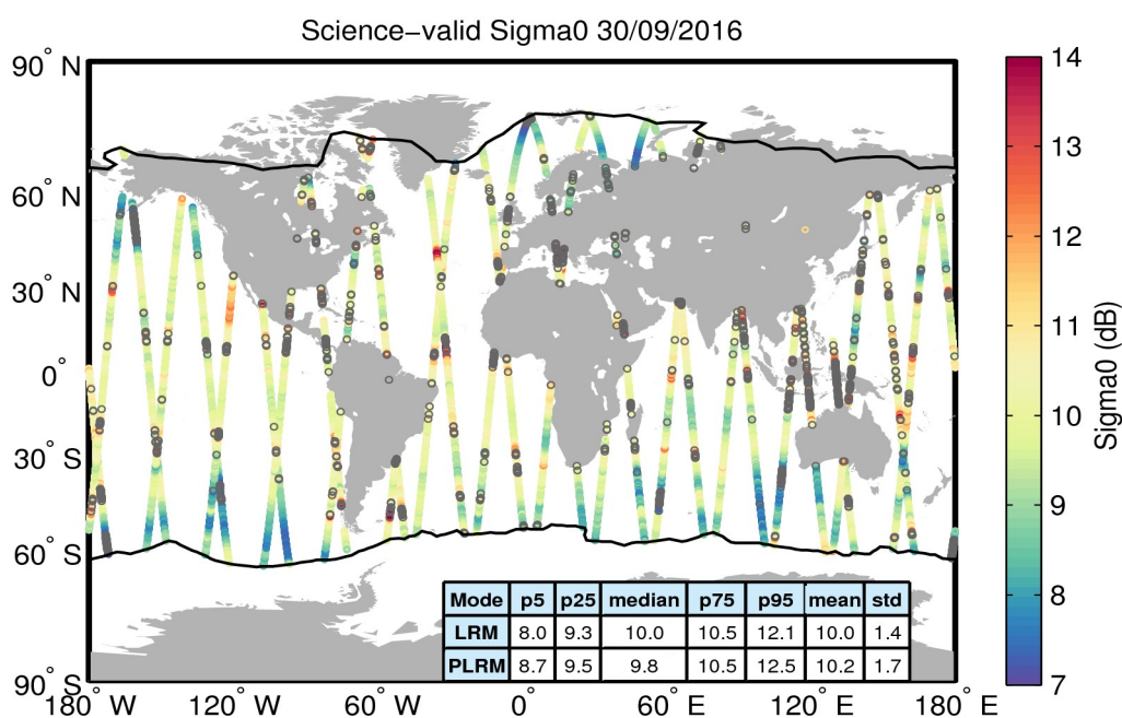
Figure 27. Geographical distribution of science-valid sigma0 data over oceans and lakes for 30/09/2016. The statistical values shown in the table refer to the sigma0 in dB and are calculated separately for LRM and PLRM regions. The black lines mark the outer limit of the Arctic and Antarctic polar polygons. Gray circles denote records that have been rejected based on the editing criteria described in Table 4.
