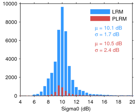
Figure 25. Histogram of flag-valid sigma0 over oceans and lakes for LRM (blue) and PLRM (red) for 30/09/2016. The mean ( \mu ) and standard deviation ( \sigma ) are also shown. Note that values outside [4 20] dB are excluded from the histogram for the sake of readability but not from the computation of \mu and \sigma .
