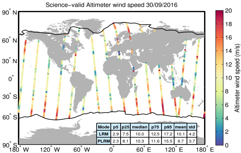
Figure 34. Geographical distribution of science-valid wind data over oceans and lakes for 30/09/2016. The statistical values shown in the table refer to the wind in m/s and are calculated separately for LRM and PLRM regions. The black lines mark the outer limit of the Arctic and Antarctic polar polygons. Gray circles denote records that have been rejected based on the editing criteria described in Table 5.
