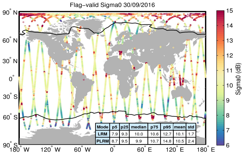
Figure 23. Geographical distribution of flag-valid sigma0 data over oceans and lakes for 30/09/2016. The statistical values shown in the table refer to the sigma0 in dB and are calculated separately for LRM and PLRM regions. Measurements taken over polar polygons have been excluded from the computation of the statistical values. The black lines mark the outer limit of the Arctic and Antarctic polar polygons.
