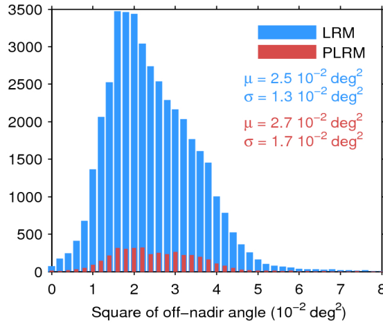
Figure 39. Histogram of flag-valid mispointing over oceans and lakes for LRM (blue) and PLRM (red) for 30/09/2016. Only positive values have been considered. The mean ( \mu ) and standard deviation ( \sigma ) are also shown. Note that values larger than 8 \cdot 10^{-2} \text{ deg}^2 are excluded from the histogram for the sake of readability but not from the computation of \mu and \sigma .
