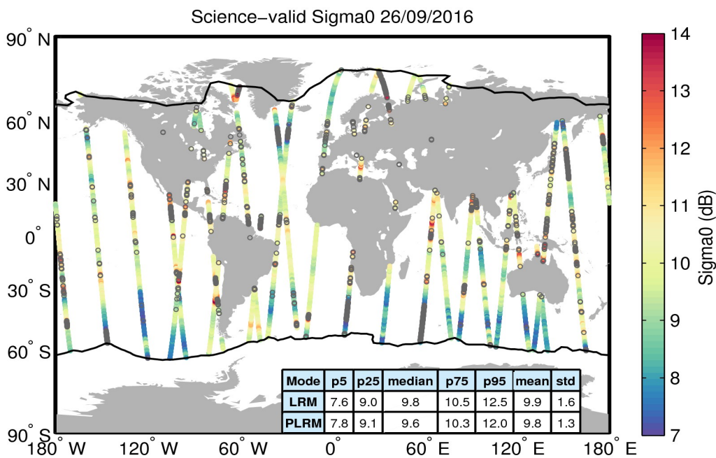
Figure 27. Geographical distribution of science-valid sigma0 data over oceans and lakes for 26/09/2016. The statistical values shown in the table refer to the sigma0 in dB and are calculated separately for LRM and PLRM regions. The black lines mark the outer limit of the Arctic and Antarctic polar polygons. Gray circles denote records that have been rejected based on the editing criteria described in Table 4.
