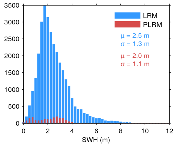
Figure 20. Histogram of science-valid SWH over oceans and lakes for LRM (blue) and PLRM (red) for 26/09/2016. The mean ( \mu ) and standard deviation ( \sigma ) are also shown. Note that values larger than 12 m are excluded from the histogram for the sake of readability but not from the computation of \mu and \sigma .
