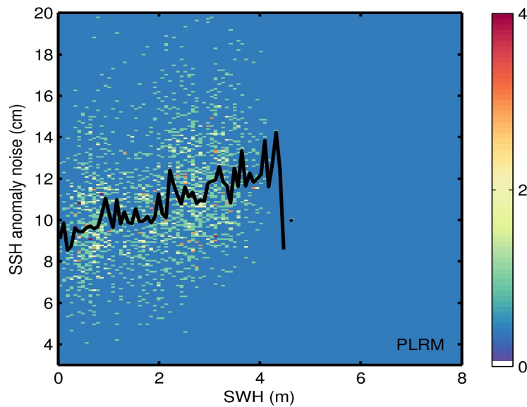
Figure 9. 2D histogram showing flag-valid SSH anomaly noise as a function of SWH for LRM (top) and PLRM (bottom) for 26/09/2016. The black line denotes the median SSH anomaly noise as a function of SWH.
