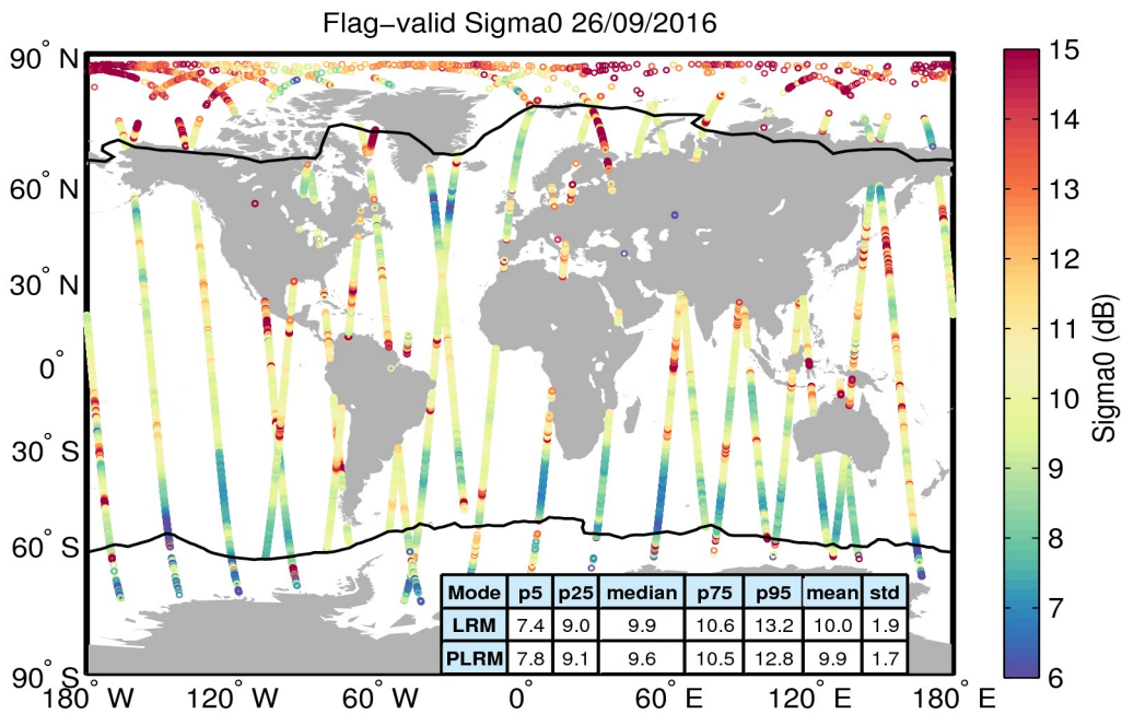
Figure 23. Geographical distribution of flag-valid sigma0 data over oceans and lakes for 26/09/2016. The statistical values shown in the table refer to the sigma0 in dB and are calculated separately for LRM and PLRM regions. Measurements taken over polar polygons have been excluded from the computation of the statistical values. The black lines mark the outer limit of the Arctic and Antarctic polar polygons.
