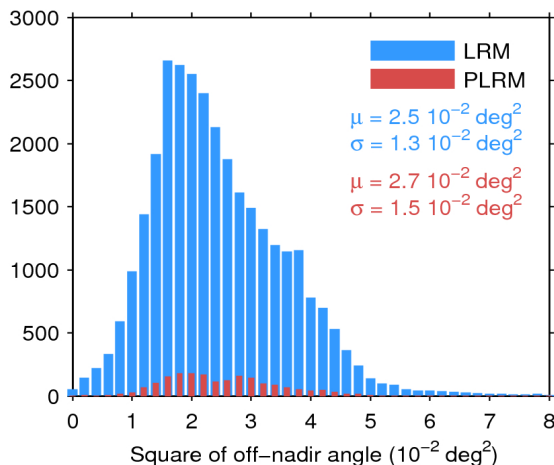
Figure 39. Histogram of flag-valid mispointing over oceans and lakes for LRM (blue) and PLRM (red) for 26/09/2016. Only positive values have been considered. The mean ( \mu ) and standard deviation ( \sigma ) are also shown. Note that values larger than 8 \cdot 10^{-2} \text{ deg}^2 are excluded from the histogram for the sake of readability but not from the computation of \mu and \sigma .
