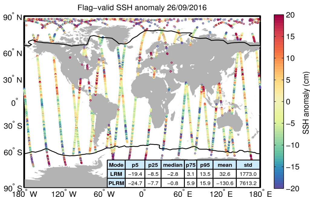
Figure 5. Geographical distribution of flag-valid 1-Hz SSH anomaly data over oceans and lakes for 26/09/2016. The statistical values shown in the table refer to the SSH anomaly in cm and are calculated separately for LRM and PLRM regions. Measurements taken over polar polygons have been excluded from the computation of the statistical values. The black lines mark the outer limit of the Arctic and Antarctic polar polygons.
