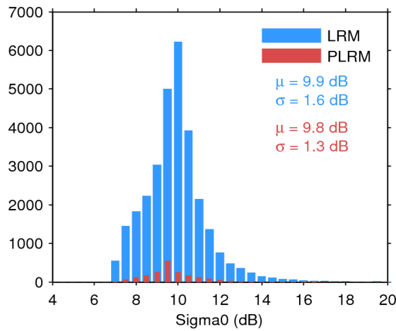
Figure 28. Histogram of science-valid sigma0 over oceans and lakes for LRM (blue) and PLRM (red) for 26/09/2016. The mean ( \mu ) and standard deviation ( \sigma ) are also shown. Note that values outside [4 20] dB are excluded from the histogram for the sake of readability but not from the computation of \mu and \sigma .
