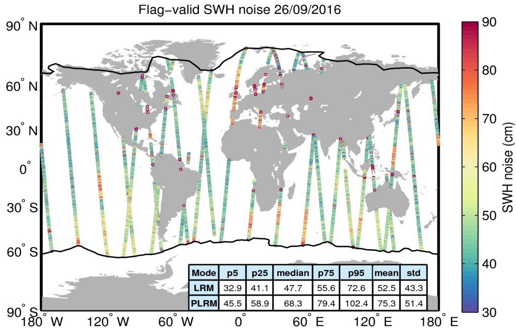
Figure 18. Geographical distribution of flag-valid 20-Hz SWH measurement noise over oceans and lakes for 26/09/2016. The statistical values shown in the table refer to the SWH noise and are calculated separately for LRM and PLRM regions. Measurements taken over polar polygons have been excluded from the computation of the statistical values. The black lines mark the outer limit of the Arctic and Antarctic polar polygons.
