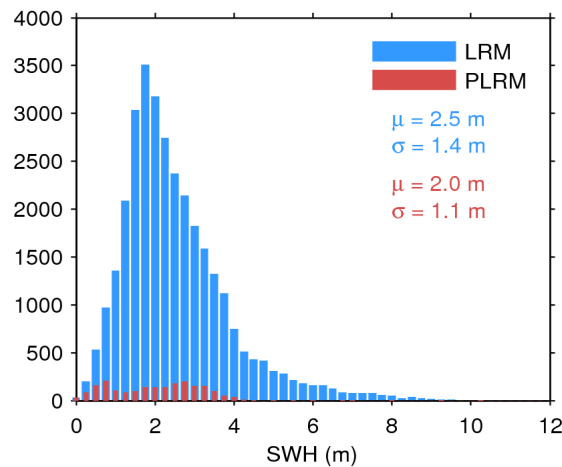
Figure 17. Histogram of flag-valid SWH over oceans and lakes for LRM (blue) and PLRM (red) for 26/09/2016. The mean ( \mu ) and standard deviation ( \sigma ) are also shown. Note that values larger than 12 m are excluded from the histogram for the sake of readability but not from the computation of \mu and \sigma .
