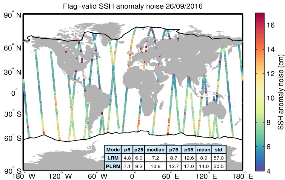
Figure 8. Geographical distribution of flag-valid 20-Hz SSH anomaly measurement noise over oceans and lakes for 26/09/2016. The statistical values shown in the table refer to the SSH anomaly noise and are calculated separately for LRM and PLRM regions. Measurements taken over polar polygons have been excluded from the computation of the statistical values. The black lines mark the outer limit of the Arctic and Antarctic polar polygons.
