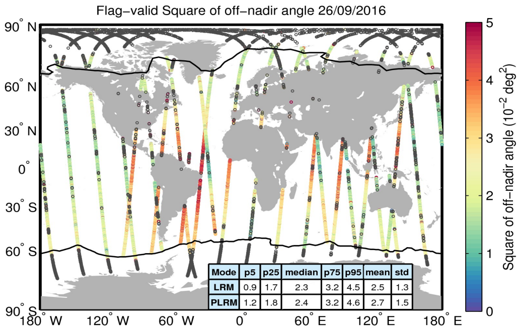
Figure 37. Geographical distribution of flag-valid mispointing data over oceans and lakes for 26/09/2016. The statistical values shown in the table refer to the mispointing in 10^{-2} deg 2 and are calculated separately for LRM and PLRM regions. Measurements taken over polar polygons have been excluded from the computation of the statistical values. The black lines mark the outer limit of the Arctic and Antarctic polar polygons. Gray circles denote negative values.
