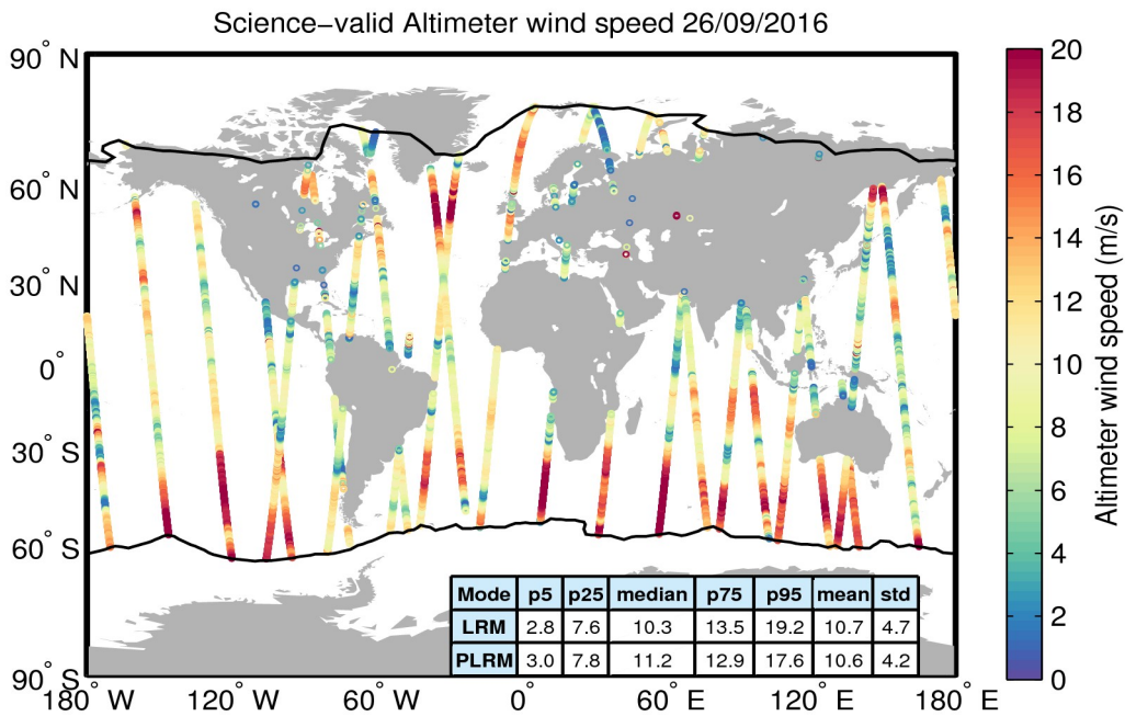
Figure 34. Geographical distribution of science-valid wind data over oceans and lakes for 26/09/2016. The statistical values shown in the table refer to the wind in m/s and are calculated separately for LRM and PLRM regions. The black lines mark the outer limit of the Arctic and Antarctic polar polygons. Gray circles denote records that have been rejected based on the editing criteria described in Table 5.
