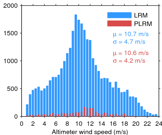
Figure 35. Histogram of science-valid wind over oceans and lakes for LRM (blue) and PLRM (red) for 26/09/2016. The mean ( \mu ) and standard deviation ( \sigma ) are also shown. Note that values larger than 24 m/s are excluded from the histogram for the sake of readability but not from the computation of \mu and \sigma .
