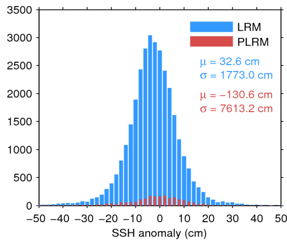
Figure 7. Histogram of flag-valid SSH anomaly over oceans and lakes for LRM (blue) and PLRM (red) for 26/09/2016. The mean ( \mu ) and standard deviation ( \sigma ) are also shown. Note that values outside [-50\ 50] cm are excluded from the histogram for the sake of readability but not from the computation of \mu and \sigma .
