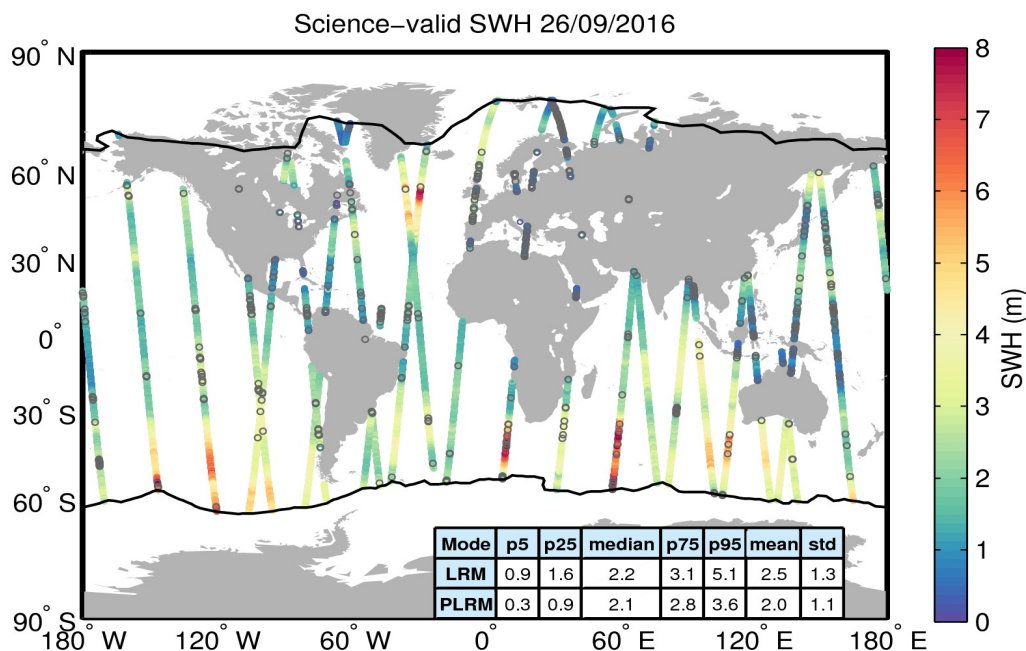
Figure 19. Geographical distribution of science-valid SWH data over oceans and lakes for 26/09/2016. The statistical values shown in the table refer to the SWH in m and are calculated separately for LRM and PLRM regions. The black lines mark the outer limit of the Arctic and Antarctic polar polygons. Gray circles denote records that have been rejected based on the editing criteria described in Table 3.
