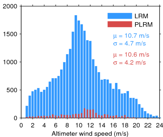
Figure 33. Histogram of flag-valid wind over oceans and lakes for LRM (blue) and PLRM (red) for 26/09/2016. The mean ( \mu ) and standard deviation ( \sigma ) are also shown. Note that values larger than 24 m/s are excluded from the histogram for the sake of readability but not from the computation of \mu and \sigma .
