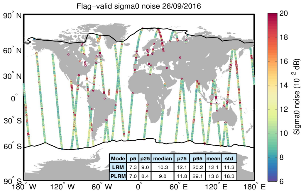
Figure 26. Geographical distribution of flag-valid 20-Hz sigma0 measurement noise over oceans and lakes for 26/09/2016. The statistical values shown in the table refer to the sigma0 noise and are calculated separately for LRM and PLRM regions. Measurements taken over polar polygons have been excluded from the computation of the statistical values. The black lines mark the outer limit of the Arctic and Antarctic polar polygons.
