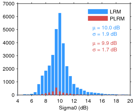
Figure 25. Histogram of flag-valid sigma0 over oceans and lakes for LRM (blue) and PLRM (red) for 26/09/2016. The mean ( \mu ) and standard deviation ( \sigma ) are also shown. Note that values outside [4 20] dB are excluded from the histogram for the sake of readability but not from the computation of \mu and \sigma .
