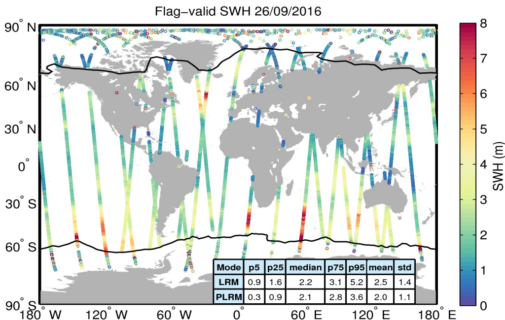
Figure 15. Geographical distribution of flag-valid SWH data over oceans and lakes for 26/09/2016. The statistical values shown in the table refer to the SWH in m and are calculated separately for LRM and PLRM regions. Measurements taken over polar polygons have been excluded from the computation of the statistical values. The black lines mark the outer limit of the Arctic and Antarctic polar polygons.
