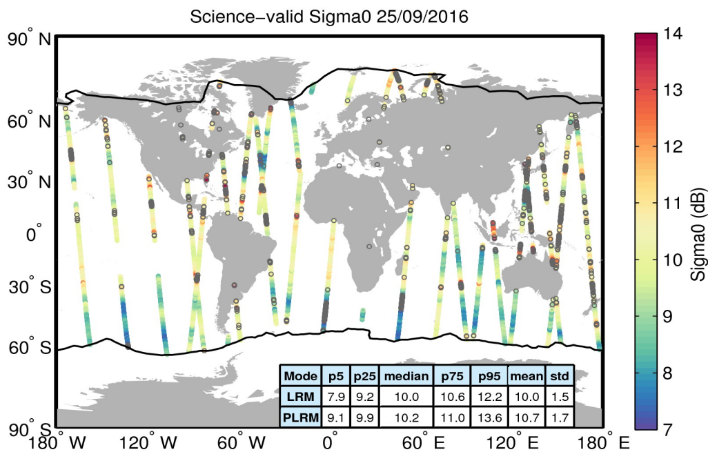
Figure 27. Geographical distribution of science-valid sigma0 data over oceans and lakes for 25/09/2016. The statistical values shown in the table refer to the sigma0 in dB and are calculated separately for LRM and PLRM regions. The black lines mark the outer limit of the Arctic and Antarctic polar polygons. Gray circles denote records that have been rejected based on the editing criteria described in Table 4.
