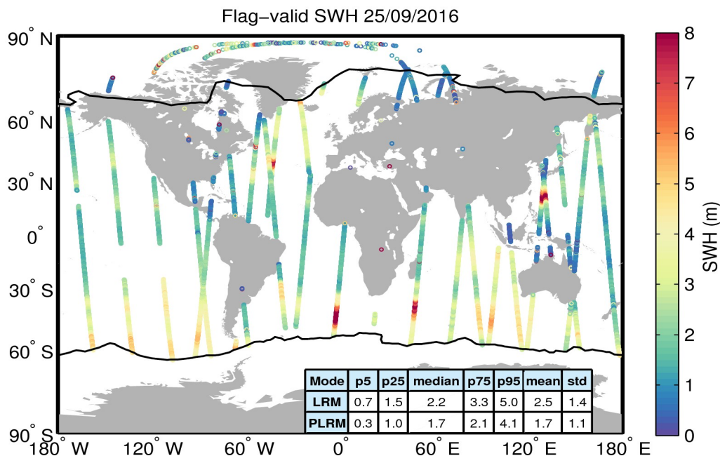
Figure 15. Geographical distribution of flag-valid SWH data over oceans and lakes for 25/09/2016. The statistical values shown in the table refer to the SWH in m and are calculated separately for LRM and PLRM regions. Measurements taken over polar polygons have been excluded from the computation of the statistical values. The black lines mark the outer limit of the Arctic and Antarctic polar polygons.
