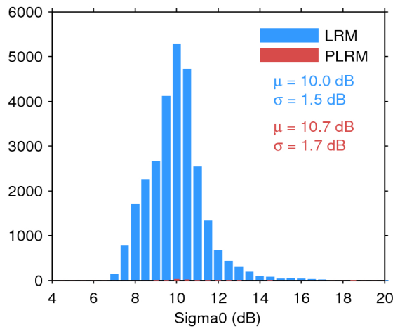
Figure 28. Histogram of science-valid sigma0 over oceans and lakes for LRM (blue) and PLRM (red) for 25/09/2016. The mean ( \mu ) and standard deviation ( \sigma ) are also shown. Note that values outside [4 20] dB are excluded from the histogram for the sake of readability but not from the computation of \mu and \sigma .
