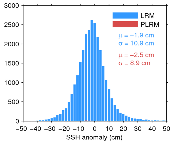
Figure 11. Histogram of science-valid SSH anomaly over oceans and lakes for LRM (blue) and PLRM (red) for 25/09/2016. The mean ( \mu ) and standard deviation ( \sigma ) are also shown. Note that values outside [-50\ 50] cm are excluded from the histogram for the sake of readability but not from the computation of \mu and \sigma .
