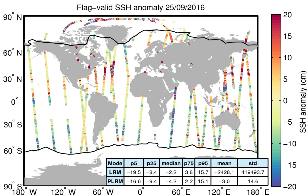
Figure 5. Geographical distribution of flag-valid 1-Hz SSH anomaly data over oceans and lakes for 25/09/2016. The statistical values shown in the table refer to the SSH anomaly in cm and are calculated separately for LRM and PLRM regions. Measurements taken over polar polygons have been excluded from the computation of the statistical values. The black lines mark the outer limit of the Arctic and Antarctic polar polygons.
