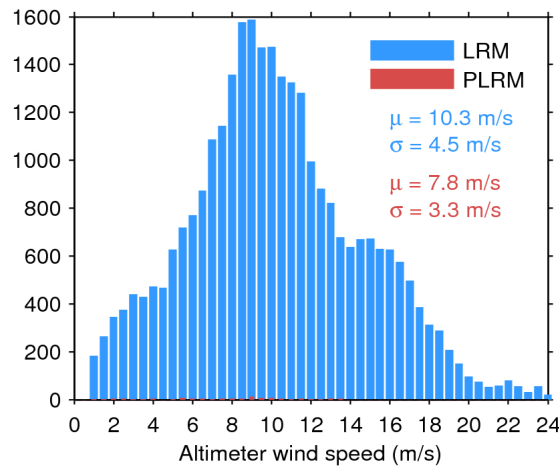
Figure 33. Histogram of flag-valid wind over oceans and lakes for LRM (blue) and PLRM (red) for 25/09/2016. The mean ( \mu ) and standard deviation ( \sigma ) are also shown. Note that values larger than 24 m/s are excluded from the histogram for the sake of readability but not from the computation of \mu and \sigma .
