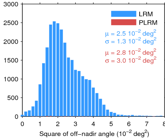
Figure 39. Histogram of flag-valid mispointing over oceans and lakes for LRM (blue) and PLRM (red) for 25/09/2016. Only positive values have been considered. The mean ( \mu ) and standard deviation ( \sigma ) are also shown. Note that values larger than 8 \cdot 10^{-2} \text{ deg}^2 are excluded from the histogram for the sake of readability but not from the computation of \mu and \sigma .
