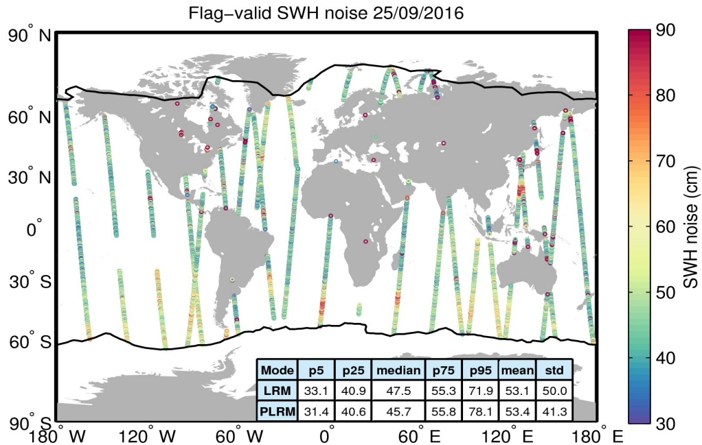
Figure 18. Geographical distribution of flag-valid 20-Hz SWH measurement noise over oceans and lakes for 25/09/2016. The statistical values shown in the table refer to the SWH noise and are calculated separately for LRM and PLRM regions. Measurements taken over polar polygons have been excluded from the computation of the statistical values. The black lines mark the outer limit of the Arctic and Antarctic polar polygons.
