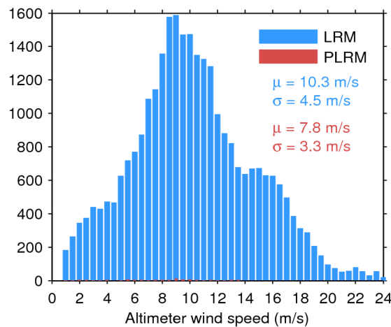
Figure 35. Histogram of science-valid wind over oceans and lakes for LRM (blue) and PLRM (red) for 25/09/2016. The mean ( \mu ) and standard deviation ( \sigma ) are also shown. Note that values larger than 24 m/s are excluded from the histogram for the sake of readability but not from the computation of \mu and \sigma .
