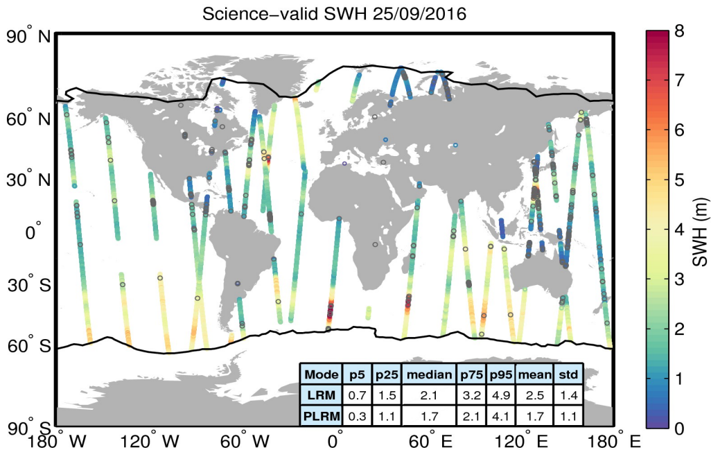
Figure 19. Geographical distribution of science-valid SWH data over oceans and lakes for 25/09/2016. The statistical values shown in the table refer to the SWH in m and are calculated separately for LRM and PLRM regions. The black lines mark the outer limit of the Arctic and Antarctic polar polygons. Gray circles denote records that have been rejected based on the editing criteria described in Table 3.
