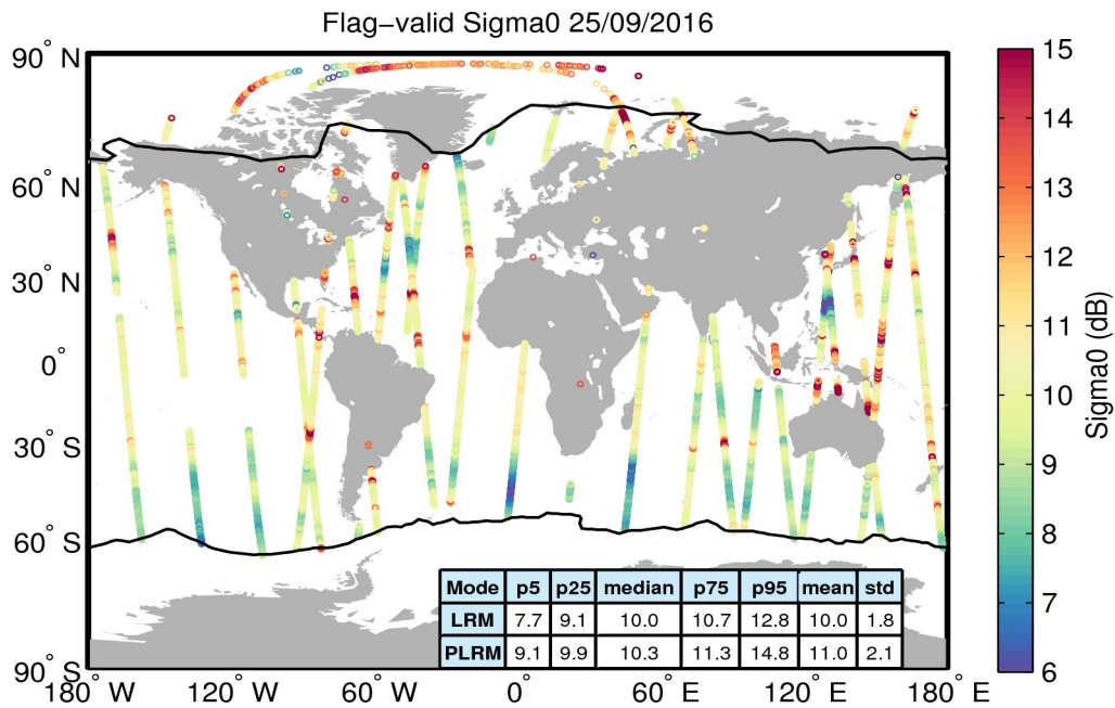
Figure 23. Geographical distribution of flag-valid sigma0 data over oceans and lakes for 25/09/2016. The statistical values shown in the table refer to the sigma0 in dB and are calculated separately for LRM and PLRM regions. Measurements taken over polar polygons have been excluded from the computation of the statistical values. The black lines mark the outer limit of the Arctic and Antarctic polar polygons.
