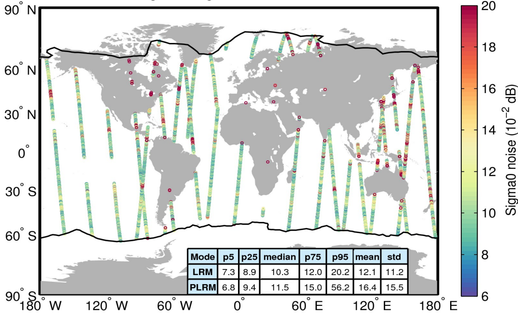
Flag-valid sigma0 noise 25/09/2016
