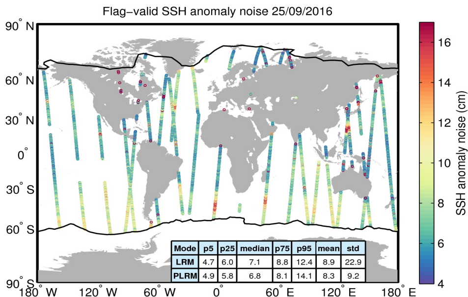
Figure 8. Geographical distribution of flag-valid 20-Hz SSH anomaly measurement noise over oceans and lakes for 25/09/2016. The statistical values shown in the table refer to the SSH anomaly noise and are calculated separately for LRM and PLRM regions. Measurements taken over polar polygons have been excluded from the computation of the statistical values. The black lines mark the outer limit of the Arctic and Antarctic polar polygons.
