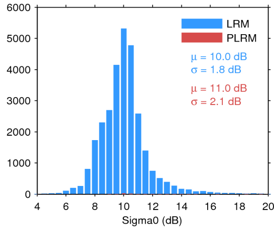
Figure 25. Histogram of flag-valid sigma0 over oceans and lakes for LRM (blue) and PLRM (red) for 25/09/2016. The mean ( \mu ) and standard deviation ( \sigma ) are also shown. Note that values outside [4 20] dB are excluded from the histogram for the sake of readability but not from the computation of \mu and \sigma .
