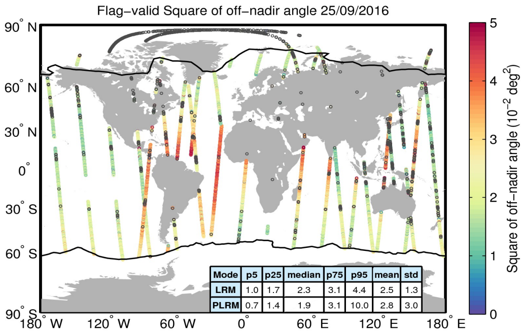
Figure 37. Geographical distribution of flag-valid mispointing data over oceans and lakes for 25/09/2016. The statistical values shown in the table refer to the mispointing in 10^{-2} deg 2 and are calculated separately for LRM and PLRM regions. Measurements taken over polar polygons have been excluded from the computation of the statistical values. The black lines mark the outer limit of the Arctic and Antarctic polar polygons. Gray circles denote negative values.
