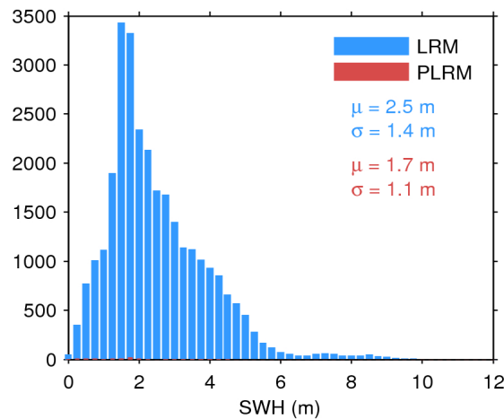
Figure 17. Histogram of flag-valid SWH over oceans and lakes for LRM (blue) and PLRM (red) for 25/09/2016. The mean ( \mu ) and standard deviation ( \sigma ) are also shown. Note that values larger than 12 m are excluded from the histogram for the sake of readability but not from the computation of \mu and \sigma .
