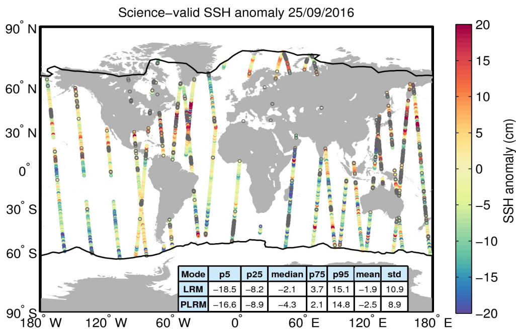
Figure 10. Geographical distribution of science-valid SSH anomaly data over oceans and lakes for 25/09/2016. The statistical values shown in the table refer to the SSH anomaly in cm and are calculated separately for LRM and PLRM regions. The black lines mark the outer limit of the Arctic and Antarctic polar polygons. Gray circles denote records that have been rejected based on the editing criteria described in Table 2.
