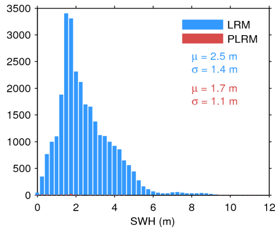
Figure 20. Histogram of science-valid SWH over oceans and lakes for LRM (blue) and PLRM (red) for 25/09/2016. The mean ( \mu ) and standard deviation ( \sigma ) are also shown. Note that values larger than 12 m are excluded from the histogram for the sake of readability but not from the computation of \mu and \sigma .
