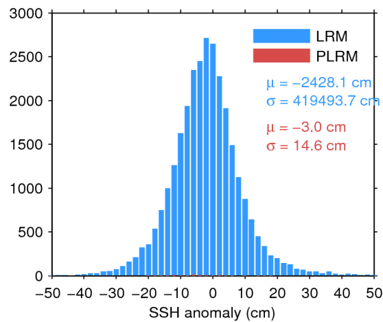
Figure 7. Histogram of flag-valid SSH anomaly over oceans and lakes for LRM (blue) and PLRM (red) for 25/09/2016. The mean ( \mu ) and standard deviation ( \sigma ) are also shown. Note that values outside [-50\ 50] cm are excluded from the histogram for the sake of readability but not from the computation of \mu and \sigma .
