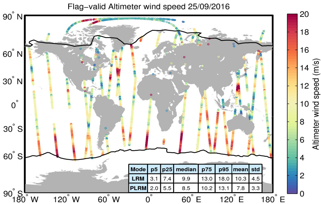
Figure 31. Geographical distribution of flag-valid wind data over oceans and lakes for 25/09/2016. The statistical values shown in the table refer to the wind in m/s and are calculated separately for LRM and PLRM regions. Measurements taken over polar polygons have been excluded from the computation of the statistical values. The black lines mark the outer limit of the Arctic and Antarctic polar polygons.
