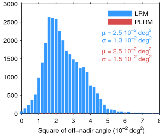
Figure 39. Histogram of flag-valid mispointing over oceans and lakes for LRM (blue) and PLRM (red) for 24/09/2016. Only positive values have been considered. The mean ( \mu ) and standard deviation ( \sigma ) are also shown. Note that values larger than 8 \cdot 10^{-2} \text{ deg}^2 are excluded from the histogram for the sake of readability but not from the computation of \mu and \sigma .
