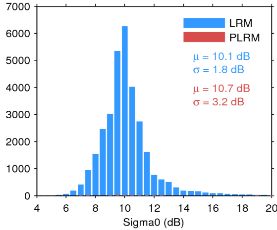
Figure 25. Histogram of flag-valid sigma0 over oceans and lakes for LRM (blue) and PLRM (red) for 24/09/2016. The mean ( \mu ) and standard deviation ( \sigma ) are also shown. Note that values outside [4 20] dB are excluded from the histogram for the sake of readability but not from the computation of \mu and \sigma .
