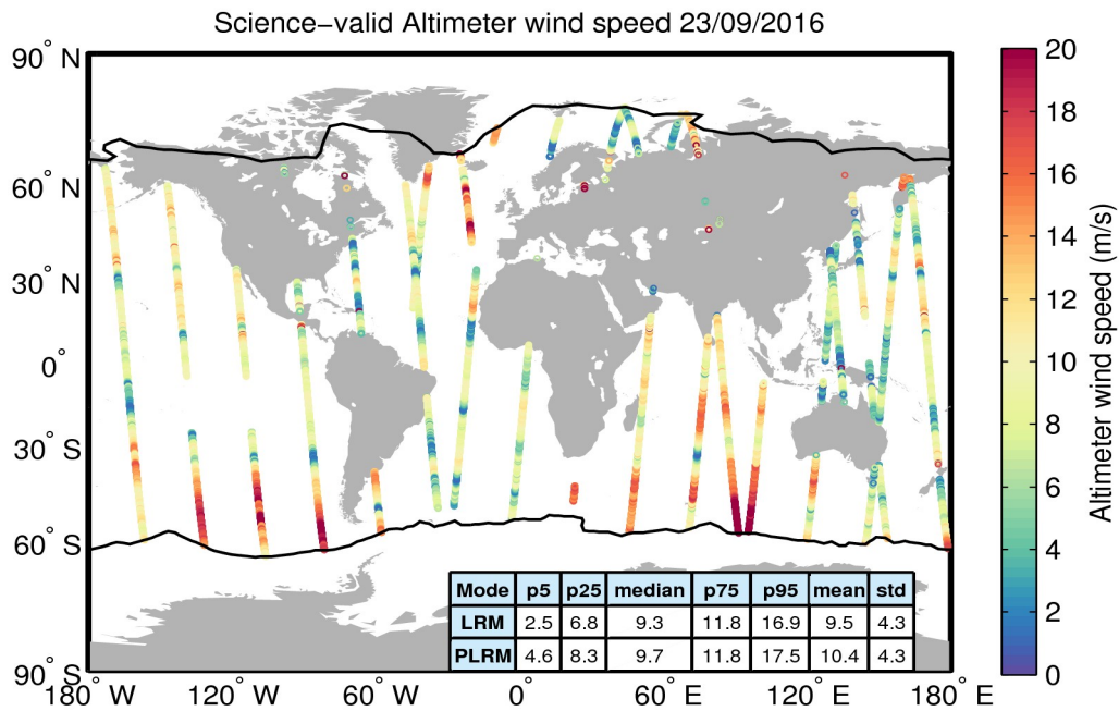
Figure 34. Geographical distribution of science-valid wind data over oceans and lakes for 23/09/2016. The statistical values shown in the table refer to the wind in m/s and are calculated separately for LRM and PLRM regions. The black lines mark the outer limit of the Arctic and Antarctic polar polygons. Gray circles denote records that have been rejected based on the editing criteria described in Table 5.
