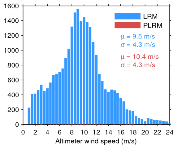
Figure 35. Histogram of science-valid wind over oceans and lakes for LRM (blue) and PLRM (red) for 23/09/2016. The mean ( \mu ) and standard deviation ( \sigma ) are also shown. Note that values larger than 24 m/s are excluded from the histogram for the sake of readability but not from the computation of \mu and \sigma .
