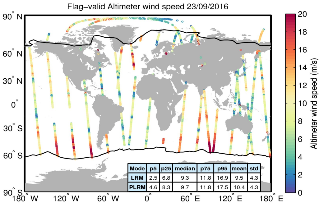
Figure 31. Geographical distribution of flag-valid wind data over oceans and lakes for 23/09/2016. The statistical values shown in the table refer to the wind in m/s and are calculated separately for LRM and PLRM regions. Measurements taken over polar polygons have been excluded from the computation of the statistical values. The black lines mark the outer limit of the Arctic and Antarctic polar polygons.
