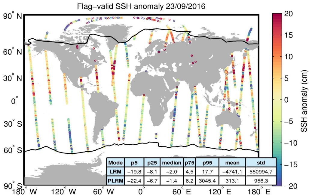
Figure 5. Geographical distribution of flag-valid 1-Hz SSH anomaly data over oceans and lakes for 23/09/2016. The statistical values shown in the table refer to the SSH anomaly in cm and are calculated separately for LRM and PLRM regions. Measurements taken over polar polygons have been excluded from the computation of the statistical values. The black lines mark the outer limit of the Arctic and Antarctic polar polygons.
