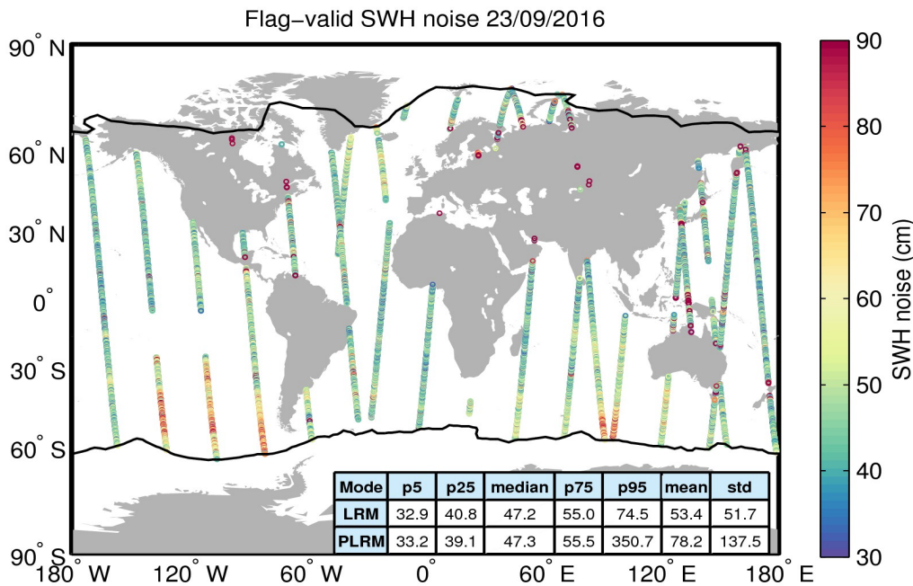
Figure 18. Geographical distribution of flag-valid 20-Hz SWH measurement noise over oceans and lakes for 23/09/2016. The statistical values shown in the table refer to the SWH noise and are calculated separately for LRM and PLRM regions. Measurements taken over polar polygons have been excluded from the computation of the statistical values. The black lines mark the outer limit of the Arctic and Antarctic polar polygons.
