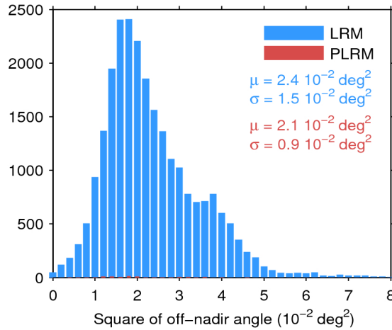
Figure 39. Histogram of flag-valid mispointing over oceans and lakes for LRM (blue) and PLRM (red) for 23/09/2016. Only positive values have been considered. The mean ( \mu ) and standard deviation ( \sigma ) are also shown. Note that values larger than 8 \times 10^{-2} \text{ deg}^2 are excluded from the histogram for the sake of readability but not from the computation of \mu and \sigma .
