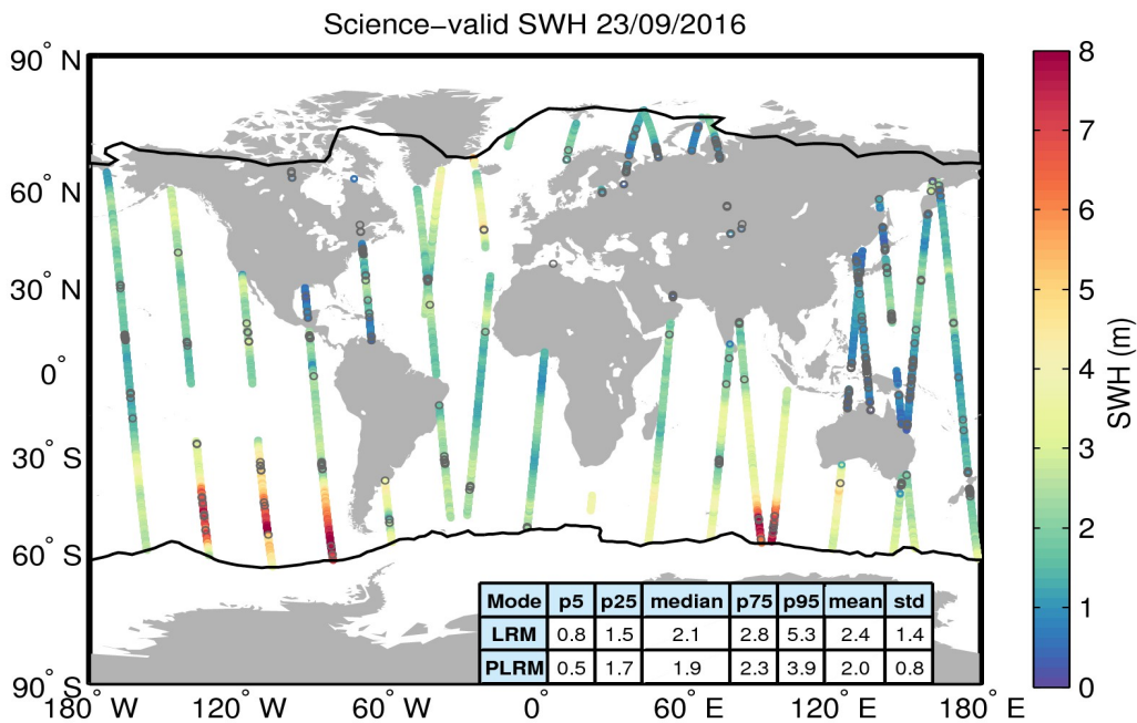
Figure 19. Geographical distribution of science-valid SWH data over oceans and lakes for 23/09/2016. The statistical values shown in the table refer to the SWH in m and are calculated separately for LRM and PLRM regions. The black lines mark the outer limit of the Arctic and Antarctic polar polygons. Gray circles denote records that have been rejected based on the editing criteria described in Table 3.
