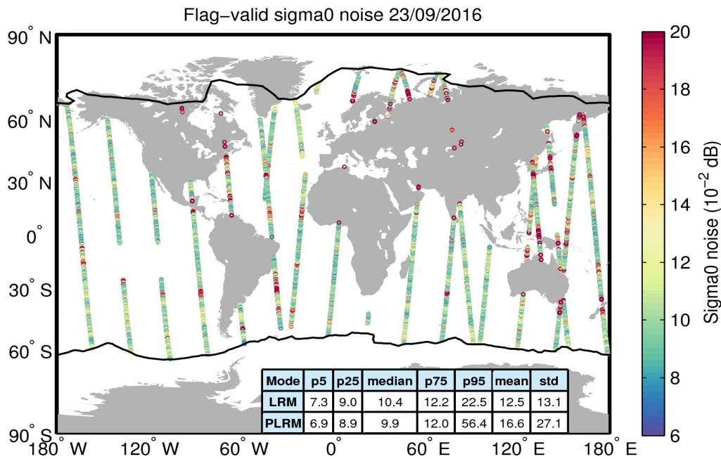
Figure 26. Geographical distribution of flag-valid 20-Hz sigma0 measurement noise over oceans and lakes for 23/09/2016. The statistical values shown in the table refer to the sigma0 noise and are calculated separately for LRM and PLRM regions. Measurements taken over polar polygons have been excluded from the computation of the statistical values. The black lines mark the outer limit of the Arctic and Antarctic polar polygons.
