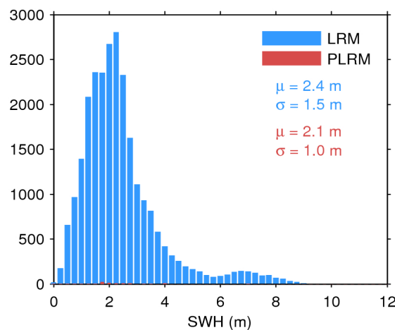
Figure 17. Histogram of flag-valid SWH over oceans and lakes for LRM (blue) and PLRM (red) for 23/09/2016. The mean ( \mu ) and standard deviation ( \sigma ) are also shown. Note that values larger than 12 m are excluded from the histogram for the sake of readability but not from the computation of \mu and \sigma .
