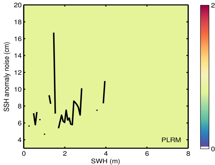
Figure 9. 2D histogram showing flag-valid SSH anomaly noise as a function of SWH for LRM (top) and PLRM (bottom) for 23/09/2016. The black line denotes the median SSH anomaly noise as a function of SWH.
