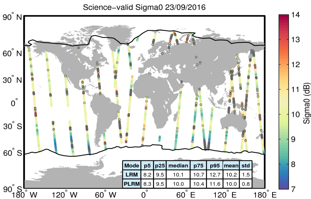
Figure 27. Geographical distribution of science-valid sigma0 data over oceans and lakes for 23/09/2016. The statistical values shown in the table refer to the sigma0 in dB and are calculated separately for LRM and PLRM regions. The black lines mark the outer limit of the Arctic and Antarctic polar polygons. Gray circles denote records that have been rejected based on the editing criteria described in Table 4.
