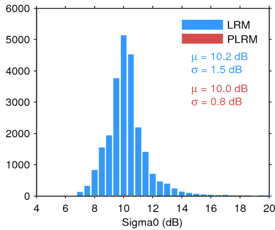
Figure 28. Histogram of science-valid sigma0 over oceans and lakes for LRM (blue) and PLRM (red) for 23/09/2016. The mean ( \mu ) and standard deviation ( \sigma ) are also shown. Note that values outside [4 20] dB are excluded from the histogram for the sake of readability but not from the computation of \mu and \sigma .
