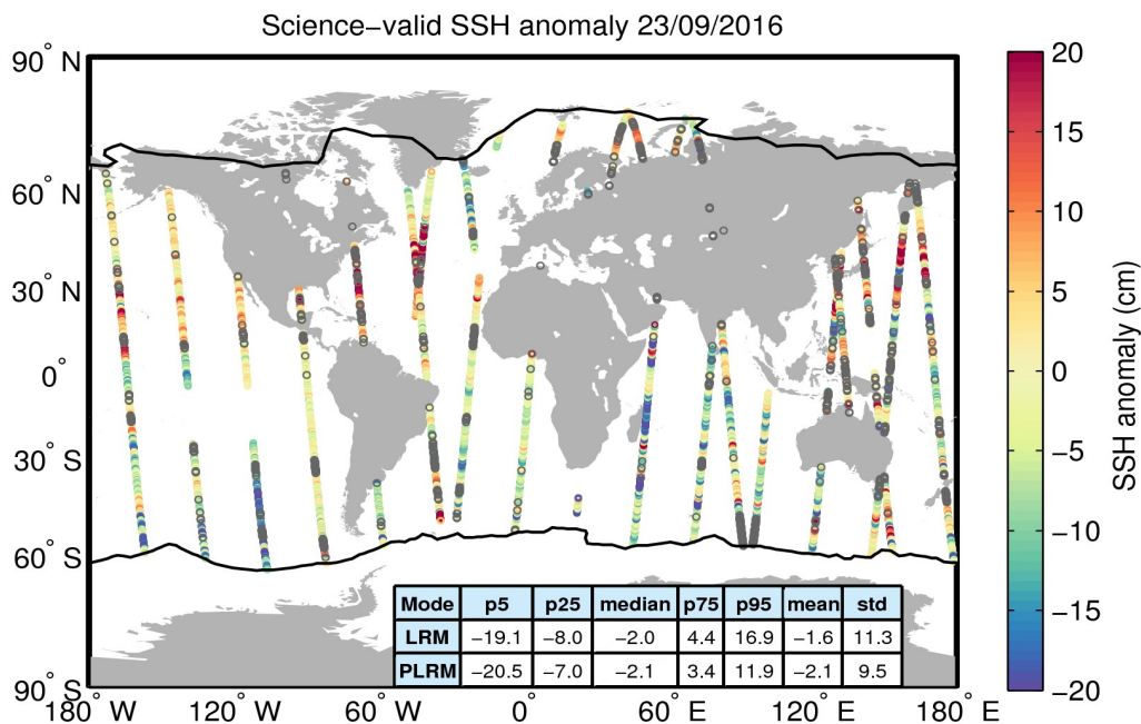
Figure 10. Geographical distribution of science-valid SSH anomaly data over oceans and lakes for 23/09/2016. The statistical values shown in the table refer to the SSH anomaly in cm and are calculated separately for LRM and PLRM regions. The black lines mark the outer limit of the Arctic and Antarctic polar polygons. Gray circles denote records that have been rejected based on the editing criteria described in Table 2.
