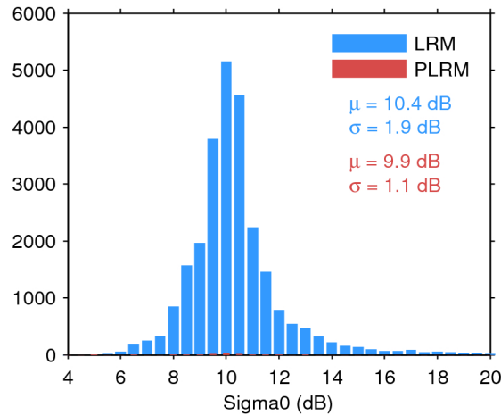
Figure 25. Histogram of flag-valid sigma0 over oceans and lakes for LRM (blue) and PLRM (red) for 23/09/2016. The mean ( \mu ) and standard deviation ( \sigma ) are also shown. Note that values outside [4 20] dB are excluded from the histogram for the sake of readability but not from the computation of \mu and \sigma .
