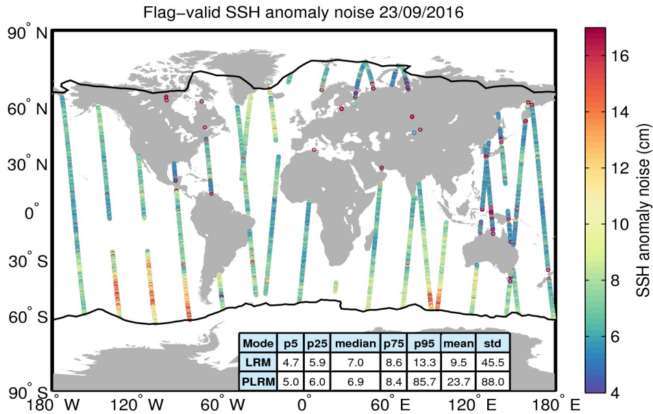
Figure 8. Geographical distribution of flag-valid 20-Hz SSH anomaly measurement noise over oceans and lakes for 23/09/2016. The statistical values shown in the table refer to the SSH anomaly noise and are calculated separately for LRM and PLRM regions. Measurements taken over polar polygons have been excluded from the computation of the statistical values. The black lines mark the outer limit of the Arctic and Antarctic polar polygons.
