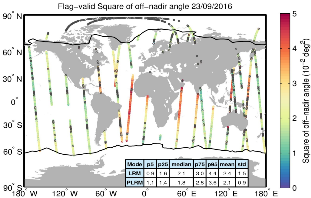
Figure 37. Geographical distribution of flag-valid mispointing data over oceans and lakes for 23/09/2016. The statistical values shown in the table refer to the mispointing in 10^{-2} deg 2 and are calculated separately for LRM and PLRM regions. Measurements taken over polar polygons have been excluded from the computation of the statistical values. The black lines mark the outer limit of the Arctic and Antarctic polar polygons. Gray circles denote negative values.
