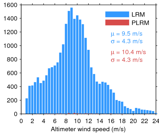
Figure 33. Histogram of flag-valid wind over oceans and lakes for LRM (blue) and PLRM (red) for 23/09/2016. The mean ( \mu ) and standard deviation ( \sigma ) are also shown. Note that values larger than 24 m/s are excluded from the histogram for the sake of readability but not from the computation of \mu and \sigma .
