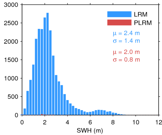
Figure 20. Histogram of science-valid SWH over oceans and lakes for LRM (blue) and PLRM (red) for 23/09/2016. The mean ( \mu ) and standard deviation ( \sigma ) are also shown. Note that values larger than 12 m are excluded from the histogram for the sake of readability but not from the computation of \mu and \sigma .
