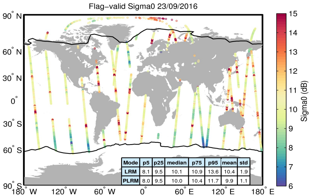
Figure 23. Geographical distribution of flag-valid sigma0 data over oceans and lakes for 23/09/2016. The statistical values shown in the table refer to the sigma0 in dB and are calculated separately for LRM and PLRM regions. Measurements taken over polar polygons have been excluded from the computation of the statistical values. The black lines mark the outer limit of the Arctic and Antarctic polar polygons.
