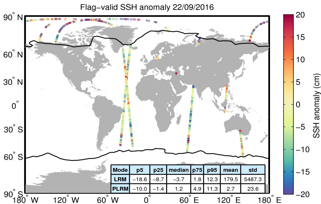
Figure 5. Geographical distribution of flag-valid 1-Hz SSH anomaly data over oceans and lakes for 22/09/2016. The statistical values shown in the table refer to the SSH anomaly in cm and are calculated separately for LRM and PLRM regions. Measurements taken over polar polygons have been excluded from the computation of the statistical values. The black lines mark the outer limit of the Arctic and Antarctic polar polygons.
