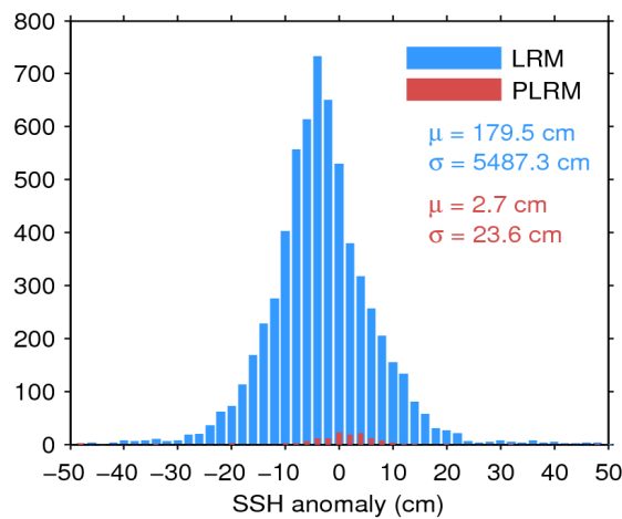
Figure 7. Histogram of flag-valid SSH anomaly over oceans and lakes for LRM (blue) and PLRM (red) for 22/09/2016. The mean ( \mu ) and standard deviation ( \sigma ) are also shown. Note that values outside [-50 50] cm are excluded from the histogram for the sake of readability but not from the computation of \mu and \sigma .
