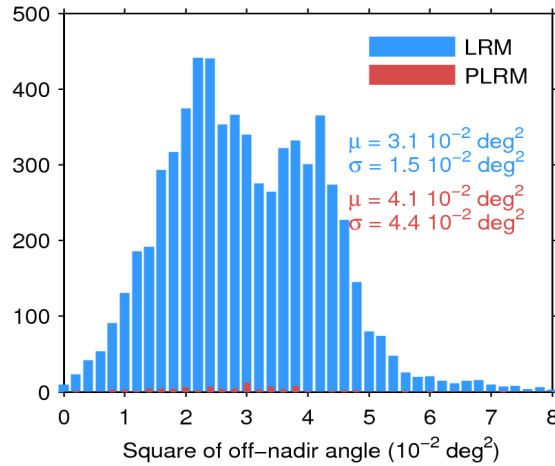
Figure 39. Histogram of flag-valid mispointing over oceans and lakes for LRM (blue) and PLRM (red) for 22/09/2016. Only positive values have been considered. The mean ( \mu ) and standard deviation ( \sigma ) are also shown. Note that values larger than 8 \cdot 10^{-2} \text{ deg}^2 are excluded from the histogram for the sake of readability but not from the computation of \mu and \sigma .
