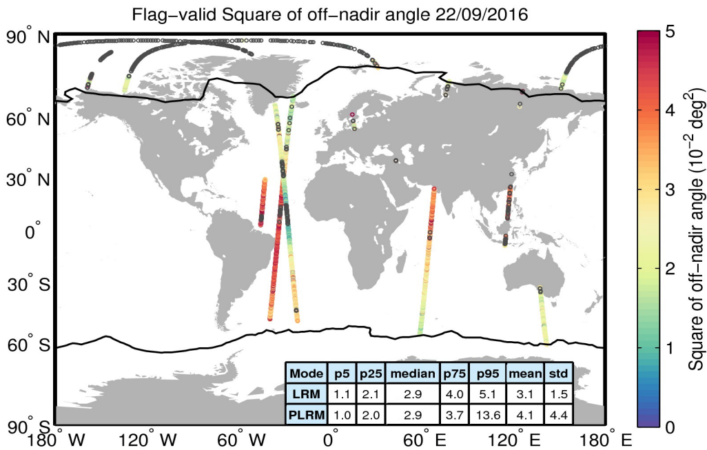
Figure 37. Geographical distribution of flag-valid mispointing data over oceans and lakes for 22/09/2016. The statistical values shown in the table refer to the mispointing in 10^{-2} deg 2 and are calculated separately for LRM and PLRM regions. Measurements taken over polar polygons have been excluded from the computation of the statistical values. The black lines mark the outer limit of the Arctic and Antarctic polar polygons. Gray circles denote negative values.
