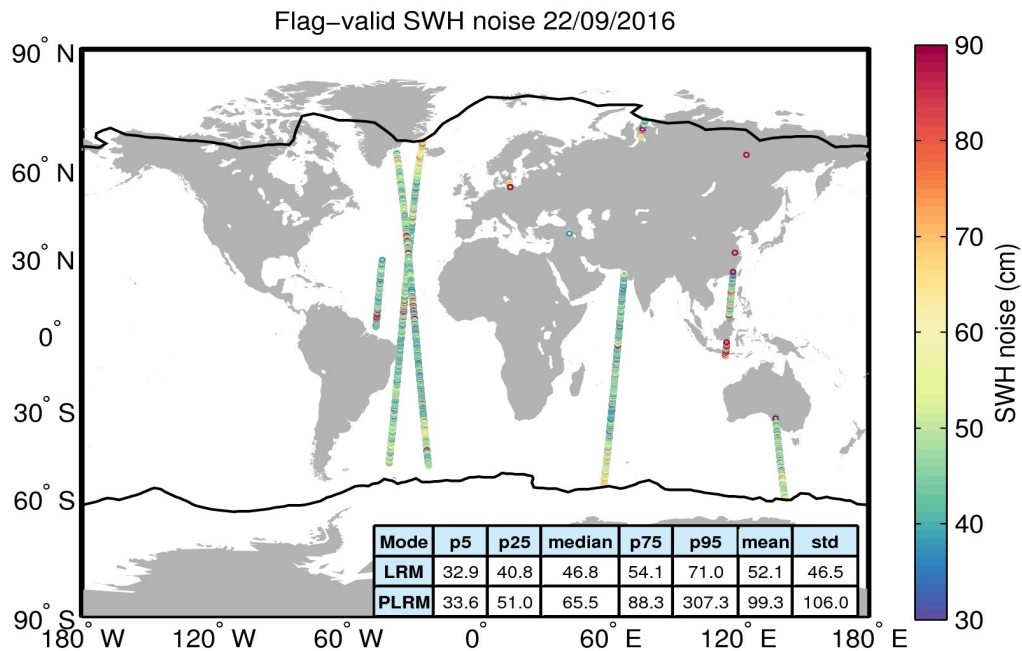
Figure 18. Geographical distribution of flag-valid 20-Hz SWH measurement noise over oceans and lakes for 22/09/2016. The statistical values shown in the table refer to the SWH noise and are calculated separately for LRM and PLRM regions. Measurements taken over polar polygons have been excluded from the computation of the statistical values. The black lines mark the outer limit of the Arctic and Antarctic polar polygons.
