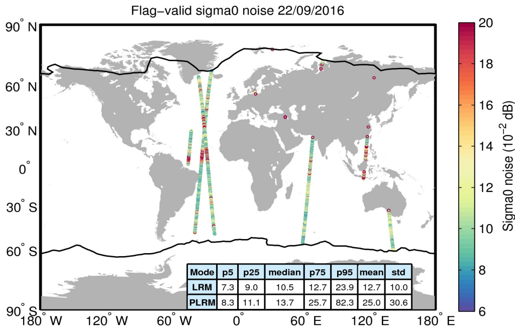
Figure 26. Geographical distribution of flag-valid 20-Hz sigma0 measurement noise over oceans and lakes for 22/09/2016. The statistical values shown in the table refer to the sigma0 noise and are calculated separately for LRM and PLRM regions. Measurements taken over polar polygons have been excluded from the computation of the statistical values. The black lines mark the outer limit of the Arctic and Antarctic polar polygons.
