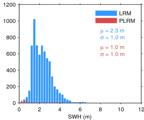
Figure 17. Histogram of flag-valid SWH over oceans and lakes for LRM (blue) and PLRM (red) for 22/09/2016. The mean ( \mu ) and standard deviation ( \sigma ) are also shown. Note that values larger than 12 m are excluded from the histogram for the sake of readability but not from the computation of \mu and \sigma .
