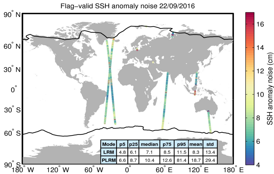
Figure 8. Geographical distribution of flag-valid 20-Hz SSH anomaly measurement noise over oceans and lakes for 22/09/2016. The statistical values shown in the table refer to the SSH anomaly noise and are calculated separately for LRM and PLRM regions. Measurements taken over polar polygons have been excluded from the computation of the statistical values. The black lines mark the outer limit of the Arctic and Antarctic polar polygons.
