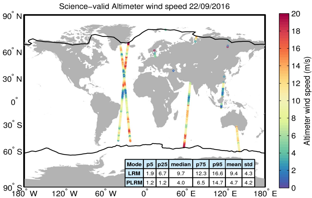
Figure 34. Geographical distribution of science-valid wind data over oceans and lakes for 22/09/2016. The statistical values shown in the table refer to the wind in m/s and are calculated separately for LRM and PLRM regions. The black lines mark the outer limit of the Arctic and Antarctic polar polygons. Gray circles denote records that have been rejected based on the editing criteria described in Table 5.
