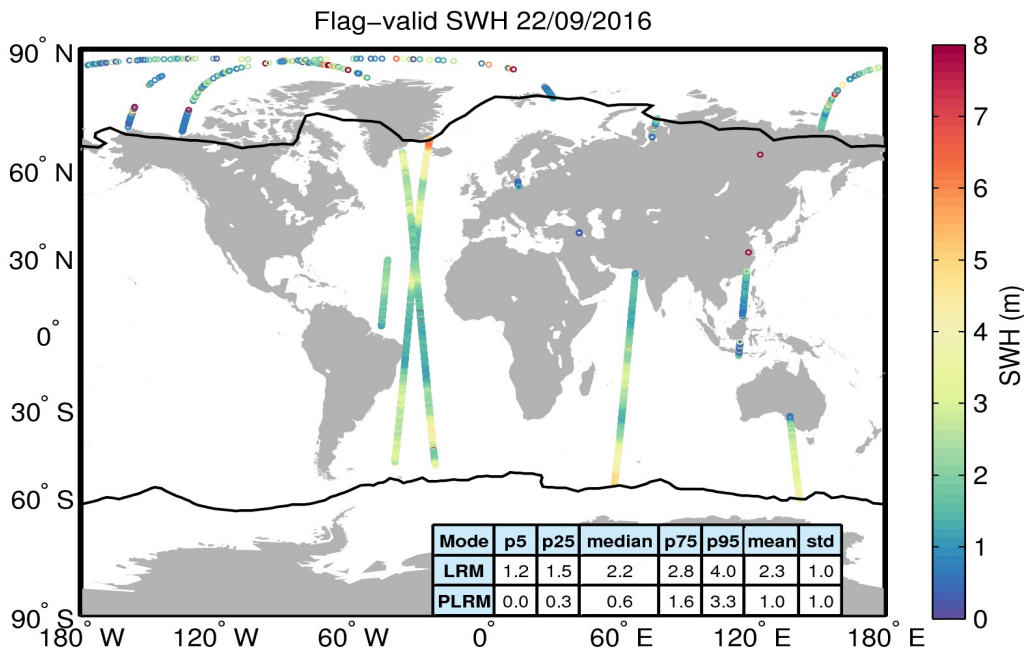
Figure 15. Geographical distribution of flag-valid SWH data over oceans and lakes for 22/09/2016. The statistical values shown in the table refer to the SWH in m and are calculated separately for LRM and PLRM regions. Measurements taken over polar polygons have been excluded from the computation of the statistical values. The black lines mark the outer limit of the Arctic and Antarctic polar polygons.
