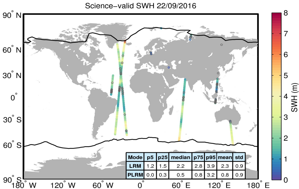
Figure 19. Geographical distribution of science-valid SWH data over oceans and lakes for 22/09/2016. The statistical values shown in the table refer to the SWH in m and are calculated separately for LRM and PLRM regions. The black lines mark the outer limit of the Arctic and Antarctic polar polygons. Gray circles denote records that have been rejected based on the editing criteria described in Table 3.
