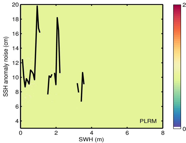
Figure 9. 2D histogram showing flag-valid SSH anomaly noise as a function of SWH for LRM (top) and PLRM (bottom) for 22/09/2016. The black line denotes the median SSH anomaly noise as a function of SWH.
