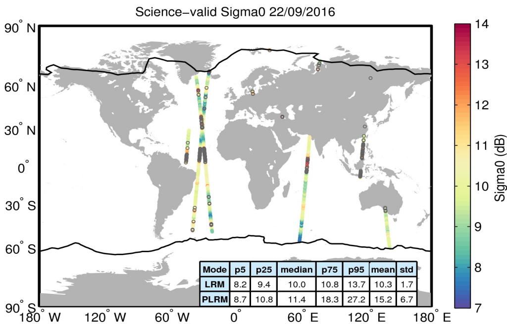
Figure 27. Geographical distribution of science-valid sigma0 data over oceans and lakes for 22/09/2016. The statistical values shown in the table refer to the sigma0 in dB and are calculated separately for LRM and PLRM regions. The black lines mark the outer limit of the Arctic and Antarctic polar polygons. Gray circles denote records that have been rejected based on the editing criteria described in Table 4.
