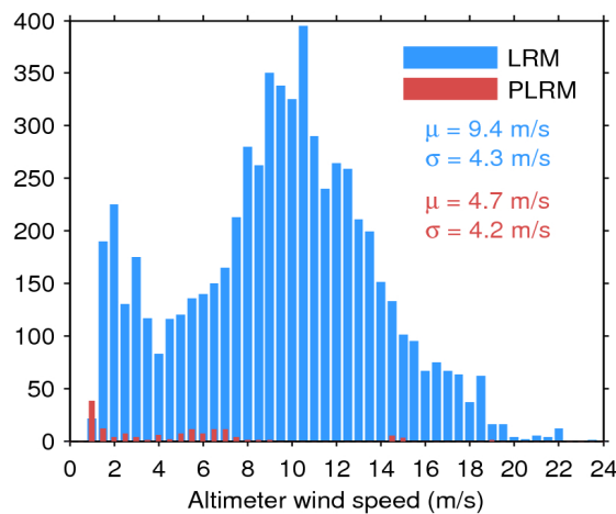
Figure 35. Histogram of science-valid wind over oceans and lakes for LRM (blue) and PLRM (red) for 22/09/2016. The mean ( \mu ) and standard deviation ( \sigma ) are also shown. Note that values larger than 24 m/s are excluded from the histogram for the sake of readability but not from the computation of \mu and \sigma .
