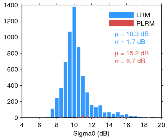
Figure 28. Histogram of science-valid sigma0 over oceans and lakes for LRM (blue) and PLRM (red) for 22/09/2016. The mean ( \mu ) and standard deviation ( \sigma ) are also shown. Note that values outside [4 20] dB are excluded from the histogram for the sake of readability but not from the computation of \mu and \sigma .
