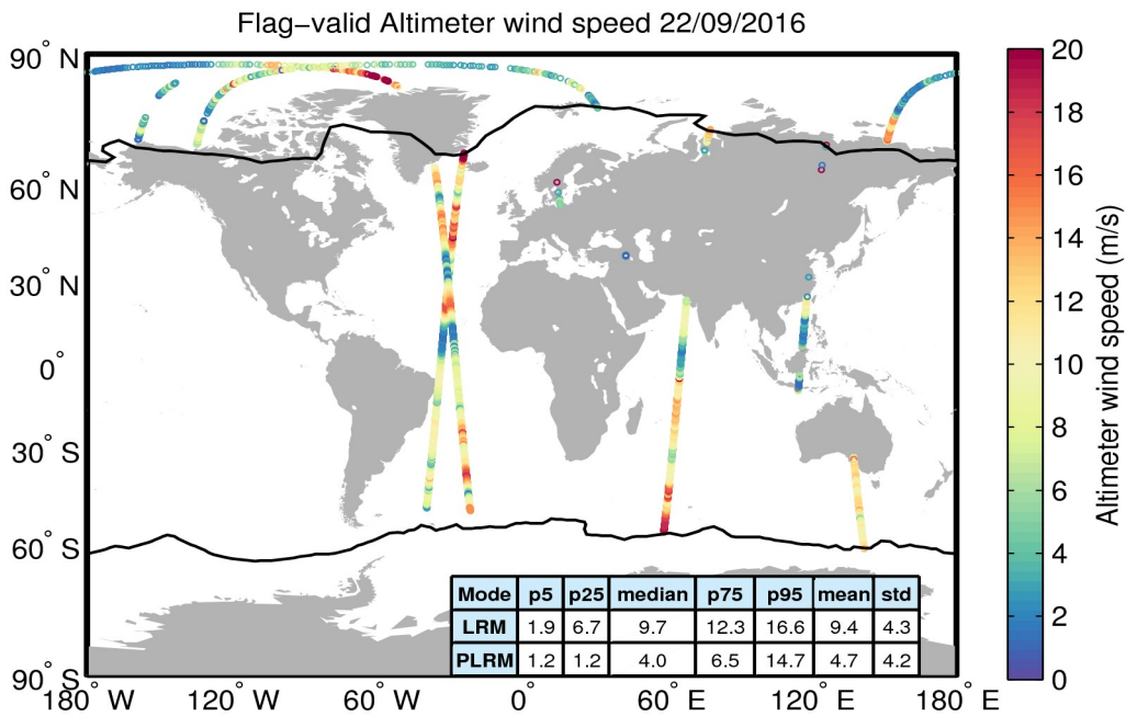
Figure 31. Geographical distribution of flag-valid wind data over oceans and lakes for 22/09/2016. The statistical values shown in the table refer to the wind in m/s and are calculated separately for LRM and PLRM regions. Measurements taken over polar polygons have been excluded from the computation of the statistical values. The black lines mark the outer limit of the Arctic and Antarctic polar polygons.
