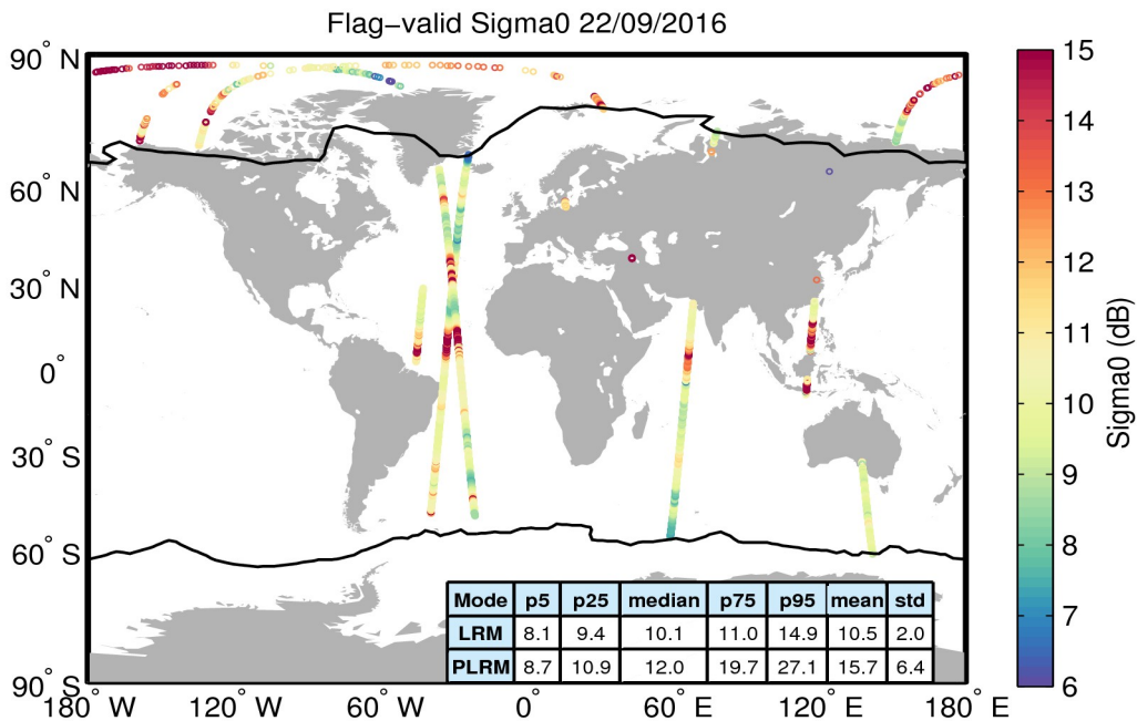
Figure 23. Geographical distribution of flag-valid sigma0 data over oceans and lakes for 22/09/2016. The statistical values shown in the table refer to the sigma0 in dB and are calculated separately for LRM and PLRM regions. Measurements taken over polar polygons have been excluded from the computation of the statistical values. The black lines mark the outer limit of the Arctic and Antarctic polar polygons.
