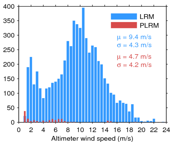
Figure 33. Histogram of flag-valid wind over oceans and lakes for LRM (blue) and PLRM (red) for 22/09/2016. The mean ( \mu ) and standard deviation ( \sigma ) are also shown. Note that values larger than 24 m/s are excluded from the histogram for the sake of readability but not from the computation of \mu and \sigma .
