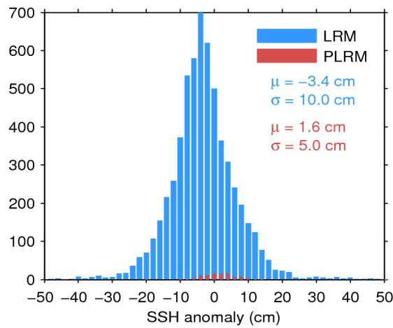
Figure 11. Histogram of science-valid SSH anomaly over oceans and lakes for LRM (blue) and PLRM (red) for 22/09/2016. The mean ( \mu ) and standard deviation ( \sigma ) are also shown. Note that values outside [-50 50] cm are excluded from the histogram for the sake of readability but not from the computation of \mu and \sigma .
