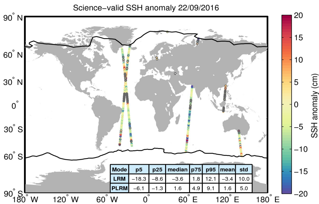
Figure 10. Geographical distribution of science-valid SSH anomaly data over oceans and lakes for 22/09/2016. The statistical values shown in the table refer to the SSH anomaly in cm and are calculated separately for LRM and PLRM regions. The black lines mark the outer limit of the Arctic and Antarctic polar polygons. Gray circles denote records that have been rejected based on the editing criteria described in Table 2.
