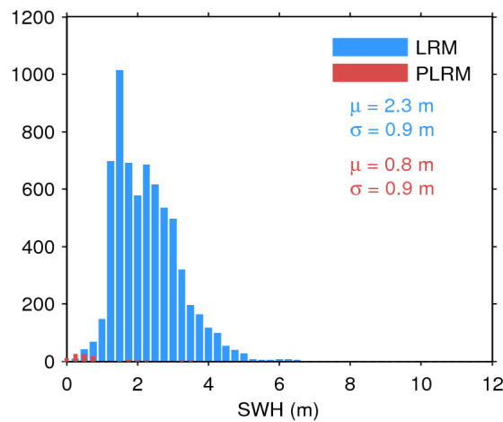
Figure 20. Histogram of science-valid SWH over oceans and lakes for LRM (blue) and PLRM (red) for 22/09/2016. The mean ( \mu ) and standard deviation ( \sigma ) are also shown. Note that values larger than 12 m are excluded from the histogram for the sake of readability but not from the computation of \mu and \sigma .
