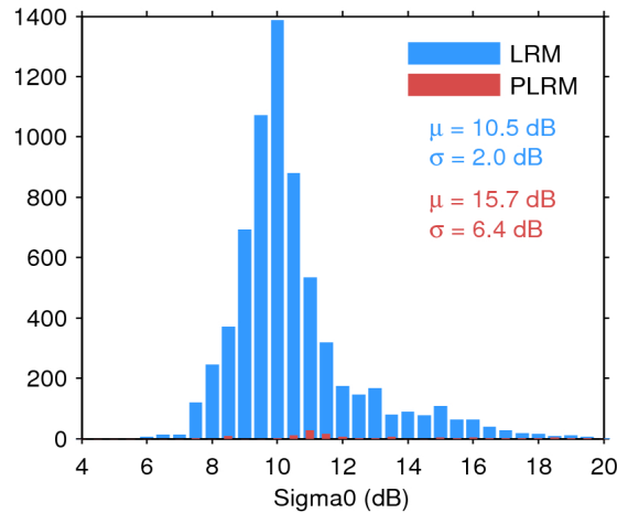
Figure 25. Histogram of flag-valid sigma0 over oceans and lakes for LRM (blue) and PLRM (red) for 22/09/2016. The mean ( \mu ) and standard deviation ( \sigma ) are also shown. Note that values outside [4 20] dB are excluded from the histogram for the sake of readability but not from the computation of \mu and \sigma .
