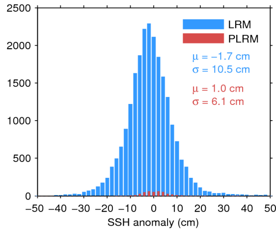
Figure 11. Histogram of science-valid SSH anomaly over oceans and lakes for LRM (blue) and PLRM (red) for 20/09/2016. The mean ( \mu ) and standard deviation ( \sigma ) are also shown. Note that values outside [-50\ 50] cm are excluded from the histogram for the sake of readability but not from the computation of \mu and \sigma .
