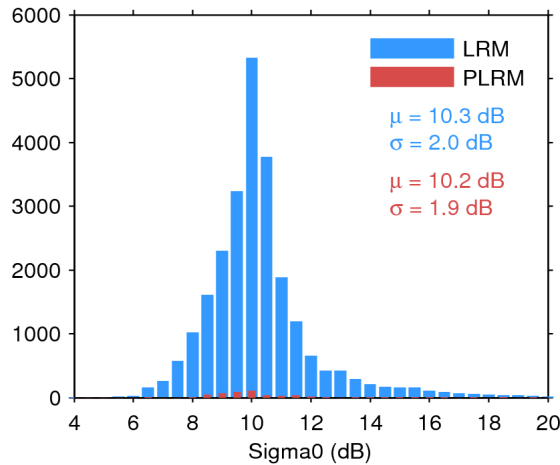
Figure 25. Histogram of flag-valid sigma0 over oceans and lakes for LRM (blue) and PLRM (red) for 20/09/2016. The mean ( \mu ) and standard deviation ( \sigma ) are also shown. Note that values outside [4 20] dB are excluded from the histogram for the sake of readability but not from the computation of \mu and \sigma .
