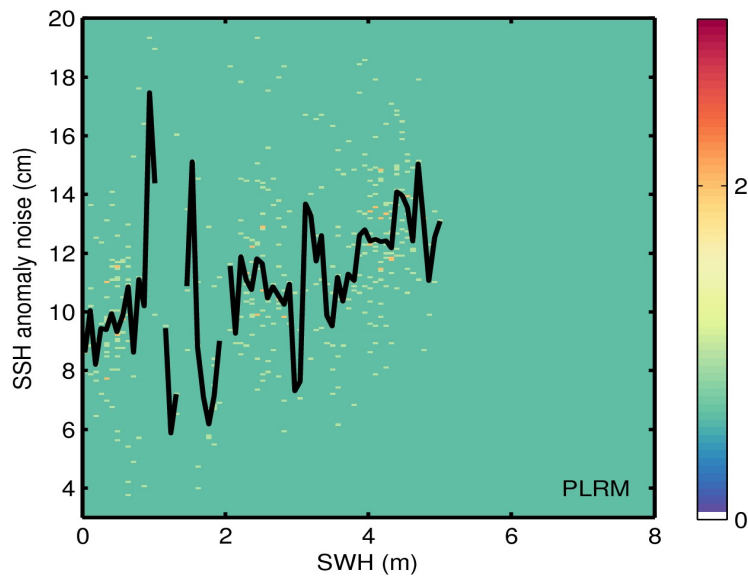
Figure 9. 2D histogram showing flag-valid SSH anomaly noise as a function of SWH for LRM (top) and PLRM (bottom) for 20/09/2016. The black line denotes the median SSH anomaly noise as a function of SWH.
