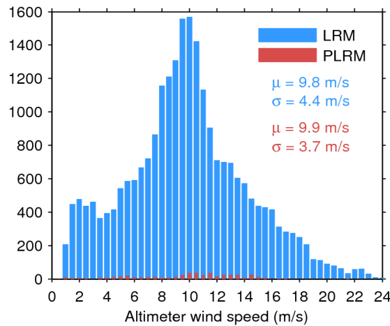
Figure 33. Histogram of flag-valid wind over oceans and lakes for LRM (blue) and PLRM (red) for 20/09/2016. The mean ( \mu ) and standard deviation ( \sigma ) are also shown. Note that values larger than 24 m/s are excluded from the histogram for the sake of readability but not from the computation of \mu and \sigma .
