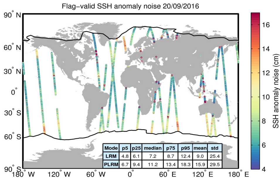
Figure 8. Geographical distribution of flag-valid 20-Hz SSH anomaly measurement noise over oceans and lakes for 20/09/2016. The statistical values shown in the table refer to the SSH anomaly noise and are calculated separately for LRM and PLRM regions. Measurements taken over polar polygons have been excluded from the computation of the statistical values. The black lines mark the outer limit of the Arctic and Antarctic polar polygons.
