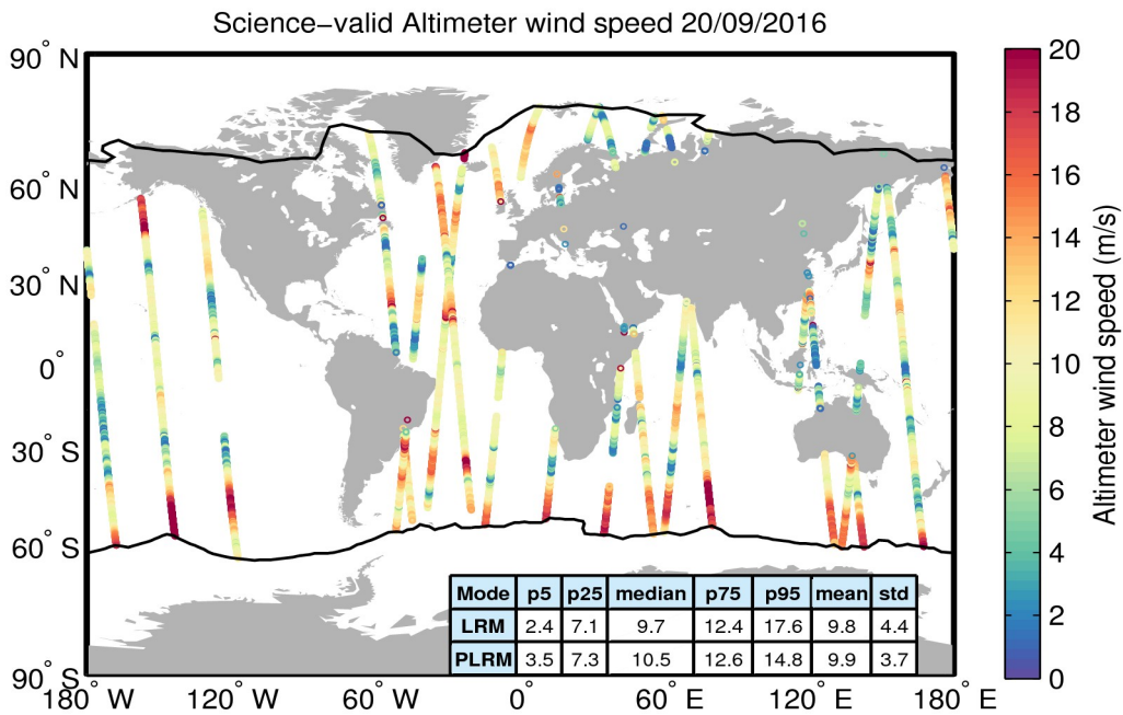
Figure 34. Geographical distribution of science-valid wind data over oceans and lakes for 20/09/2016. The statistical values shown in the table refer to the wind in m/s and are calculated separately for LRM and PLRM regions. The black lines mark the outer limit of the Arctic and Antarctic polar polygons. Gray circles denote records that have been rejected based on the editing criteria described in Table 5.
