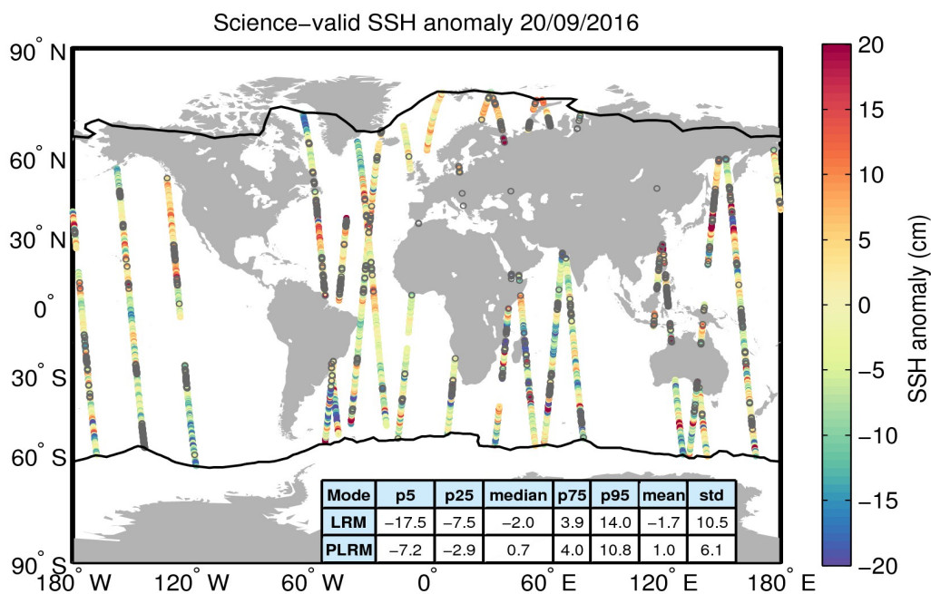
Figure 10. Geographical distribution of science-valid SSH anomaly data over oceans and lakes for 20/09/2016. The statistical values shown in the table refer to the SSH anomaly in cm and are calculated separately for LRM and PLRM regions. The black lines mark the outer limit of the Arctic and Antarctic polar polygons. Gray circles denote records that have been rejected based on the editing criteria described in Table 2.
