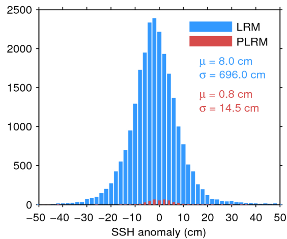
Figure 7. Histogram of flag-valid SSH anomaly over oceans and lakes for LRM (blue) and PLRM (red) for 20/09/2016. The mean ( \mu ) and standard deviation ( \sigma ) are also shown. Note that values outside [-50\ 50] cm are excluded from the histogram for the sake of readability but not from the computation of \mu and \sigma .
