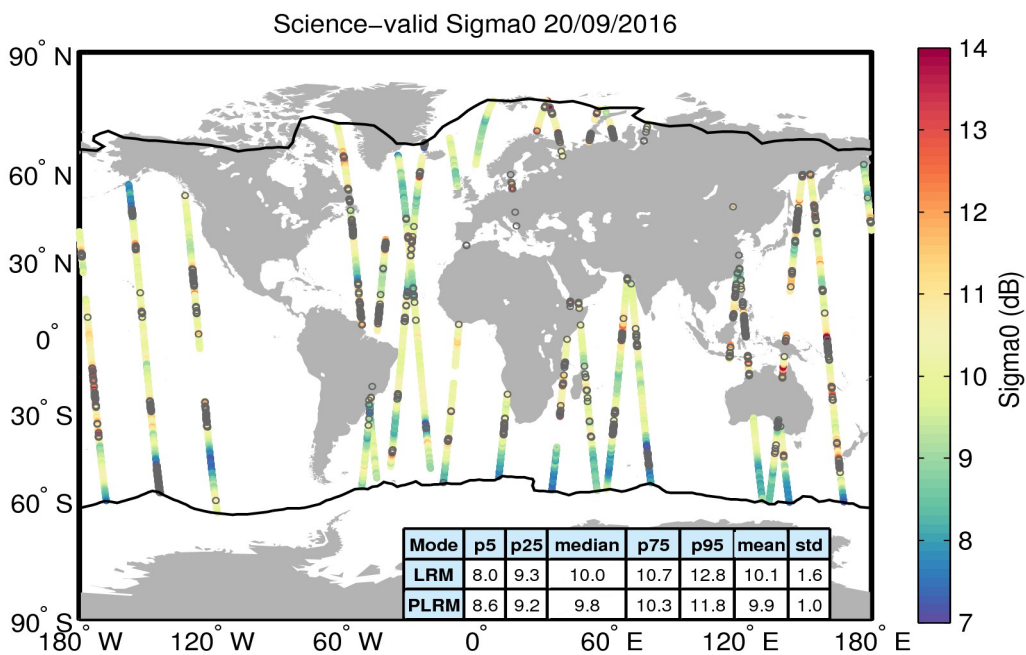
Figure 27. Geographical distribution of science-valid sigma0 data over oceans and lakes for 20/09/2016. The statistical values shown in the table refer to the sigma0 in dB and are calculated separately for LRM and PLRM regions. The black lines mark the outer limit of the Arctic and Antarctic polar polygons. Gray circles denote records that have been rejected based on the editing criteria described in Table 4.
