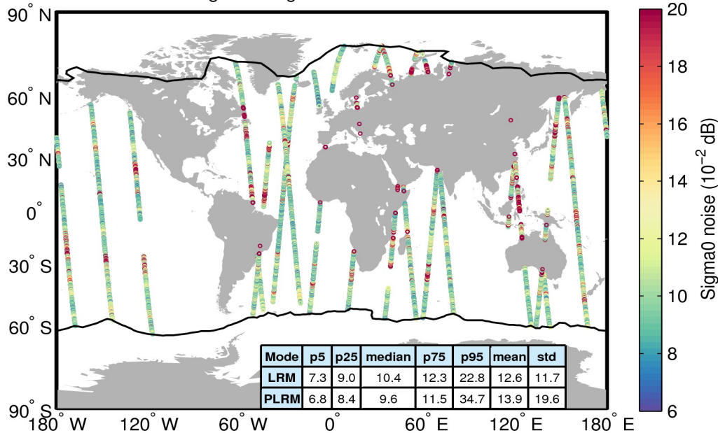
Flag-valid sigma0 noise 20/09/2016
