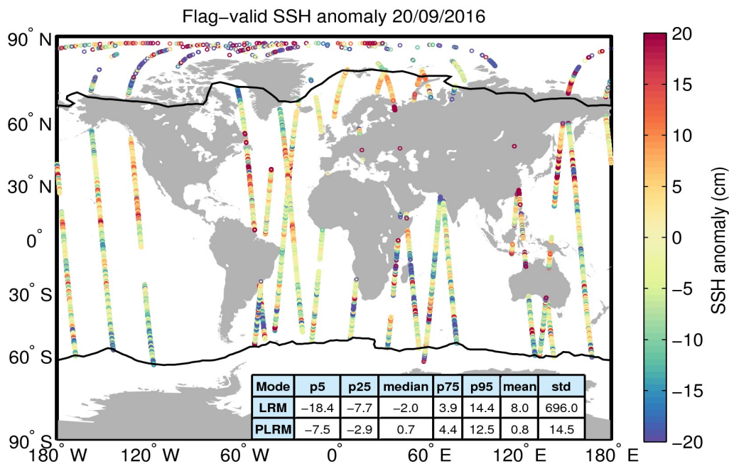
Figure 5. Geographical distribution of flag-valid 1-Hz SSH anomaly data over oceans and lakes for 20/09/2016. The statistical values shown in the table refer to the SSH anomaly in cm and are calculated separately for LRM and PLRM regions. Measurements taken over polar polygons have been excluded from the computation of the statistical values. The black lines mark the outer limit of the Arctic and Antarctic polar polygons.
