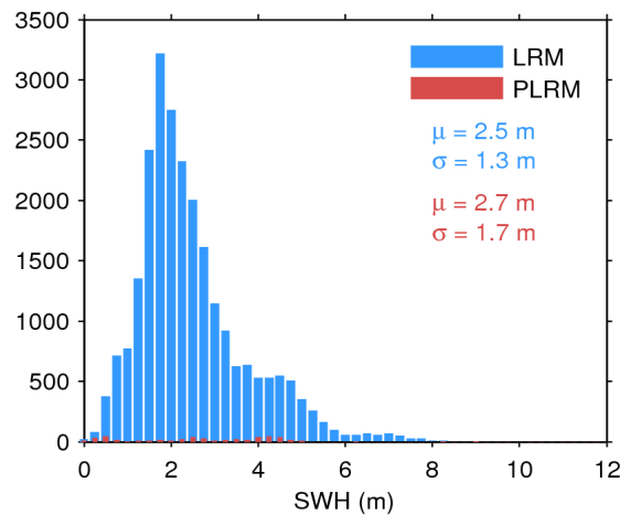
Figure 17. Histogram of flag-valid SWH over oceans and lakes for LRM (blue) and PLRM (red) for 20/09/2016. The mean ( \mu ) and standard deviation ( \sigma ) are also shown. Note that values larger than 12 m are excluded from the histogram for the sake of readability but not from the computation of \mu and \sigma .
