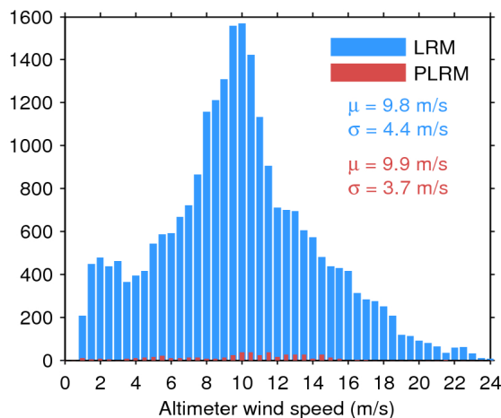
Figure 35. Histogram of science-valid wind over oceans and lakes for LRM (blue) and PLRM (red) for 20/09/2016. The mean ( \mu ) and standard deviation ( \sigma ) are also shown. Note that values larger than 24 m/s are excluded from the histogram for the sake of readability but not from the computation of \mu and \sigma .
