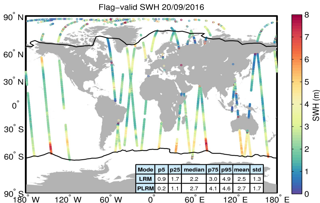
Figure 15. Geographical distribution of flag-valid SWH data over oceans and lakes for 20/09/2016. The statistical values shown in the table refer to the SWH in m and are calculated separately for LRM and PLRM regions. Measurements taken over polar polygons have been excluded from the computation of the statistical values. The black lines mark the outer limit of the Arctic and Antarctic polar polygons.
