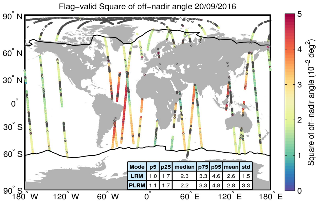
Figure 37. Geographical distribution of flag-valid mispointing data over oceans and lakes for 20/09/2016. The statistical values shown in the table refer to the mispointing in 10^{-2} deg 2 and are calculated separately for LRM and PLRM regions. Measurements taken over polar polygons have been excluded from the computation of the statistical values. The black lines mark the outer limit of the Arctic and Antarctic polar polygons. Gray circles denote negative values.
