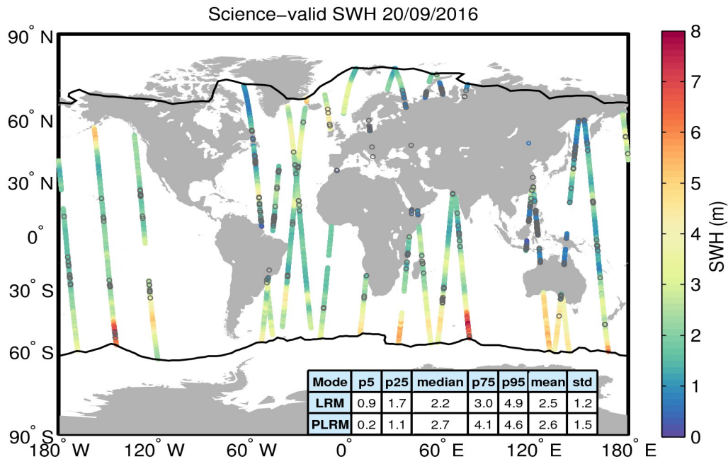
Figure 19. Geographical distribution of science-valid SWH data over oceans and lakes for 20/09/2016. The statistical values shown in the table refer to the SWH in m and are calculated separately for LRM and PLRM regions. The black lines mark the outer limit of the Arctic and Antarctic polar polygons. Gray circles denote records that have been rejected based on the editing criteria described in Table 3.
