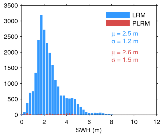
Figure 20. Histogram of science-valid SWH over oceans and lakes for LRM (blue) and PLRM (red) for 20/09/2016. The mean ( \mu ) and standard deviation ( \sigma ) are also shown. Note that values larger than 12 m are excluded from the histogram for the sake of readability but not from the computation of \mu and \sigma .
