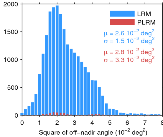
Figure 39. Histogram of flag-valid mispointing over oceans and lakes for LRM (blue) and PLRM (red) for 20/09/2016. Only positive values have been considered. The mean ( \mu ) and standard deviation ( \sigma ) are also shown. Note that values larger than 8 \cdot 10^{-2} \text{ deg}^2 are excluded from the histogram for the sake of readability but not from the computation of \mu and \sigma .
