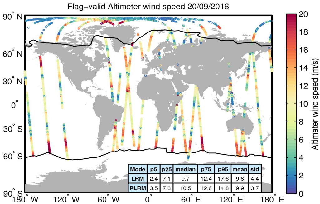
Figure 31. Geographical distribution of flag-valid wind data over oceans and lakes for 20/09/2016. The statistical values shown in the table refer to the wind in m/s and are calculated separately for LRM and PLRM regions. Measurements taken over polar polygons have been excluded from the computation of the statistical values. The black lines mark the outer limit of the Arctic and Antarctic polar polygons.
