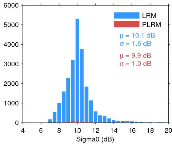
Figure 28. Histogram of science-valid sigma0 over oceans and lakes for LRM (blue) and PLRM (red) for 20/09/2016. The mean ( \mu ) and standard deviation ( \sigma ) are also shown. Note that values outside [4 20] dB are excluded from the histogram for the sake of readability but not from the computation of \mu and \sigma .
