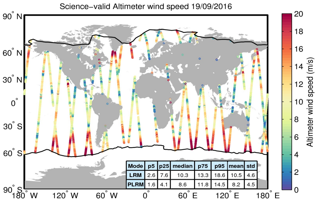
Figure 34. Geographical distribution of science-valid wind data over oceans and lakes for 19/09/2016. The statistical values shown in the table refer to the wind in m/s and are calculated separately for LRM and PLRM regions. The black lines mark the outer limit of the Arctic and Antarctic polar polygons. Gray circles denote records that have been rejected based on the editing criteria described in Table 5.
