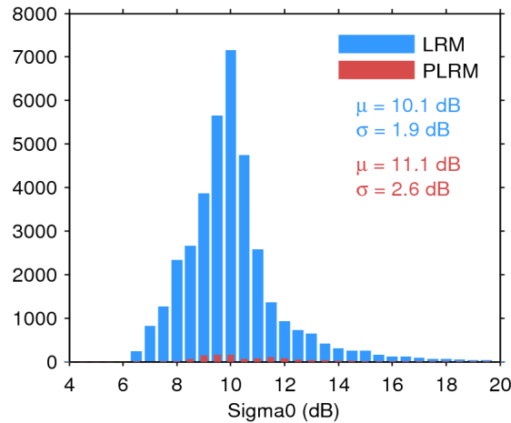
Figure 25. Histogram of flag-valid sigma0 over oceans and lakes for LRM (blue) and PLRM (red) for 19/09/2016. The mean ( \mu ) and standard deviation ( \sigma ) are also shown. Note that values outside [4 20] dB are excluded from the histogram for the sake of readability but not from the computation of \mu and \sigma .
