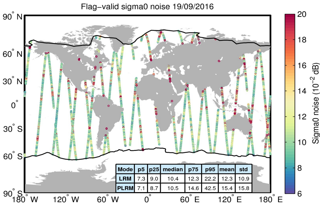
Figure 26. Geographical distribution of flag-valid 20-Hz sigma0 measurement noise over oceans and lakes for 19/09/2016. The statistical values shown in the table refer to the sigma0 noise and are calculated separately for LRM and PLRM regions. Measurements taken over polar polygons have been excluded from the computation of the statistical values. The black lines mark the outer limit of the Arctic and Antarctic polar polygons.
