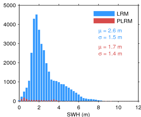
Figure 17. Histogram of flag-valid SWH over oceans and lakes for LRM (blue) and PLRM (red) for 19/09/2016. The mean ( \mu ) and standard deviation ( \sigma ) are also shown. Note that values larger than 12 m are excluded from the histogram for the sake of readability but not from the computation of \mu and \sigma .
