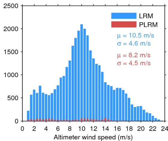
Figure 35. Histogram of science-valid wind over oceans and lakes for LRM (blue) and PLRM (red) for 19/09/2016. The mean ( \mu ) and standard deviation ( \sigma ) are also shown. Note that values larger than 24 m/s are excluded from the histogram for the sake of readability but not from the computation of \mu and \sigma .
