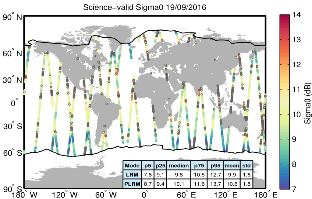
Figure 27. Geographical distribution of science-valid sigma0 data over oceans and lakes for 19/09/2016. The statistical values shown in the table refer to the sigma0 in dB and are calculated separately for LRM and PLRM regions. The black lines mark the outer limit of the Arctic and Antarctic polar polygons. Gray circles denote records that have been rejected based on the editing criteria described in Table 4.
