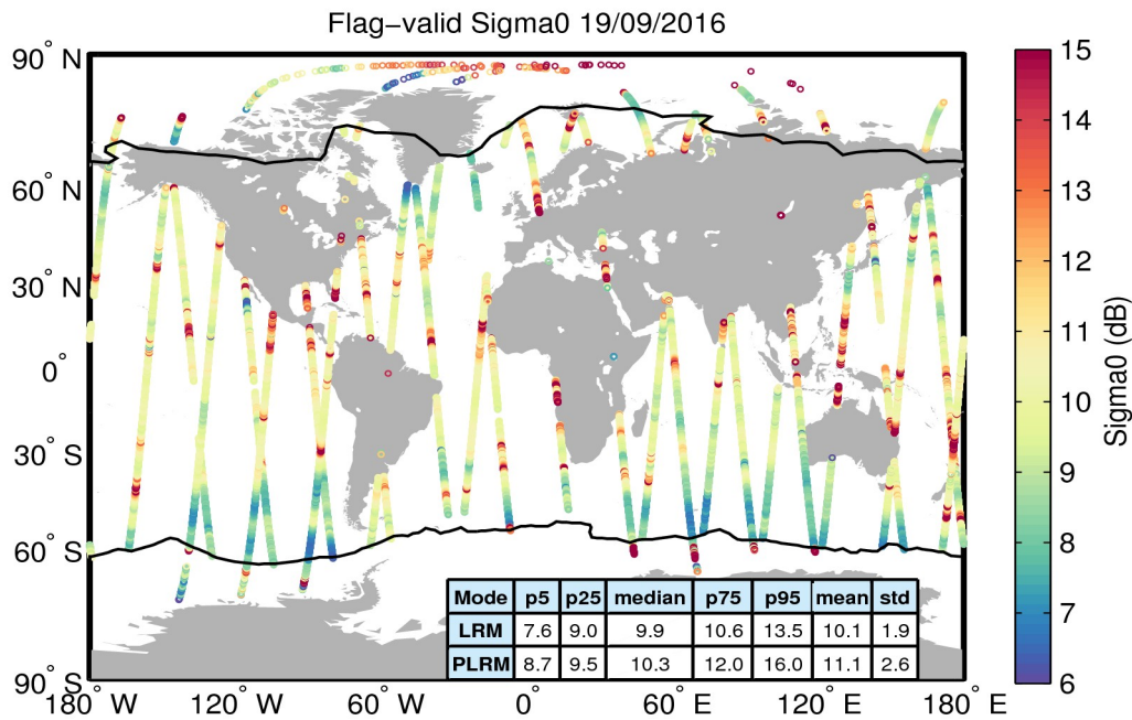
Figure 23. Geographical distribution of flag-valid sigma0 data over oceans and lakes for 19/09/2016. The statistical values shown in the table refer to the sigma0 in dB and are calculated separately for LRM and PLRM regions. Measurements taken over polar polygons have been excluded from the computation of the statistical values. The black lines mark the outer limit of the Arctic and Antarctic polar polygons.
