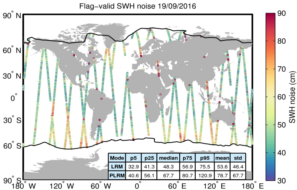
Figure 18. Geographical distribution of flag-valid 20-Hz SWH measurement noise over oceans and lakes for 19/09/2016. The statistical values shown in the table refer to the SWH noise and are calculated separately for LRM and PLRM regions. Measurements taken over polar polygons have been excluded from the computation of the statistical values. The black lines mark the outer limit of the Arctic and Antarctic polar polygons.
