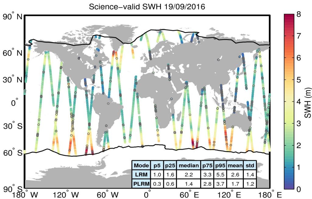
Figure 19. Geographical distribution of science-valid SWH data over oceans and lakes for 19/09/2016. The statistical values shown in the table refer to the SWH in m and are calculated separately for LRM and PLRM regions. The black lines mark the outer limit of the Arctic and Antarctic polar polygons. Gray circles denote records that have been rejected based on the editing criteria described in Table 3.
