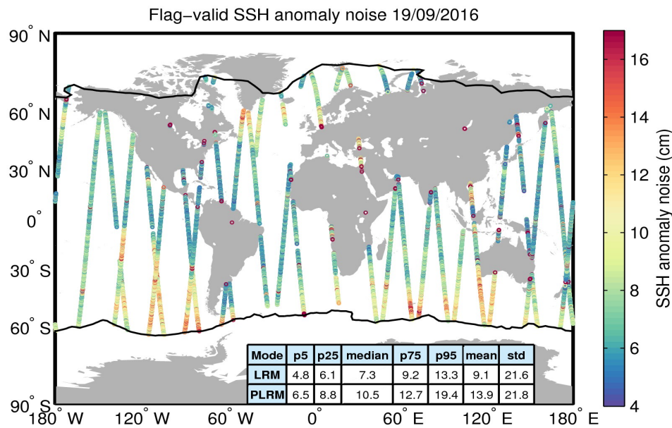
Figure 8. Geographical distribution of flag-valid 20-Hz SSH anomaly measurement noise over oceans and lakes for 19/09/2016. The statistical values shown in the table refer to the SSH anomaly noise and are calculated separately for LRM and PLRM regions. Measurements taken over polar polygons have been excluded from the computation of the statistical values. The black lines mark the outer limit of the Arctic and Antarctic polar polygons.
