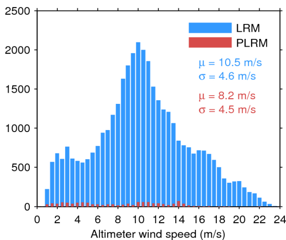
Figure 33. Histogram of flag-valid wind over oceans and lakes for LRM (blue) and PLRM (red) for 19/09/2016. The mean ( \mu ) and standard deviation ( \sigma ) are also shown. Note that values larger than 24 m/s are excluded from the histogram for the sake of readability but not from the computation of \mu and \sigma .
