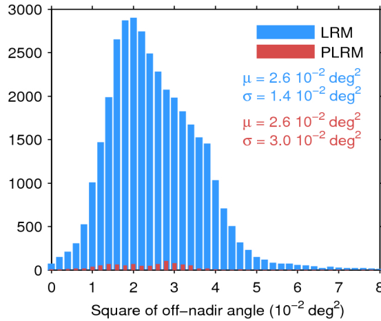
Figure 39. Histogram of flag-valid mispointing over oceans and lakes for LRM (blue) and PLRM (red) for 19/09/2016. Only positive values have been considered. The mean ( \mu ) and standard deviation ( \sigma ) are also shown. Note that values larger than 8 \cdot 10^{-2} \text{ deg}^2 are excluded from the histogram for the sake of readability but not from the computation of \mu and \sigma .
