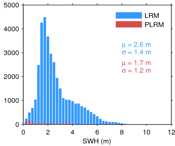
Figure 20. Histogram of science-valid SWH over oceans and lakes for LRM (blue) and PLRM (red) for 19/09/2016. The mean ( \mu ) and standard deviation ( \sigma ) are also shown. Note that values larger than 12 m are excluded from the histogram for the sake of readability but not from the computation of \mu and \sigma .
