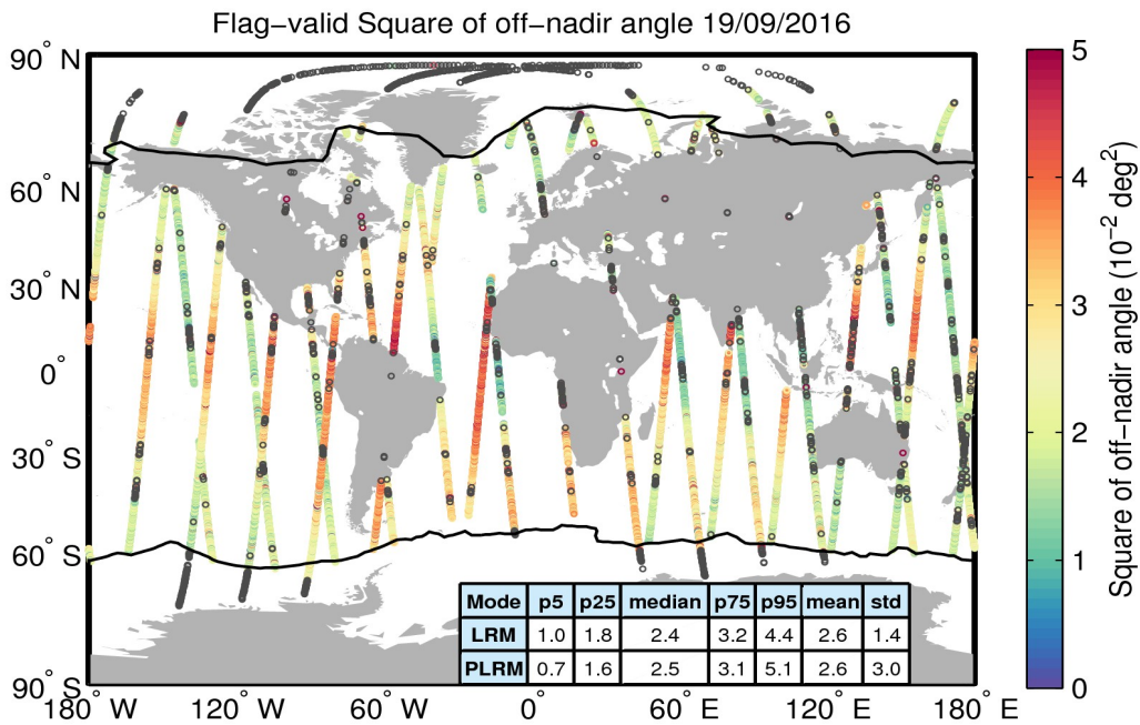
Figure 37. Geographical distribution of flag-valid mispointing data over oceans and lakes for 19/09/2016. The statistical values shown in the table refer to the mispointing in 10^{-2} deg 2 and are calculated separately for LRM and PLRM regions. Measurements taken over polar polygons have been excluded from the computation of the statistical values. The black lines mark the outer limit of the Arctic and Antarctic polar polygons. Gray circles denote negative values.
