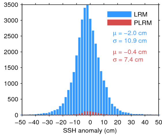
Figure 11. Histogram of science-valid SSH anomaly over oceans and lakes for LRM (blue) and PLRM (red) for 19/09/2016. The mean ( \mu ) and standard deviation ( \sigma ) are also shown. Note that values outside [-50 50] cm are excluded from the histogram for the sake of readability but not from the computation of \mu and \sigma .
