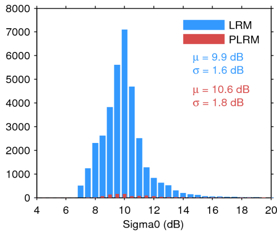
Figure 28. Histogram of science-valid sigma0 over oceans and lakes for LRM (blue) and PLRM (red) for 19/09/2016. The mean ( \mu ) and standard deviation ( \sigma ) are also shown. Note that values outside [4 20] dB are excluded from the histogram for the sake of readability but not from the computation of \mu and \sigma .
