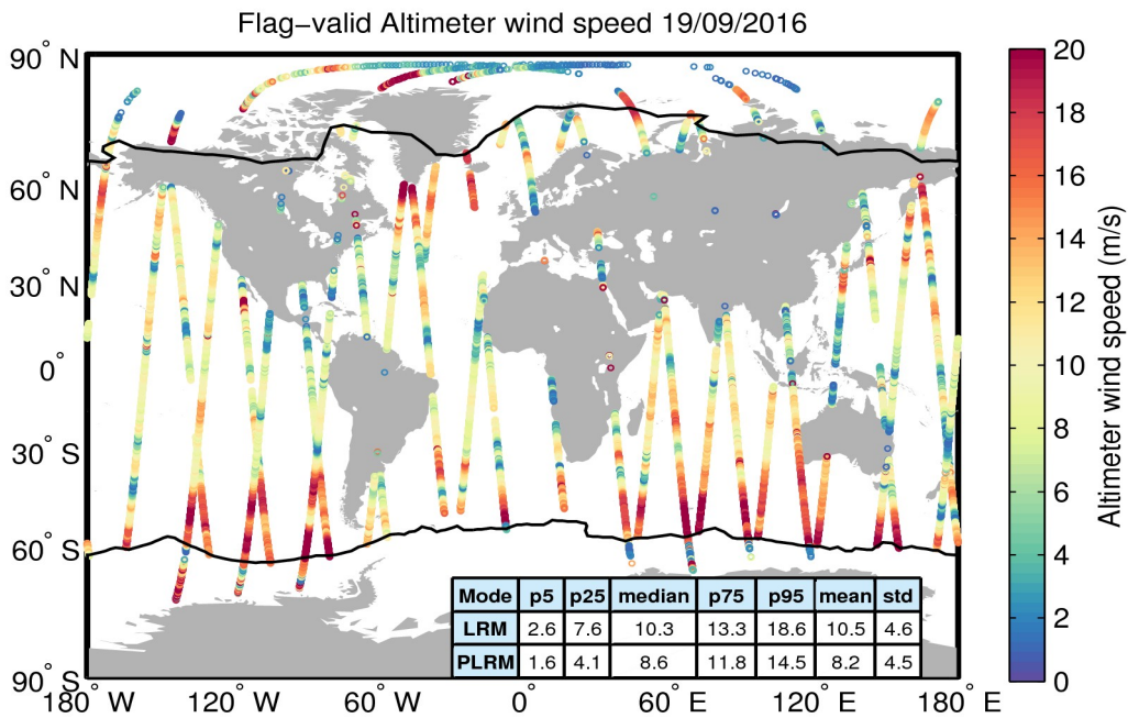
Figure 31. Geographical distribution of flag-valid wind data over oceans and lakes for 19/09/2016. The statistical values shown in the table refer to the wind in m/s and are calculated separately for LRM and PLRM regions. Measurements taken over polar polygons have been excluded from the computation of the statistical values. The black lines mark the outer limit of the Arctic and Antarctic polar polygons.
