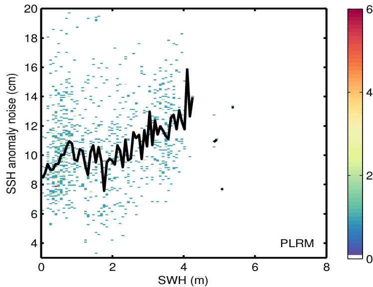
Figure 9. 2D histogram showing flag-valid SSH anomaly noise as a function of SWH for LRM (top) and PLRM (bottom) for 19/09/2016. The black line denotes the median SSH anomaly noise as a function of SWH.
