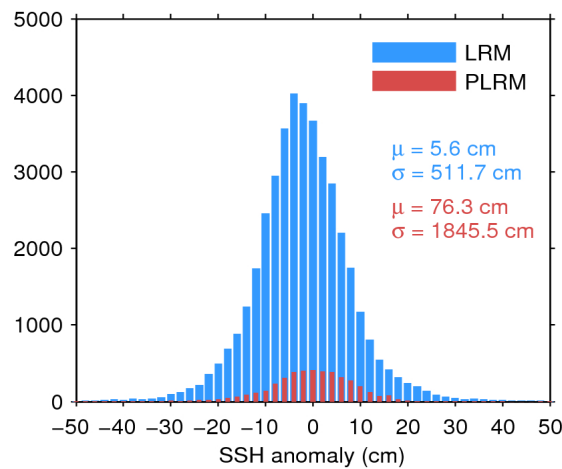
Figure 7. Histogram of flag-valid SSH anomaly over oceans and lakes for LRM (blue) and PLRM (red) for 17/09/2016. The mean ( \mu ) and standard deviation ( \sigma ) are also shown. Note that values outside [-50 \ 50] cm are excluded from the histogram for the sake of readability but not from the computation of \mu and \sigma .
