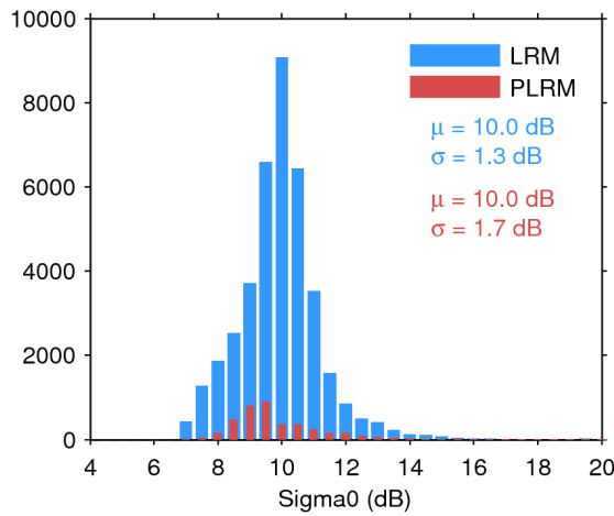
Figure 28. Histogram of science-valid sigma0 over oceans and lakes for LRM (blue) and PLRM (red) for 17/09/2016. The mean ( \mu ) and standard deviation ( \sigma ) are also shown. Note that values outside [4 20] dB are excluded from the histogram for the sake of readability but not from the computation of \mu and \sigma .
