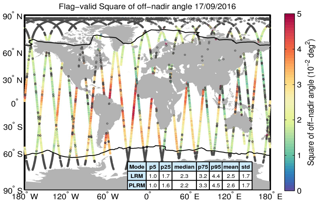
Figure 37. Geographical distribution of flag-valid mispointing data over oceans and lakes for 17/09/2016. The statistical values shown in the table refer to the mispointing in 10^{-2} deg 2 and are calculated separately for LRM and PLRM regions. Measurements taken over polar polygons have been excluded from the computation of the statistical values. The black lines mark the outer limit of the Arctic and Antarctic polar polygons. Gray circles denote negative values.
