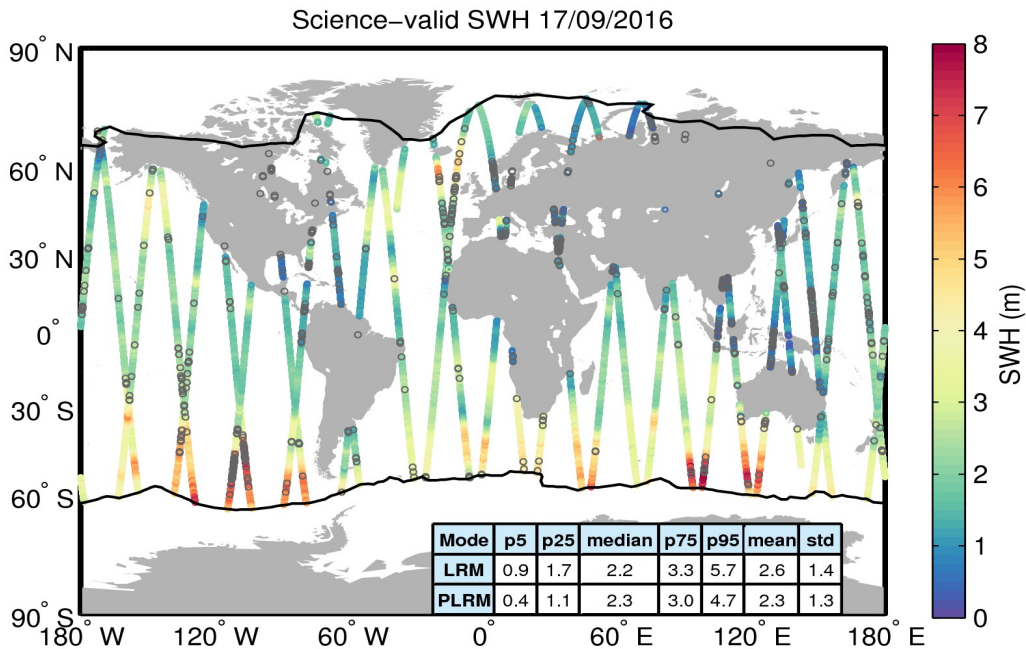
Figure 19. Geographical distribution of science-valid SWH data over oceans and lakes for 17/09/2016. The statistical values shown in the table refer to the SWH in m and are calculated separately for LRM and PLRM regions. The black lines mark the outer limit of the Arctic and Antarctic polar polygons. Gray circles denote records that have been rejected based on the editing criteria described in Table 3.
