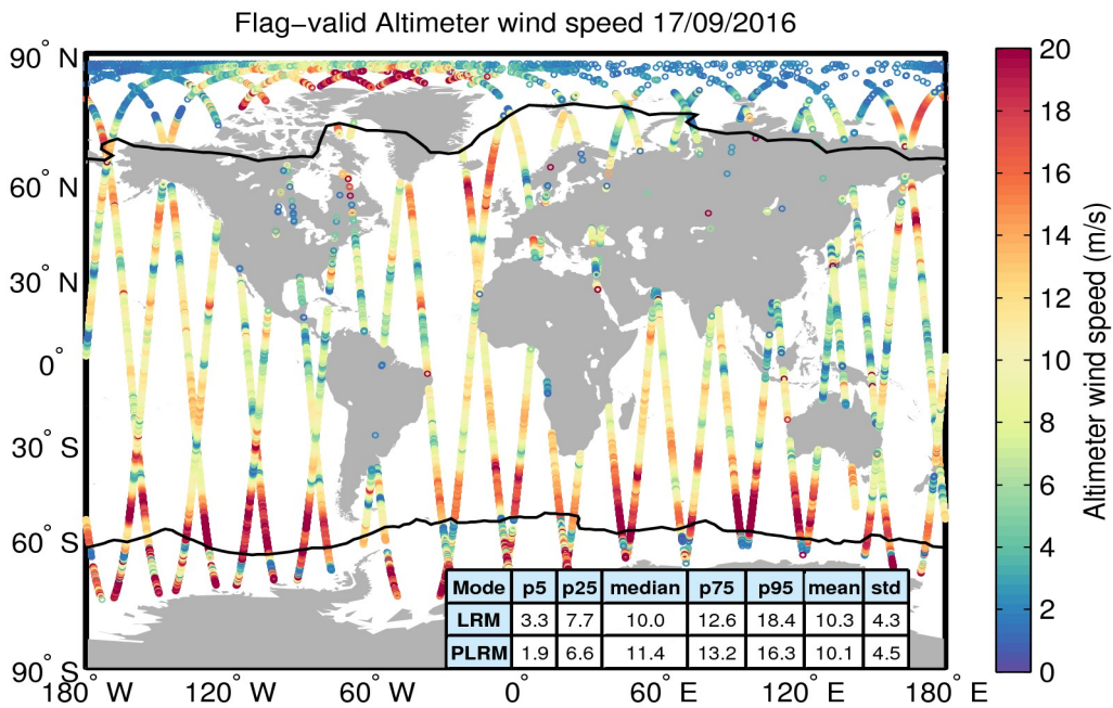
Figure 31. Geographical distribution of flag-valid wind data over oceans and lakes for 17/09/2016. The statistical values shown in the table refer to the wind in m/s and are calculated separately for LRM and PLRM regions. Measurements taken over polar polygons have been excluded from the computation of the statistical values. The black lines mark the outer limit of the Arctic and Antarctic polar polygons.
