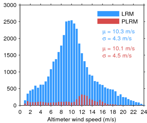
Figure 33. Histogram of flag-valid wind over oceans and lakes for LRM (blue) and PLRM (red) for 17/09/2016. The mean ( \mu ) and standard deviation ( \sigma ) are also shown. Note that values larger than 24 m/s are excluded from the histogram for the sake of readability but not from the computation of \mu and \sigma .
