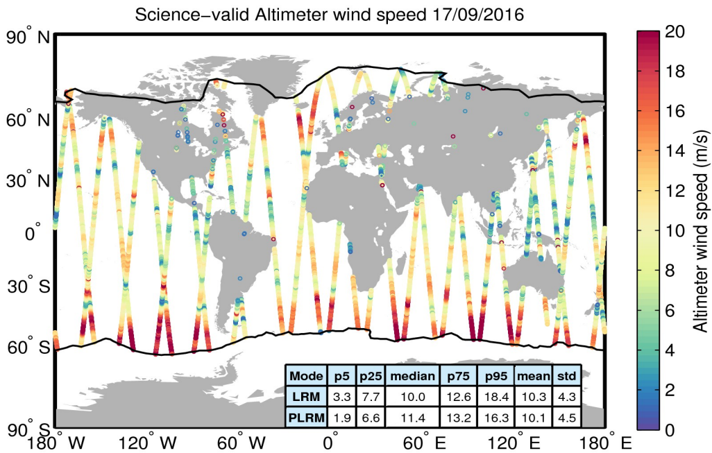
Figure 34. Geographical distribution of science-valid wind data over oceans and lakes for 17/09/2016. The statistical values shown in the table refer to the wind in m/s and are calculated separately for LRM and PLRM regions. The black lines mark the outer limit of the Arctic and Antarctic polar polygons. Gray circles denote records that have been rejected based on the editing criteria described in Table 5.
