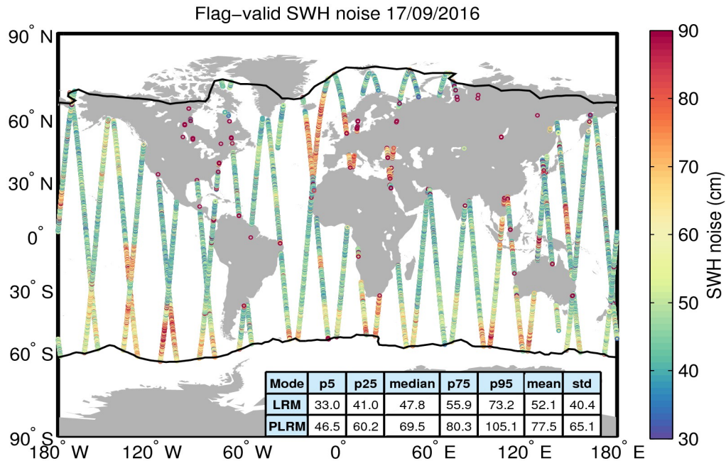
Figure 18. Geographical distribution of flag-valid 20-Hz SWH measurement noise over oceans and lakes for 17/09/2016. The statistical values shown in the table refer to the SWH noise and are calculated separately for LRM and PLRM regions. Measurements taken over polar polygons have been excluded from the computation of the statistical values. The black lines mark the outer limit of the Arctic and Antarctic polar polygons.
