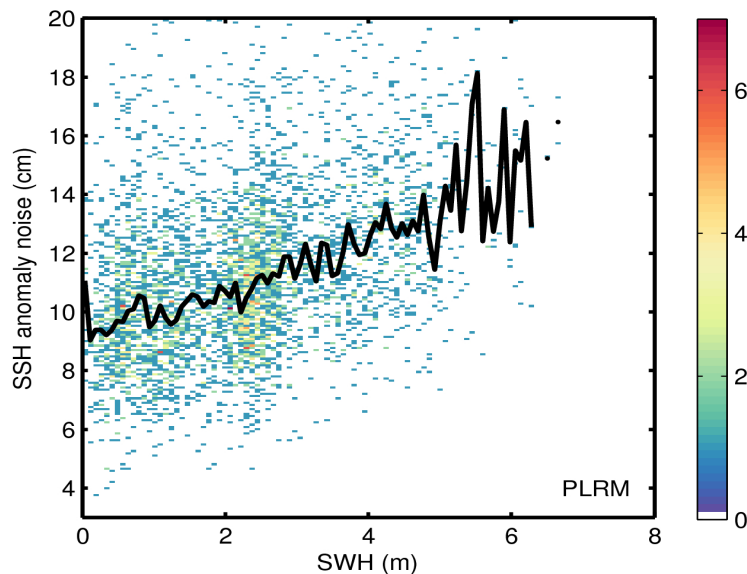
Figure 9. 2D histogram showing flag-valid SSH anomaly noise as a function of SWH for LRM (top) and PLRM (bottom) for 17/09/2016. The black line denotes the median SSH anomaly noise as a function of SWH.
