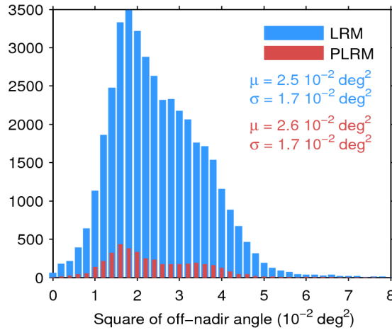
Figure 39. Histogram of flag-valid mispointing over oceans and lakes for LRM (blue) and PLRM (red) for 17/09/2016. Only positive values have been considered. The mean ( \mu ) and standard deviation ( \sigma ) are also shown. Note that values larger than 8 \cdot 10^{-2} \text{ deg}^2 are excluded from the histogram for the sake of readability but not from the computation of \mu and \sigma .
