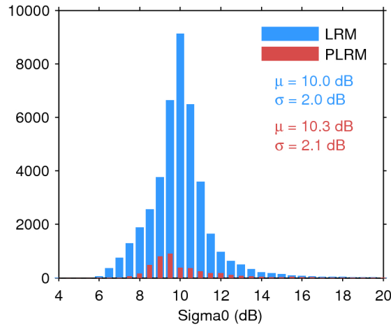
Figure 25. Histogram of flag-valid sigma0 over oceans and lakes for LRM (blue) and PLRM (red) for 17/09/2016. The mean ( \mu ) and standard deviation ( \sigma ) are also shown. Note that values outside [4 20] dB are excluded from the histogram for the sake of readability but not from the computation of \mu and \sigma .
