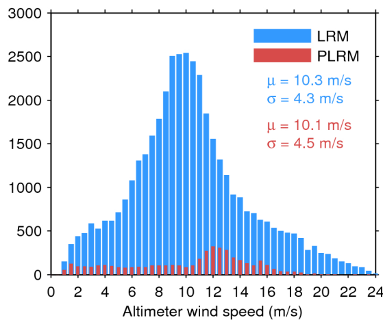
Figure 35. Histogram of science-valid wind over oceans and lakes for LRM (blue) and PLRM (red) for 17/09/2016. The mean ( \mu ) and standard deviation ( \sigma ) are also shown. Note that values larger than 24 m/s are excluded from the histogram for the sake of readability but not from the computation of \mu and \sigma .
