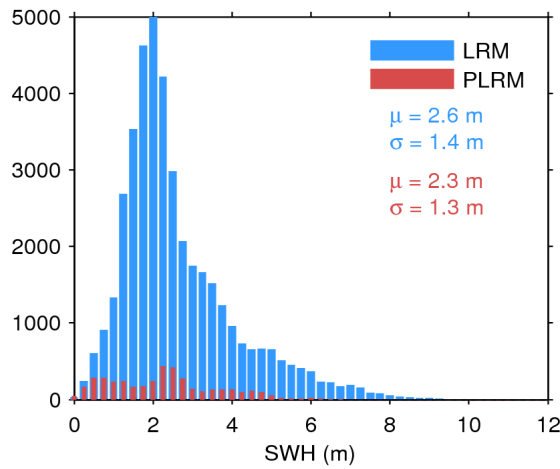
Figure 20. Histogram of science-valid SWH over oceans and lakes for LRM (blue) and PLRM (red) for 17/09/2016. The mean ( \mu ) and standard deviation ( \sigma ) are also shown. Note that values larger than 12 m are excluded from the histogram for the sake of readability but not from the computation of \mu and \sigma .
