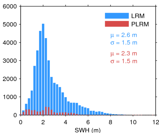
Figure 17. Histogram of flag-valid SWH over oceans and lakes for LRM (blue) and PLRM (red) for 17/09/2016. The mean ( \mu ) and standard deviation ( \sigma ) are also shown. Note that values larger than 12 m are excluded from the histogram for the sake of readability but not from the computation of \mu and \sigma .
