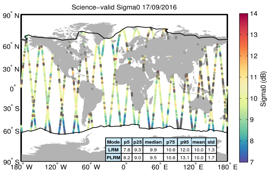
Figure 27. Geographical distribution of science-valid sigma0 data over oceans and lakes for 17/09/2016. The statistical values shown in the table refer to the sigma0 in dB and are calculated separately for LRM and PLRM regions. The black lines mark the outer limit of the Arctic and Antarctic polar polygons. Gray circles denote records that have been rejected based on the editing criteria described in Table 4.
