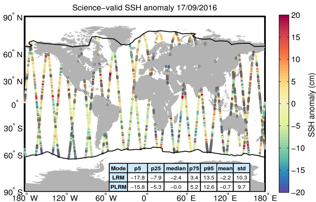
Figure 10. Geographical distribution of science-valid SSH anomaly data over oceans and lakes for 17/09/2016. The statistical values shown in the table refer to the SSH anomaly in cm and are calculated separately for LRM and PLRM regions. The black lines mark the outer limit of the Arctic and Antarctic polar polygons. Gray circles denote records that have been rejected based on the editing criteria described in Table 2.
