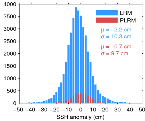
Figure 11. Histogram of science-valid SSH anomaly over oceans and lakes for LRM (blue) and PLRM (red) for 17/09/2016. The mean ( \mu ) and standard deviation ( \sigma ) are also shown. Note that values outside [-50 50] cm are excluded from the histogram for the sake of readability but not from the computation of \mu and \sigma .
