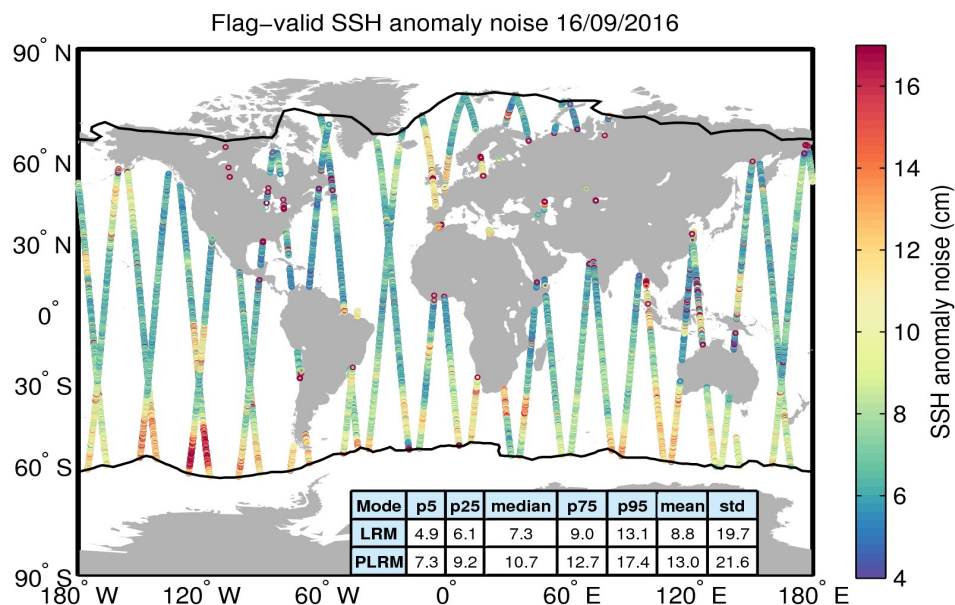
Figure 8. Geographical distribution of flag-valid 20-Hz SSH anomaly measurement noise over oceans and lakes for 16/09/2016. The statistical values shown in the table refer to the SSH anomaly noise and are calculated separately for LRM and PLRM regions. Measurements taken over polar polygons have been excluded from the computation of the statistical values. The black lines mark the outer limit of the Arctic and Antarctic polar polygons.
