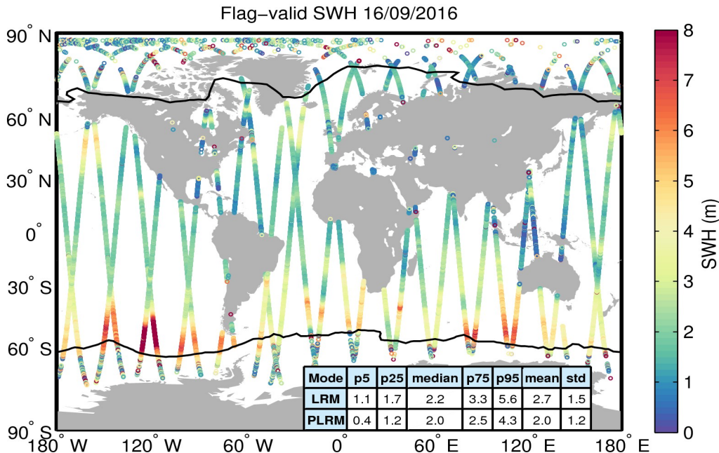
Figure 15. Geographical distribution of flag-valid SWH data over oceans and lakes for 16/09/2016. The statistical values shown in the table refer to the SWH in m and are calculated separately for LRM and PLRM regions. Measurements taken over polar polygons have been excluded from the computation of the statistical values. The black lines mark the outer limit of the Arctic and Antarctic polar polygons.
