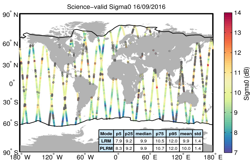
Figure 27. Geographical distribution of science-valid sigma0 data over oceans and lakes for 16/09/2016. The statistical values shown in the table refer to the sigma0 in dB and are calculated separately for LRM and PLRM regions. The black lines mark the outer limit of the Arctic and Antarctic polar polygons. Gray circles denote records that have been rejected based on the editing criteria described in Table 4.
