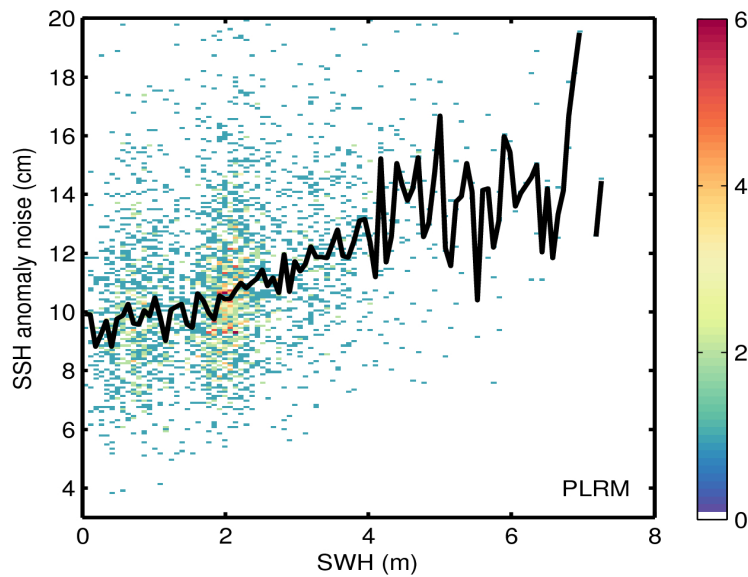
Figure 9. 2D histogram showing flag-valid SSH anomaly noise as a function of SWH for LRM (top) and PLRM (bottom) for 16/09/2016. The black line denotes the median SSH anomaly noise as a function of SWH.
