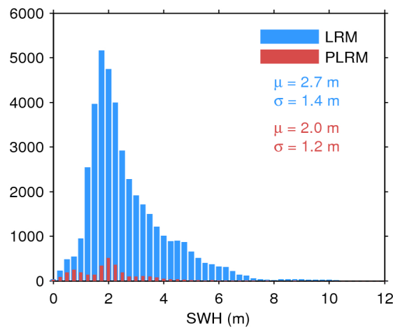
Figure 20. Histogram of science-valid SWH over oceans and lakes for LRM (blue) and PLRM (red) for 16/09/2016. The mean ( \mu ) and standard deviation ( \sigma ) are also shown. Note that values larger than 12 m are excluded from the histogram for the sake of readability but not from the computation of \mu and \sigma .
