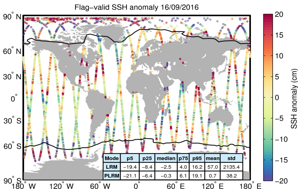
Figure 5. Geographical distribution of flag-valid 1-Hz SSH anomaly data over oceans and lakes for 16/09/2016. The statistical values shown in the table refer to the SSH anomaly in cm and are calculated separately for LRM and PLRM regions. Measurements taken over polar polygons have been excluded from the computation of the statistical values. The black lines mark the outer limit of the Arctic and Antarctic polar polygons.
