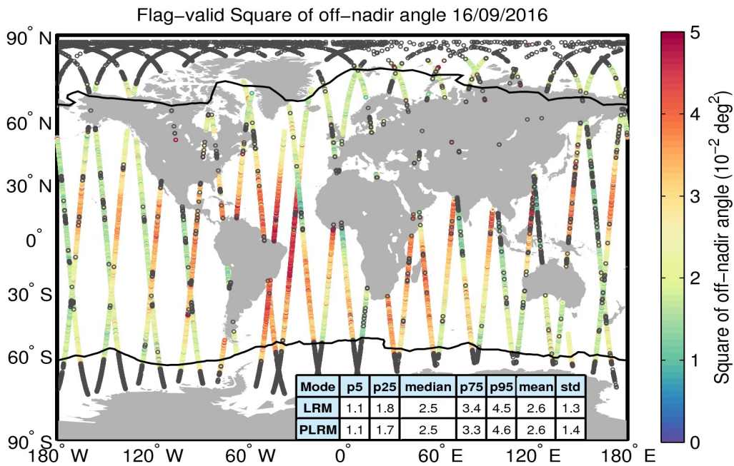
Figure 37. Geographical distribution of flag-valid mispointing data over oceans and lakes for 16/09/2016. The statistical values shown in the table refer to the mispointing in 10^{-2} deg 2 and are calculated separately for LRM and PLRM regions. Measurements taken over polar polygons have been excluded from the computation of the statistical values. The black lines mark the outer limit of the Arctic and Antarctic polar polygons. Gray circles denote negative values.
