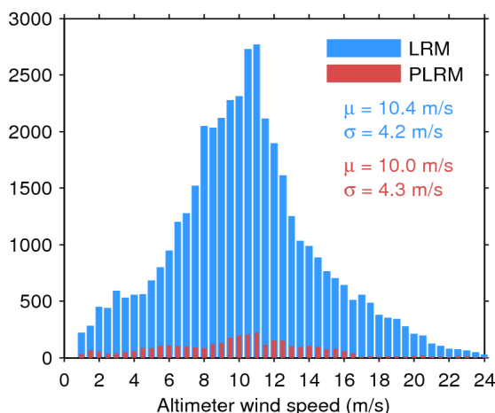
Figure 33. Histogram of flag-valid wind over oceans and lakes for LRM (blue) and PLRM (red) for 16/09/2016. The mean ( \mu ) and standard deviation ( \sigma ) are also shown. Note that values larger than 24 m/s are excluded from the histogram for the sake of readability but not from the computation of \mu and \sigma .
