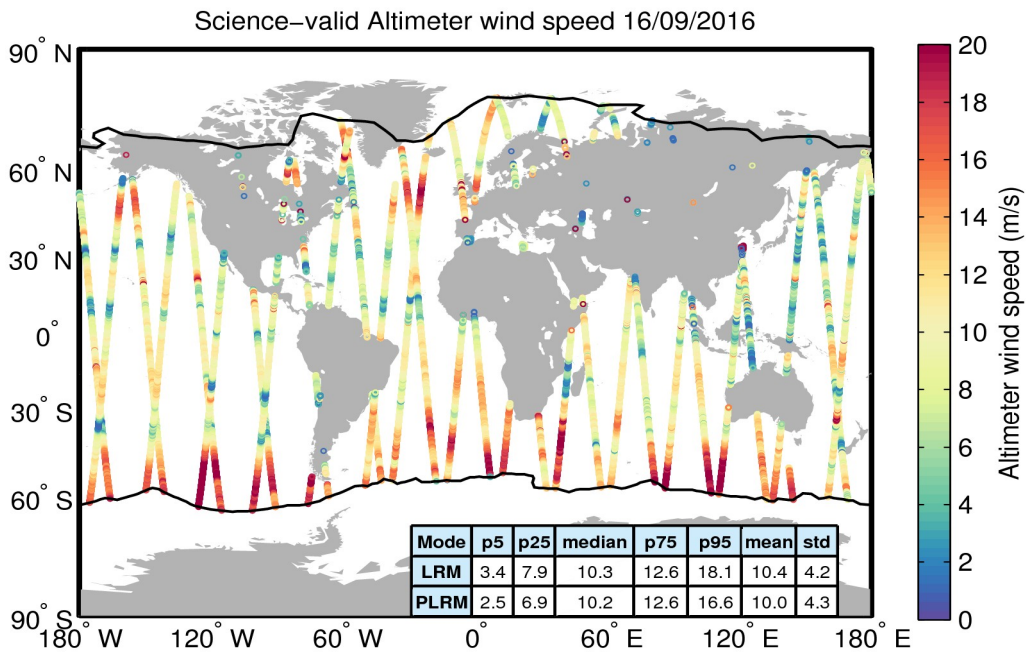
Figure 34. Geographical distribution of science-valid wind data over oceans and lakes for 16/09/2016. The statistical values shown in the table refer to the wind in m/s and are calculated separately for LRM and PLRM regions. The black lines mark the outer limit of the Arctic and Antarctic polar polygons. Gray circles denote records that have been rejected based on the editing criteria described in Table 5.
