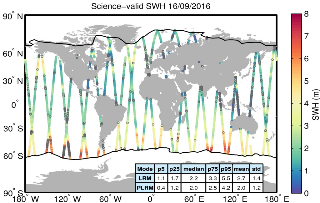
Figure 19. Geographical distribution of science-valid SWH data over oceans and lakes for 16/09/2016. The statistical values shown in the table refer to the SWH in m and are calculated separately for LRM and PLRM regions. The black lines mark the outer limit of the Arctic and Antarctic polar polygons. Gray circles denote records that have been rejected based on the editing criteria described in Table 3.
