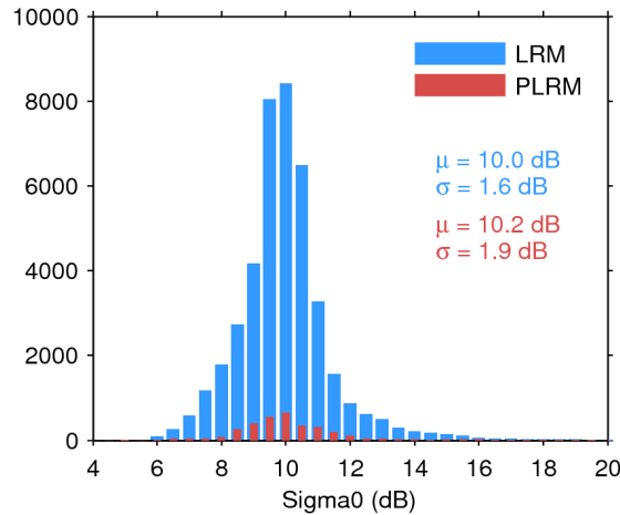
Figure 25. Histogram of flag-valid sigma0 over oceans and lakes for LRM (blue) and PLRM (red) for 16/09/2016. The mean ( \mu ) and standard deviation ( \sigma ) are also shown. Note that values outside [4 20] dB are excluded from the histogram for the sake of readability but not from the computation of \mu and \sigma .
