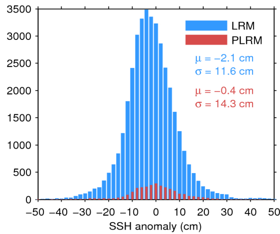
Figure 11. Histogram of science-valid SSH anomaly over oceans and lakes for LRM (blue) and PLRM (red) for 16/09/2016. The mean ( \mu ) and standard deviation ( \sigma ) are also shown. Note that values outside [-50 50] cm are excluded from the histogram for the sake of readability but not from the computation of \mu and \sigma .
