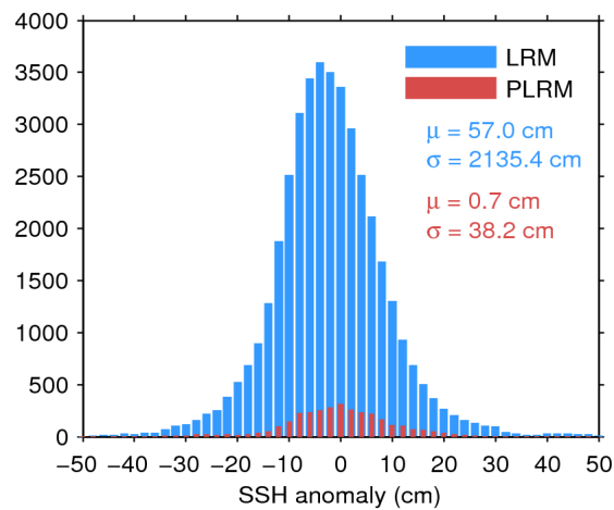
Figure 7. Histogram of flag-valid SSH anomaly over oceans and lakes for LRM (blue) and PLRM (red) for 16/09/2016. The mean ( \mu ) and standard deviation ( \sigma ) are also shown. Note that values outside [-50 \ 50] cm are excluded from the histogram for the sake of readability but not from the computation of \mu and \sigma .
