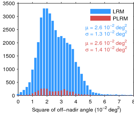
Figure 39. Histogram of flag-valid mispointing over oceans and lakes for LRM (blue) and PLRM (red) for 16/09/2016. Only positive values have been considered. The mean ( \mu ) and standard deviation ( \sigma ) are also shown. Note that values larger than 8 \cdot 10^{-2} \text{ deg}^2 are excluded from the histogram for the sake of readability but not from the computation of \mu and \sigma .
