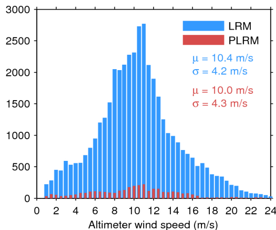
Figure 35. Histogram of science-valid wind over oceans and lakes for LRM (blue) and PLRM (red) for 16/09/2016. The mean ( \mu ) and standard deviation ( \sigma ) are also shown. Note that values larger than 24 m/s are excluded from the histogram for the sake of readability but not from the computation of \mu and \sigma .
