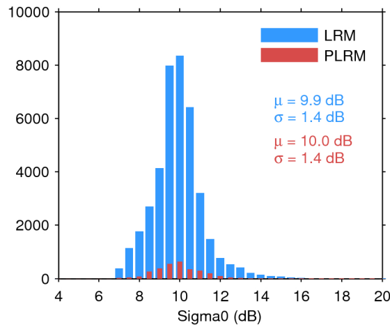
Figure 28. Histogram of science-valid sigma0 over oceans and lakes for LRM (blue) and PLRM (red) for 16/09/2016. The mean ( \mu ) and standard deviation ( \sigma ) are also shown. Note that values outside [4 20] dB are excluded from the histogram for the sake of readability but not from the computation of \mu and \sigma .
