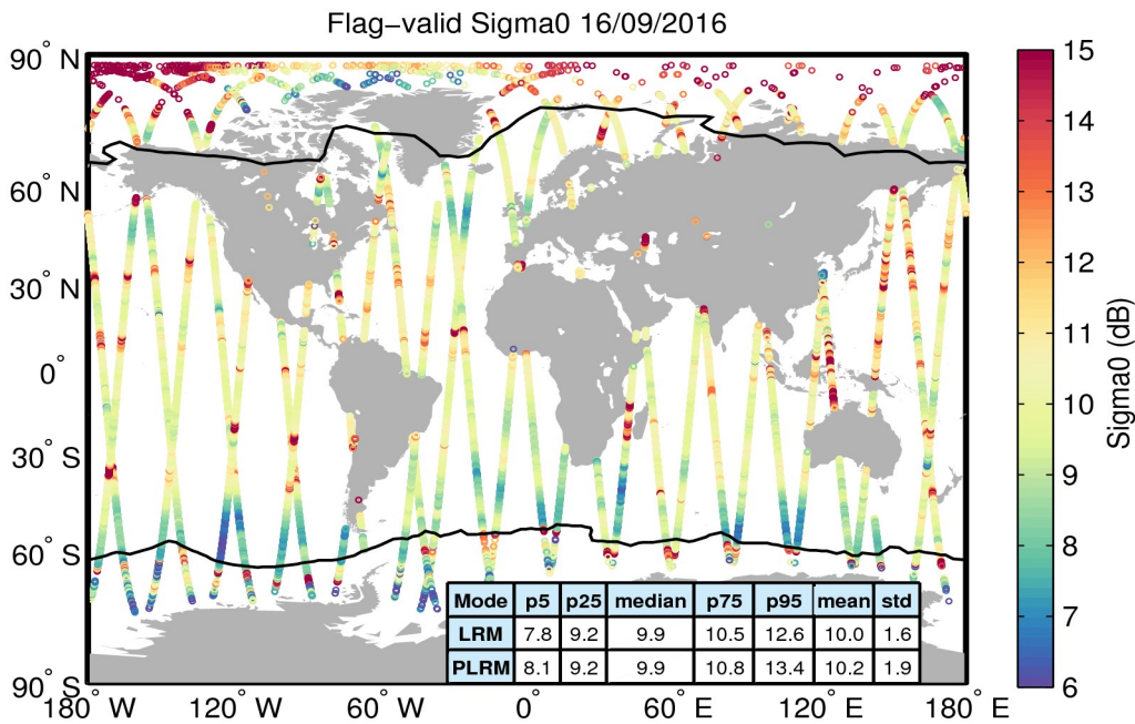
Figure 23. Geographical distribution of flag-valid sigma0 data over oceans and lakes for 16/09/2016. The statistical values shown in the table refer to the sigma0 in dB and are calculated separately for LRM and PLRM regions. Measurements taken over polar polygons have been excluded from the computation of the statistical values. The black lines mark the outer limit of the Arctic and Antarctic polar polygons.
