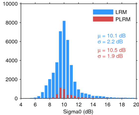
Figure 25. Histogram of flag-valid sigma0 over oceans and lakes for LRM (blue) and PLRM (red) for 15/09/2016. The mean ( \mu ) and standard deviation ( \sigma ) are also shown. Note that values outside [4 20] dB are excluded from the histogram for the sake of readability but not from the computation of \mu and \sigma .
