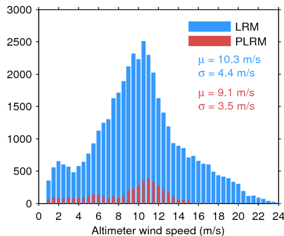
Figure 35. Histogram of science-valid wind over oceans and lakes for LRM (blue) and PLRM (red) for 15/09/2016. The mean ( \mu ) and standard deviation ( \sigma ) are also shown. Note that values larger than 24 m/s are excluded from the histogram for the sake of readability but not from the computation of \mu and \sigma .
