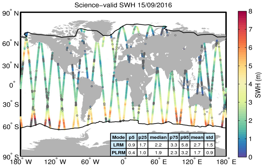
Figure 19. Geographical distribution of science-valid SWH data over oceans and lakes for 15/09/2016. The statistical values shown in the table refer to the SWH in m and are calculated separately for LRM and PLRM regions. The black lines mark the outer limit of the Arctic and Antarctic polar polygons. Gray circles denote records that have been rejected based on the editing criteria described in Table 3.
