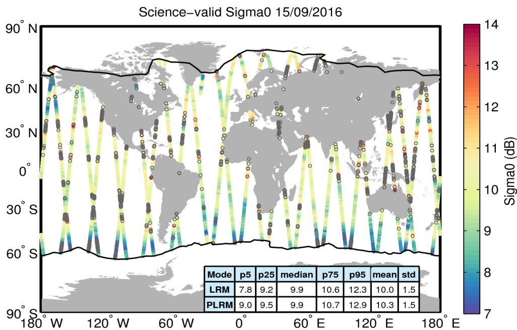
Figure 27. Geographical distribution of science-valid sigma0 data over oceans and lakes for 15/09/2016. The statistical values shown in the table refer to the sigma0 in dB and are calculated separately for LRM and PLRM regions. The black lines mark the outer limit of the Arctic and Antarctic polar polygons. Gray circles denote records that have been rejected based on the editing criteria described in Table 4.
