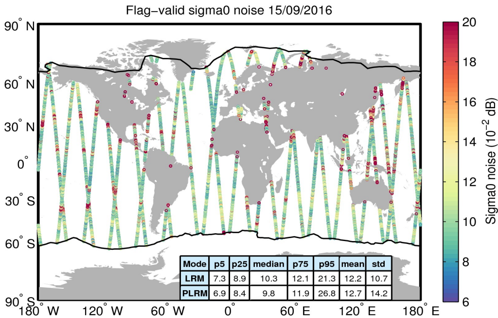
Figure 26. Geographical distribution of flag-valid 20-Hz sigma0 measurement noise over oceans and lakes for 15/09/2016. The statistical values shown in the table refer to the sigma0 noise and are calculated separately for LRM and PLRM regions. Measurements taken over polar polygons have been excluded from the computation of the statistical values. The black lines mark the outer limit of the Arctic and Antarctic polar polygons.
