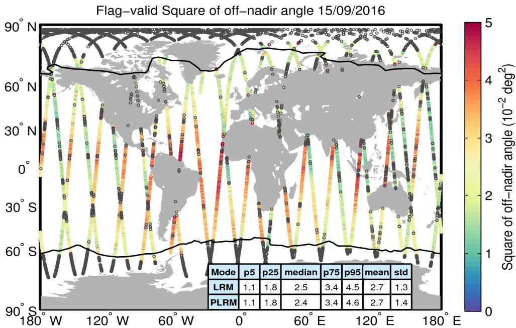
Figure 37. Geographical distribution of flag-valid mispointing data over oceans and lakes for 15/09/2016. The statistical values shown in the table refer to the mispointing in 10^{-2} deg 2 and are calculated separately for LRM and PLRM regions. Measurements taken over polar polygons have been excluded from the computation of the statistical values. The black lines mark the outer limit of the Arctic and Antarctic polar polygons. Gray circles denote negative values.
