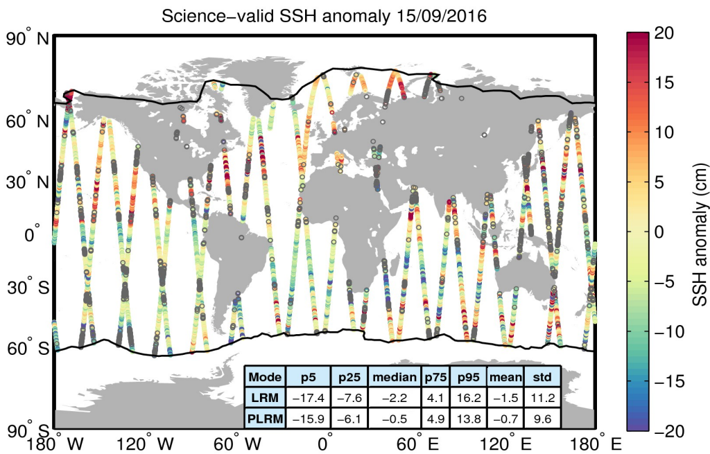
Figure 10. Geographical distribution of science-valid SSH anomaly data over oceans and lakes for 15/09/2016. The statistical values shown in the table refer to the SSH anomaly in cm and are calculated separately for LRM and PLRM regions. The black lines mark the outer limit of the Arctic and Antarctic polar polygons. Gray circles denote records that have been rejected based on the editing criteria described in Table 2.
