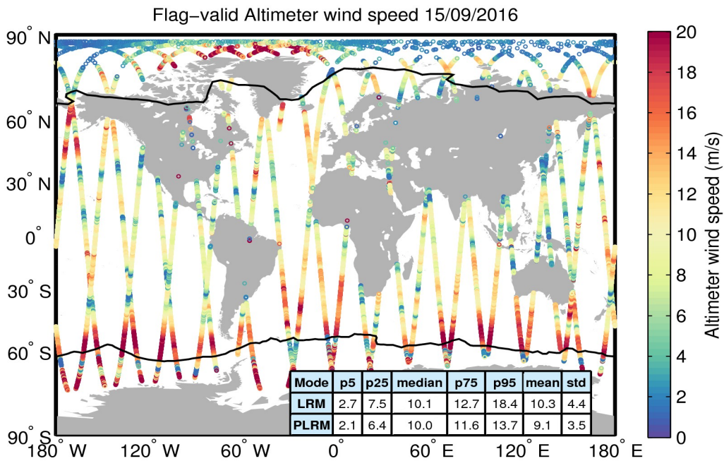
Figure 31. Geographical distribution of flag-valid wind data over oceans and lakes for 15/09/2016. The statistical values shown in the table refer to the wind in m/s and are calculated separately for LRM and PLRM regions. Measurements taken over polar polygons have been excluded from the computation of the statistical values. The black lines mark the outer limit of the Arctic and Antarctic polar polygons.
