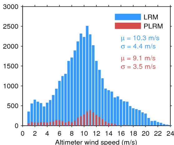
Figure 33. Histogram of flag-valid wind over oceans and lakes for LRM (blue) and PLRM (red) for 15/09/2016. The mean ( \mu ) and standard deviation ( \sigma ) are also shown. Note that values larger than 24 m/s are excluded from the histogram for the sake of readability but not from the computation of \mu and \sigma .
