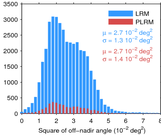
Figure 39. Histogram of flag-valid mispointing over oceans and lakes for LRM (blue) and PLRM (red) for 15/09/2016. Only positive values have been considered. The mean ( \mu ) and standard deviation ( \sigma ) are also shown. Note that values larger than 8 \cdot 10^{-2} \text{ deg}^2 are excluded from the histogram for the sake of readability but not from the computation of \mu and \sigma .
