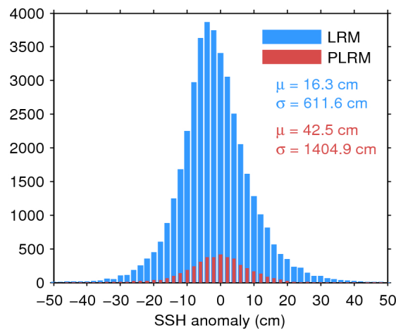
Figure 7. Histogram of flag-valid SSH anomaly over oceans and lakes for LRM (blue) and PLRM (red) for 15/09/2016. The mean ( \mu ) and standard deviation ( \sigma ) are also shown. Note that values outside [-50\ 50] cm are excluded from the histogram for the sake of readability but not from the computation of \mu and \sigma .
