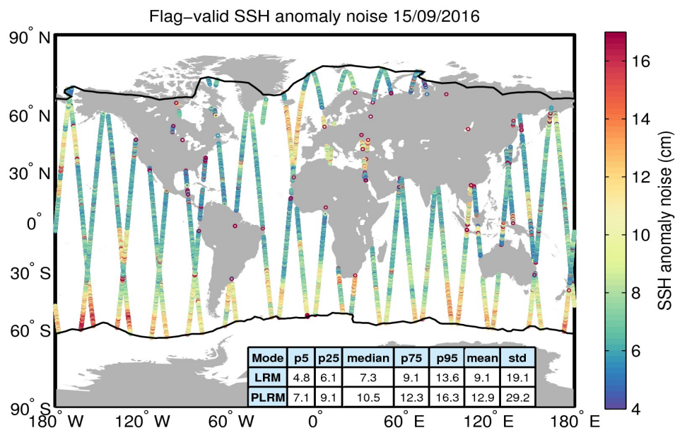
Figure 8. Geographical distribution of flag-valid 20-Hz SSH anomaly measurement noise over oceans and lakes for 15/09/2016. The statistical values shown in the table refer to the SSH anomaly noise and are calculated separately for LRM and PLRM regions. Measurements taken over polar polygons have been excluded from the computation of the statistical values. The black lines mark the outer limit of the Arctic and Antarctic polar polygons.
