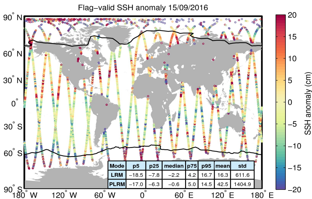
Figure 5. Geographical distribution of flag-valid 1-Hz SSH anomaly data over oceans and lakes for 15/09/2016. The statistical values shown in the table refer to the SSH anomaly in cm and are calculated separately for LRM and PLRM regions. Measurements taken over polar polygons have been excluded from the computation of the statistical values. The black lines mark the outer limit of the Arctic and Antarctic polar polygons.
