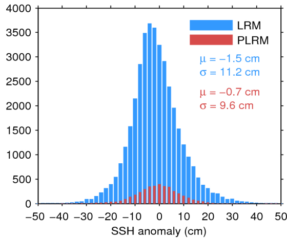
Figure 11. Histogram of science-valid SSH anomaly over oceans and lakes for LRM (blue) and PLRM (red) for 15/09/2016. The mean ( \mu ) and standard deviation ( \sigma ) are also shown. Note that values outside [-50 50] cm are excluded from the histogram for the sake of readability but not from the computation of \mu and \sigma .
