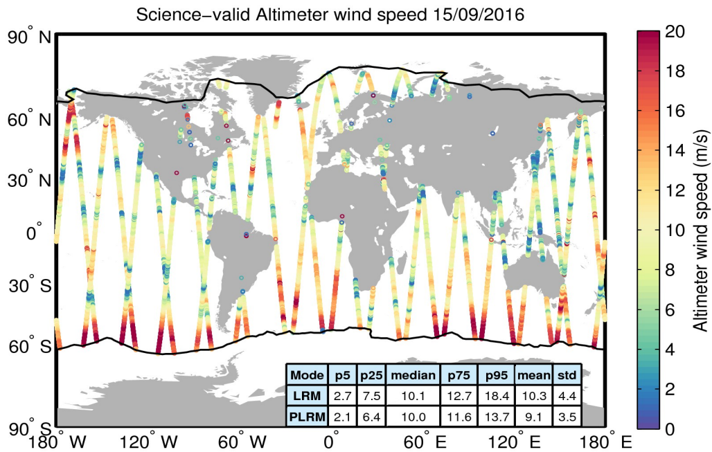
Figure 34. Geographical distribution of science-valid wind data over oceans and lakes for 15/09/2016. The statistical values shown in the table refer to the wind in m/s and are calculated separately for LRM and PLRM regions. The black lines mark the outer limit of the Arctic and Antarctic polar polygons. Gray circles denote records that have been rejected based on the editing criteria described in Table 5.
