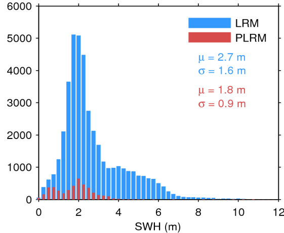
Figure 17. Histogram of flag-valid SWH over oceans and lakes for LRM (blue) and PLRM (red) for 15/09/2016. The mean ( \mu ) and standard deviation ( \sigma ) are also shown. Note that values larger than 12 m are excluded from the histogram for the sake of readability but not from the computation of \mu and \sigma .
