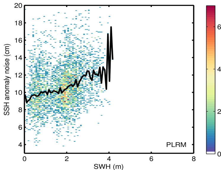
Figure 9. 2D histogram showing flag-valid SSH anomaly noise as a function of SWH for LRM (top) and PLRM (bottom) for 15/09/2016. The black line denotes the median SSH anomaly noise as a function of SWH.
