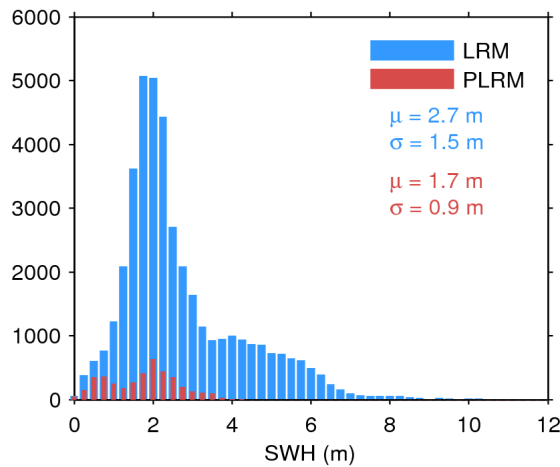
Figure 20. Histogram of science-valid SWH over oceans and lakes for LRM (blue) and PLRM (red) for 15/09/2016. The mean ( \mu ) and standard deviation ( \sigma ) are also shown. Note that values larger than 12 m are excluded from the histogram for the sake of readability but not from the computation of \mu and \sigma .
