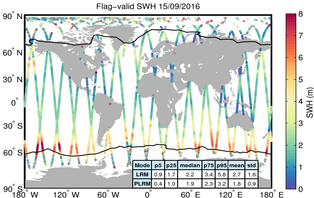
Figure 15. Geographical distribution of flag-valid SWH data over oceans and lakes for 15/09/2016. The statistical values shown in the table refer to the SWH in m and are calculated separately for LRM and PLRM regions. Measurements taken over polar polygons have been excluded from the computation of the statistical values. The black lines mark the outer limit of the Arctic and Antarctic polar polygons.
