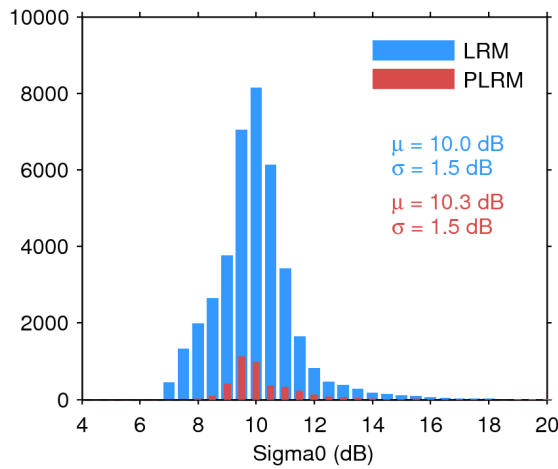
Figure 28. Histogram of science-valid sigma0 over oceans and lakes for LRM (blue) and PLRM (red) for 15/09/2016. The mean ( \mu ) and standard deviation ( \sigma ) are also shown. Note that values outside [4 20] dB are excluded from the histogram for the sake of readability but not from the computation of \mu and \sigma .
