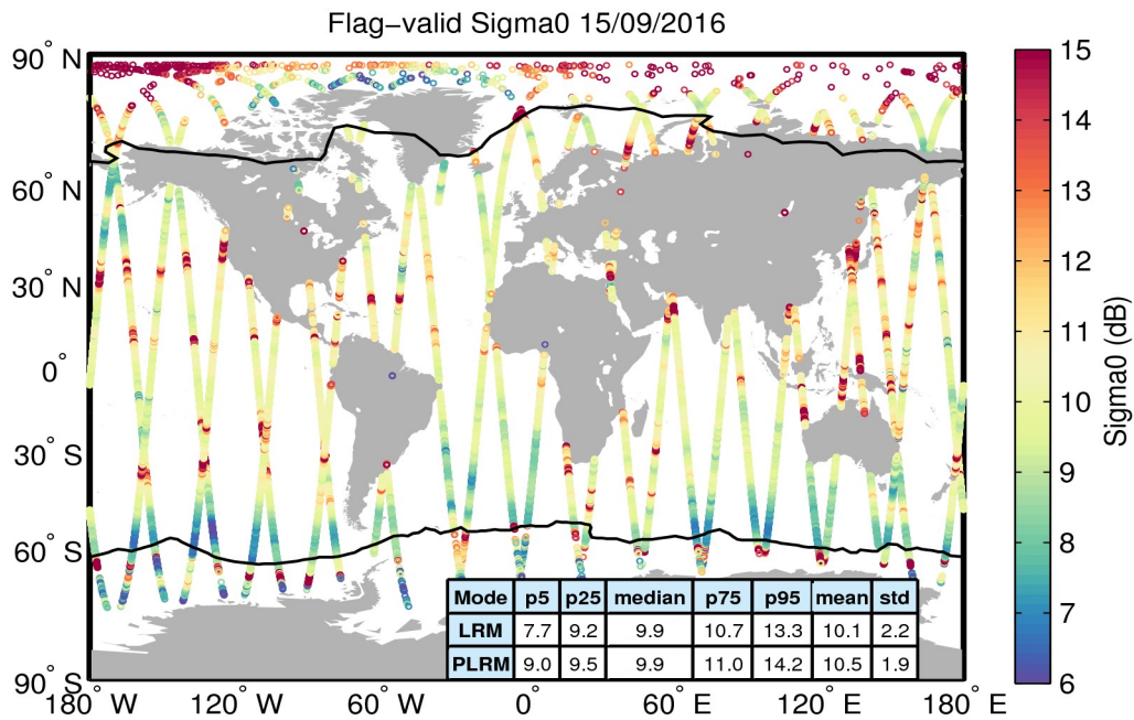
Figure 23. Geographical distribution of flag-valid sigma0 data over oceans and lakes for 15/09/2016. The statistical values shown in the table refer to the sigma0 in dB and are calculated separately for LRM and PLRM regions. Measurements taken over polar polygons have been excluded from the computation of the statistical values. The black lines mark the outer limit of the Arctic and Antarctic polar polygons.
