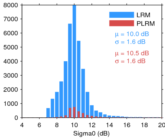
Figure 28. Histogram of science-valid sigma0 over oceans and lakes for LRM (blue) and PLRM (red) for 14/09/2016. The mean ( \mu ) and standard deviation ( \sigma ) are also shown. Note that values outside [4 20] dB are excluded from the histogram for the sake of readability but not from the computation of \mu and \sigma .
