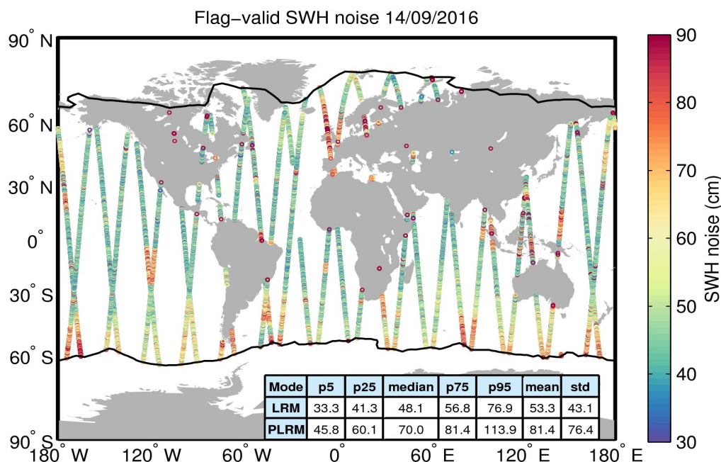
Figure 18. Geographical distribution of flag-valid 20-Hz SWH measurement noise over oceans and lakes for 14/09/2016. The statistical values shown in the table refer to the SWH noise and are calculated separately for LRM and PLRM regions. Measurements taken over polar polygons have been excluded from the computation of the statistical values. The black lines mark the outer limit of the Arctic and Antarctic polar polygons.
