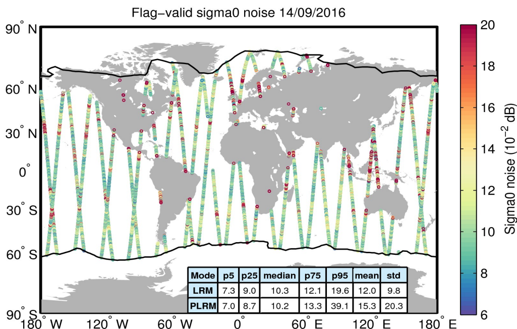
Figure 26. Geographical distribution of flag-valid 20-Hz sigma0 measurement noise over oceans and lakes for 14/09/2016. The statistical values shown in the table refer to the sigma0 noise and are calculated separately for LRM and PLRM regions. Measurements taken over polar polygons have been excluded from the computation of the statistical values. The black lines mark the outer limit of the Arctic and Antarctic polar polygons.
