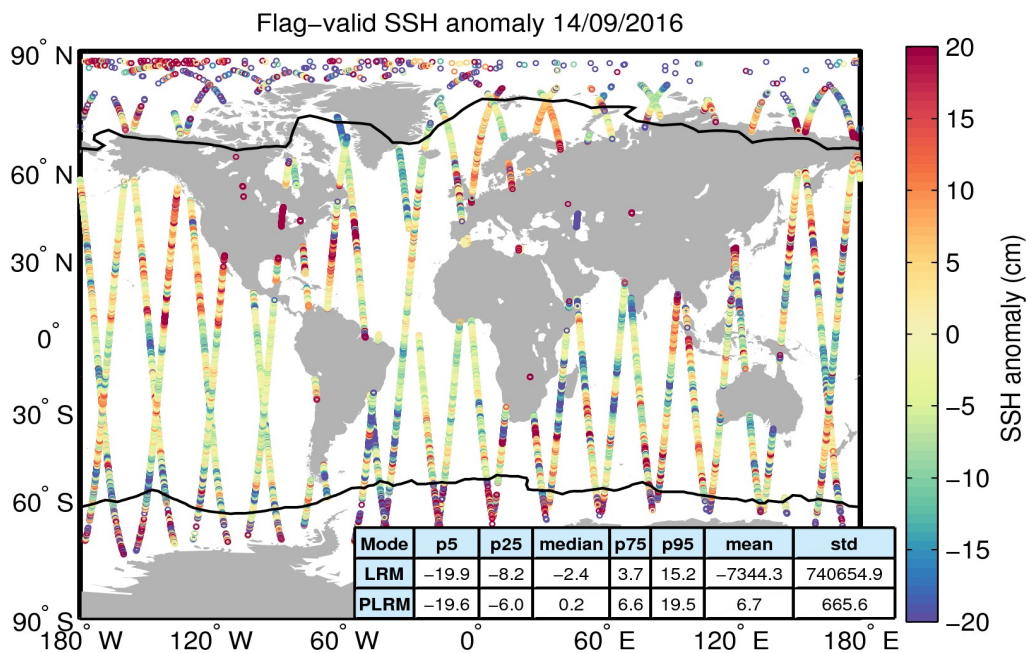
Figure 5. Geographical distribution of flag-valid 1-Hz SSH anomaly data over oceans and lakes for 14/09/2016. The statistical values shown in the table refer to the SSH anomaly in cm and are calculated separately for LRM and PLRM regions. Measurements taken over polar polygons have been excluded from the computation of the statistical values. The black lines mark the outer limit of the Arctic and Antarctic polar polygons.
