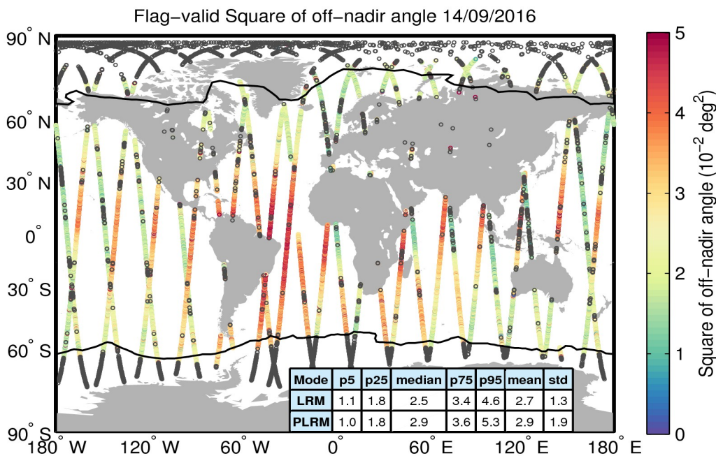
Figure 37. Geographical distribution of flag-valid mispointing data over oceans and lakes for 14/09/2016. The statistical values shown in the table refer to the mispointing in 10^{-2} deg 2 and are calculated separately for LRM and PLRM regions. Measurements taken over polar polygons have been excluded from the computation of the statistical values. The black lines mark the outer limit of the Arctic and Antarctic polar polygons. Gray circles denote negative values.
