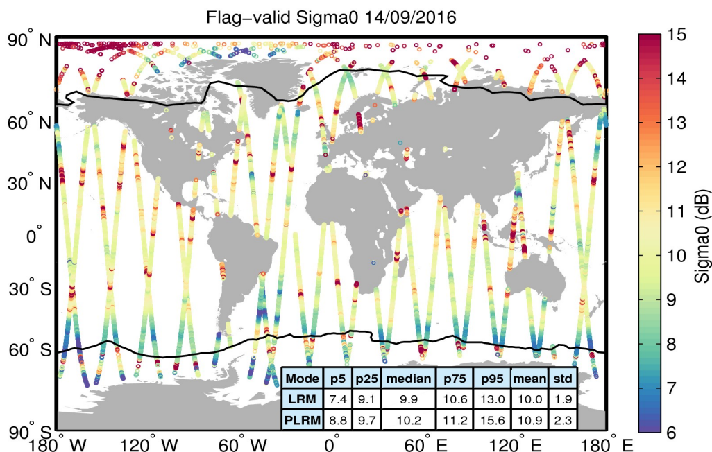
Figure 23. Geographical distribution of flag-valid sigma0 data over oceans and lakes for 14/09/2016. The statistical values shown in the table refer to the sigma0 in dB and are calculated separately for LRM and PLRM regions. Measurements taken over polar polygons have been excluded from the computation of the statistical values. The black lines mark the outer limit of the Arctic and Antarctic polar polygons.
