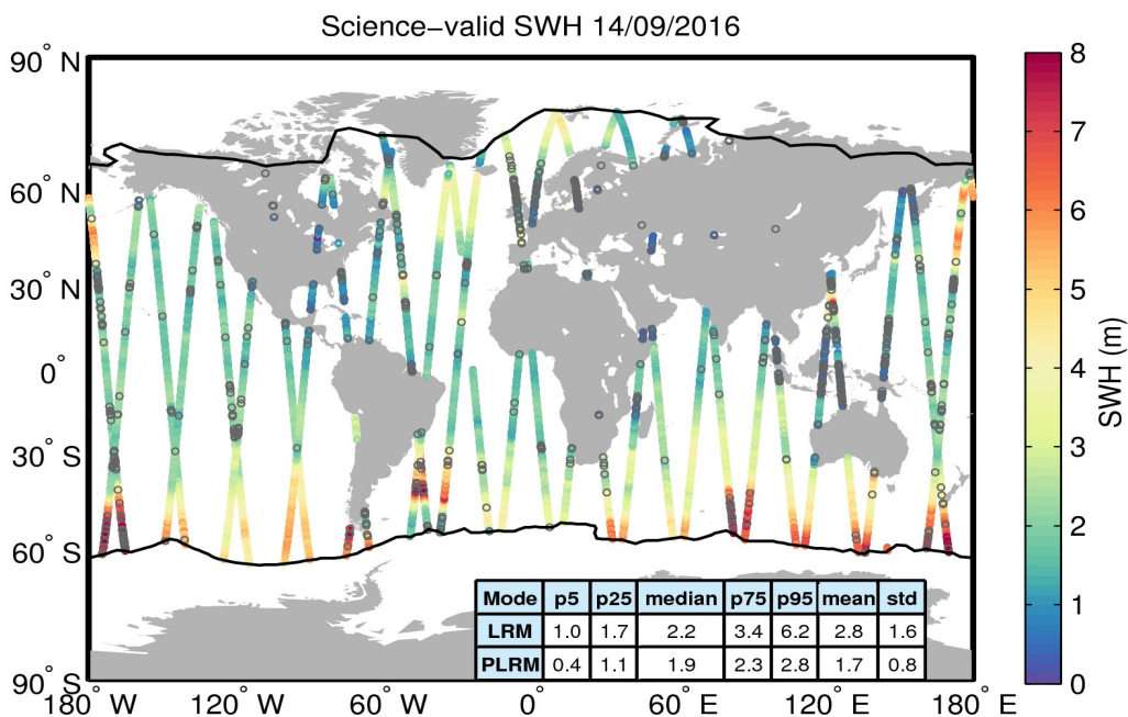
Figure 19. Geographical distribution of science-valid SWH data over oceans and lakes for 14/09/2016. The statistical values shown in the table refer to the SWH in m and are calculated separately for LRM and PLRM regions. The black lines mark the outer limit of the Arctic and Antarctic polar polygons. Gray circles denote records that have been rejected based on the editing criteria described in Table 3.
