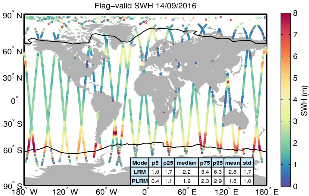
Figure 15. Geographical distribution of flag-valid SWH data over oceans and lakes for 14/09/2016. The statistical values shown in the table refer to the SWH in m and are calculated separately for LRM and PLRM regions. Measurements taken over polar polygons have been excluded from the computation of the statistical values. The black lines mark the outer limit of the Arctic and Antarctic polar polygons.
