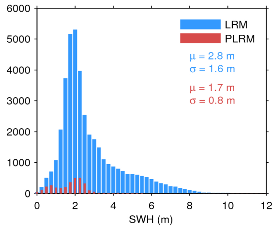
Figure 20. Histogram of science-valid SWH over oceans and lakes for LRM (blue) and PLRM (red) for 14/09/2016. The mean ( \mu ) and standard deviation ( \sigma ) are also shown. Note that values larger than 12 m are excluded from the histogram for the sake of readability but not from the computation of \mu and \sigma .
