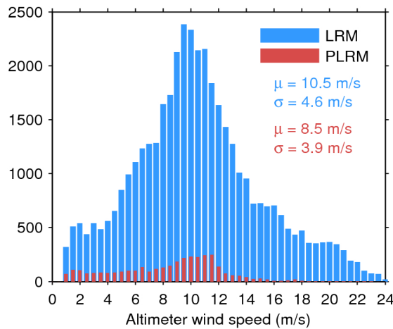
Figure 33. Histogram of flag-valid wind over oceans and lakes for LRM (blue) and PLRM (red) for 14/09/2016. The mean ( \mu ) and standard deviation ( \sigma ) are also shown. Note that values larger than 24 m/s are excluded from the histogram for the sake of readability but not from the computation of \mu and \sigma .
