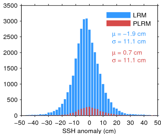
Figure 11. Histogram of science-valid SSH anomaly over oceans and lakes for LRM (blue) and PLRM (red) for 14/09/2016. The mean ( \mu ) and standard deviation ( \sigma ) are also shown. Note that values outside [-50 50] cm are excluded from the histogram for the sake of readability but not from the computation of \mu and \sigma .
