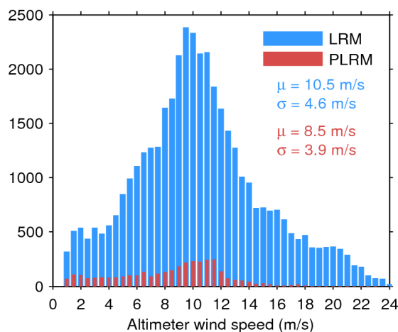
Figure 35. Histogram of science-valid wind over oceans and lakes for LRM (blue) and PLRM (red) for 14/09/2016. The mean ( \mu ) and standard deviation ( \sigma ) are also shown. Note that values larger than 24 m/s are excluded from the histogram for the sake of readability but not from the computation of \mu and \sigma .
