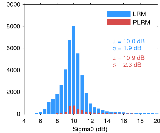
Figure 25. Histogram of flag-valid sigma0 over oceans and lakes for LRM (blue) and PLRM (red) for 14/09/2016. The mean ( \mu ) and standard deviation ( \sigma ) are also shown. Note that values outside [4 20] dB are excluded from the histogram for the sake of readability but not from the computation of \mu and \sigma .
