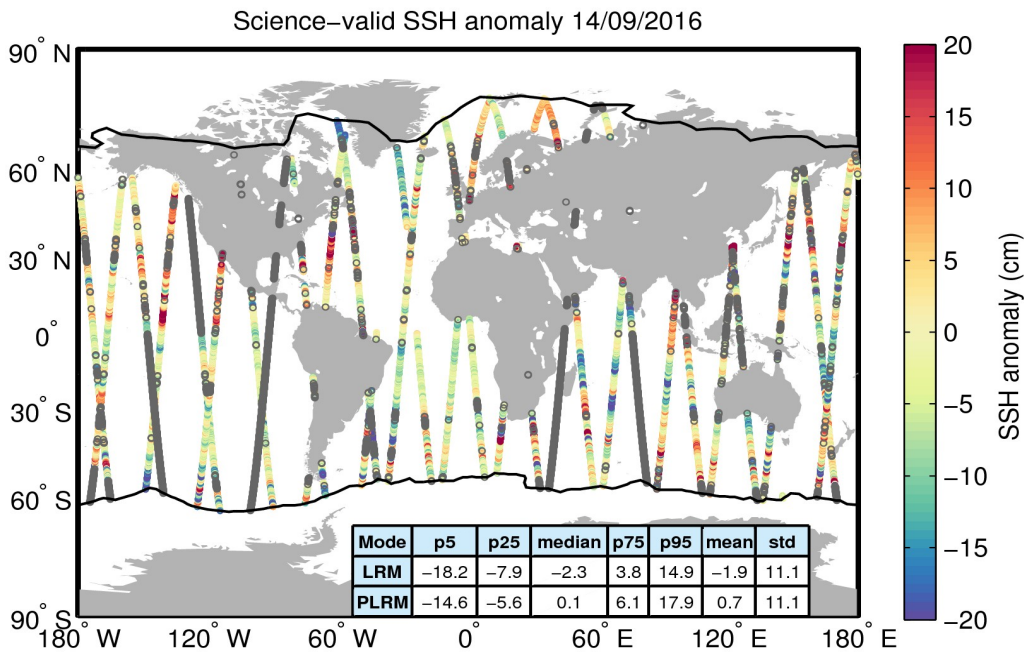
Figure 10. Geographical distribution of science-valid SSH anomaly data over oceans and lakes for 14/09/2016. The statistical values shown in the table refer to the SSH anomaly in cm and are calculated separately for LRM and PLRM regions. The black lines mark the outer limit of the Arctic and Antarctic polar polygons. Gray circles denote records that have been rejected based on the editing criteria described in Table 2.
