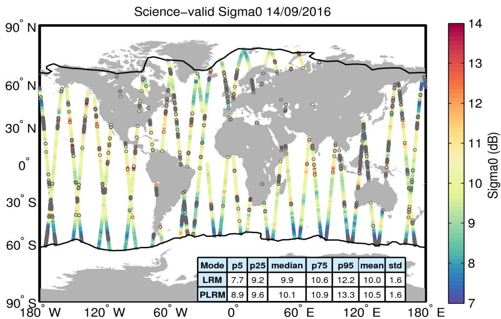
Figure 27. Geographical distribution of science-valid sigma0 data over oceans and lakes for 14/09/2016. The statistical values shown in the table refer to the sigma0 in dB and are calculated separately for LRM and PLRM regions. The black lines mark the outer limit of the Arctic and Antarctic polar polygons. Gray circles denote records that have been rejected based on the editing criteria described in Table 4.
