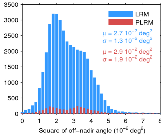
Figure 39. Histogram of flag-valid mispointing over oceans and lakes for LRM (blue) and PLRM (red) for 14/09/2016. Only positive values have been considered. The mean ( \mu ) and standard deviation ( \sigma ) are also shown. Note that values larger than 8 \cdot 10^{-2} \text{ deg}^2 are excluded from the histogram for the sake of readability but not from the computation of \mu and \sigma .
