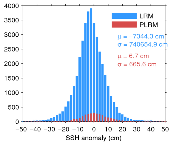
Figure 7. Histogram of flag-valid SSH anomaly over oceans and lakes for LRM (blue) and PLRM (red) for 14/09/2016. The mean ( \mu ) and standard deviation ( \sigma ) are also shown. Note that values outside [-50\ 50] cm are excluded from the histogram for the sake of readability but not from the computation of \mu and \sigma .
