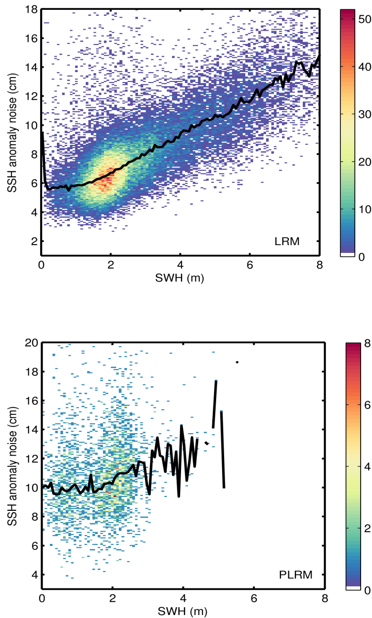
Figure 9. 2D histogram showing flag-valid SSH anomaly noise as a function of SWH for LRM (top) and PLRM (bottom) for 14/09/2016. The black line denotes the median SSH anomaly noise as a function of SWH.
