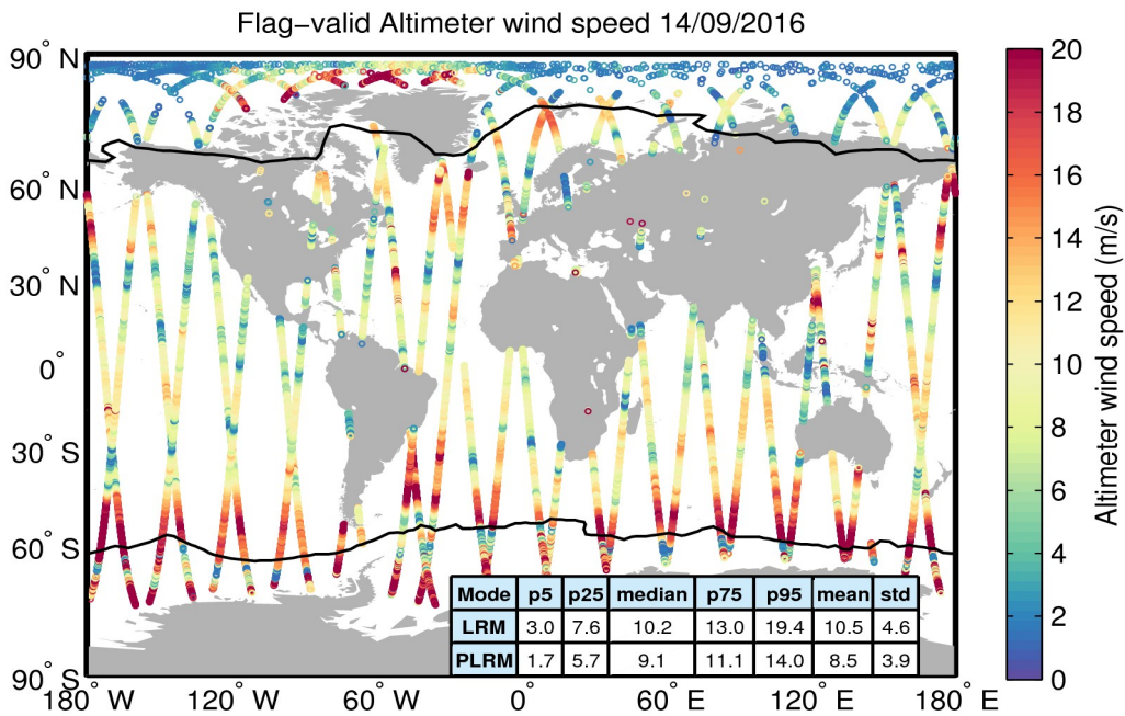
Figure 31. Geographical distribution of flag-valid wind data over oceans and lakes for 14/09/2016. The statistical values shown in the table refer to the wind in m/s and are calculated separately for LRM and PLRM regions. Measurements taken over polar polygons have been excluded from the computation of the statistical values. The black lines mark the outer limit of the Arctic and Antarctic polar polygons.
