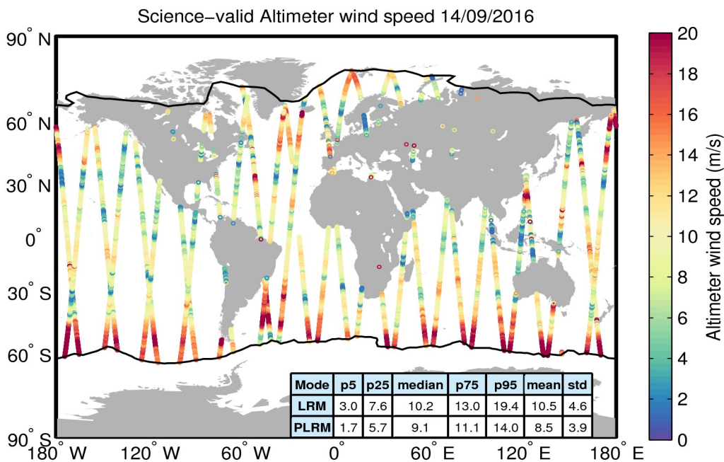
Figure 34. Geographical distribution of science-valid wind data over oceans and lakes for 14/09/2016. The statistical values shown in the table refer to the wind in m/s and are calculated separately for LRM and PLRM regions. The black lines mark the outer limit of the Arctic and Antarctic polar polygons. Gray circles denote records that have been rejected based on the editing criteria described in Table 5.
