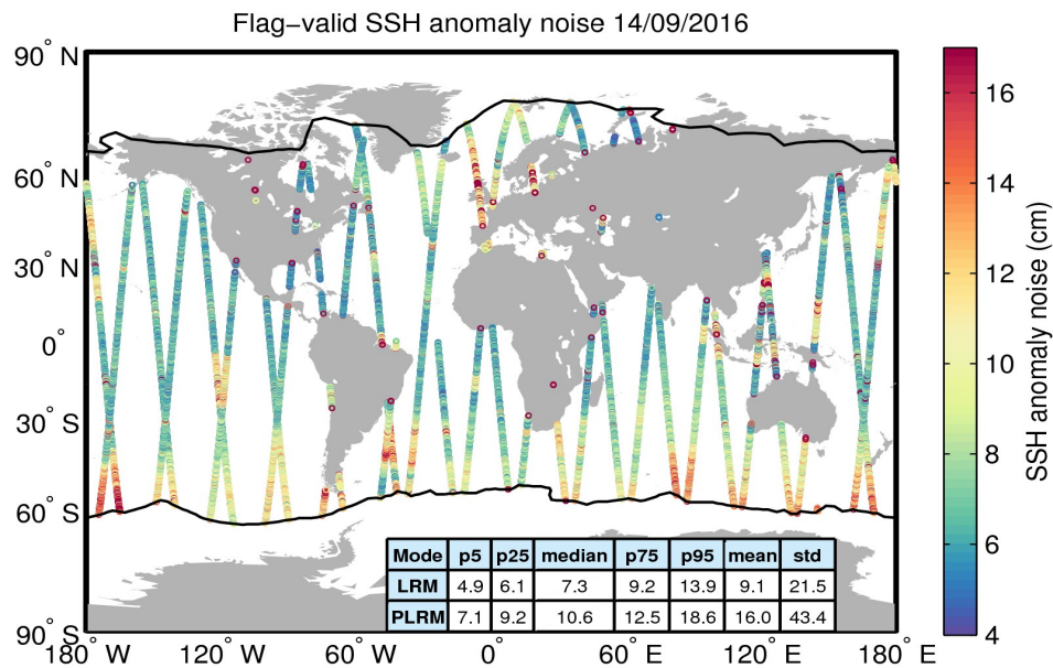
Figure 8. Geographical distribution of flag-valid 20-Hz SSH anomaly measurement noise over oceans and lakes for 14/09/2016. The statistical values shown in the table refer to the SSH anomaly noise and are calculated separately for LRM and PLRM regions. Measurements taken over polar polygons have been excluded from the computation of the statistical values. The black lines mark the outer limit of the Arctic and Antarctic polar polygons.
