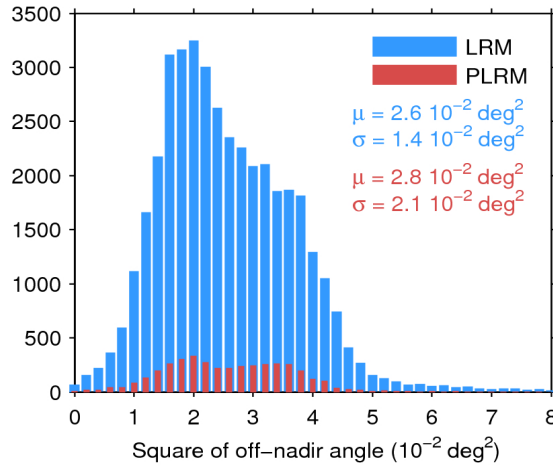
Figure 39. Histogram of flag-valid mispointing over oceans and lakes for LRM (blue) and PLRM (red) for 13/09/2016. Only positive values have been considered. The mean ( \mu ) and standard deviation ( \sigma ) are also shown. Note that values larger than 8 \cdot 10^{-2} \text{ deg}^2 are excluded from the histogram for the sake of readability but not from the computation of \mu and \sigma .
