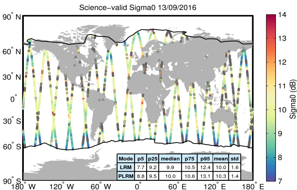
Figure 27. Geographical distribution of science-valid sigma0 data over oceans and lakes for 13/09/2016. The statistical values shown in the table refer to the sigma0 in dB and are calculated separately for LRM and PLRM regions. The black lines mark the outer limit of the Arctic and Antarctic polar polygons. Gray circles denote records that have been rejected based on the editing criteria described in Table 4.
