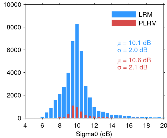
Figure 25. Histogram of flag-valid sigma0 over oceans and lakes for LRM (blue) and PLRM (red) for 13/09/2016. The mean ( \mu ) and standard deviation ( \sigma ) are also shown. Note that values outside [4 20] dB are excluded from the histogram for the sake of readability but not from the computation of \mu and \sigma .
