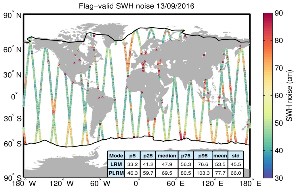
Figure 18. Geographical distribution of flag-valid 20-Hz SWH measurement noise over oceans and lakes for 13/09/2016. The statistical values shown in the table refer to the SWH noise and are calculated separately for LRM and PLRM regions. Measurements taken over polar polygons have been excluded from the computation of the statistical values. The black lines mark the outer limit of the Arctic and Antarctic polar polygons.
