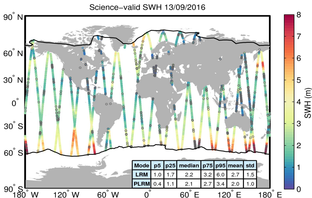
Figure 19. Geographical distribution of science-valid SWH data over oceans and lakes for 13/09/2016. The statistical values shown in the table refer to the SWH in m and are calculated separately for LRM and PLRM regions. The black lines mark the outer limit of the Arctic and Antarctic polar polygons. Gray circles denote records that have been rejected based on the editing criteria described in Table 3.
