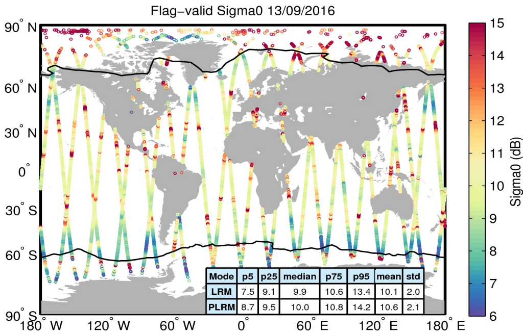
Figure 23. Geographical distribution of flag-valid sigma0 data over oceans and lakes for 13/09/2016. The statistical values shown in the table refer to the sigma0 in dB and are calculated separately for LRM and PLRM regions. Measurements taken over polar polygons have been excluded from the computation of the statistical values. The black lines mark the outer limit of the Arctic and Antarctic polar polygons.
