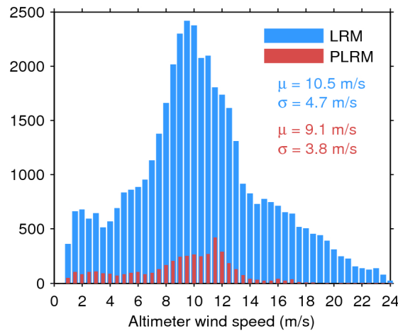
Figure 33. Histogram of flag-valid wind over oceans and lakes for LRM (blue) and PLRM (red) for 13/09/2016. The mean ( \mu ) and standard deviation ( \sigma ) are also shown. Note that values larger than 24 m/s are excluded from the histogram for the sake of readability but not from the computation of \mu and \sigma .
