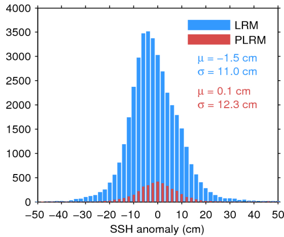
Figure 11. Histogram of science-valid SSH anomaly over oceans and lakes for LRM (blue) and PLRM (red) for 13/09/2016. The mean ( \mu ) and standard deviation ( \sigma ) are also shown. Note that values outside [-50 50] cm are excluded from the histogram for the sake of readability but not from the computation of \mu and \sigma .
