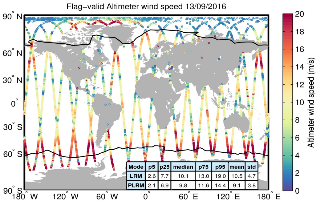
Figure 31. Geographical distribution of flag-valid wind data over oceans and lakes for 13/09/2016. The statistical values shown in the table refer to the wind in m/s and are calculated separately for LRM and PLRM regions. Measurements taken over polar polygons have been excluded from the computation of the statistical values. The black lines mark the outer limit of the Arctic and Antarctic polar polygons.
