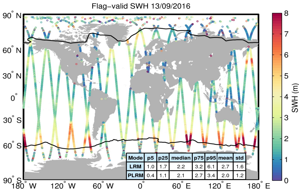
Figure 15. Geographical distribution of flag-valid SWH data over oceans and lakes for 13/09/2016. The statistical values shown in the table refer to the SWH in m and are calculated separately for LRM and PLRM regions. Measurements taken over polar polygons have been excluded from the computation of the statistical values. The black lines mark the outer limit of the Arctic and Antarctic polar polygons.
