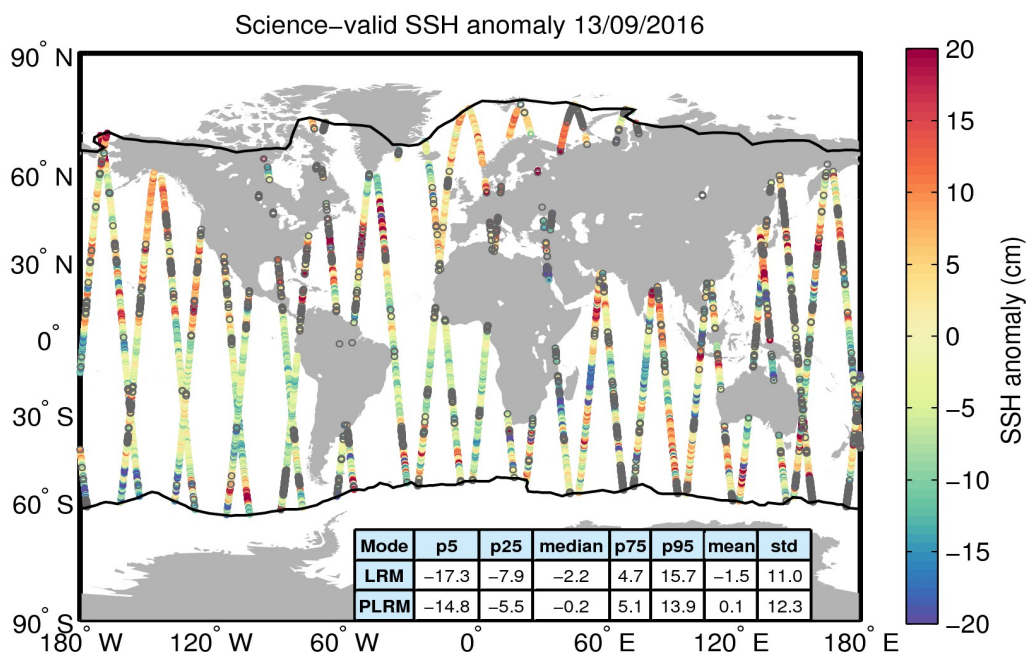
Figure 10. Geographical distribution of science-valid SSH anomaly data over oceans and lakes for 13/09/2016. The statistical values shown in the table refer to the SSH anomaly in cm and are calculated separately for LRM and PLRM regions. The black lines mark the outer limit of the Arctic and Antarctic polar polygons. Gray circles denote records that have been rejected based on the editing criteria described in Table 2.
