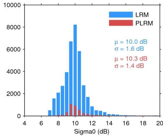
Figure 28. Histogram of science-valid sigma0 over oceans and lakes for LRM (blue) and PLRM (red) for 13/09/2016. The mean ( \mu ) and standard deviation ( \sigma ) are also shown. Note that values outside [4 20] dB are excluded from the histogram for the sake of readability but not from the computation of \mu and \sigma .
