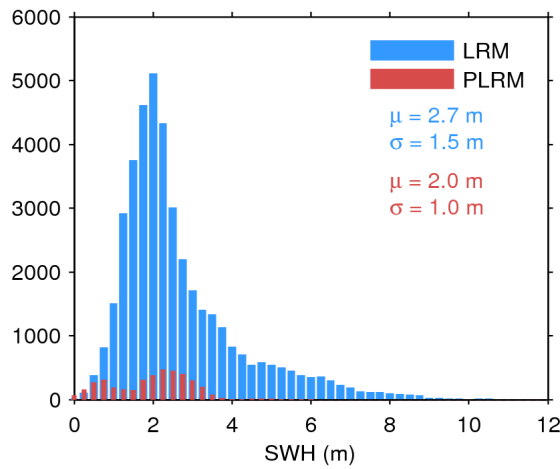
Figure 20. Histogram of science-valid SWH over oceans and lakes for LRM (blue) and PLRM (red) for 13/09/2016. The mean ( \mu ) and standard deviation ( \sigma ) are also shown. Note that values larger than 12 m are excluded from the histogram for the sake of readability but not from the computation of \mu and \sigma .
