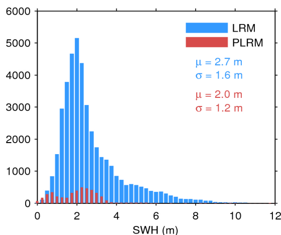
Figure 17. Histogram of flag-valid SWH over oceans and lakes for LRM (blue) and PLRM (red) for 13/09/2016. The mean ( \mu ) and standard deviation ( \sigma ) are also shown. Note that values larger than 12 m are excluded from the histogram for the sake of readability but not from the computation of \mu and \sigma .
