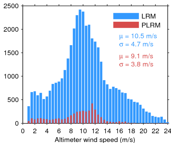
Figure 35. Histogram of science-valid wind over oceans and lakes for LRM (blue) and PLRM (red) for 13/09/2016. The mean ( \mu ) and standard deviation ( \sigma ) are also shown. Note that values larger than 24 m/s are excluded from the histogram for the sake of readability but not from the computation of \mu and \sigma .
