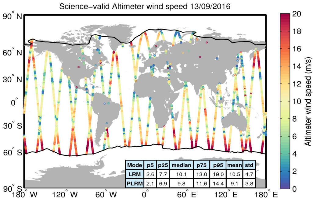
Figure 34. Geographical distribution of science-valid wind data over oceans and lakes for 13/09/2016. The statistical values shown in the table refer to the wind in m/s and are calculated separately for LRM and PLRM regions. The black lines mark the outer limit of the Arctic and Antarctic polar polygons. Gray circles denote records that have been rejected based on the editing criteria described in Table 5.
