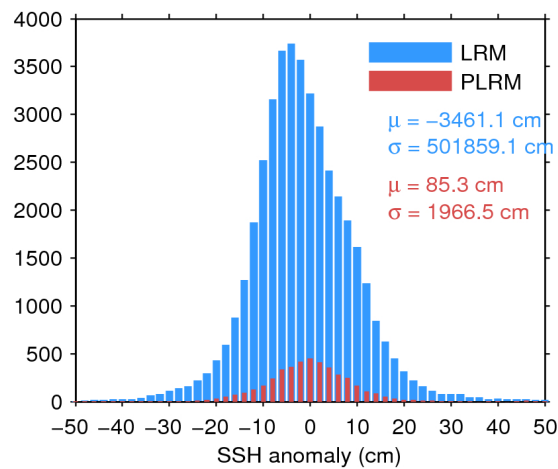
Figure 7. Histogram of flag-valid SSH anomaly over oceans and lakes for LRM (blue) and PLRM (red) for 13/09/2016. The mean ( \mu ) and standard deviation ( \sigma ) are also shown. Note that values outside [-50\ 50] cm are excluded from the histogram for the sake of readability but not from the computation of \mu and \sigma .
