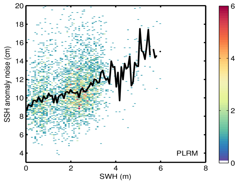
Figure 9. 2D histogram showing flag-valid SSH anomaly noise as a function of SWH for LRM (top) and PLRM (bottom) for 13/09/2016. The black line denotes the median SSH anomaly noise as a function of SWH.
