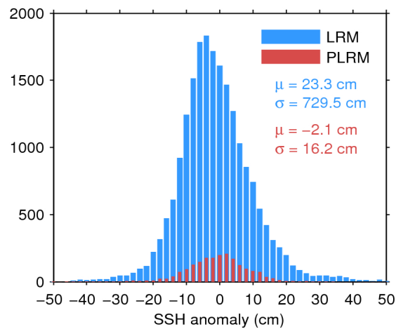
Figure 7. Histogram of flag-valid SSH anomaly over oceans and lakes for LRM (blue) and PLRM (red) for 11/09/2016. The mean ( \mu ) and standard deviation ( \sigma ) are also shown. Note that values outside [-50 \ 50] cm are excluded from the histogram for the sake of readability but not from the computation of \mu and \sigma .
