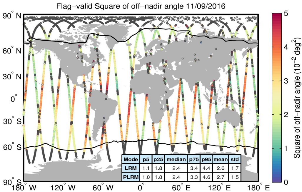
Figure 37. Geographical distribution of flag-valid mispointing data over oceans and lakes for 11/09/2016. The statistical values shown in the table refer to the mispointing in 10^{-2} deg 2 and are calculated separately for LRM and PLRM regions. Measurements taken over polar polygons have been excluded from the computation of the statistical values. The black lines mark the outer limit of the Arctic and Antarctic polar polygons. Gray circles denote negative values.
