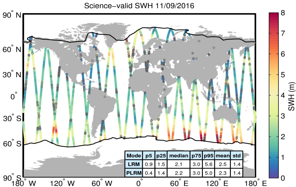
Figure 19. Geographical distribution of science-valid SWH data over oceans and lakes for 11/09/2016. The statistical values shown in the table refer to the SWH in m and are calculated separately for LRM and PLRM regions. The black lines mark the outer limit of the Arctic and Antarctic polar polygons. Gray circles denote records that have been rejected based on the editing criteria described in Table 3.
