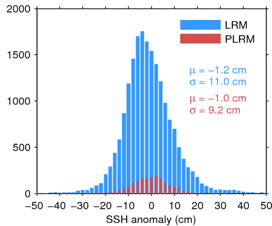
Figure 11. Histogram of science-valid SSH anomaly over oceans and lakes for LRM (blue) and PLRM (red) for 11/09/2016. The mean ( \mu ) and standard deviation ( \sigma ) are also shown. Note that values outside [-50\ 50] cm are excluded from the histogram for the sake of readability but not from the computation of \mu and \sigma .
