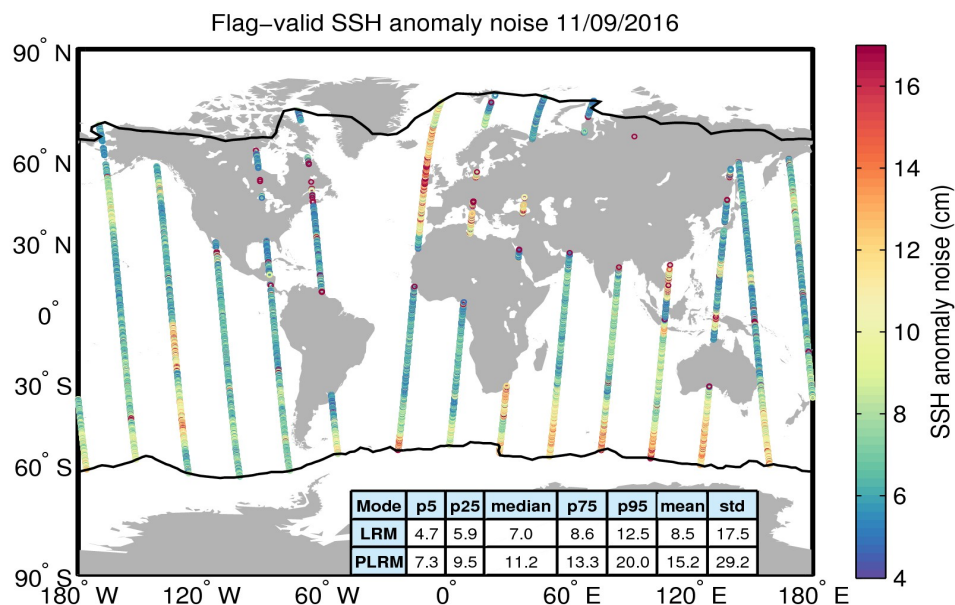
Figure 8. Geographical distribution of flag-valid 20-Hz SSH anomaly measurement noise over oceans and lakes for 11/09/2016. The statistical values shown in the table refer to the SSH anomaly noise and are calculated separately for LRM and PLRM regions. Measurements taken over polar polygons have been excluded from the computation of the statistical values. The black lines mark the outer limit of the Arctic and Antarctic polar polygons.
