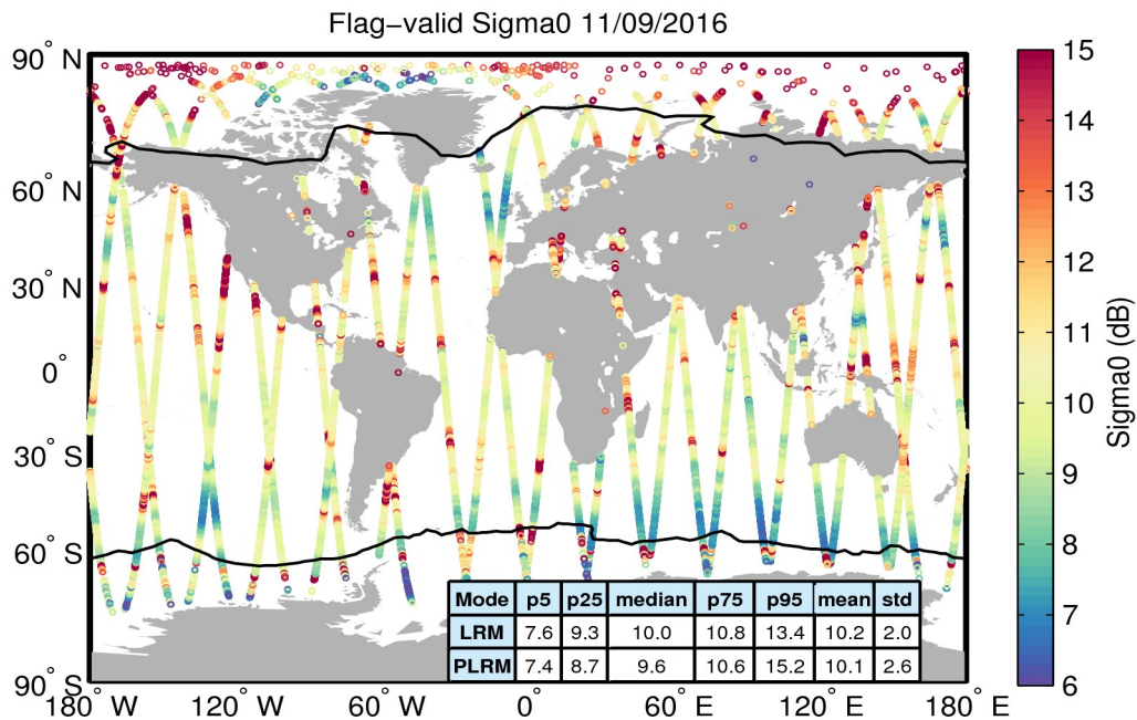
Figure 23. Geographical distribution of flag-valid sigma0 data over oceans and lakes for 11/09/2016. The statistical values shown in the table refer to the sigma0 in dB and are calculated separately for LRM and PLRM regions. Measurements taken over polar polygons have been excluded from the computation of the statistical values. The black lines mark the outer limit of the Arctic and Antarctic polar polygons.
