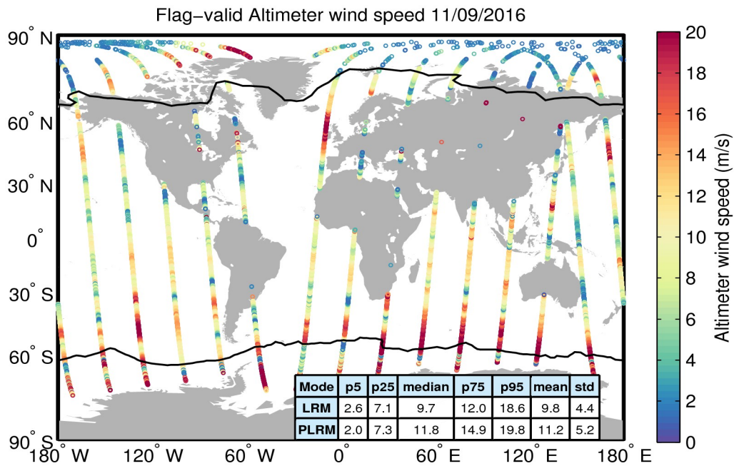
Figure 31. Geographical distribution of flag-valid wind data over oceans and lakes for 11/09/2016. The statistical values shown in the table refer to the wind in m/s and are calculated separately for LRM and PLRM regions. Measurements taken over polar polygons have been excluded from the computation of the statistical values. The black lines mark the outer limit of the Arctic and Antarctic polar polygons.
