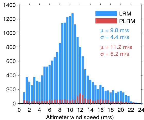
Figure 35. Histogram of science-valid wind over oceans and lakes for LRM (blue) and PLRM (red) for 11/09/2016. The mean ( \mu ) and standard deviation ( \sigma ) are also shown. Note that values larger than 24 m/s are excluded from the histogram for the sake of readability but not from the computation of \mu and \sigma .
