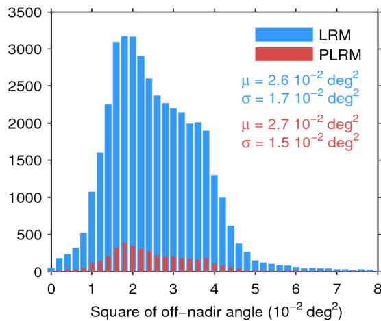
Figure 39. Histogram of flag-valid mispointing over oceans and lakes for LRM (blue) and PLRM (red) for 11/09/2016. Only positive values have been considered. The mean ( \mu ) and standard deviation ( \sigma ) are also shown. Note that values larger than 8 \cdot 10^{-2} \text{ deg}^2 are excluded from the histogram for the sake of readability but not from the computation of \mu and \sigma .
