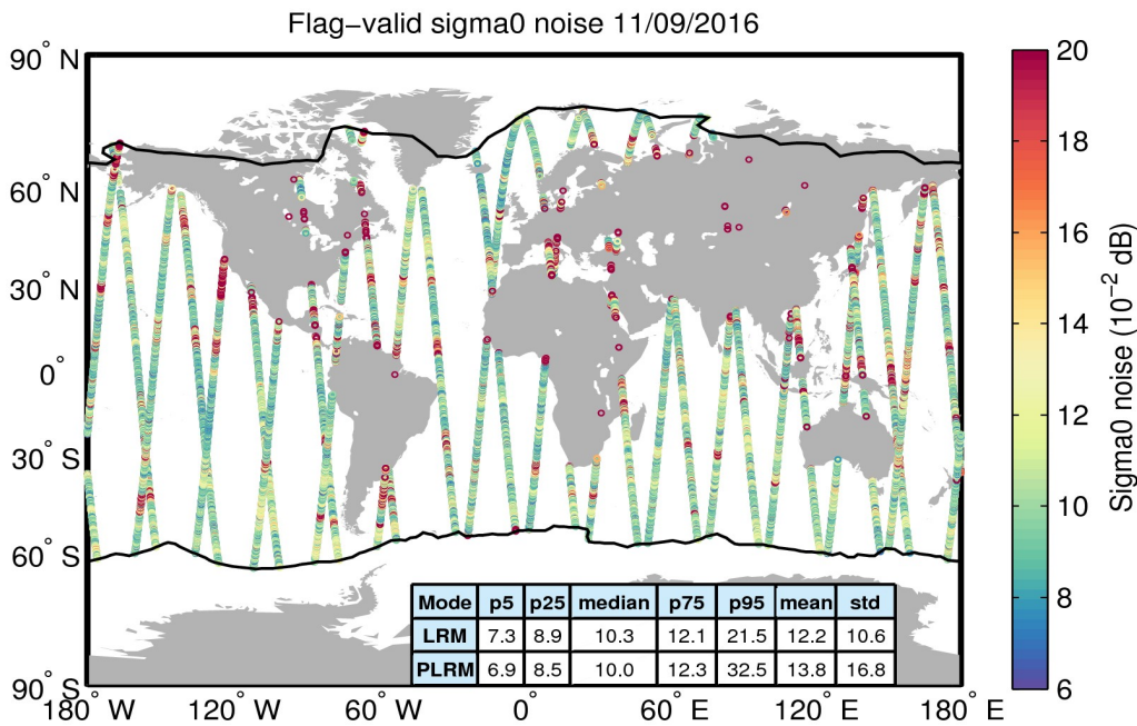
Figure 26. Geographical distribution of flag-valid 20-Hz sigma0 measurement noise over oceans and lakes for 11/09/2016. The statistical values shown in the table refer to the sigma0 noise and are calculated separately for LRM and PLRM regions. Measurements taken over polar polygons have been excluded from the computation of the statistical values. The black lines mark the outer limit of the Arctic and Antarctic polar polygons.
