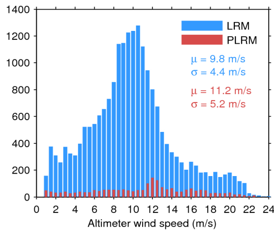
Figure 33. Histogram of flag-valid wind over oceans and lakes for LRM (blue) and PLRM (red) for 11/09/2016. The mean ( \mu ) and standard deviation ( \sigma ) are also shown. Note that values larger than 24 m/s are excluded from the histogram for the sake of readability but not from the computation of \mu and \sigma .
