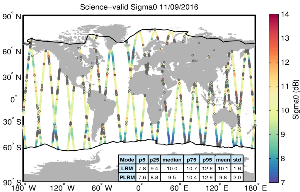
Figure 27. Geographical distribution of science-valid sigma0 data over oceans and lakes for 11/09/2016. The statistical values shown in the table refer to the sigma0 in dB and are calculated separately for LRM and PLRM regions. The black lines mark the outer limit of the Arctic and Antarctic polar polygons. Gray circles denote records that have been rejected based on the editing criteria described in Table 4.
