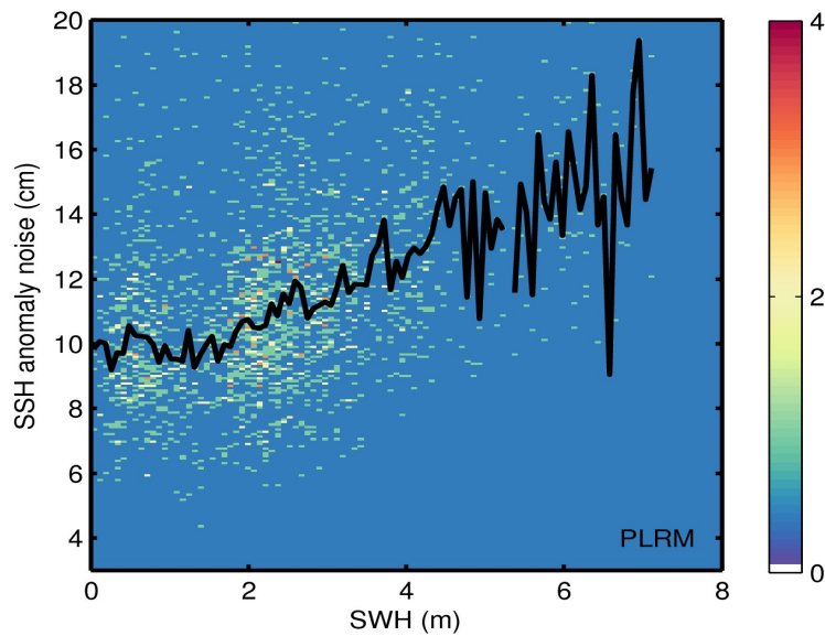
Figure 9. 2D histogram showing flag-valid SSH anomaly noise as a function of SWH for LRM (top) and PLRM (bottom) for 11/09/2016. The black line denotes the median SSH anomaly noise as a function of SWH.
