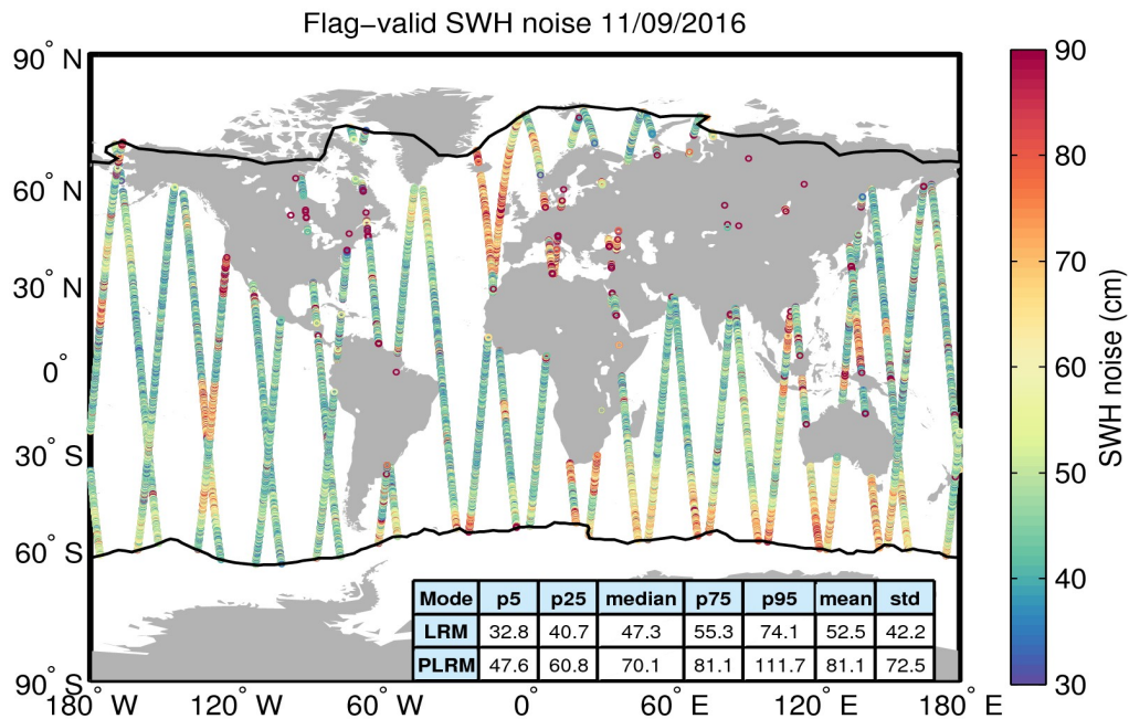
Figure 18. Geographical distribution of flag-valid 20-Hz SWH measurement noise over oceans and lakes for 11/09/2016. The statistical values shown in the table refer to the SWH noise and are calculated separately for LRM and PLRM regions. Measurements taken over polar polygons have been excluded from the computation of the statistical values. The black lines mark the outer limit of the Arctic and Antarctic polar polygons.
