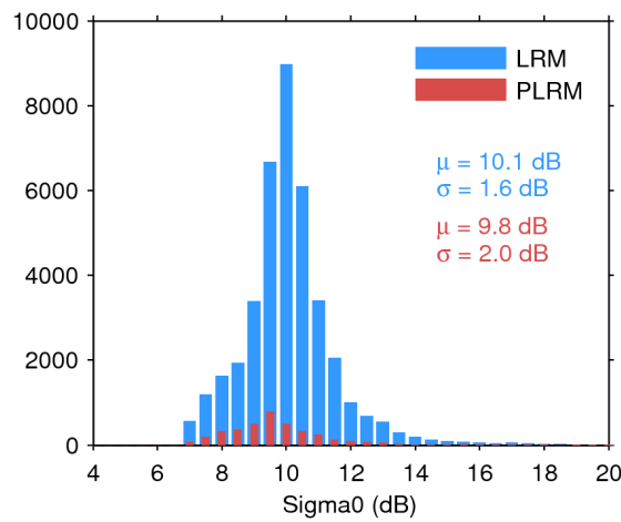
Figure 28. Histogram of science-valid sigma0 over oceans and lakes for LRM (blue) and PLRM (red) for 11/09/2016. The mean ( \mu ) and standard deviation ( \sigma ) are also shown. Note that values outside [4 20] dB are excluded from the histogram for the sake of readability but not from the computation of \mu and \sigma .
