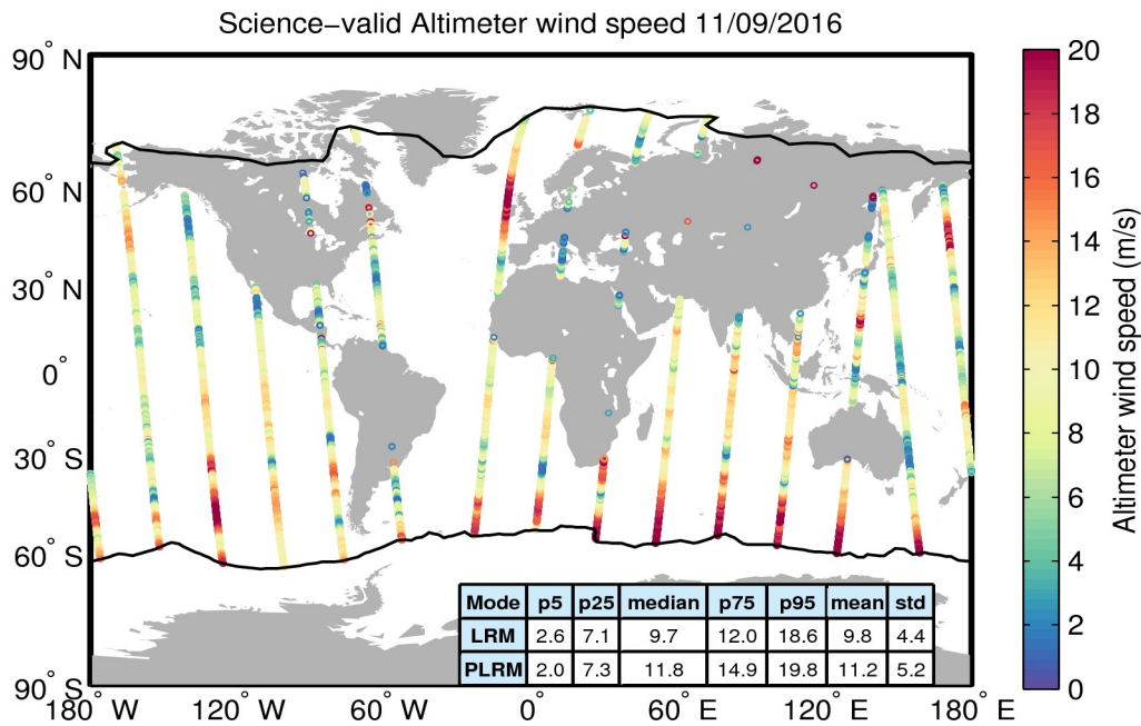
Figure 34. Geographical distribution of science-valid wind data over oceans and lakes for 11/09/2016. The statistical values shown in the table refer to the wind in m/s and are calculated separately for LRM and PLRM regions. The black lines mark the outer limit of the Arctic and Antarctic polar polygons. Gray circles denote records that have been rejected based on the editing criteria described in Table 5.
