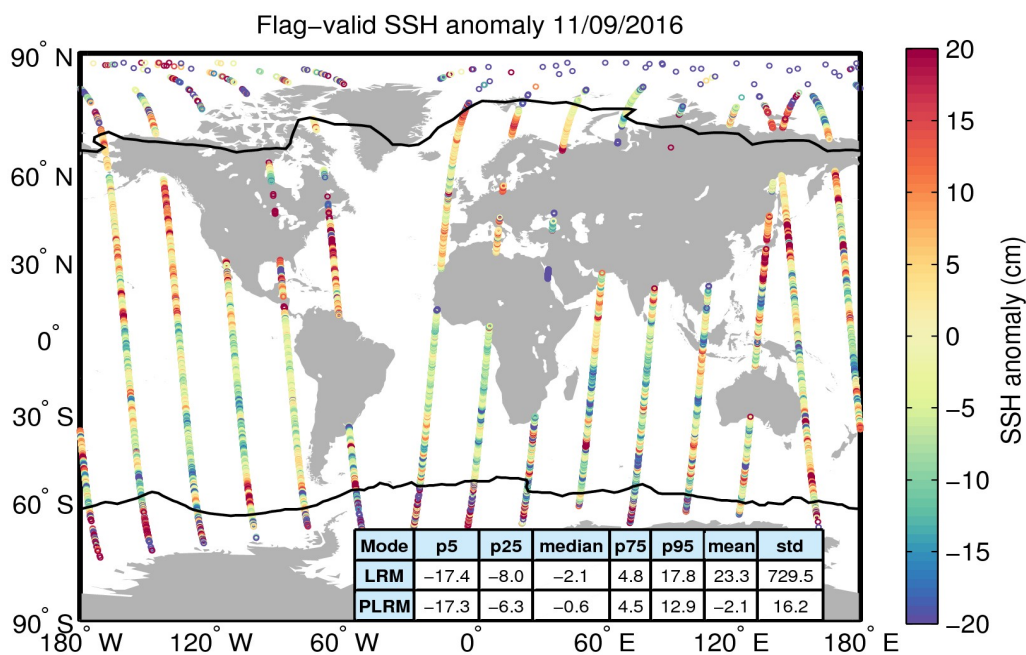
Figure 5. Geographical distribution of flag-valid 1-Hz SSH anomaly data over oceans and lakes for 11/09/2016. The statistical values shown in the table refer to the SSH anomaly in cm and are calculated separately for LRM and PLRM regions. Measurements taken over polar polygons have been excluded from the computation of the statistical values. The black lines mark the outer limit of the Arctic and Antarctic polar polygons.
