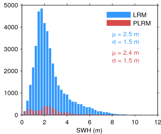
Figure 17. Histogram of flag-valid SWH over oceans and lakes for LRM (blue) and PLRM (red) for 11/09/2016. The mean ( \mu ) and standard deviation ( \sigma ) are also shown. Note that values larger than 12 m are excluded from the histogram for the sake of readability but not from the computation of \mu and \sigma .
