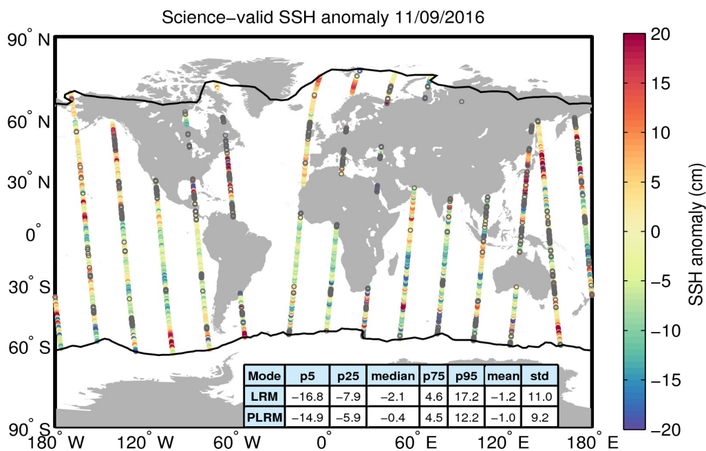
Figure 10. Geographical distribution of science-valid SSH anomaly data over oceans and lakes for 11/09/2016. The statistical values shown in the table refer to the SSH anomaly in cm and are calculated separately for LRM and PLRM regions. The black lines mark the outer limit of the Arctic and Antarctic polar polygons. Gray circles denote records that have been rejected based on the editing criteria described in Table 2.
