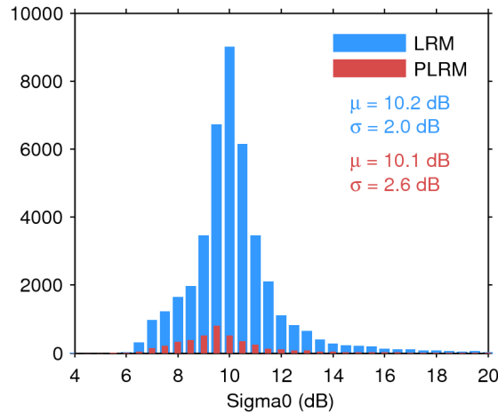
Figure 25. Histogram of flag-valid sigma0 over oceans and lakes for LRM (blue) and PLRM (red) for 11/09/2016. The mean ( \mu ) and standard deviation ( \sigma ) are also shown. Note that values outside [4 20] dB are excluded from the histogram for the sake of readability but not from the computation of \mu and \sigma .
