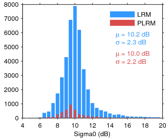
Figure 25. Histogram of flag-valid sigma0 over oceans and lakes for LRM (blue) and PLRM (red) for 09/09/2016. The mean ( \mu ) and standard deviation ( \sigma ) are also shown. Note that values outside [4 20] dB are excluded from the histogram for the sake of readability but not from the computation of \mu and \sigma .
