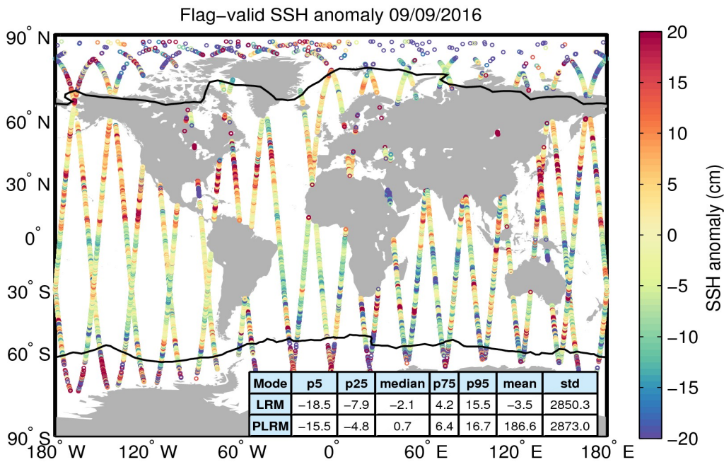
Figure 5. Geographical distribution of flag-valid 1-Hz SSH anomaly data over oceans and lakes for 09/09/2016. The statistical values shown in the table refer to the SSH anomaly in cm and are calculated separately for LRM and PLRM regions. Measurements taken over polar polygons have been excluded from the computation of the statistical values. The black lines mark the outer limit of the Arctic and Antarctic polar polygons.
