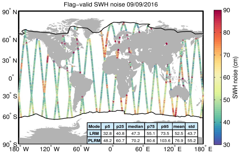
Figure 18. Geographical distribution of flag-valid 20-Hz SWH measurement noise over oceans and lakes for 09/09/2016. The statistical values shown in the table refer to the SWH noise and are calculated separately for LRM and PLRM regions. Measurements taken over polar polygons have been excluded from the computation of the statistical values. The black lines mark the outer limit of the Arctic and Antarctic polar polygons.
