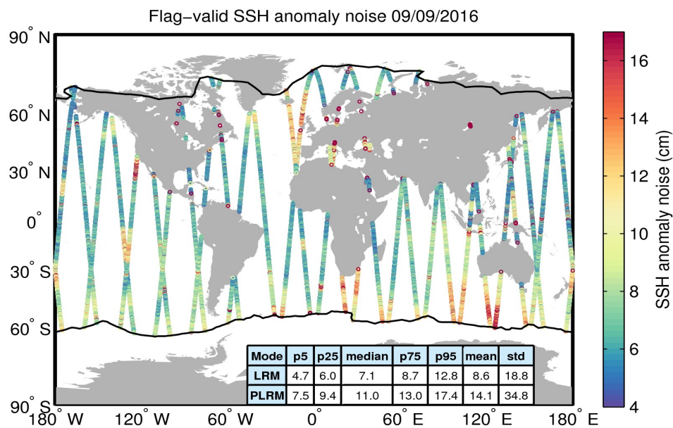
Figure 8. Geographical distribution of flag-valid 20-Hz SSH anomaly measurement noise over oceans and lakes for 09/09/2016. The statistical values shown in the table refer to the SSH anomaly noise and are calculated separately for LRM and PLRM regions. Measurements taken over polar polygons have been excluded from the computation of the statistical values. The black lines mark the outer limit of the Arctic and Antarctic polar polygons.
