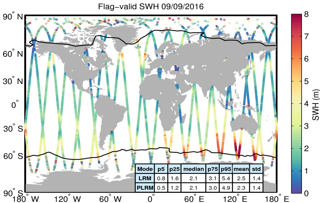
Figure 15. Geographical distribution of flag-valid SWH data over oceans and lakes for 09/09/2016. The statistical values shown in the table refer to the SWH in m and are calculated separately for LRM and PLRM regions. Measurements taken over polar polygons have been excluded from the computation of the statistical values. The black lines mark the outer limit of the Arctic and Antarctic polar polygons.
