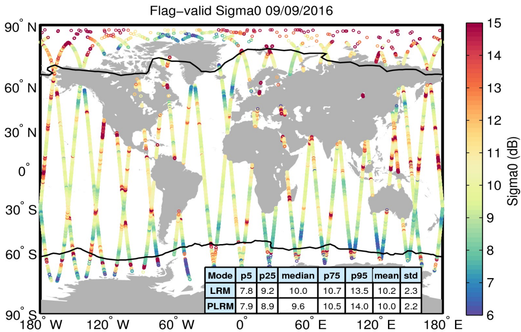
Figure 23. Geographical distribution of flag-valid sigma0 data over oceans and lakes for 09/09/2016. The statistical values shown in the table refer to the sigma0 in dB and are calculated separately for LRM and PLRM regions. Measurements taken over polar polygons have been excluded from the computation of the statistical values. The black lines mark the outer limit of the Arctic and Antarctic polar polygons.
