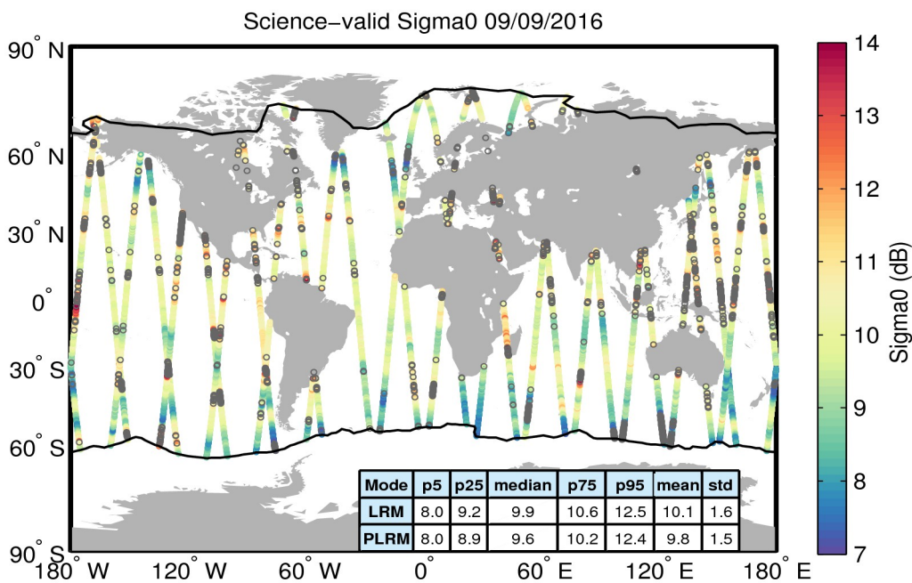
Figure 27. Geographical distribution of science-valid sigma0 data over oceans and lakes for 09/09/2016. The statistical values shown in the table refer to the sigma0 in dB and are calculated separately for LRM and PLRM regions. The black lines mark the outer limit of the Arctic and Antarctic polar polygons. Gray circles denote records that have been rejected based on the editing criteria described in Table 4.
