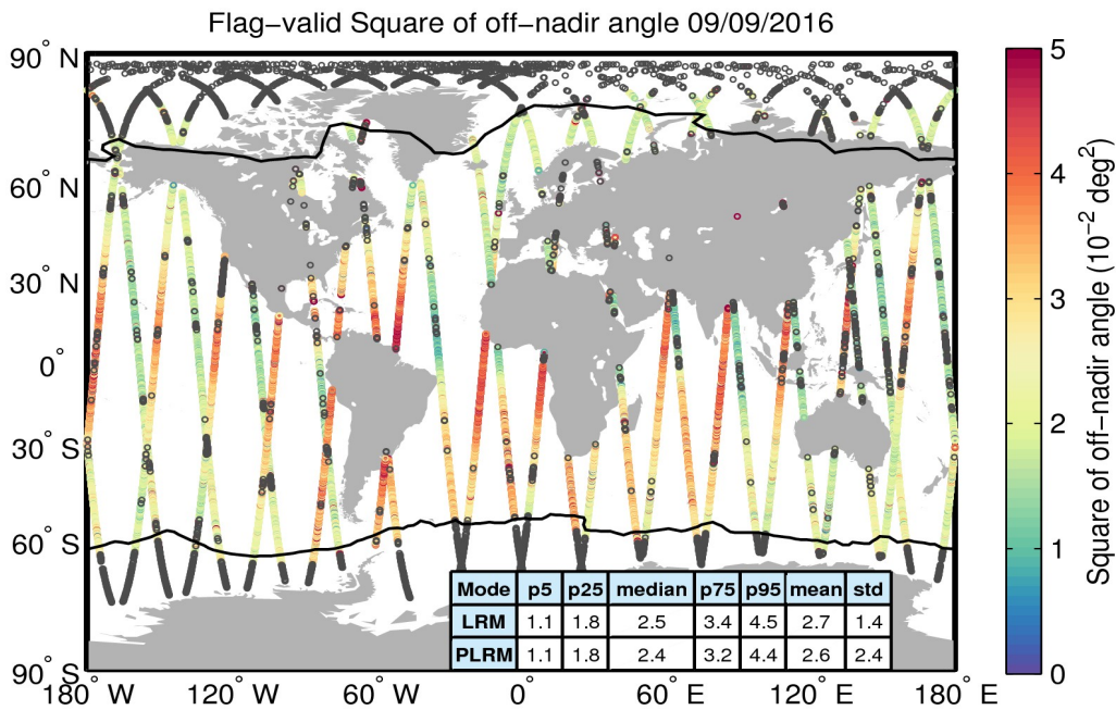
Figure 37. Geographical distribution of flag-valid mispointing data over oceans and lakes for 09/09/2016. The statistical values shown in the table refer to the mispointing in 10^{-2} deg 2 and are calculated separately for LRM and PLRM regions. Measurements taken over polar polygons have been excluded from the computation of the statistical values. The black lines mark the outer limit of the Arctic and Antarctic polar polygons. Gray circles denote negative values.
