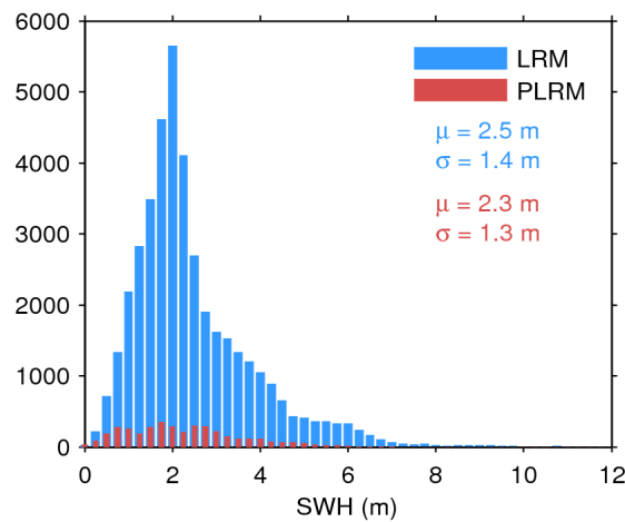
Figure 20. Histogram of science-valid SWH over oceans and lakes for LRM (blue) and PLRM (red) for 09/09/2016. The mean ( \mu ) and standard deviation ( \sigma ) are also shown. Note that values larger than 12 m are excluded from the histogram for the sake of readability but not from the computation of \mu and \sigma .
