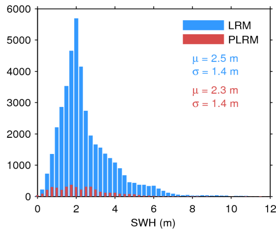
Figure 17. Histogram of flag-valid SWH over oceans and lakes for LRM (blue) and PLRM (red) for 09/09/2016. The mean ( \mu ) and standard deviation ( \sigma ) are also shown. Note that values larger than 12 m are excluded from the histogram for the sake of readability but not from the computation of \mu and \sigma .
