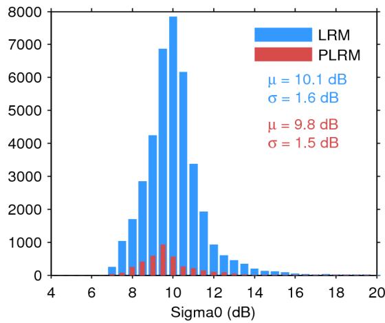
Figure 28. Histogram of science-valid sigma0 over oceans and lakes for LRM (blue) and PLRM (red) for 09/09/2016. The mean ( \mu ) and standard deviation ( \sigma ) are also shown. Note that values outside [4 20] dB are excluded from the histogram for the sake of readability but not from the computation of \mu and \sigma .
