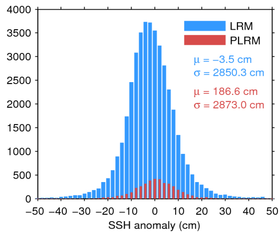
Figure 7. Histogram of flag-valid SSH anomaly over oceans and lakes for LRM (blue) and PLRM (red) for 09/09/2016. The mean ( \mu ) and standard deviation ( \sigma ) are also shown. Note that values outside [-50\ 50] cm are excluded from the histogram for the sake of readability but not from the computation of \mu and \sigma .
