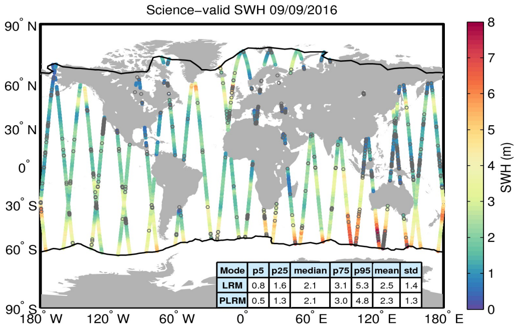
Figure 19. Geographical distribution of science-valid SWH data over oceans and lakes for 09/09/2016. The statistical values shown in the table refer to the SWH in m and are calculated separately for LRM and PLRM regions. The black lines mark the outer limit of the Arctic and Antarctic polar polygons. Gray circles denote records that have been rejected based on the editing criteria described in Table 3.
