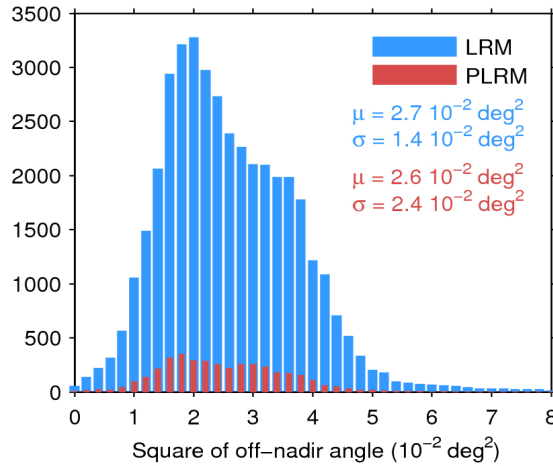
Figure 39. Histogram of flag-valid mispointing over oceans and lakes for LRM (blue) and PLRM (red) for 09/09/2016. Only positive values have been considered. The mean ( \mu ) and standard deviation ( \sigma ) are also shown. Note that values larger than 8 \cdot 10^{-2} \text{ deg}^2 are excluded from the histogram for the sake of readability but not from the computation of \mu and \sigma .
