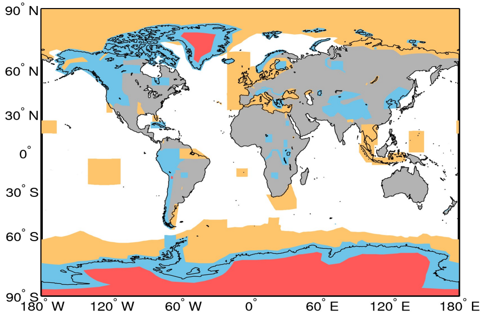
Figure A1. Extent of the regions defining the geographical mode mask for 09/09/2016. The regions where SAR, and SARIn are operated are denoted by the orange and blue polygons, respectively. LRM is operated over areas of the continental ice sheets (red polygons) and over oceans and land not covered by other modes.
