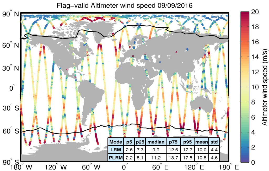
Figure 31. Geographical distribution of flag-valid wind data over oceans and lakes for 09/09/2016. The statistical values shown in the table refer to the wind in m/s and are calculated separately for LRM and PLRM regions. Measurements taken over polar polygons have been excluded from the computation of the statistical values. The black lines mark the outer limit of the Arctic and Antarctic polar polygons.
