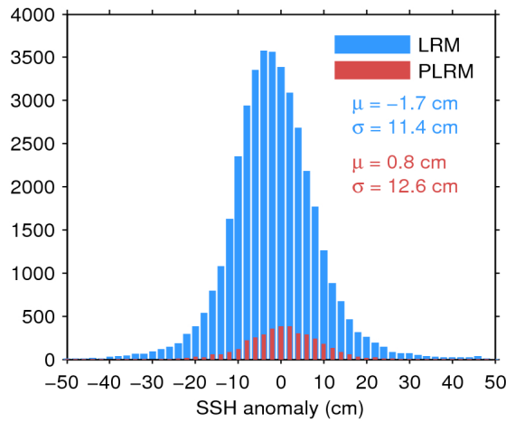
Figure 11. Histogram of science-valid SSH anomaly over oceans and lakes for LRM (blue) and PLRM (red) for 09/09/2016. The mean ( \mu ) and standard deviation ( \sigma ) are also shown. Note that values outside [-50 50] cm are excluded from the histogram for the sake of readability but not from the computation of \mu and \sigma .
