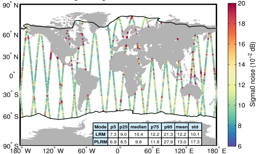
Flag-valid sigma0 noise 09/09/2016
