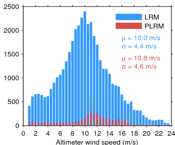
Figure 33. Histogram of flag-valid wind over oceans and lakes for LRM (blue) and PLRM (red) for 09/09/2016. The mean ( \mu ) and standard deviation ( \sigma ) are also shown. Note that values larger than 24 m/s are excluded from the histogram for the sake of readability but not from the computation of \mu and \sigma .
