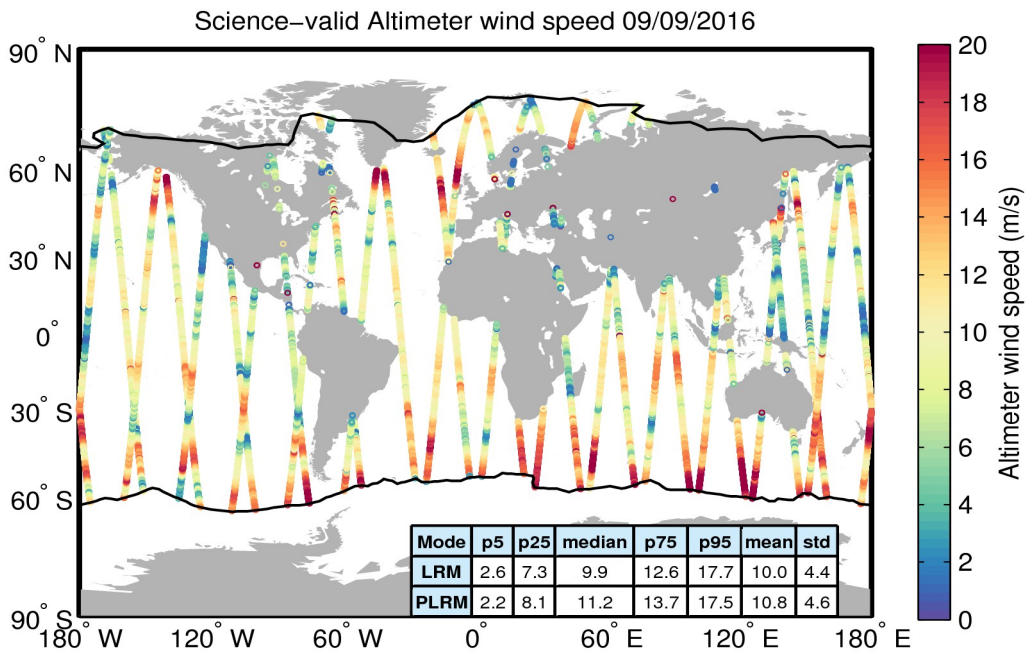
Figure 34. Geographical distribution of science-valid wind data over oceans and lakes for 09/09/2016. The statistical values shown in the table refer to the wind in m/s and are calculated separately for LRM and PLRM regions. The black lines mark the outer limit of the Arctic and Antarctic polar polygons. Gray circles denote records that have been rejected based on the editing criteria described in Table 5.
