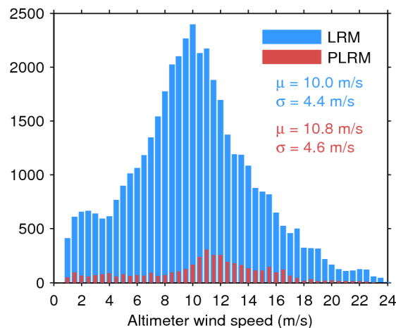
Figure 35. Histogram of science-valid wind over oceans and lakes for LRM (blue) and PLRM (red) for 09/09/2016. The mean ( \mu ) and standard deviation ( \sigma ) are also shown. Note that values larger than 24 m/s are excluded from the histogram for the sake of readability but not from the computation of \mu and \sigma .
