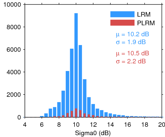
Figure 25. Histogram of flag-valid sigma0 over oceans and lakes for LRM (blue) and PLRM (red) for 08/09/2016. The mean ( \mu ) and standard deviation ( \sigma ) are also shown. Note that values outside [4 20] dB are excluded from the histogram for the sake of readability but not from the computation of \mu and \sigma .
