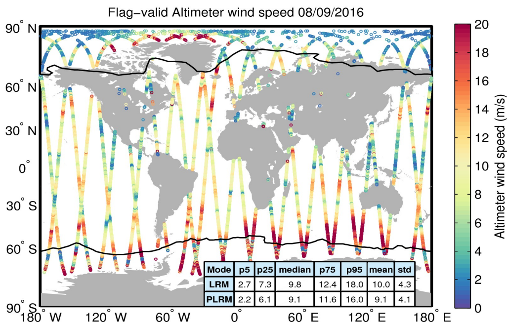
Figure 31. Geographical distribution of flag-valid wind data over oceans and lakes for 08/09/2016. The statistical values shown in the table refer to the wind in m/s and are calculated separately for LRM and PLRM regions. Measurements taken over polar polygons have been excluded from the computation of the statistical values. The black lines mark the outer limit of the Arctic and Antarctic polar polygons.
