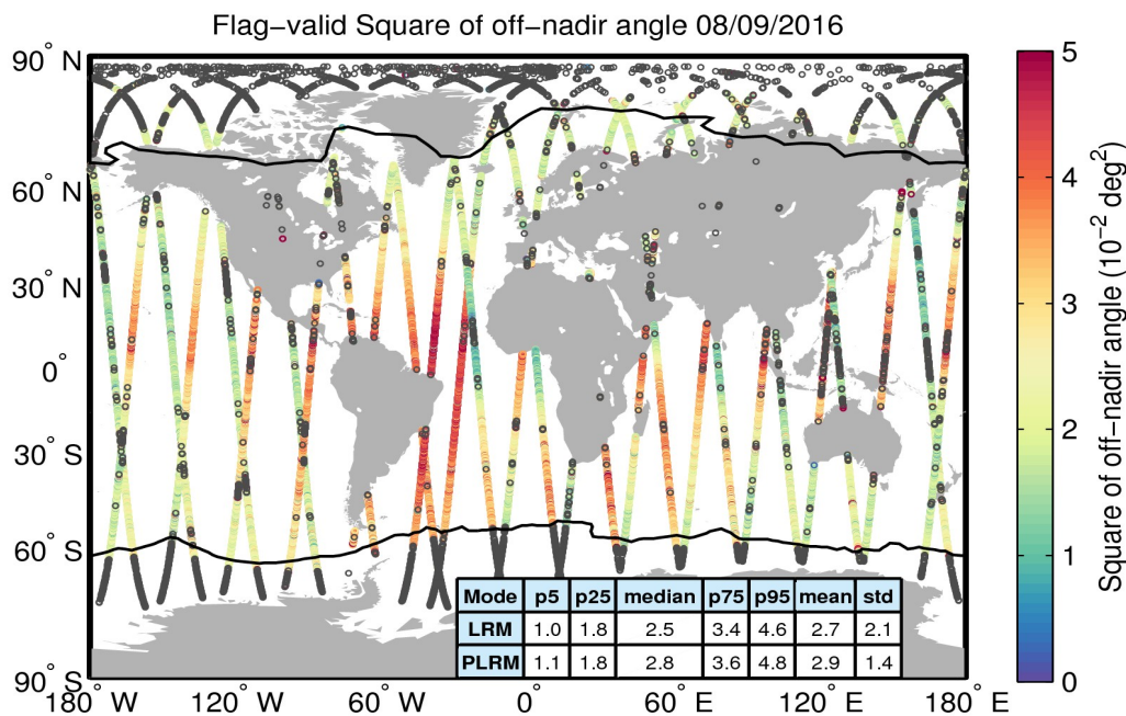
Figure 37. Geographical distribution of flag-valid mispointing data over oceans and lakes for 08/09/2016. The statistical values shown in the table refer to the mispointing in 10^{-2} deg 2 and are calculated separately for LRM and PLRM regions. Measurements taken over polar polygons have been excluded from the computation of the statistical values. The black lines mark the outer limit of the Arctic and Antarctic polar polygons. Gray circles denote negative values.
