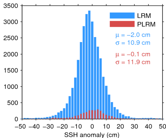
Figure 11. Histogram of science-valid SSH anomaly over oceans and lakes for LRM (blue) and PLRM (red) for 08/09/2016. The mean ( \mu ) and standard deviation ( \sigma ) are also shown. Note that values outside [-50 50] cm are excluded from the histogram for the sake of readability but not from the computation of \mu and \sigma .
