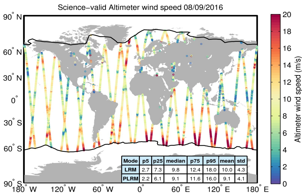
Figure 34. Geographical distribution of science-valid wind data over oceans and lakes for 08/09/2016. The statistical values shown in the table refer to the wind in m/s and are calculated separately for LRM and PLRM regions. The black lines mark the outer limit of the Arctic and Antarctic polar polygons. Gray circles denote records that have been rejected based on the editing criteria described in Table 5.
