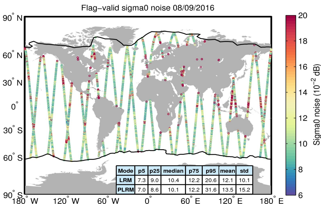
Figure 26. Geographical distribution of flag-valid 20-Hz sigma0 measurement noise over oceans and lakes for 08/09/2016. The statistical values shown in the table refer to the sigma0 noise and are calculated separately for LRM and PLRM regions. Measurements taken over polar polygons have been excluded from the computation of the statistical values. The black lines mark the outer limit of the Arctic and Antarctic polar polygons.
