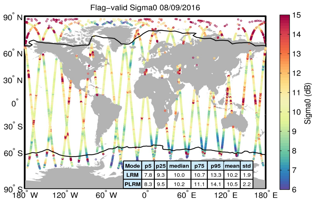
Figure 23. Geographical distribution of flag-valid sigma0 data over oceans and lakes for 08/09/2016. The statistical values shown in the table refer to the sigma0 in dB and are calculated separately for LRM and PLRM regions. Measurements taken over polar polygons have been excluded from the computation of the statistical values. The black lines mark the outer limit of the Arctic and Antarctic polar polygons.
