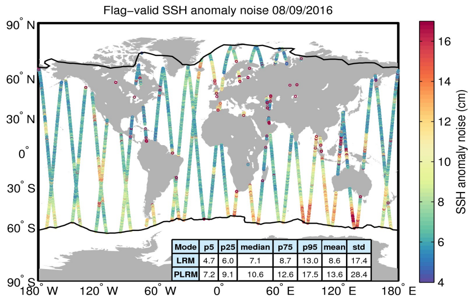
Figure 8. Geographical distribution of flag-valid 20-Hz SSH anomaly measurement noise over oceans and lakes for 08/09/2016. The statistical values shown in the table refer to the SSH anomaly noise and are calculated separately for LRM and PLRM regions. Measurements taken over polar polygons have been excluded from the computation of the statistical values. The black lines mark the outer limit of the Arctic and Antarctic polar polygons.
