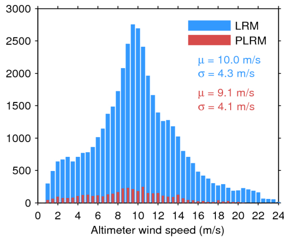
Figure 33. Histogram of flag-valid wind over oceans and lakes for LRM (blue) and PLRM (red) for 08/09/2016. The mean ( \mu ) and standard deviation ( \sigma ) are also shown. Note that values larger than 24 m/s are excluded from the histogram for the sake of readability but not from the computation of \mu and \sigma .
