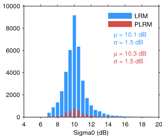
Figure 28. Histogram of science-valid sigma0 over oceans and lakes for LRM (blue) and PLRM (red) for 08/09/2016. The mean ( \mu ) and standard deviation ( \sigma ) are also shown. Note that values outside [4 20] dB are excluded from the histogram for the sake of readability but not from the computation of \mu and \sigma .
