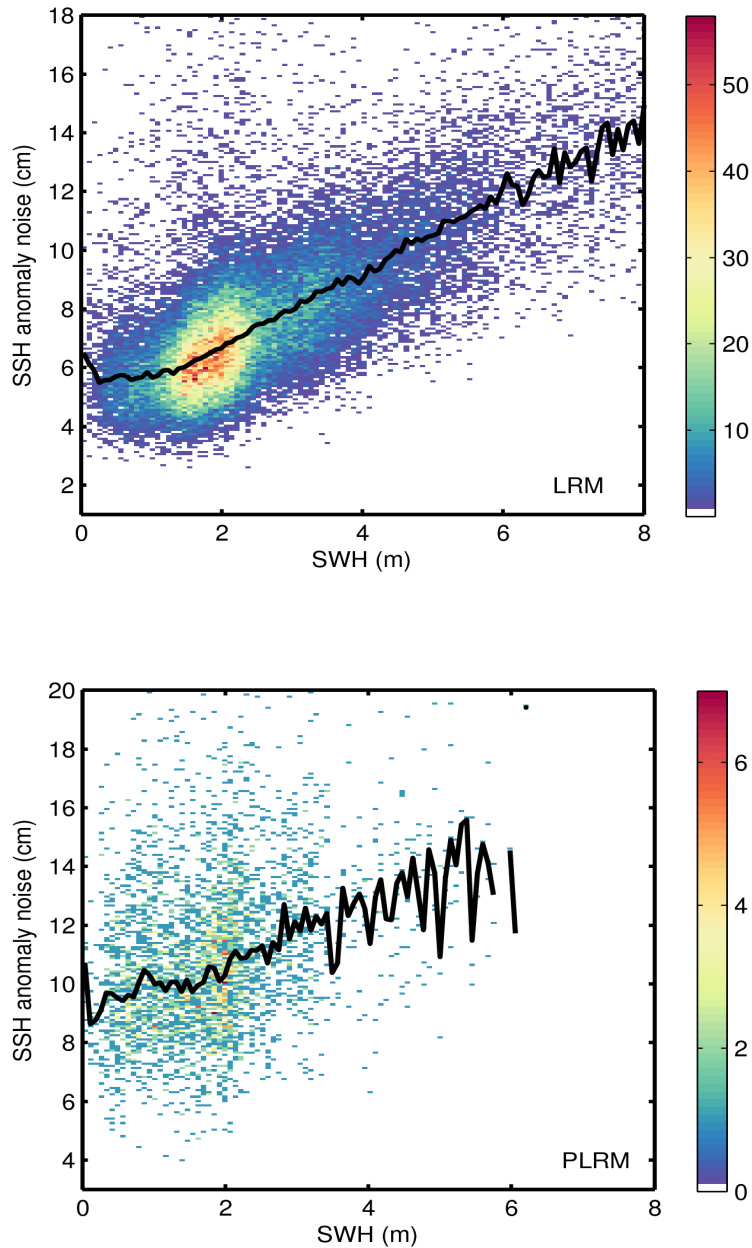
Figure 9. 2D histogram showing flag-valid SSH anomaly noise as a function of SWH for LRM (top) and PLRM (bottom) for 08/09/2016. The black line denotes the median SSH anomaly noise as a function of SWH.
