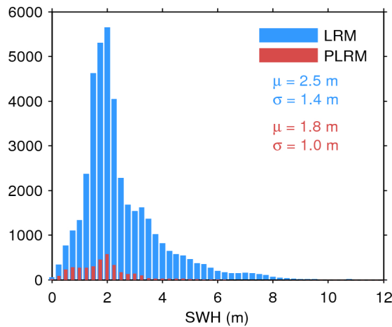
Figure 20. Histogram of science-valid SWH over oceans and lakes for LRM (blue) and PLRM (red) for 08/09/2016. The mean ( \mu ) and standard deviation ( \sigma ) are also shown. Note that values larger than 12 m are excluded from the histogram for the sake of readability but not from the computation of \mu and \sigma .
