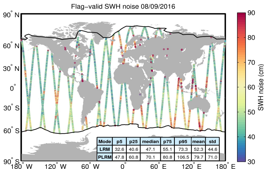
Figure 18. Geographical distribution of flag-valid 20-Hz SWH measurement noise over oceans and lakes for 08/09/2016. The statistical values shown in the table refer to the SWH noise and are calculated separately for LRM and PLRM regions. Measurements taken over polar polygons have been excluded from the computation of the statistical values. The black lines mark the outer limit of the Arctic and Antarctic polar polygons.
