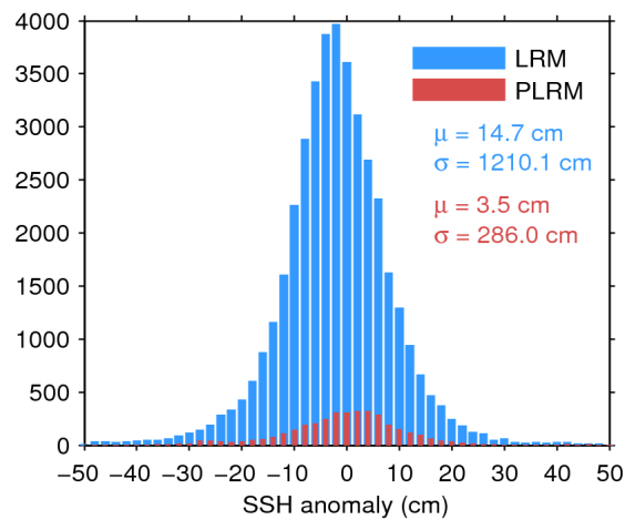
Figure 7. Histogram of flag-valid SSH anomaly over oceans and lakes for LRM (blue) and PLRM (red) for 08/09/2016. The mean ( \mu ) and standard deviation ( \sigma ) are also shown. Note that values outside [-50\ 50] cm are excluded from the histogram for the sake of readability but not from the computation of \mu and \sigma .
