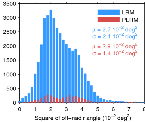
Figure 39. Histogram of flag-valid mispointing over oceans and lakes for LRM (blue) and PLRM (red) for 08/09/2016. Only positive values have been considered. The mean ( \mu ) and standard deviation ( \sigma ) are also shown. Note that values larger than 8 \cdot 10^{-2} \text{ deg}^2 are excluded from the histogram for the sake of readability but not from the computation of \mu and \sigma .
