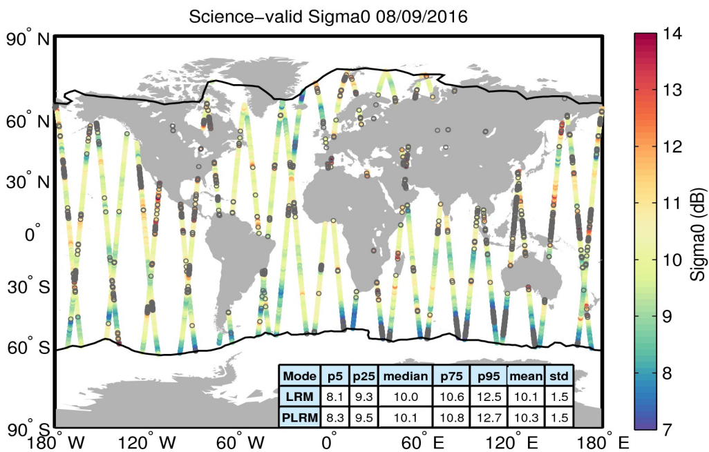
Figure 27. Geographical distribution of science-valid sigma0 data over oceans and lakes for 08/09/2016. The statistical values shown in the table refer to the sigma0 in dB and are calculated separately for LRM and PLRM regions. The black lines mark the outer limit of the Arctic and Antarctic polar polygons. Gray circles denote records that have been rejected based on the editing criteria described in Table 4.
