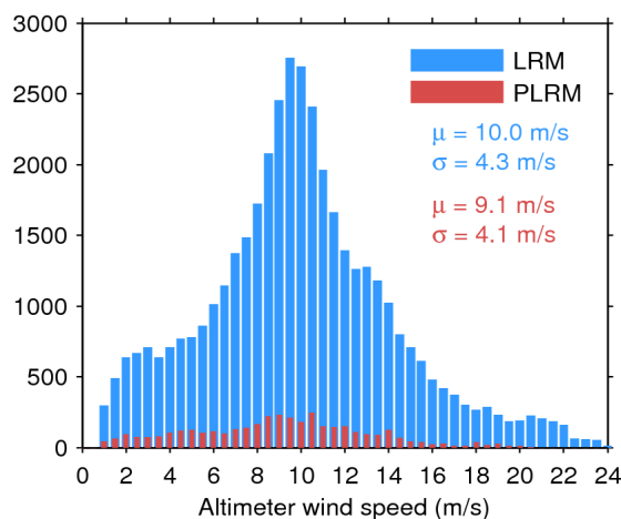
Figure 35. Histogram of science-valid wind over oceans and lakes for LRM (blue) and PLRM (red) for 08/09/2016. The mean ( \mu ) and standard deviation ( \sigma ) are also shown. Note that values larger than 24 m/s are excluded from the histogram for the sake of readability but not from the computation of \mu and \sigma .
