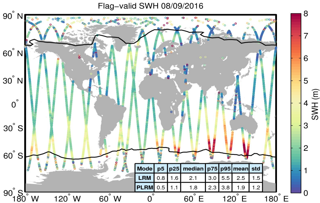
Figure 15. Geographical distribution of flag-valid SWH data over oceans and lakes for 08/09/2016. The statistical values shown in the table refer to the SWH in m and are calculated separately for LRM and PLRM regions. Measurements taken over polar polygons have been excluded from the computation of the statistical values. The black lines mark the outer limit of the Arctic and Antarctic polar polygons.
