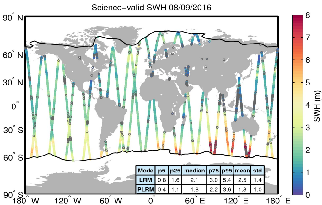
Figure 19. Geographical distribution of science-valid SWH data over oceans and lakes for 08/09/2016. The statistical values shown in the table refer to the SWH in m and are calculated separately for LRM and PLRM regions. The black lines mark the outer limit of the Arctic and Antarctic polar polygons. Gray circles denote records that have been rejected based on the editing criteria described in Table 3.
