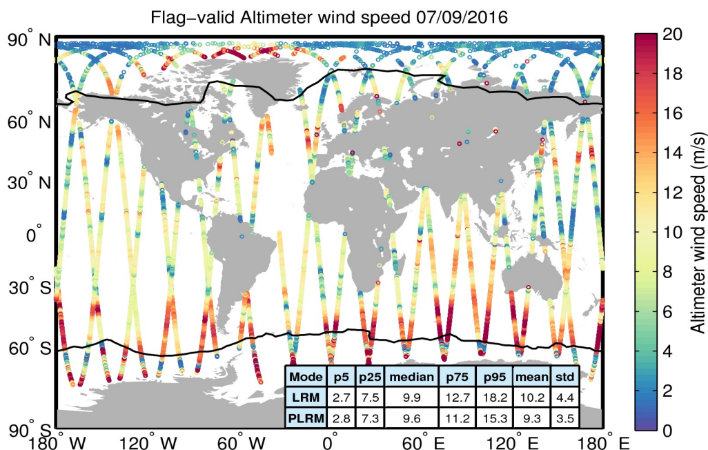
Figure 31. Geographical distribution of flag-valid wind data over oceans and lakes for 07/09/2016. The statistical values shown in the table refer to the wind in m/s and are calculated separately for LRM and PLRM regions. Measurements taken over polar polygons have been excluded from the computation of the statistical values. The black lines mark the outer limit of the Arctic and Antarctic polar polygons.
