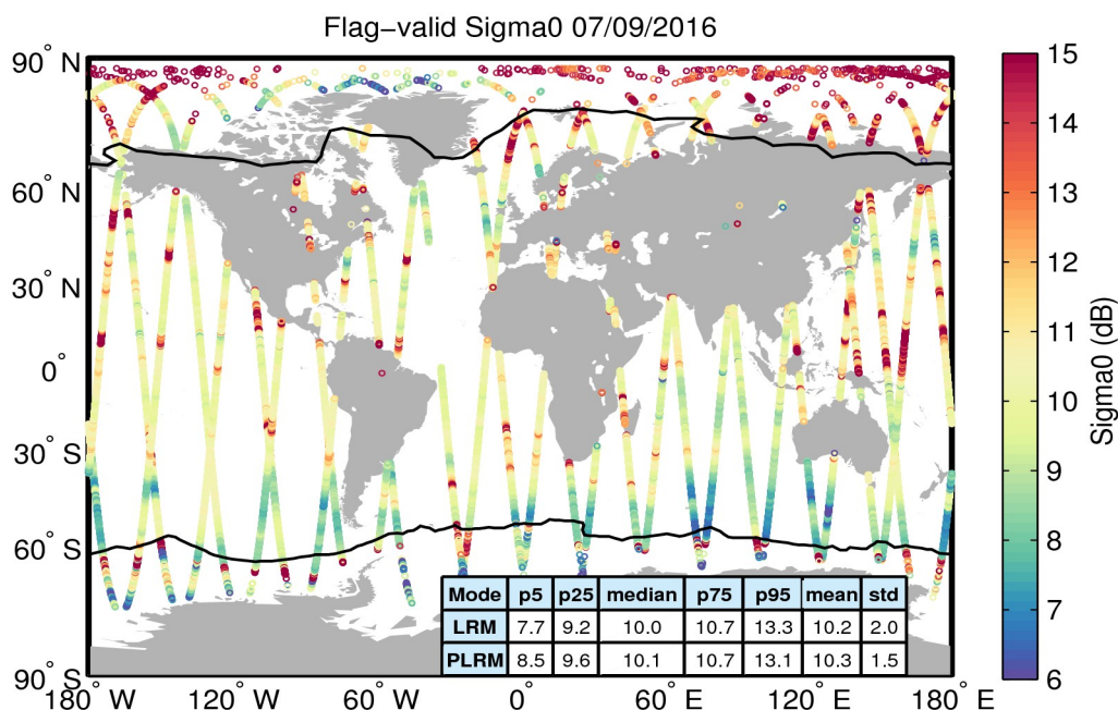
Figure 23. Geographical distribution of flag-valid sigma0 data over oceans and lakes for 07/09/2016. The statistical values shown in the table refer to the sigma0 in dB and are calculated separately for LRM and PLRM regions. Measurements taken over polar polygons have been excluded from the computation of the statistical values. The black lines mark the outer limit of the Arctic and Antarctic polar polygons.
