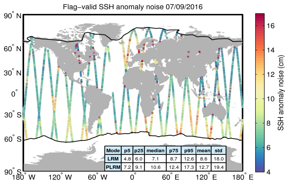
Figure 8. Geographical distribution of flag-valid 20-Hz SSH anomaly measurement noise over oceans and lakes for 07/09/2016. The statistical values shown in the table refer to the SSH anomaly noise and are calculated separately for LRM and PLRM regions. Measurements taken over polar polygons have been excluded from the computation of the statistical values. The black lines mark the outer limit of the Arctic and Antarctic polar polygons.
