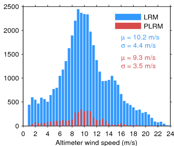
Figure 35. Histogram of science-valid wind over oceans and lakes for LRM (blue) and PLRM (red) for 07/09/2016. The mean ( \mu ) and standard deviation ( \sigma ) are also shown. Note that values larger than 24 m/s are excluded from the histogram for the sake of readability but not from the computation of \mu and \sigma .
