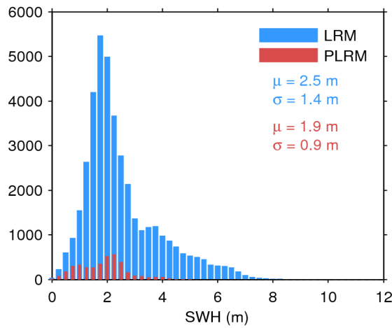
Figure 20. Histogram of science-valid SWH over oceans and lakes for LRM (blue) and PLRM (red) for 07/09/2016. The mean ( \mu ) and standard deviation ( \sigma ) are also shown. Note that values larger than 12 m are excluded from the histogram for the sake of readability but not from the computation of \mu and \sigma .
