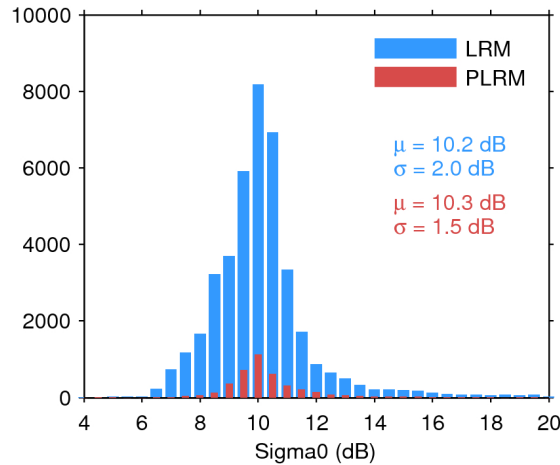
Figure 25. Histogram of flag-valid sigma0 over oceans and lakes for LRM (blue) and PLRM (red) for 07/09/2016. The mean ( \mu ) and standard deviation ( \sigma ) are also shown. Note that values outside [4 20] dB are excluded from the histogram for the sake of readability but not from the computation of \mu and \sigma .
