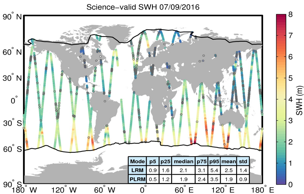
Figure 19. Geographical distribution of science-valid SWH data over oceans and lakes for 07/09/2016. The statistical values shown in the table refer to the SWH in m and are calculated separately for LRM and PLRM regions. The black lines mark the outer limit of the Arctic and Antarctic polar polygons. Gray circles denote records that have been rejected based on the editing criteria described in Table 3.
