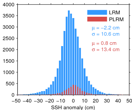
Figure 11. Histogram of science-valid SSH anomaly over oceans and lakes for LRM (blue) and PLRM (red) for 07/09/2016. The mean ( \mu ) and standard deviation ( \sigma ) are also shown. Note that values outside [-50 50] cm are excluded from the histogram for the sake of readability but not from the computation of \mu and \sigma .
