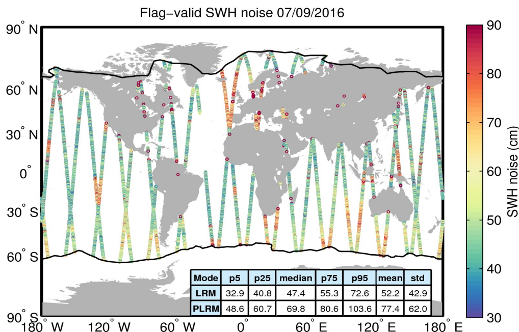
Figure 18. Geographical distribution of flag-valid 20-Hz SWH measurement noise over oceans and lakes for 07/09/2016. The statistical values shown in the table refer to the SWH noise and are calculated separately for LRM and PLRM regions. Measurements taken over polar polygons have been excluded from the computation of the statistical values. The black lines mark the outer limit of the Arctic and Antarctic polar polygons.
