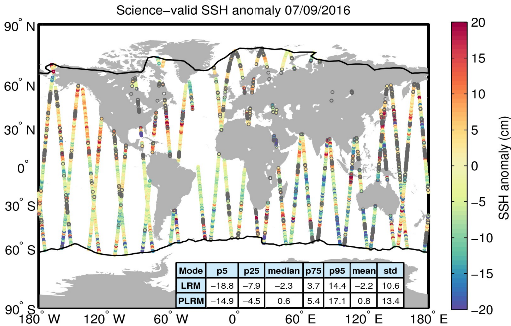
Figure 10. Geographical distribution of science-valid SSH anomaly data over oceans and lakes for 07/09/2016. The statistical values shown in the table refer to the SSH anomaly in cm and are calculated separately for LRM and PLRM regions. The black lines mark the outer limit of the Arctic and Antarctic polar polygons. Gray circles denote records that have been rejected based on the editing criteria described in Table 2.
