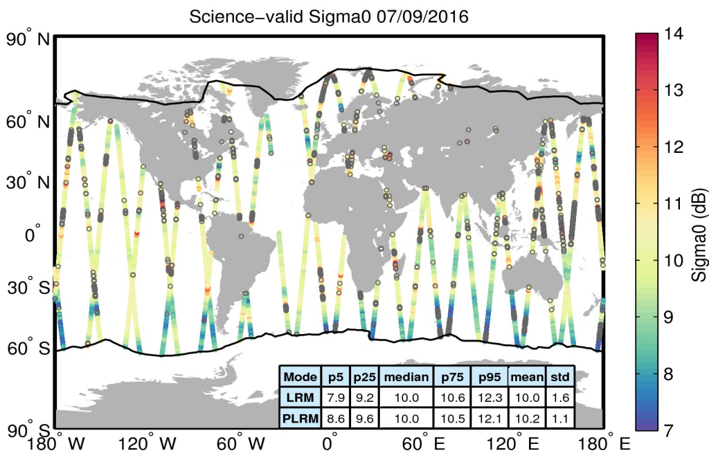
Figure 27. Geographical distribution of science-valid sigma0 data over oceans and lakes for 07/09/2016. The statistical values shown in the table refer to the sigma0 in dB and are calculated separately for LRM and PLRM regions. The black lines mark the outer limit of the Arctic and Antarctic polar polygons. Gray circles denote records that have been rejected based on the editing criteria described in Table 4.
