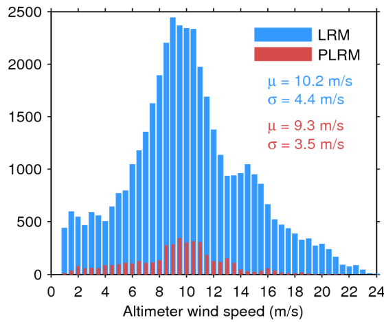
Figure 33. Histogram of flag-valid wind over oceans and lakes for LRM (blue) and PLRM (red) for 07/09/2016. The mean ( \mu ) and standard deviation ( \sigma ) are also shown. Note that values larger than 24 m/s are excluded from the histogram for the sake of readability but not from the computation of \mu and \sigma .
