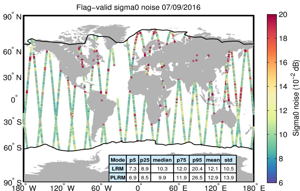
Figure 26. Geographical distribution of flag-valid 20-Hz sigma0 measurement noise over oceans and lakes for 07/09/2016. The statistical values shown in the table refer to the sigma0 noise and are calculated separately for LRM and PLRM regions. Measurements taken over polar polygons have been excluded from the computation of the statistical values. The black lines mark the outer limit of the Arctic and Antarctic polar polygons.
