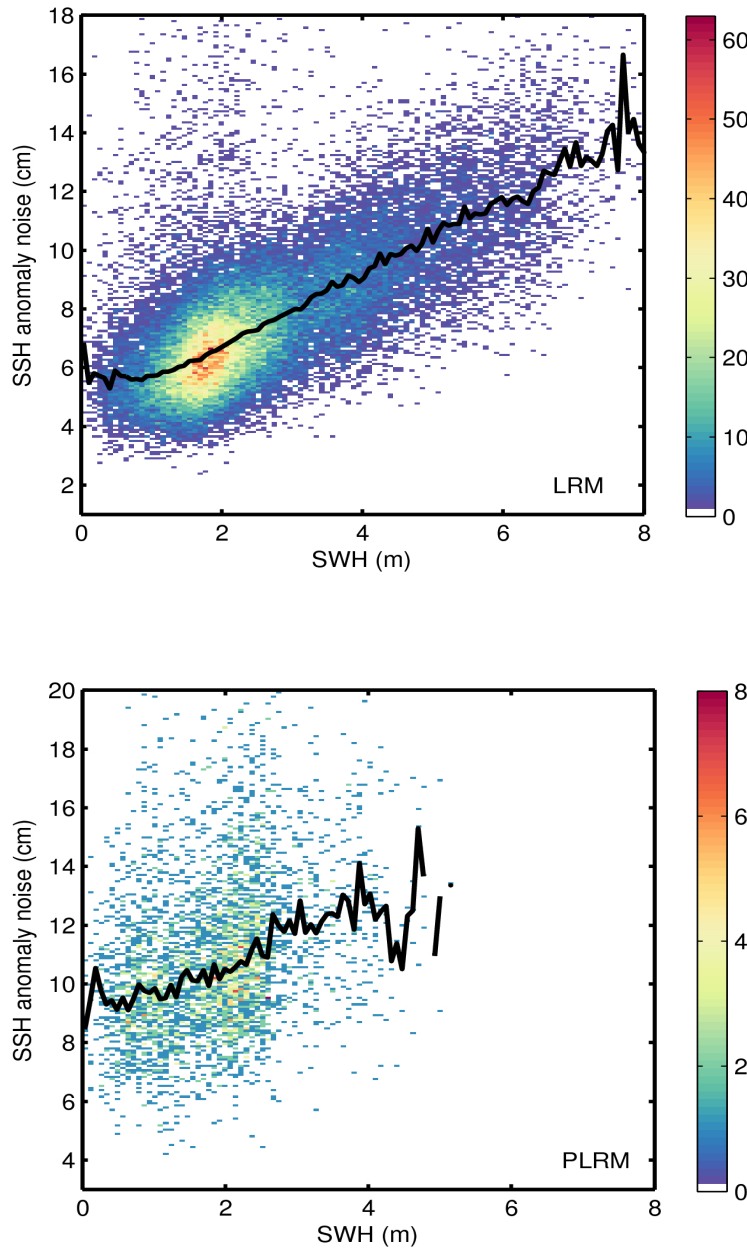
Figure 9. 2D histogram showing flag-valid SSH anomaly noise as a function of SWH for LRM (top) and PLRM (bottom) for 07/09/2016. The black line denotes the median SSH anomaly noise as a function of SWH.
