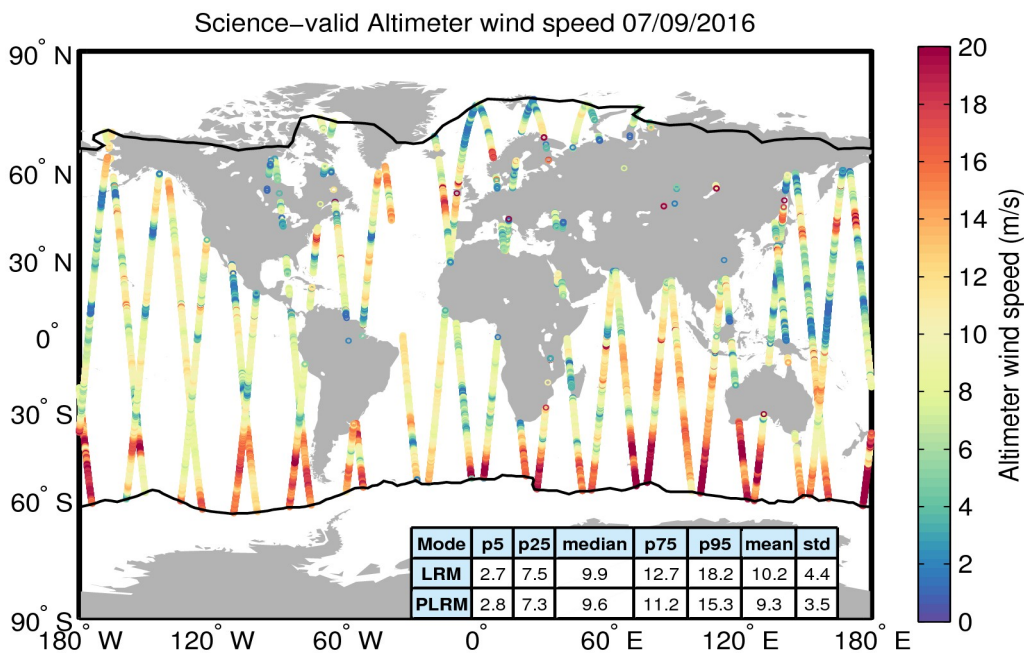
Figure 34. Geographical distribution of science-valid wind data over oceans and lakes for 07/09/2016. The statistical values shown in the table refer to the wind in m/s and are calculated separately for LRM and PLRM regions. The black lines mark the outer limit of the Arctic and Antarctic polar polygons. Gray circles denote records that have been rejected based on the editing criteria described in Table 5.
