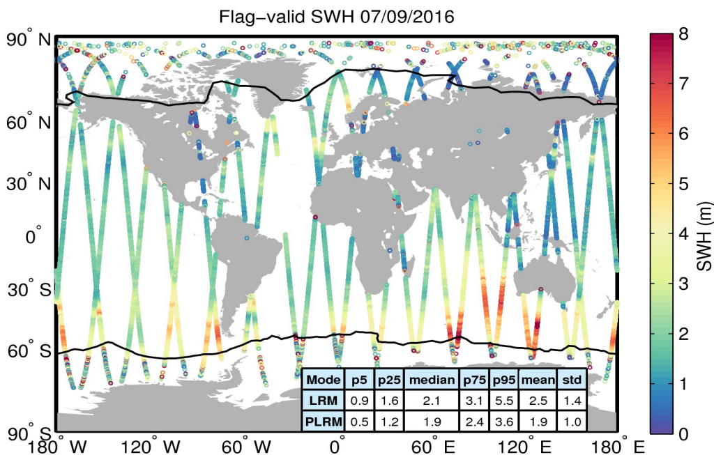
Figure 15. Geographical distribution of flag-valid SWH data over oceans and lakes for 07/09/2016. The statistical values shown in the table refer to the SWH in m and are calculated separately for LRM and PLRM regions. Measurements taken over polar polygons have been excluded from the computation of the statistical values. The black lines mark the outer limit of the Arctic and Antarctic polar polygons.
