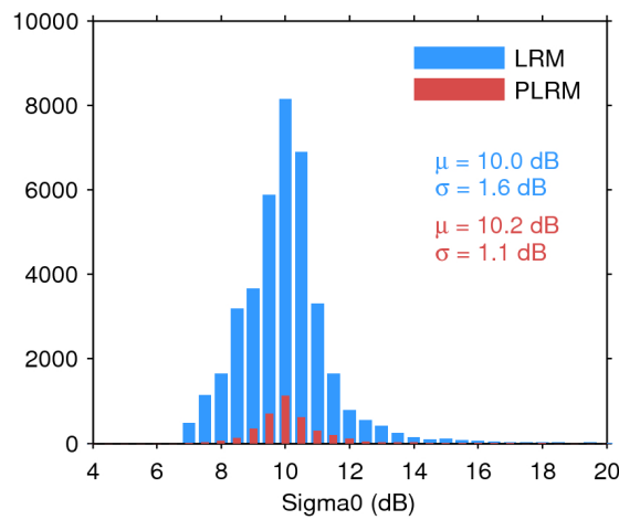
Figure 28. Histogram of science-valid sigma0 over oceans and lakes for LRM (blue) and PLRM (red) for 07/09/2016. The mean ( \mu ) and standard deviation ( \sigma ) are also shown. Note that values outside [4 20] dB are excluded from the histogram for the sake of readability but not from the computation of \mu and \sigma .
