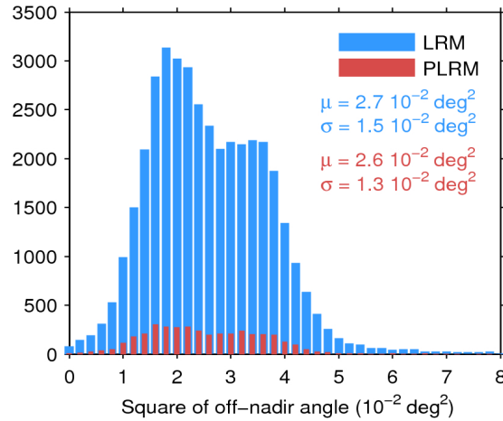
Figure 39. Histogram of flag-valid mispointing over oceans and lakes for LRM (blue) and PLRM (red) for 07/09/2016. Only positive values have been considered. The mean ( \mu ) and standard deviation ( \sigma ) are also shown. Note that values larger than 8 \cdot 10^{-2} \text{ deg}^2 are excluded from the histogram for the sake of readability but not from the computation of \mu and \sigma .
