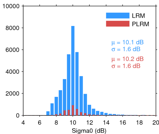
Figure 28. Histogram of science-valid sigma0 over oceans and lakes for LRM (blue) and PLRM (red) for 06/09/2016. The mean ( \mu ) and standard deviation ( \sigma ) are also shown. Note that values outside [4 20] dB are excluded from the histogram for the sake of readability but not from the computation of \mu and \sigma .
