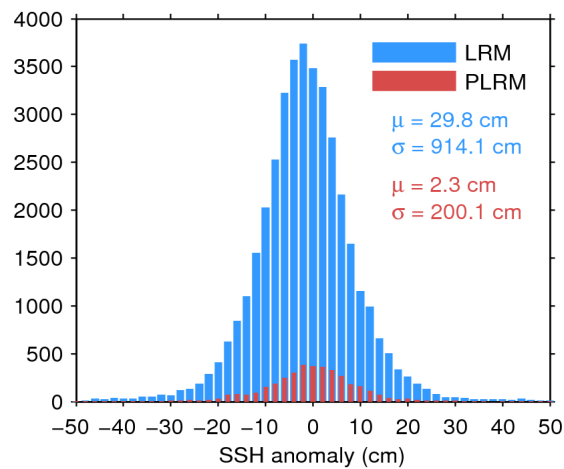
Figure 7. Histogram of flag-valid SSH anomaly over oceans and lakes for LRM (blue) and PLRM (red) for 06/09/2016. The mean ( \mu ) and standard deviation ( \sigma ) are also shown. Note that values outside [-50 50] cm are excluded from the histogram for the sake of readability but not from the computation of \mu and \sigma .
