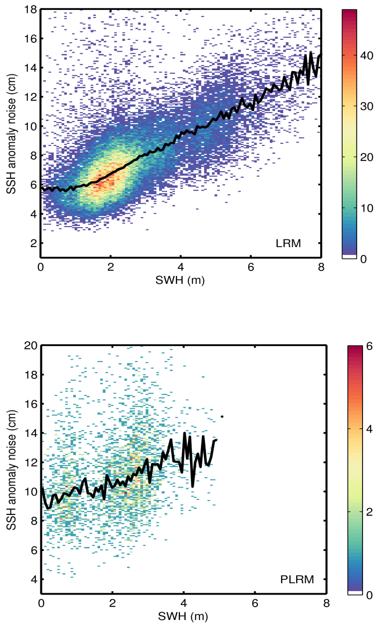
Figure 9. 2D histogram showing flag-valid SSH anomaly noise as a function of SWH for LRM (top) and PLRM (bottom) for 06/09/2016. The black line denotes the median SSH anomaly noise as a function of SWH.
