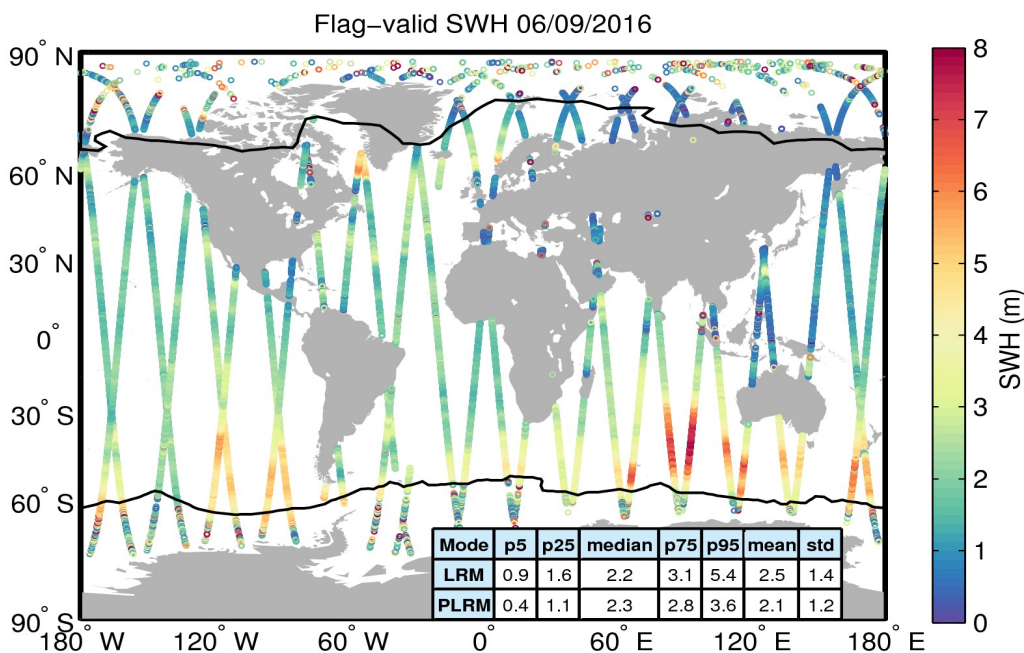
Figure 15. Geographical distribution of flag-valid SWH data over oceans and lakes for 06/09/2016. The statistical values shown in the table refer to the SWH in m and are calculated separately for LRM and PLRM regions. Measurements taken over polar polygons have been excluded from the computation of the statistical values. The black lines mark the outer limit of the Arctic and Antarctic polar polygons.
