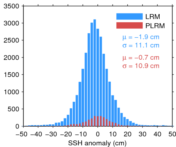
Figure 11. Histogram of science-valid SSH anomaly over oceans and lakes for LRM (blue) and PLRM (red) for 06/09/2016. The mean ( \mu ) and standard deviation ( \sigma ) are also shown. Note that values outside [-50 50] cm are excluded from the histogram for the sake of readability but not from the computation of \mu and \sigma .
