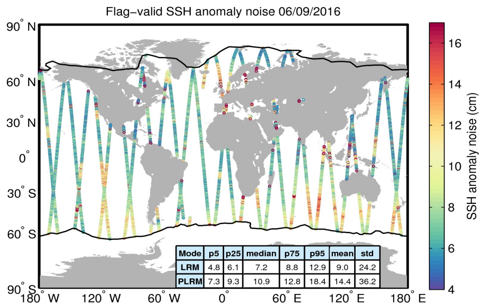
Figure 8. Geographical distribution of flag-valid 20-Hz SSH anomaly measurement noise over oceans and lakes for 06/09/2016. The statistical values shown in the table refer to the SSH anomaly noise and are calculated separately for LRM and PLRM regions. Measurements taken over polar polygons have been excluded from the computation of the statistical values. The black lines mark the outer limit of the Arctic and Antarctic polar polygons.
