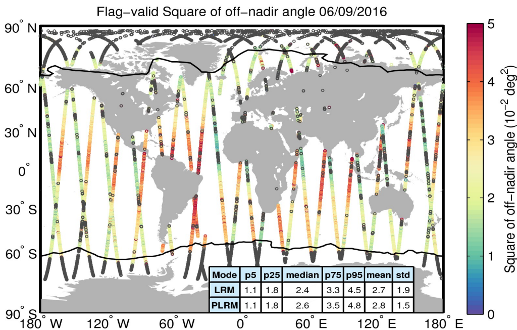
Figure 37. Geographical distribution of flag-valid mispointing data over oceans and lakes for 06/09/2016. The statistical values shown in the table refer to the mispointing in 10^{-2} deg 2 and are calculated separately for LRM and PLRM regions. Measurements taken over polar polygons have been excluded from the computation of the statistical values. The black lines mark the outer limit of the Arctic and Antarctic polar polygons. Gray circles denote negative values.
