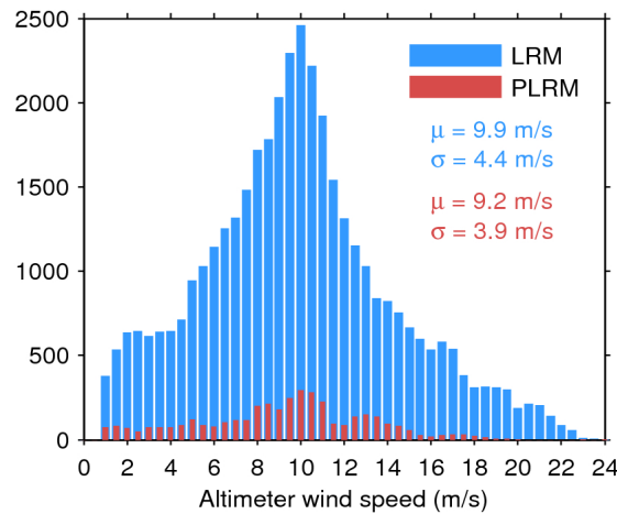
Figure 33. Histogram of flag-valid wind over oceans and lakes for LRM (blue) and PLRM (red) for 06/09/2016. The mean ( \mu ) and standard deviation ( \sigma ) are also shown. Note that values larger than 24 m/s are excluded from the histogram for the sake of readability but not from the computation of \mu and \sigma .
