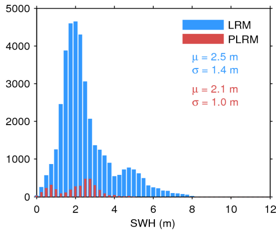
Figure 20. Histogram of science-valid SWH over oceans and lakes for LRM (blue) and PLRM (red) for 06/09/2016. The mean ( \mu ) and standard deviation ( \sigma ) are also shown. Note that values larger than 12 m are excluded from the histogram for the sake of readability but not from the computation of \mu and \sigma .
