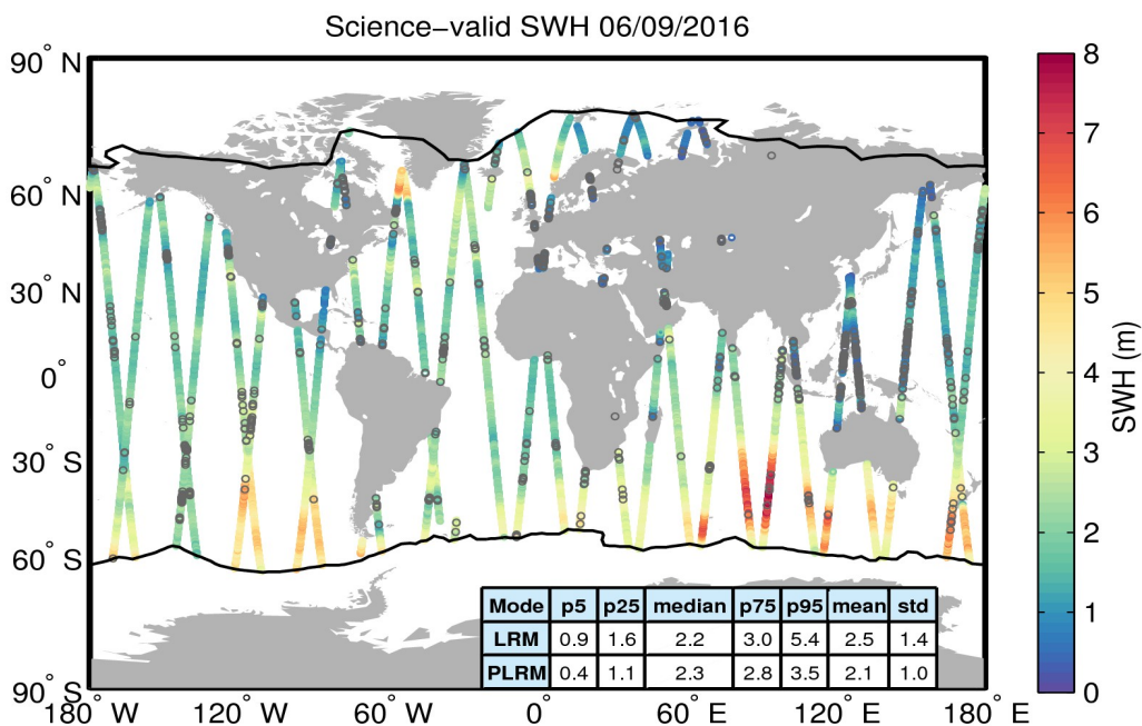
Figure 19. Geographical distribution of science-valid SWH data over oceans and lakes for 06/09/2016. The statistical values shown in the table refer to the SWH in m and are calculated separately for LRM and PLRM regions. The black lines mark the outer limit of the Arctic and Antarctic polar polygons. Gray circles denote records that have been rejected based on the editing criteria described in Table 3.
