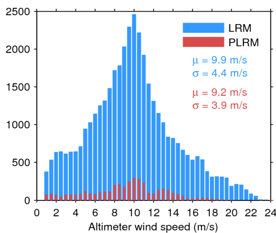
Figure 35. Histogram of science-valid wind over oceans and lakes for LRM (blue) and PLRM (red) for 06/09/2016. The mean ( \mu ) and standard deviation ( \sigma ) are also shown. Note that values larger than 24 m/s are excluded from the histogram for the sake of readability but not from the computation of \mu and \sigma .
