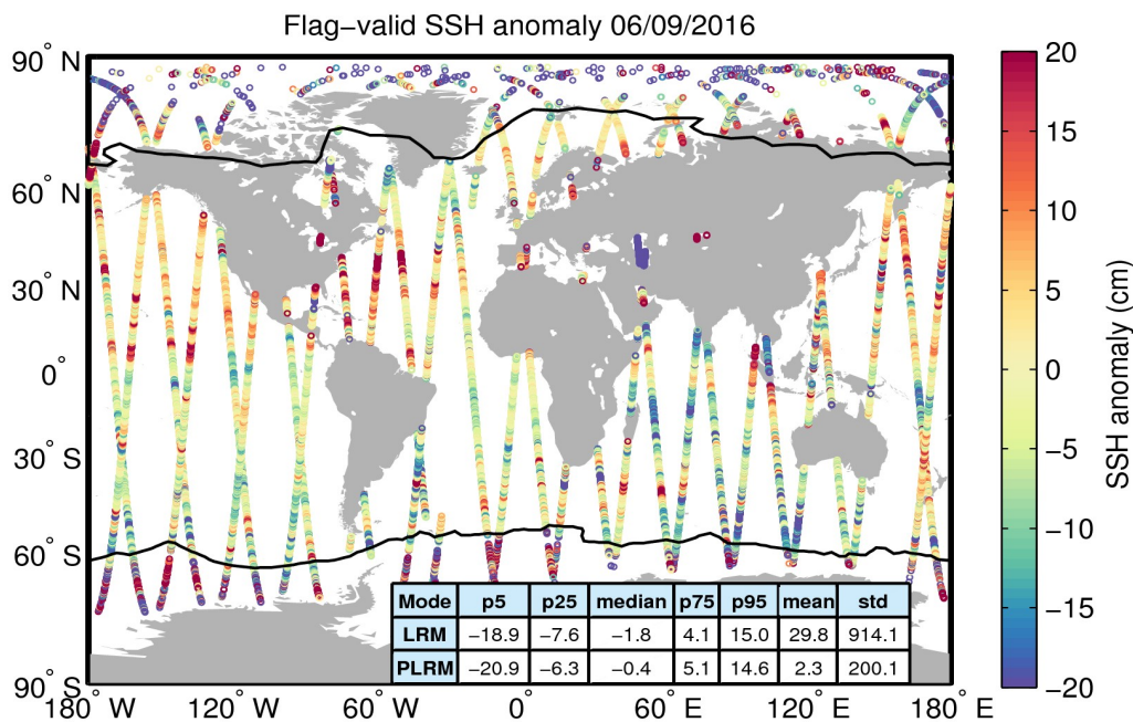
Figure 5. Geographical distribution of flag-valid 1-Hz SSH anomaly data over oceans and lakes for 06/09/2016. The statistical values shown in the table refer to the SSH anomaly in cm and are calculated separately for LRM and PLRM regions. Measurements taken over polar polygons have been excluded from the computation of the statistical values. The black lines mark the outer limit of the Arctic and Antarctic polar polygons.
