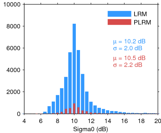
Figure 25. Histogram of flag-valid sigma0 over oceans and lakes for LRM (blue) and PLRM (red) for 06/09/2016. The mean ( \mu ) and standard deviation ( \sigma ) are also shown. Note that values outside [4 20] dB are excluded from the histogram for the sake of readability but not from the computation of \mu and \sigma .
