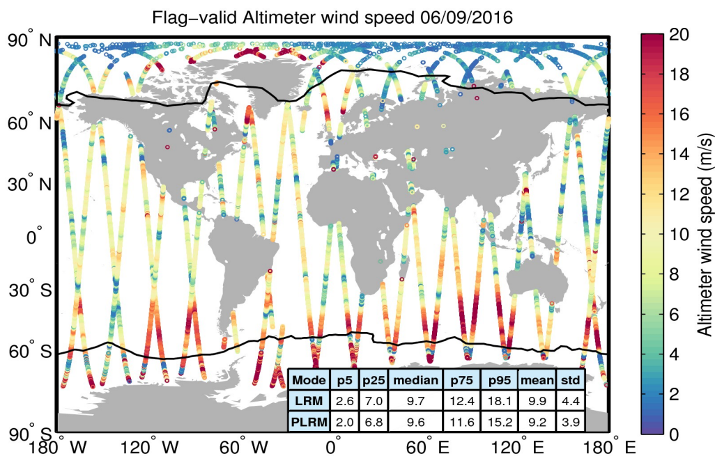
Figure 31. Geographical distribution of flag-valid wind data over oceans and lakes for 06/09/2016. The statistical values shown in the table refer to the wind in m/s and are calculated separately for LRM and PLRM regions. Measurements taken over polar polygons have been excluded from the computation of the statistical values. The black lines mark the outer limit of the Arctic and Antarctic polar polygons.
