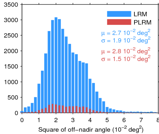
Figure 39. Histogram of flag-valid mispointing over oceans and lakes for LRM (blue) and PLRM (red) for 06/09/2016. Only positive values have been considered. The mean ( \mu ) and standard deviation ( \sigma ) are also shown. Note that values larger than 8 \cdot 10^{-2} \text{ deg}^2 are excluded from the histogram for the sake of readability but not from the computation of \mu and \sigma .
