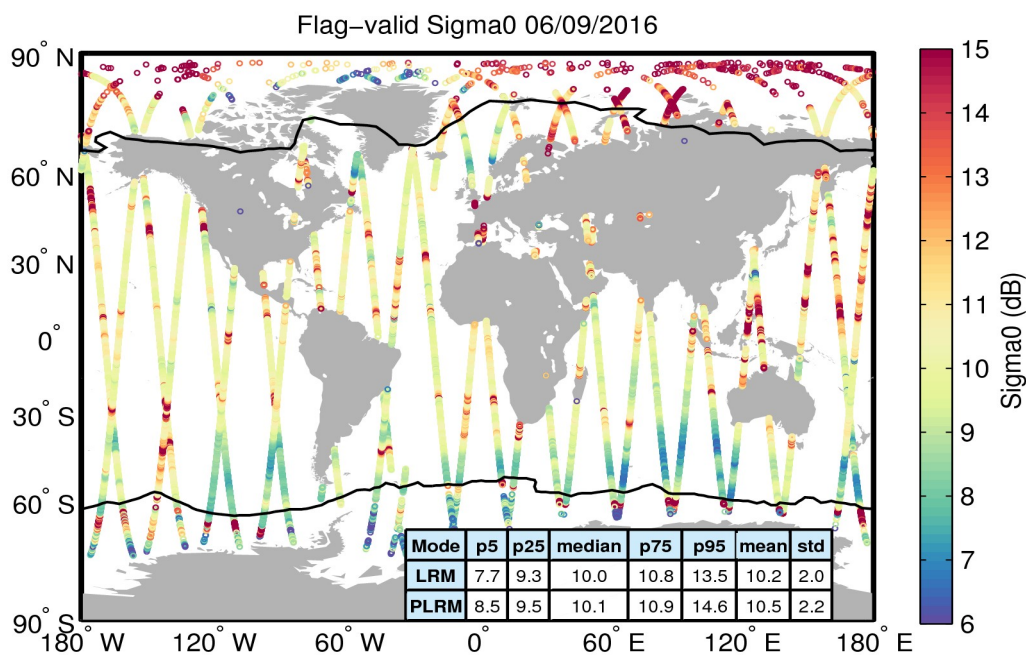
Figure 23. Geographical distribution of flag-valid sigma0 data over oceans and lakes for 06/09/2016. The statistical values shown in the table refer to the sigma0 in dB and are calculated separately for LRM and PLRM regions. Measurements taken over polar polygons have been excluded from the computation of the statistical values. The black lines mark the outer limit of the Arctic and Antarctic polar polygons.
