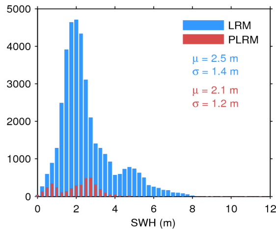
Figure 17. Histogram of flag-valid SWH over oceans and lakes for LRM (blue) and PLRM (red) for 06/09/2016. The mean ( \mu ) and standard deviation ( \sigma ) are also shown. Note that values larger than 12 m are excluded from the histogram for the sake of readability but not from the computation of \mu and \sigma .
