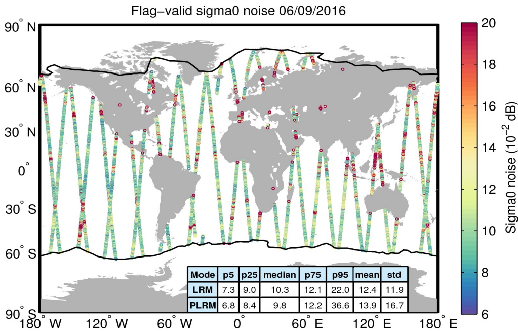
Figure 26. Geographical distribution of flag-valid 20-Hz sigma0 measurement noise over oceans and lakes for 06/09/2016. The statistical values shown in the table refer to the sigma0 noise and are calculated separately for LRM and PLRM regions. Measurements taken over polar polygons have been excluded from the computation of the statistical values. The black lines mark the outer limit of the Arctic and Antarctic polar polygons.
