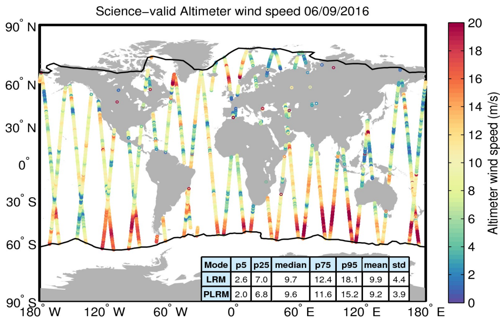
Figure 34. Geographical distribution of science-valid wind data over oceans and lakes for 06/09/2016. The statistical values shown in the table refer to the wind in m/s and are calculated separately for LRM and PLRM regions. The black lines mark the outer limit of the Arctic and Antarctic polar polygons. Gray circles denote records that have been rejected based on the editing criteria described in Table 5.
