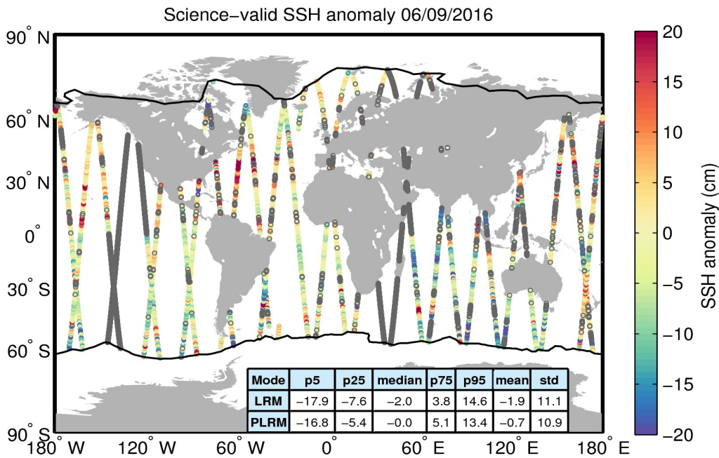
Figure 10. Geographical distribution of science-valid SSH anomaly data over oceans and lakes for 06/09/2016. The statistical values shown in the table refer to the SSH anomaly in cm and are calculated separately for LRM and PLRM regions. The black lines mark the outer limit of the Arctic and Antarctic polar polygons. Gray circles denote records that have been rejected based on the editing criteria described in Table 2.
