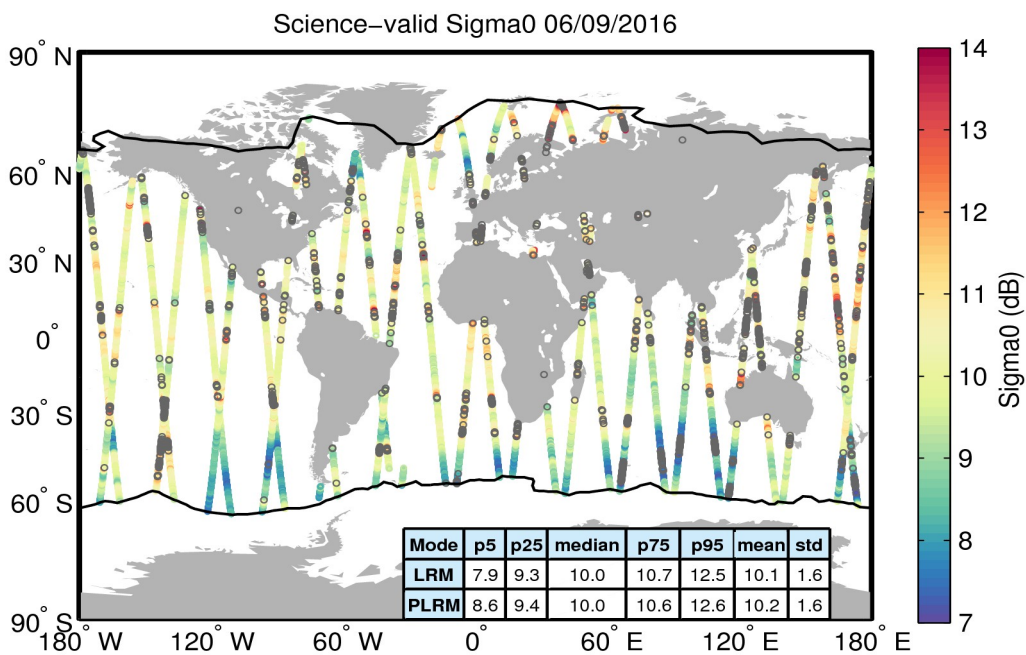
Figure 27. Geographical distribution of science-valid sigma0 data over oceans and lakes for 06/09/2016. The statistical values shown in the table refer to the sigma0 in dB and are calculated separately for LRM and PLRM regions. The black lines mark the outer limit of the Arctic and Antarctic polar polygons. Gray circles denote records that have been rejected based on the editing criteria described in Table 4.
