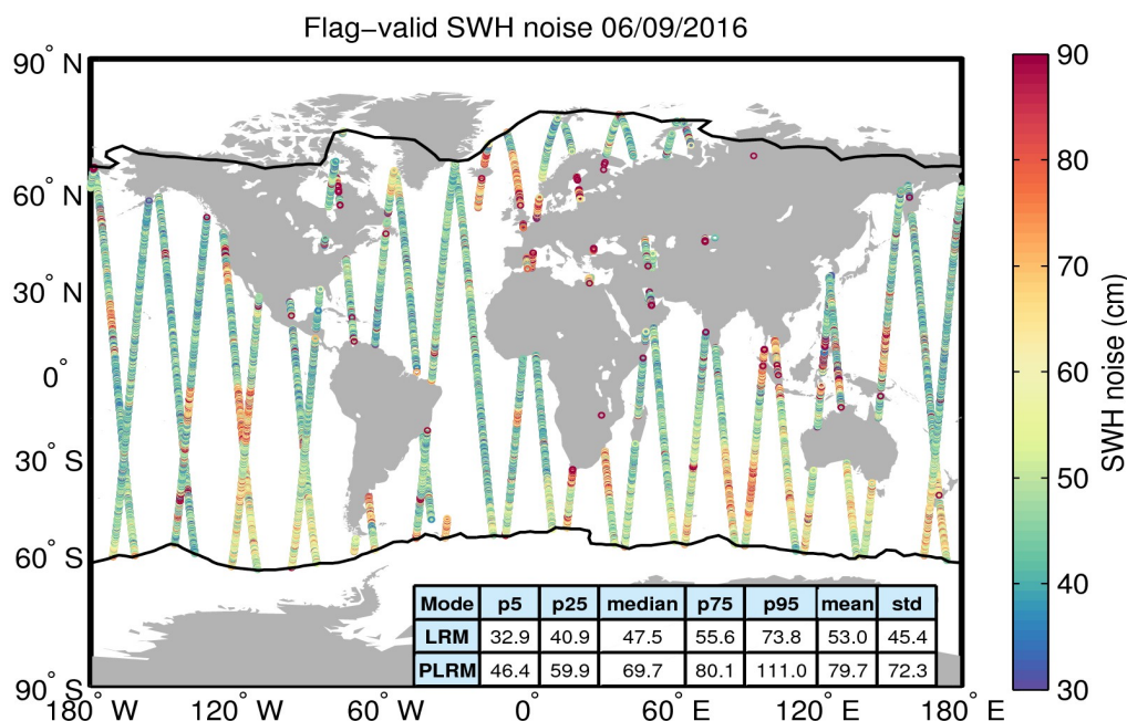
Figure 18. Geographical distribution of flag-valid 20-Hz SWH measurement noise over oceans and lakes for 06/09/2016. The statistical values shown in the table refer to the SWH noise and are calculated separately for LRM and PLRM regions. Measurements taken over polar polygons have been excluded from the computation of the statistical values. The black lines mark the outer limit of the Arctic and Antarctic polar polygons.
